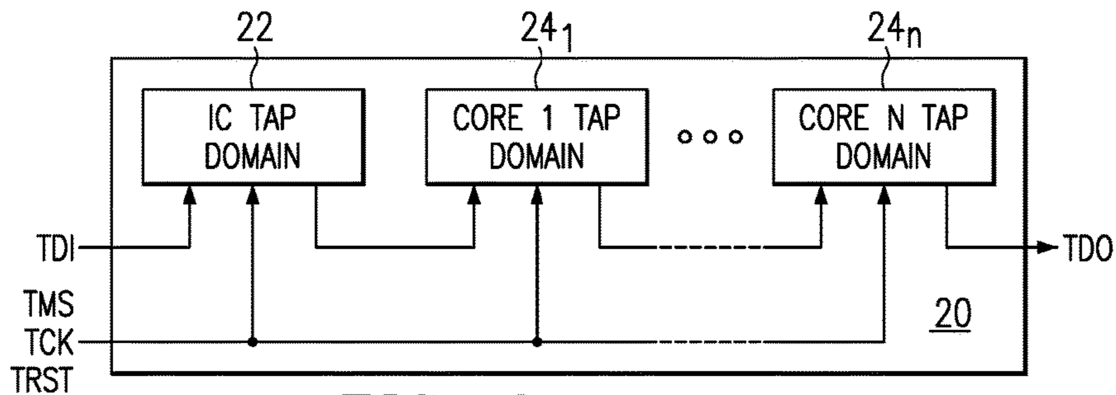
FIG. 3 (PRIOR ART)
