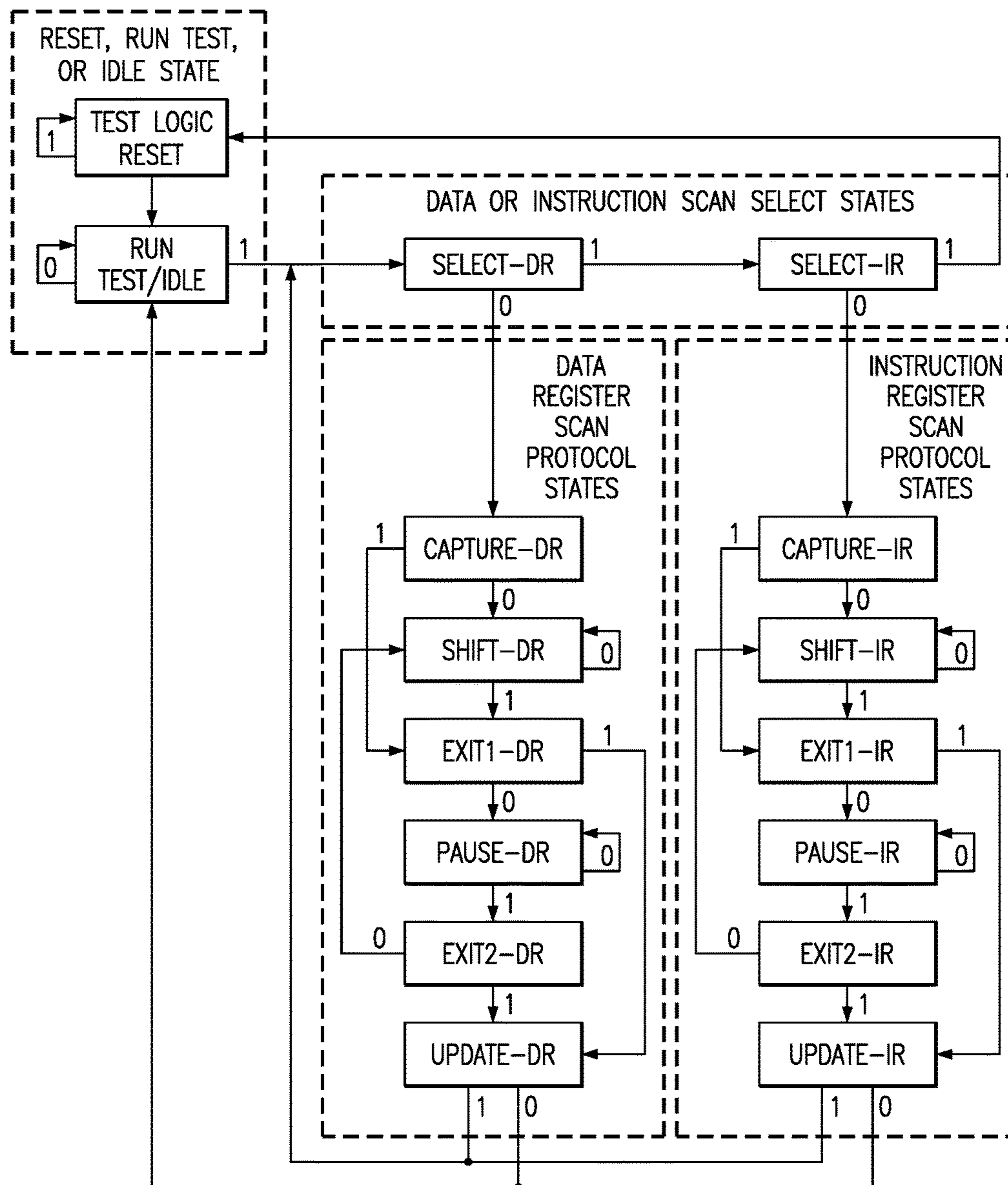
FIG. 2 (PRIOR ART)
