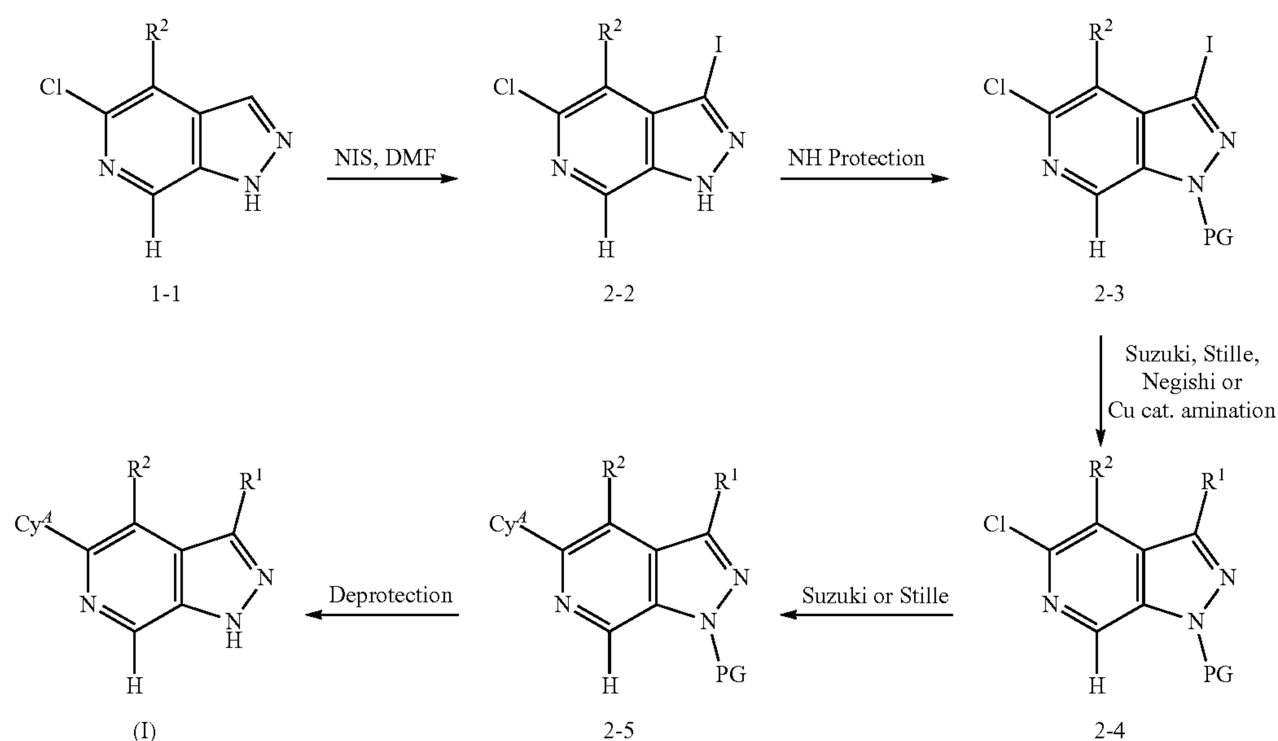
Scheme 2
