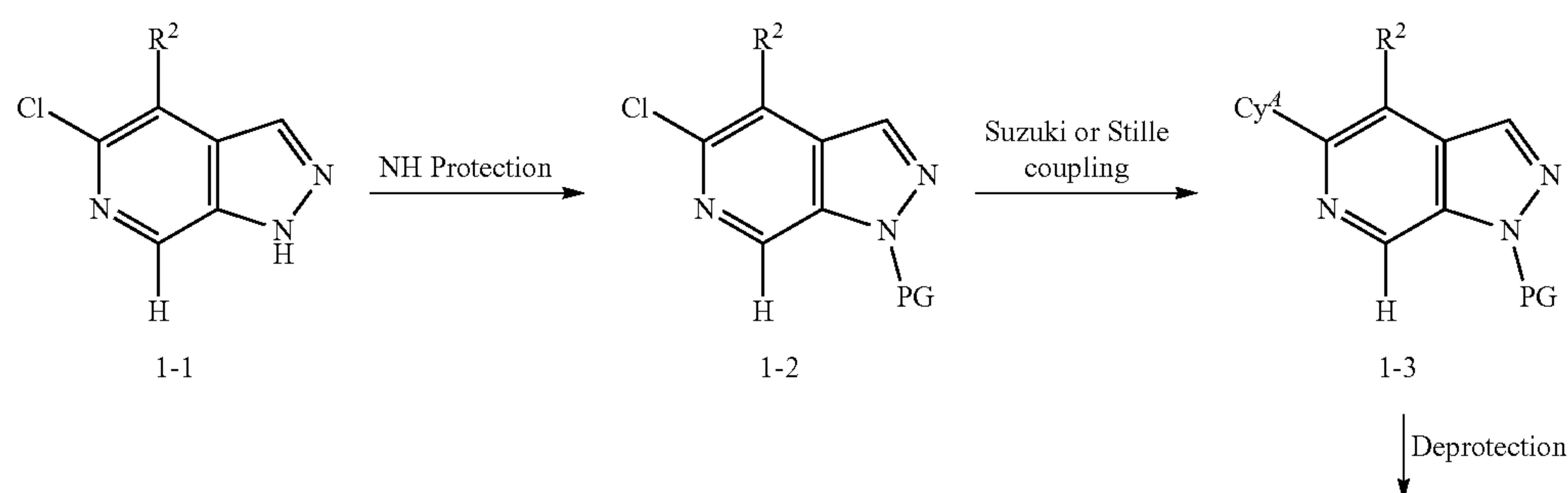
Scheme 1
