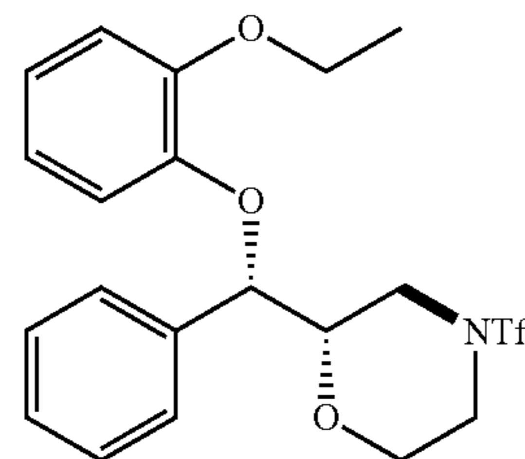
(S)-2-((S)-(2-ethoxyphenoxy)(phenyl)methyl)morpholine (S43)
