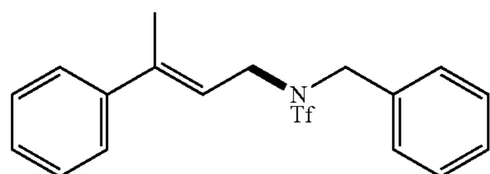
(E)-N-benzyl-1,1,1-trifluoro-N-(3-phenylbut-2-en-1-yl)methanesulfonamide (39)
