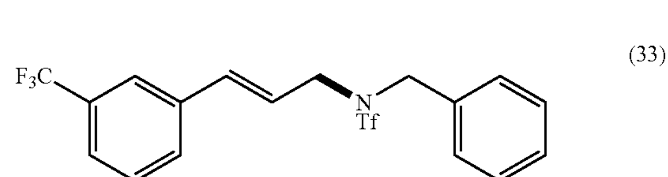
(E)-N-benzyl-N-(3-(3-(trifluoromethyl)phenyl)allyl)-1,1,1-trifluoromethanesulfonamide (33)
