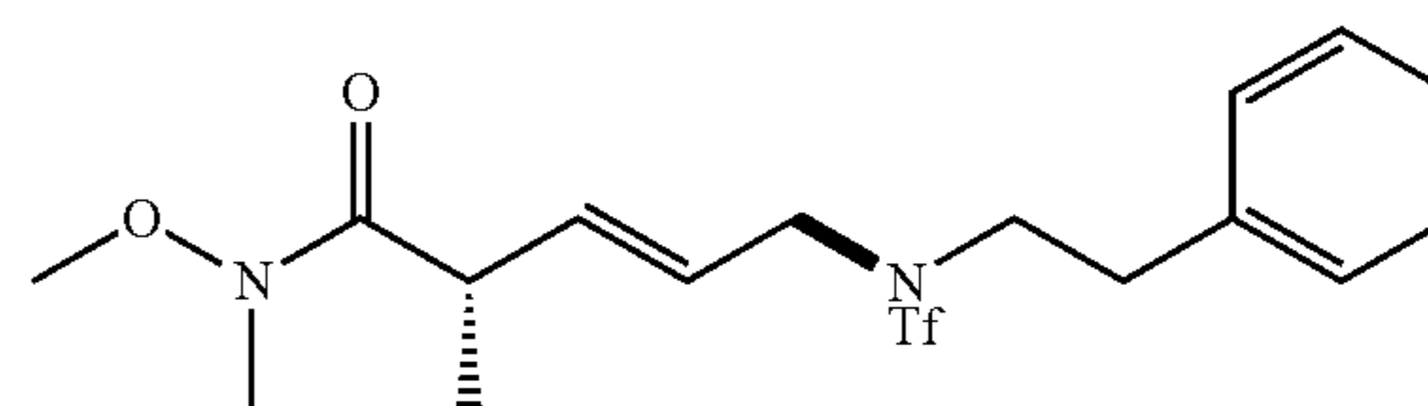
(+)-(S,E)-N-methoxy-N,2-dimethyl-5-((1,1,1-trifluoro-N-phenethylmethyl)sulfonamido)pent-3-enamide (22)
