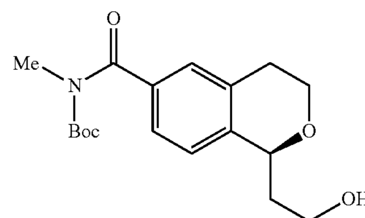
Tert-butyl (1-(2-hydroxyethyl)isochromane-6-carbonyl)(methyl)carbamate (7)
