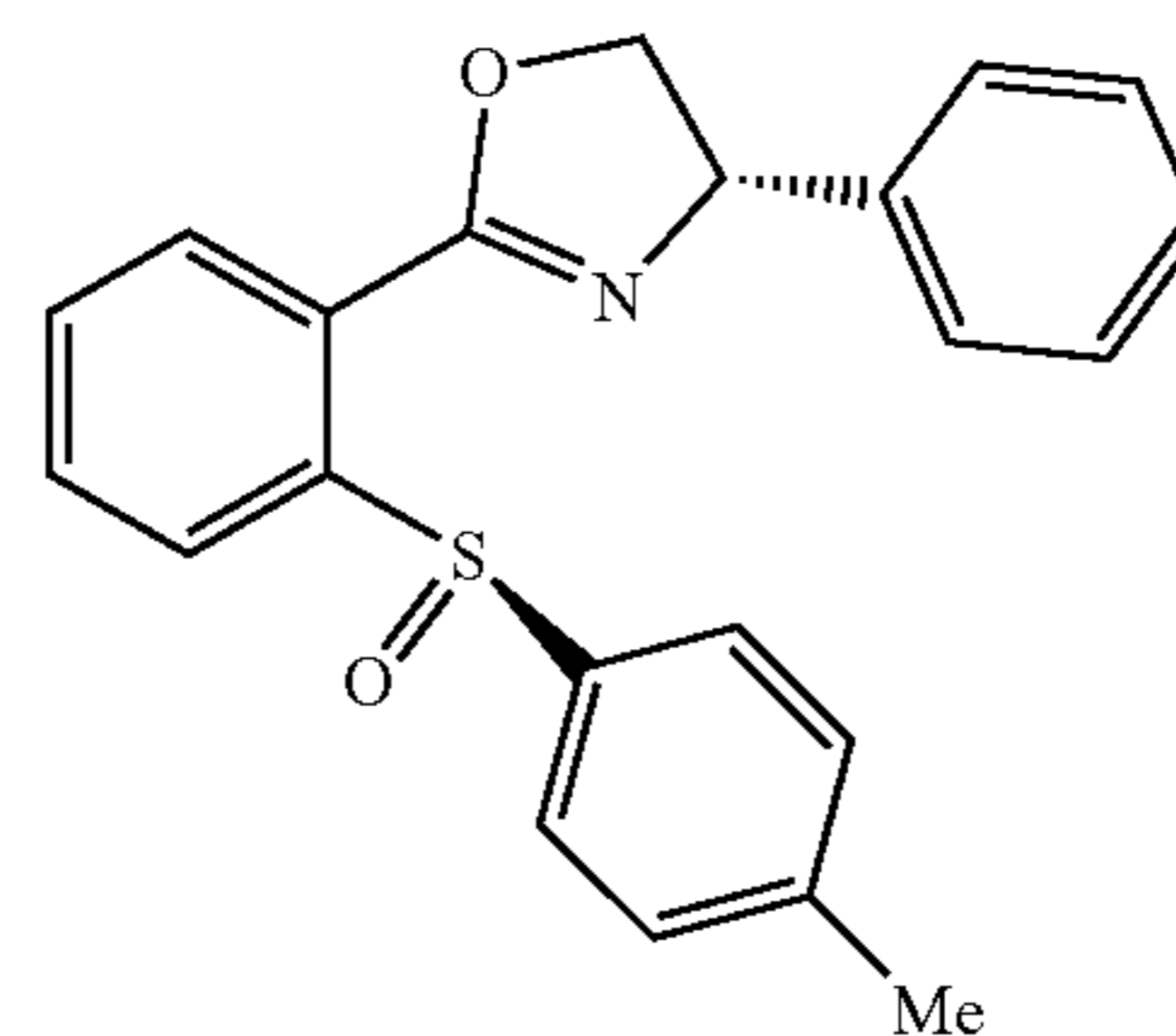
(S)-4-phenyl-2-(2-((R)-p-tolylsulfinyl)phenyl)-4,5-dihydrooxazole (L1)
