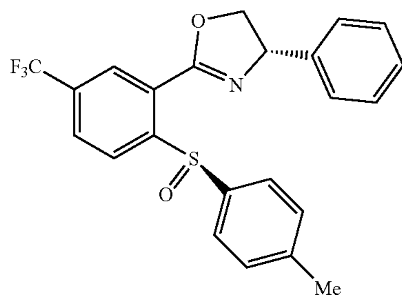
(S)-4-phenyl-2-(2-((R)-p-tolylsulfinyl)-5-(trifluoromethyl)phenyl)-4,5-dihydrooxazole (L14)
