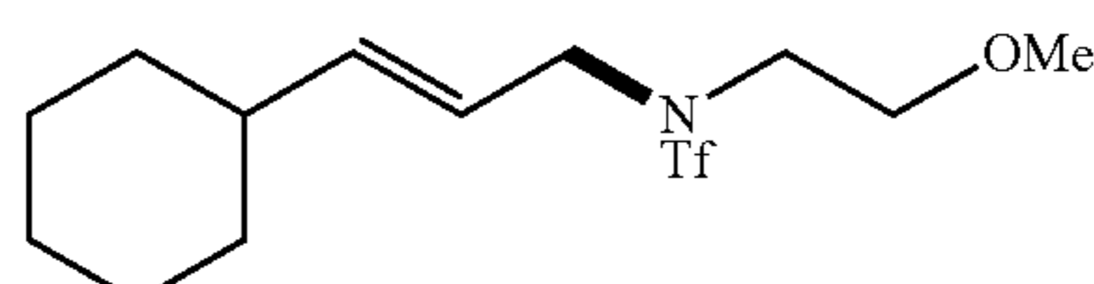
(E)-N-(3-cyclohexylallyl)-1,1,1-trifluoro-N-(2-methoxyethyl)methanesulfonamide (8)
