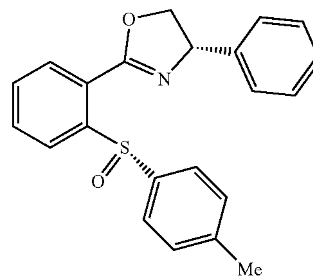
(S)-4-phenyl-2-(2-((S)-p-tolylsulfinyl)phenyl)-4,5-dihydrooxazole (L2)
