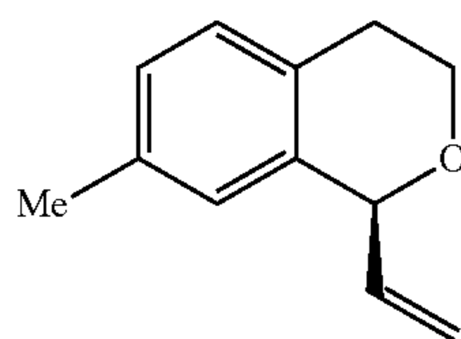
(S)-7-methyl-1-vinylisochromane (2c)
