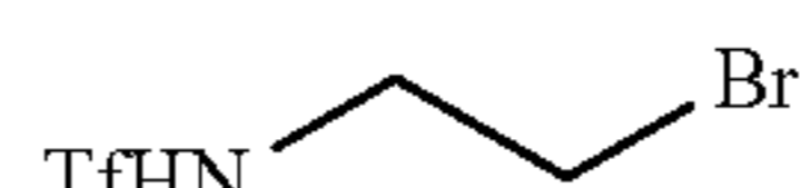
N-(2-bromoethyl)-1,1,1-trifluoromethanesulfonamide (S18)
