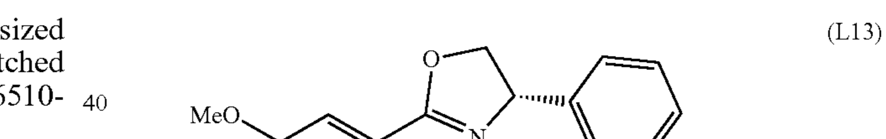
(S)-2-(5-methoxy-2-((R)-p-tolylsulfinyl)phenyl)-4-phenyl-4,5-dihydrooxazole (L13)
