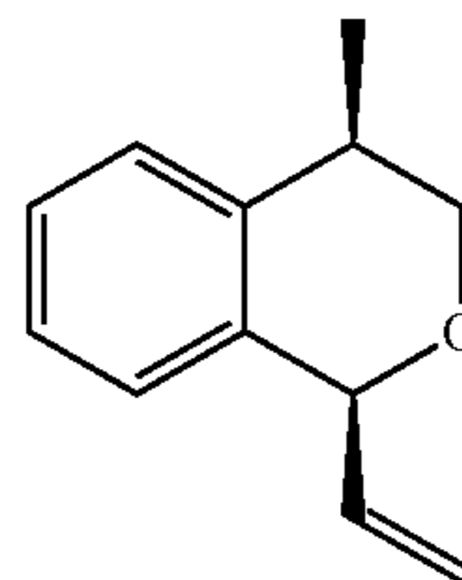
(1S,4R)-4-methyl-1-vinylisochromane (6a)
