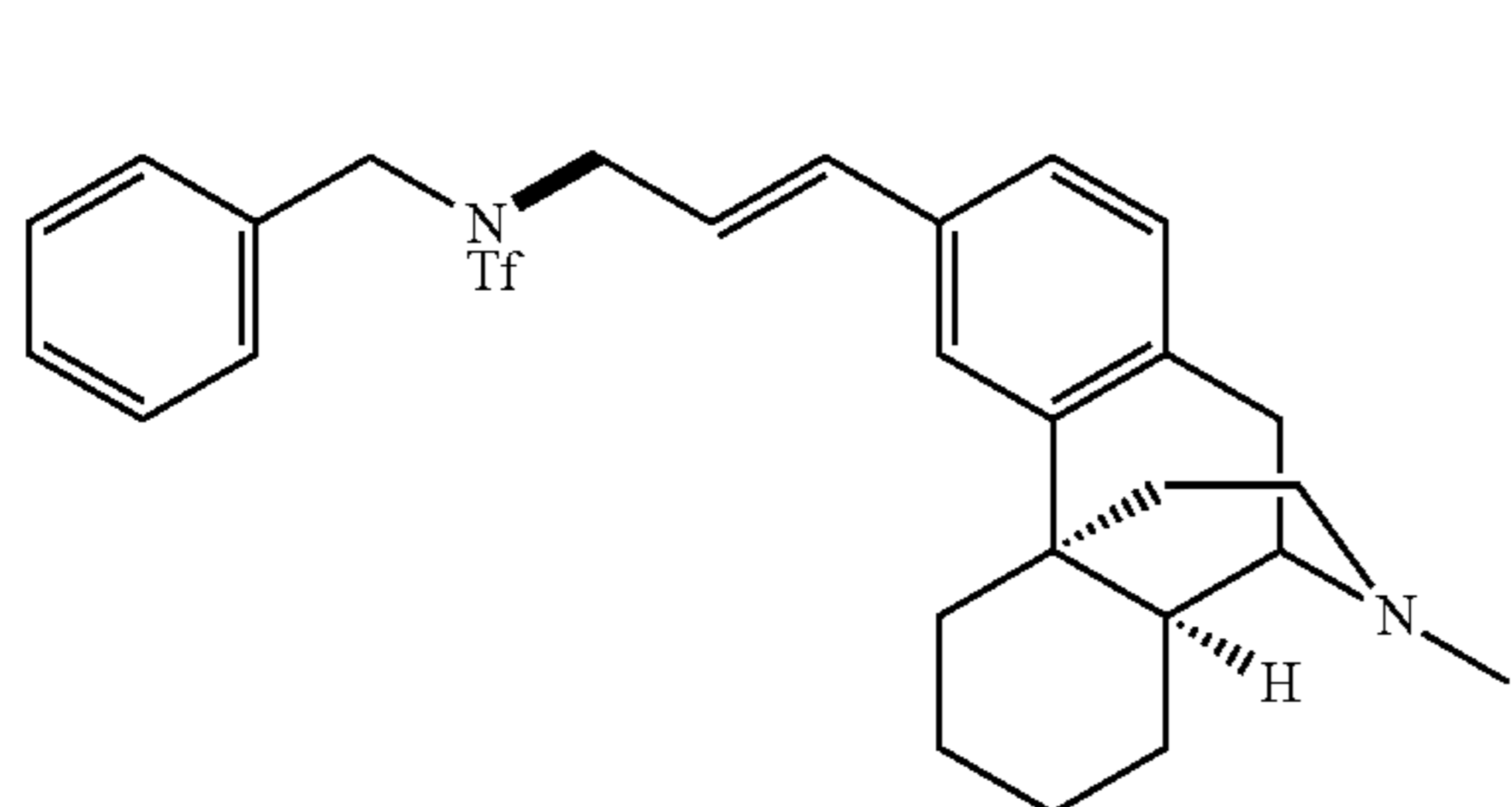
Dexamethorphan Derivative (-)-45
