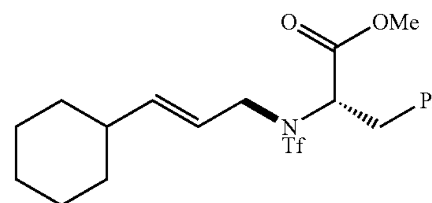
(-)-methyl (E)-N-(3-cyclohexylallyl)-N-((trifluoromethyl)sulfonyl)-L-phenylalaninate (12)
