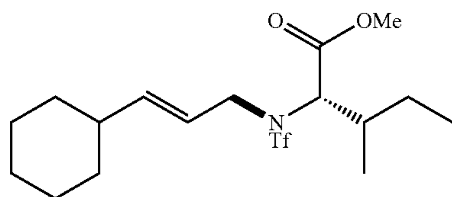
(-)-methyl N-((E)-3-cyclohexylallyl)-N-((trifluoromethyl)sulfonyl)-L-alloisoleucinate (13)
