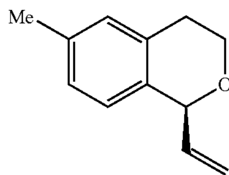
(S)-6-methyl-1-vinylisochromane (2b)
