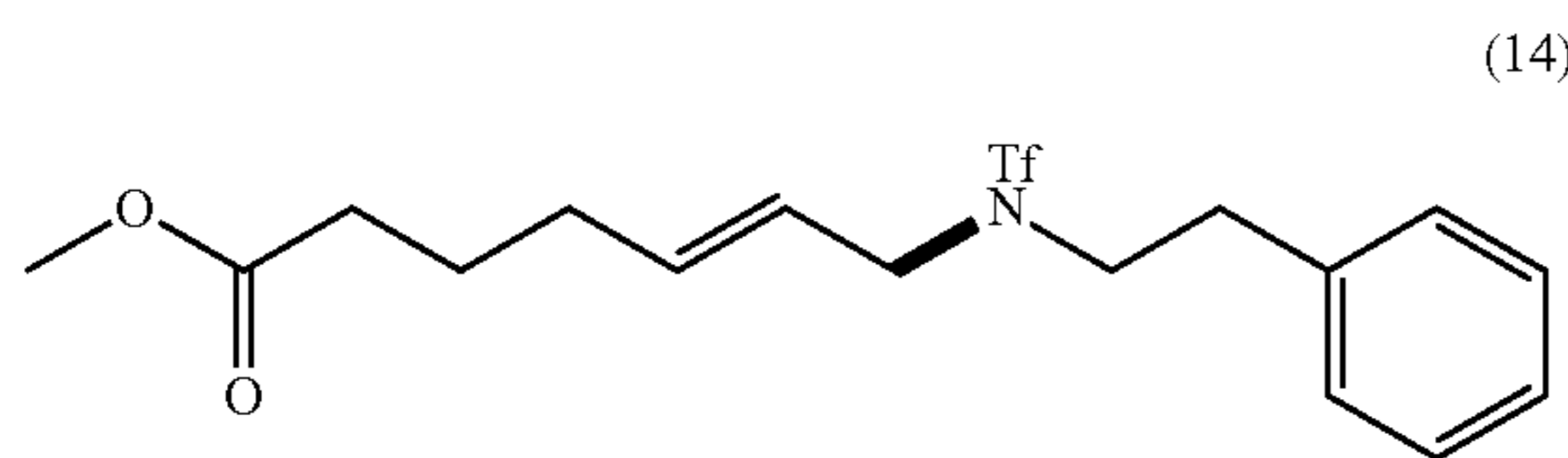
Methyl-(E)-7-((1,1,1-trifluoro-N-phenethylmethyl)sulfonamido)hept-5-enoate (14)
