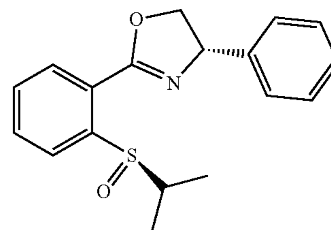
(S)-2-(2-((R)-isopropylsulfinyl)phenyl)-4-phenyl-4,5-dihydrooxazole (L5)
