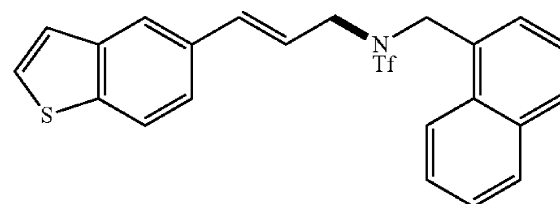
(E)-N-(3-(benzo[b]thiophen-5-yl)allyl)-1,1,1-trifluoro-N-(naphthalen-1-ylmethyl)methanesulfonamide (41)
