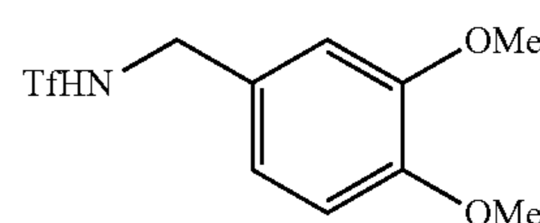
N-(3,4-dimethoxybenzyl)-1,1,1-trifluoromethanesulfonamide (S25)
