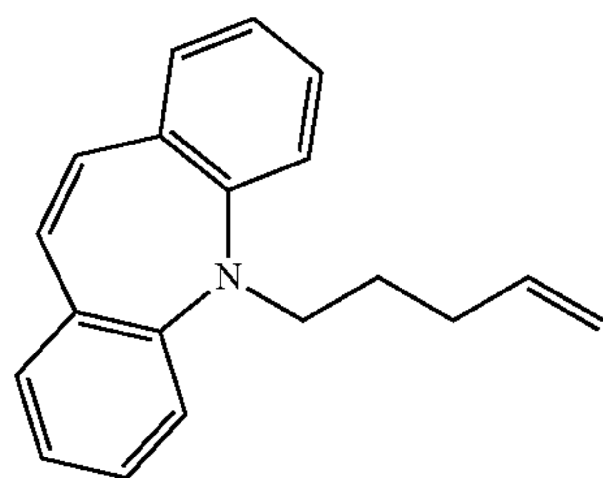
5-(pent-4-en-1-yl)-5H-dibenzo[b]azepine (S36)
