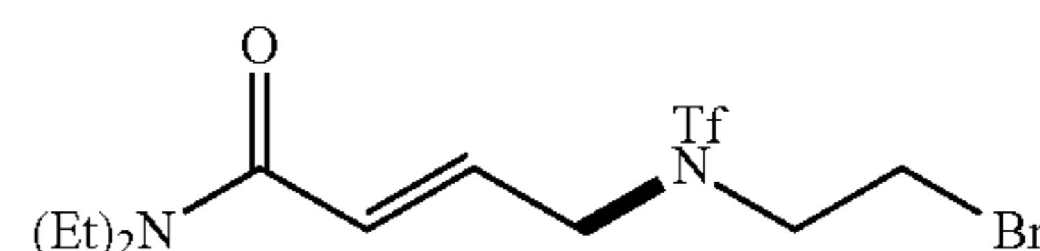
(E)-4-((N-(2-bromoethyl)-1,1,1-trifluoromethyl)sulfonamido)-N,N-diethylbut-2-enamide (15)
