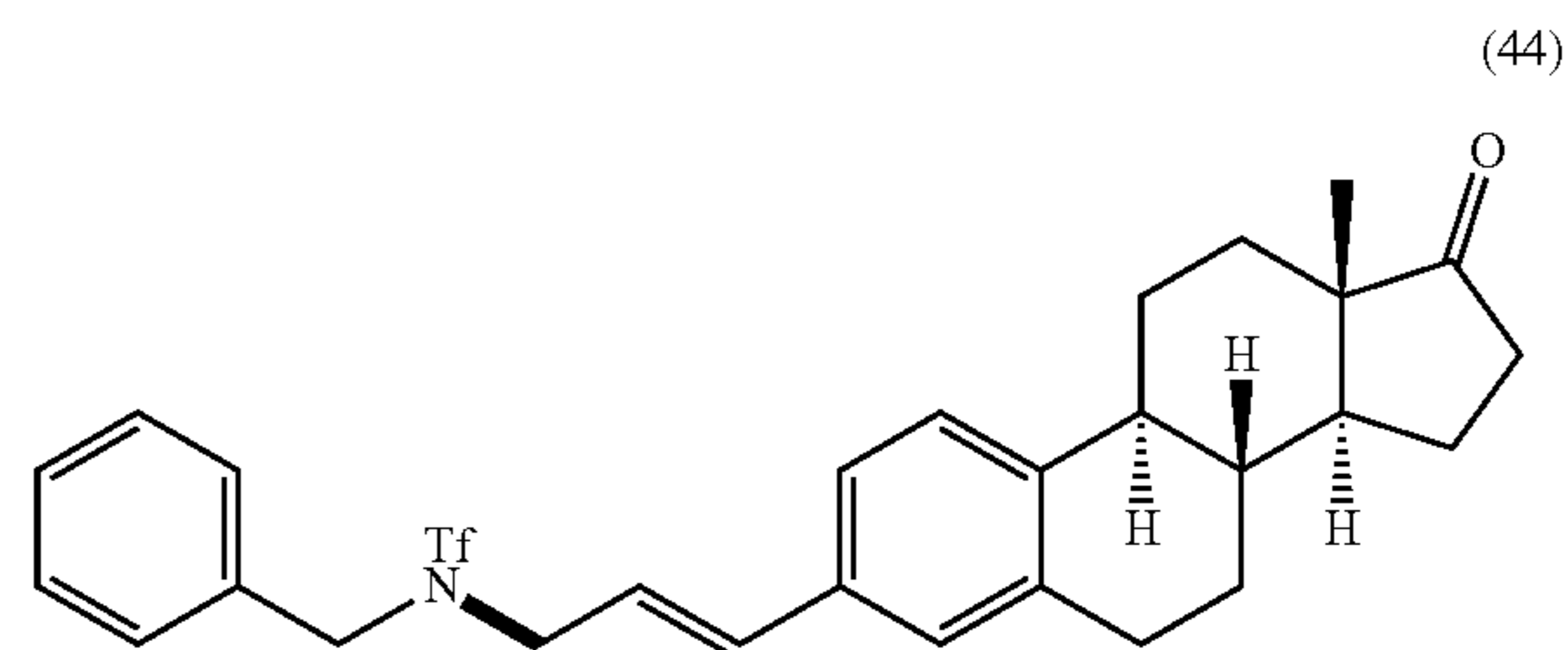
Estrone Derivative (+)-44
