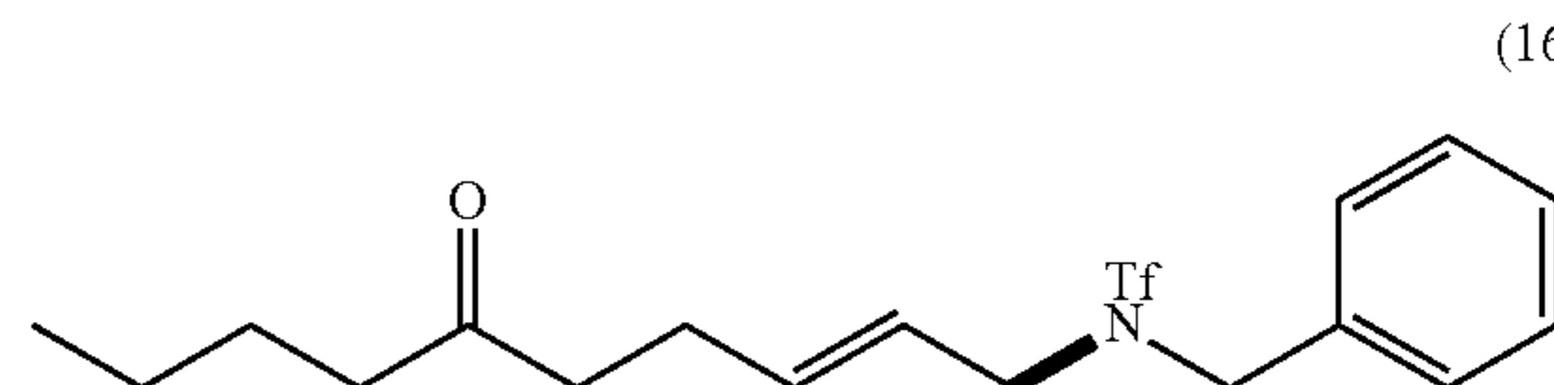
(E)-N-benzyl-1,1,1-trifluoro-N-(6-oxodec-2-en-1-yl)methane sulfonamide (16)
