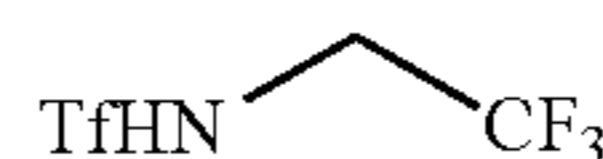
1,1,1-Trifluoro-N-(2,2,2-trifluoroethyl)methanesulfonamide (S19)
