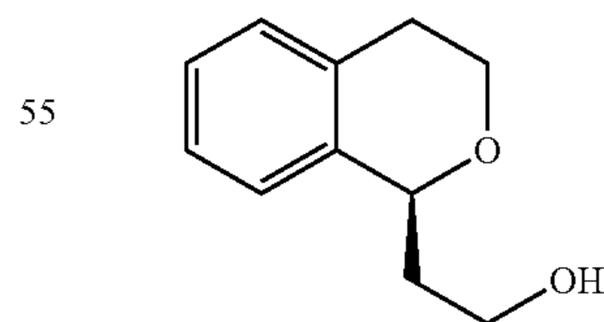
(S)-2-(isochroman-1-yl)ethan-1-ol (11)
