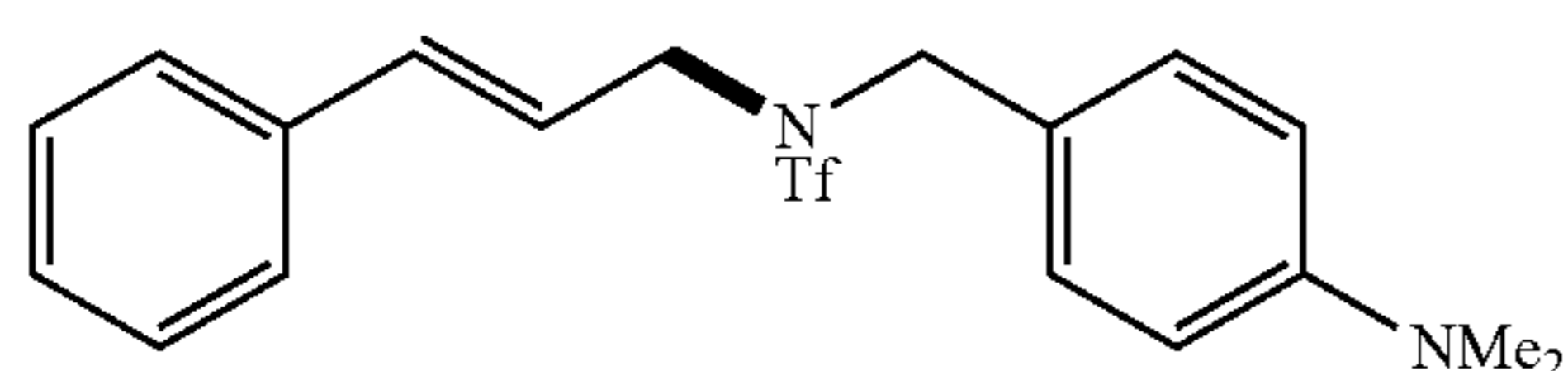
N-cinnamyl-N-(4-(dimethylamino)benzyl)-1,1,1-trifluoromethanesulfonamide (38)
