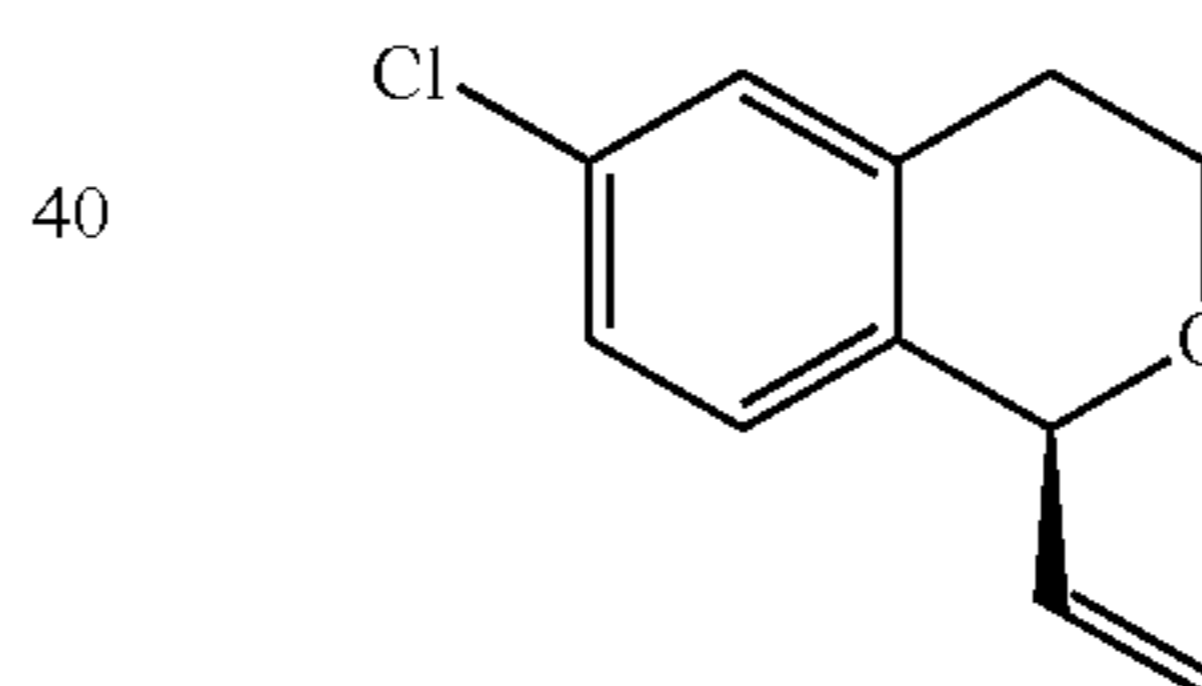
(S)-6-chloro-1-vinylisochromane (2h)
