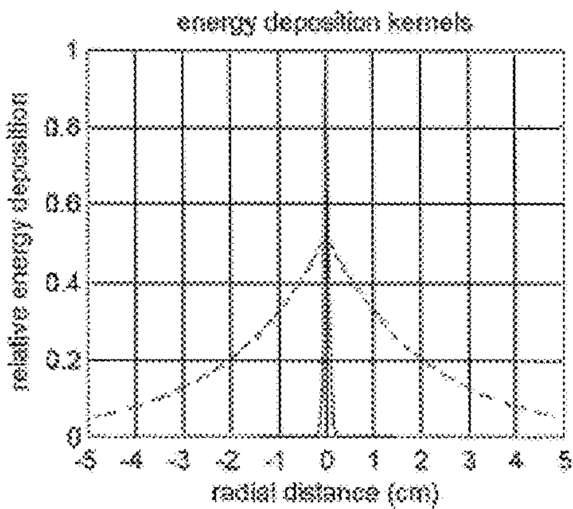
Diagram of energy deposition kernels.
