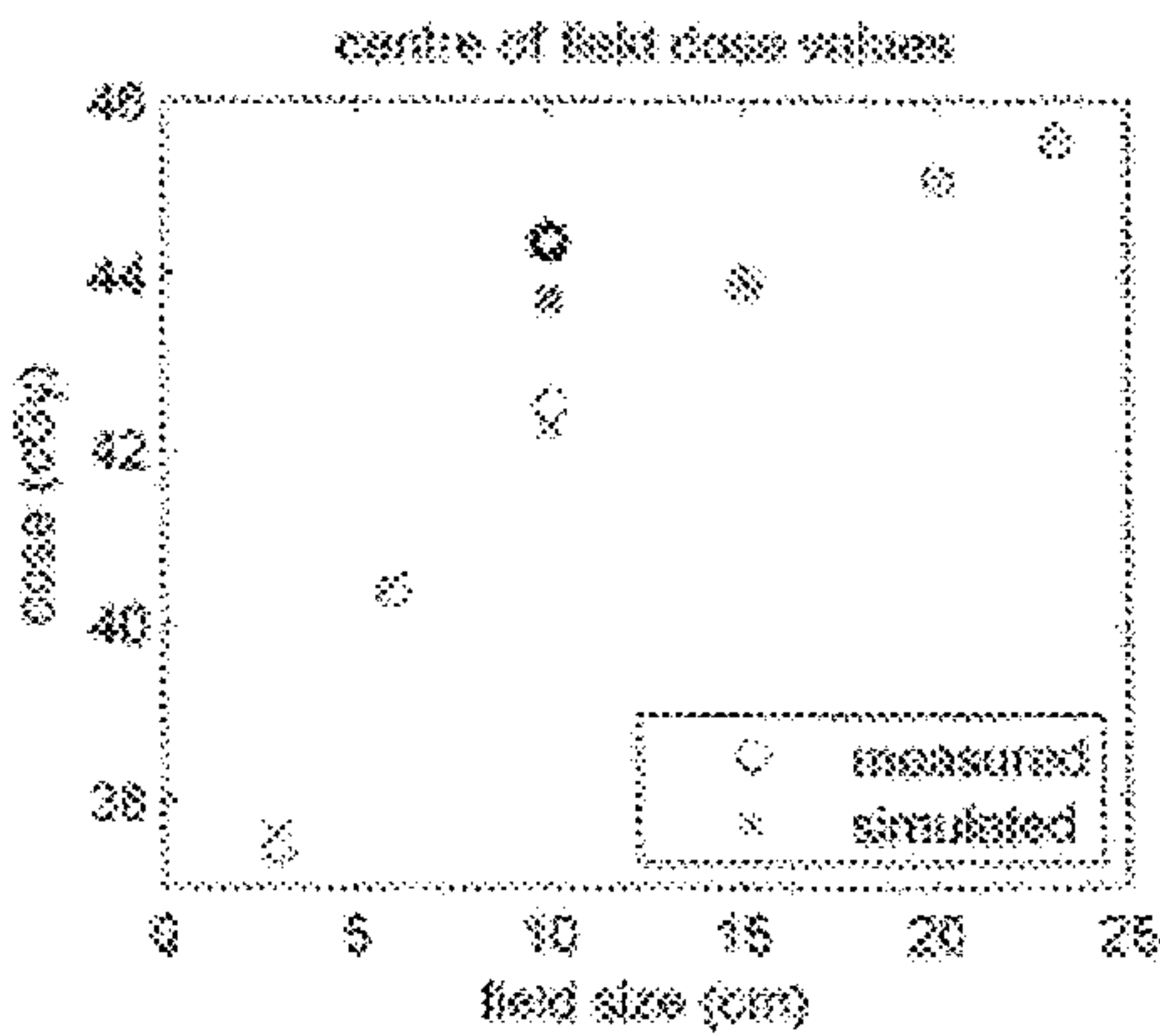
Measured and simulated point dose values from the centre of each square field. Bold markers indicate off-axis field.
