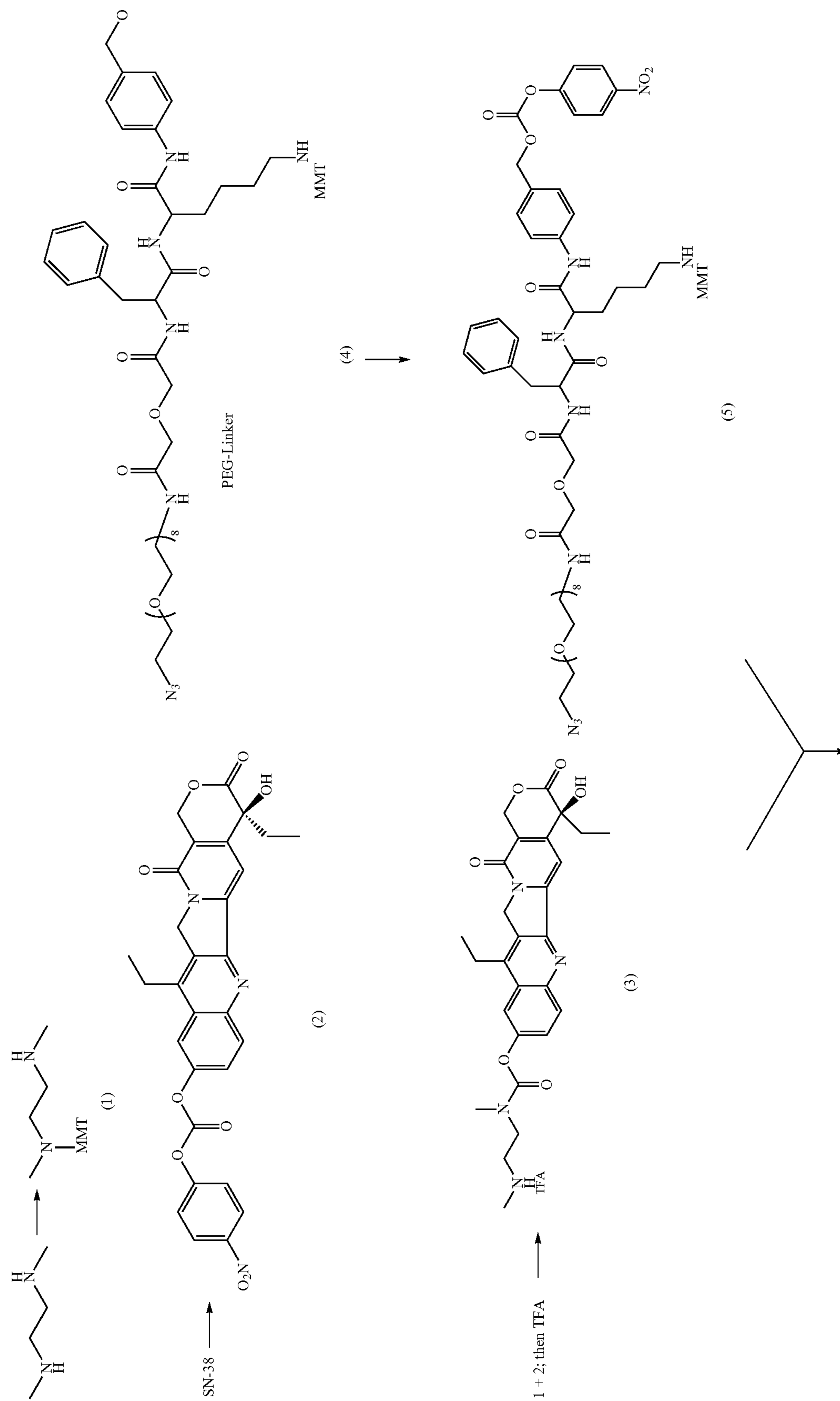
Scheme-4: Preparation of CL2E-SN-38
