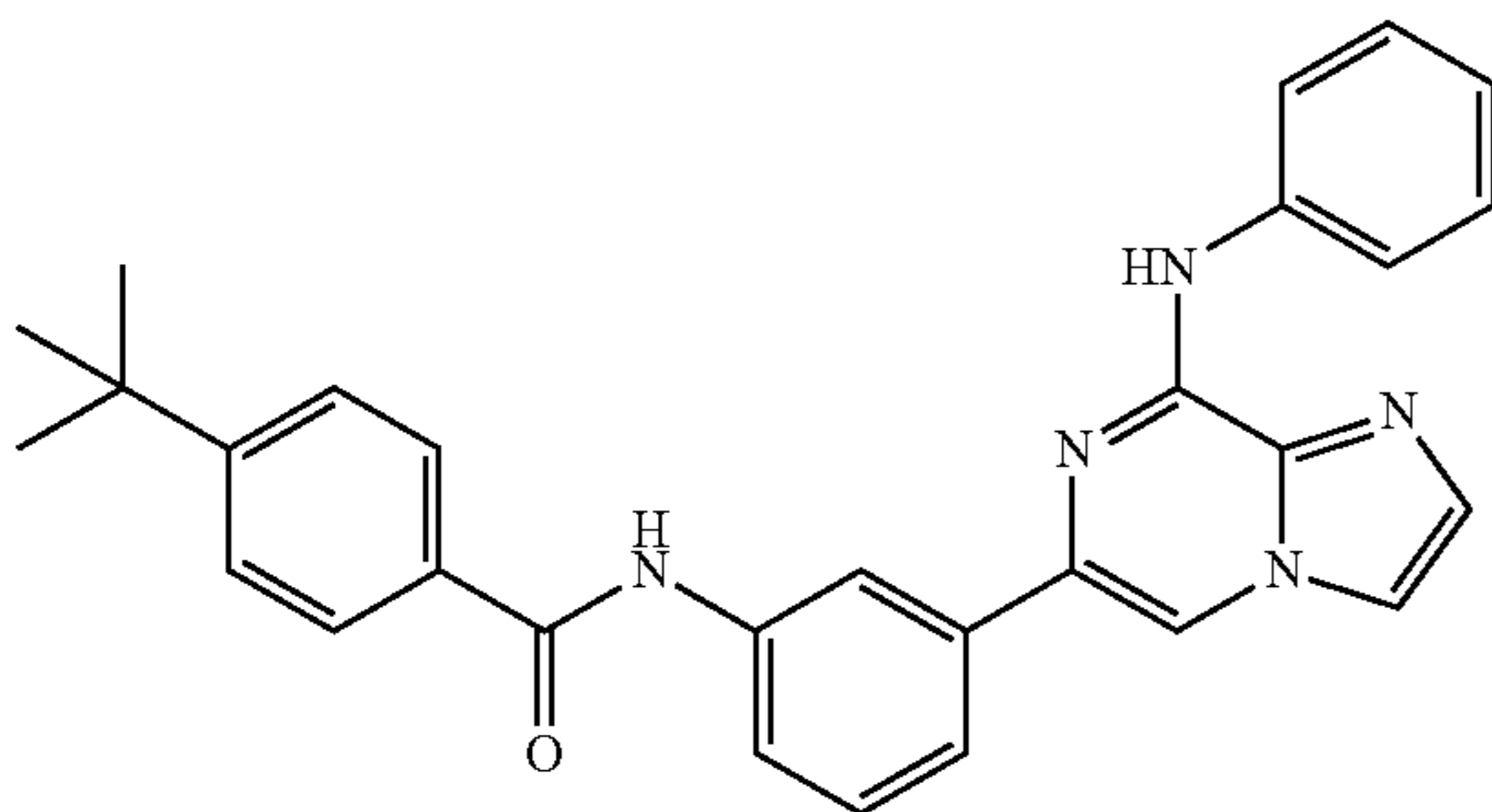
CGI-560
