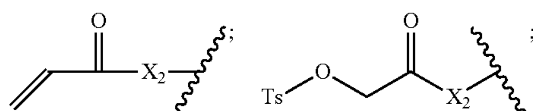
2-(tosyloxy)acetyl
