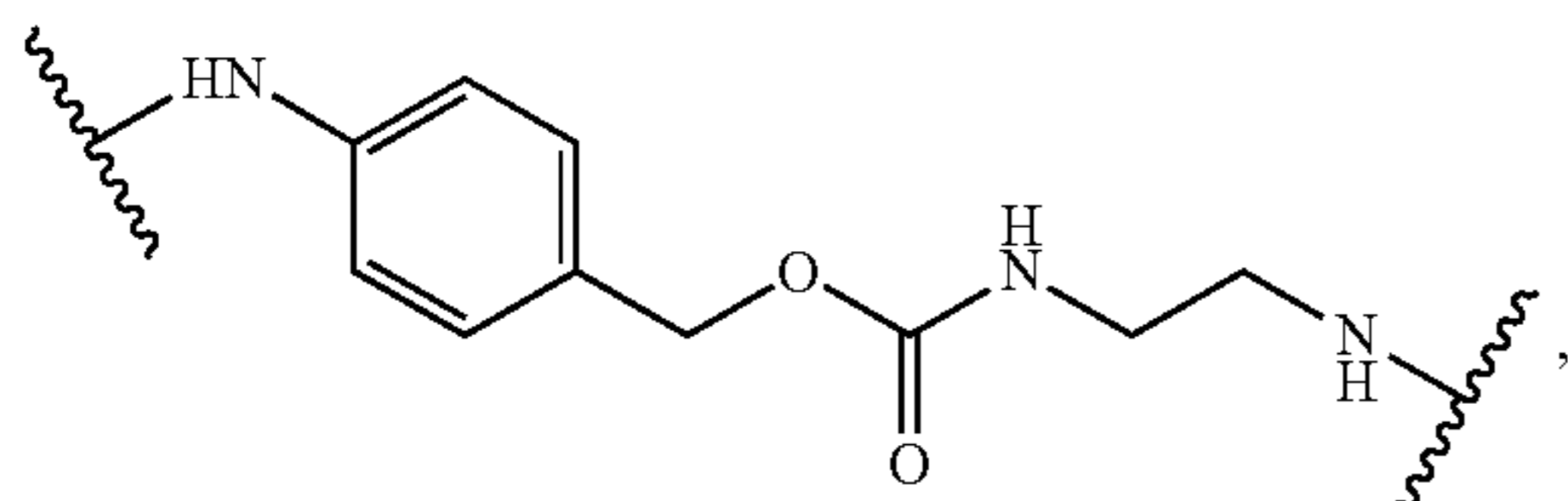
(PAB, p-aminobenzyloxycarbonyl containing)
