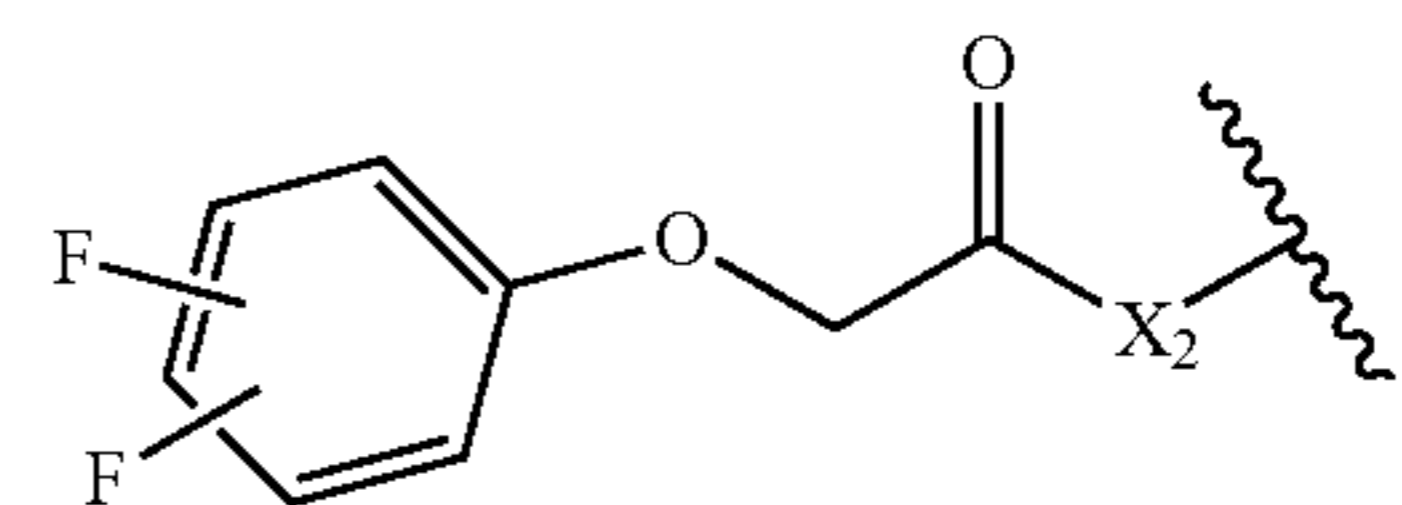
2-(difluorophenoxy)-acetyl
