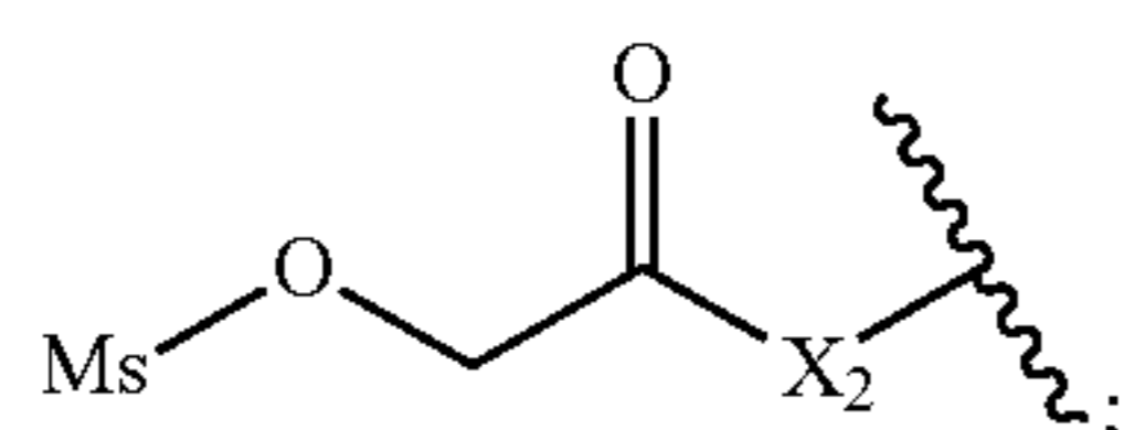
2-(mesyloxy)acetyl
