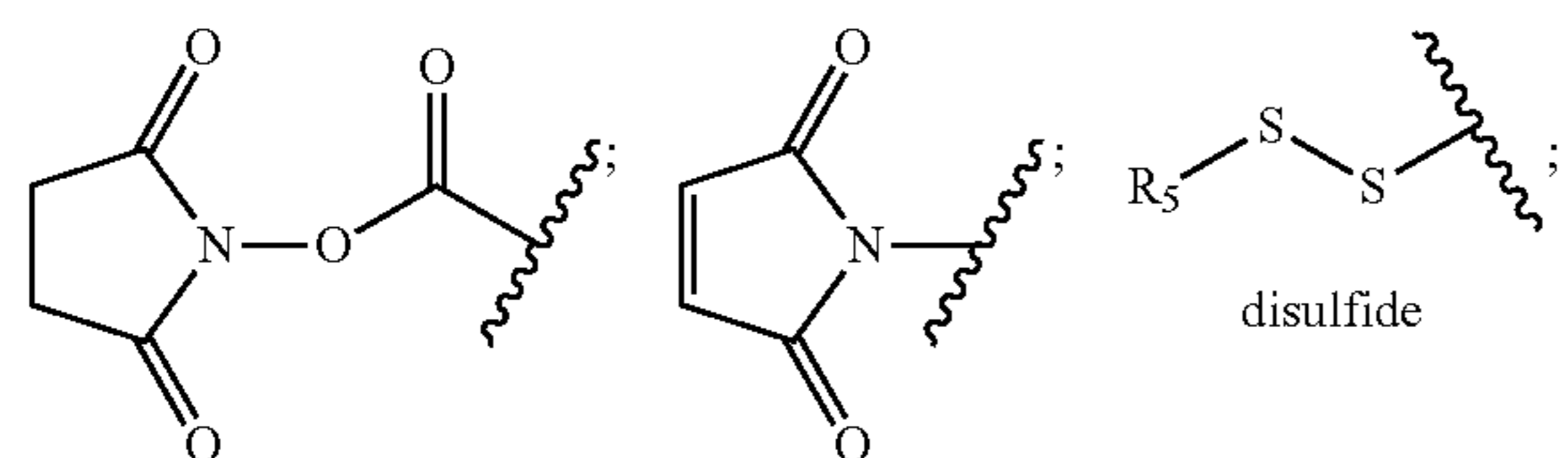
N-hydroxysuccinimide ester
