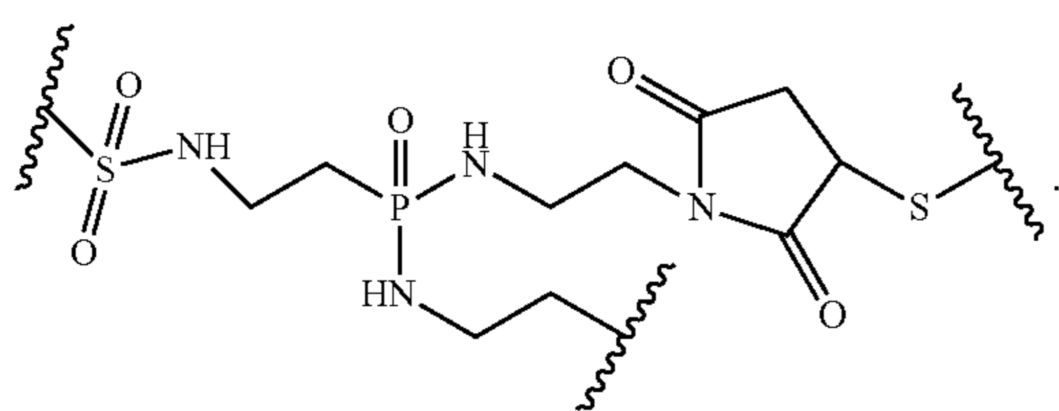
(ME, maleimidoethyl containing)
