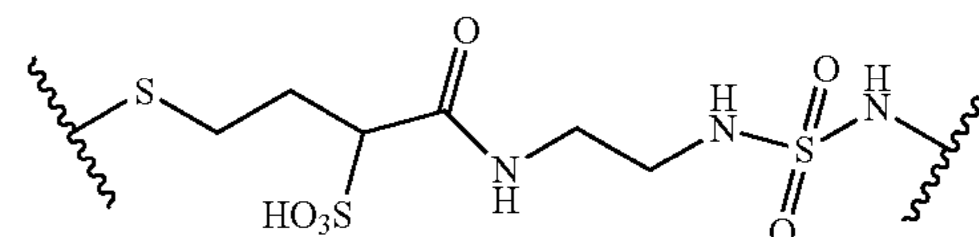
(4-thio-2-hydroxysulfonyl-butyrates, 2-sulfo-SPDB)
