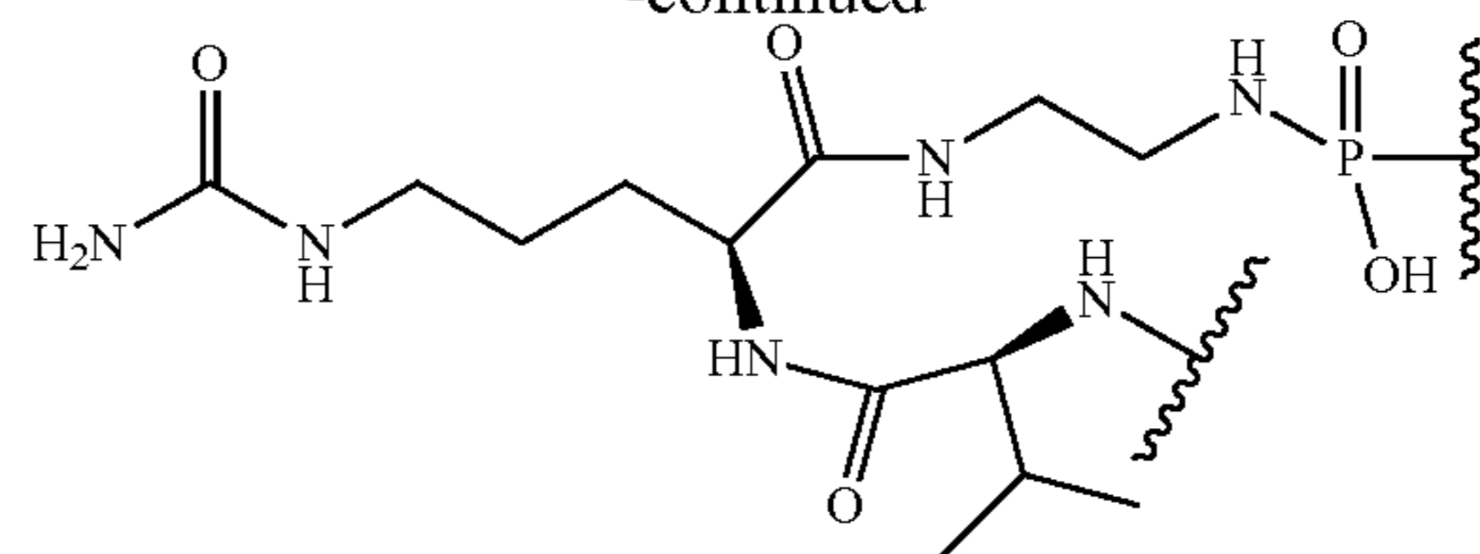
(valine-citrulline containing)
