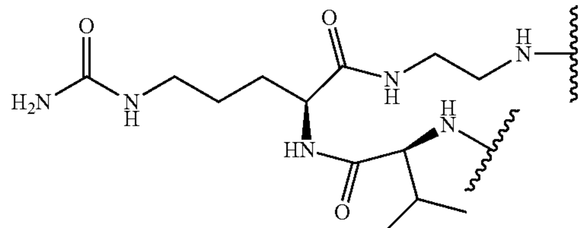
(valine-citrulline containing)
