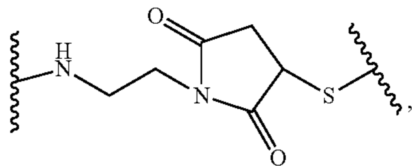
(PAB, p-aminobenzyloxycarbonyl containing)
