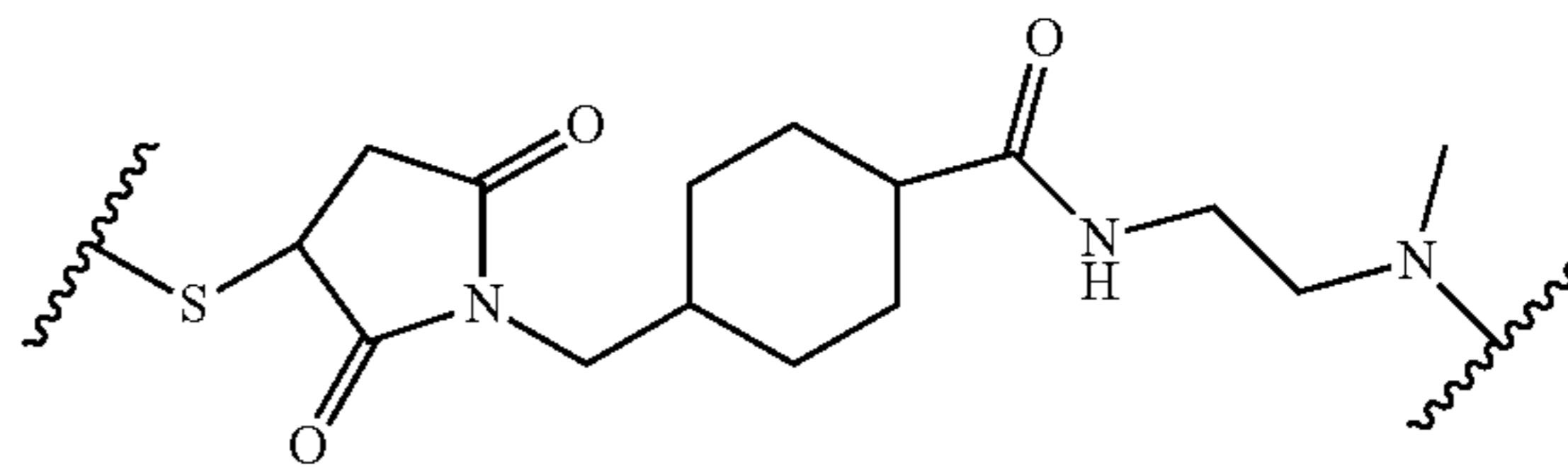
(MCC, 4-(N-maleimidomethyl)cyclohexane-1 carboxylate)
