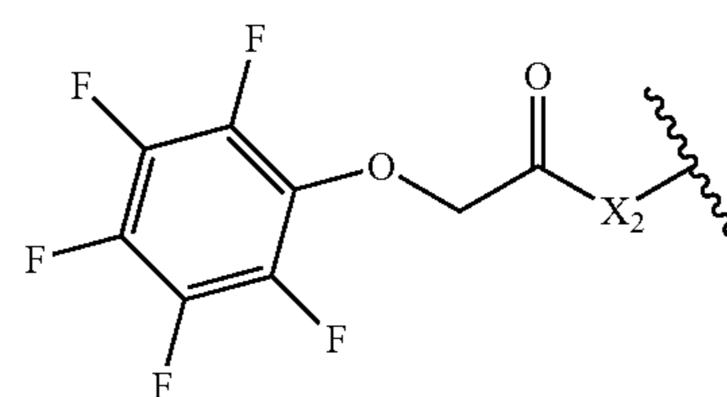
2-(pentafluorophenoxy)acetyl
