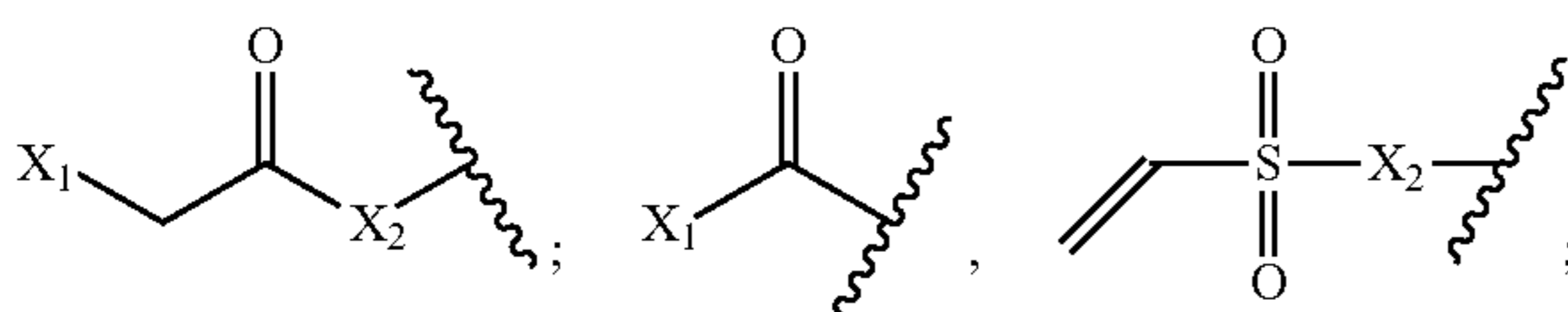
haloacetyl
