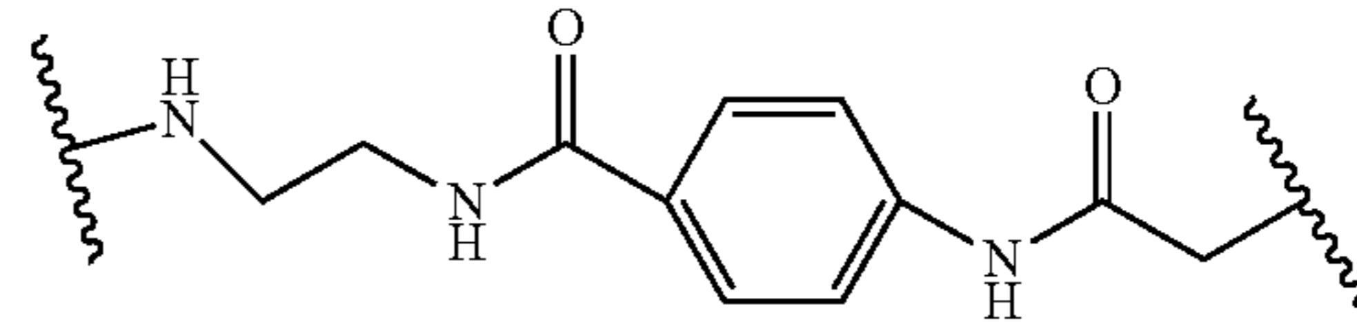
((4-acetyl)aminobenzoate containing)
