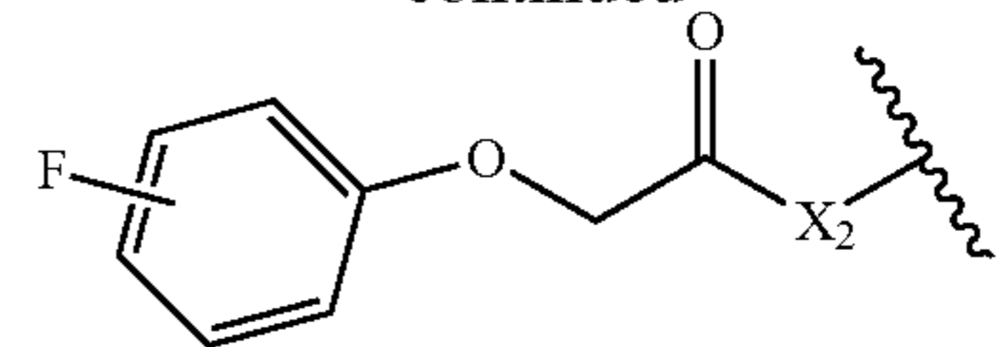
2-(fluorophenoxy)-acetyl
