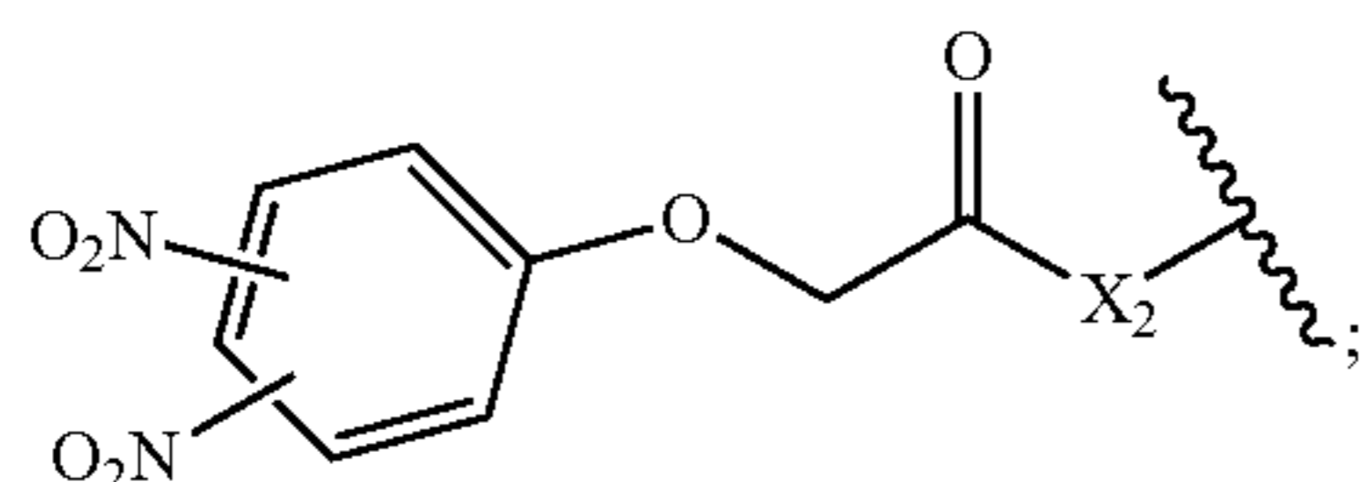
2-(dinitrophenoxy)acetyl
