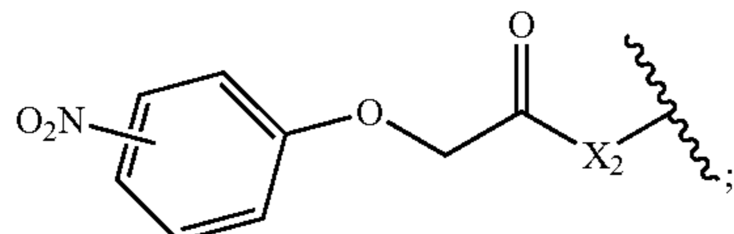
2-(nitrophenoxy)acetyl
