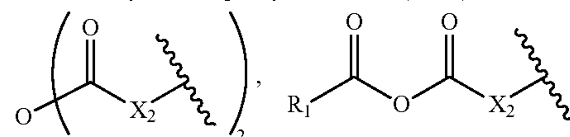
acid anhydride
