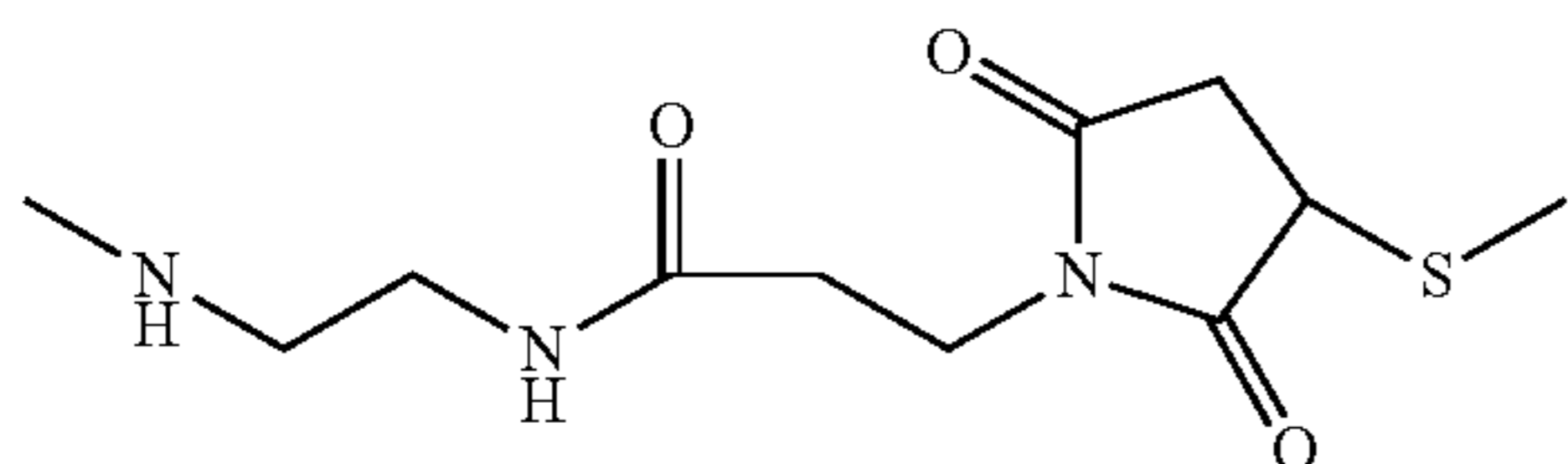
(MP, maleimidopropanoyl containing)
