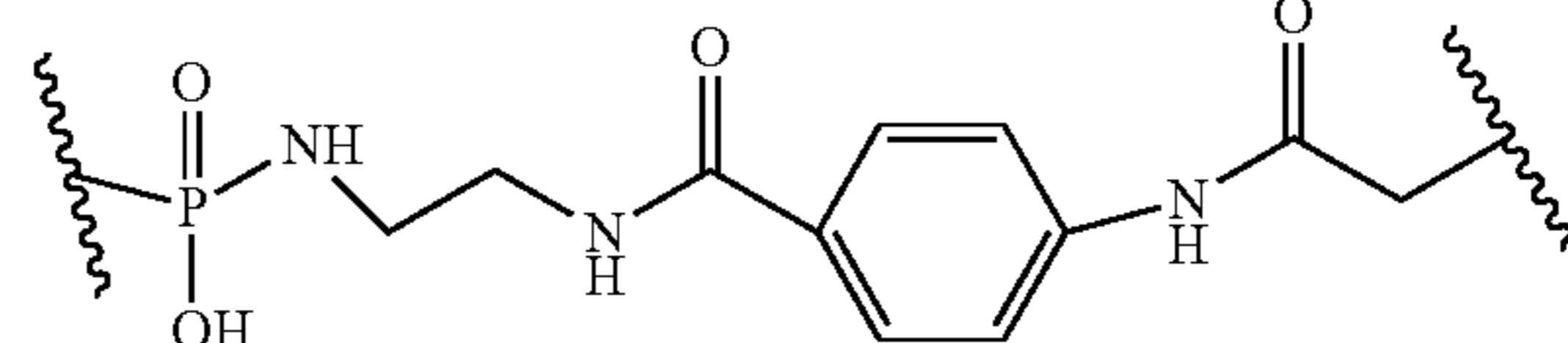
((4-acetyl)aminobenzoate containing)
