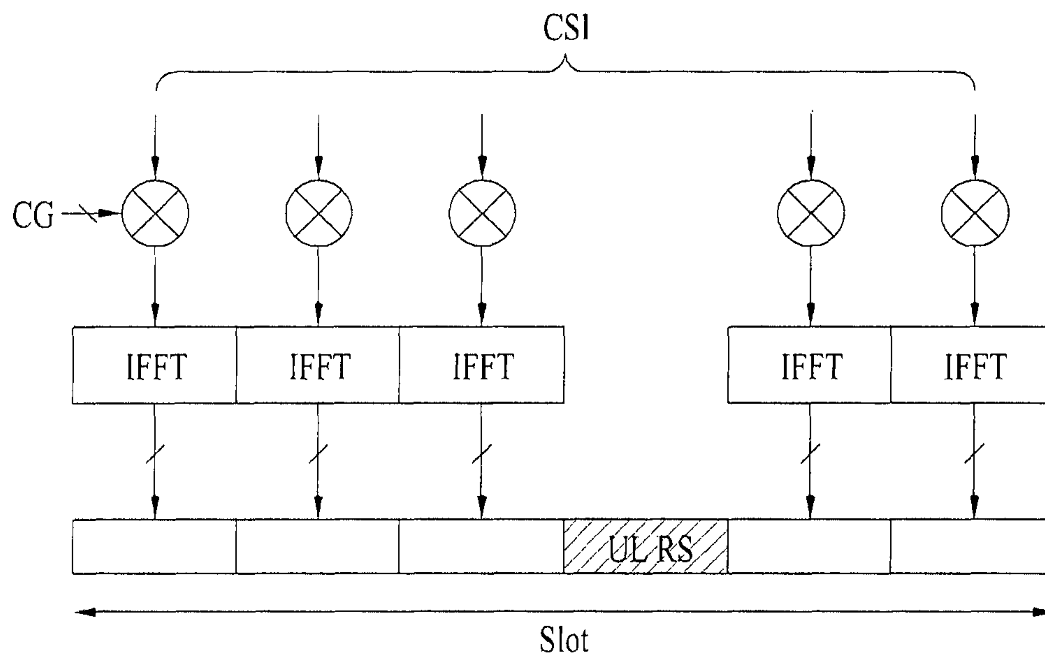
PUCCH format 2/2a/2b structure (extended CP)
