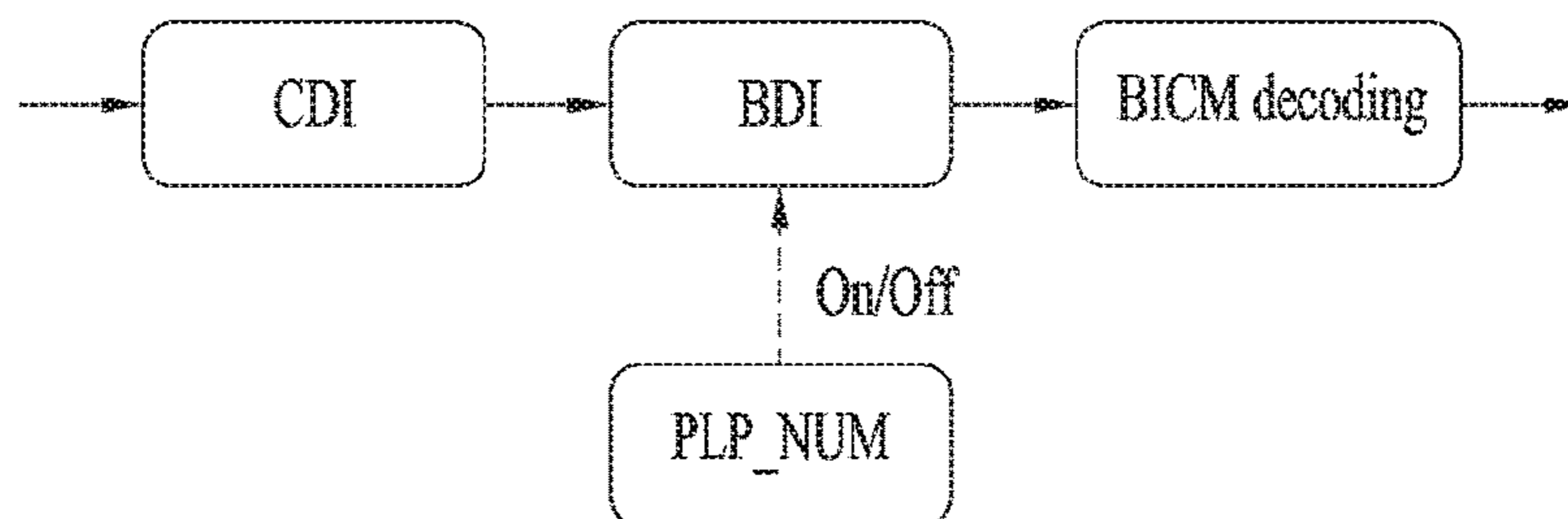
<Hybrid TDI structure: example-1>
