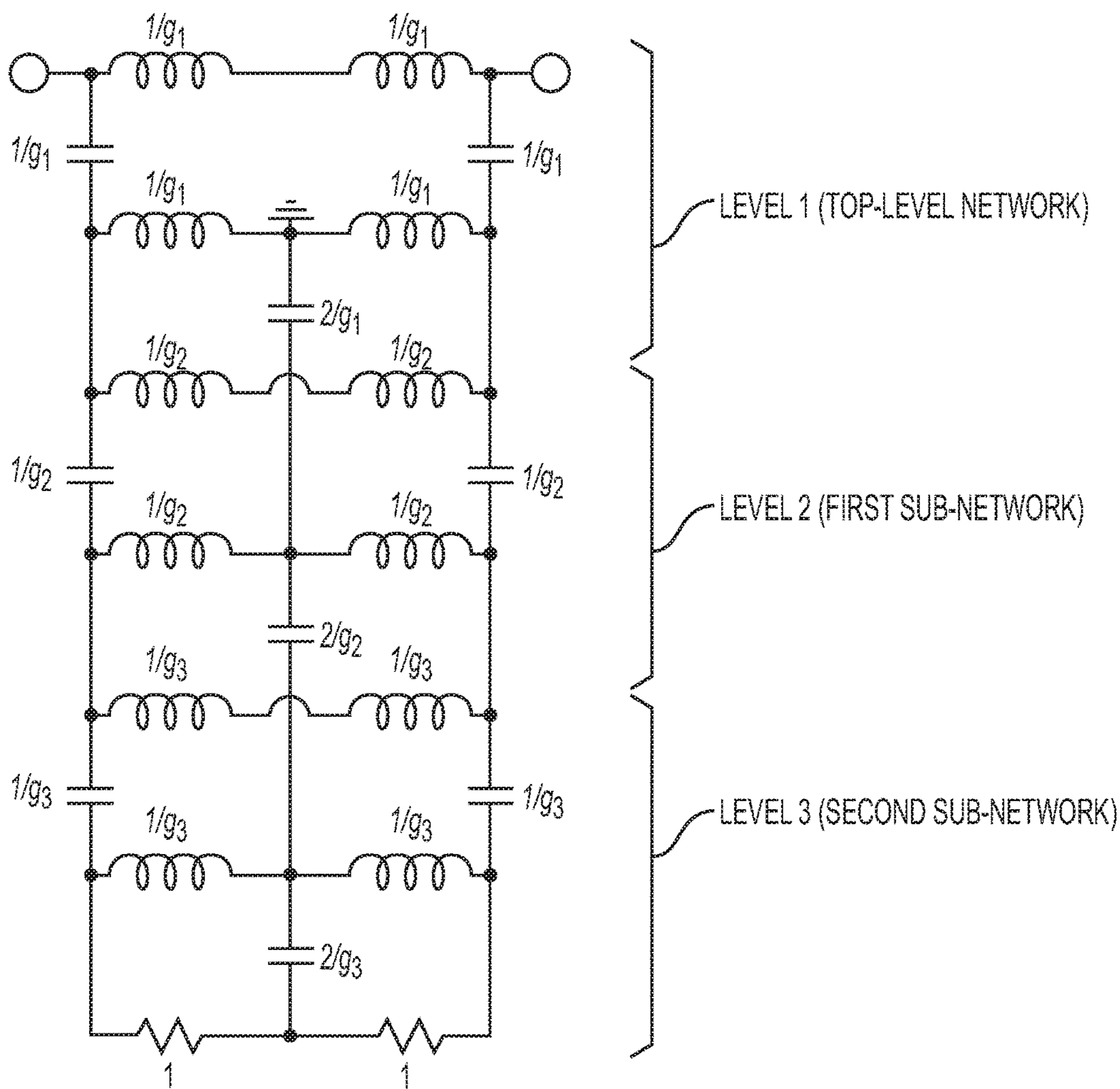
FIG. 2 PRIOR ART
