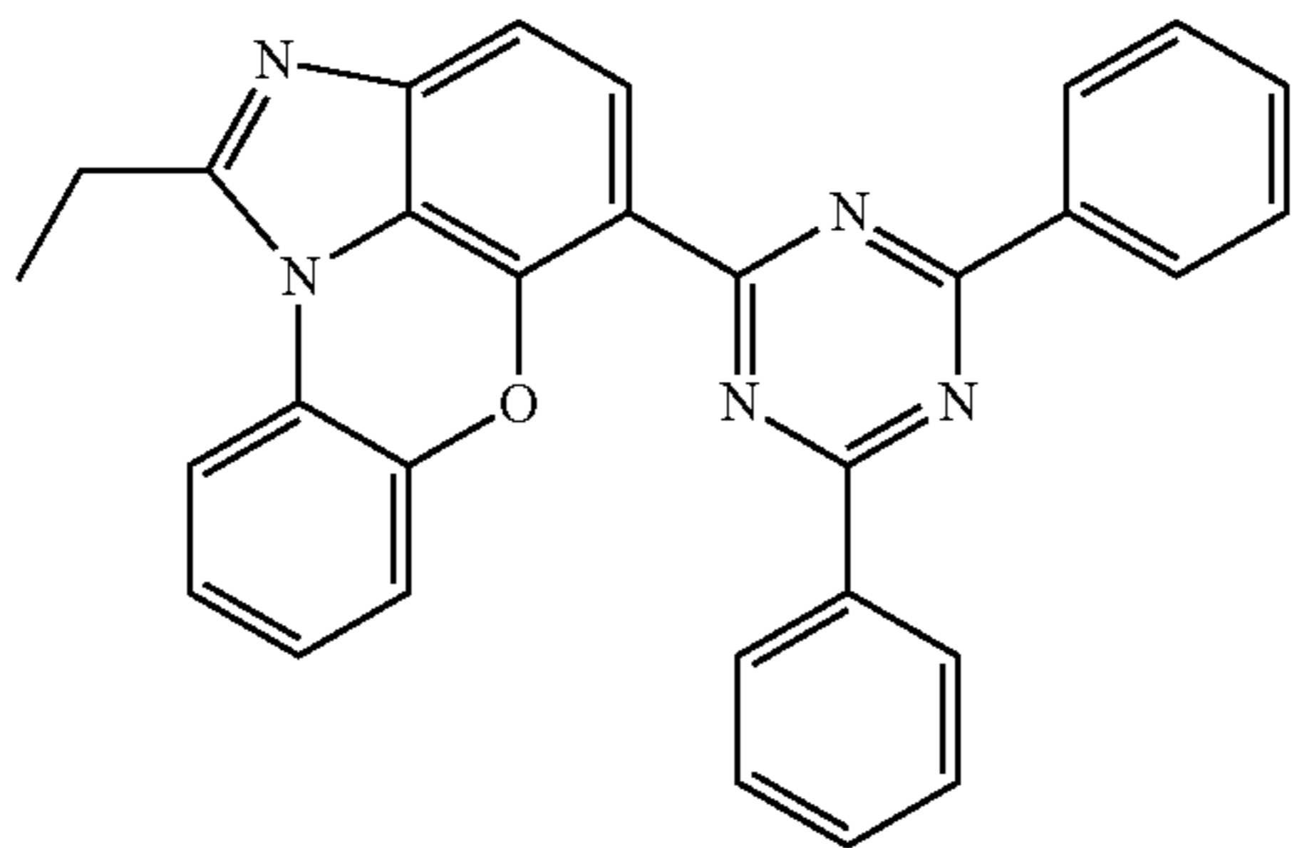
[Chemical Formula 1-9-5]
