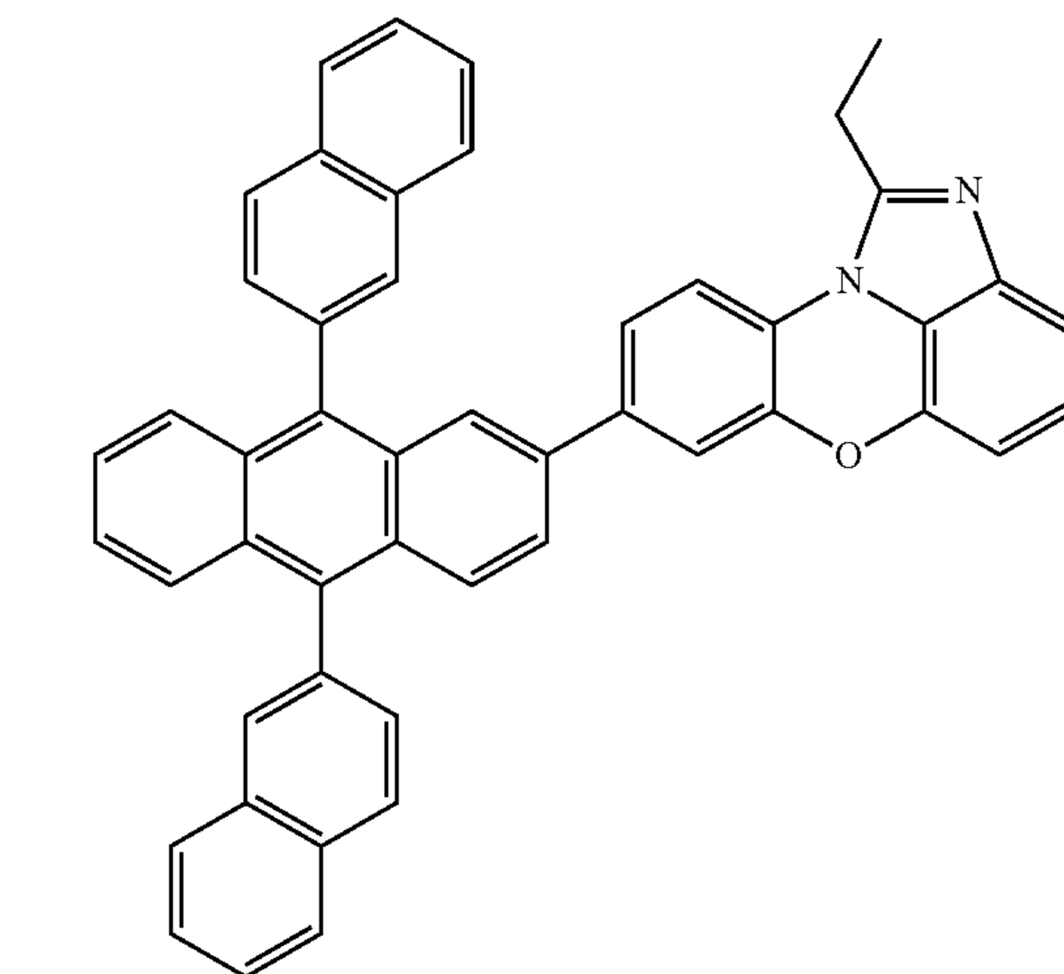
[Chemical Formula 1-3-20]
