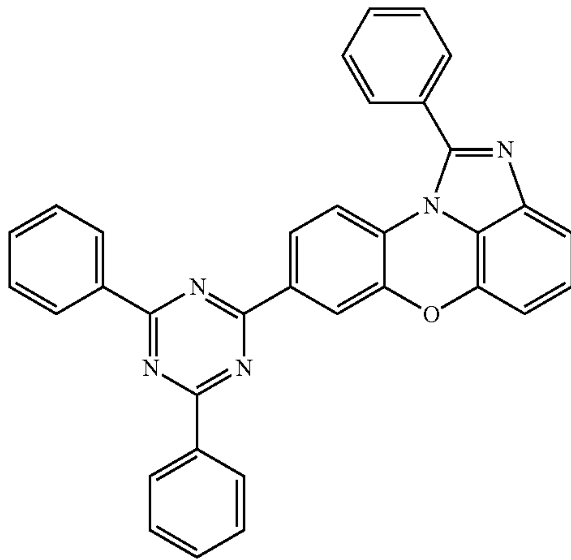
[Chemical Formula 1-4-41]
