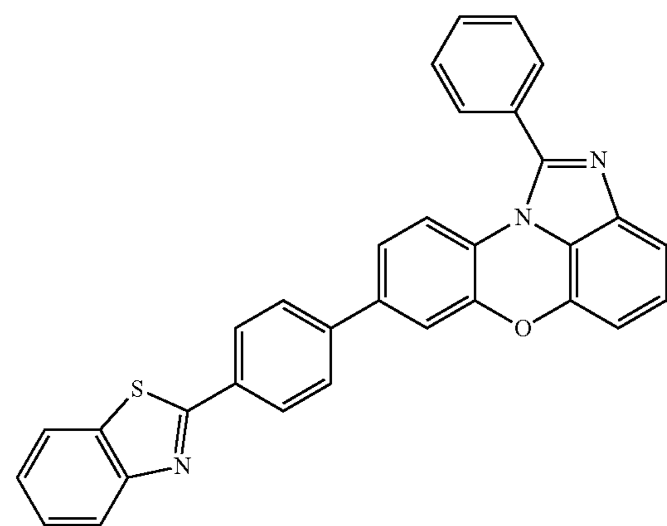
[Chemical Formula 1-4-46]
