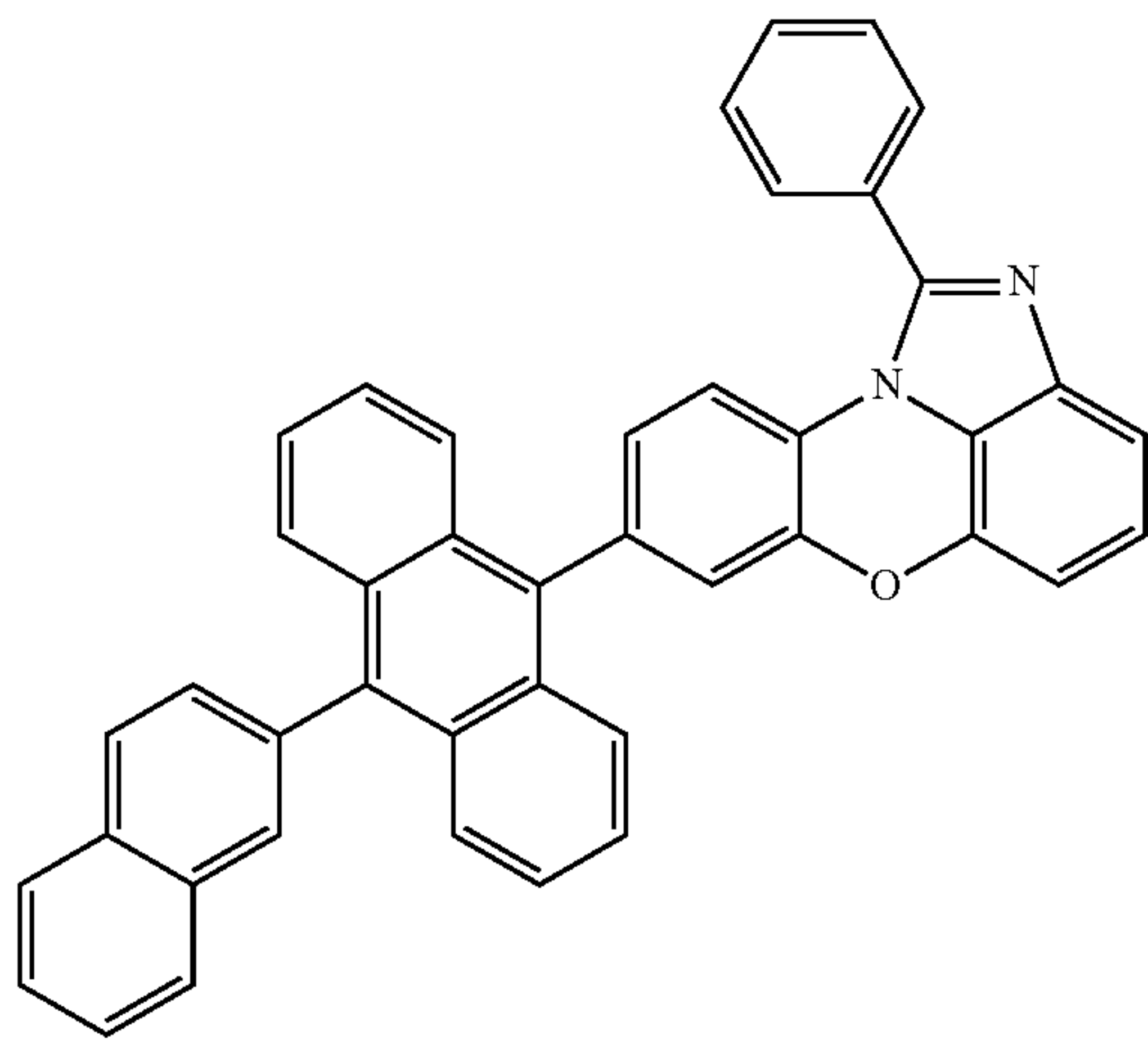
[Chemical Formula 1-4-2]
