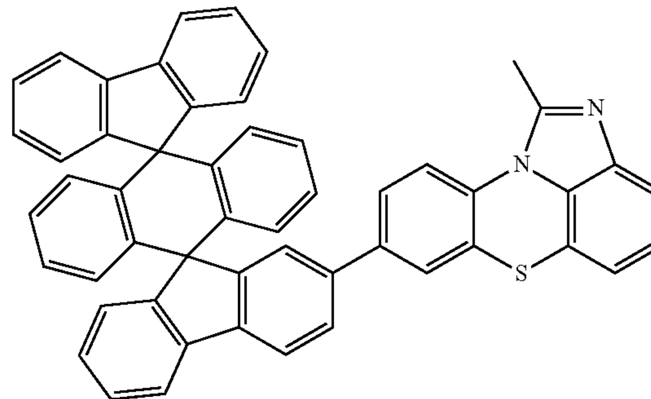
[Chemical Formula 2-2-36]
