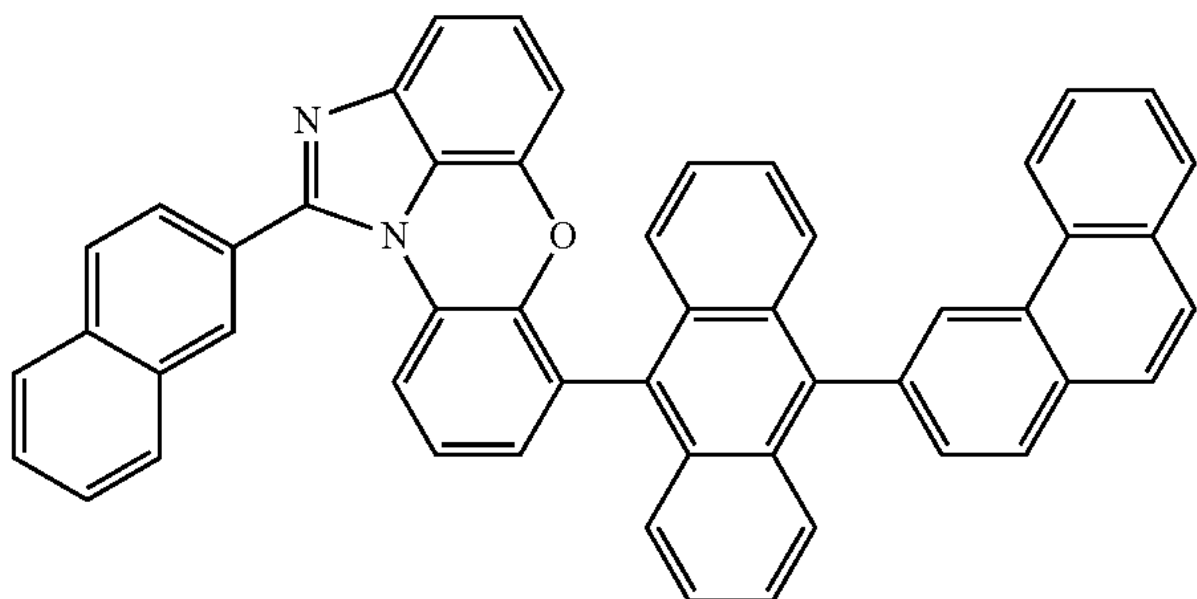
[Chemical Formula 1-6-8]
