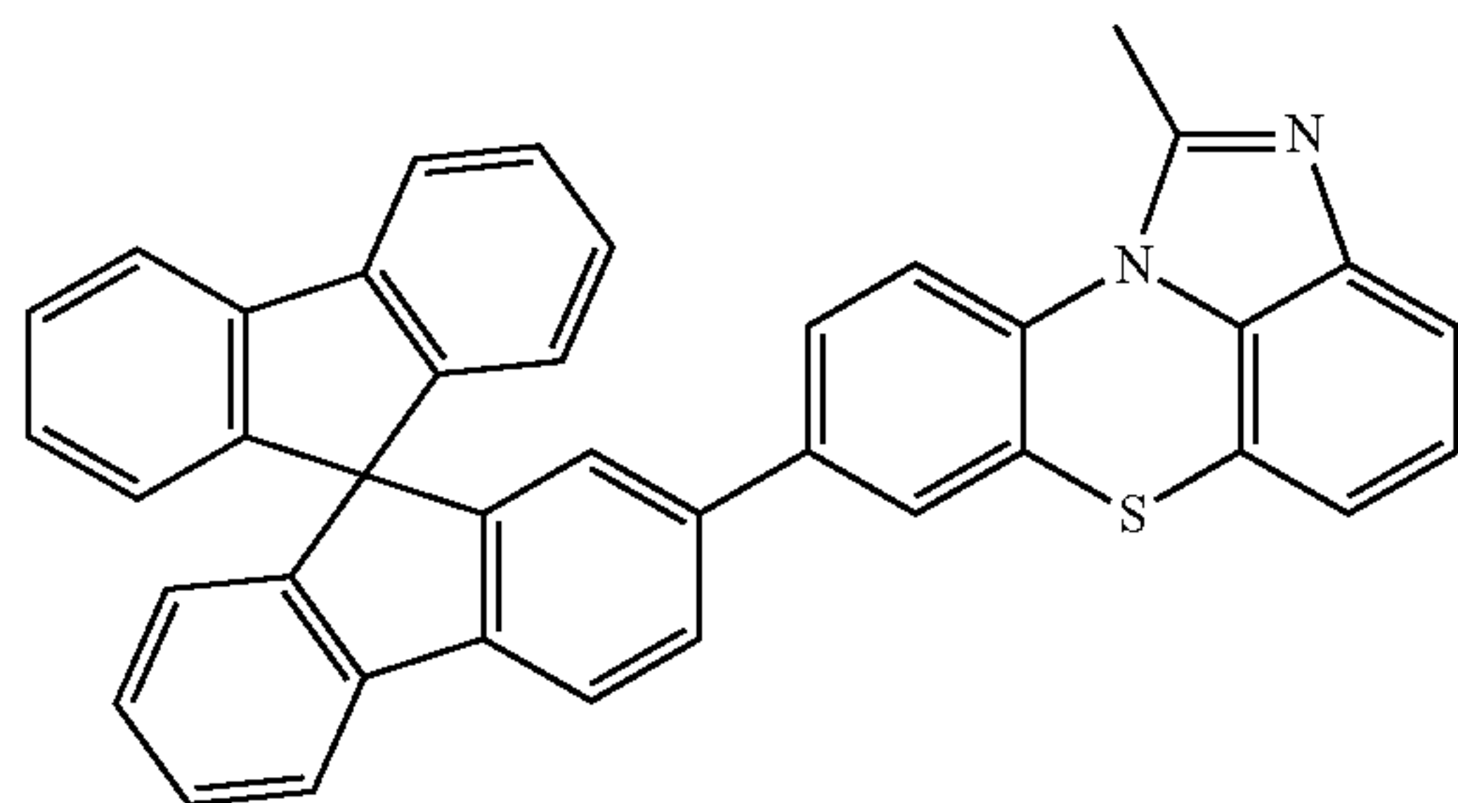
[Chemical Formula 2-2-34]
