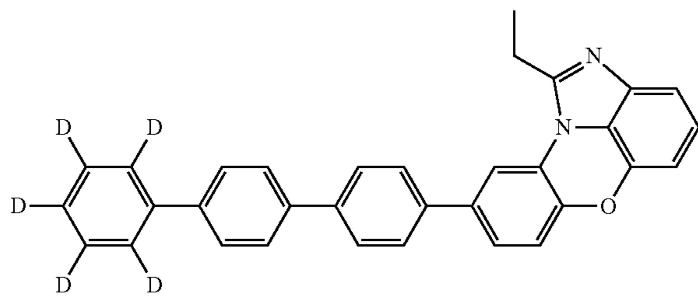
[Chemical Formula 1-7-52]
