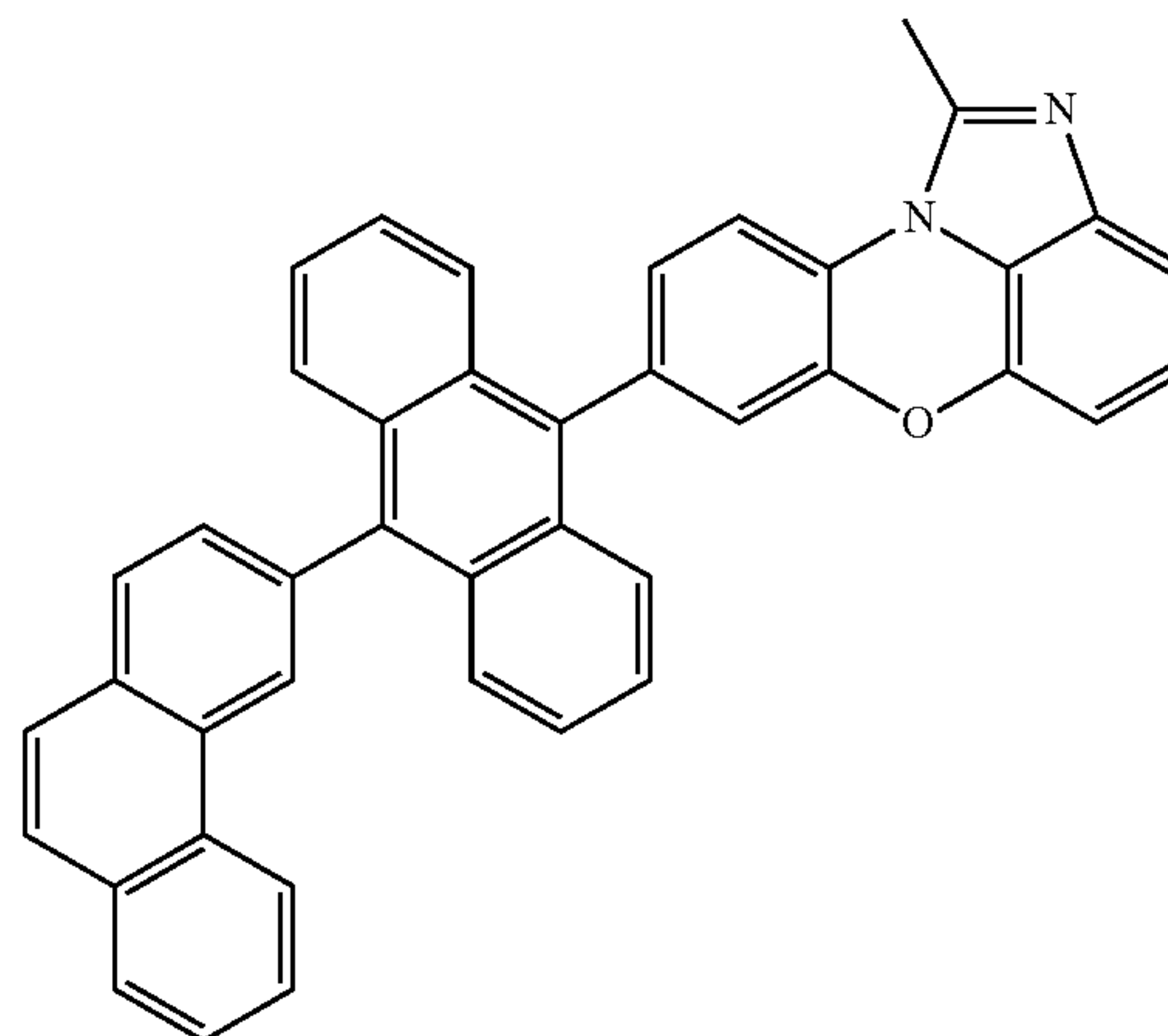
[Chemical Formula 1-2-9]
