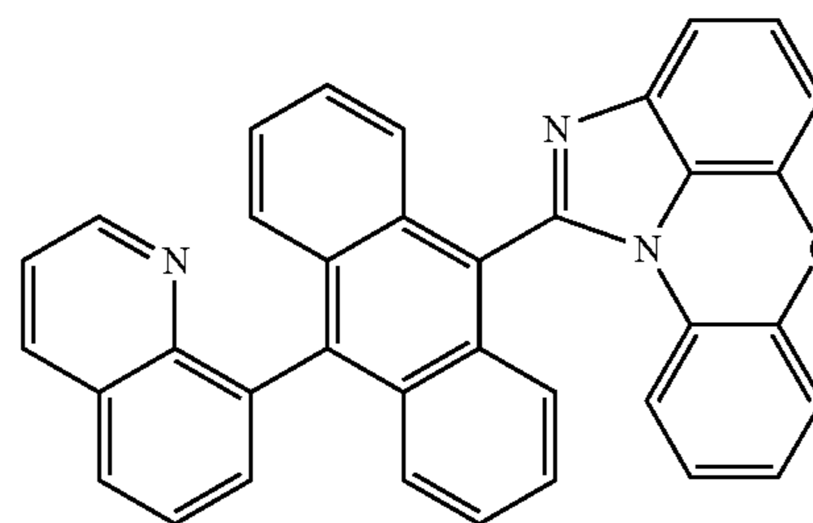
[Chemical Formula 1-1-20]
