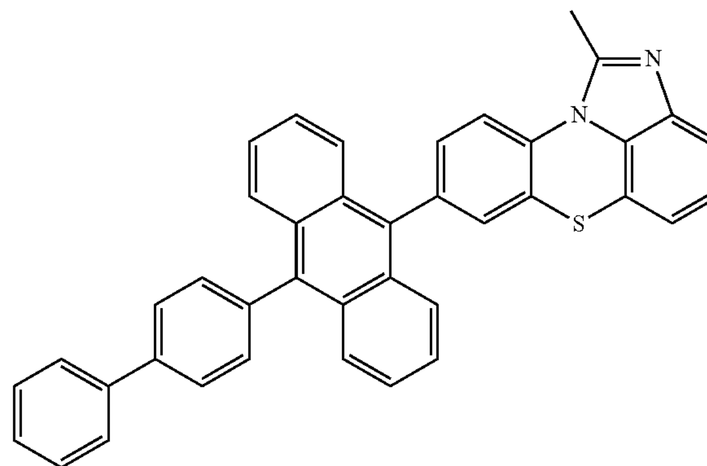
[Chemical Formula 2-2-4]
