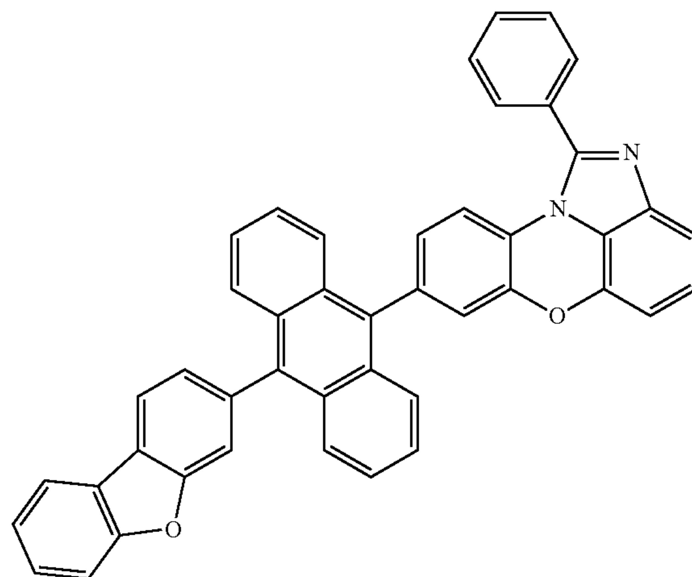
[Chemical Formula 1-4-13]
