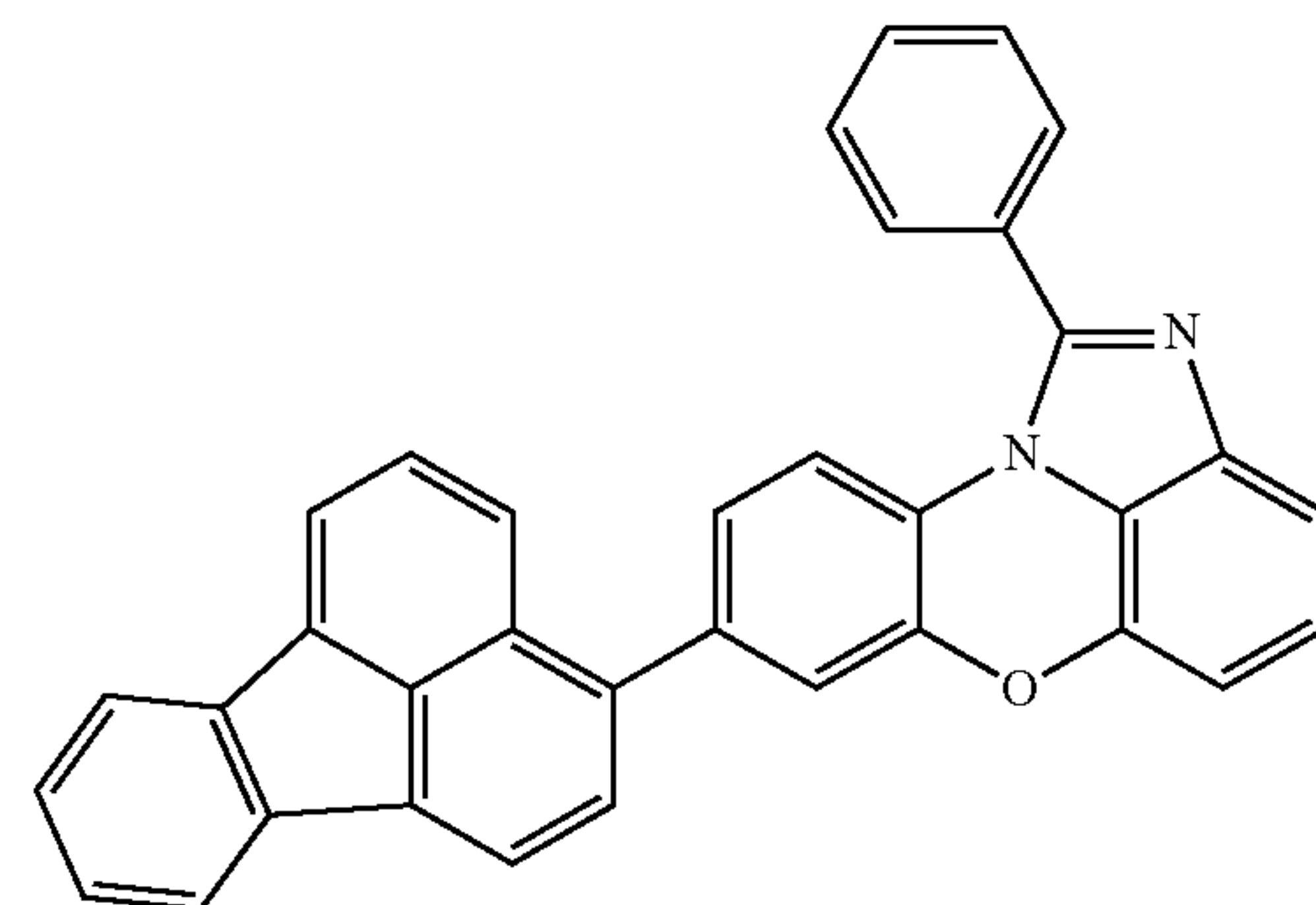
[Chemical Formula 1-4-31]
