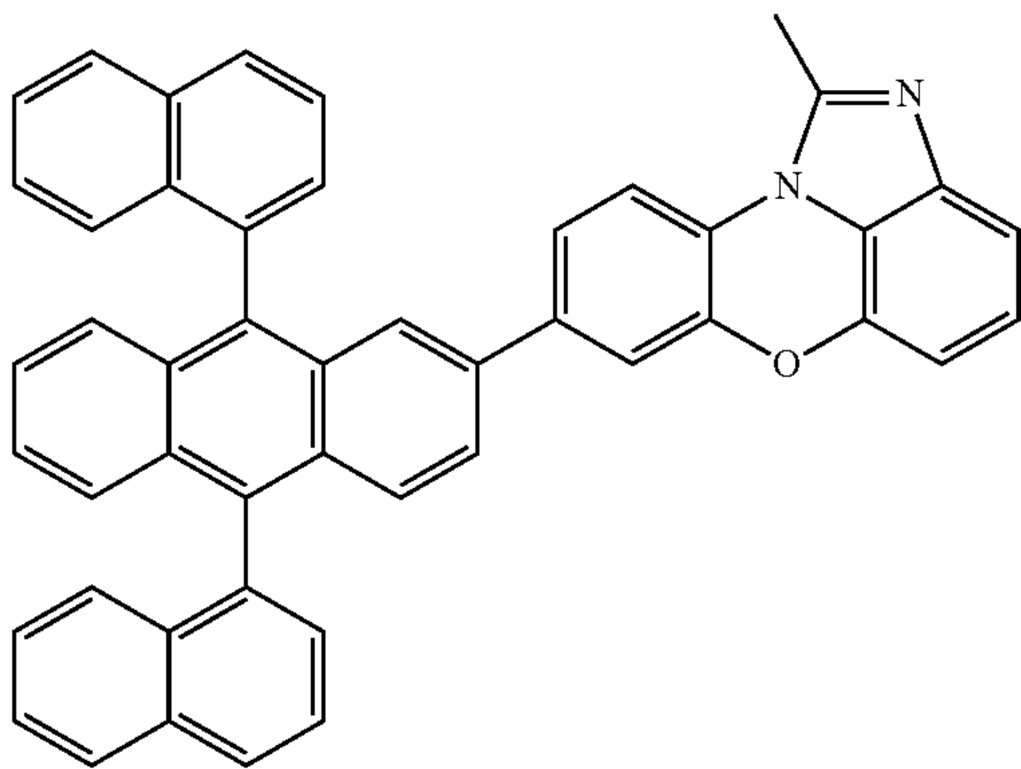
[Chemical Formula 1-2-21]
