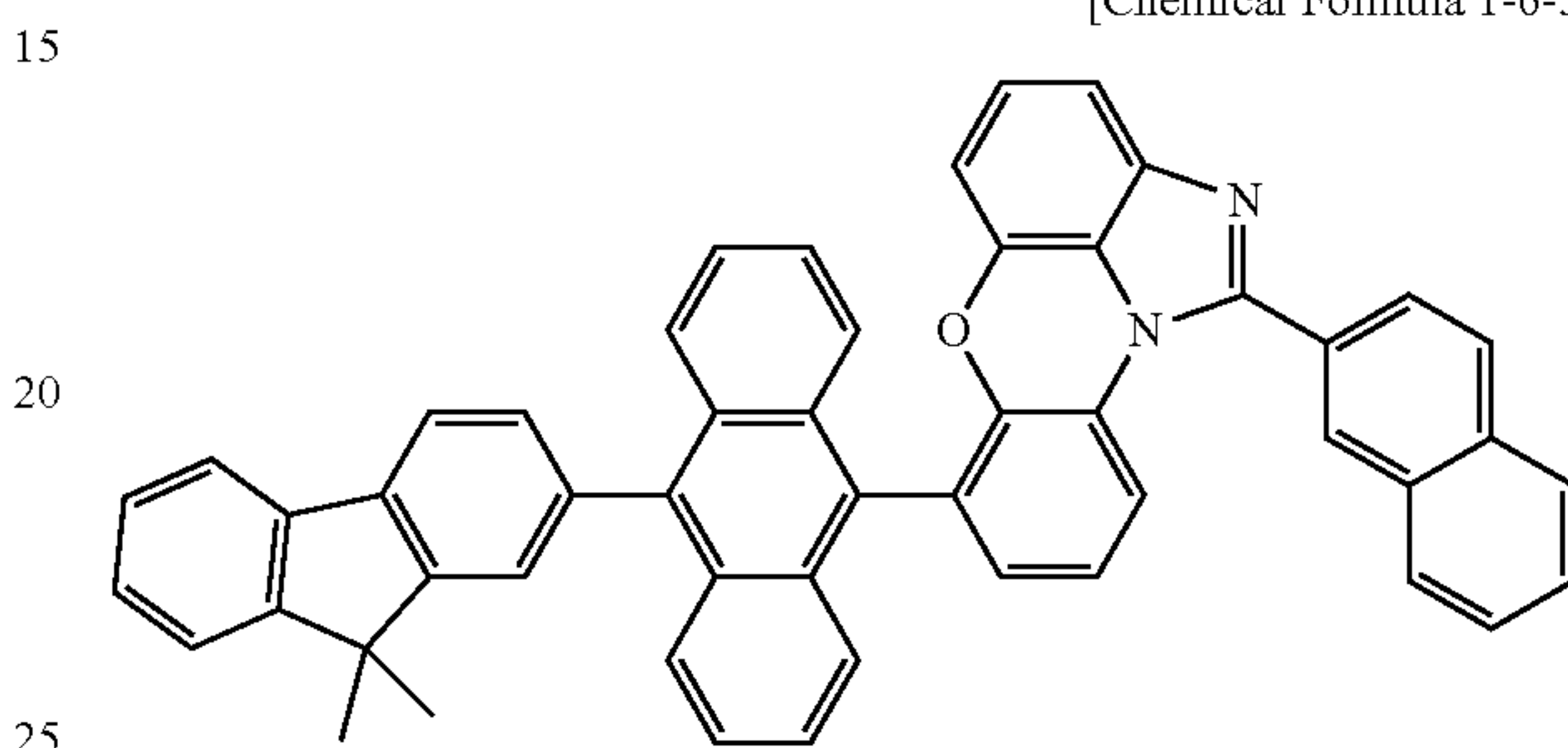
[Chemical Formula 1-6-5]
