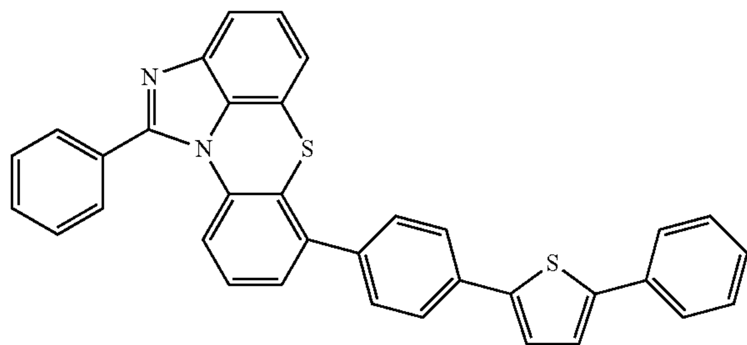
[Chemical Formula 2-2-39]
