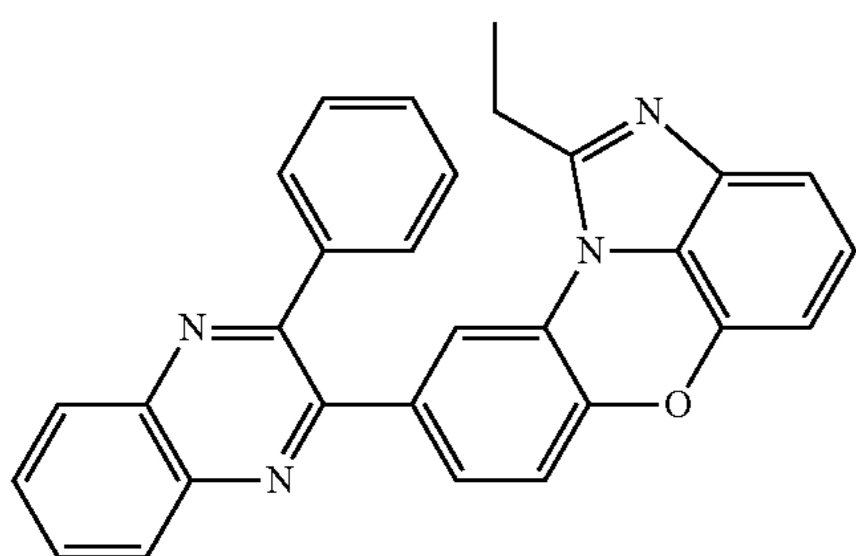
[Chemical Formula 1-7-49]
