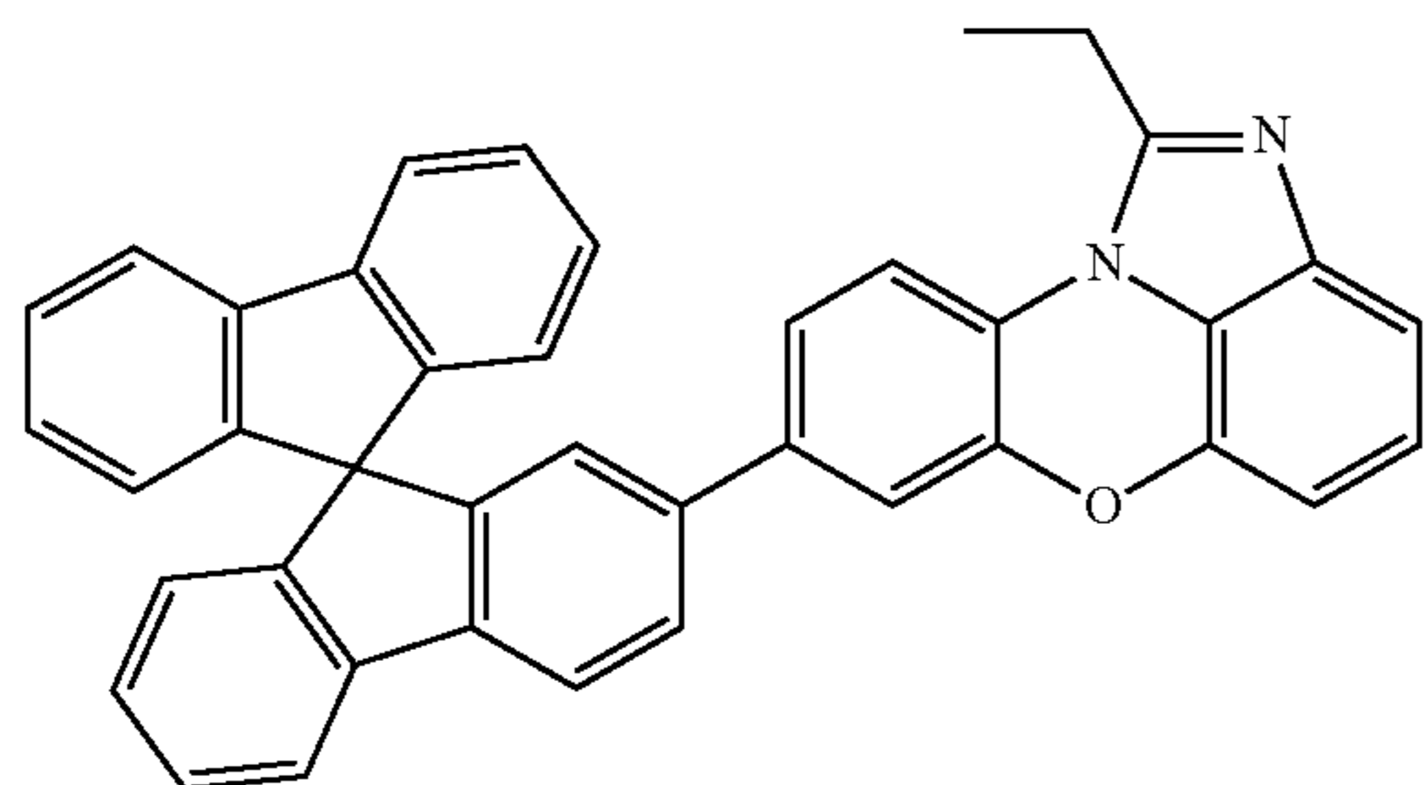
[Chemical Formula 1-3-34]
