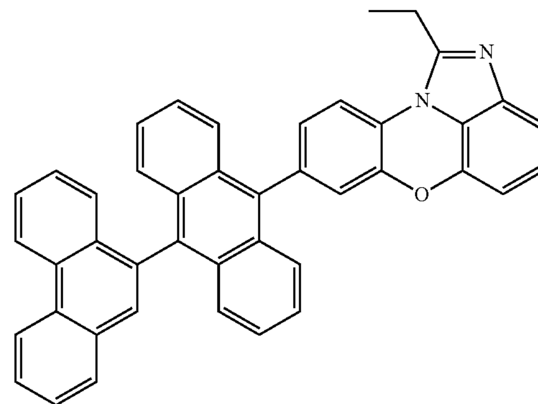
[Chemical Formula 1-3-7]
