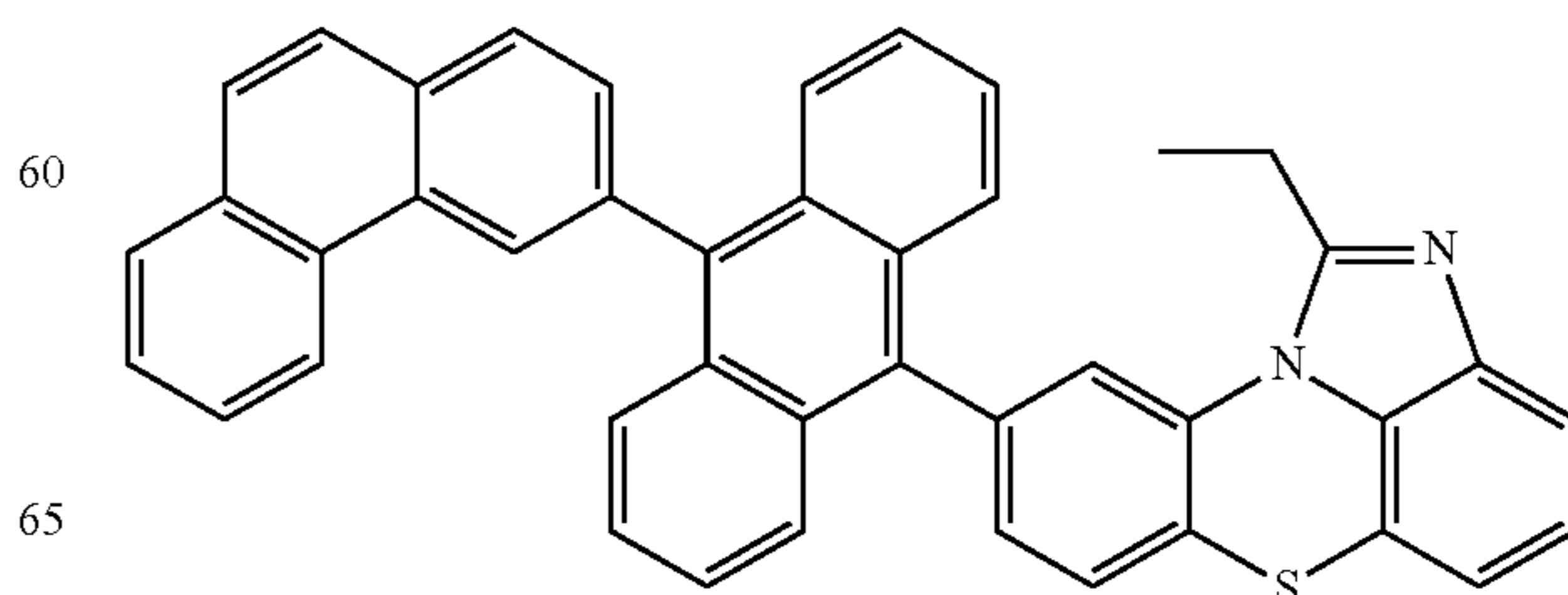
[Chemical Formula 2-3-8]
