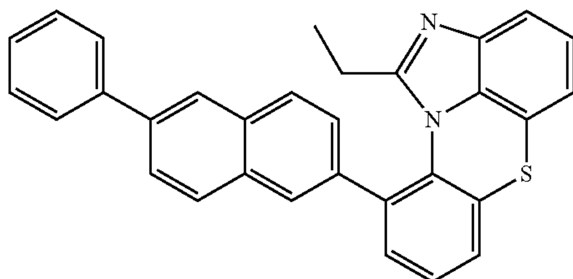
[Chemical Formula 2-3-30]
