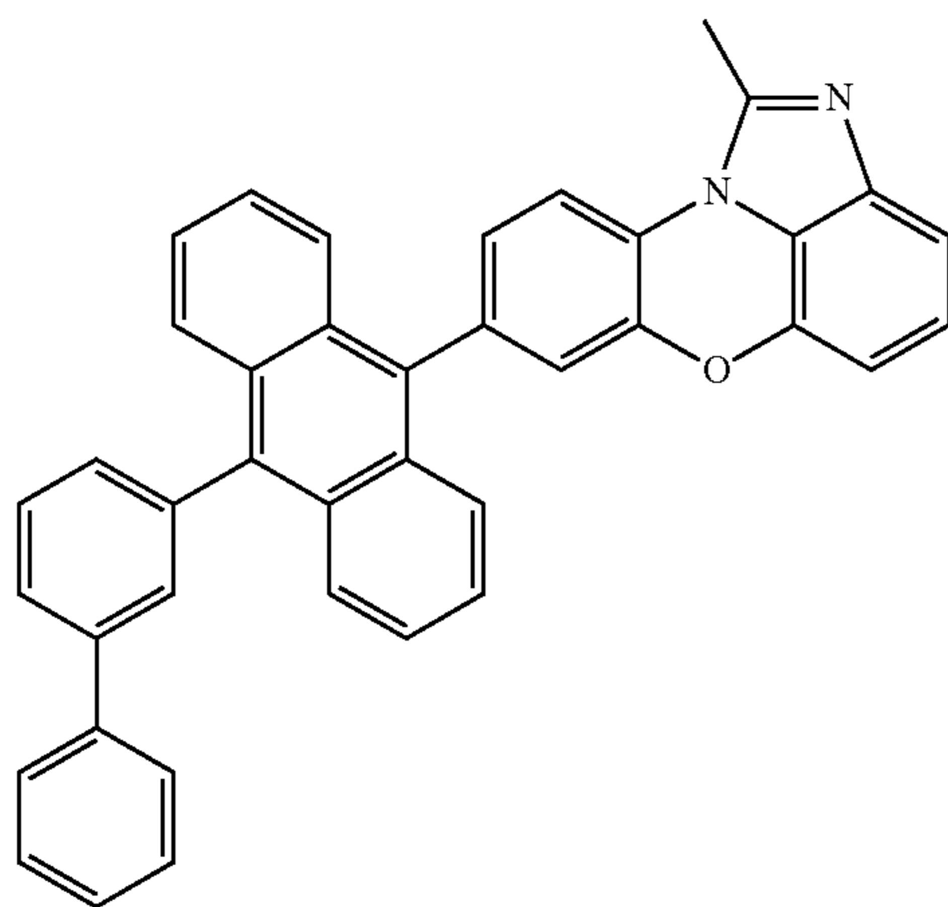
[Chemical Formula 1-2-7]
