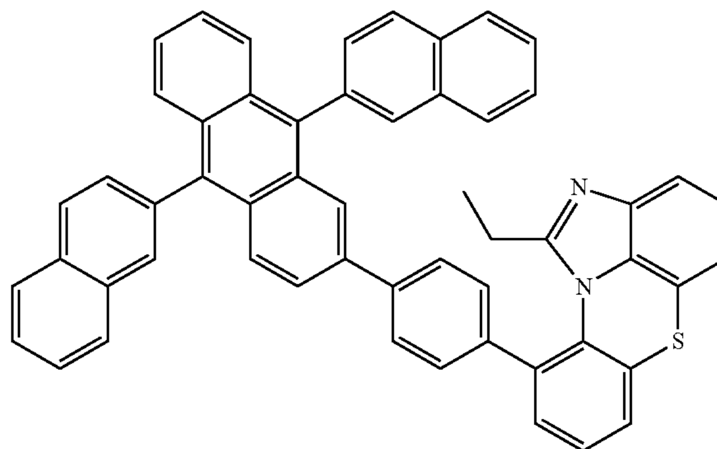
[Chemical Formula 2-3-25]
