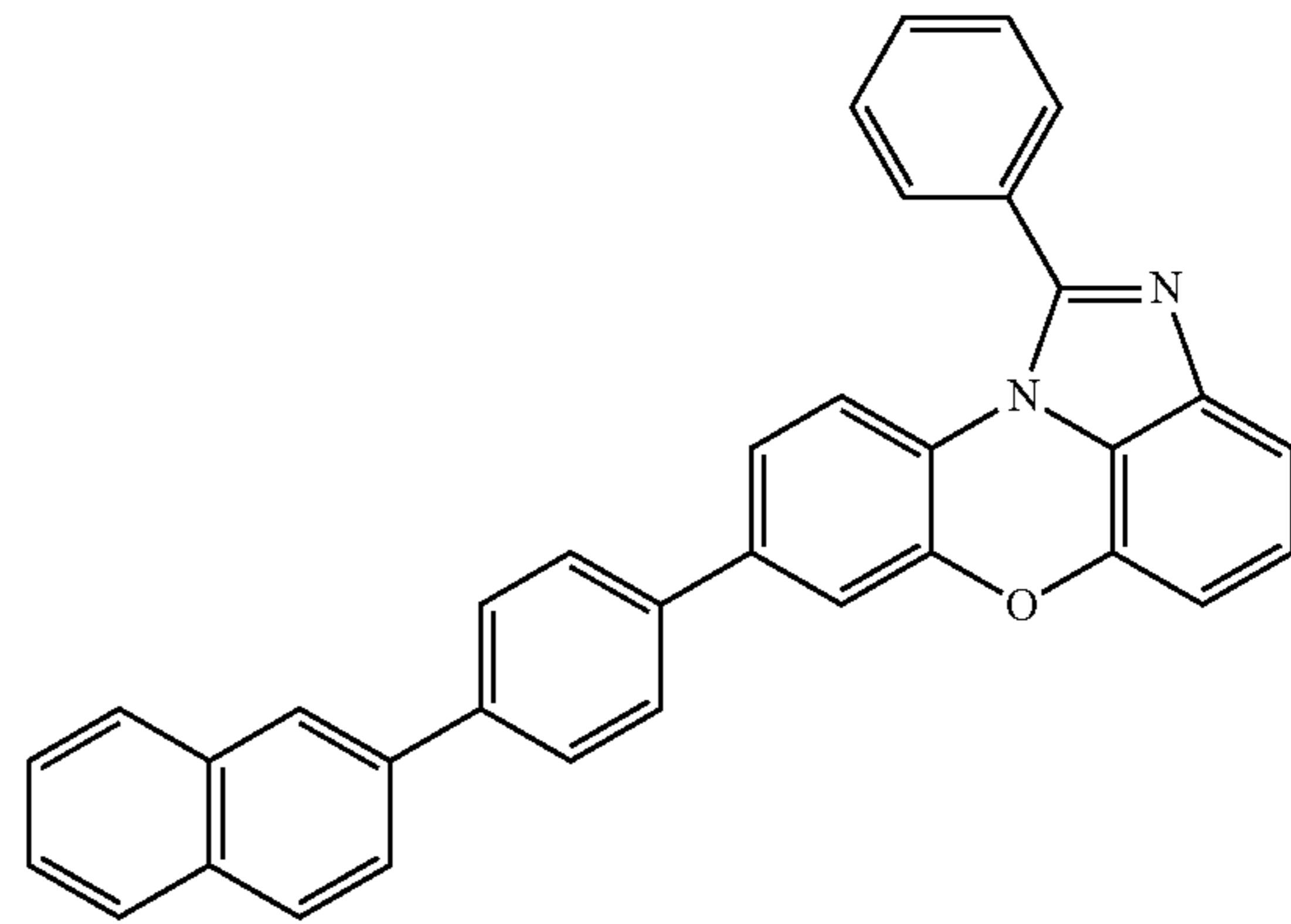
[Chemical Formula 1-4-26]
