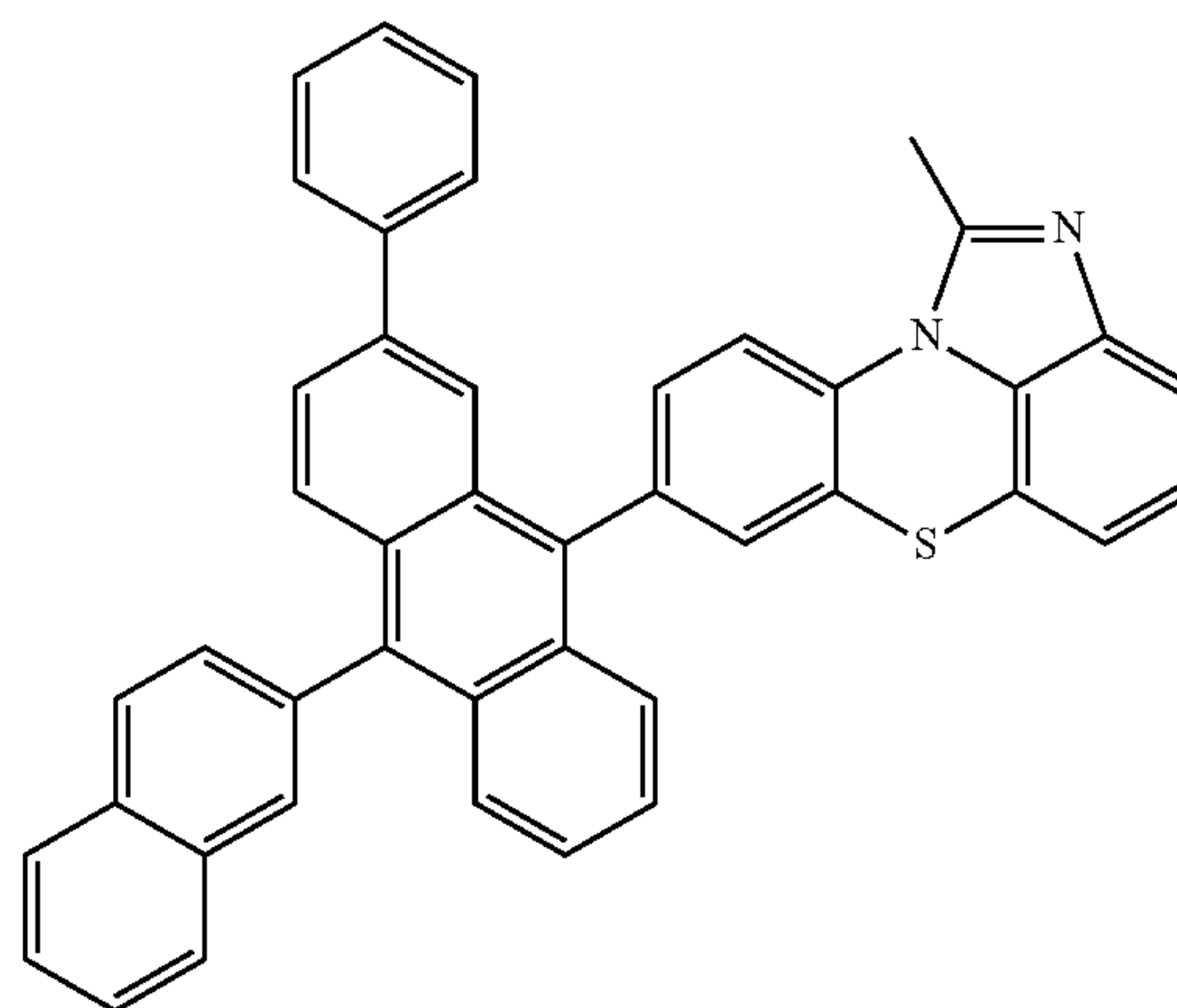
[Chemical Formula 2-2-16]
