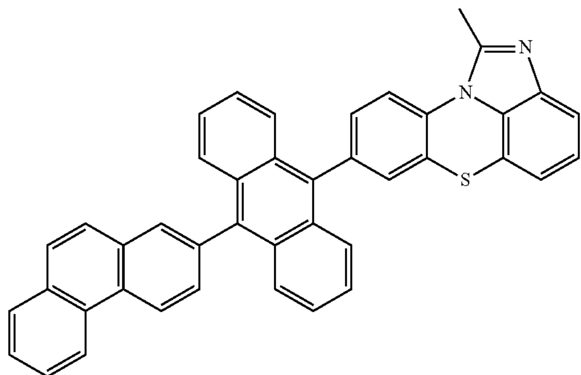
[Chemical Formula 2-2-9]
