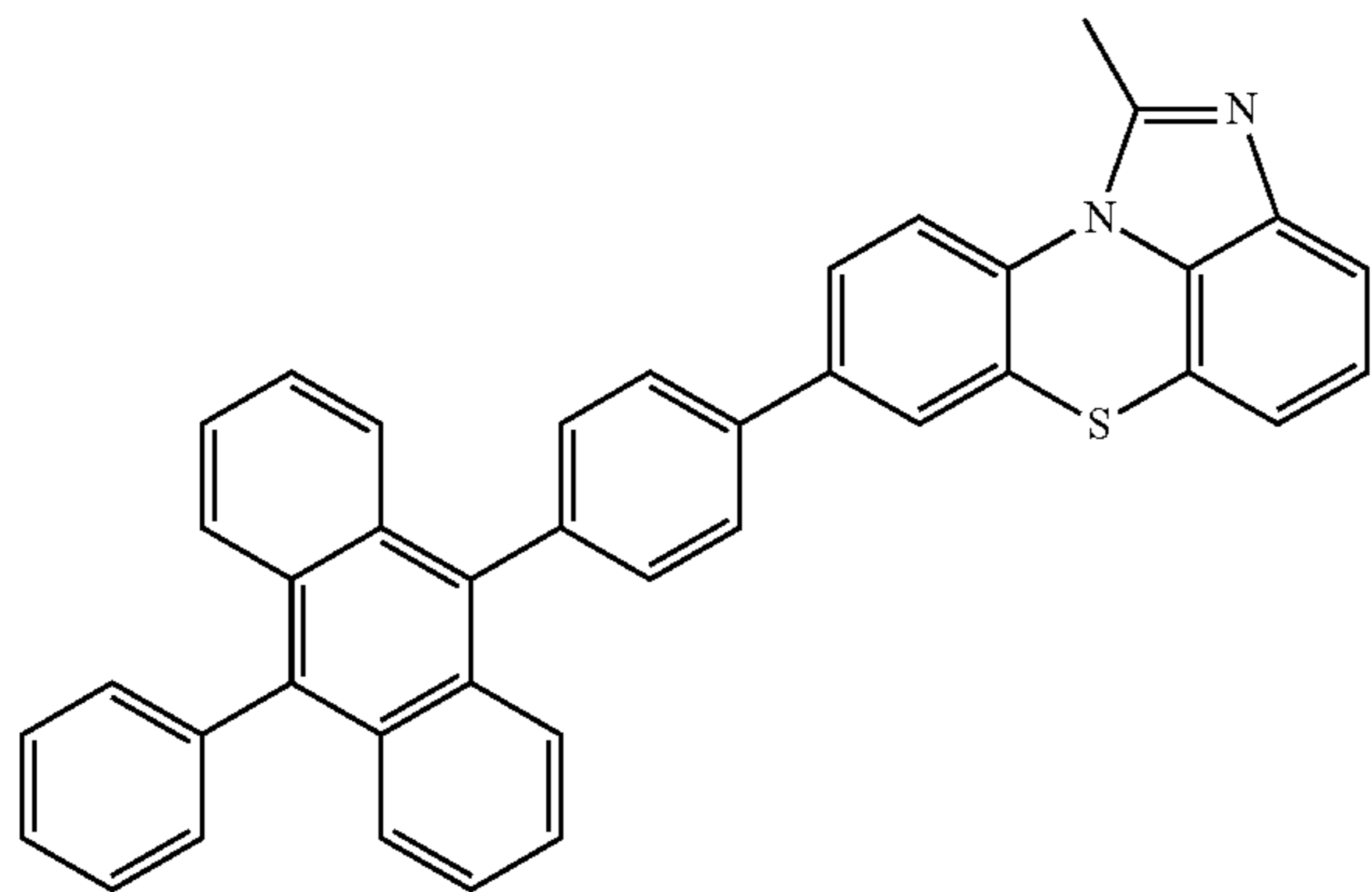
[Chemical Formula 2-2-17]
