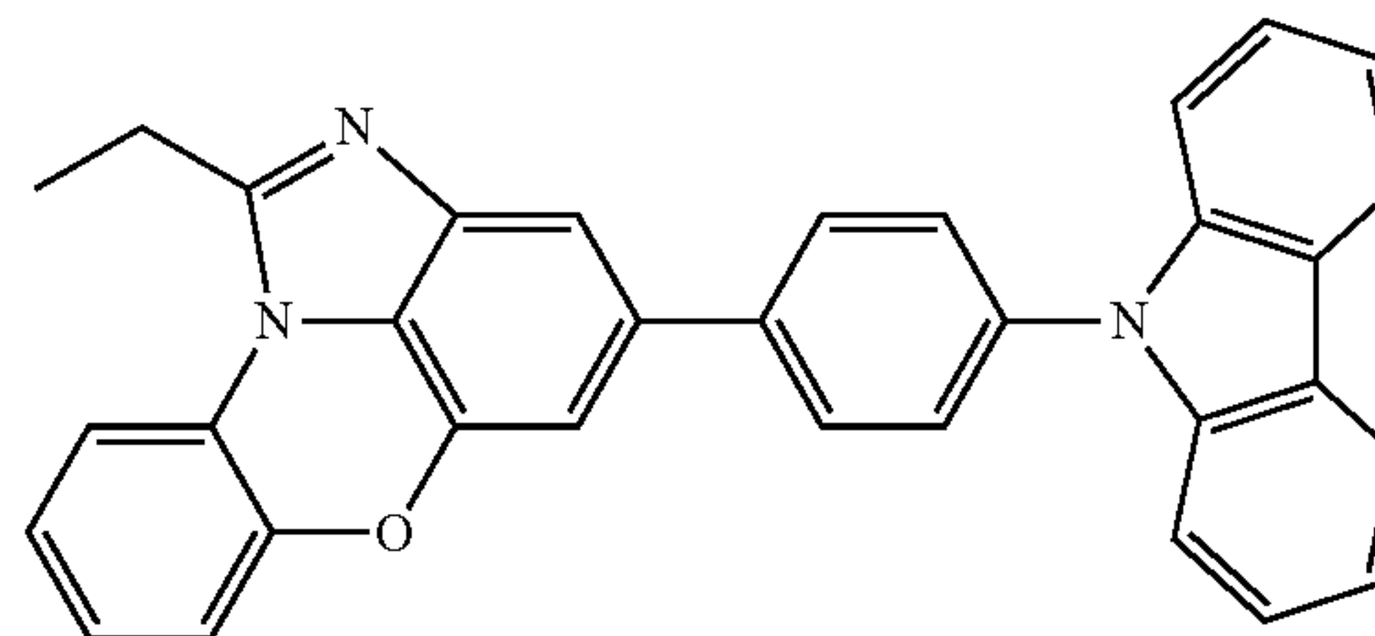
[Chemical Formula 1-10-7]
