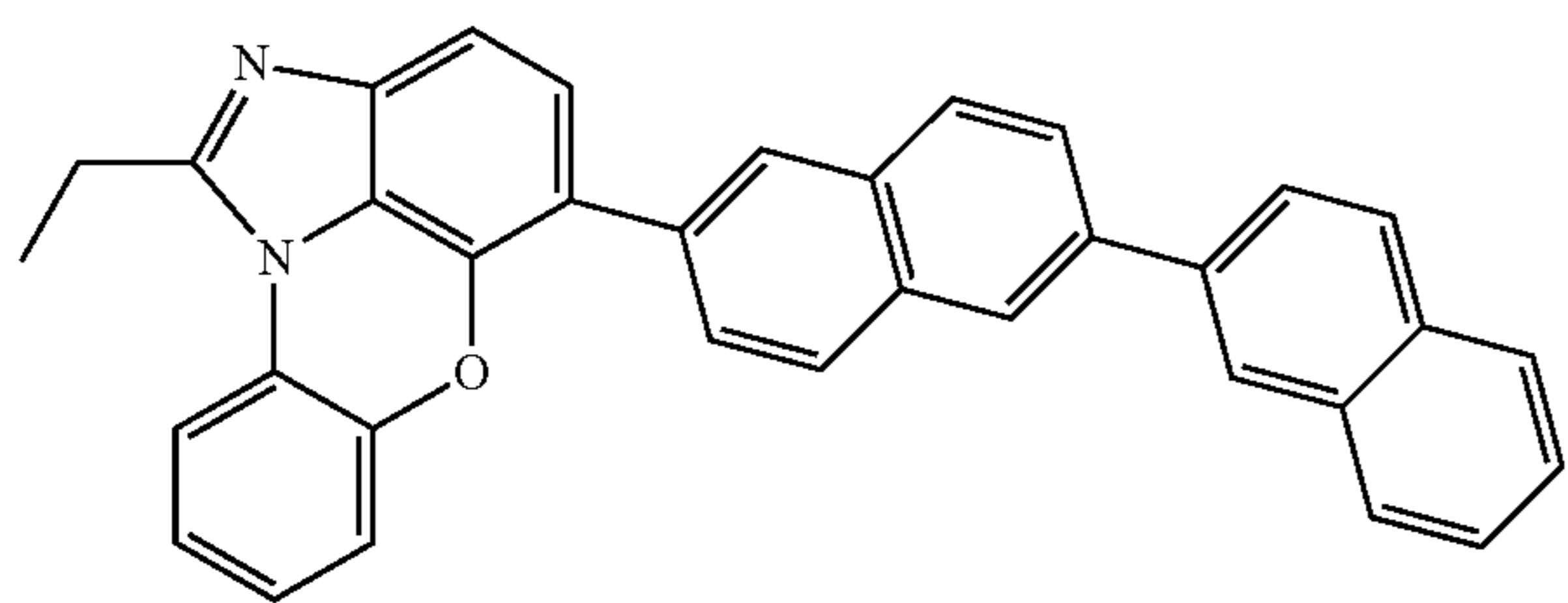
[Chemical Formula 1-9-8]
