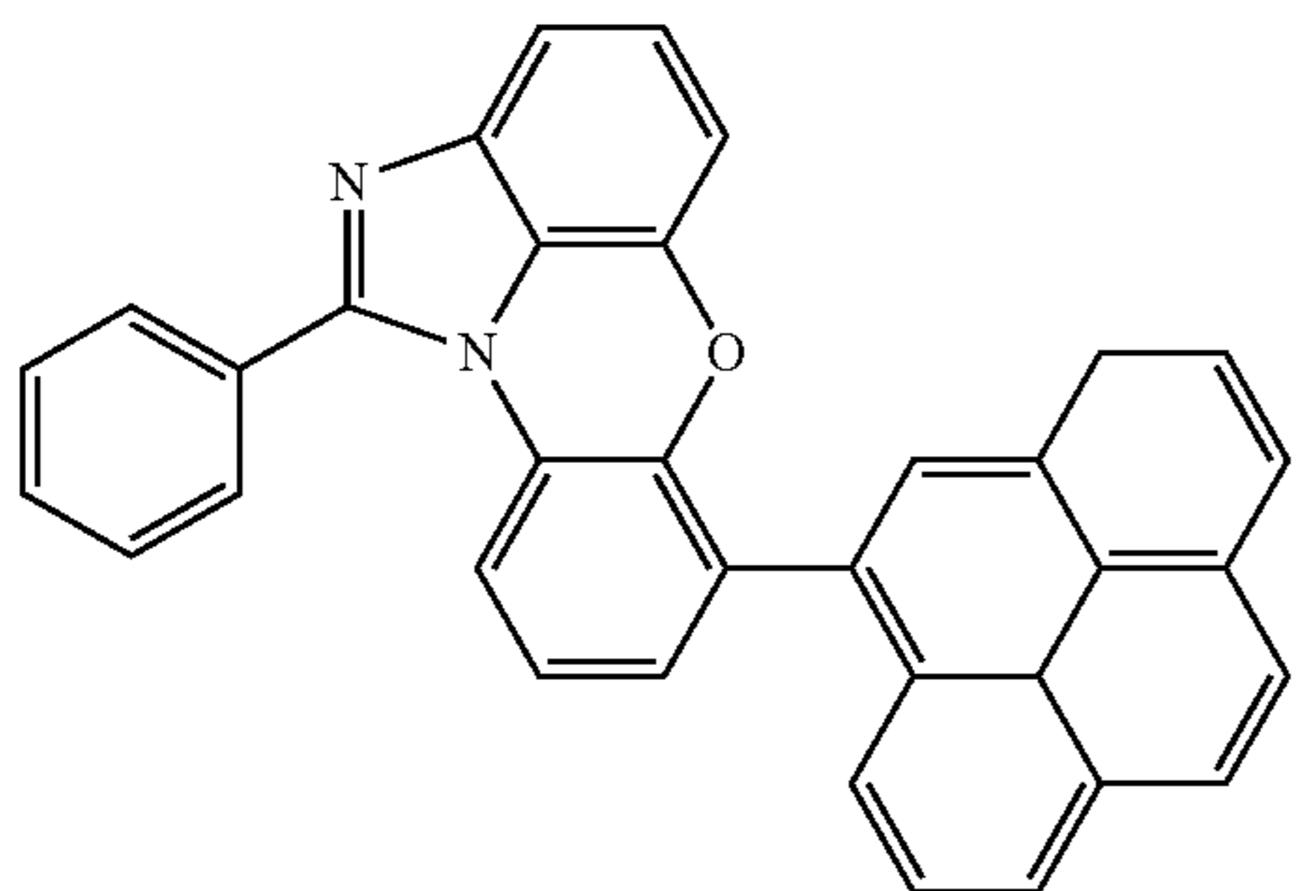
[Chemical Formula 1-6-29]
