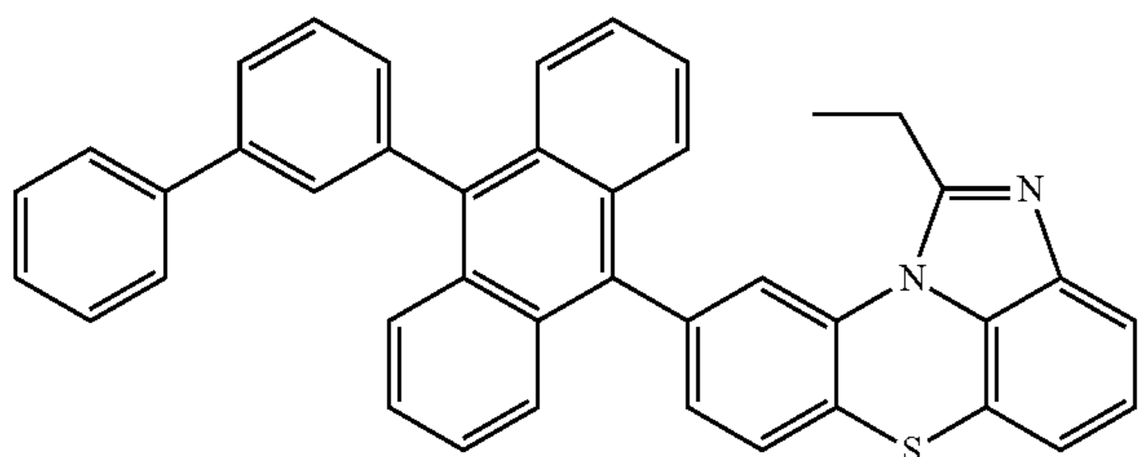
[Chemical Formula 2-3-6]
