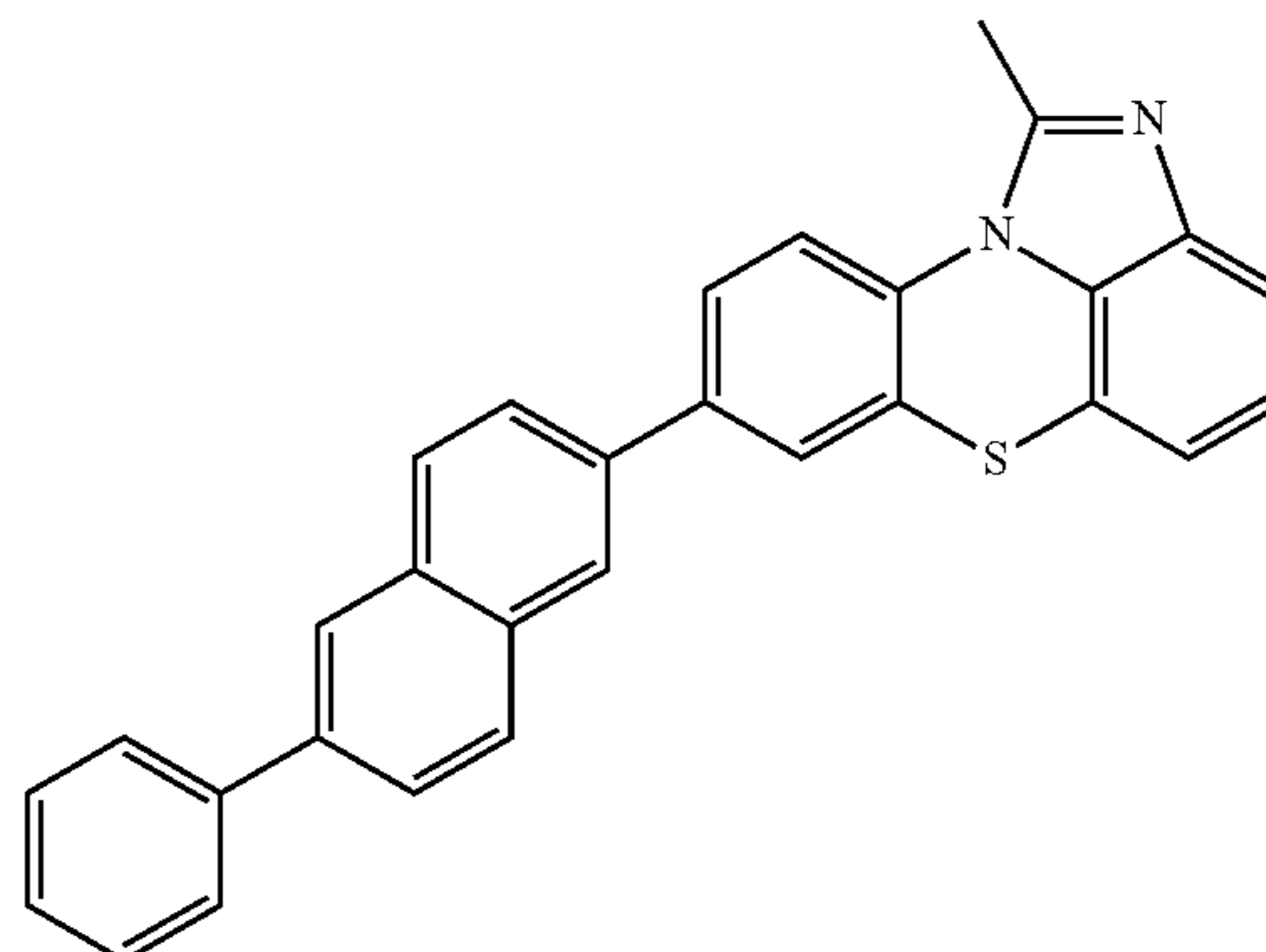
[Chemical Formula 2-2-27]
