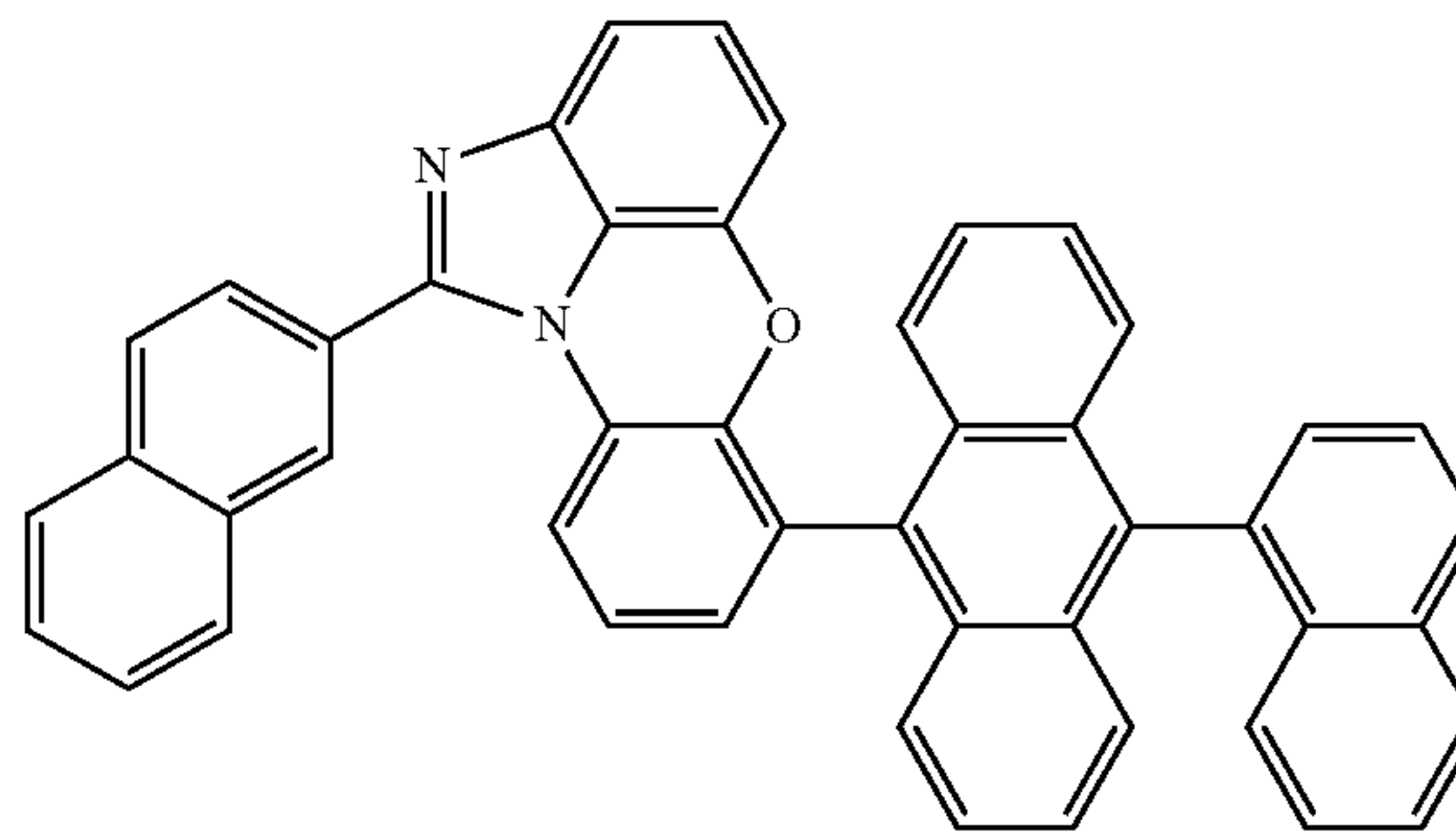
[Chemical Formula 1-6-3]
