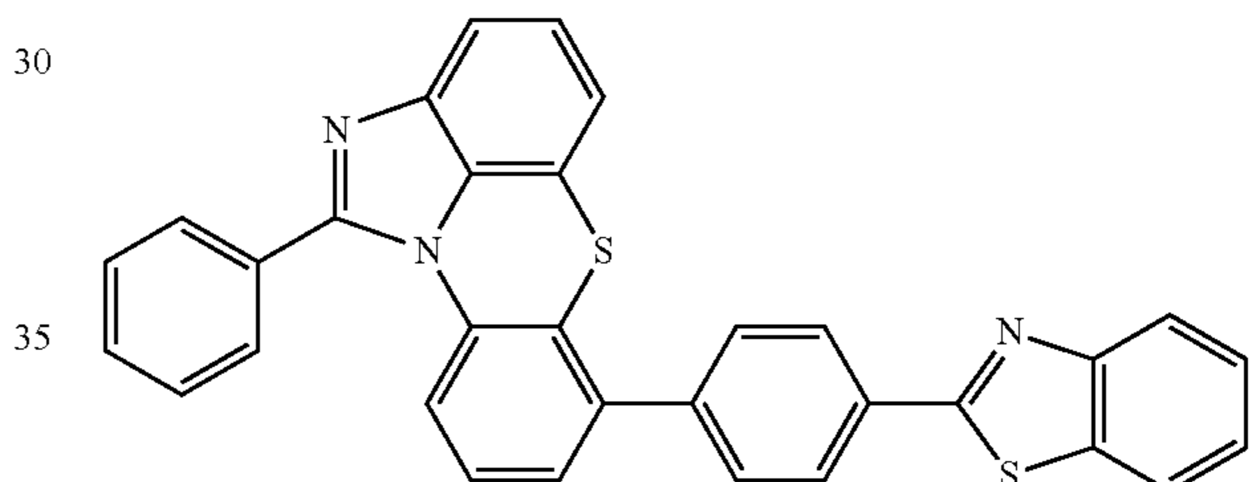
[Chemical Formula 2-2-47]
