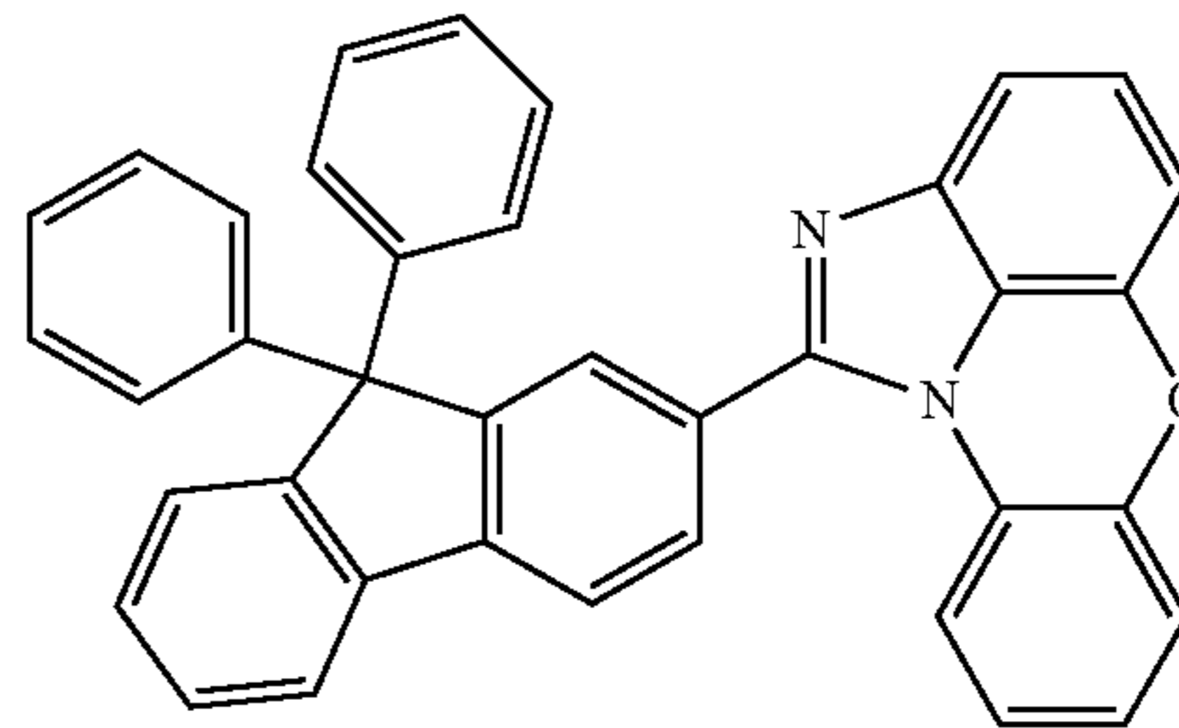
[Chemical Formula 1-1-43]
