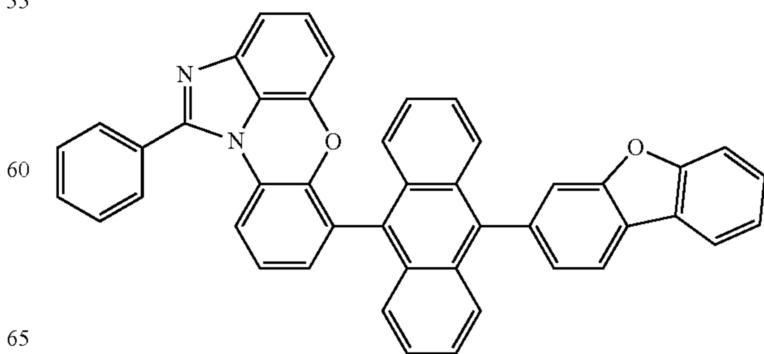
[Chemical Formula 1-6-13]
