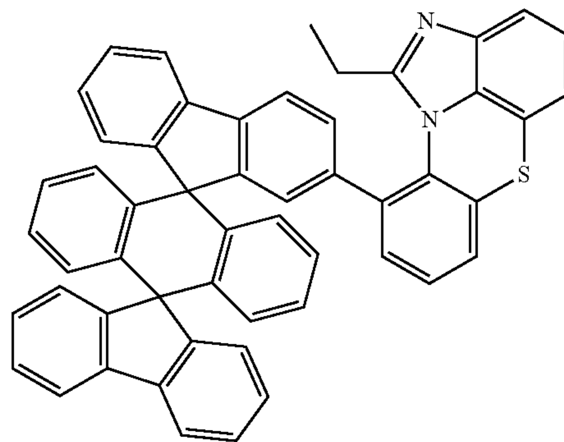
[Chemical Formula 2-3-36]
