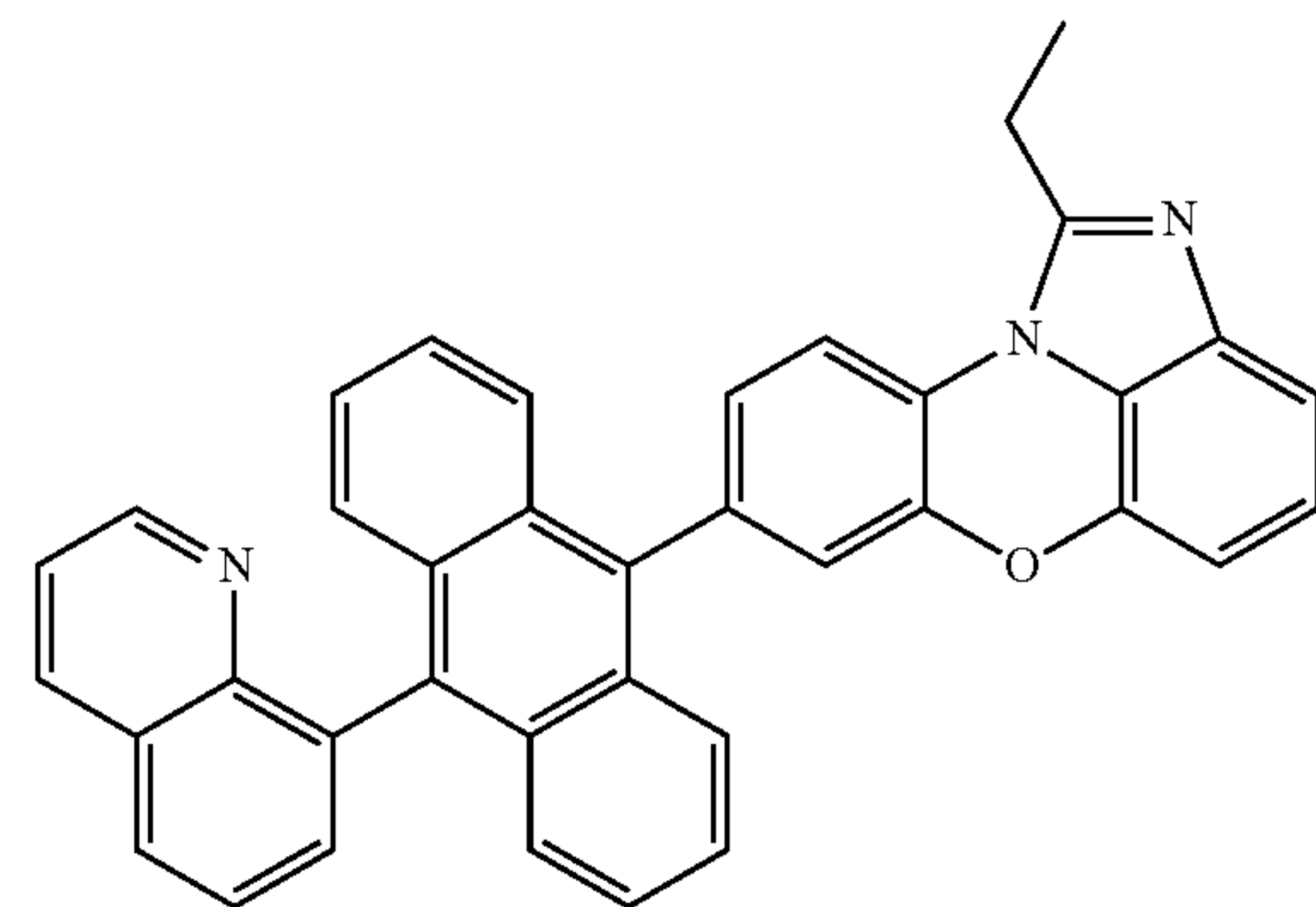
[Chemical Formula 1-3-11]
