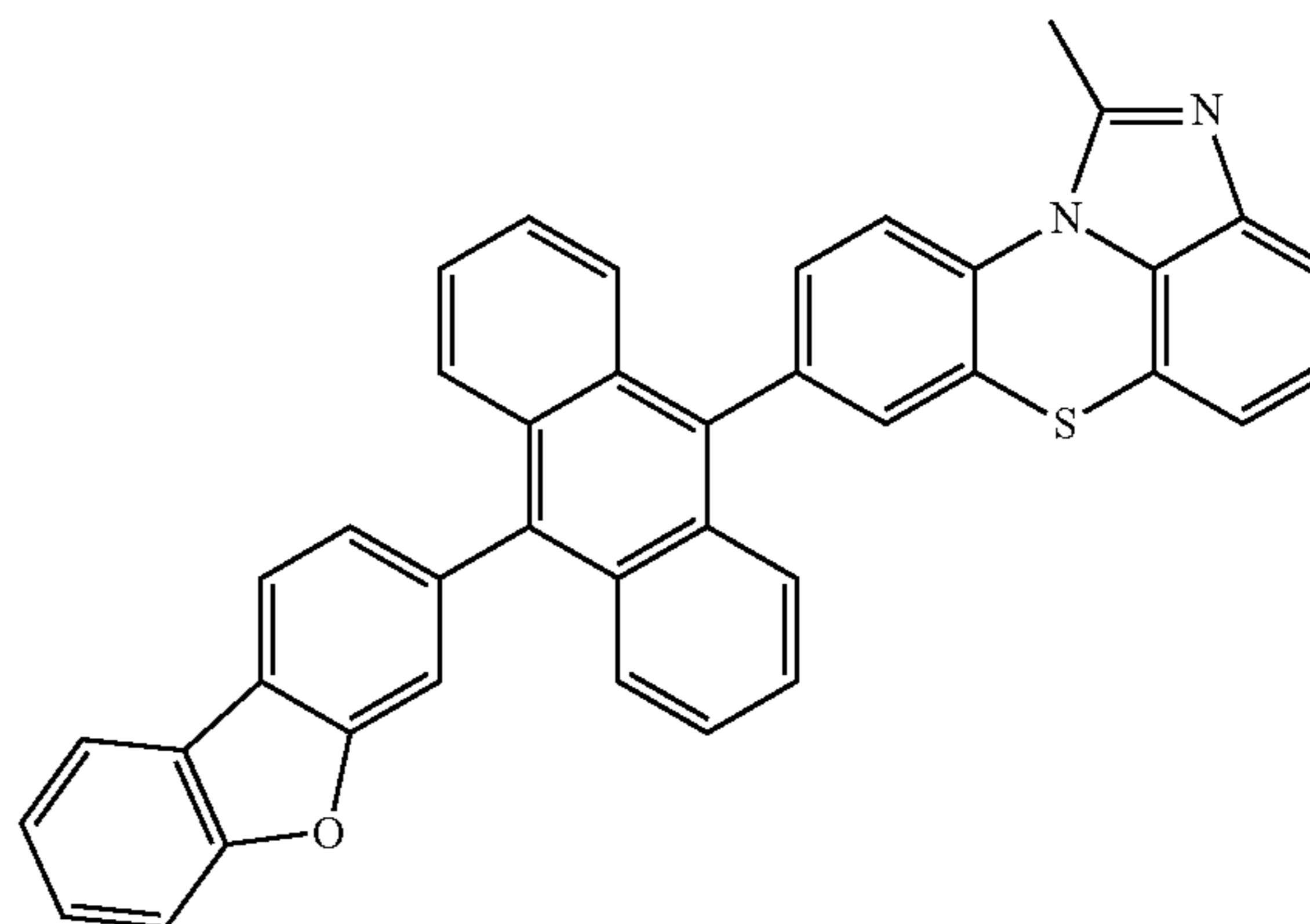
[Chemical Formula 2-2-14]
