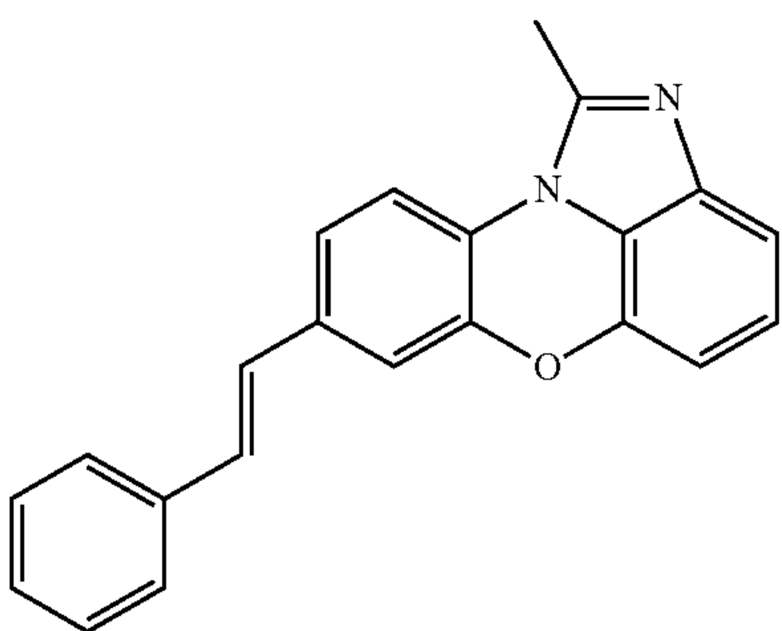
[Chemical Formula 1-2-54]
