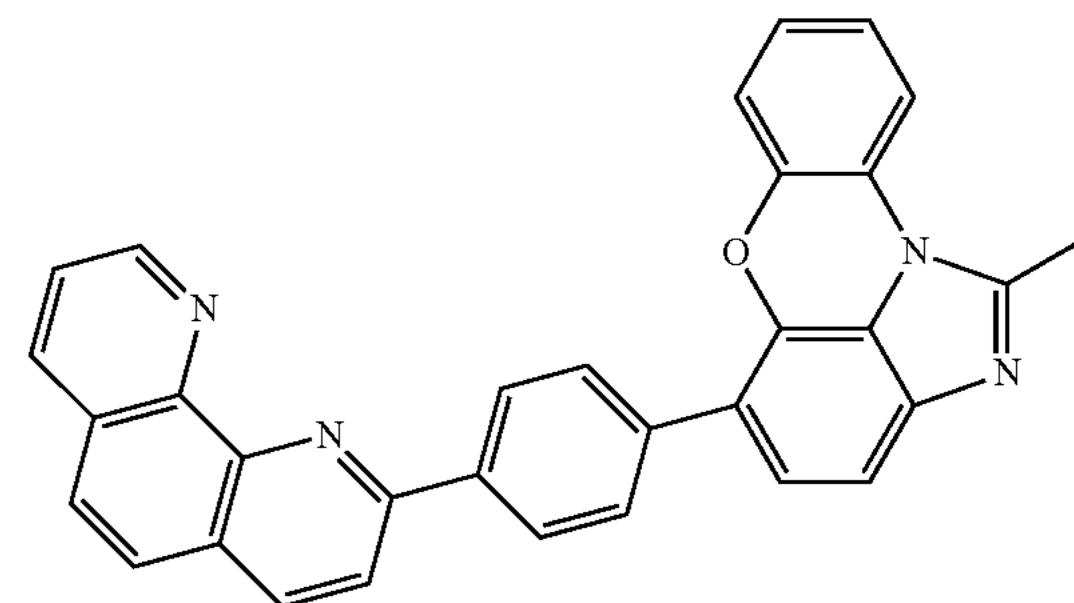
[Chemical Formula 1-9-11]
