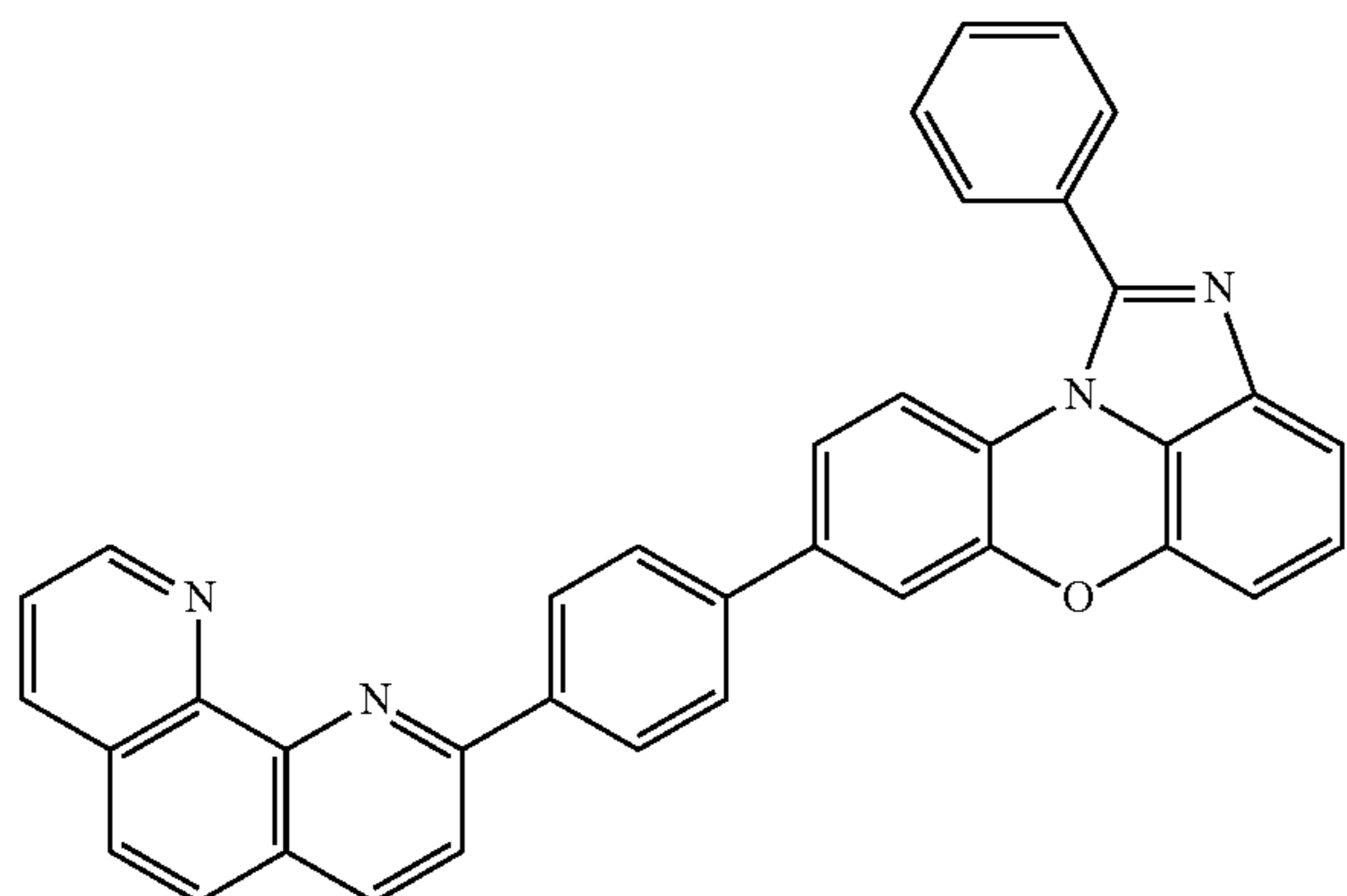
[Chemical Formula 1-4-48]
