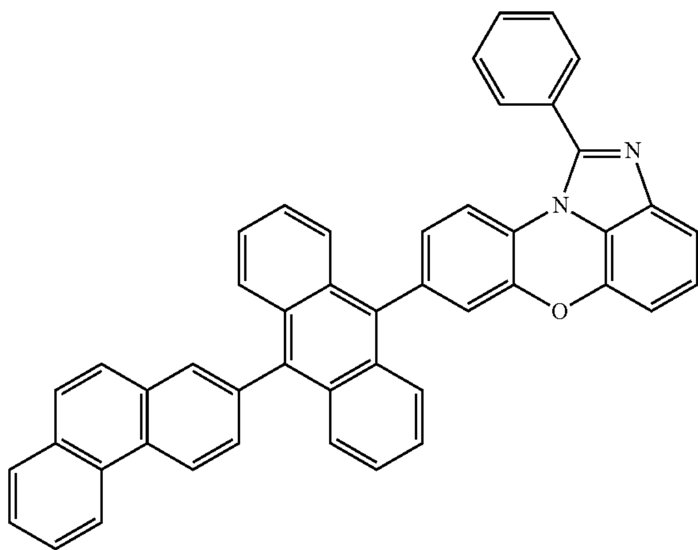
[Chemical Formula 1-4-9]
