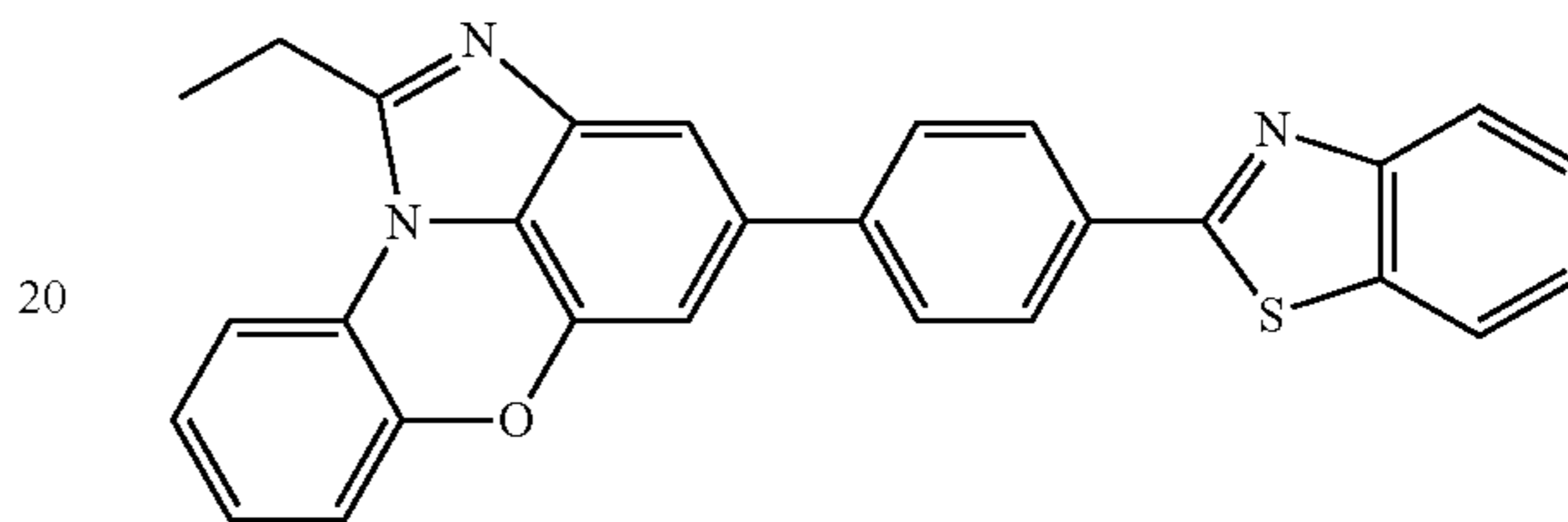
[Chemical Formula 1-10-10]
