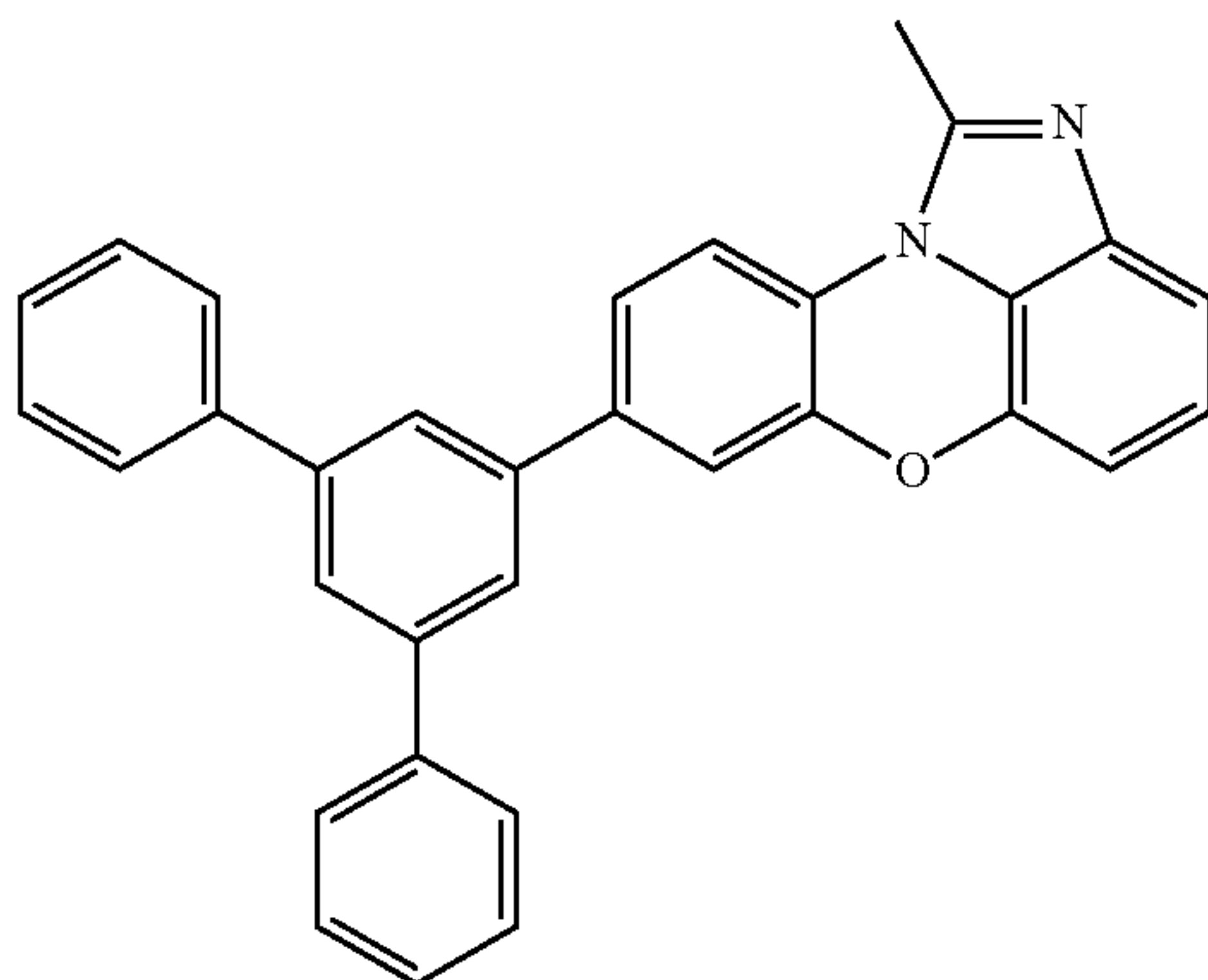
[Chemical Formula 1-2-41]
