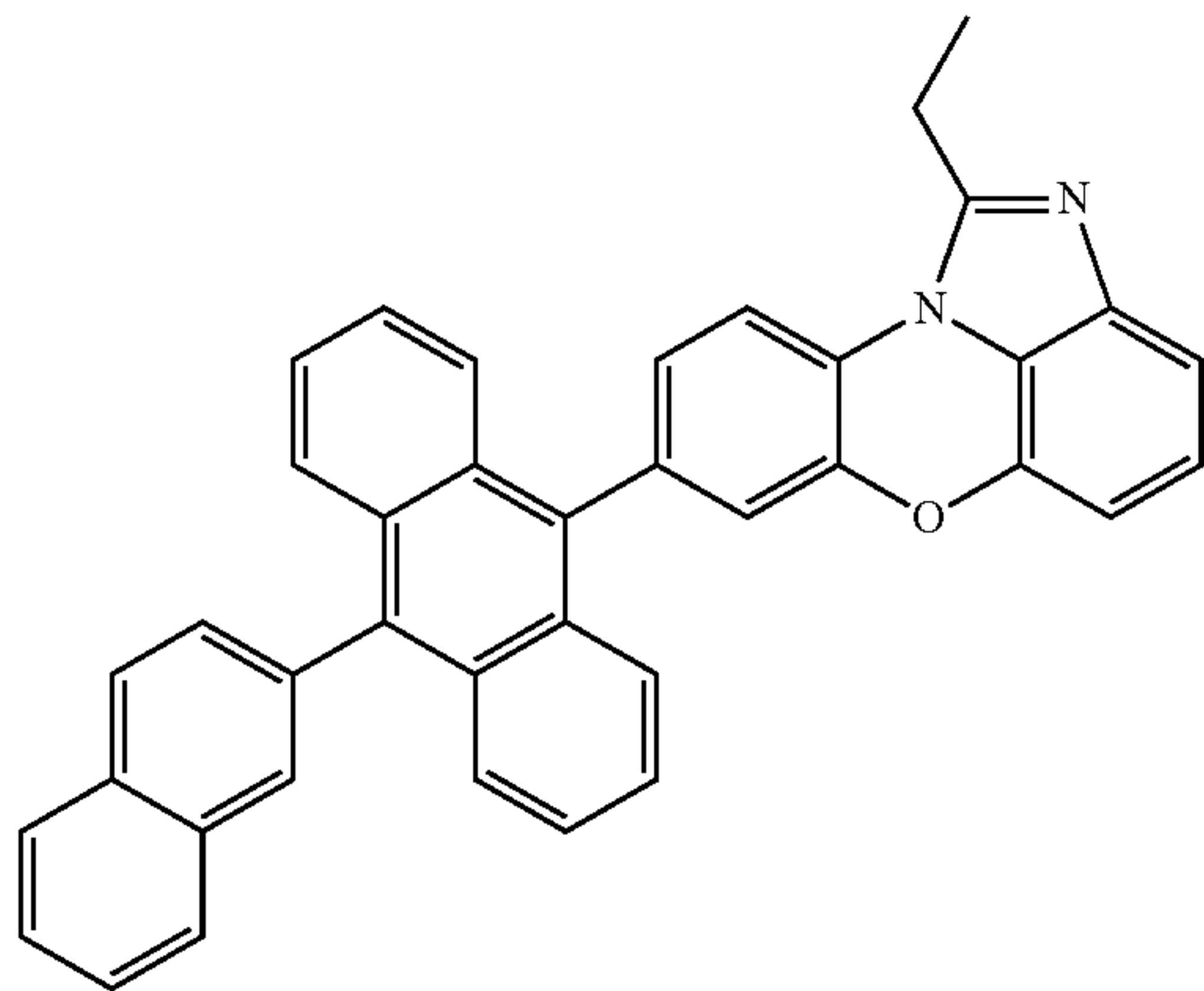
[Chemical Formula 1-3-2]
