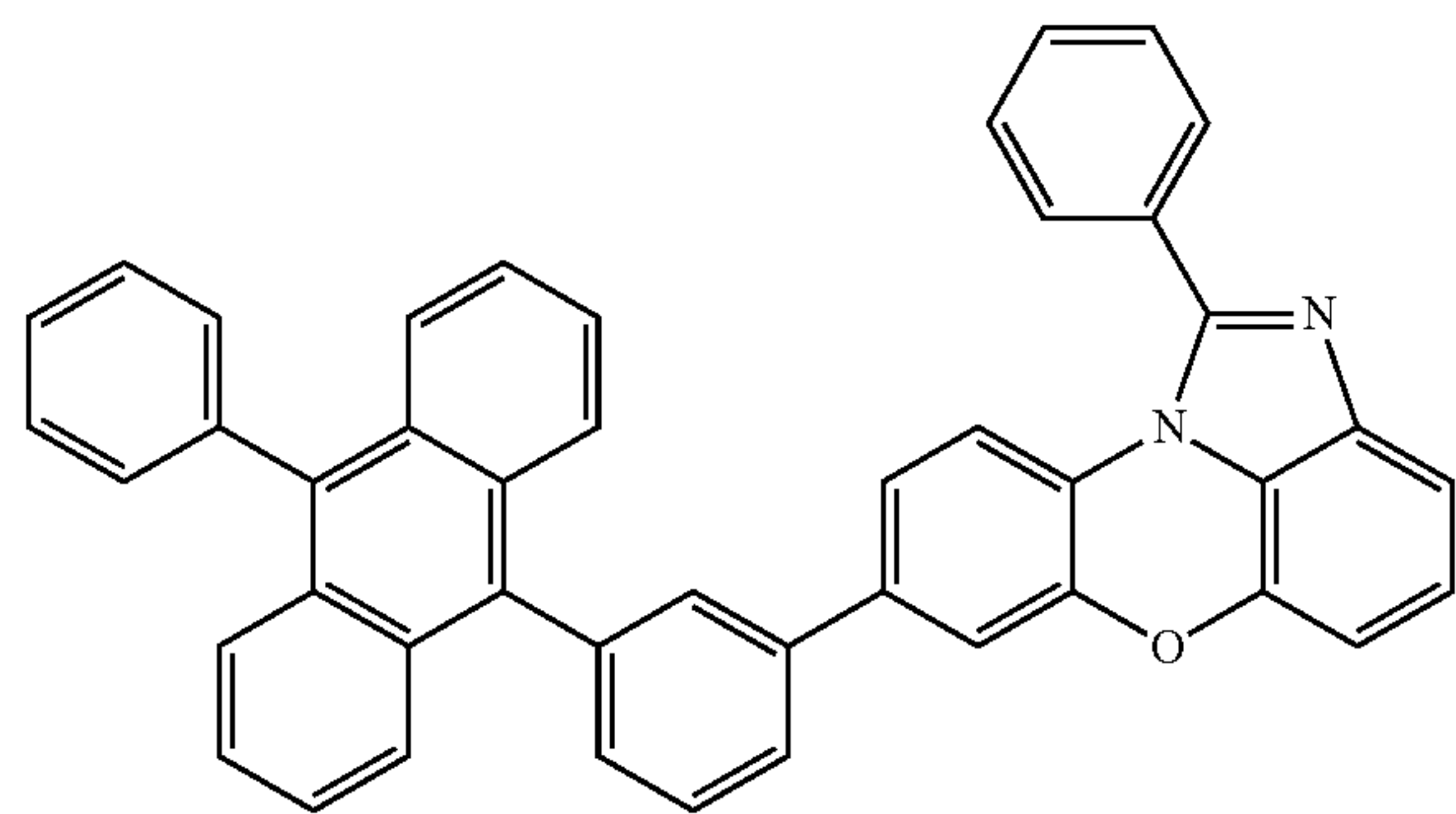
[Chemical Formula 1-4-18]
