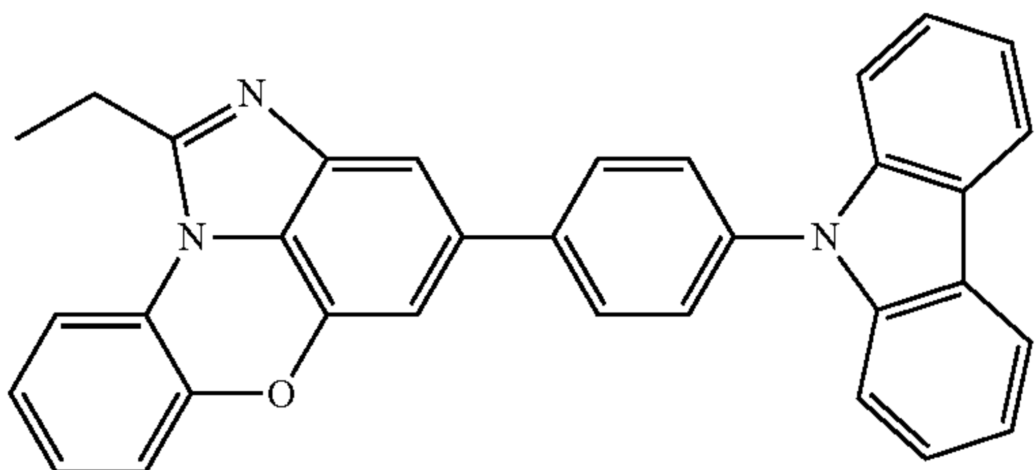
[Chemical Formula 1-10-6]
