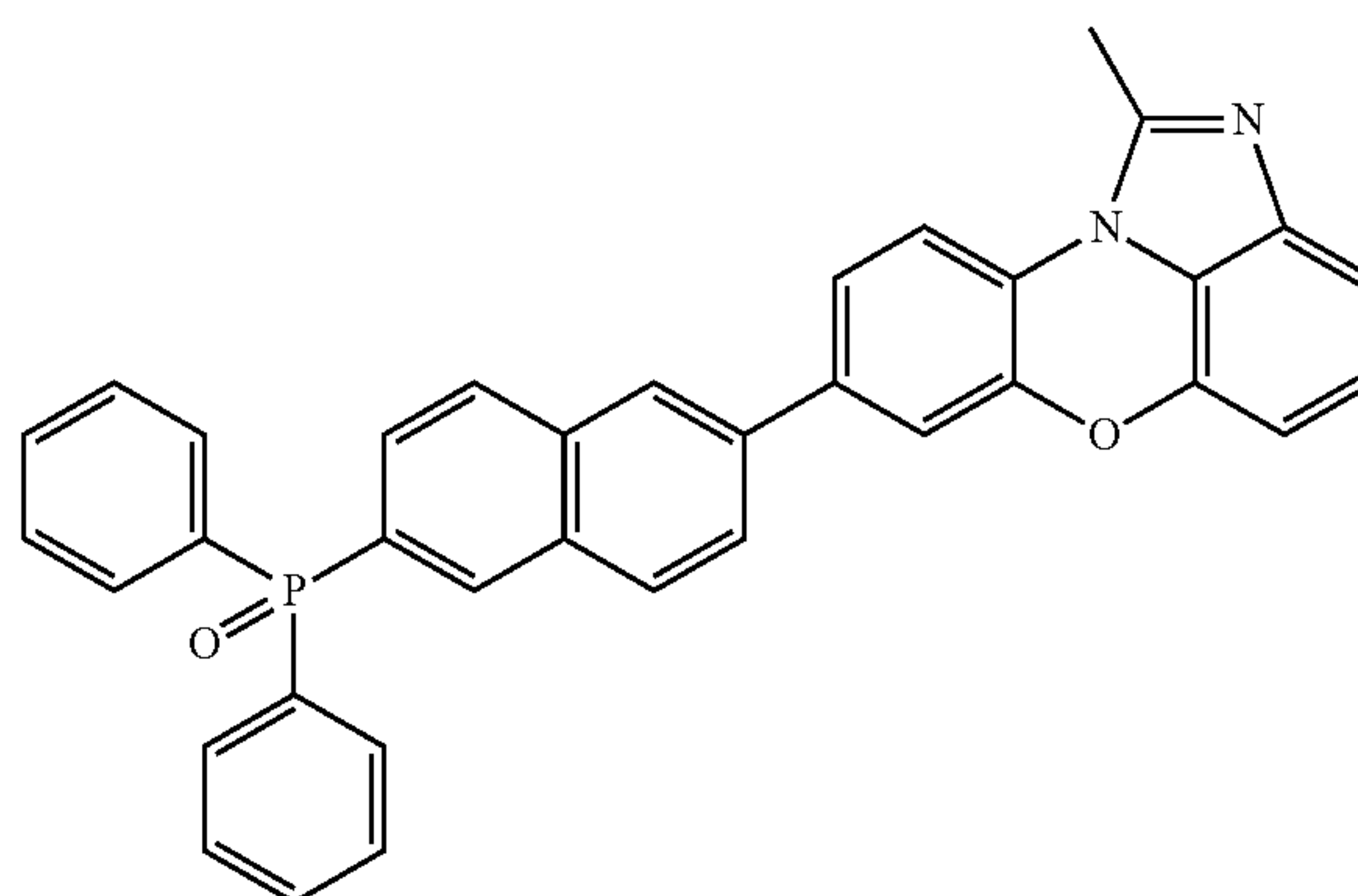
[Chemical Formula 1-5-2]
