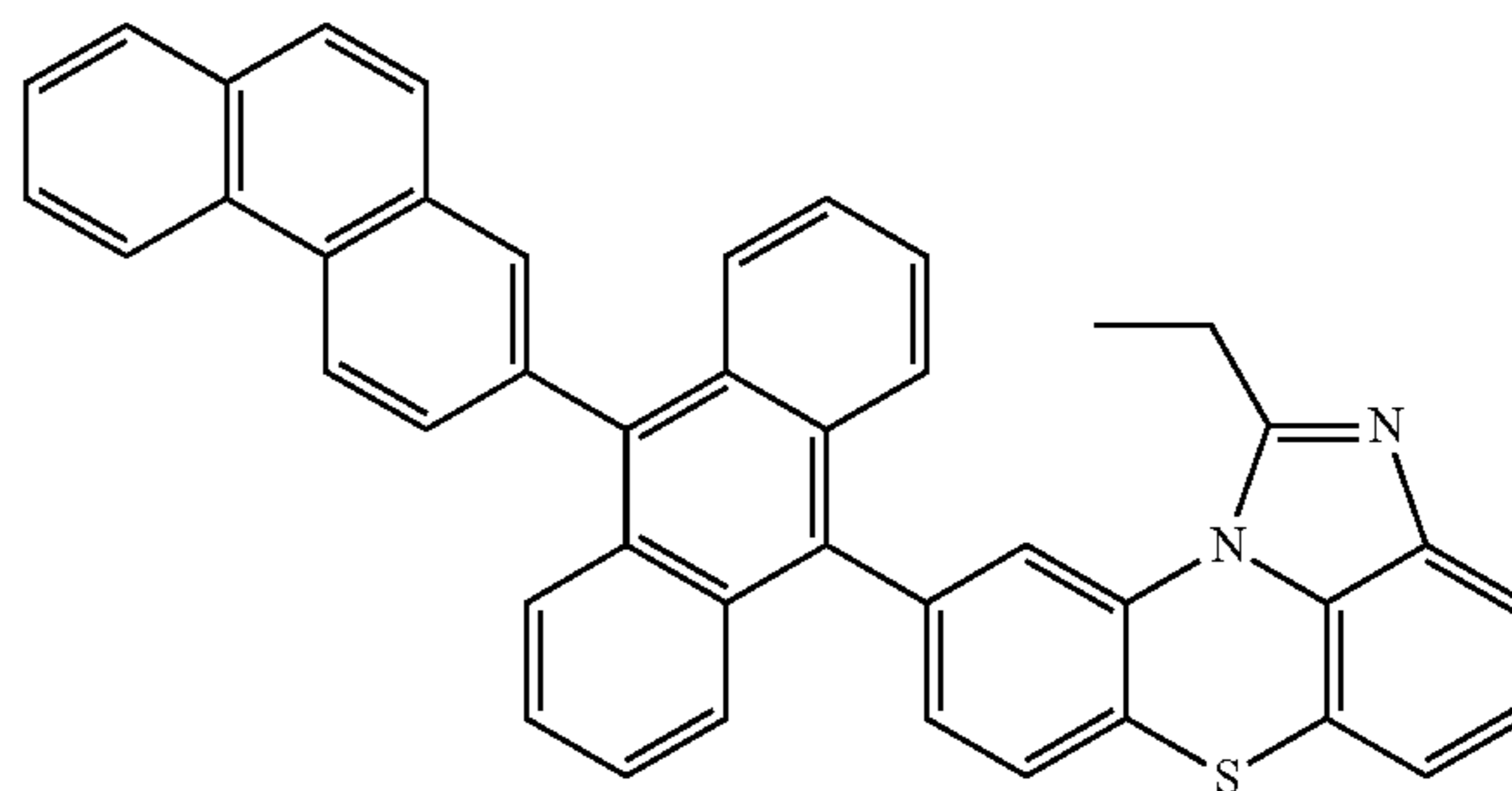
[Chemical Formula 2-3-9]
