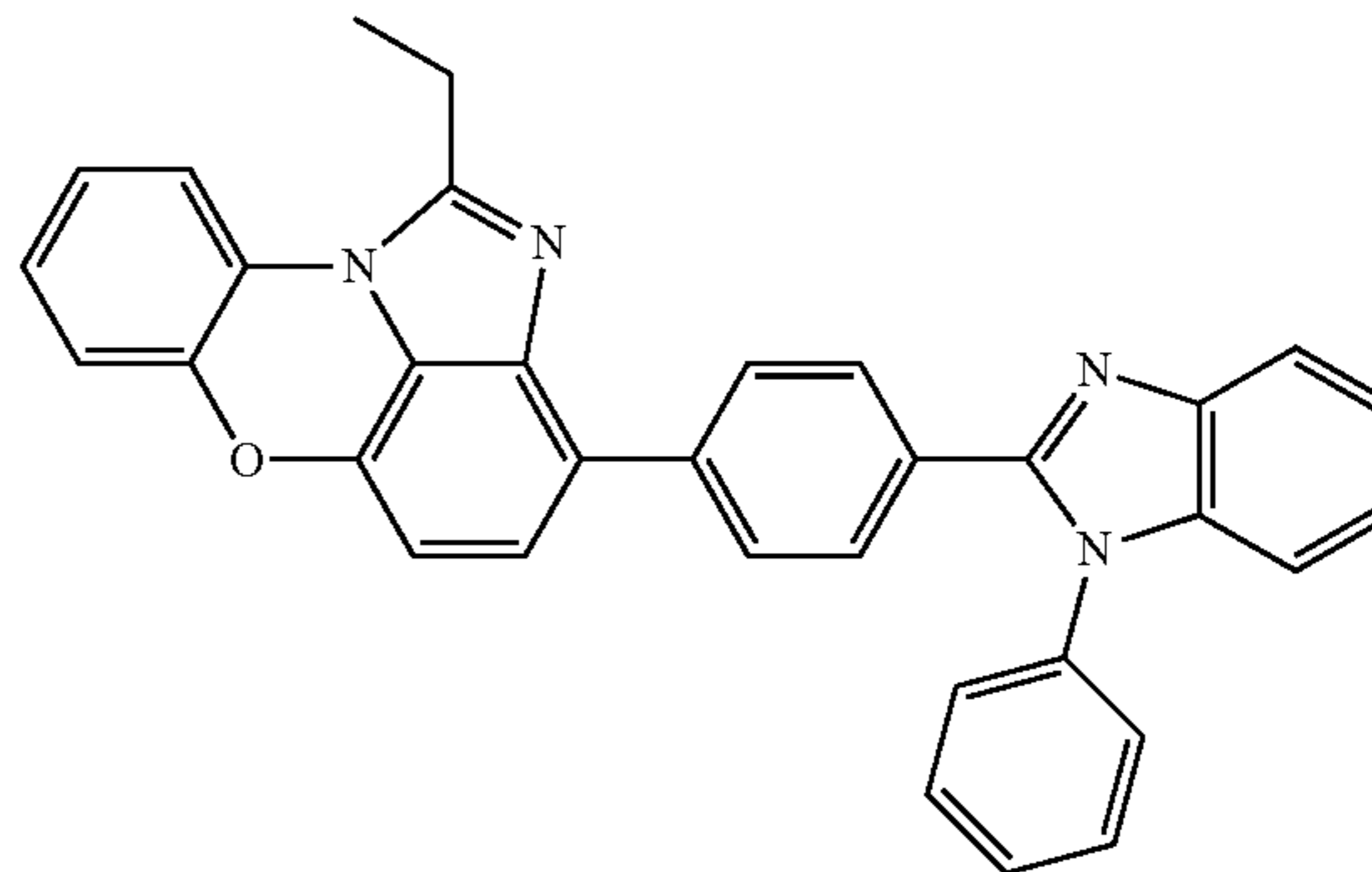
[Chemical Formula 1-11-10]
