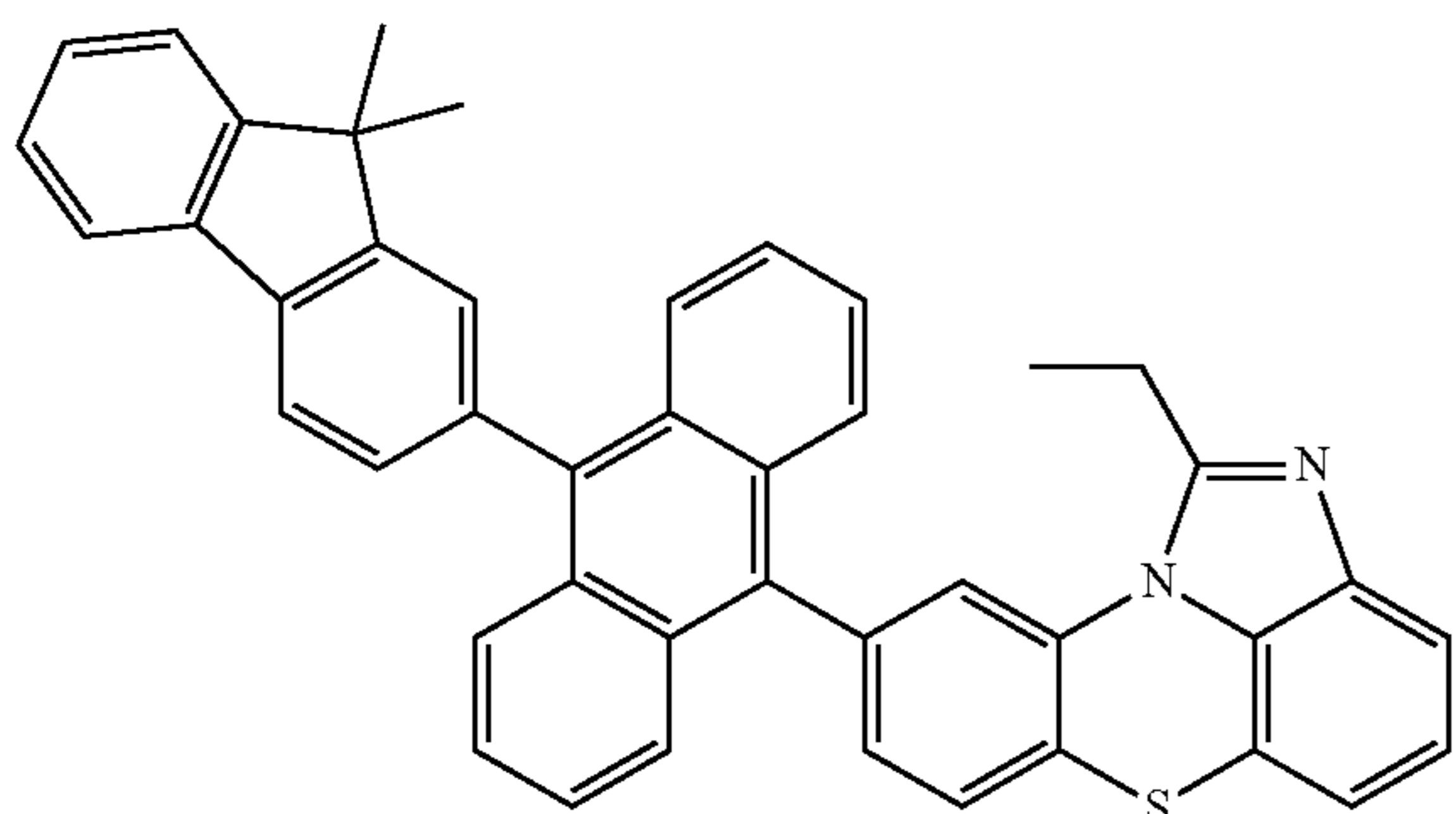
[Chemical Formula 2-3-5]
