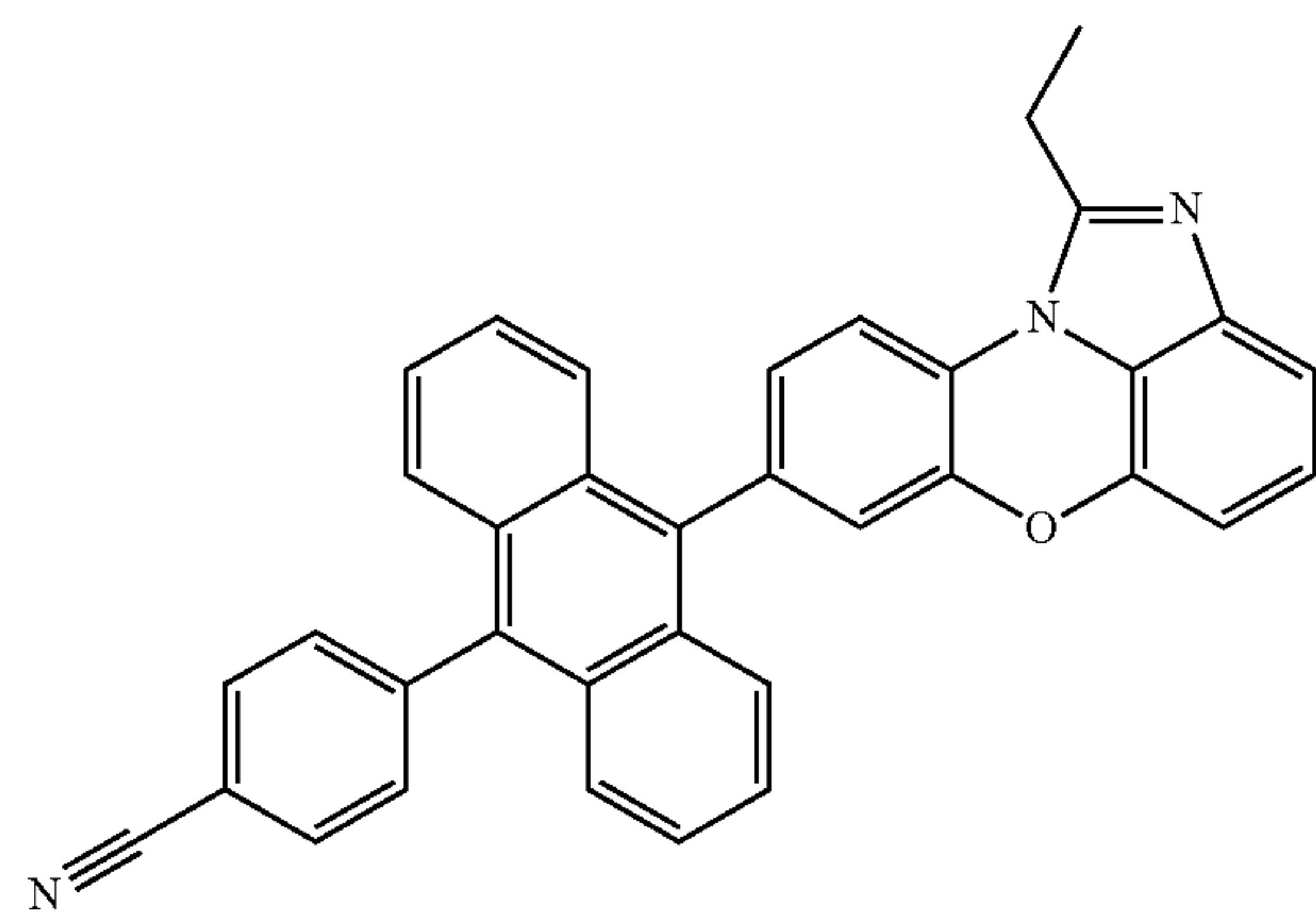
[Chemical Formula 1-3-12]
