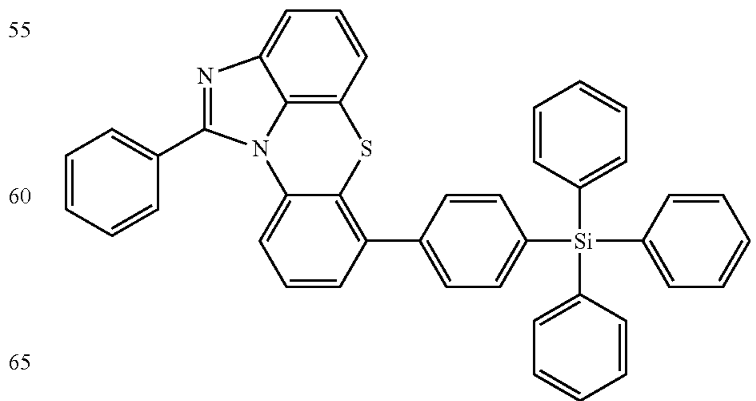
[Chemical Formula 2-2-48]
