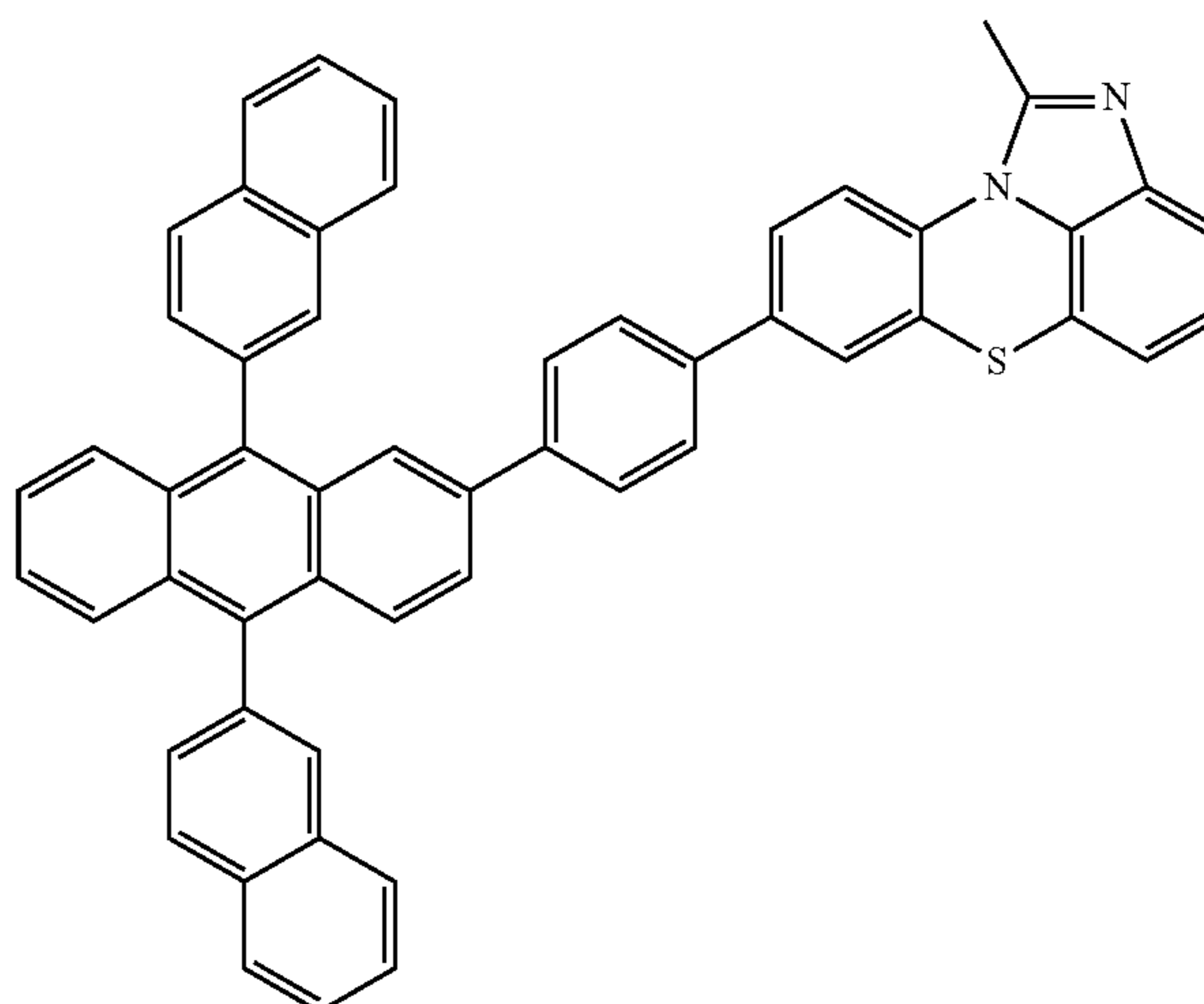
[Chemical Formula 2-2-26]
