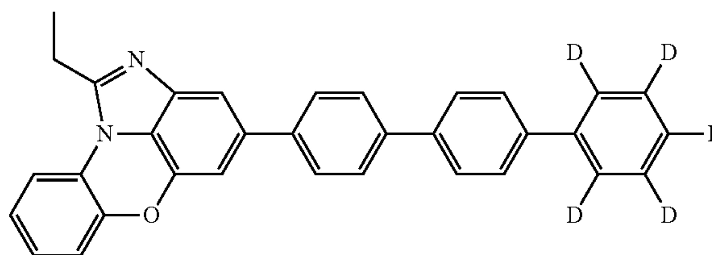
[Chemical Formula 1-10-16]
