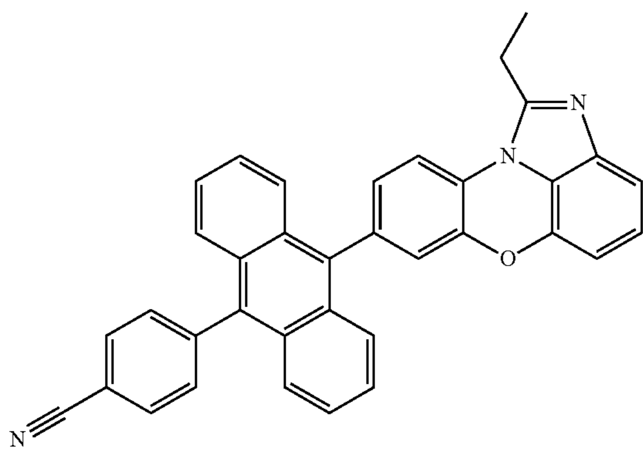
[Chemical Formula 1-3-12]
