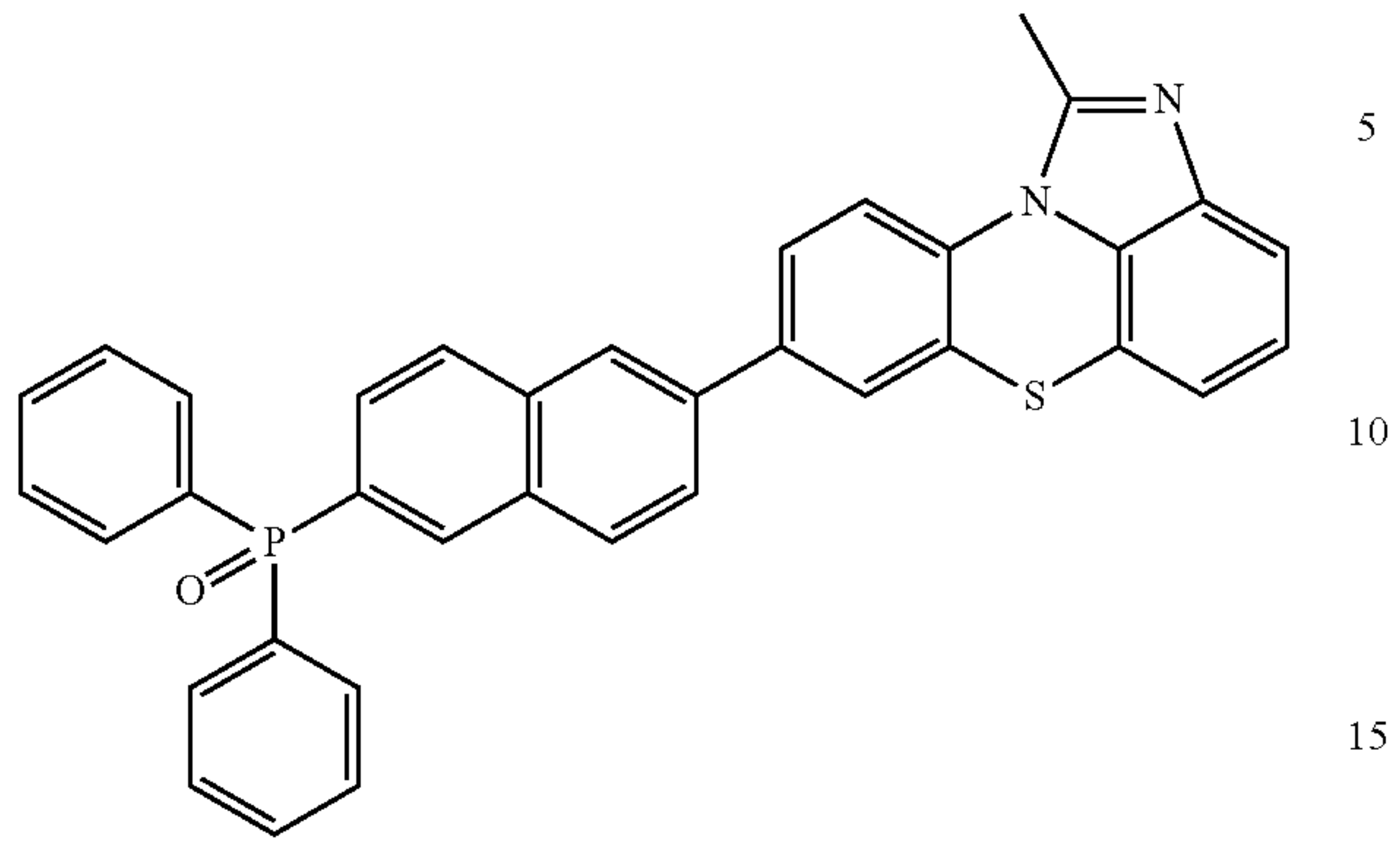
[Chemical Formula 2-4-3]
