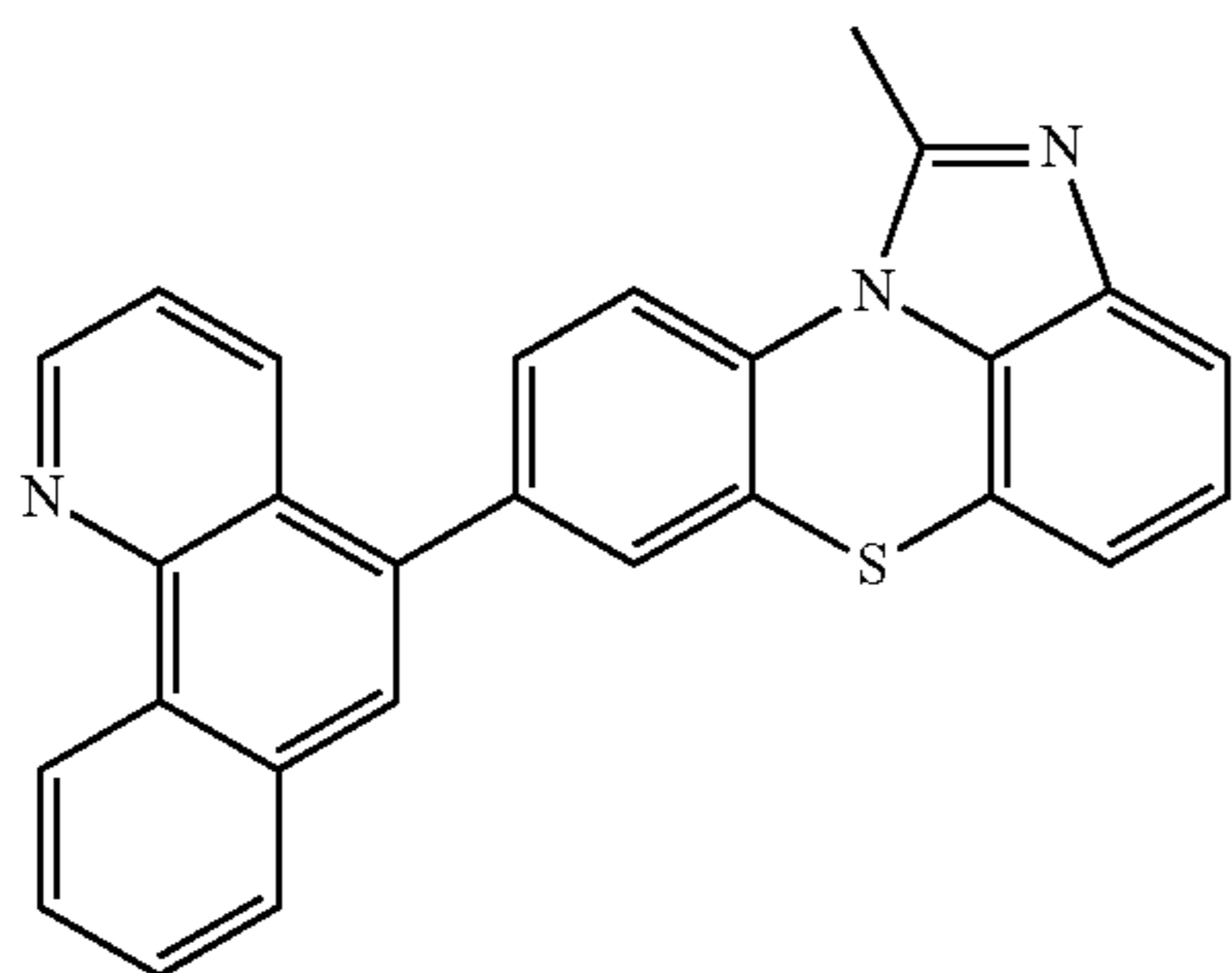
[Chemical Formula 2-2-33]
