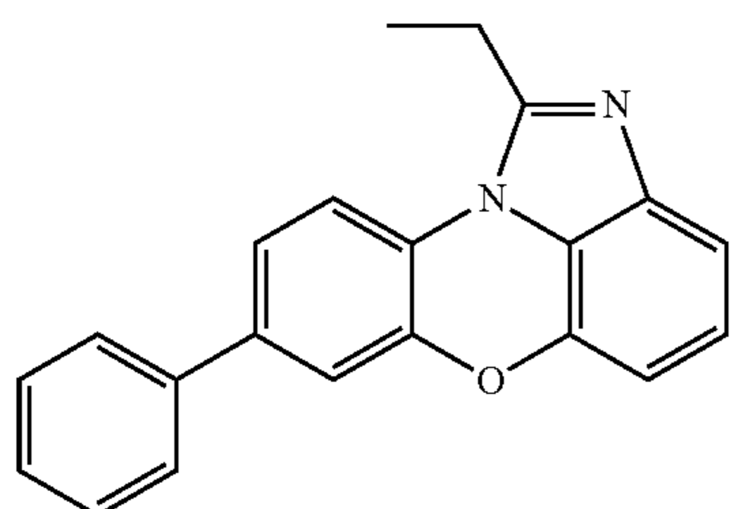
[Chemical Formula 1-3-38]
