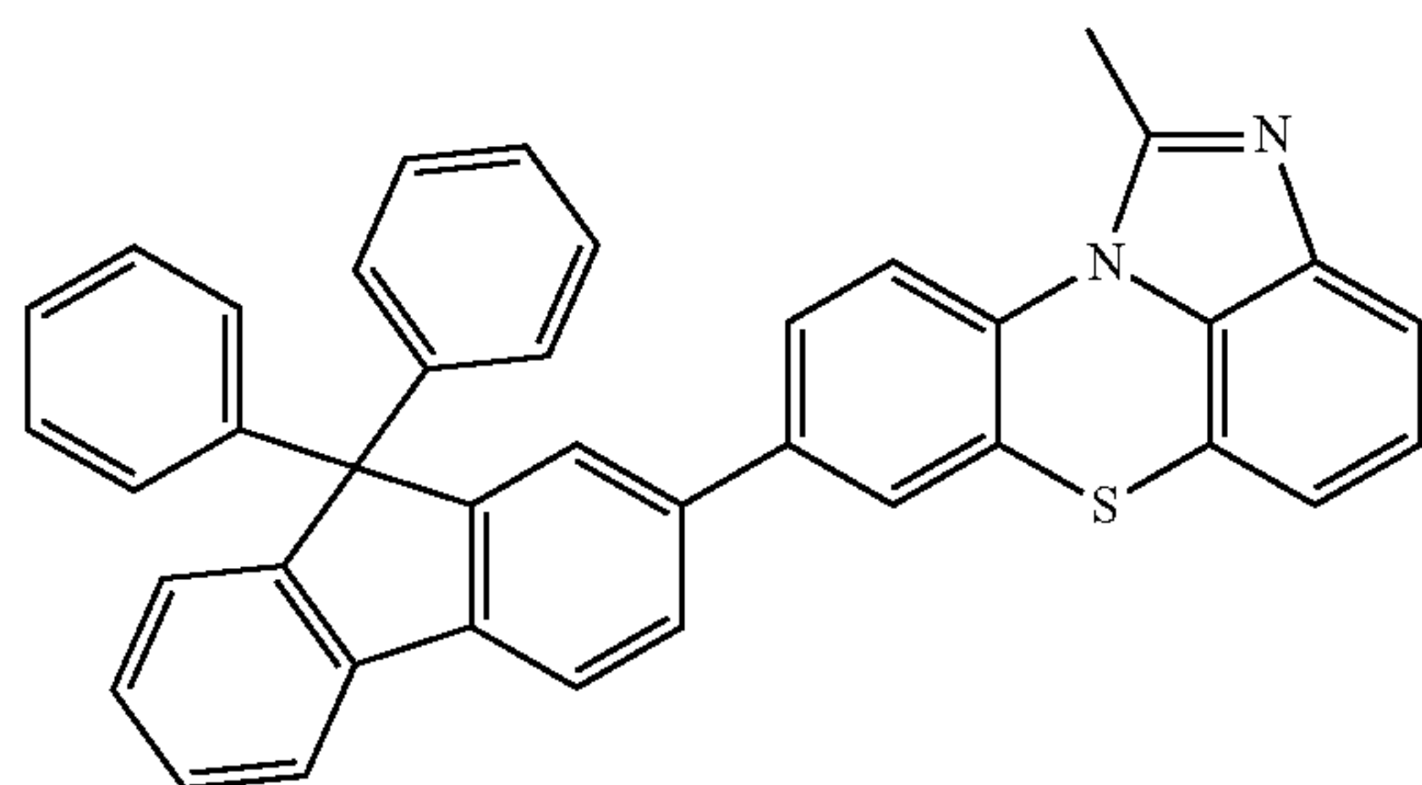
[Chemical Formula 2-2-35]
