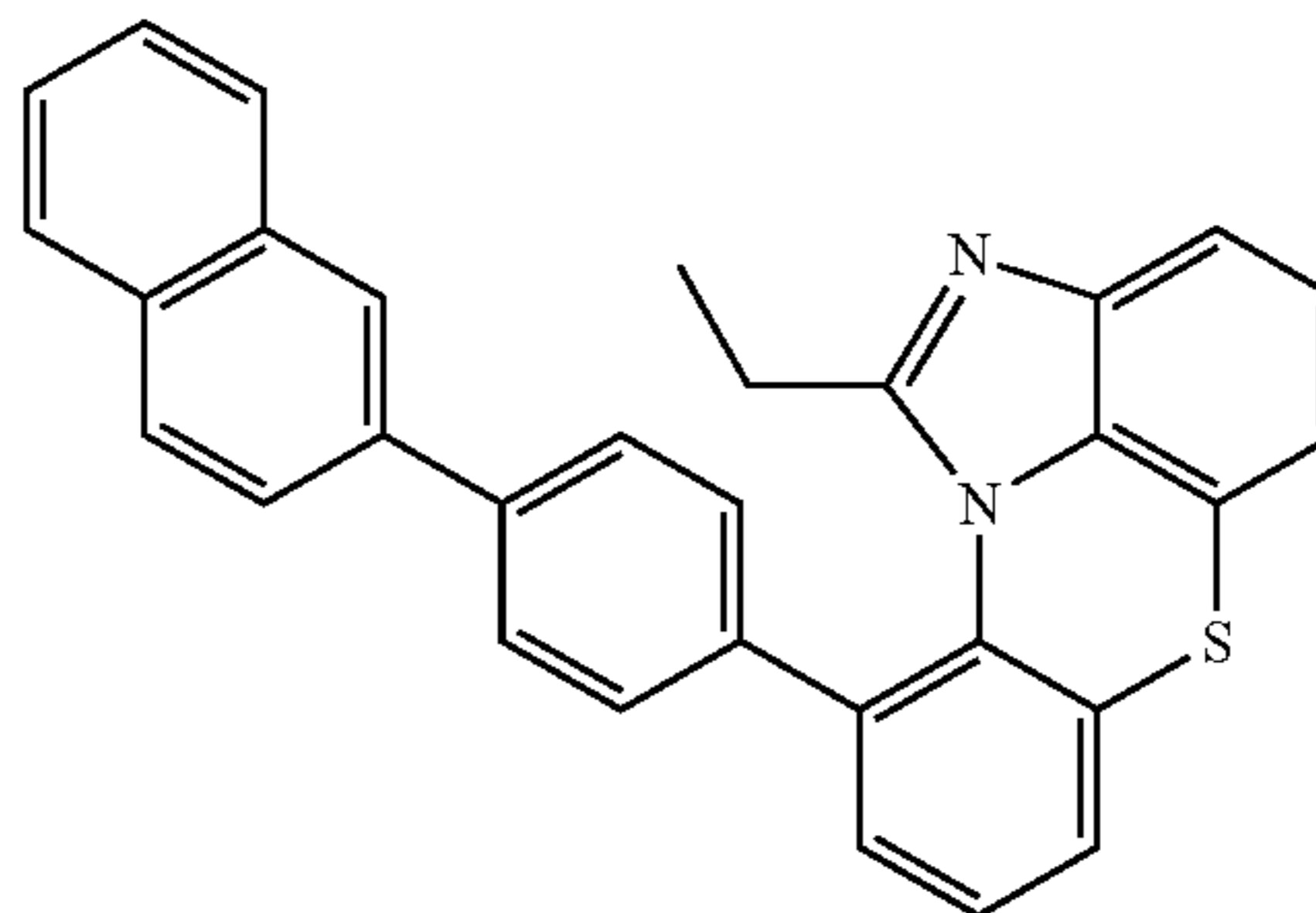
[Chemical Formula 2-3-26]
