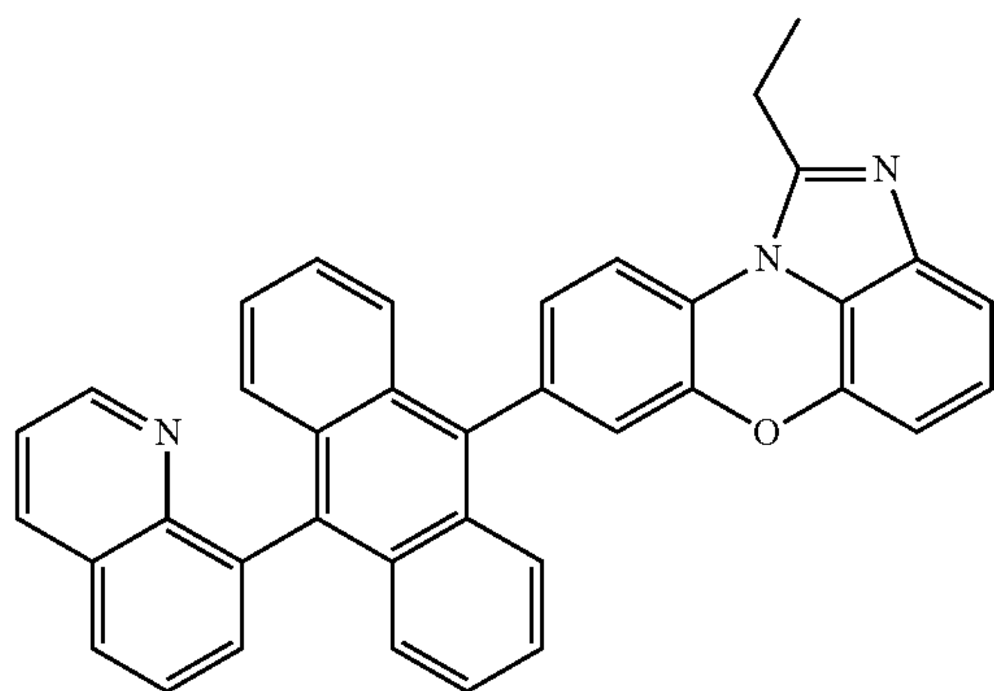
[Chemical Formula 1-3-12]
