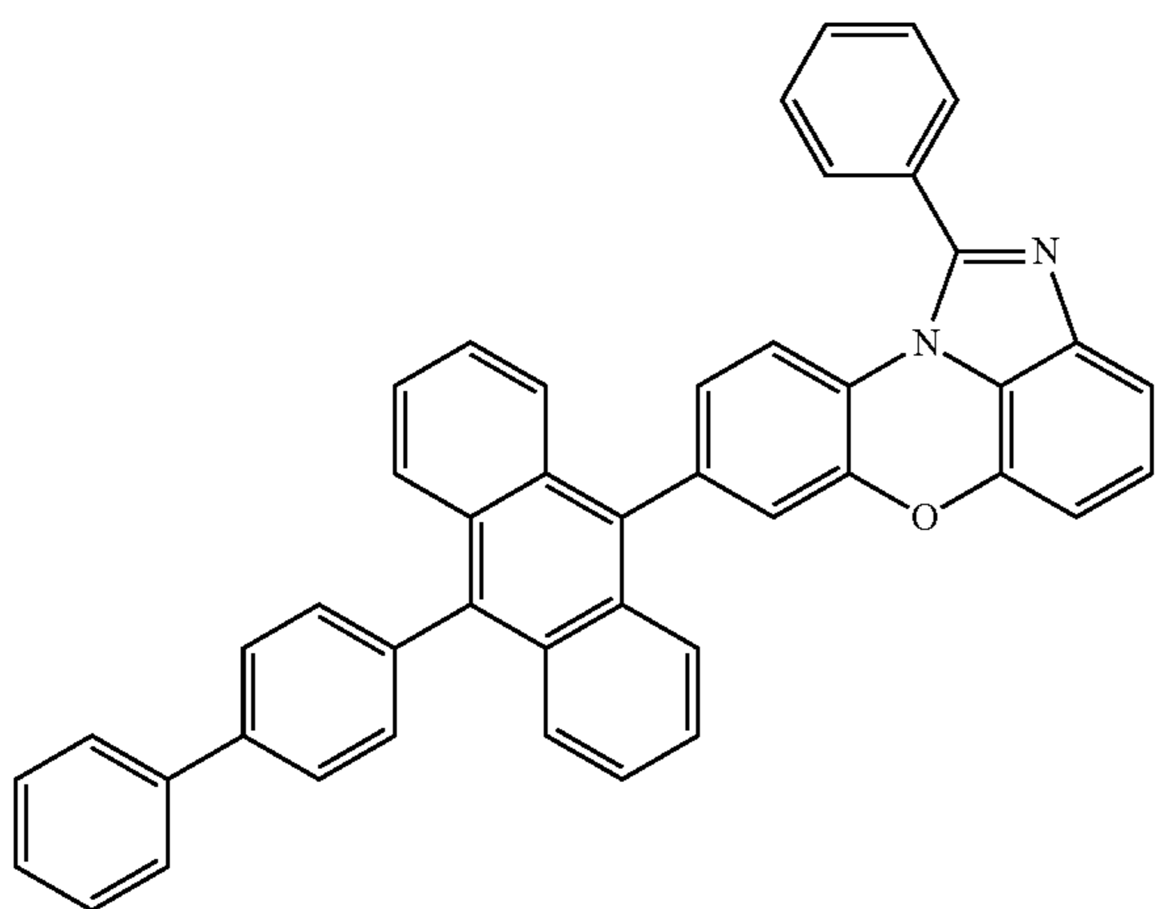
[Chemical Formula 1-4-4]
