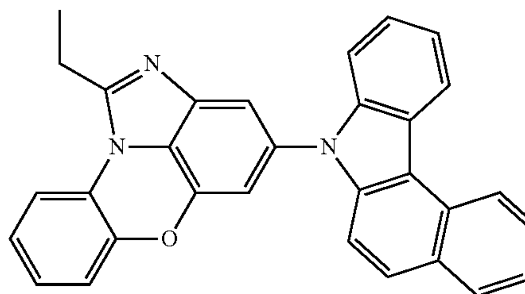
[Chemical Formula 1-10-15]
