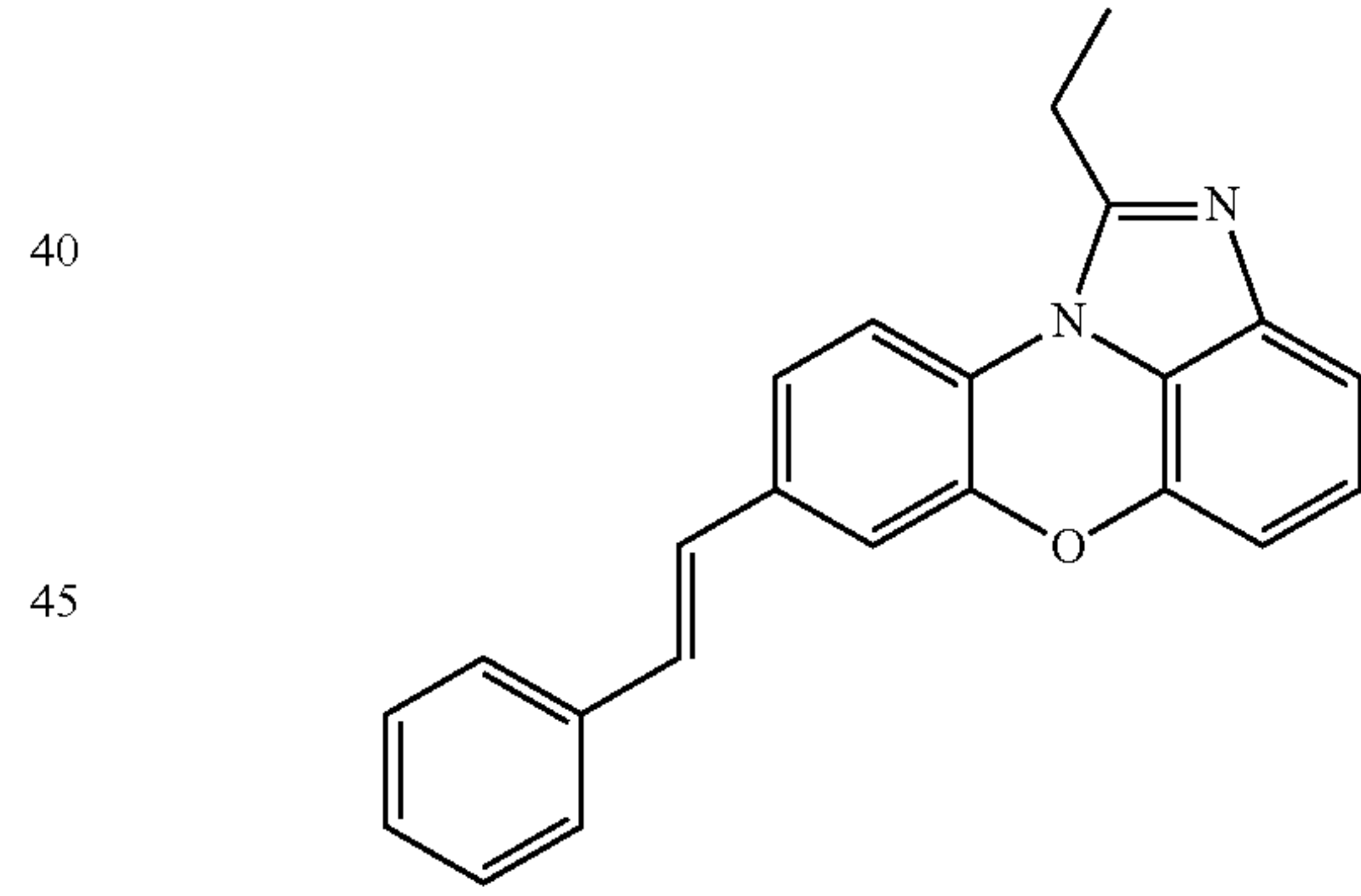
[Chemical Formula 1-4-1]
