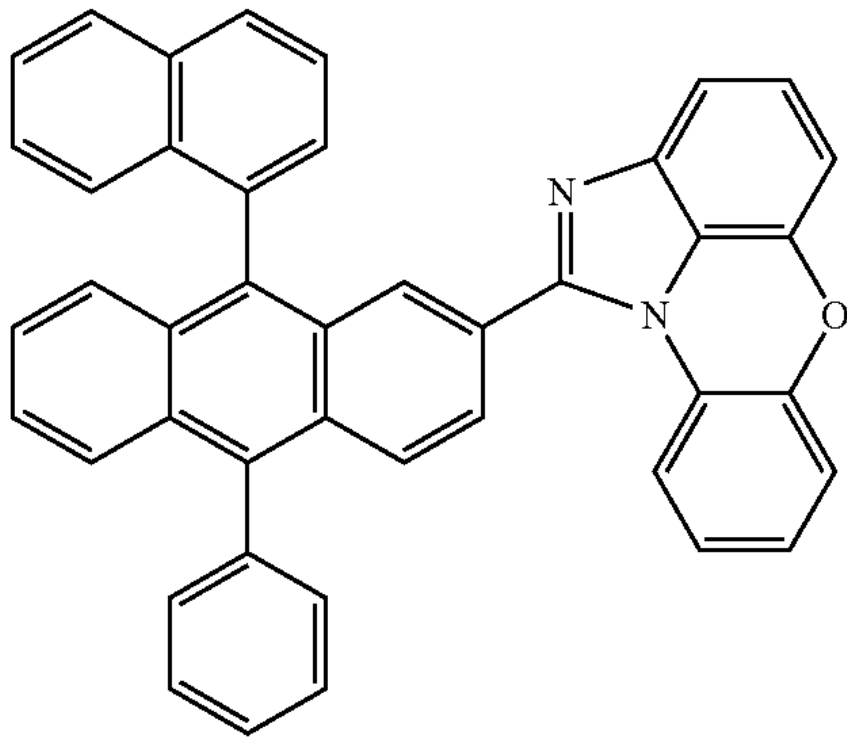
[Chemical Formula 1-1-30] 5
