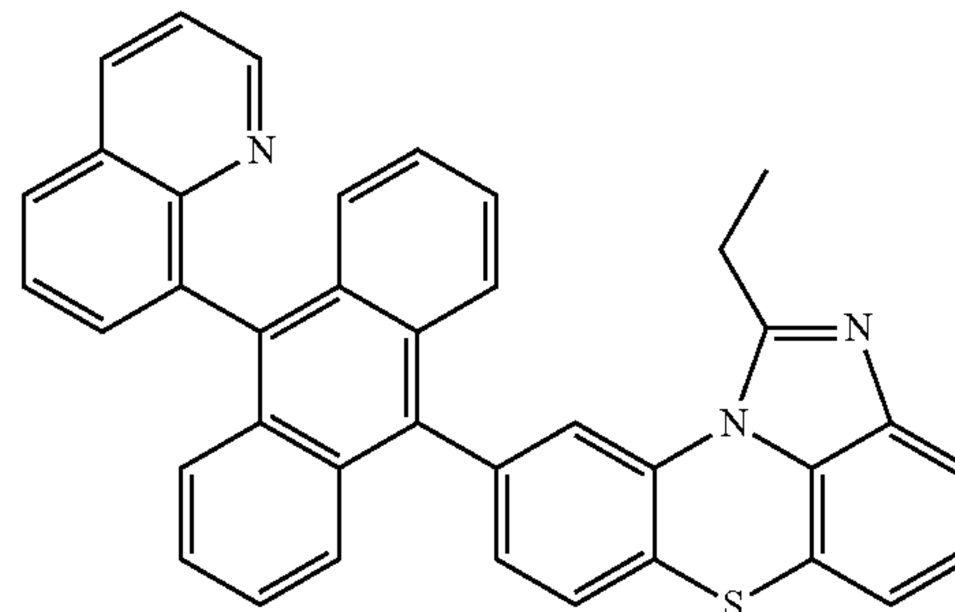
[Chemical Formula 2-3-11]
