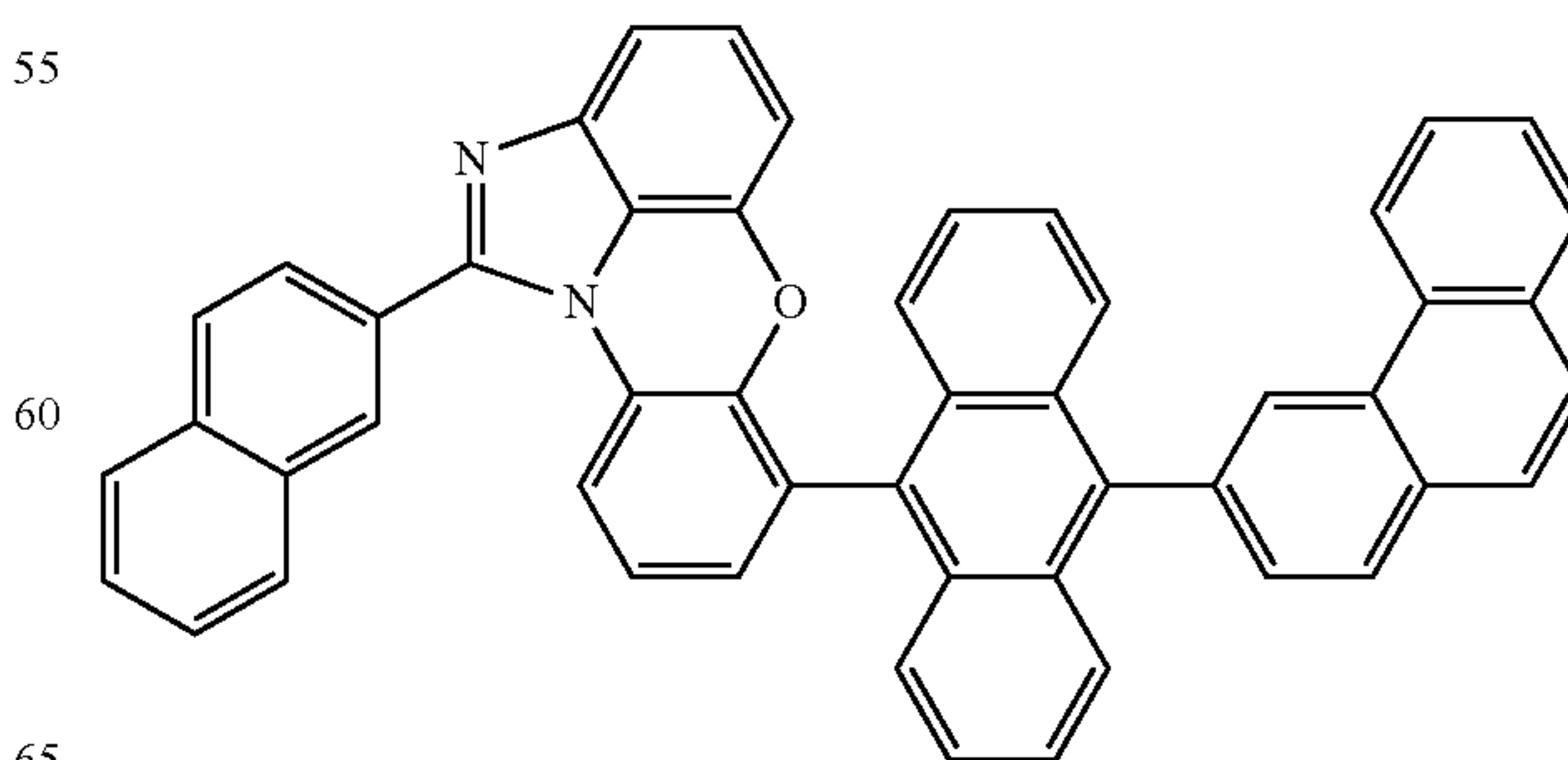
[Chemical Formula 1-6-8]
