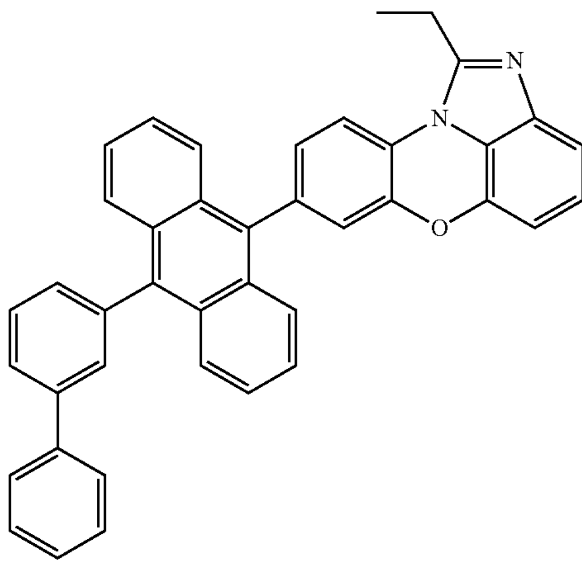
[Chemical Formula 1-3-6]
