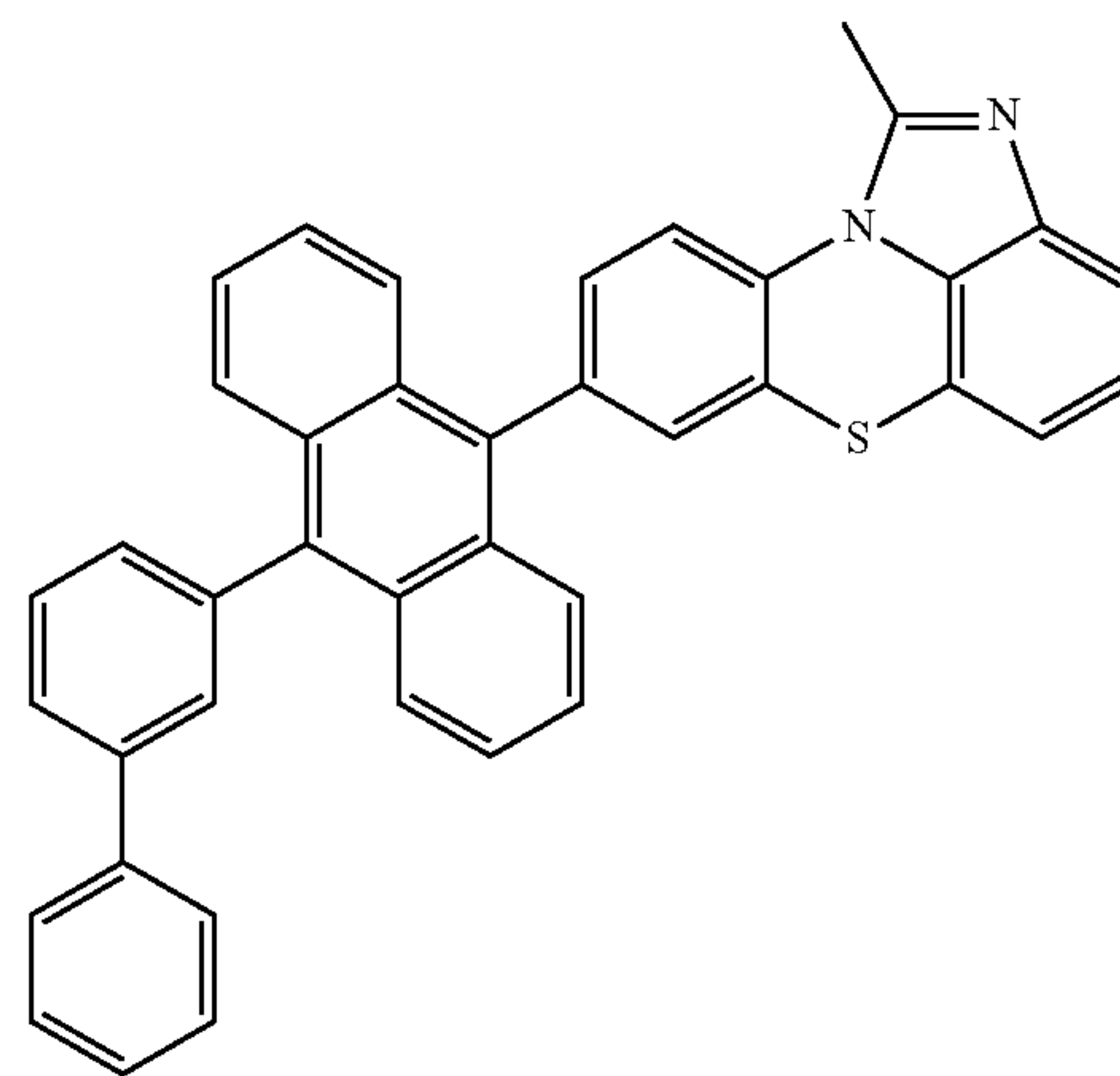
[Chemical Formula 2-2-6]
