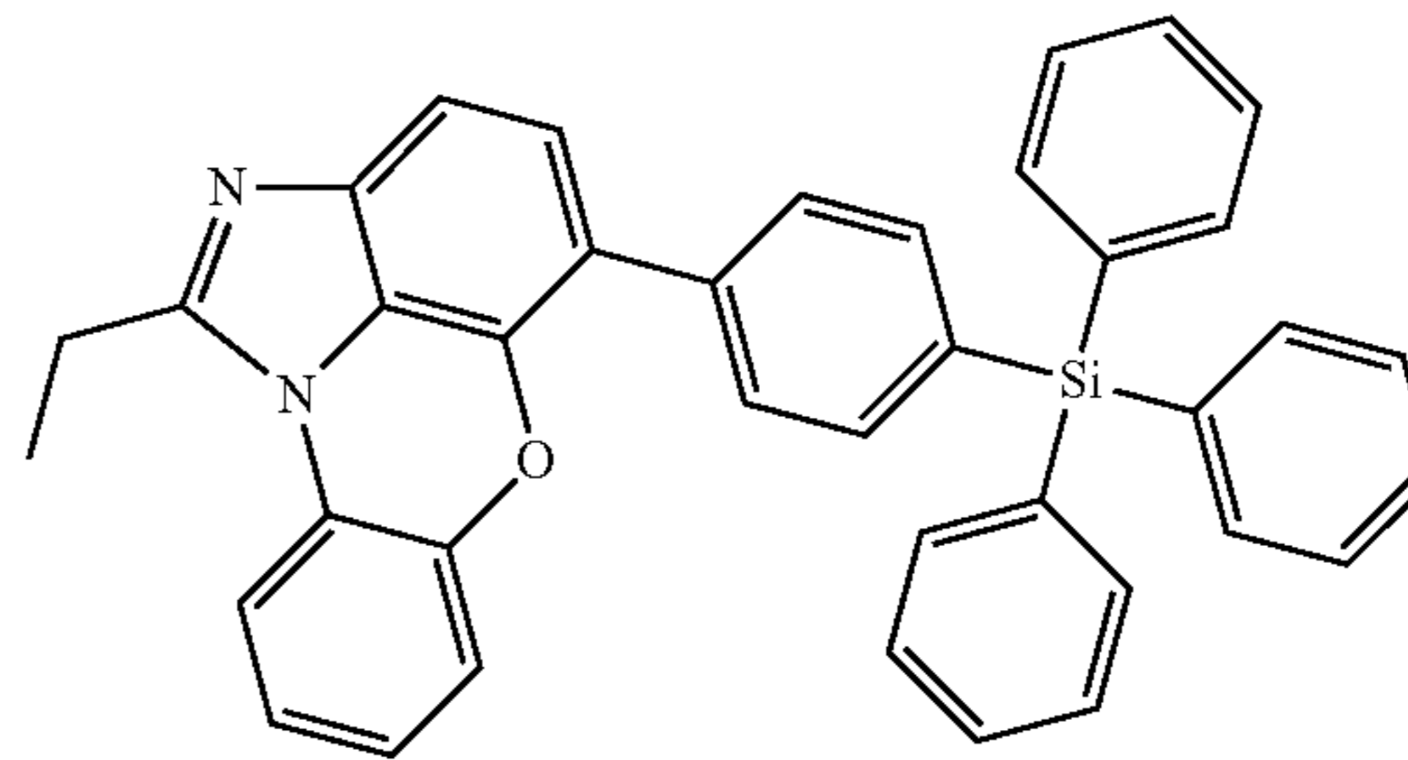
[Chemical Formula 1-9-13]
