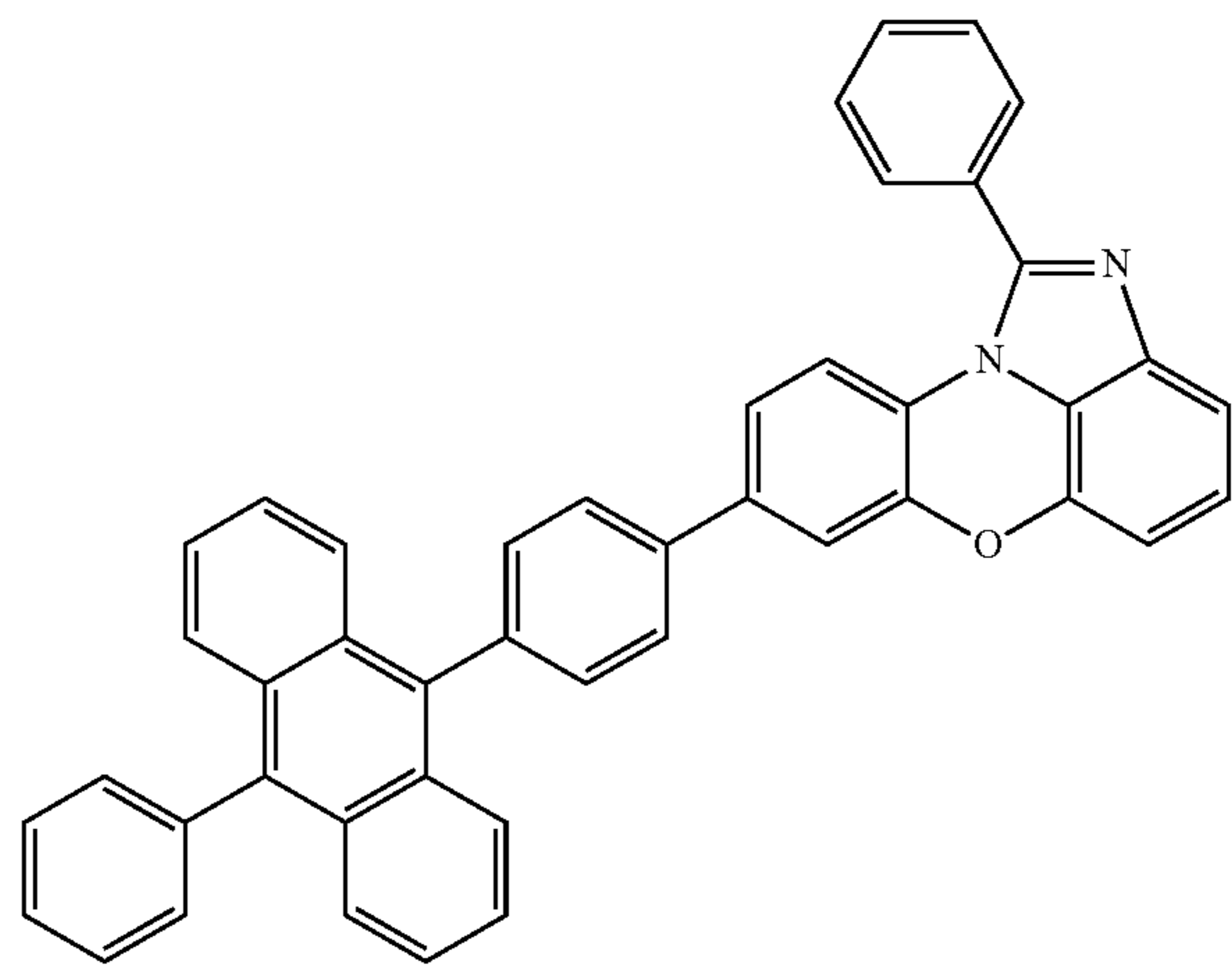
[Chemical Formula 1-4-17]
