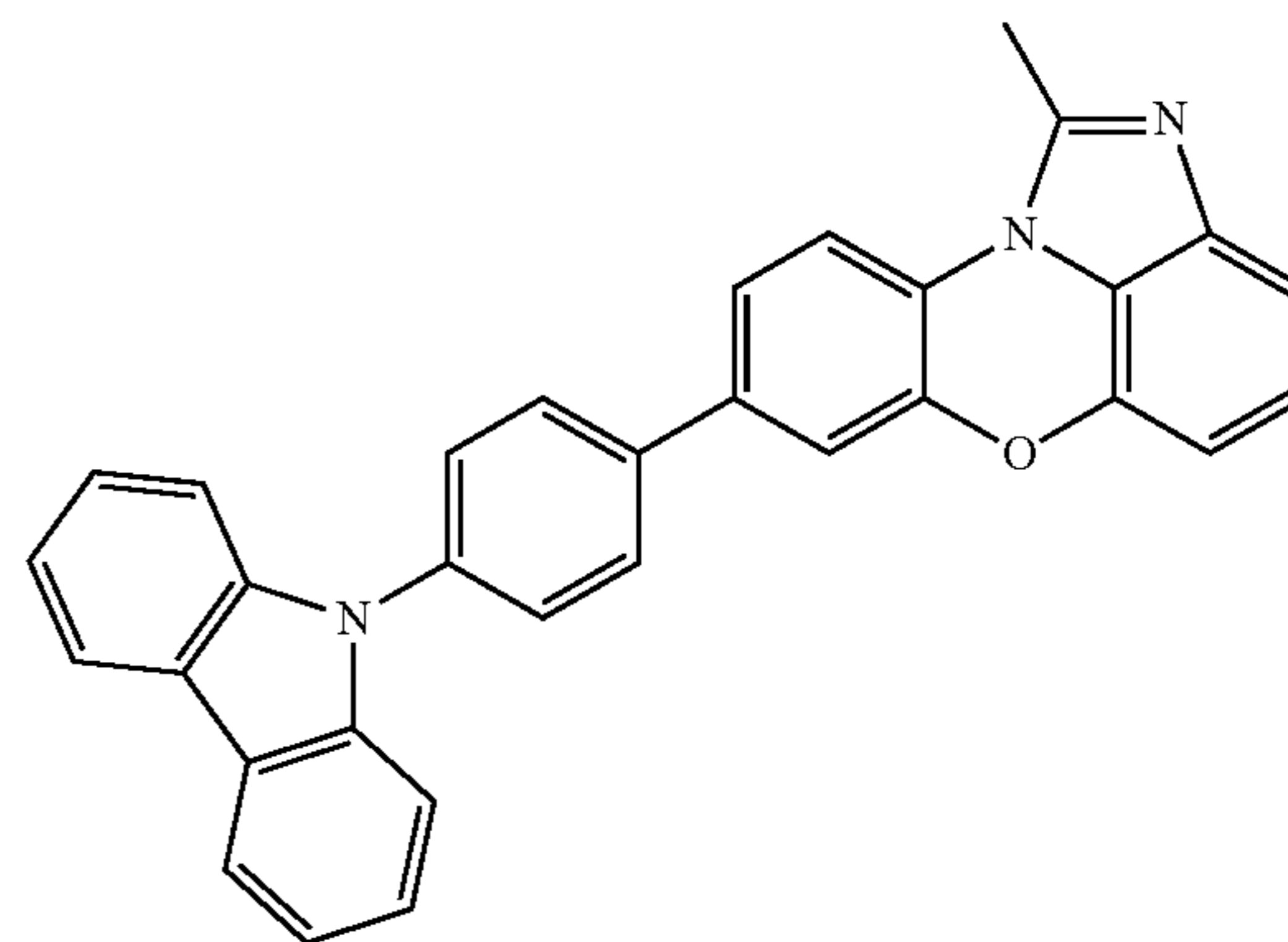
[Chemical Formula 1-2-43]
