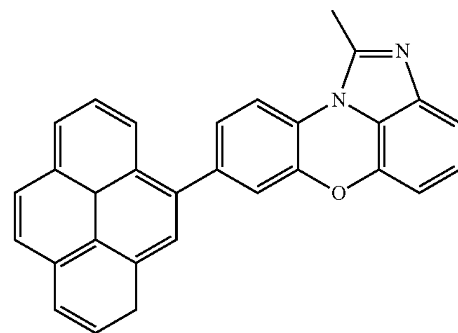
[Chemical Formula 1-2-28]
