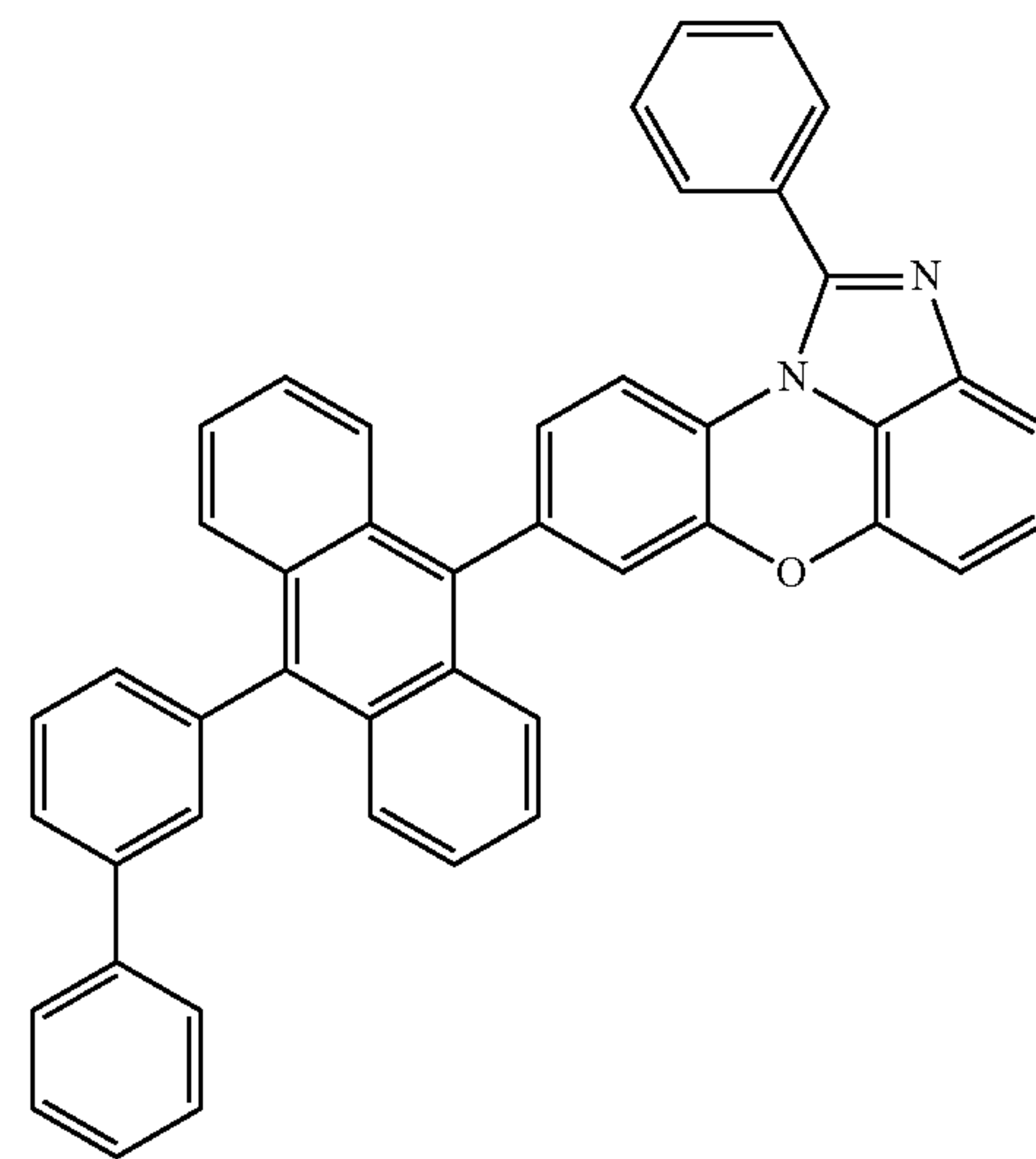
[Chemical Formula 1-4-6]
