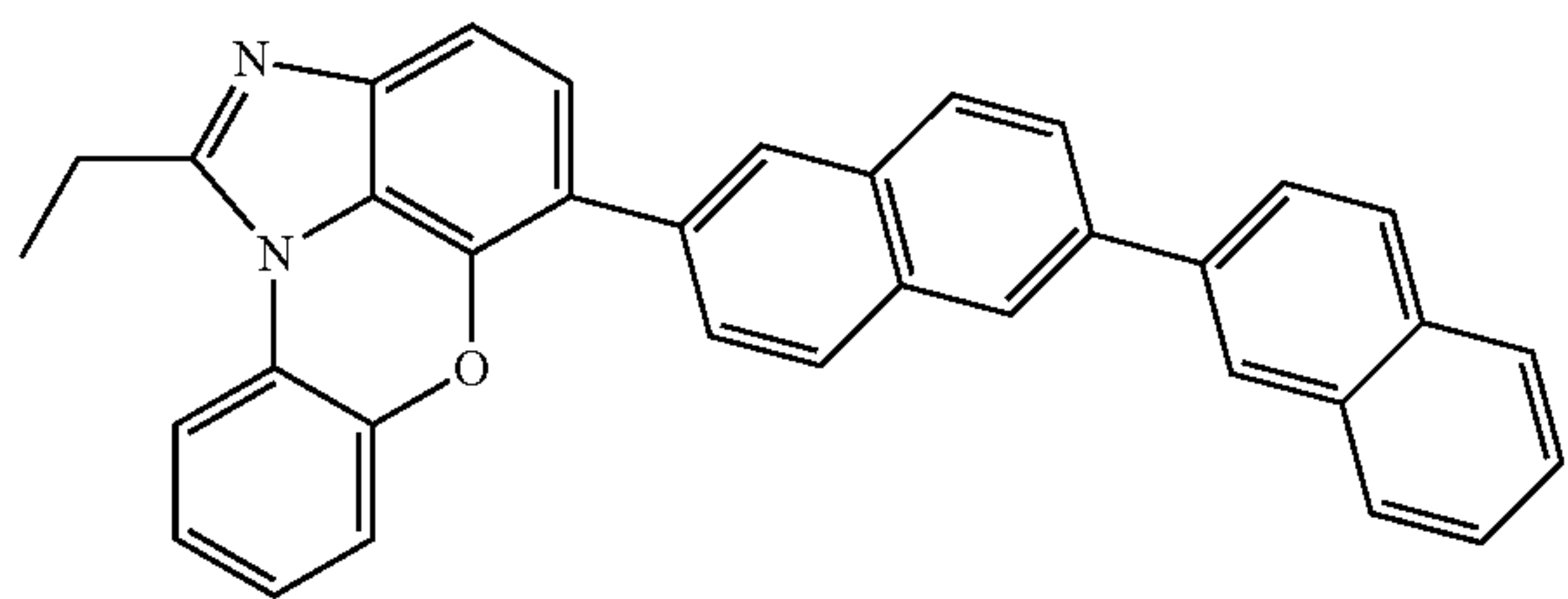
[Chemical Formula 1-9-8]
