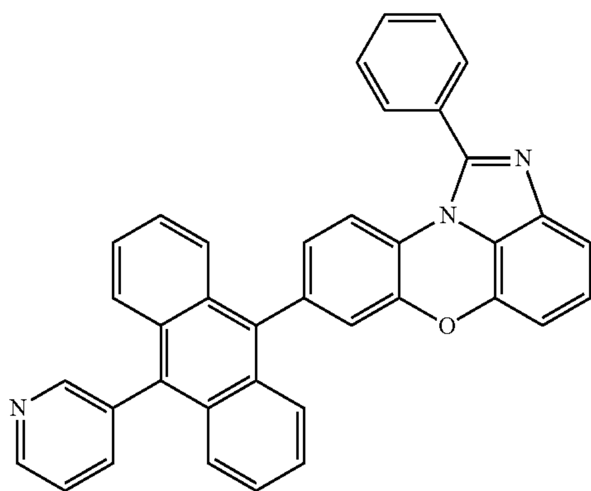
[Chemical Formula 1-4-10]
