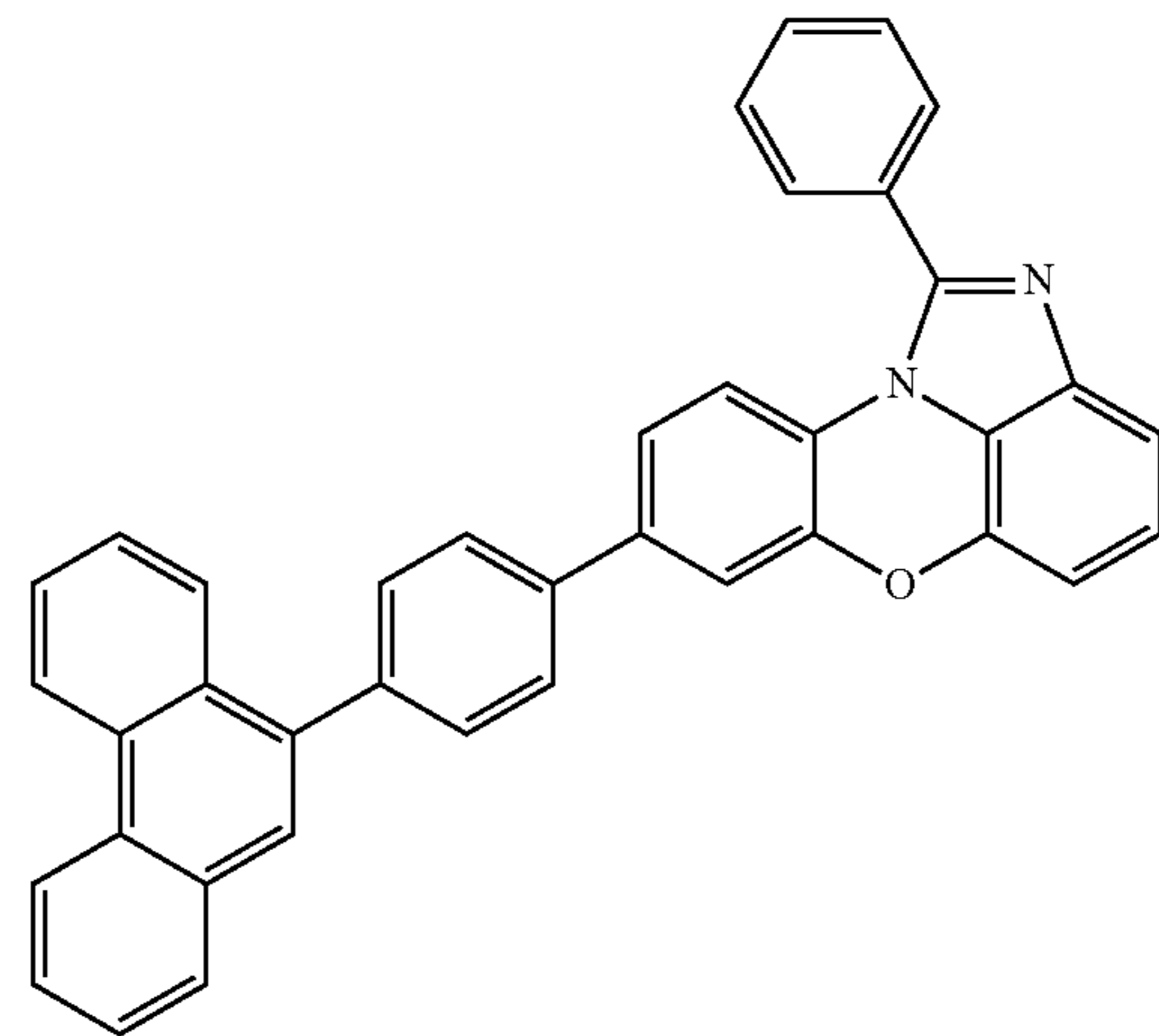
[Chemical Formula 1-4-32]
