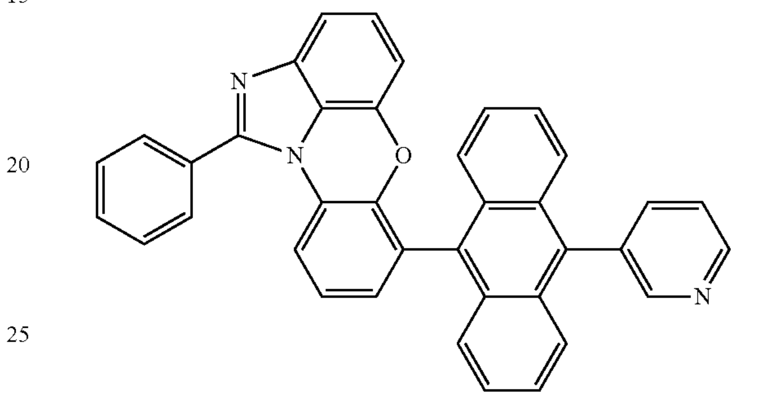
[Chemical Formula 1-6-11]
