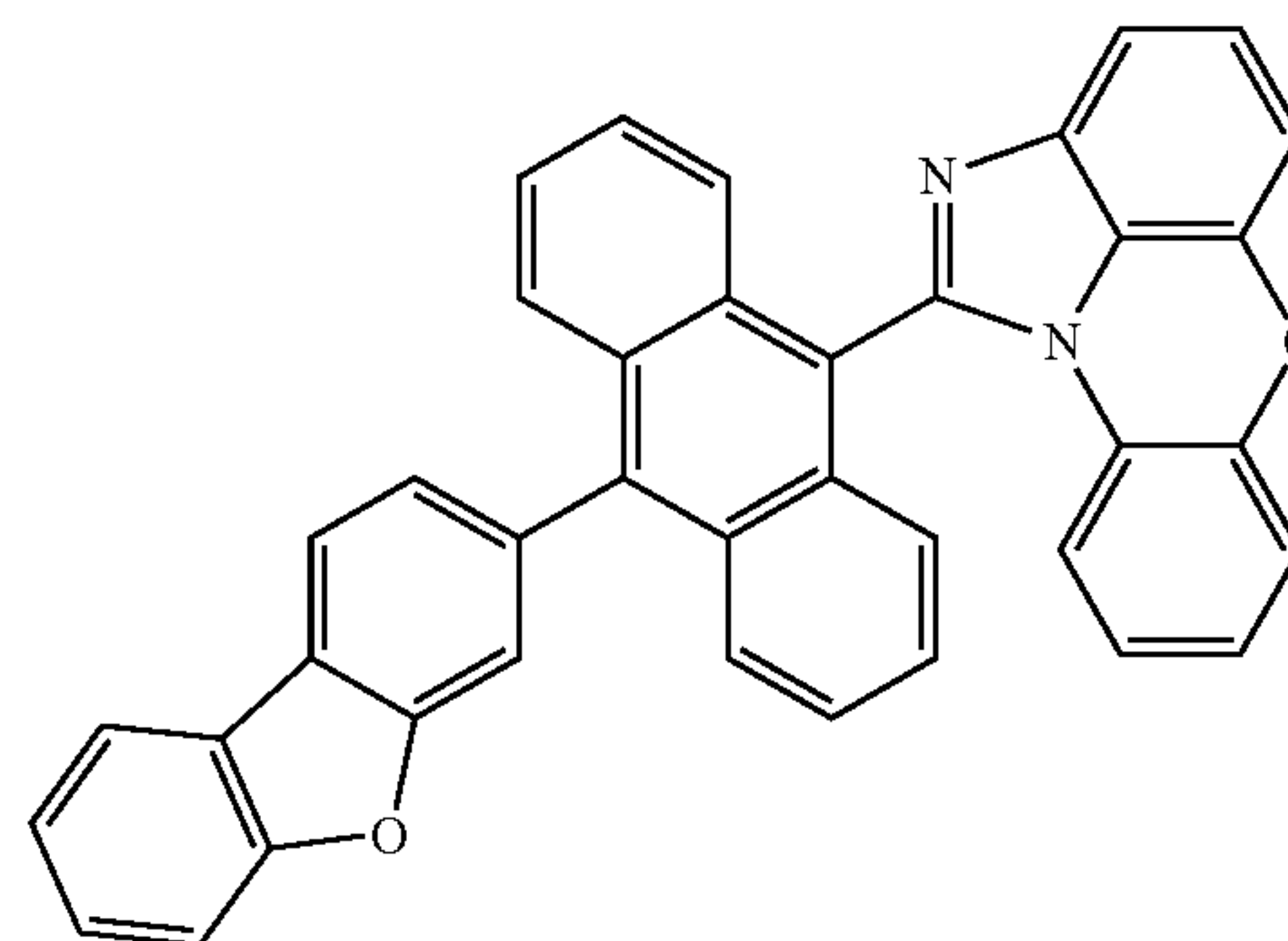
[Chemical Formula 1-1-21]
