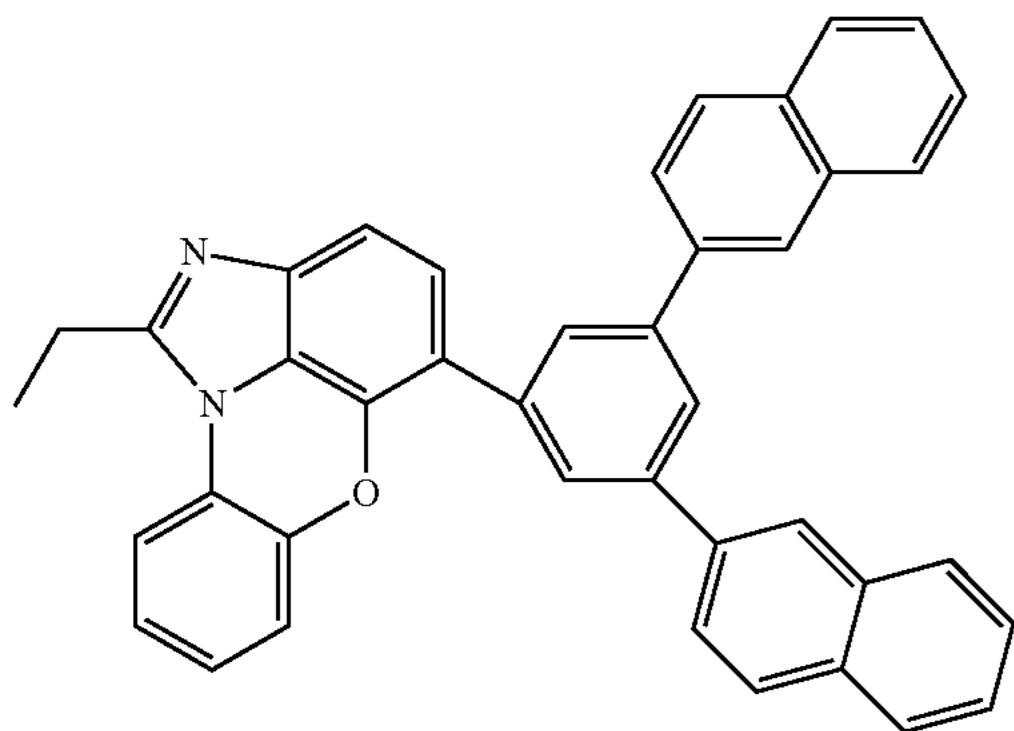
[Chemical Formula 1-9-8]
