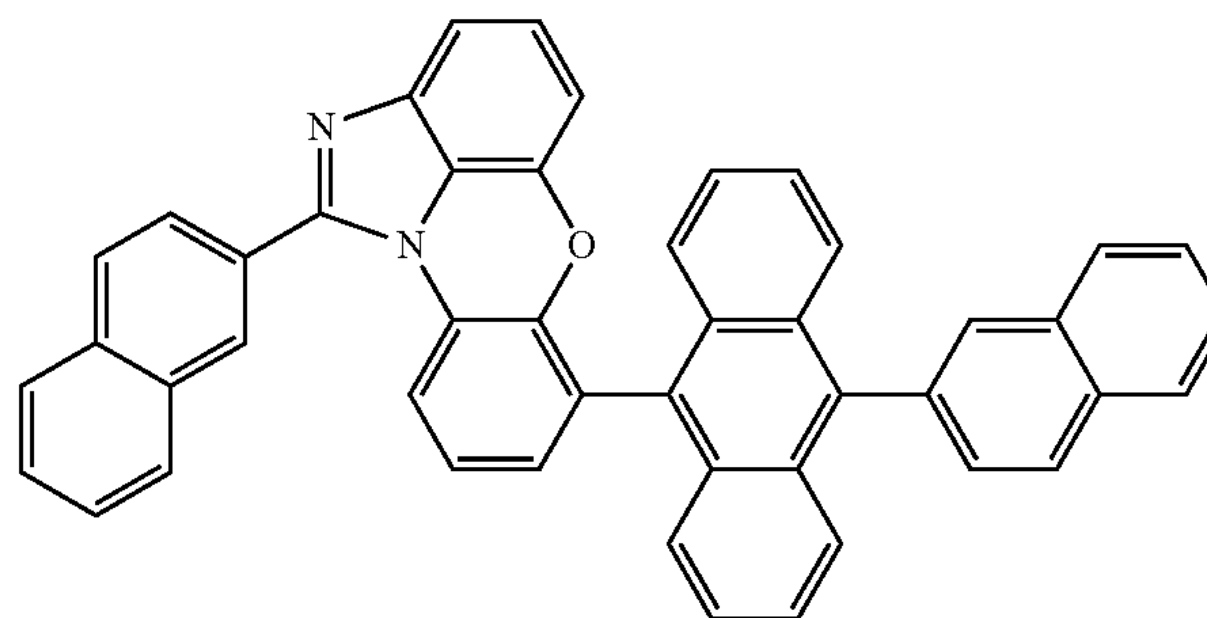
[Chemical Formula 1-6-3]
