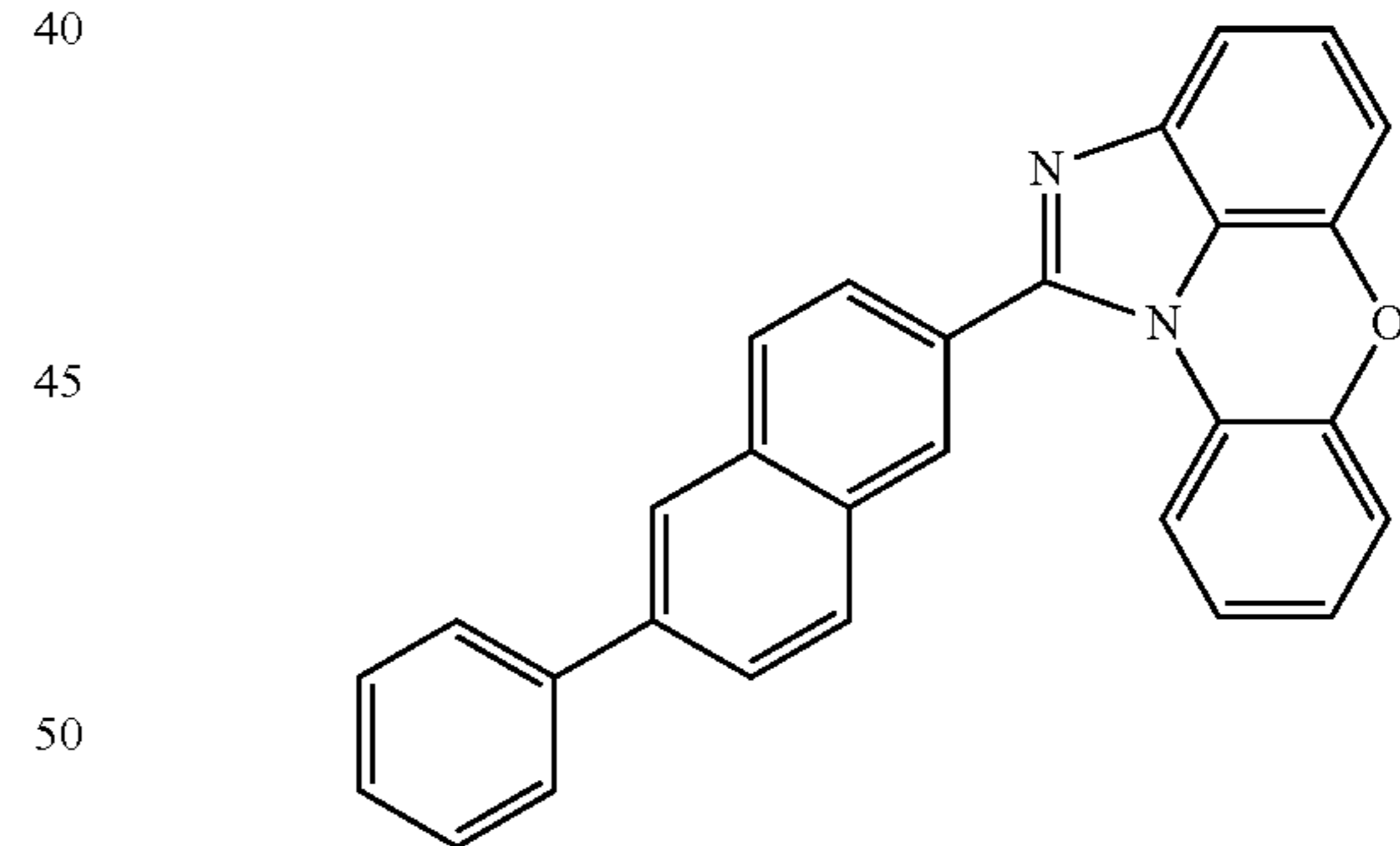
[Chemical Formula 1-1-35]
