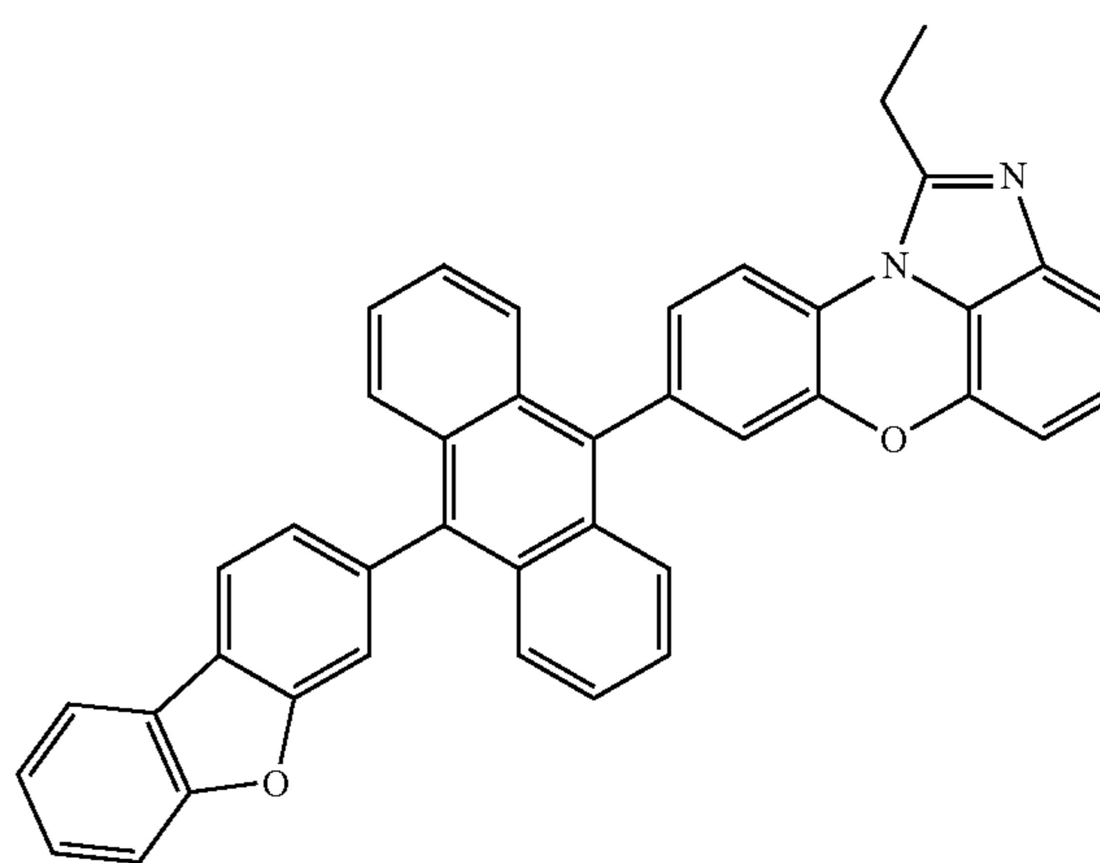
[Chemical Formula 1-3-14]
