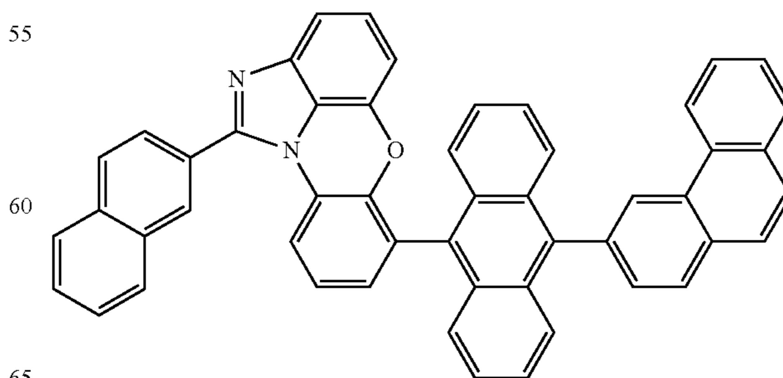
[Chemical Formula 1-6-8]
