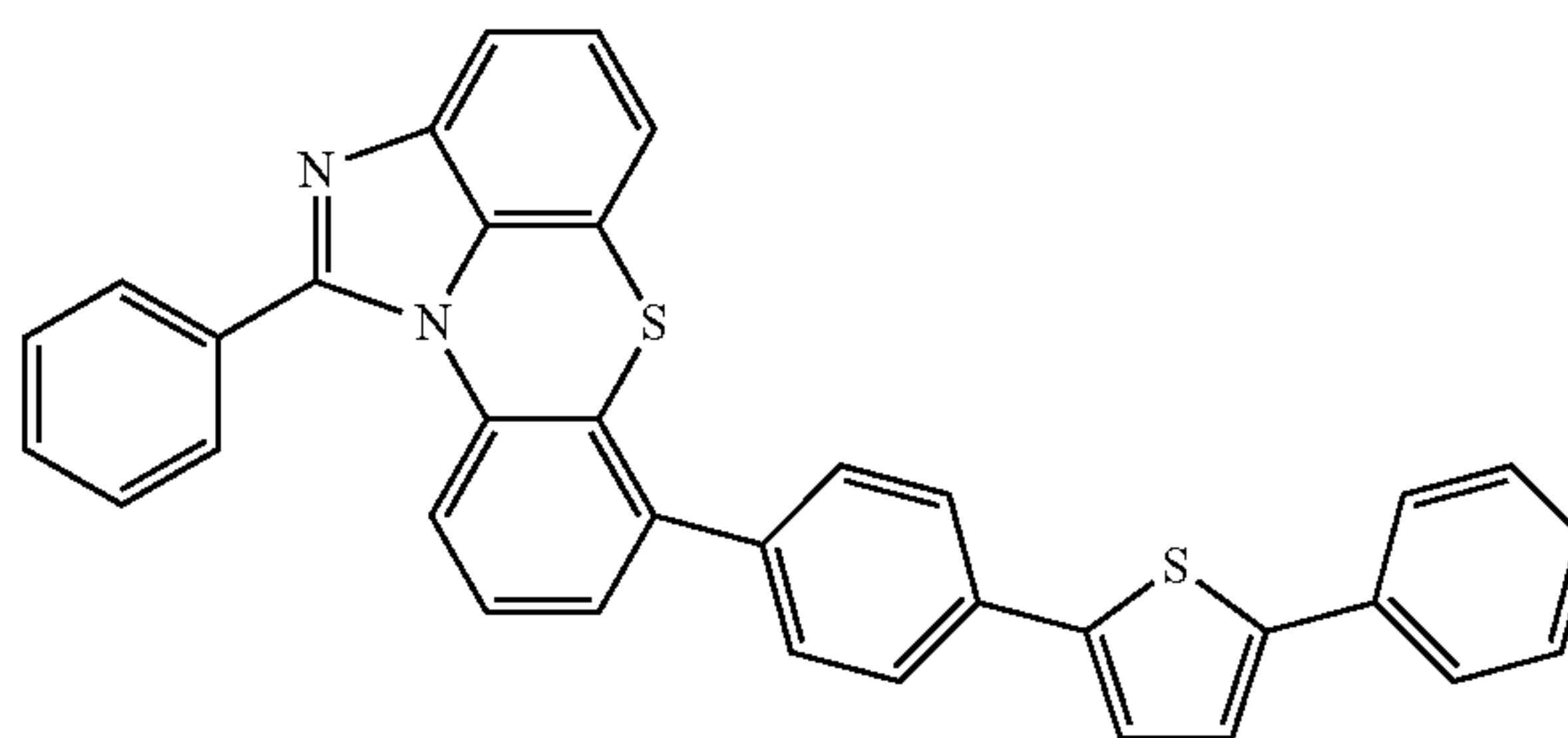
[Chemical Formula 2-2-39]
