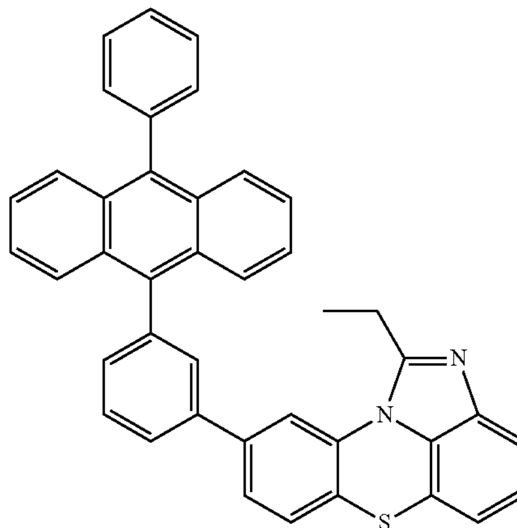
[Chemical Formula 2-3-19]
