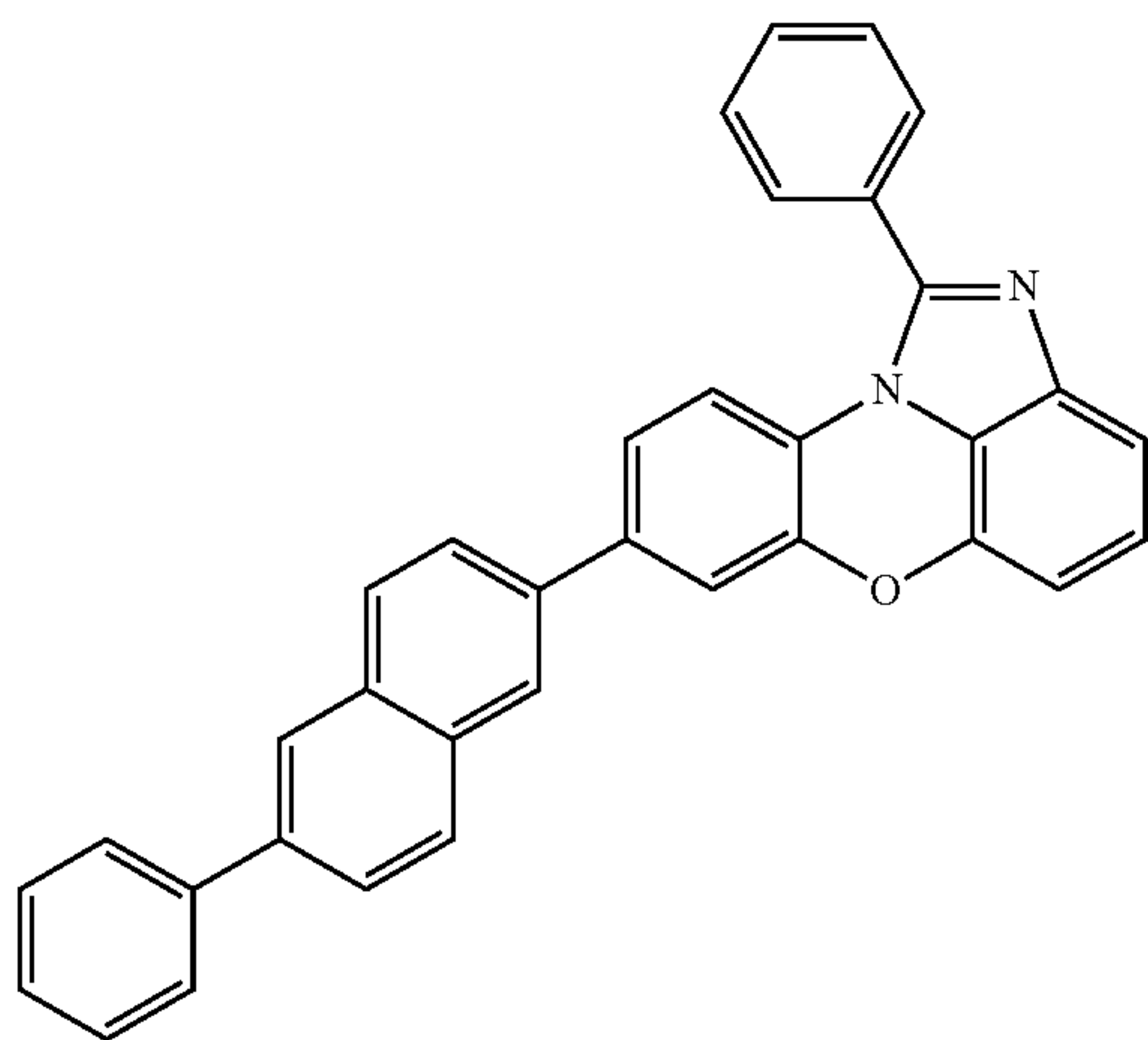
[Chemical Formula 1-4-27]
