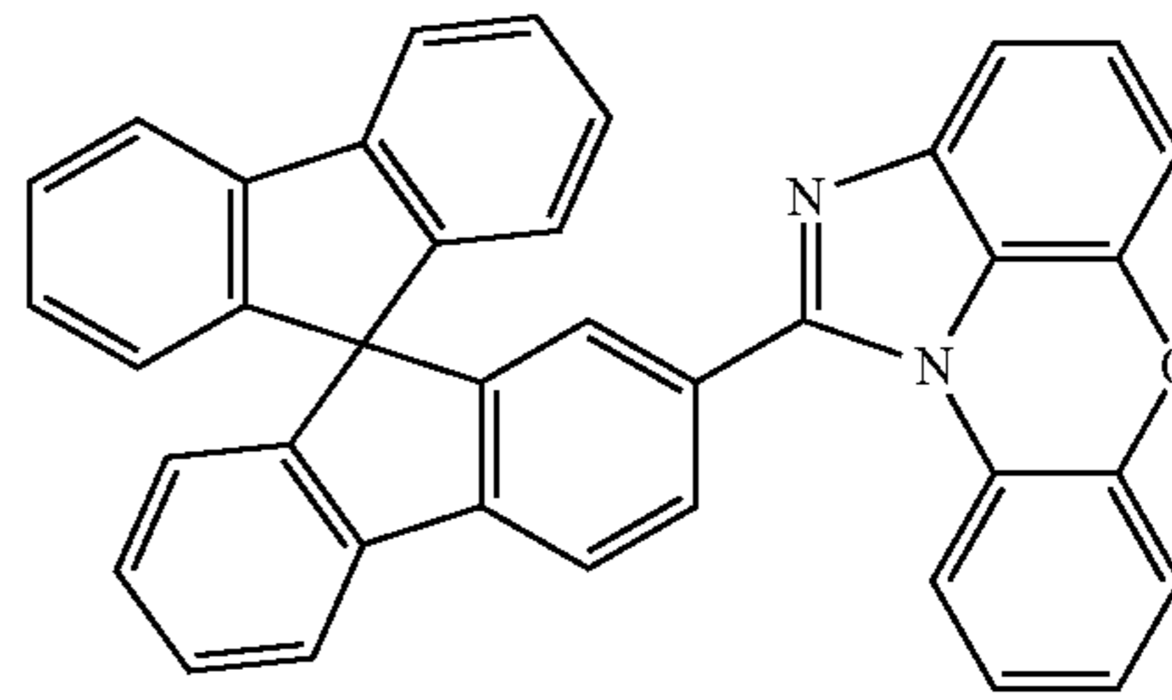
[Chemical Formula 1-1-42]
