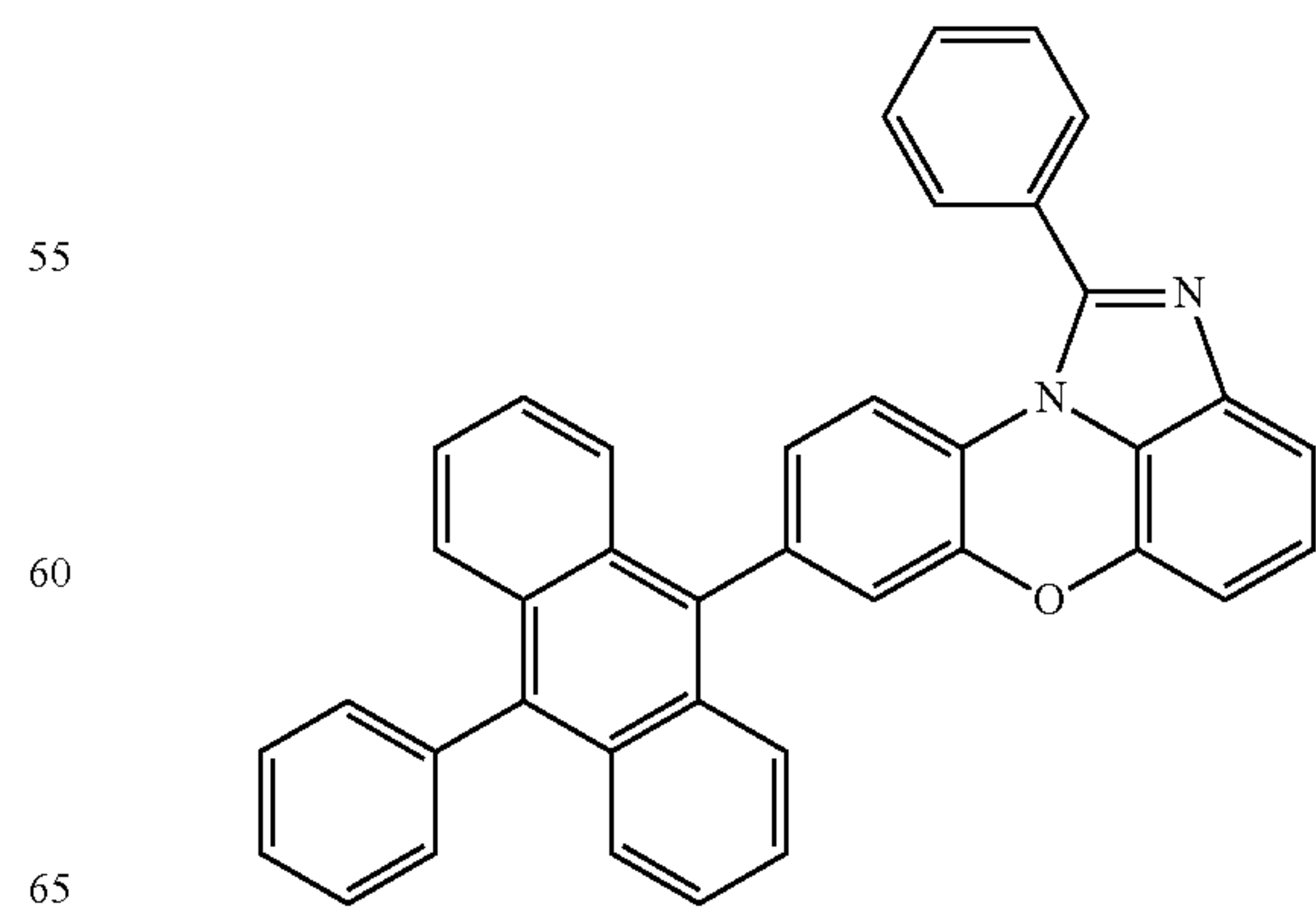
[Chemical Formula 1-4-1]
