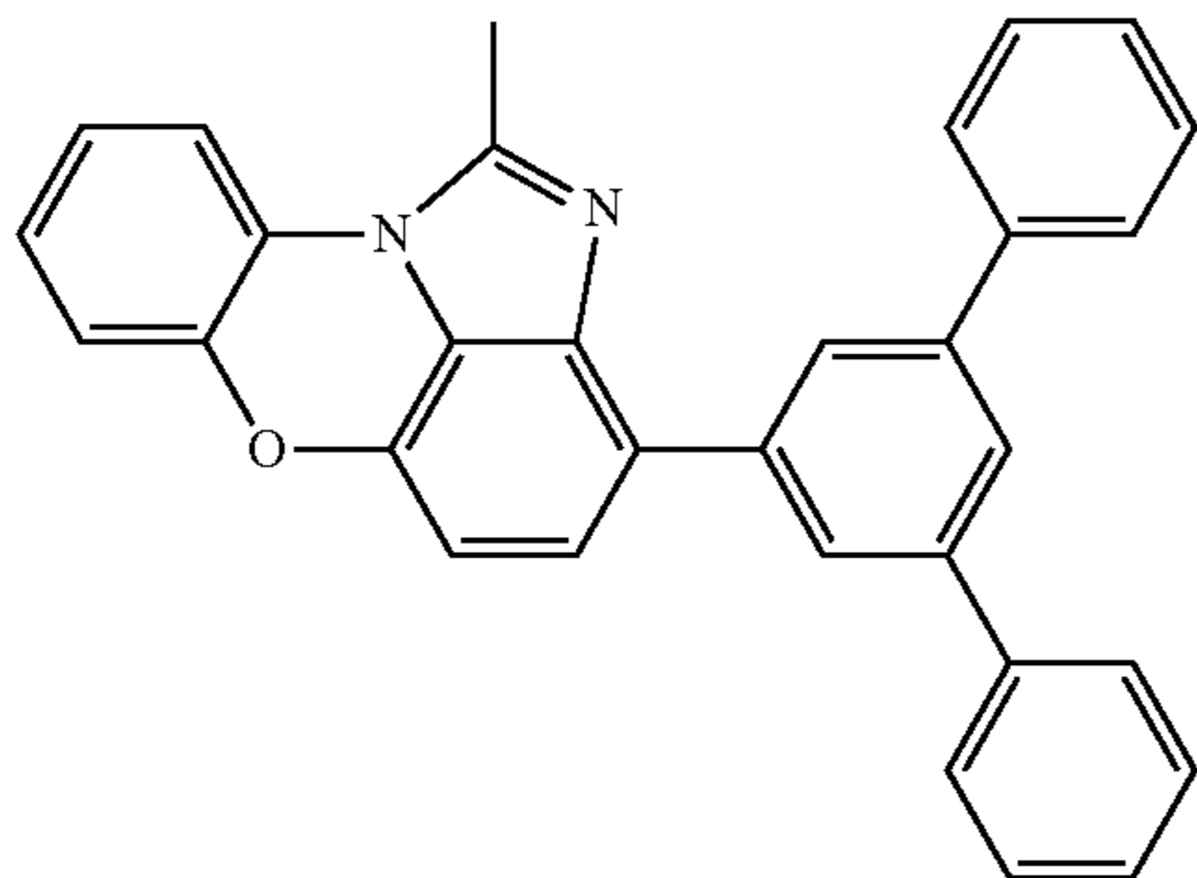
[Chemical Formula 1-11-5]
