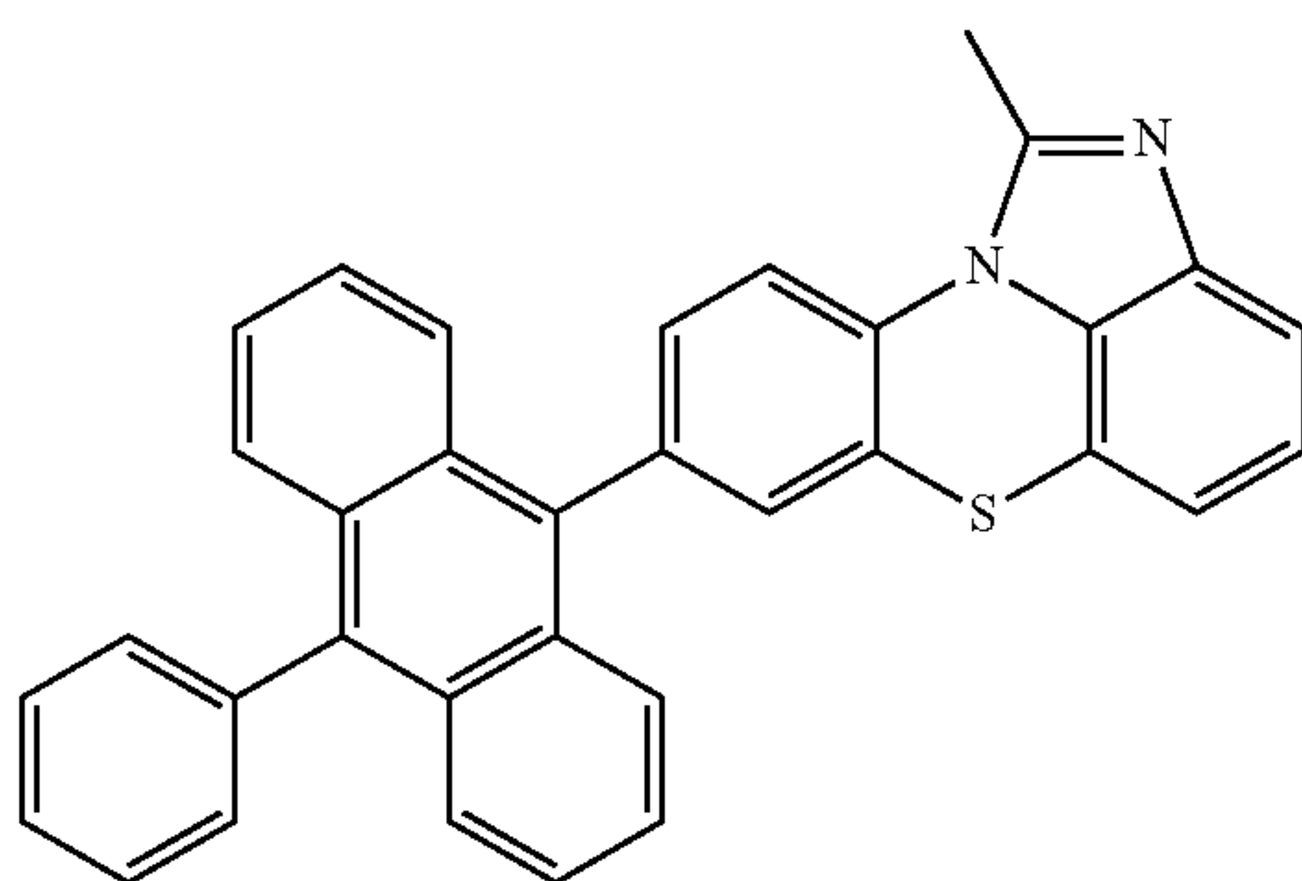
[Chemical Formula 2-2-1]
