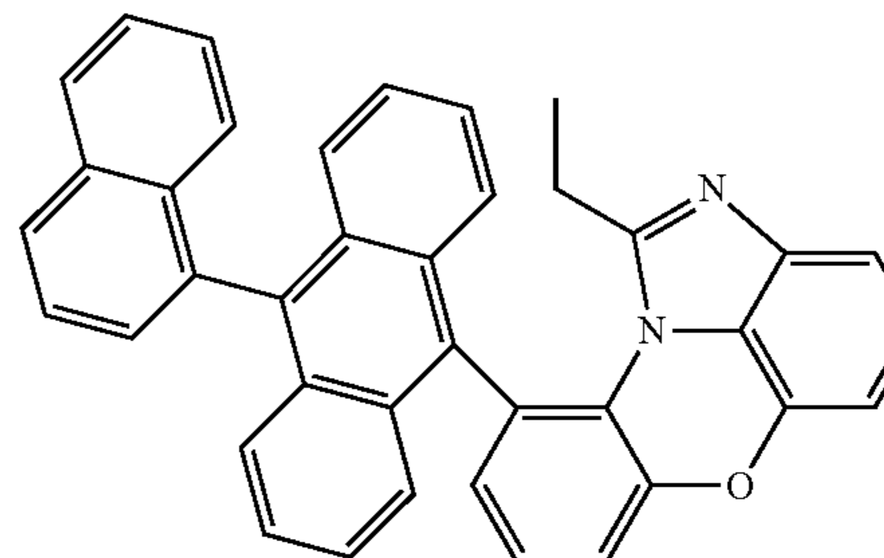
[Chemical Formula 1-8-4]
