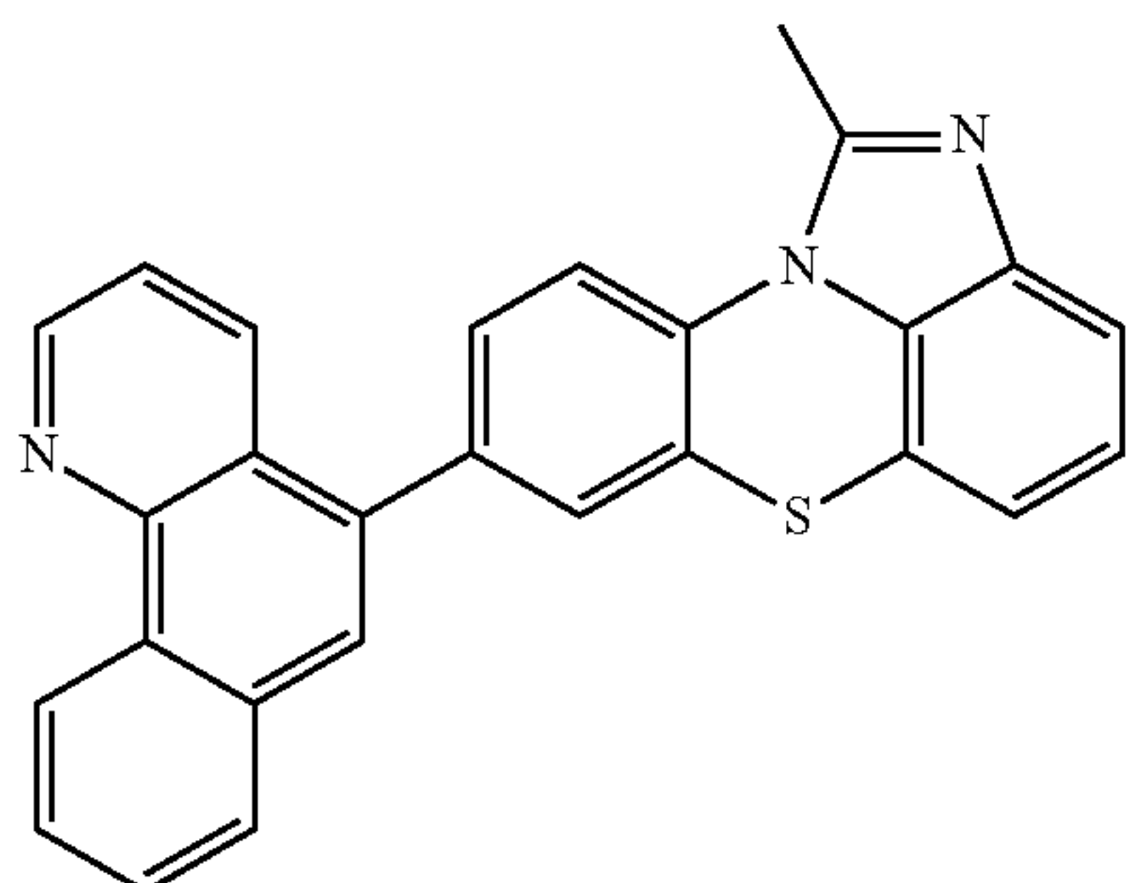
[Chemical Formula 2-2-33]
