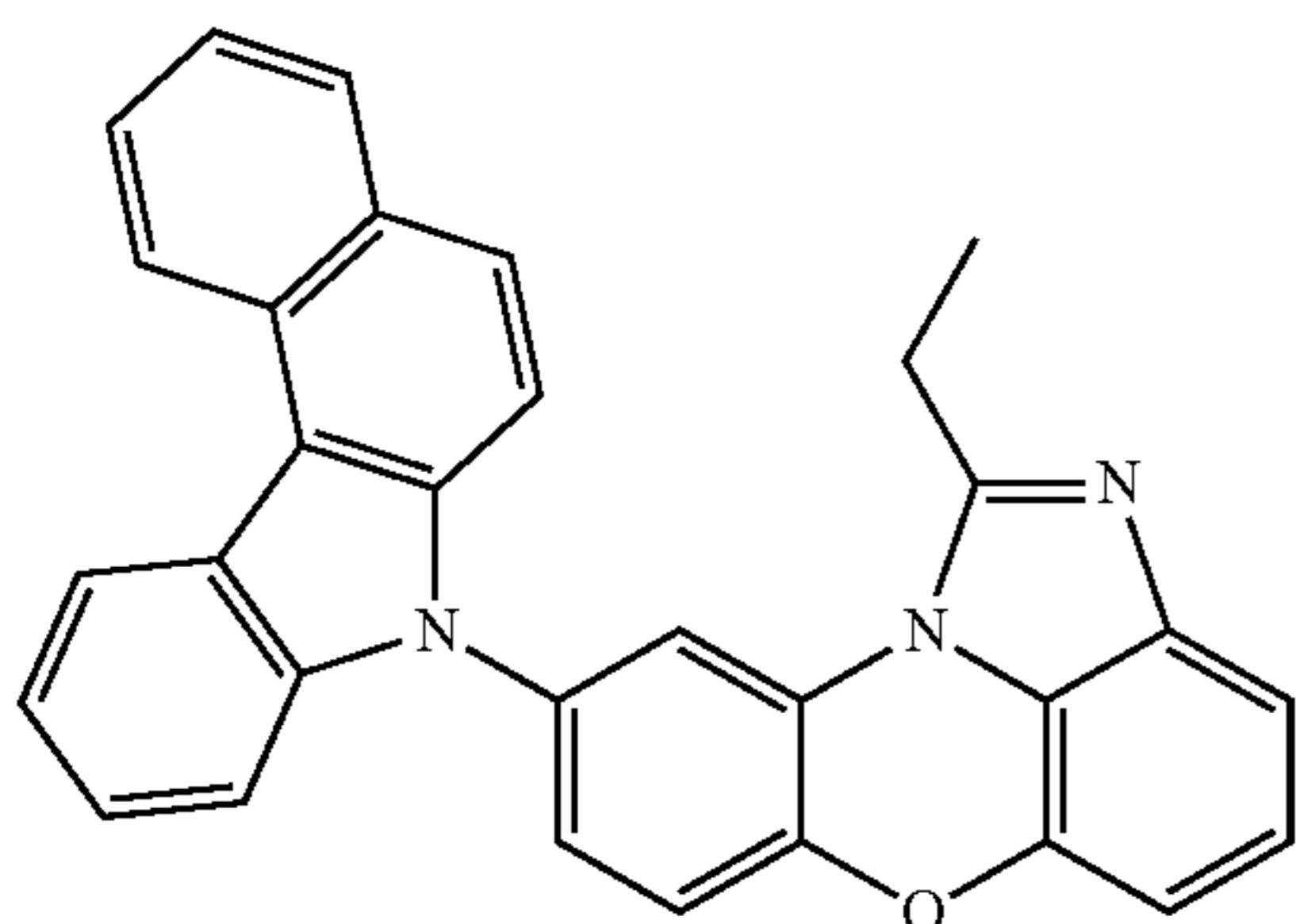
[Chemical Formula 1-7-51]
