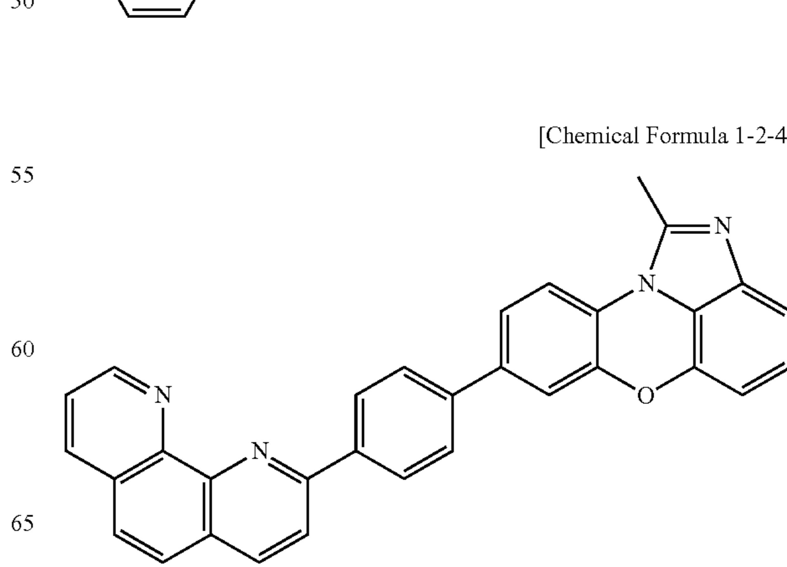
[Chemical Formula 1-2-47]
