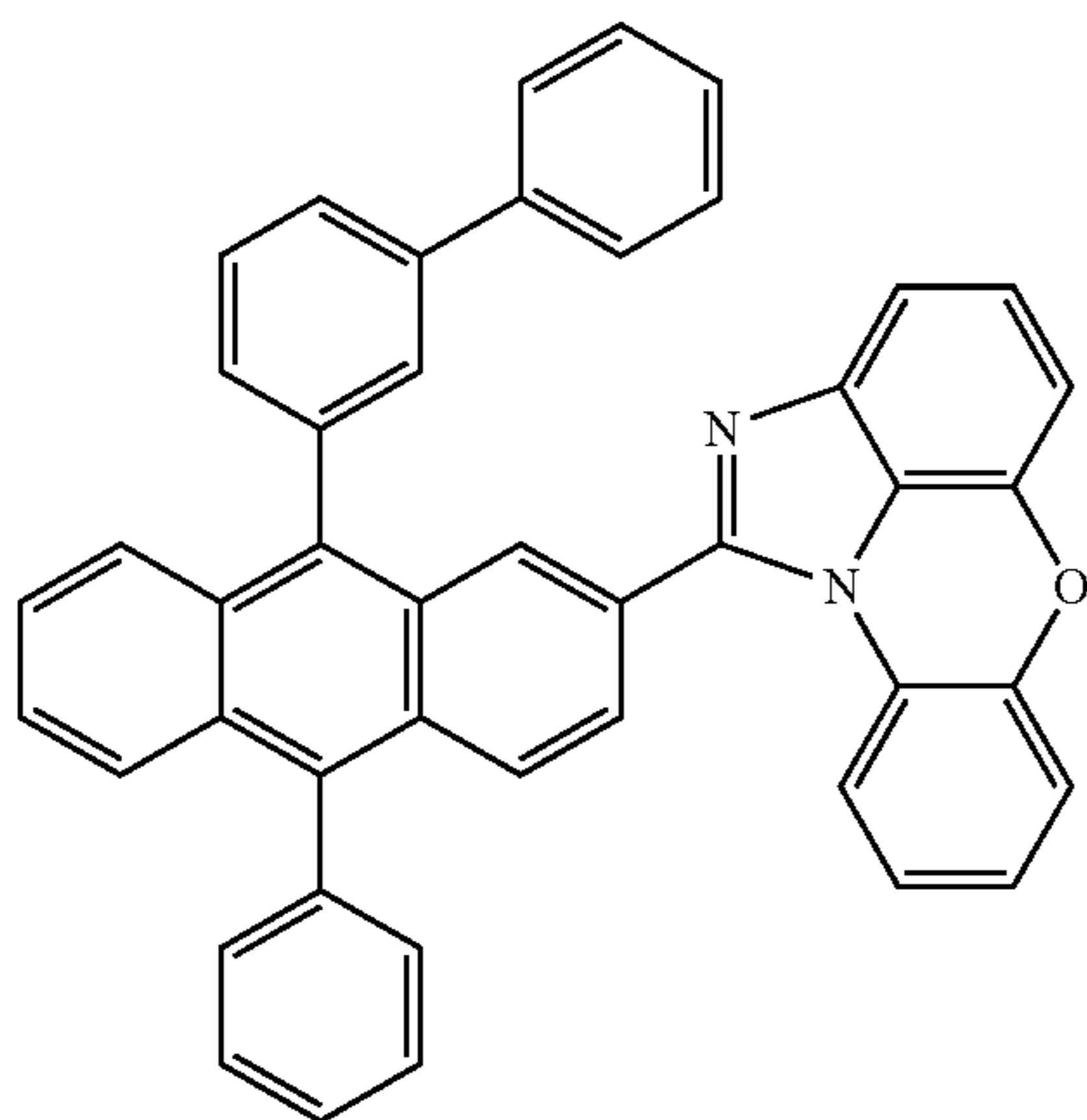
[Chemical Formula 1-1-32]
