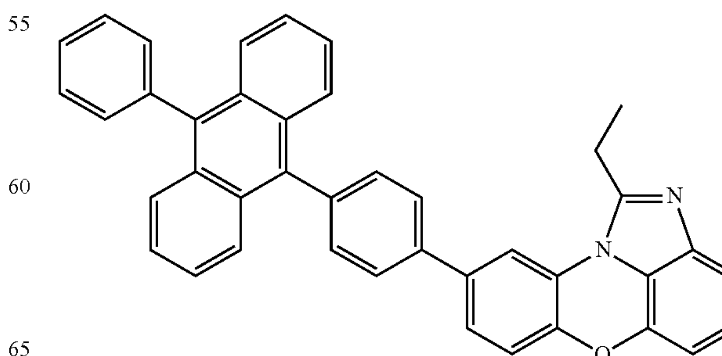
[Chemical Formula 1-7-17]
