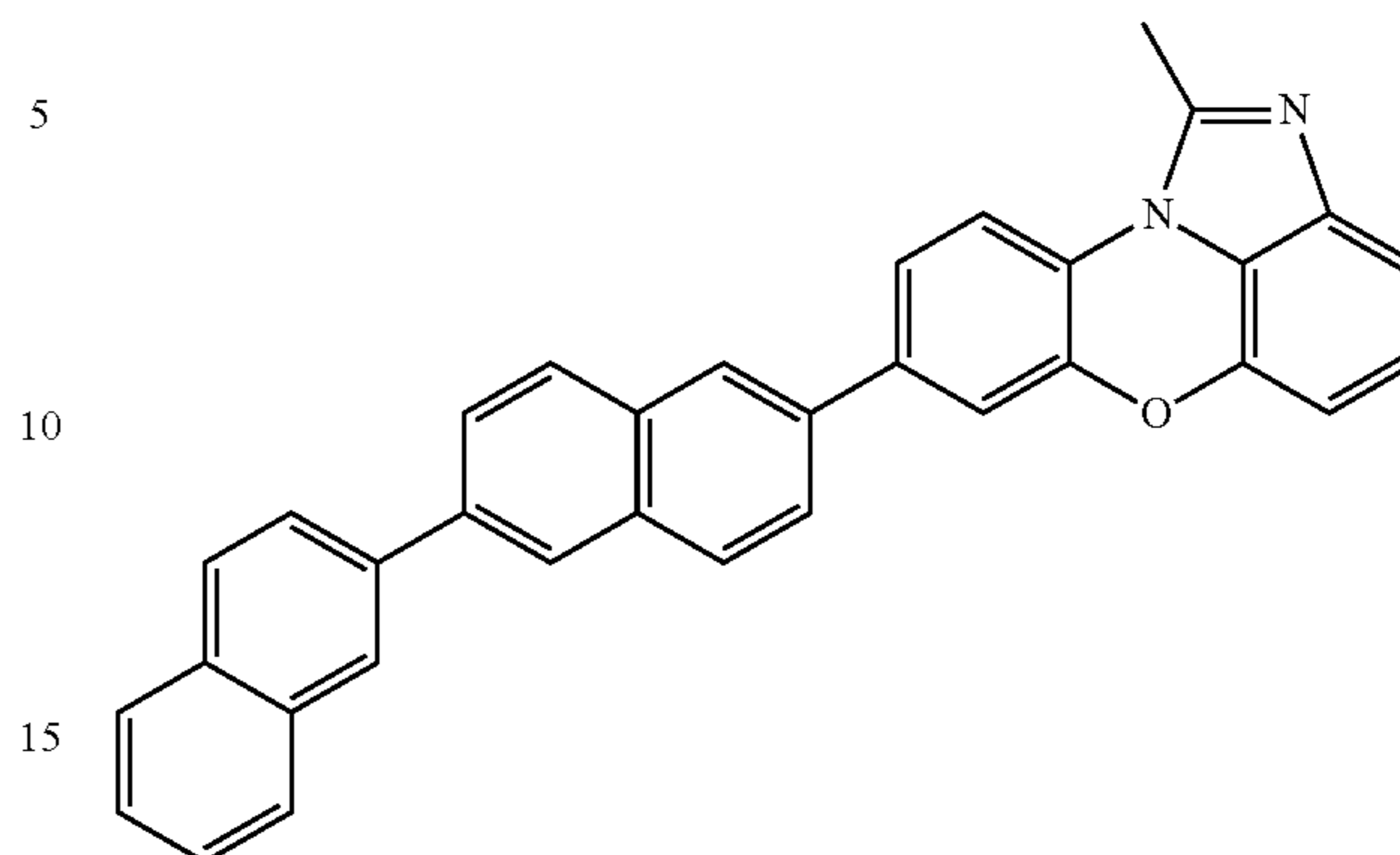
[Chemical Formula 1-2-45]
