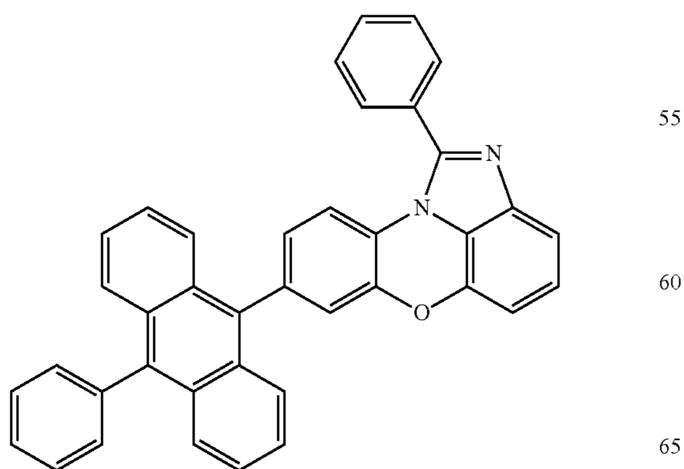
[Chemical Formula 1-4-1]
