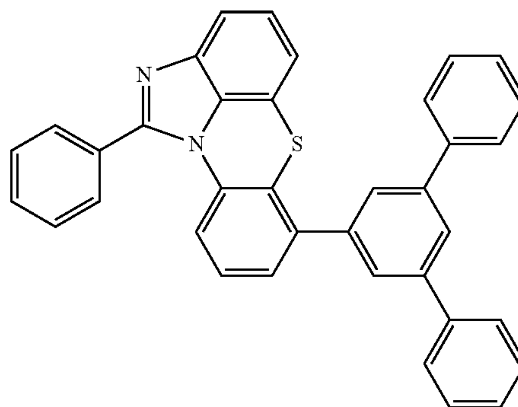
[Chemical Formula 2-2-40]
