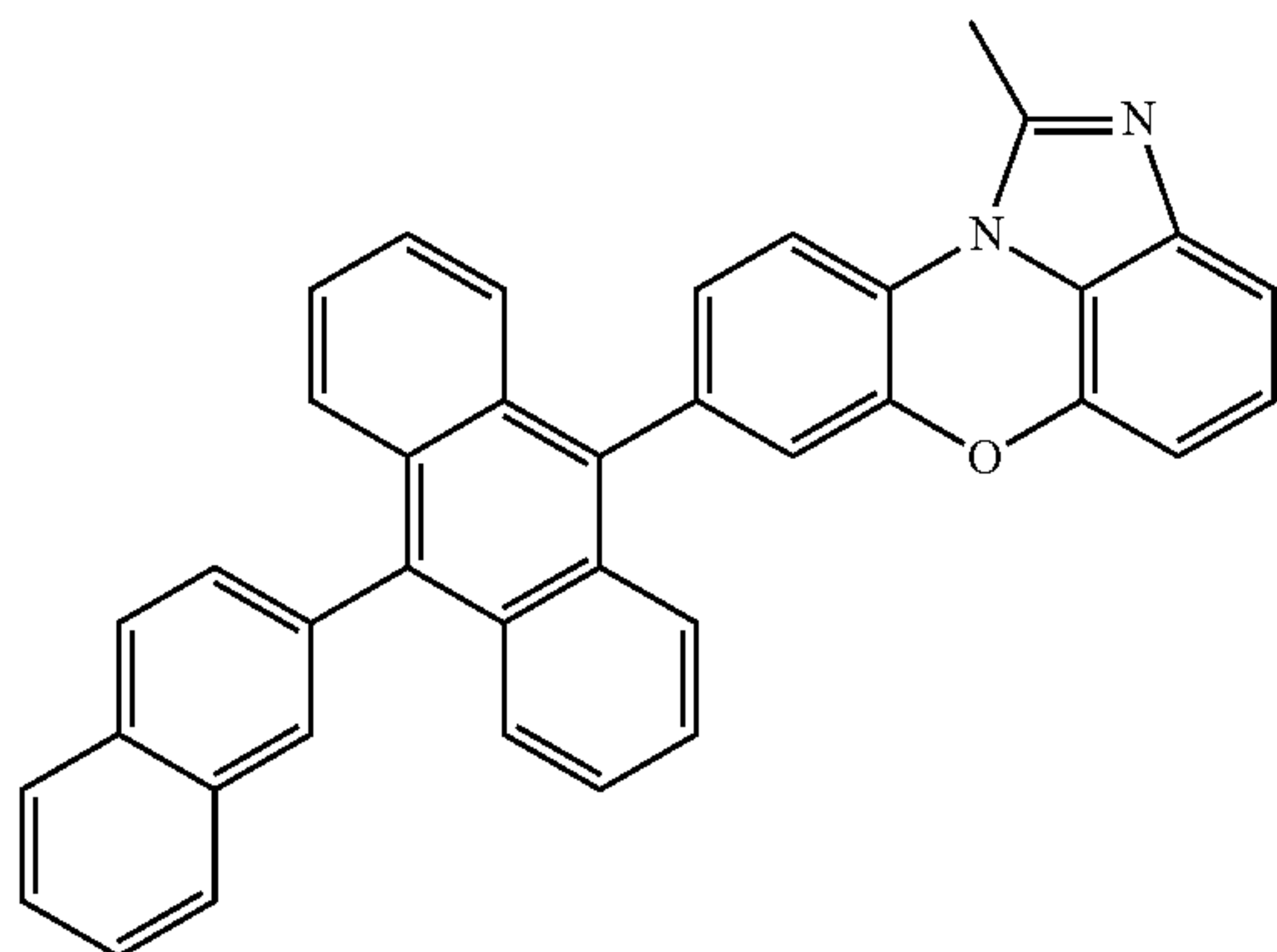
[Chemical Formula 1-2-3]
