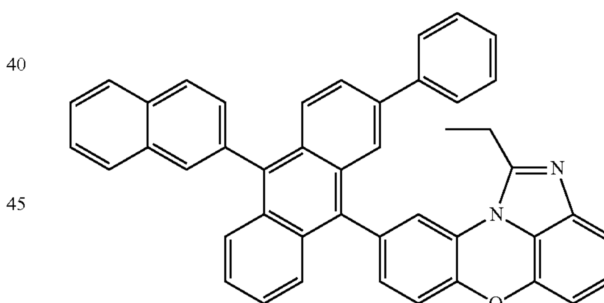
[Chemical Formula 1-7-16]
