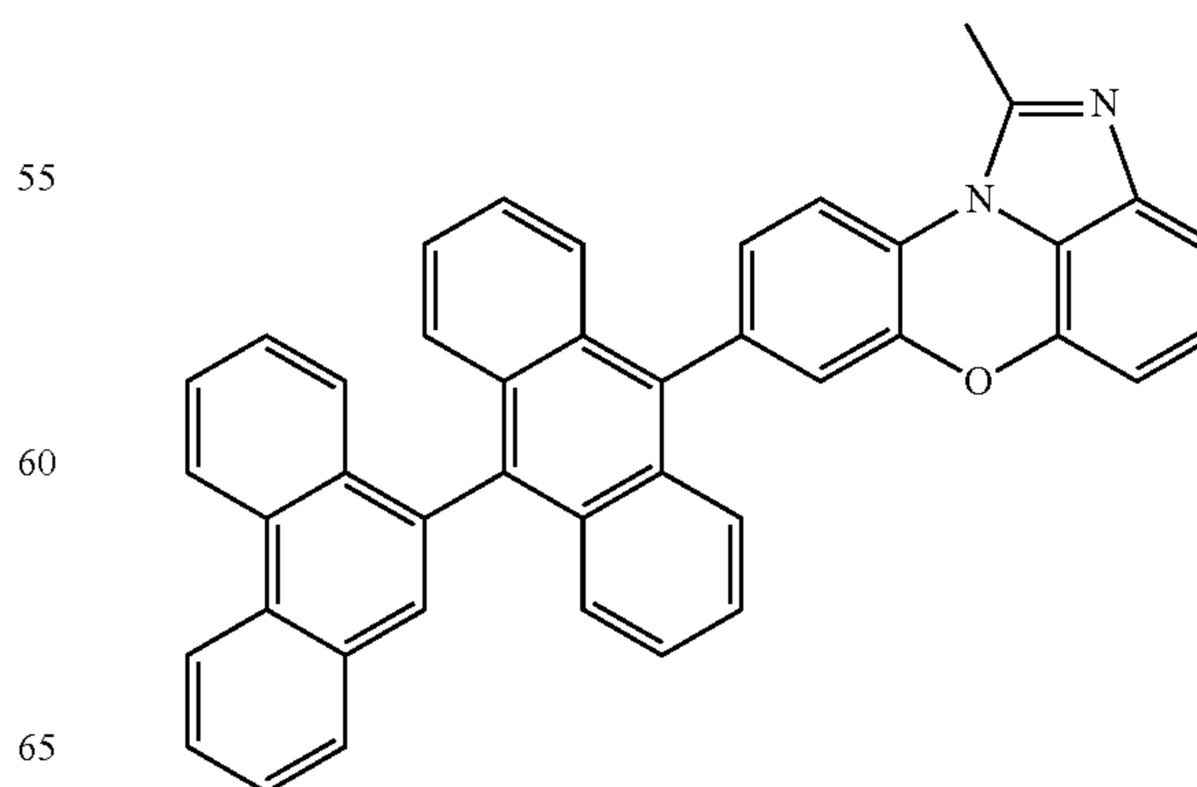
[Chemical Formula 1-2-7]
