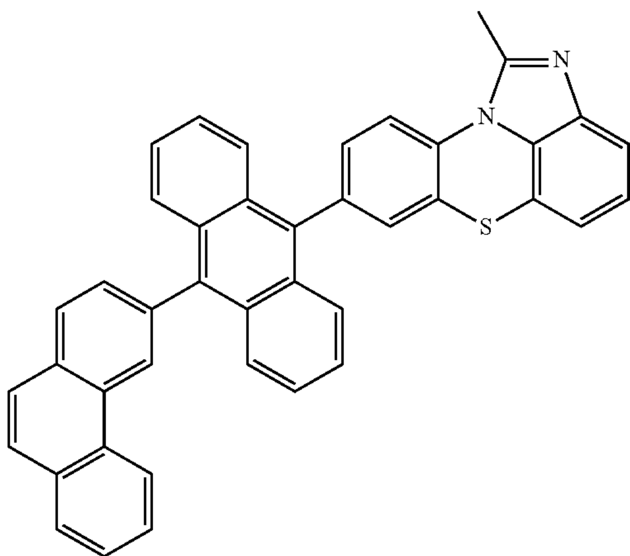
[Chemical Formula 2-2-8]
