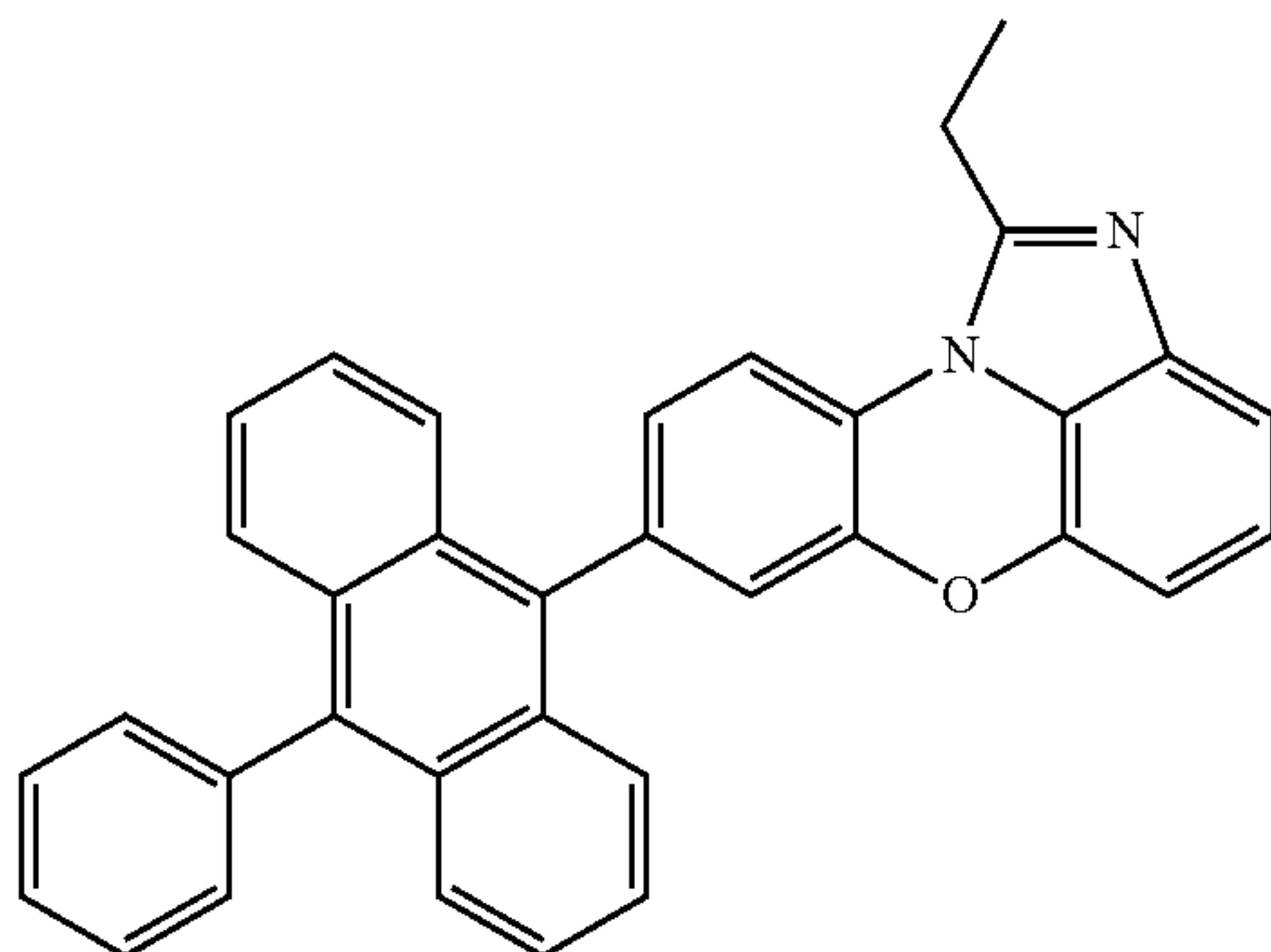
[Chemical Formula 1-3-1]
