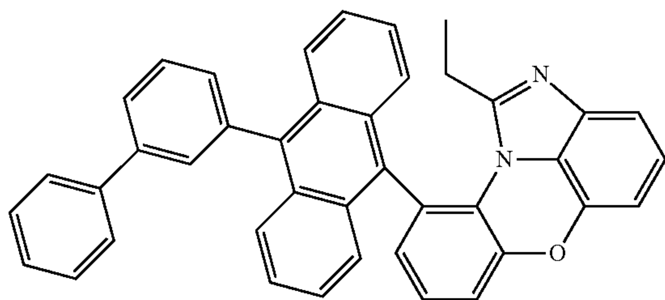
[Chemical Formula 1-8-6]
