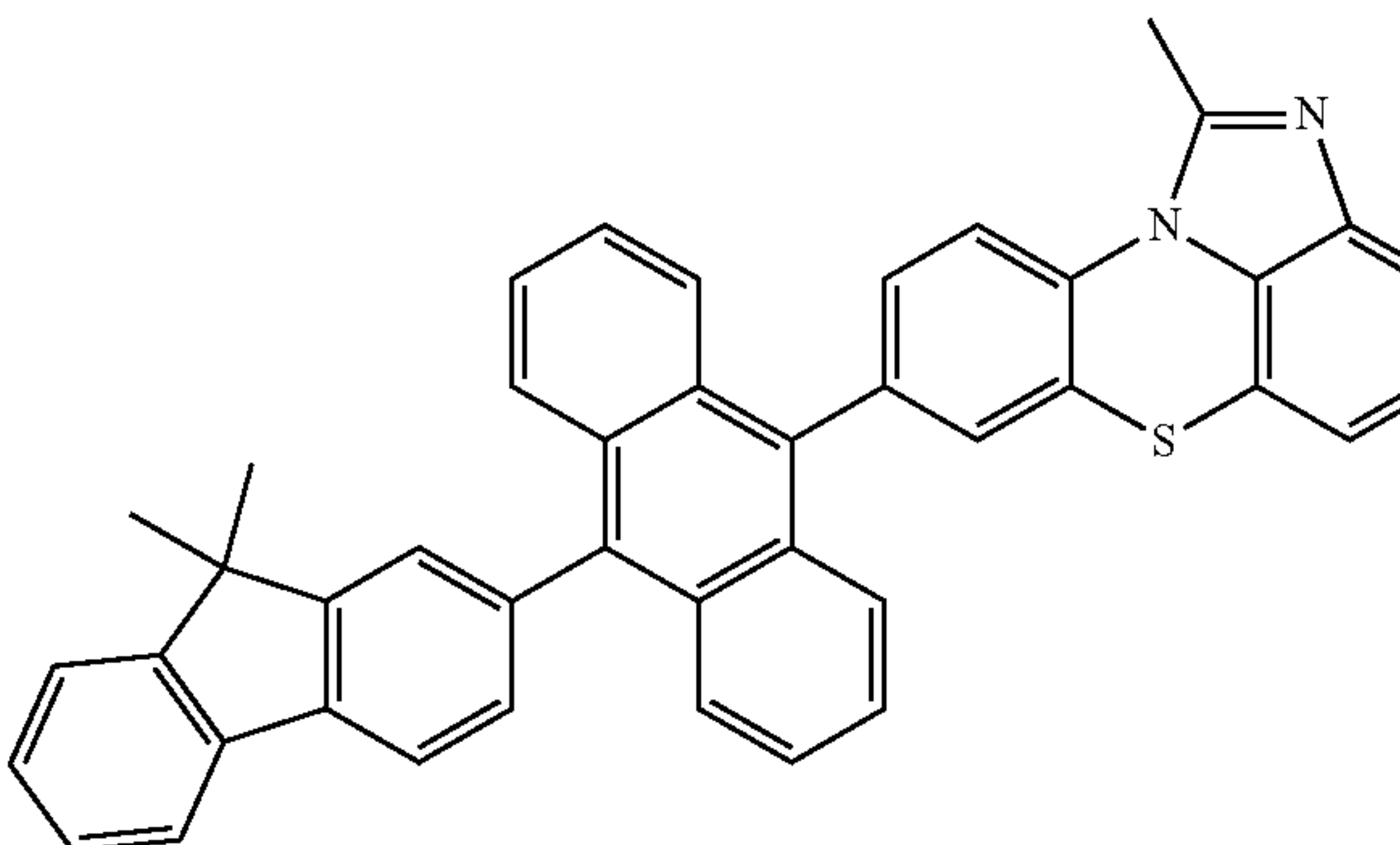
[Chemical Formula 2-2-5]
