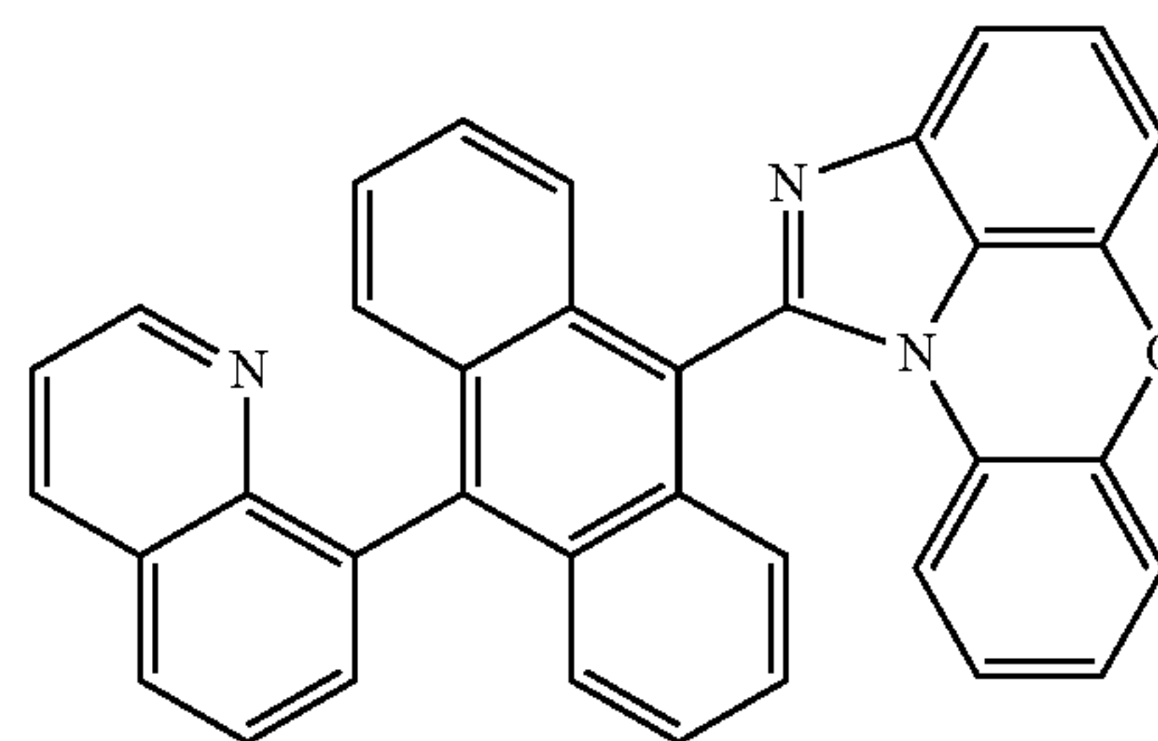
[Chemical Formula 1-1-20]
