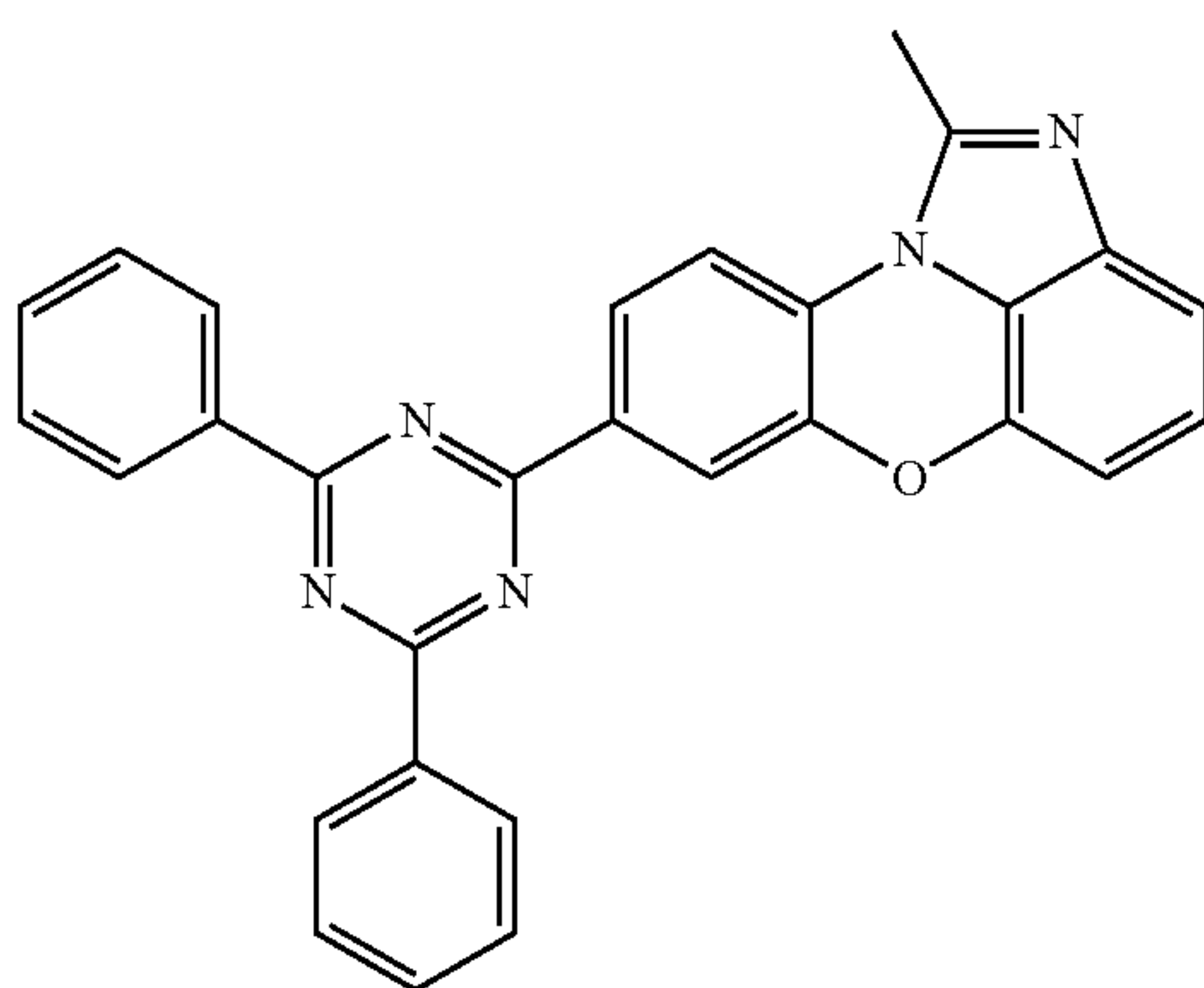
[Chemical Formula 1-2-42]
