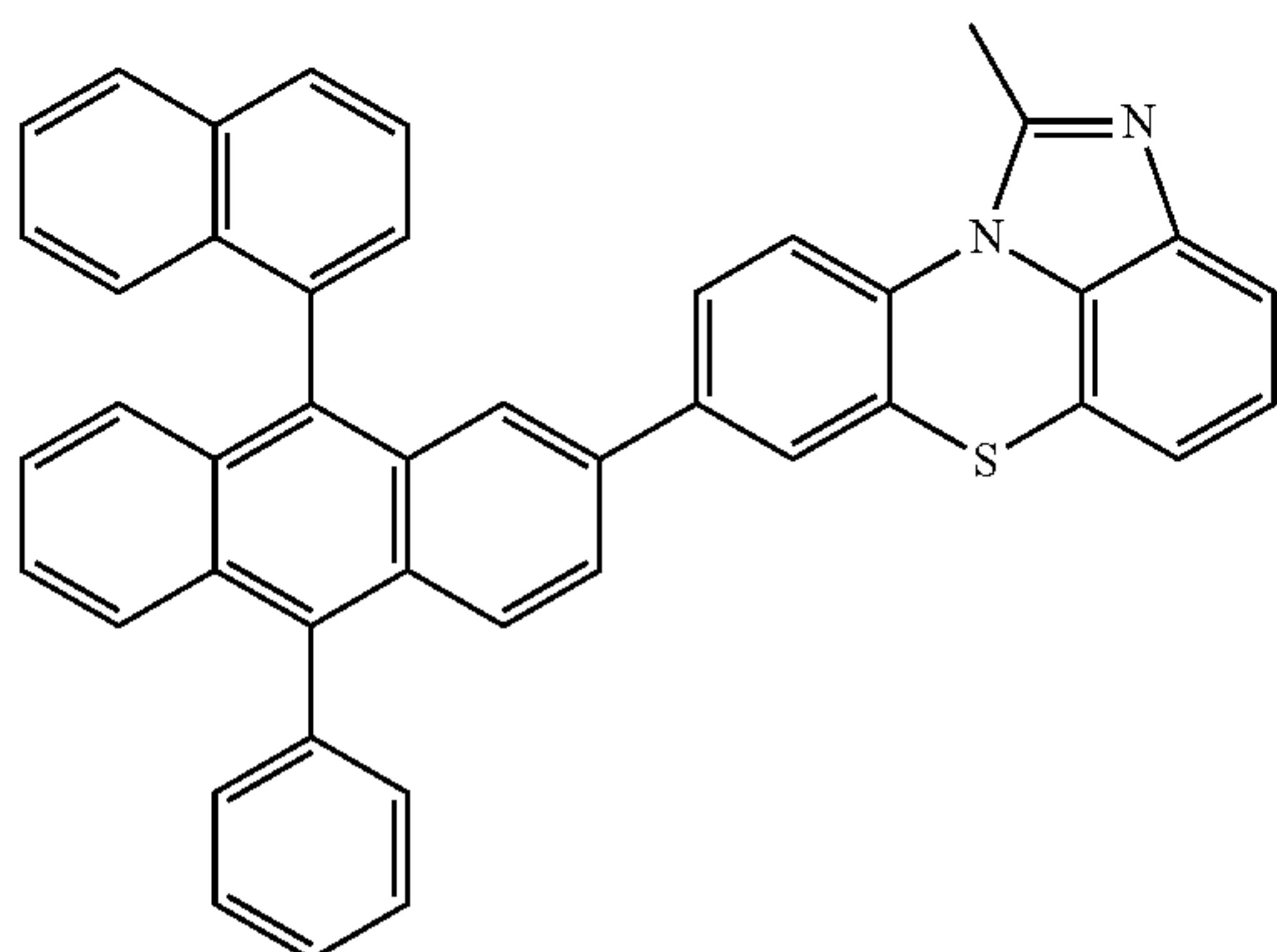
[Chemical Formula 2-2-22]
