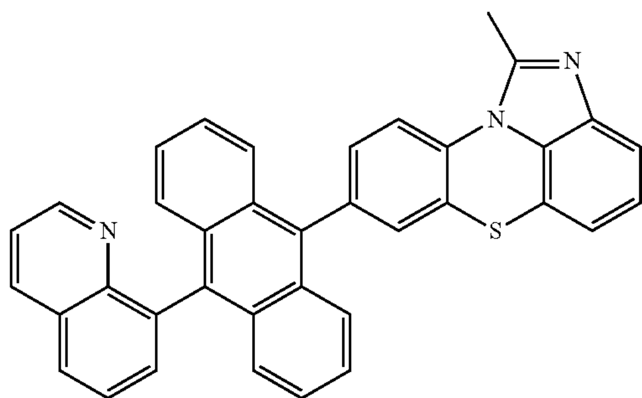
[Chemical Formula 2-2-11]
