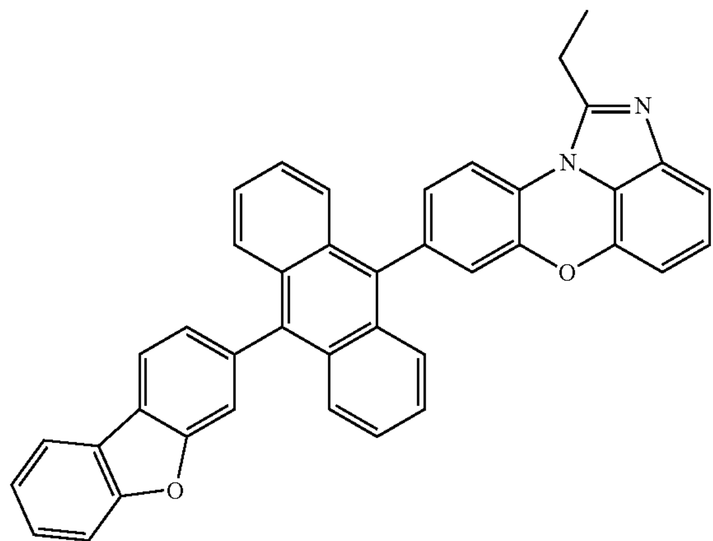
[Chemical Formula 1-3-14]
