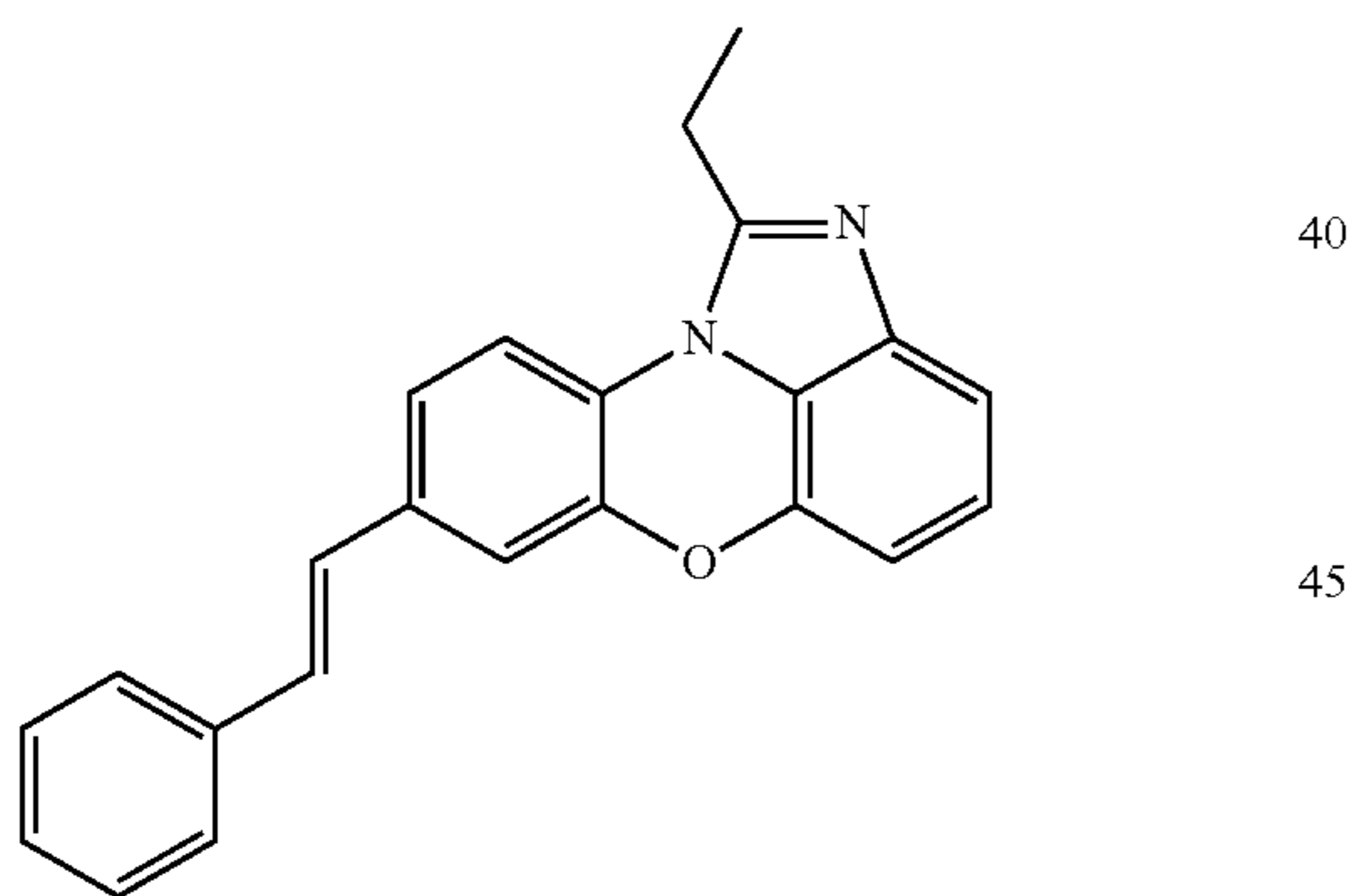
[Chemical Formula 1-4-1]
