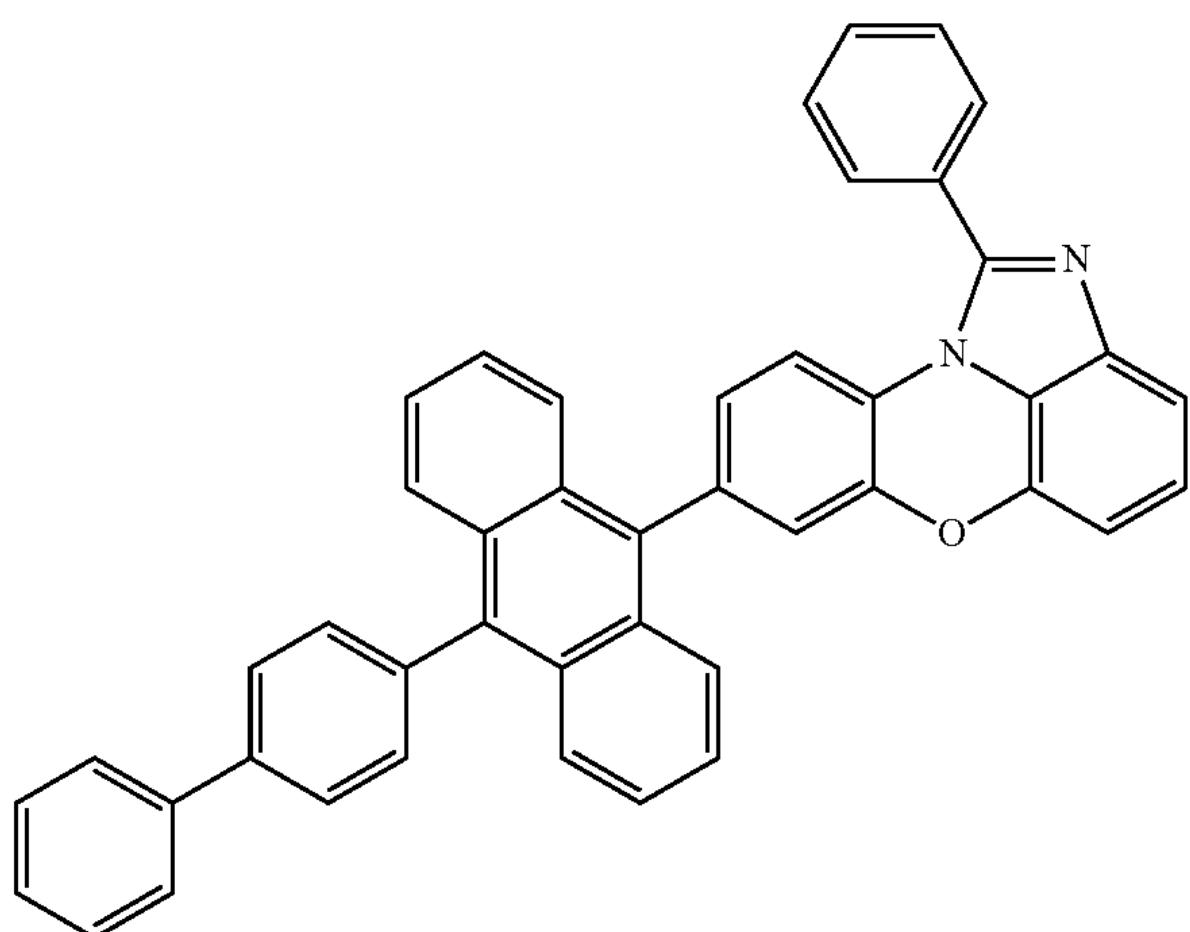
[Chemical Formula 1-4-4]
