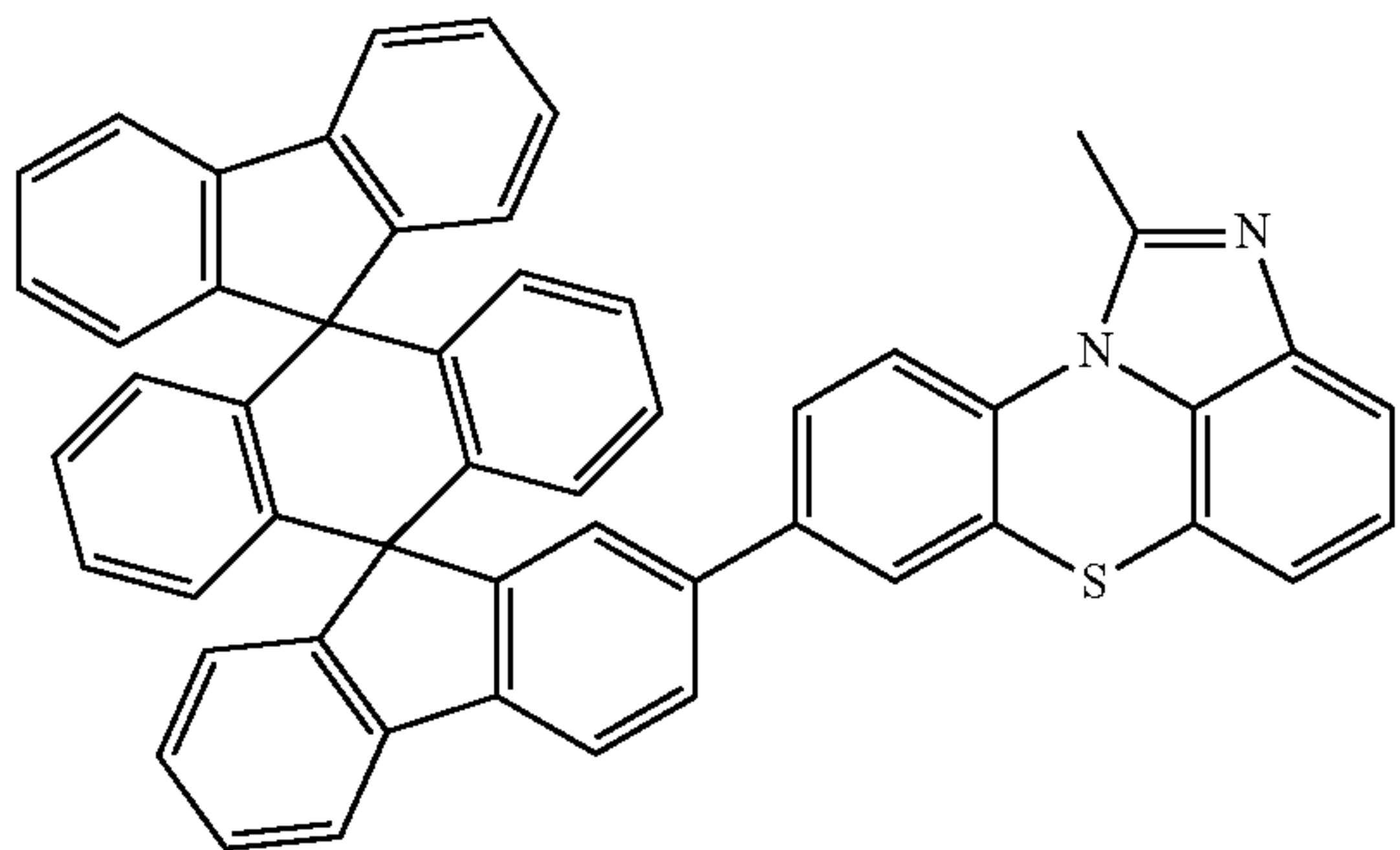
[Chemical Formula 2-2-36]
