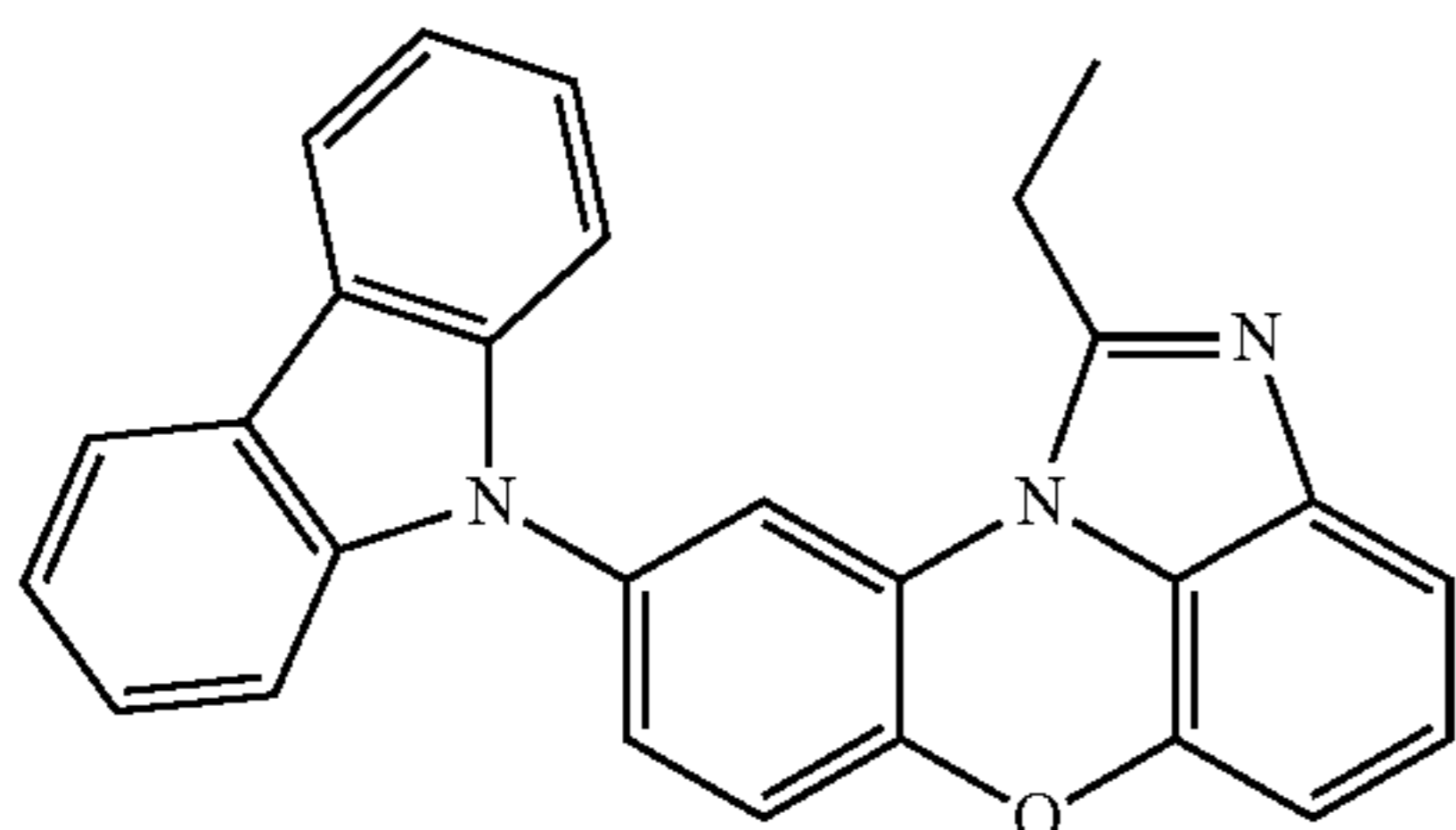
[Chemical Formula 1-7-50]
