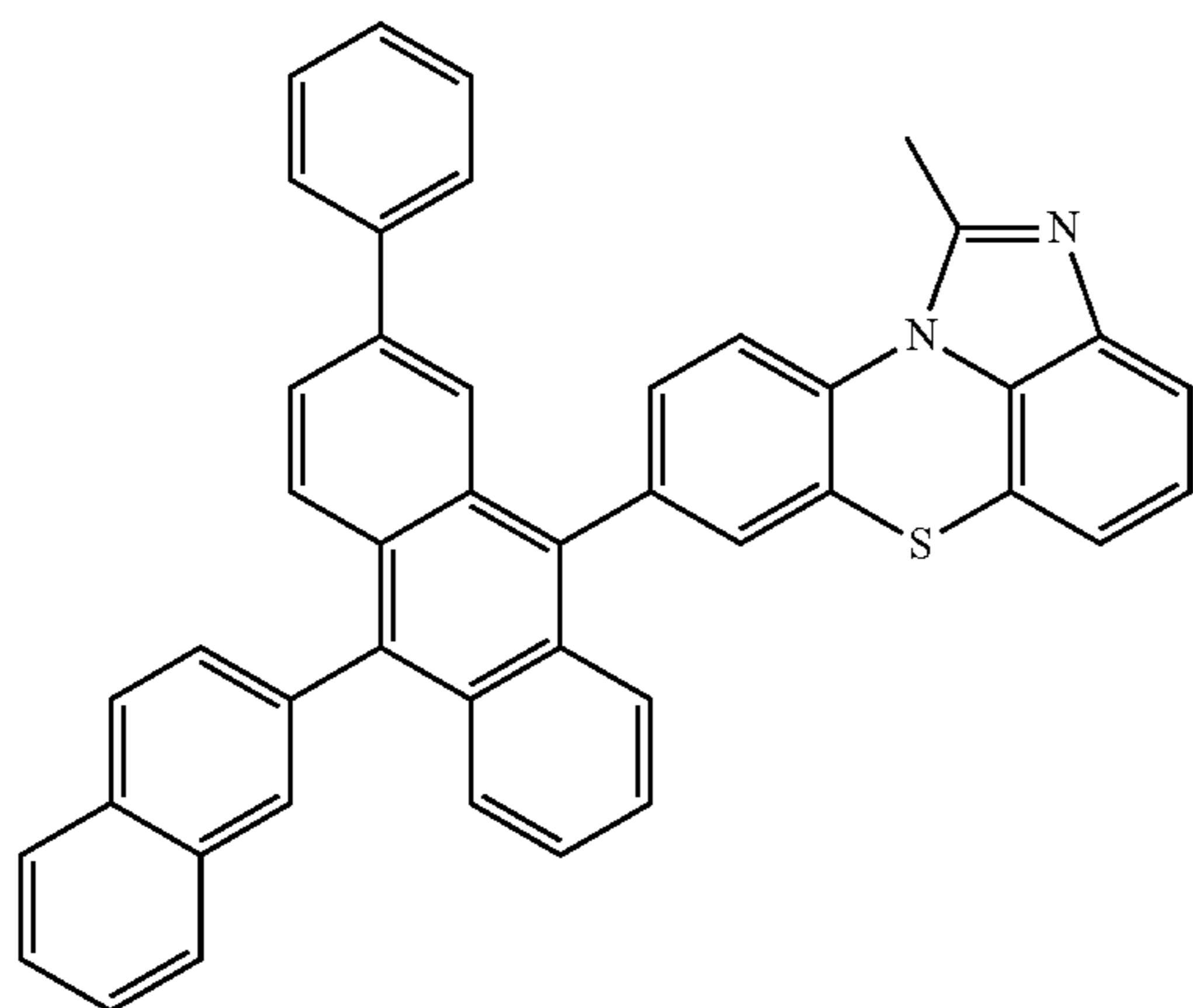
[Chemical Formula 2-2-16]
