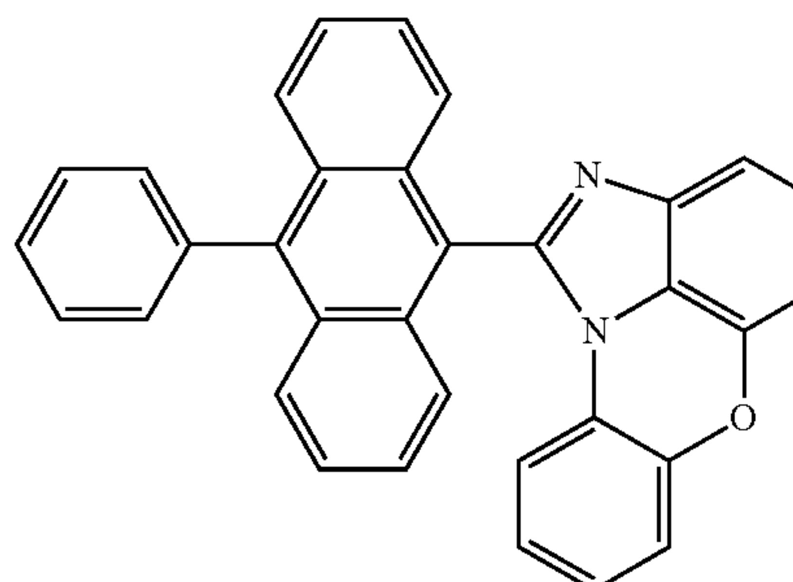
[Chemical Formula 1-1-10]
