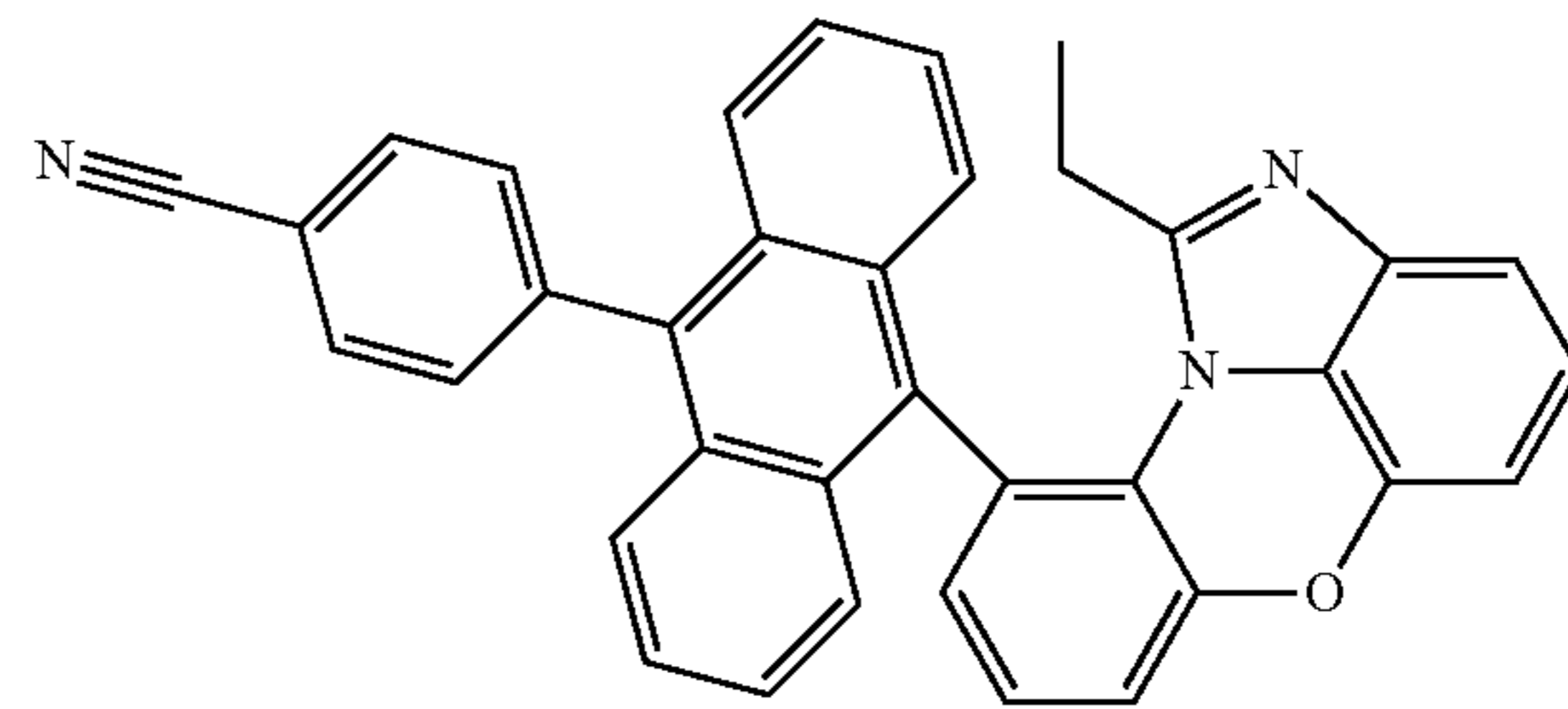
[Chemical Formula 1-8-12]
