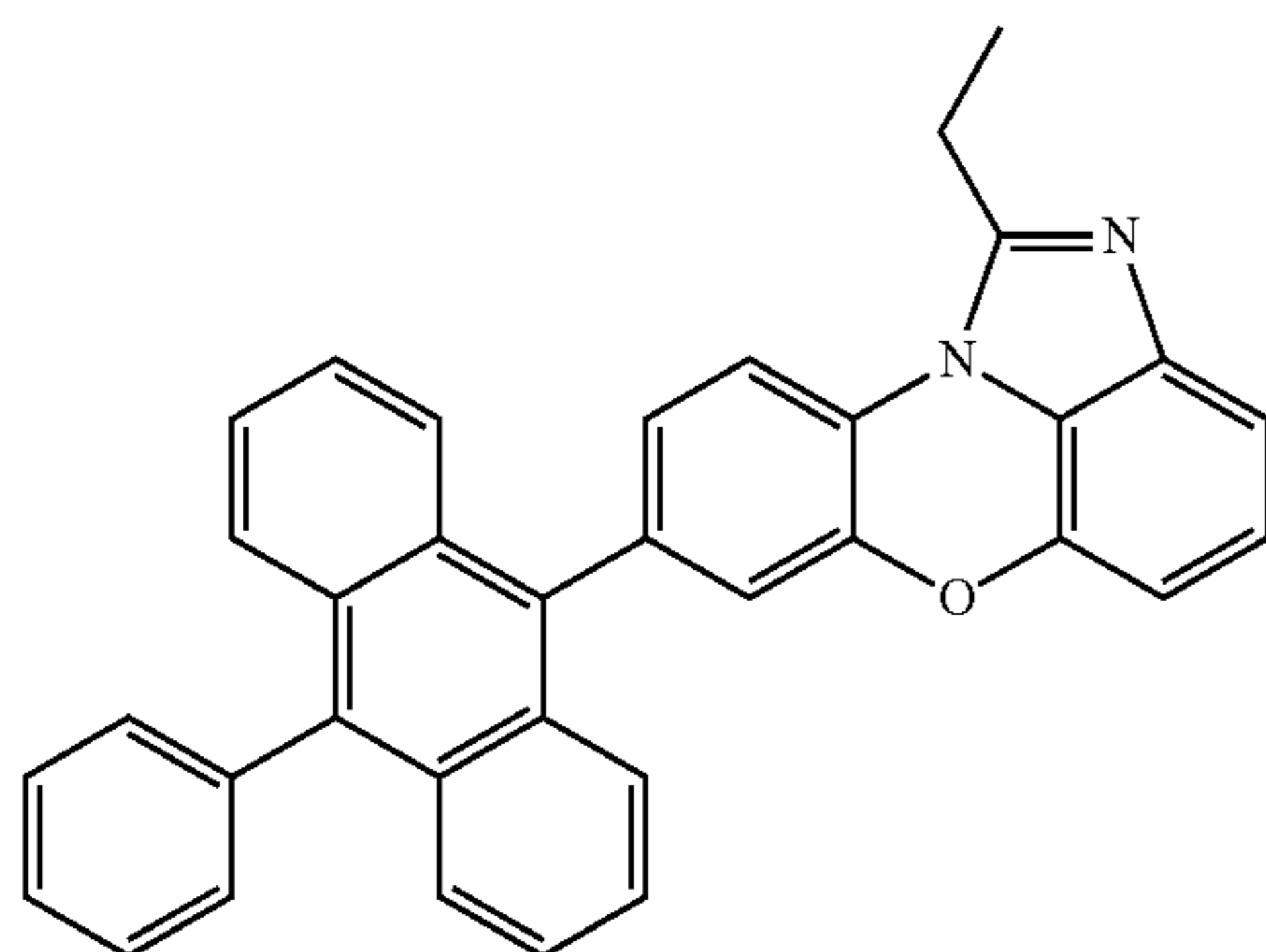
[Chemical Formula 1-3-1]
