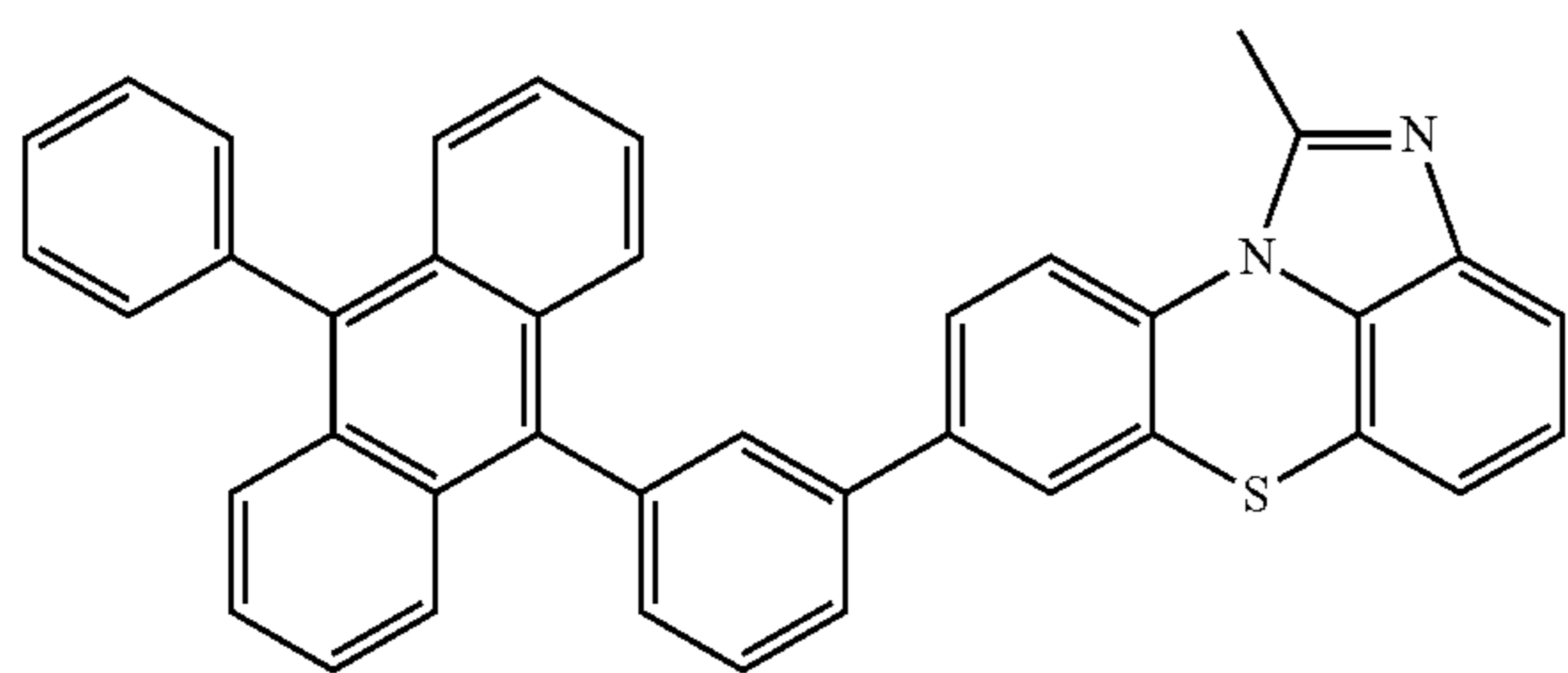
[Chemical Formula 2-2-19]
