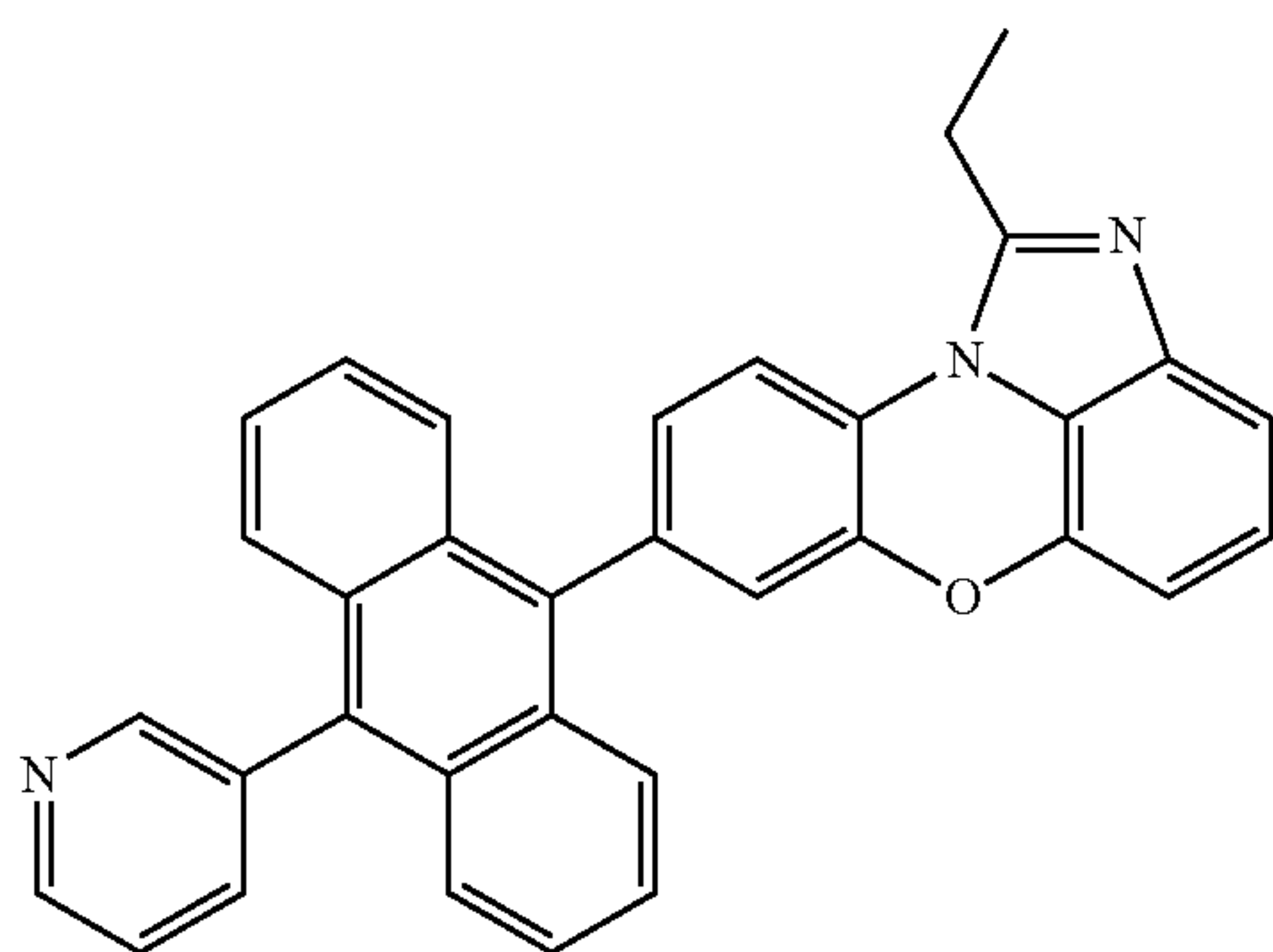
[Chemical Formula 1-3-10]
