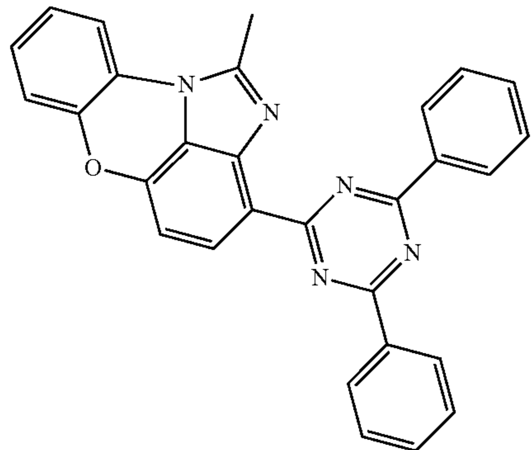
[Chemical Formula 1-11-5]
