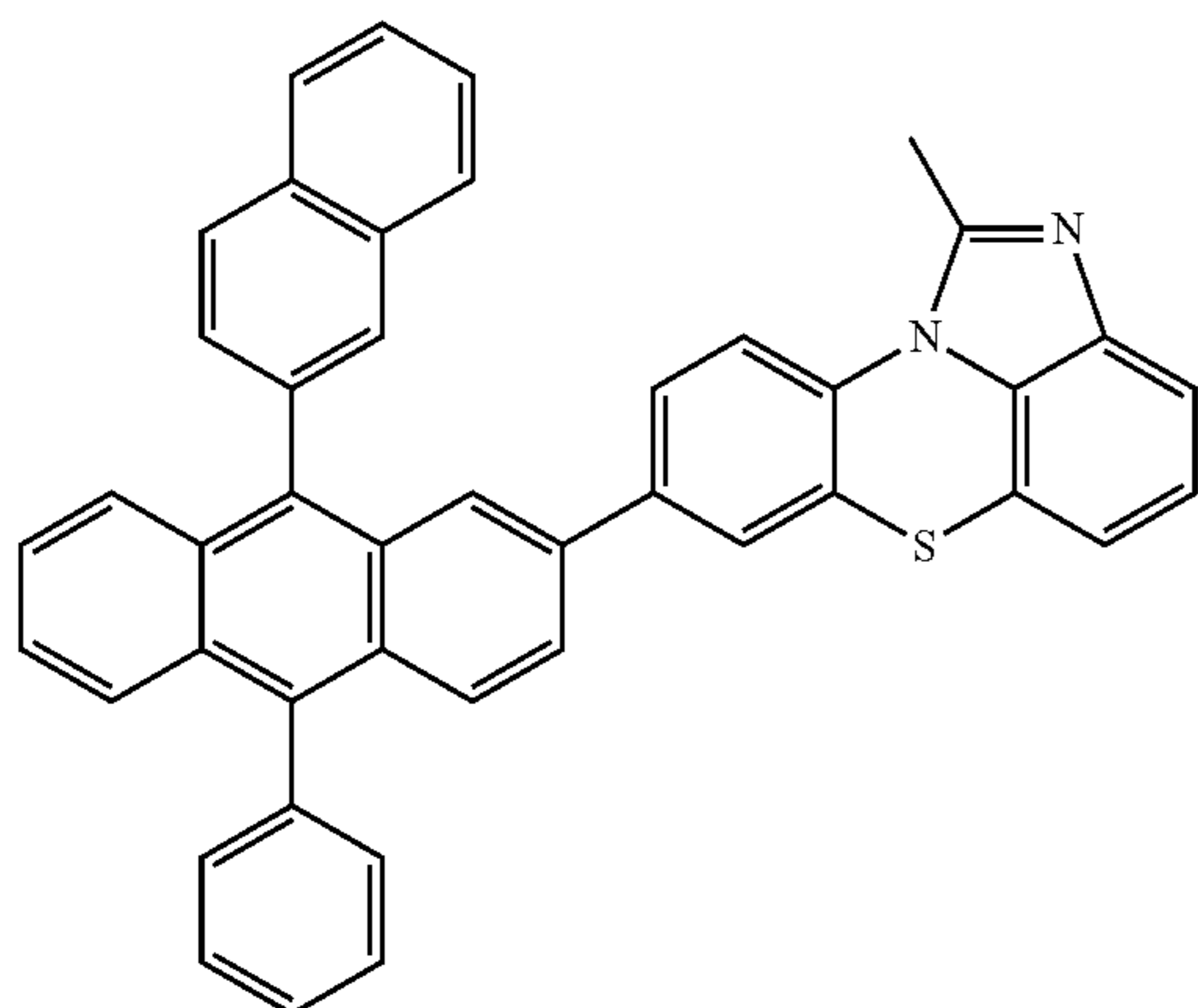
[Chemical Formula 2-2-23]
