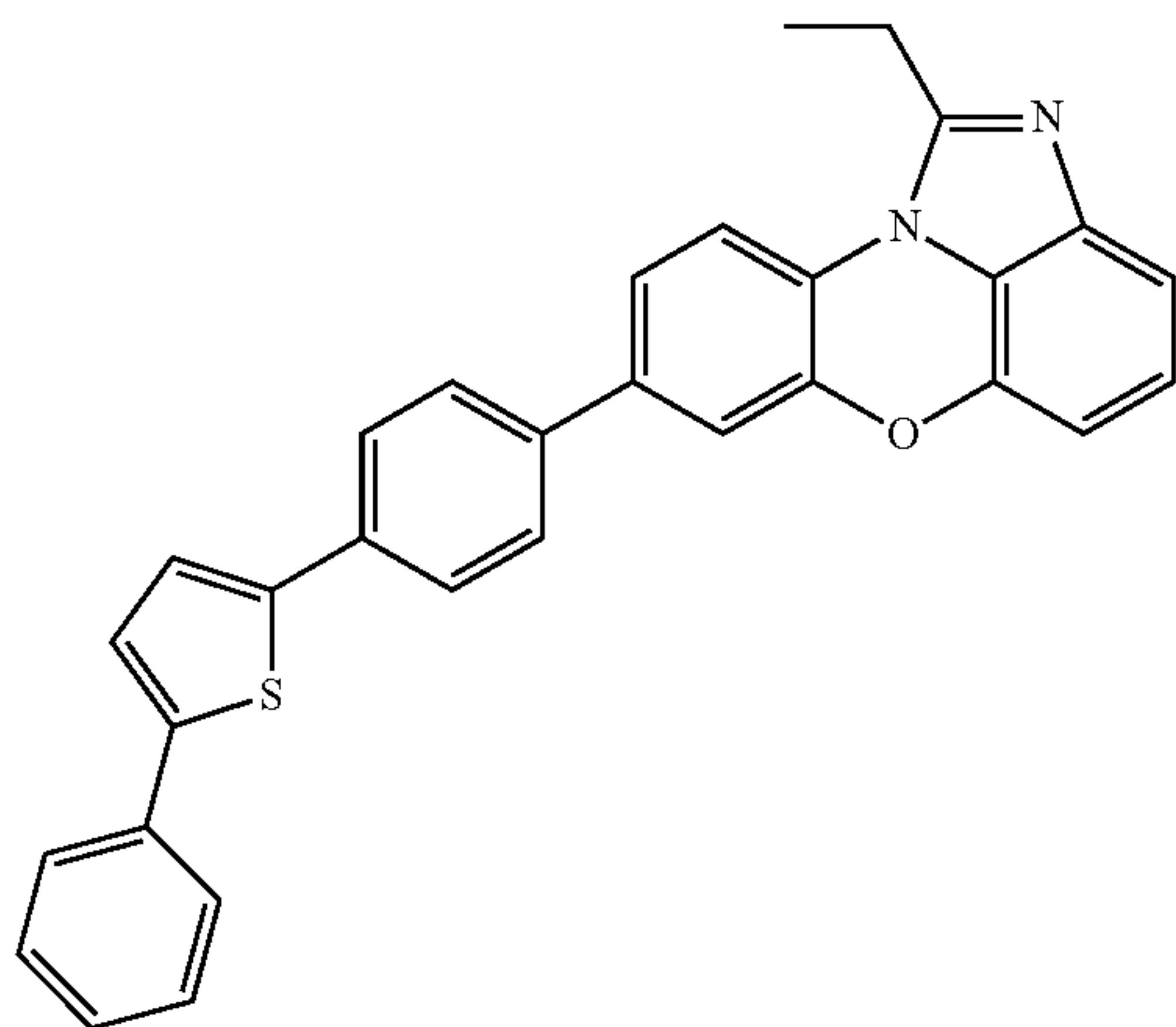
[Chemical Formula 1-3-39]
