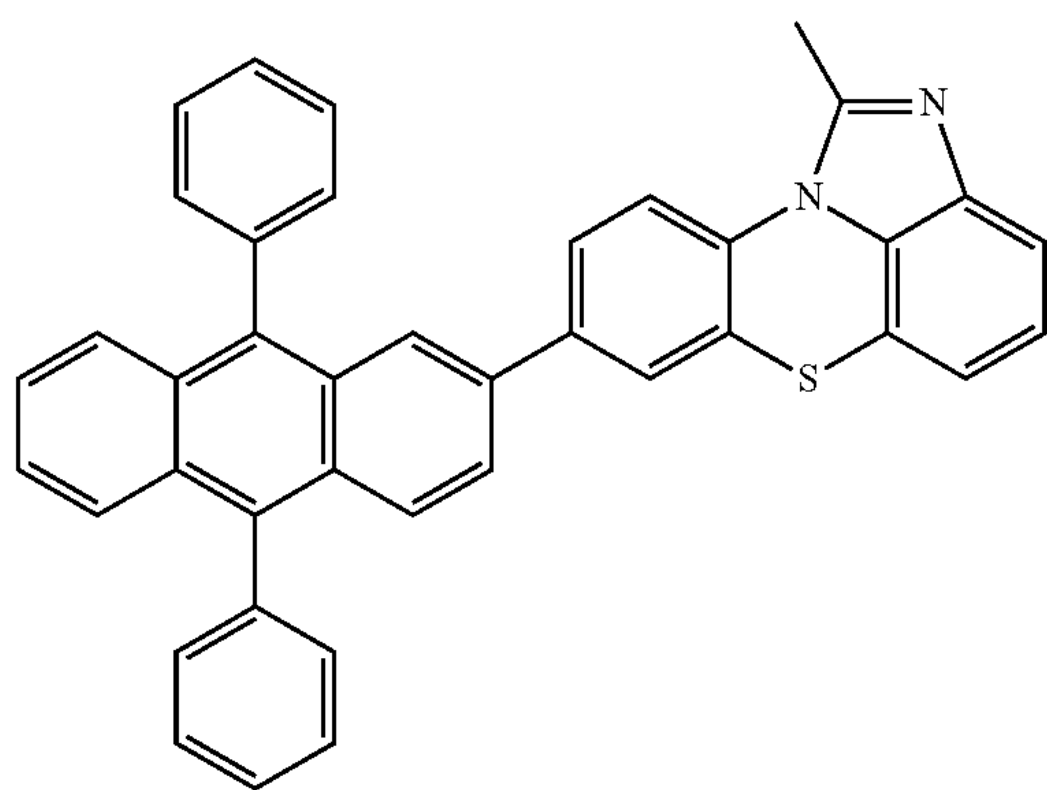
[Chemical Formula 2-2-20]
