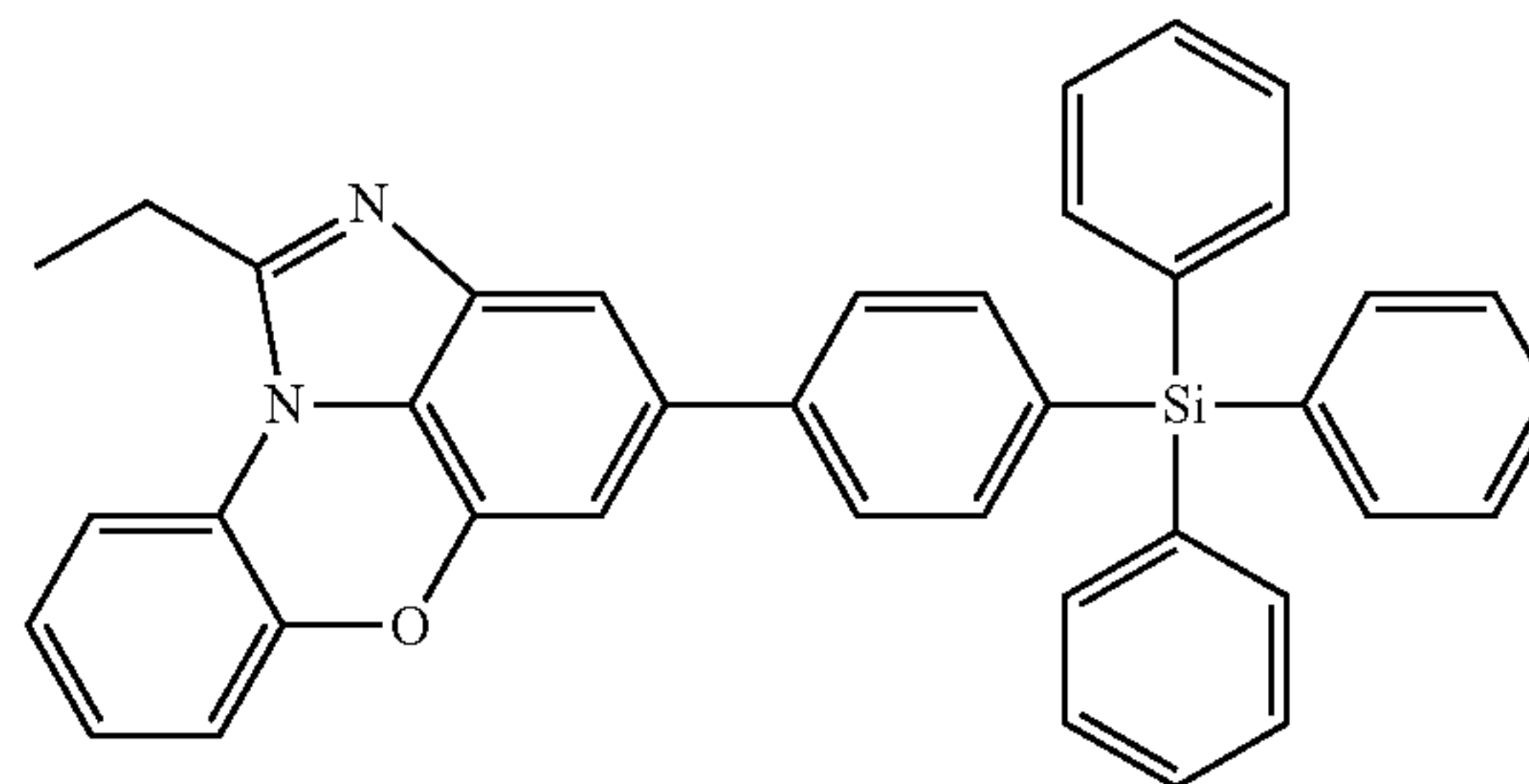
[Chemical Formula 1-10-12]
