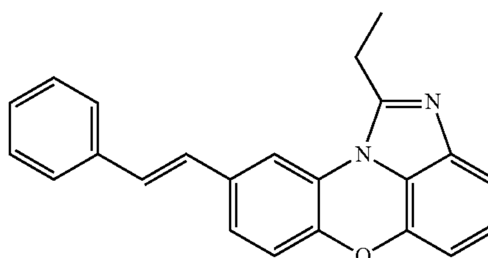
[Chemical Formula 1-8-1]
