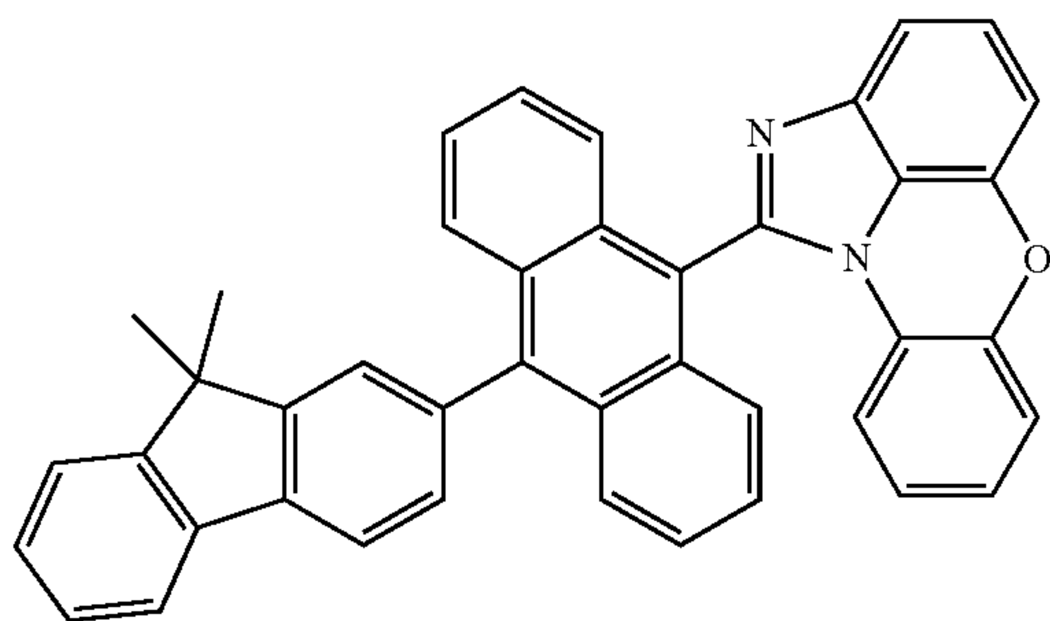
[Chemical Formula 1-1-13]
