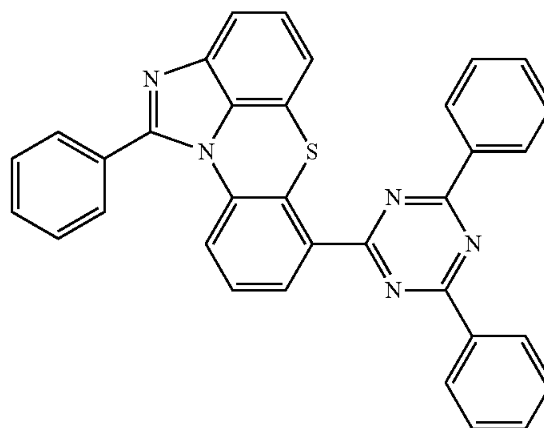
[Chemical Formula 2-2-41]
