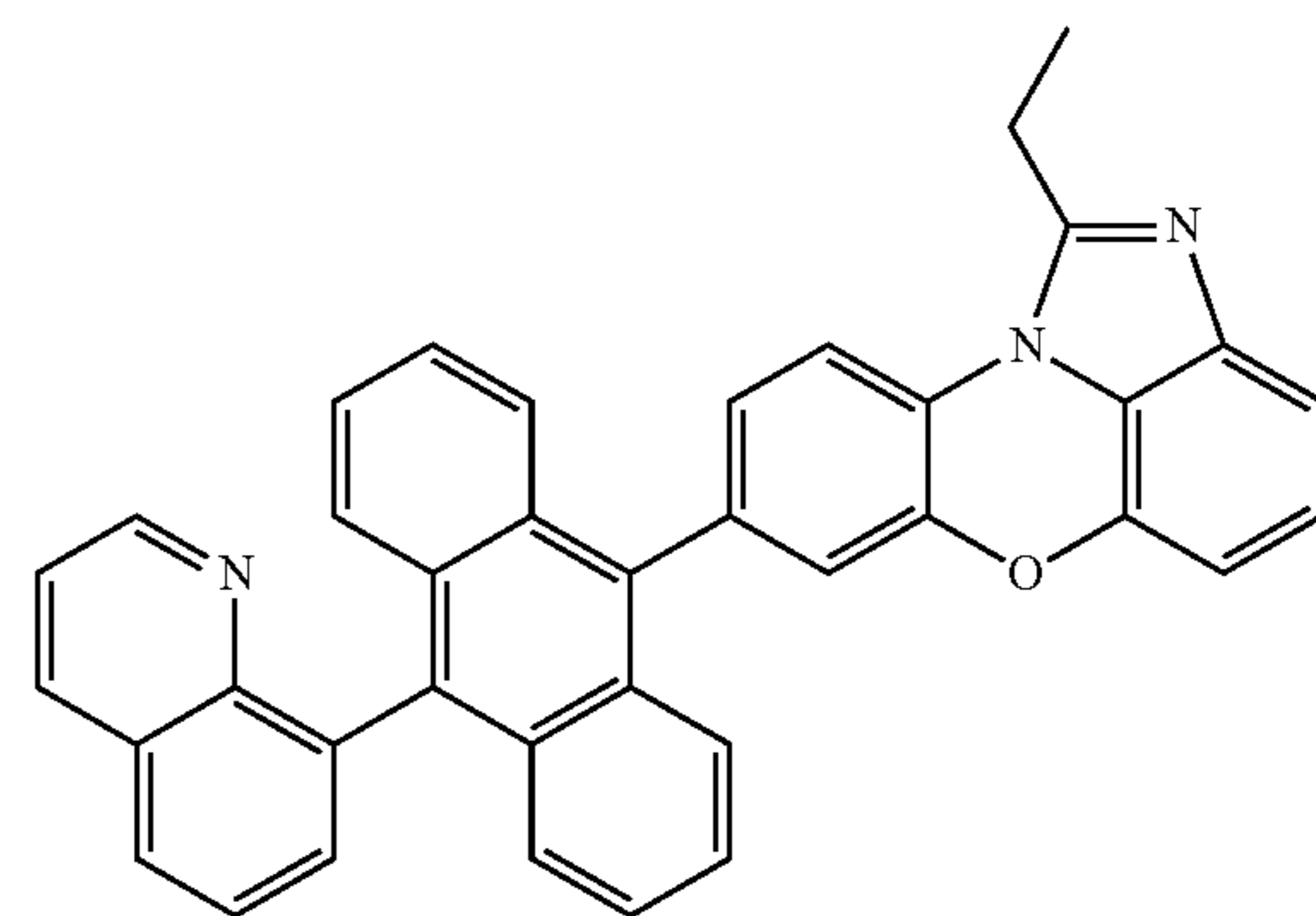
[Chemical Formula 1-3-11]
