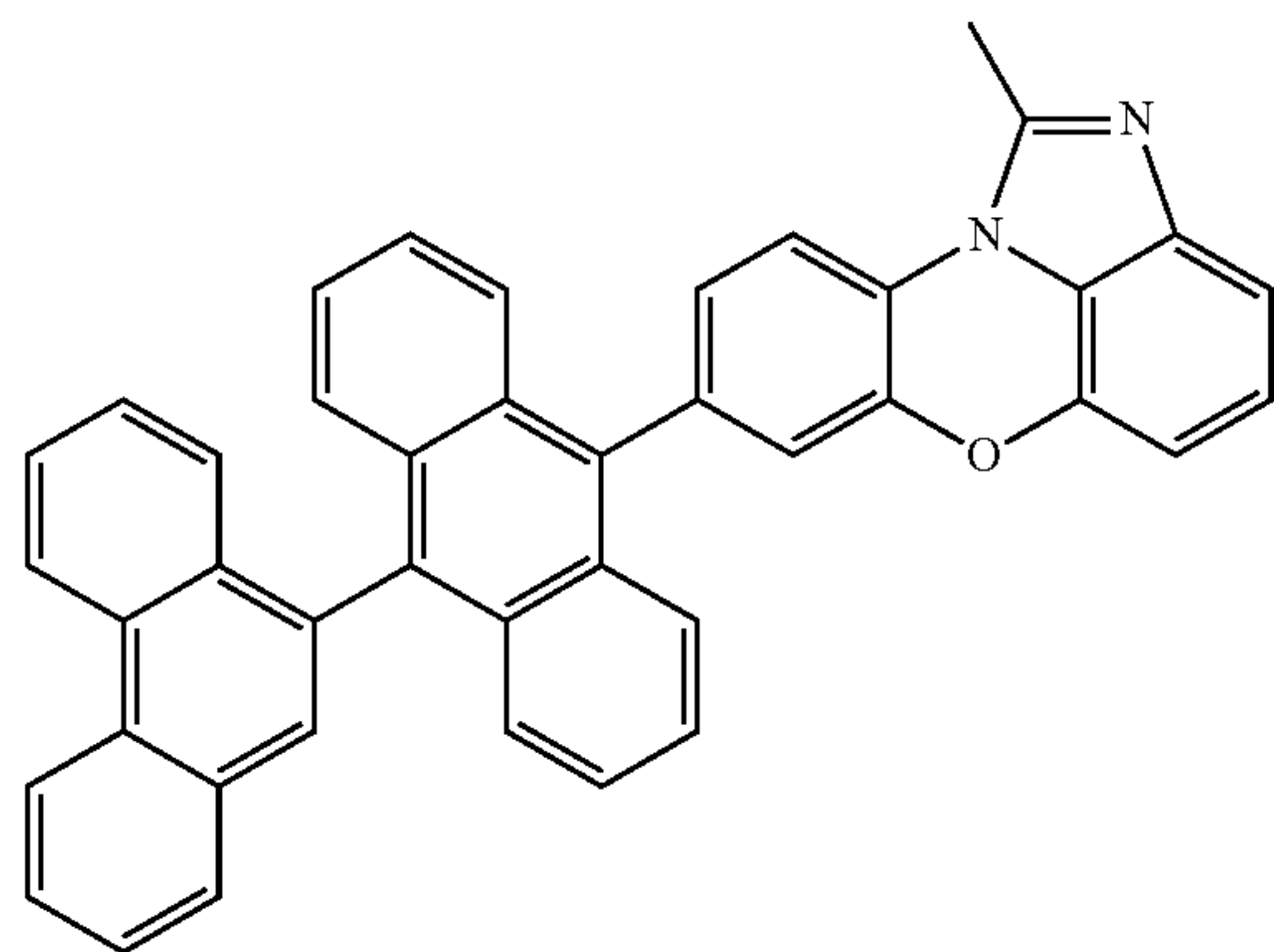
[Chemical Formula 1-2-7]
