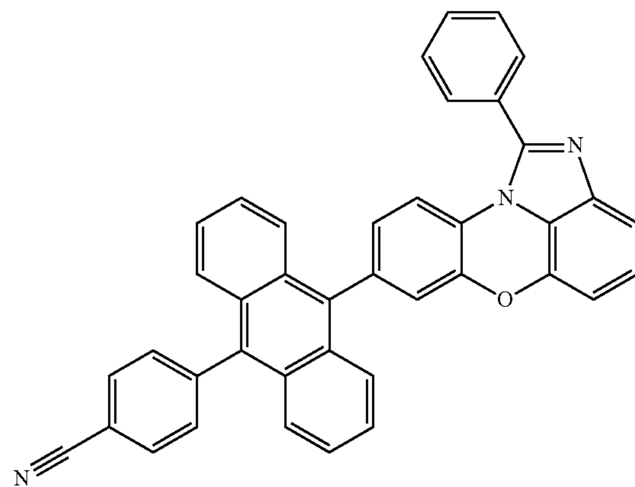
[Chemical Formula 1-4-12]
