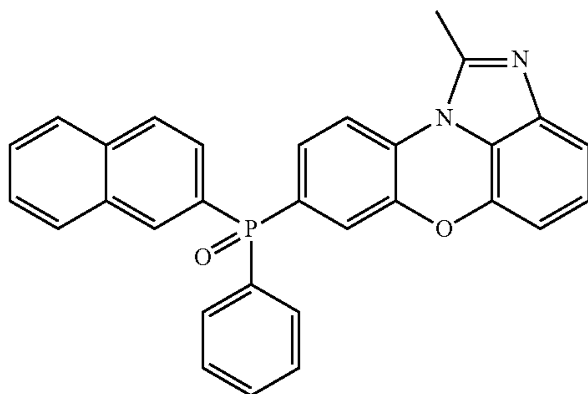
[Chemical Formula 1-5-3]
