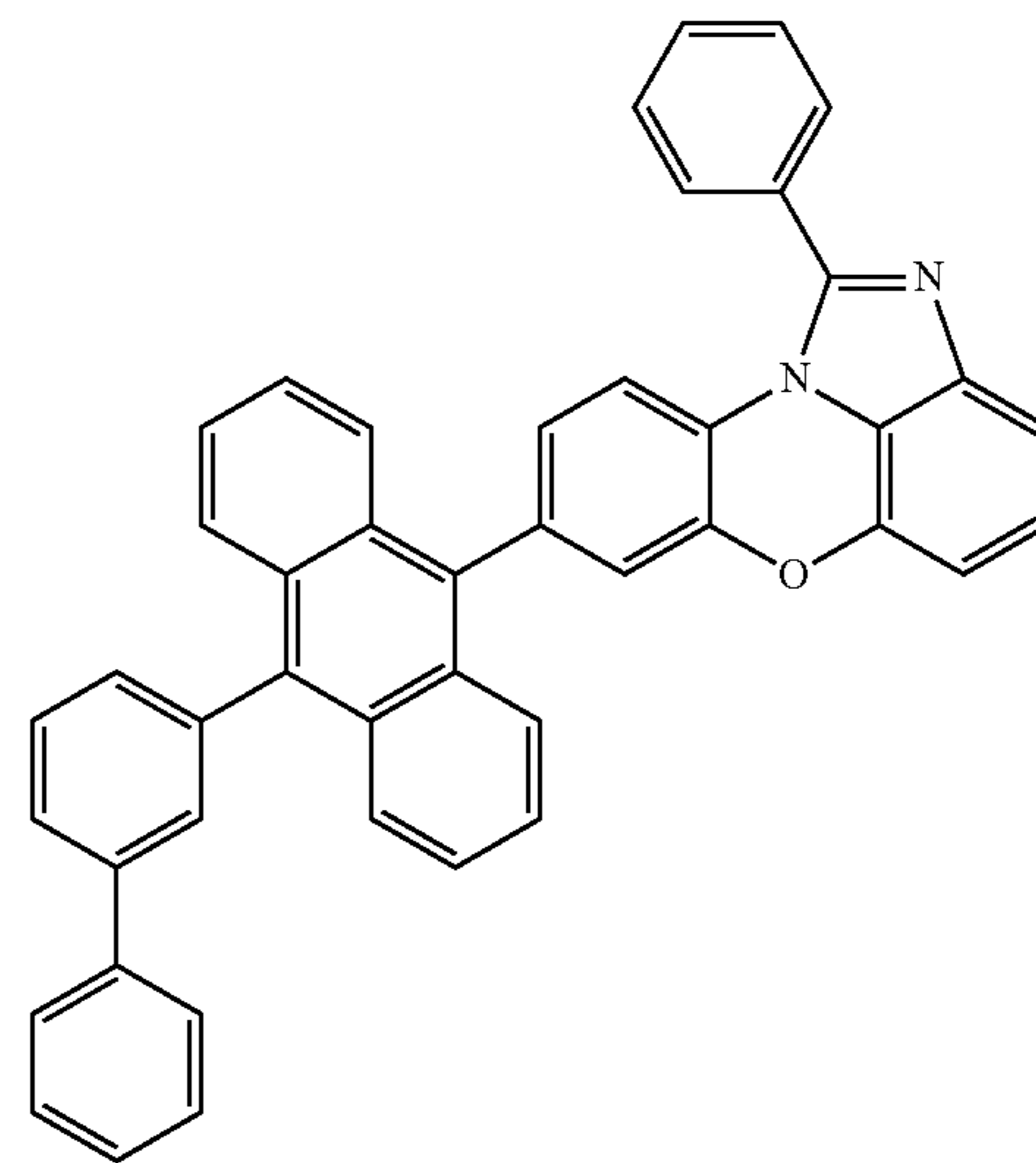
[Chemical Formula 1-4-6]
