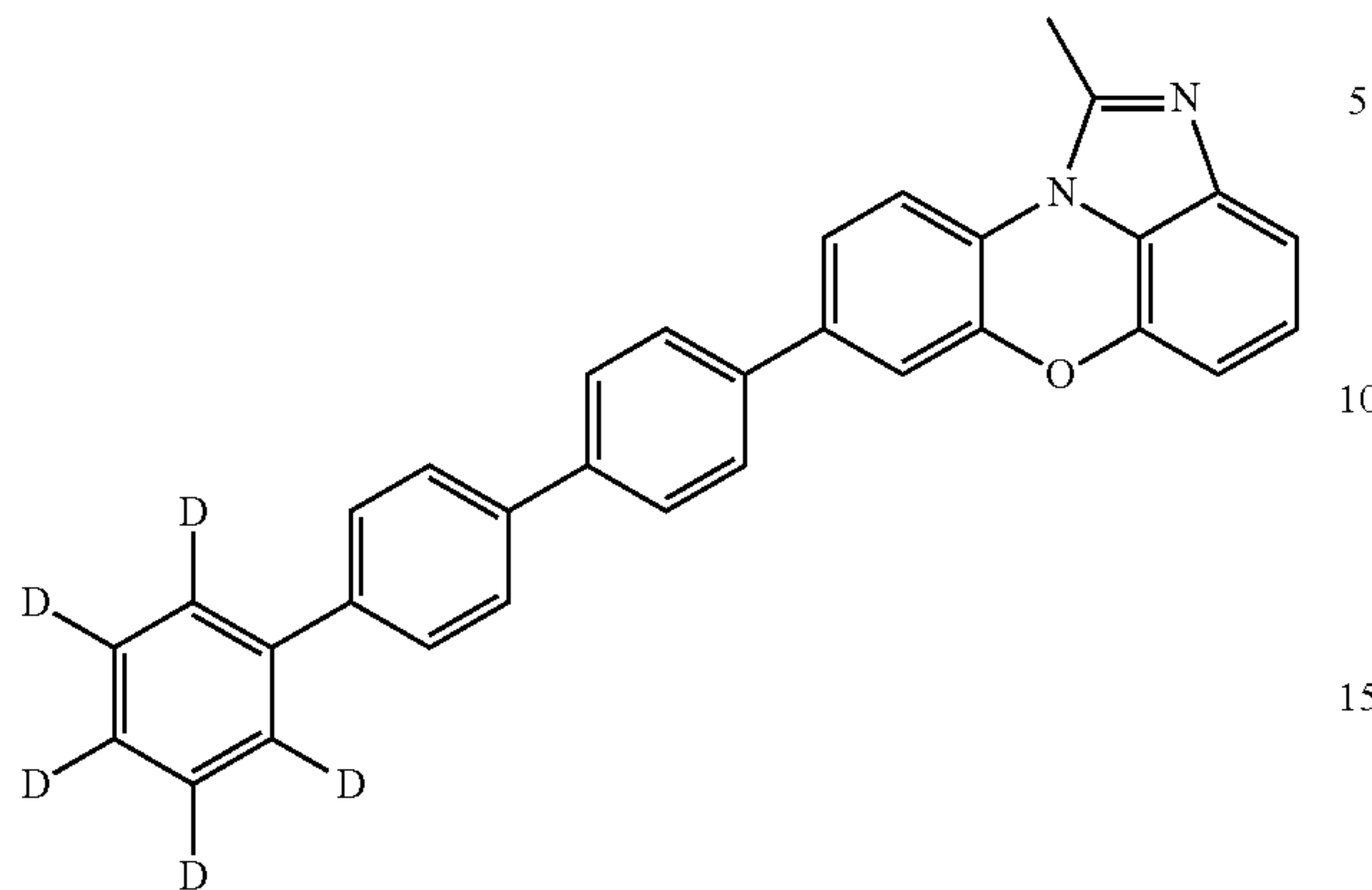
[Chemical Formula 1-2-52]
