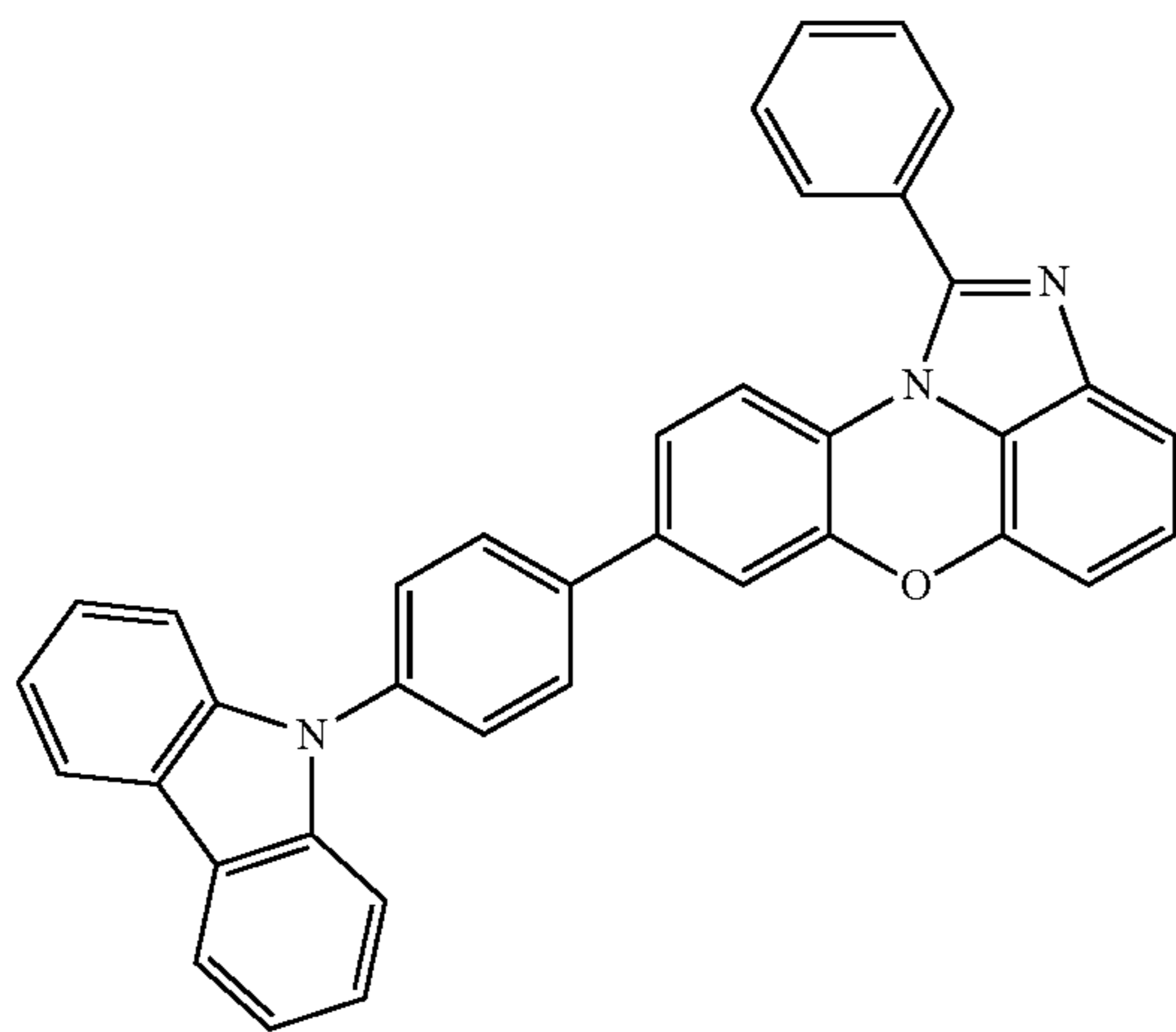
[Chemical Formula 1-4-42]
