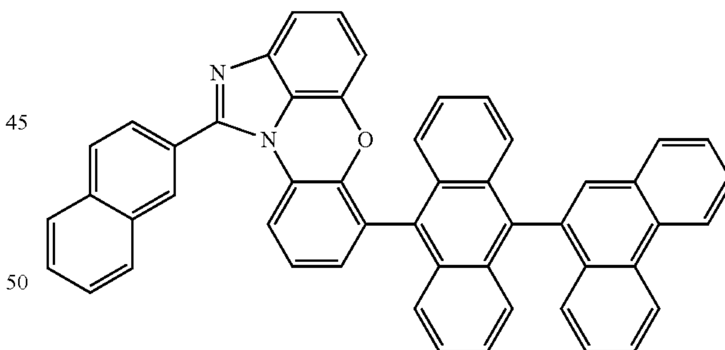
[Chemical Formula 1-6-8]
