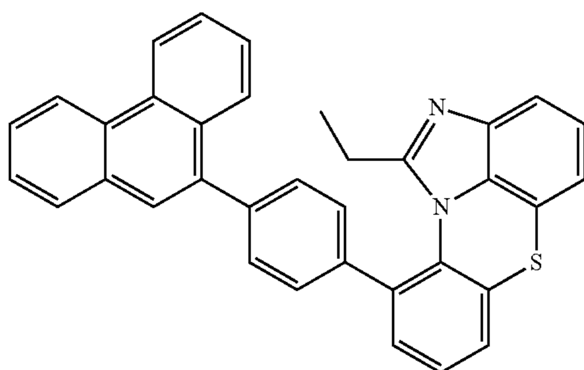
[Chemical Formula 2-3-32]
