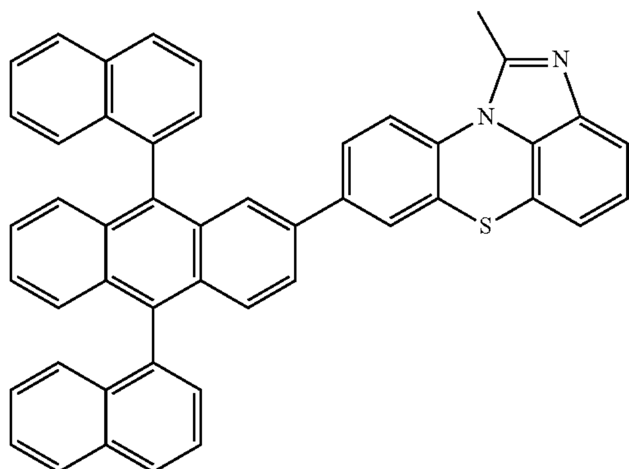
[Chemical Formula 2-2-21]
