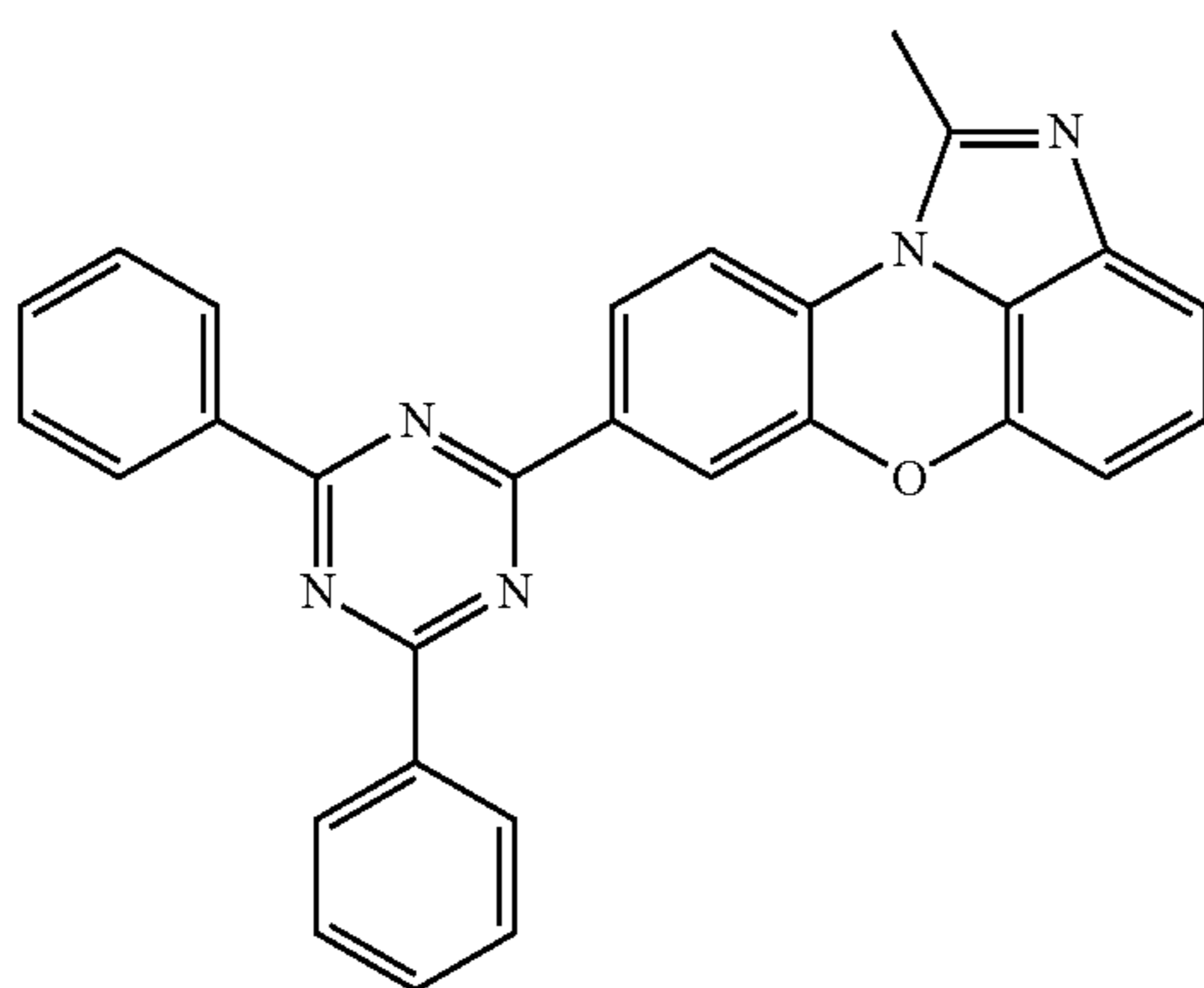
[Chemical Formula 1-2-42]
