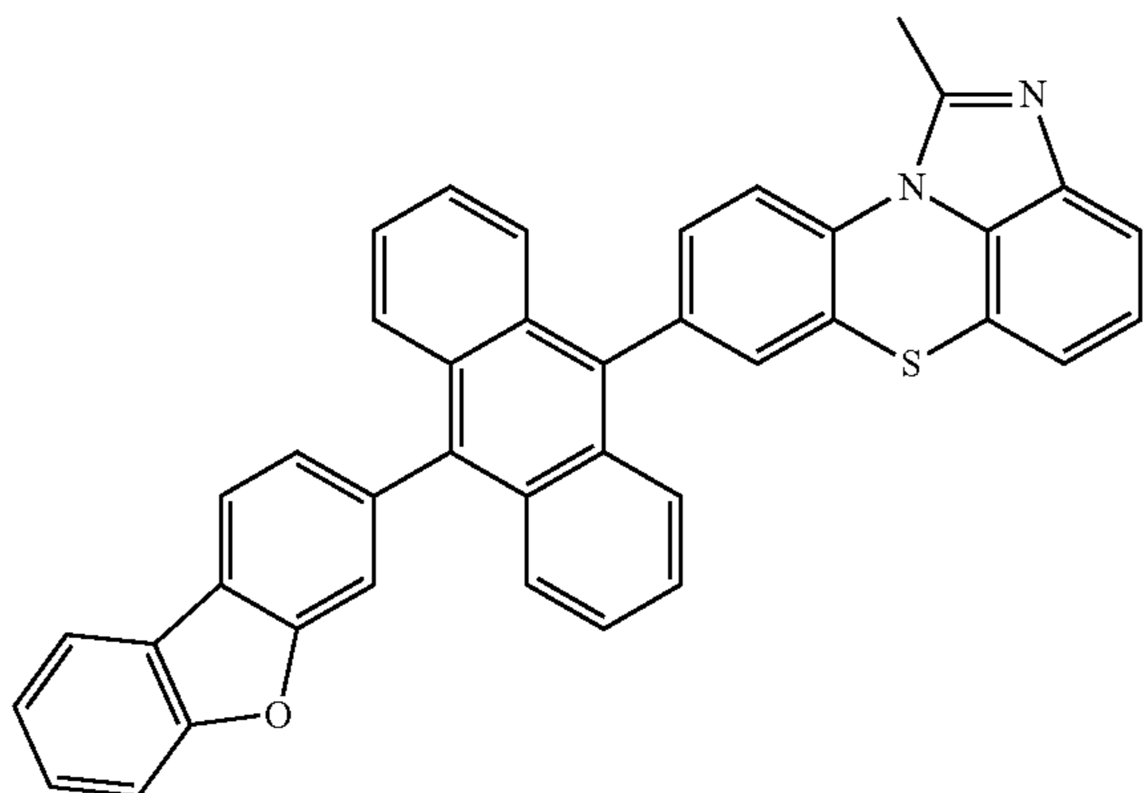
[Chemical Formula 2-2-14]
