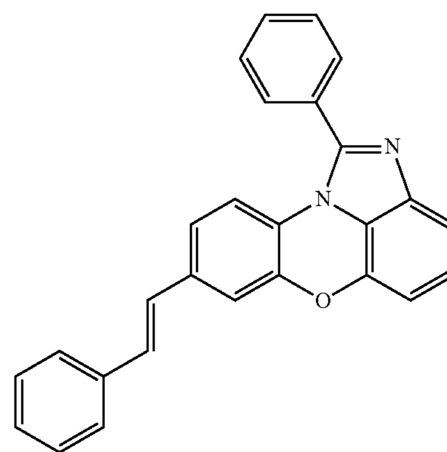
[Chemical Formula 1-4-54]
