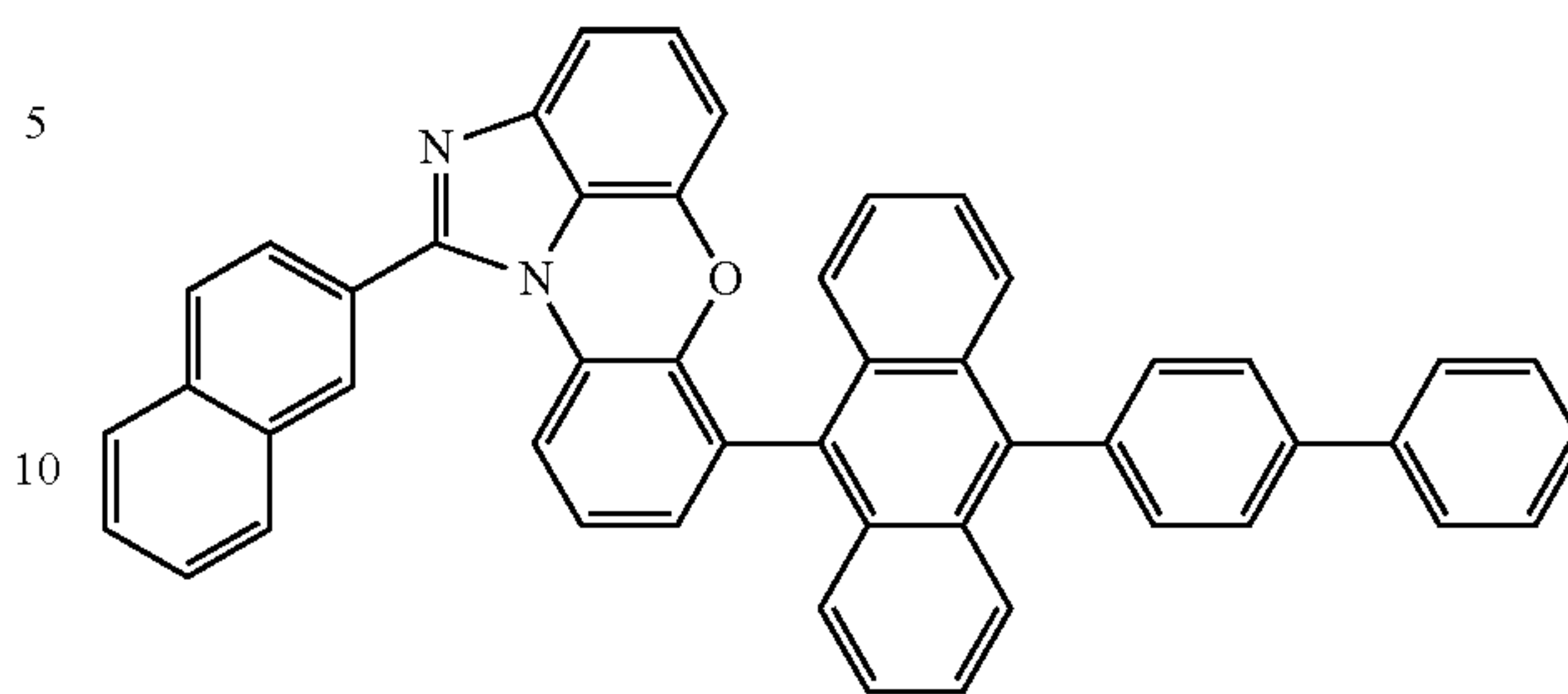
[Chemical Formula 1-6-5]
