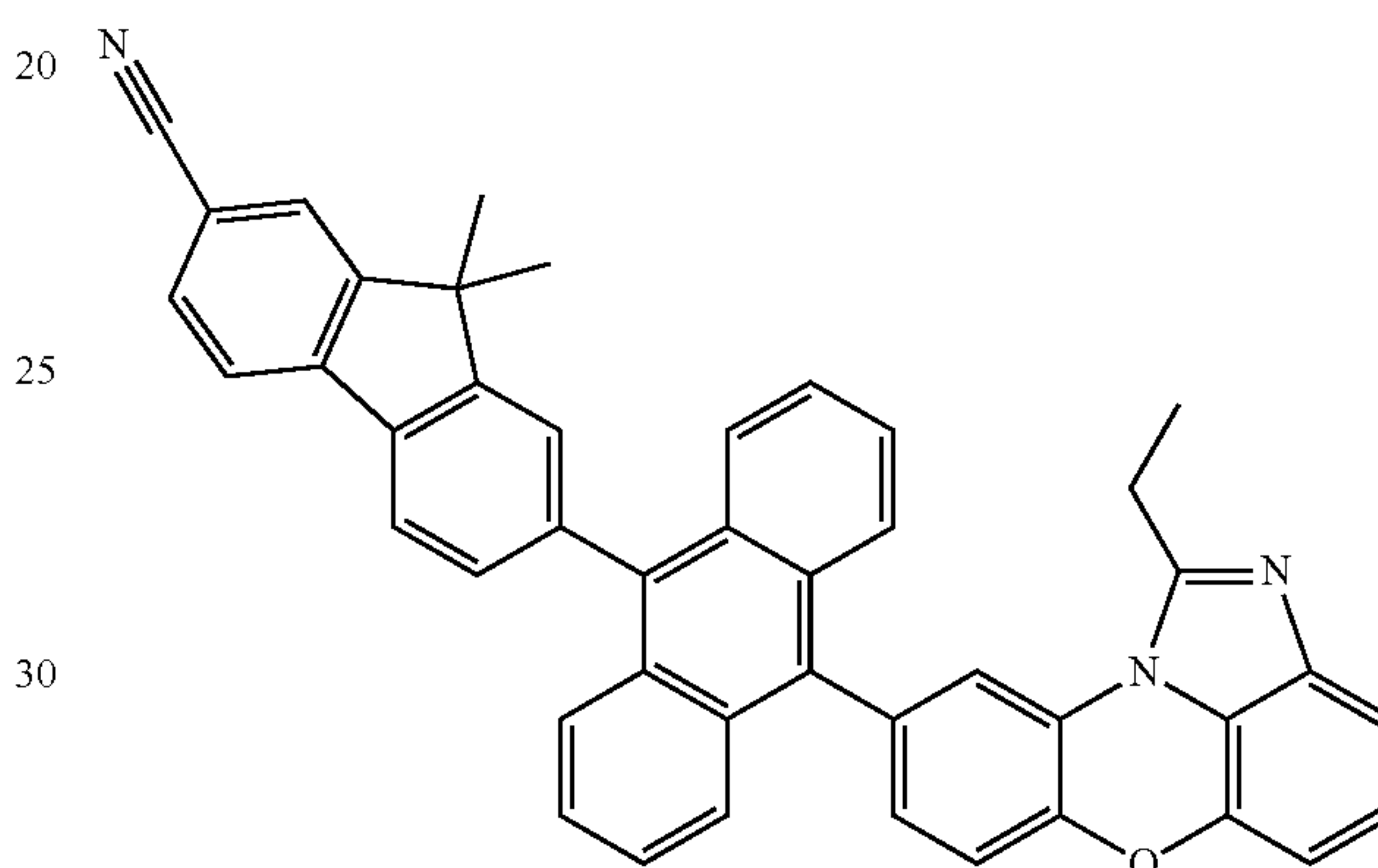
[Chemical Formula 1-7-15]
