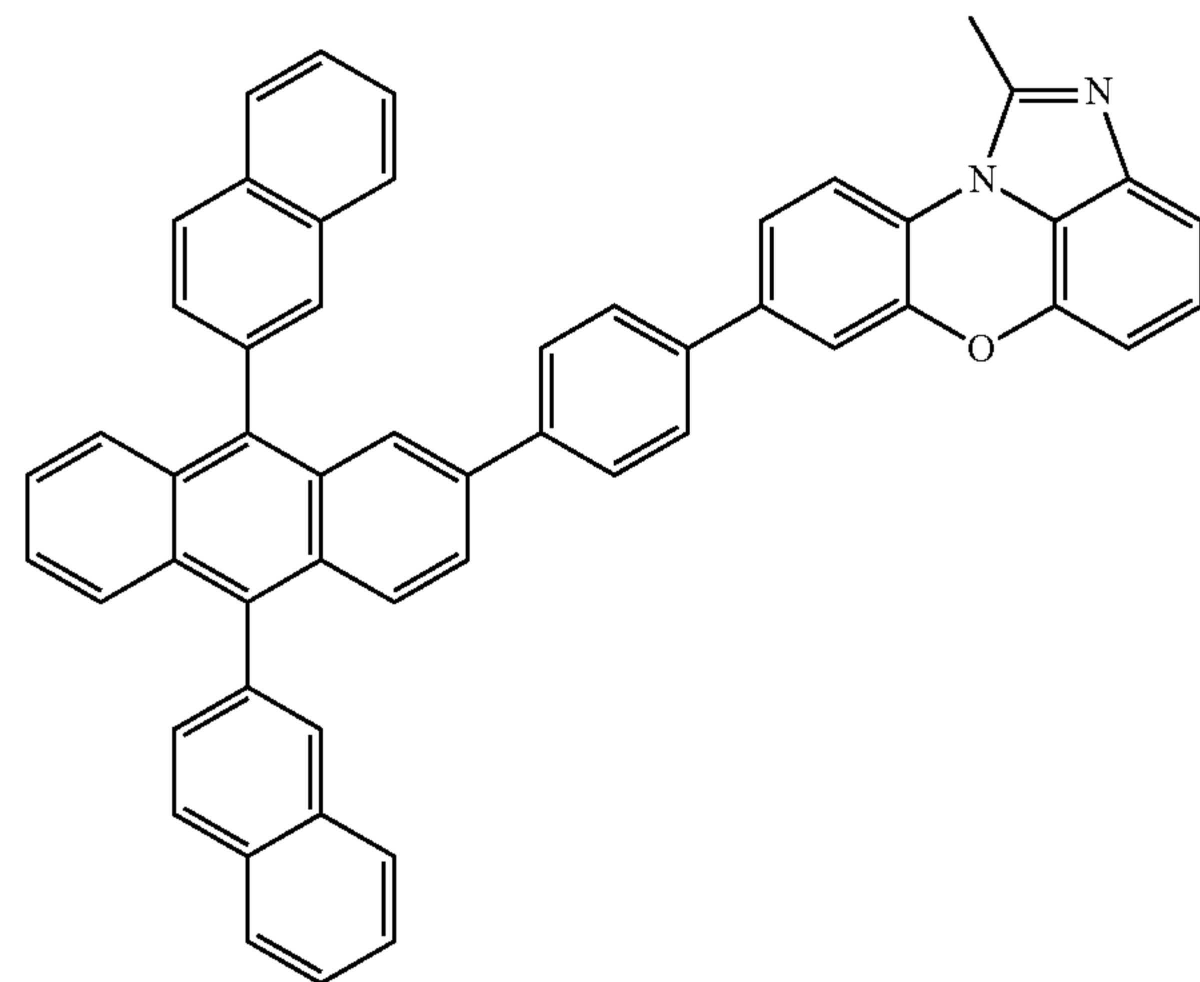
[Chemical Formula 1-2-25]
