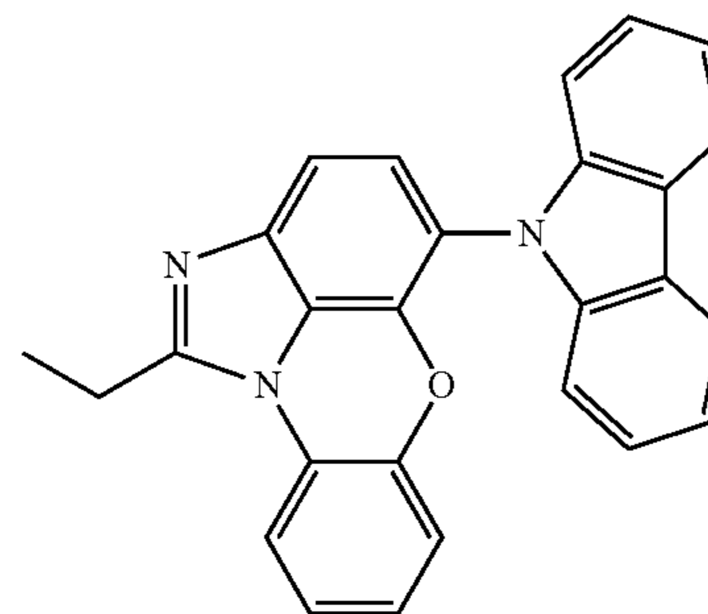
[Chemical Formula 1-9-15]
