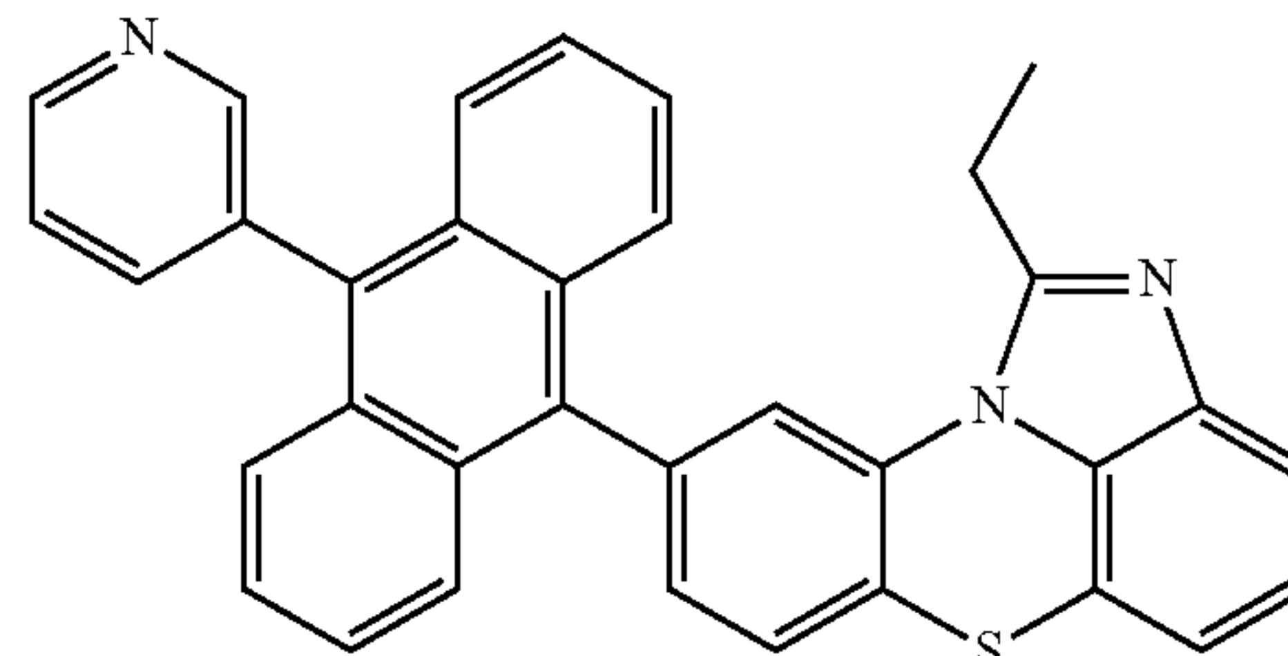
[Chemical Formula 2-3-10]
