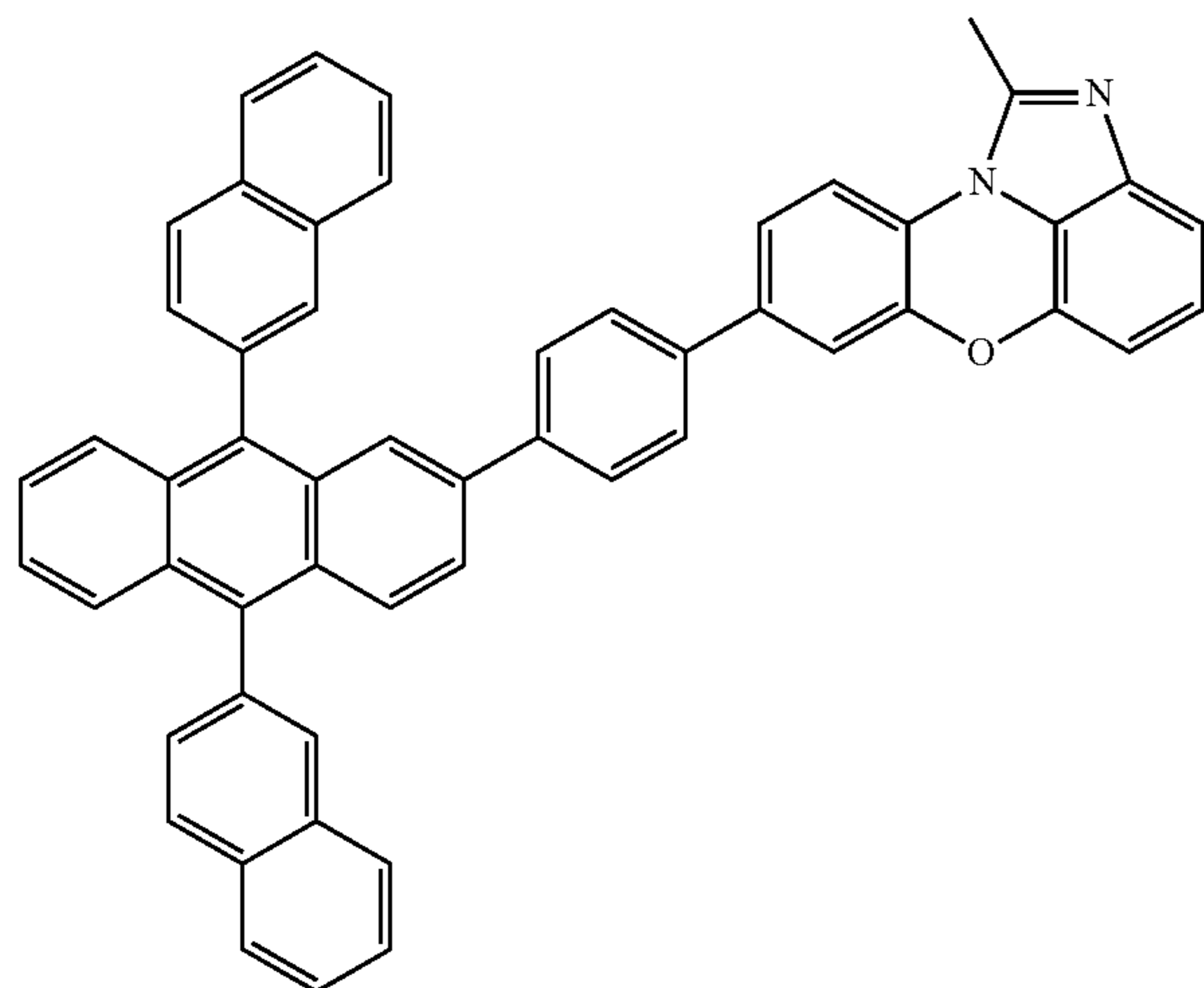
[Chemical Formula 1-2-25]
