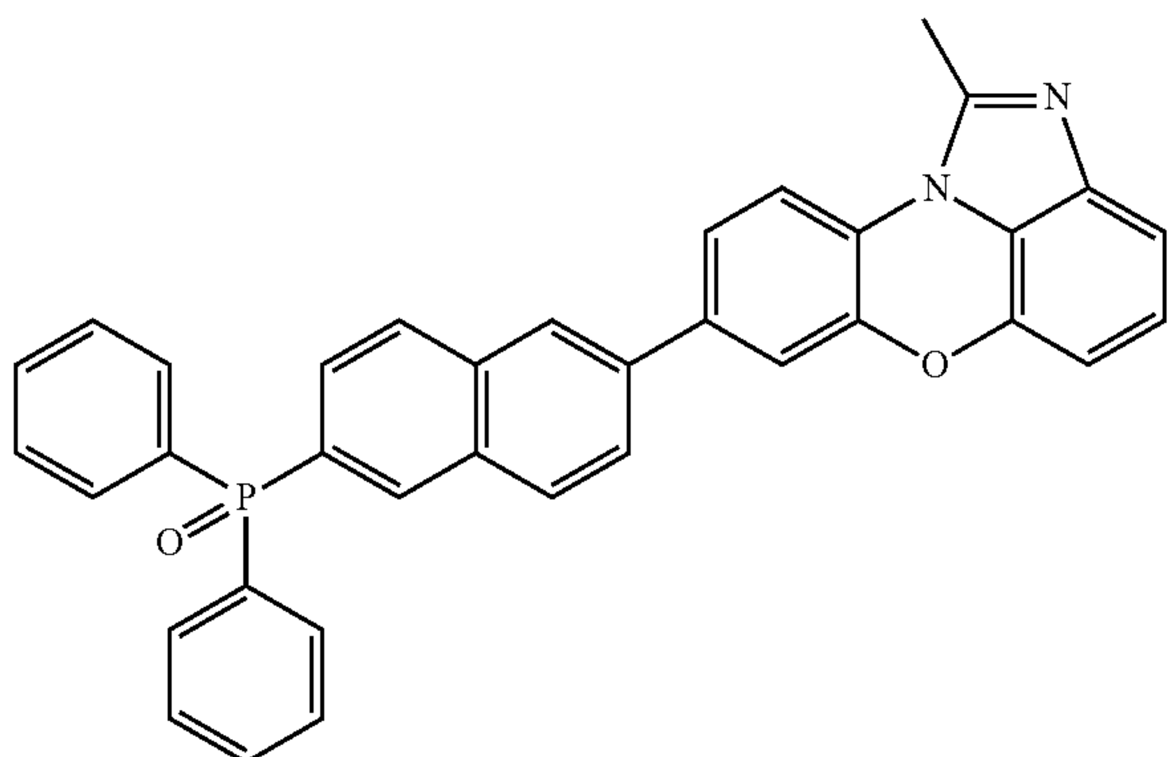
[Chemical Formula 1-5-2]
