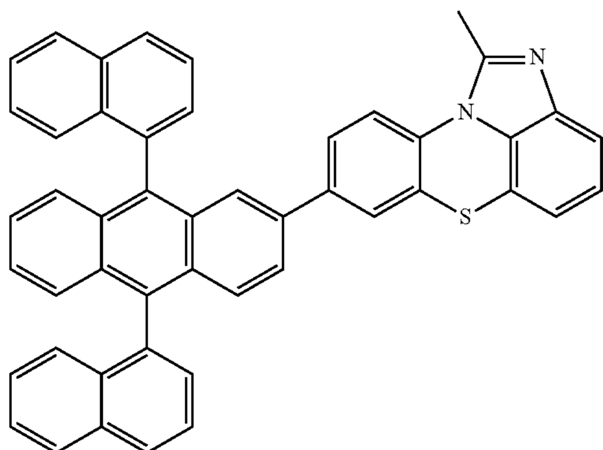
[Chemical Formula 2-2-21]
