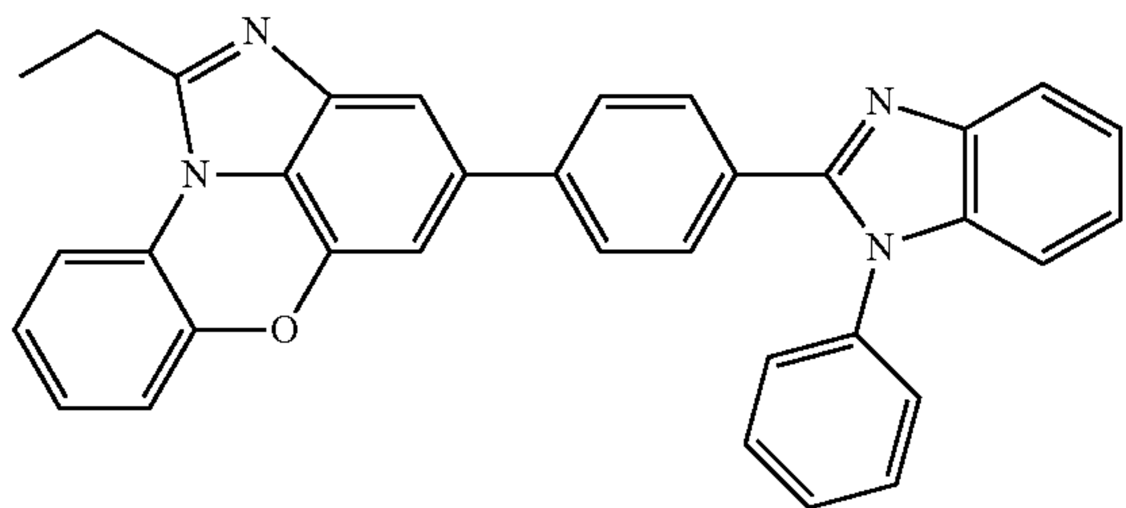
[Chemical Formula 1-10-9]
