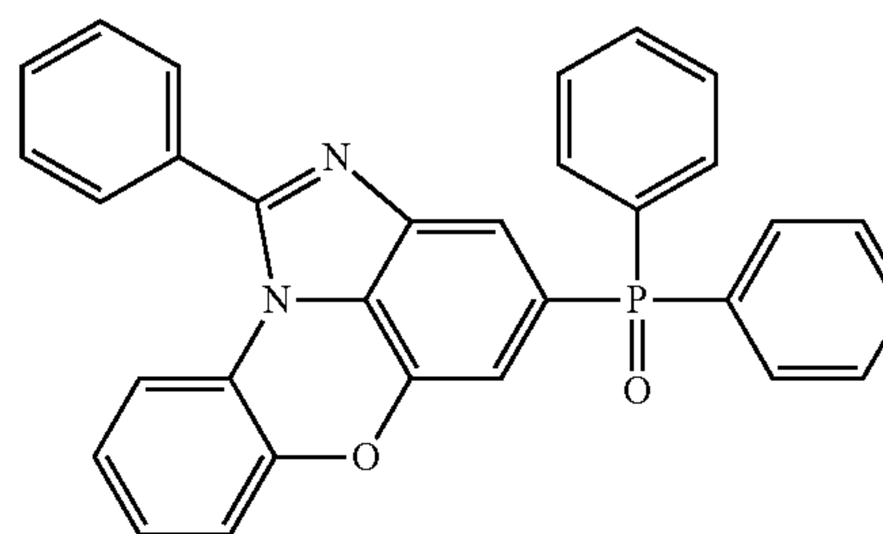
[Chemical Formula 1-6-1]
