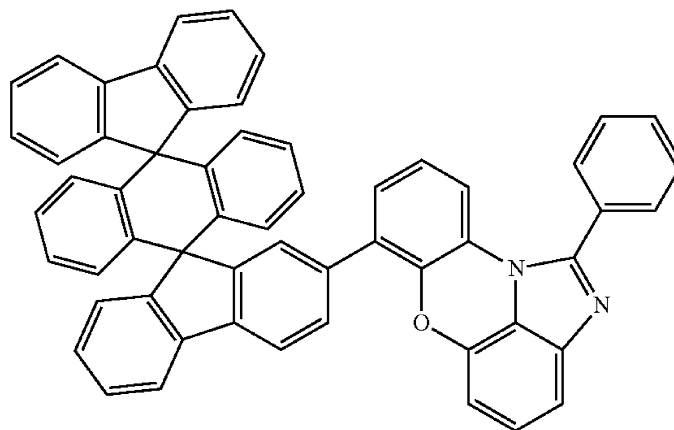
[Chemical Formula 1-6-36]
