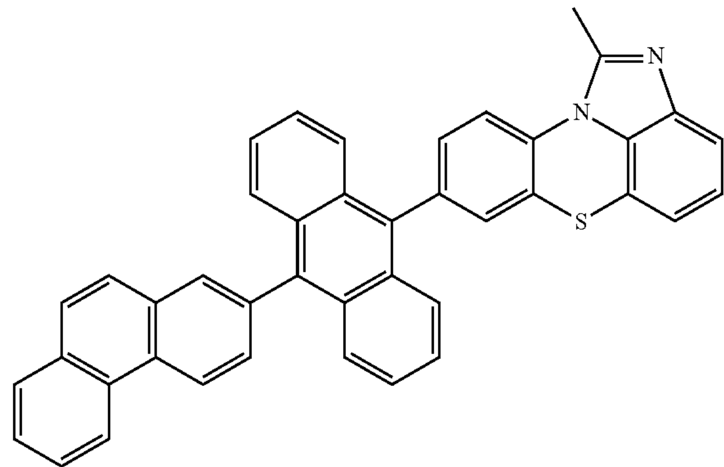
[Chemical Formula 2-2-9]
