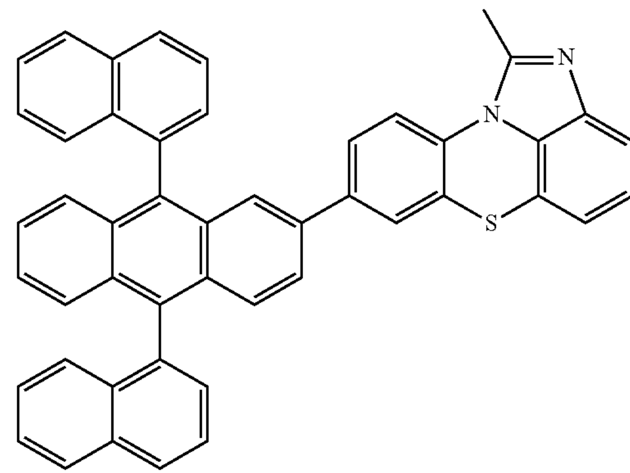
[Chemical Formula 2-2-21]
