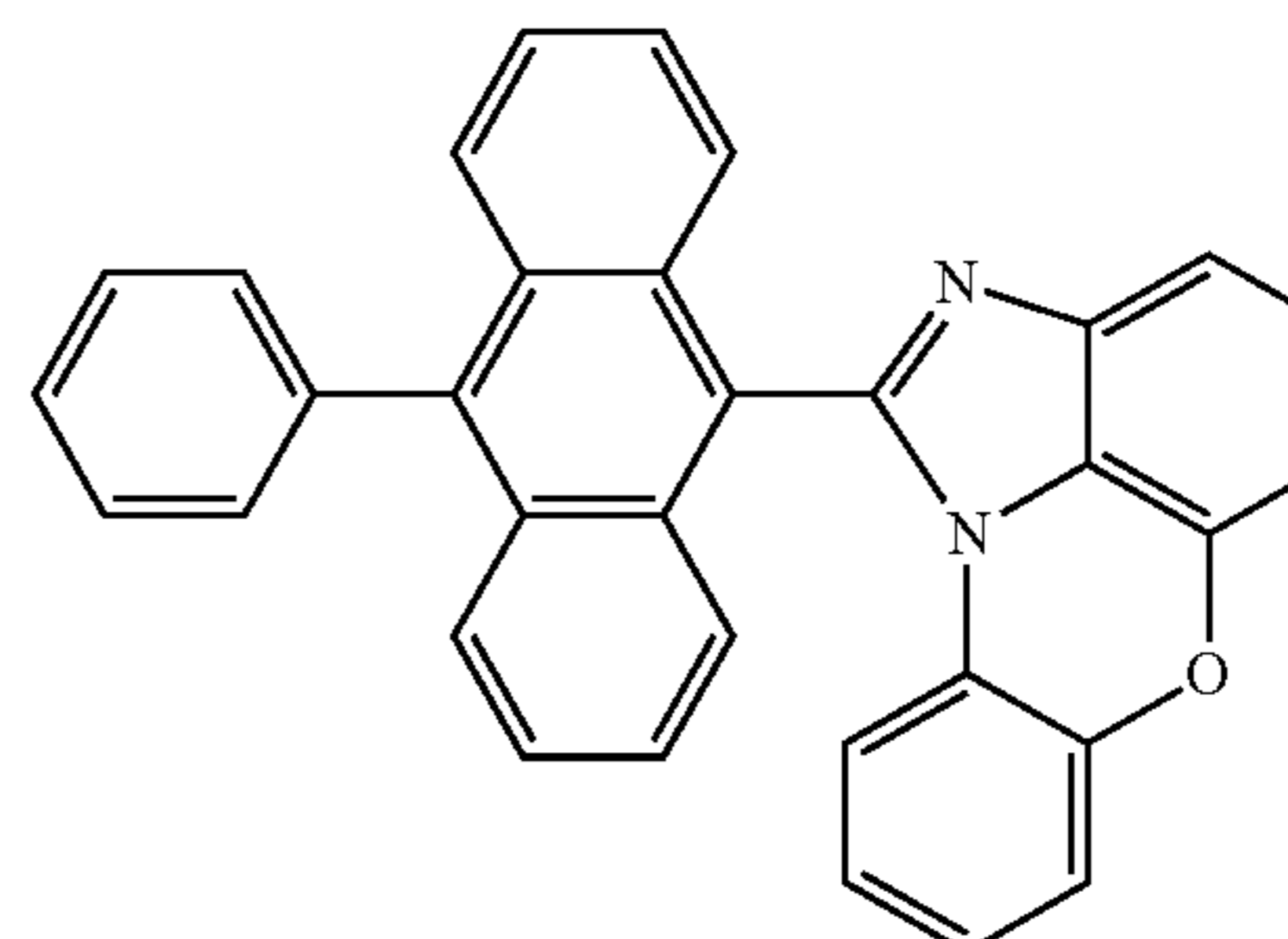
[Chemical Formula 1-1-10]
