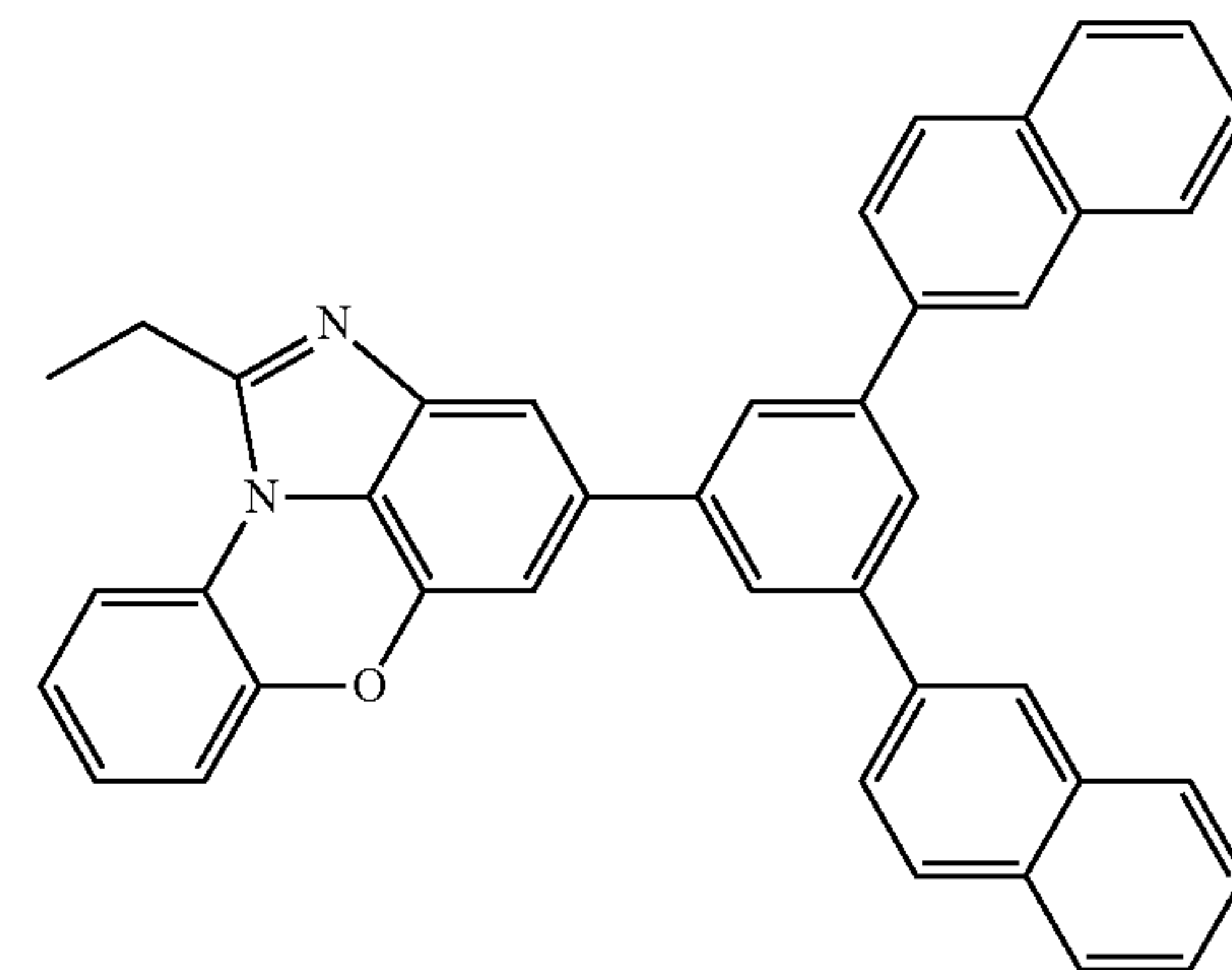
[Chemical Formula 1-10-7]
