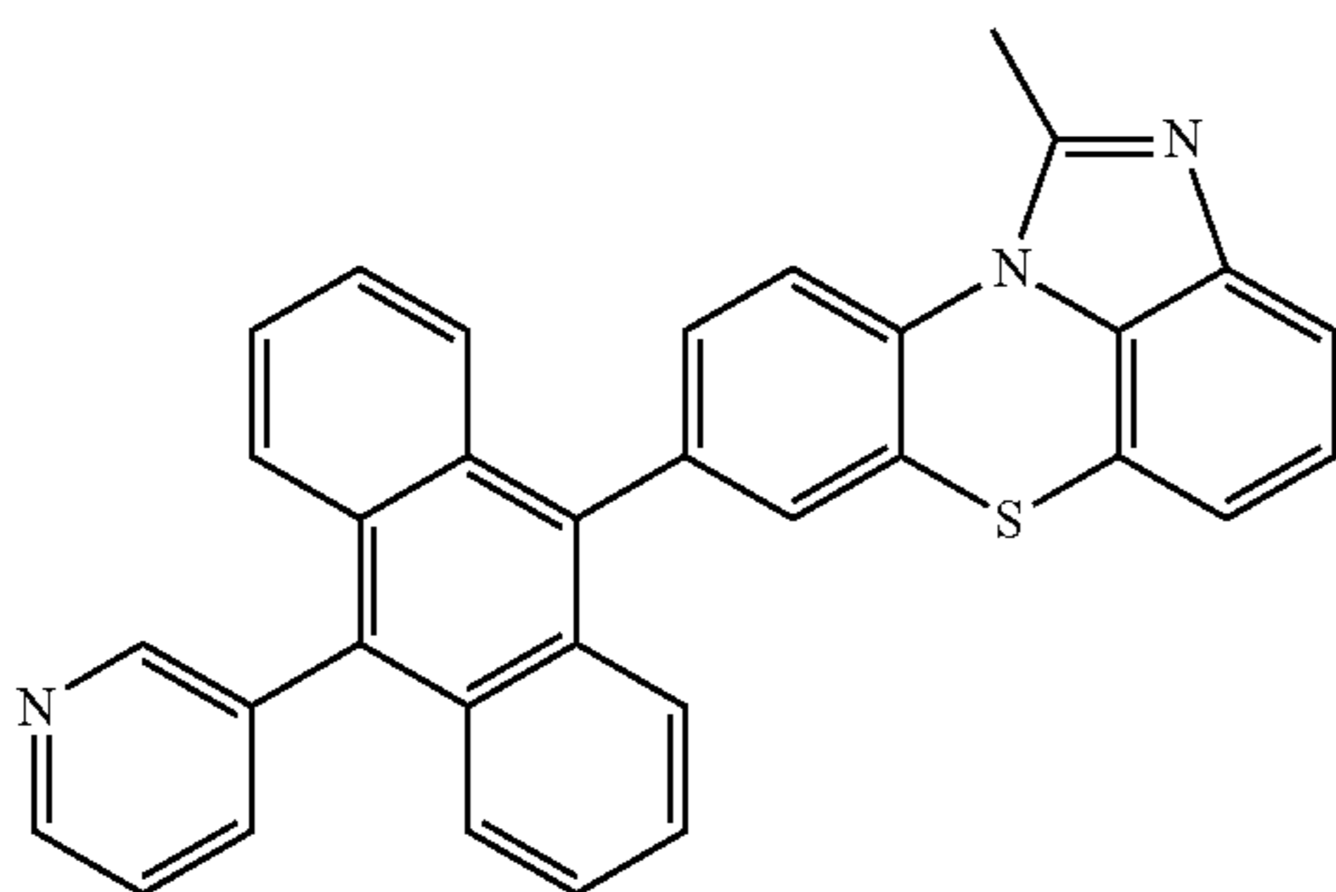
[Chemical Formula 2-2-10]
