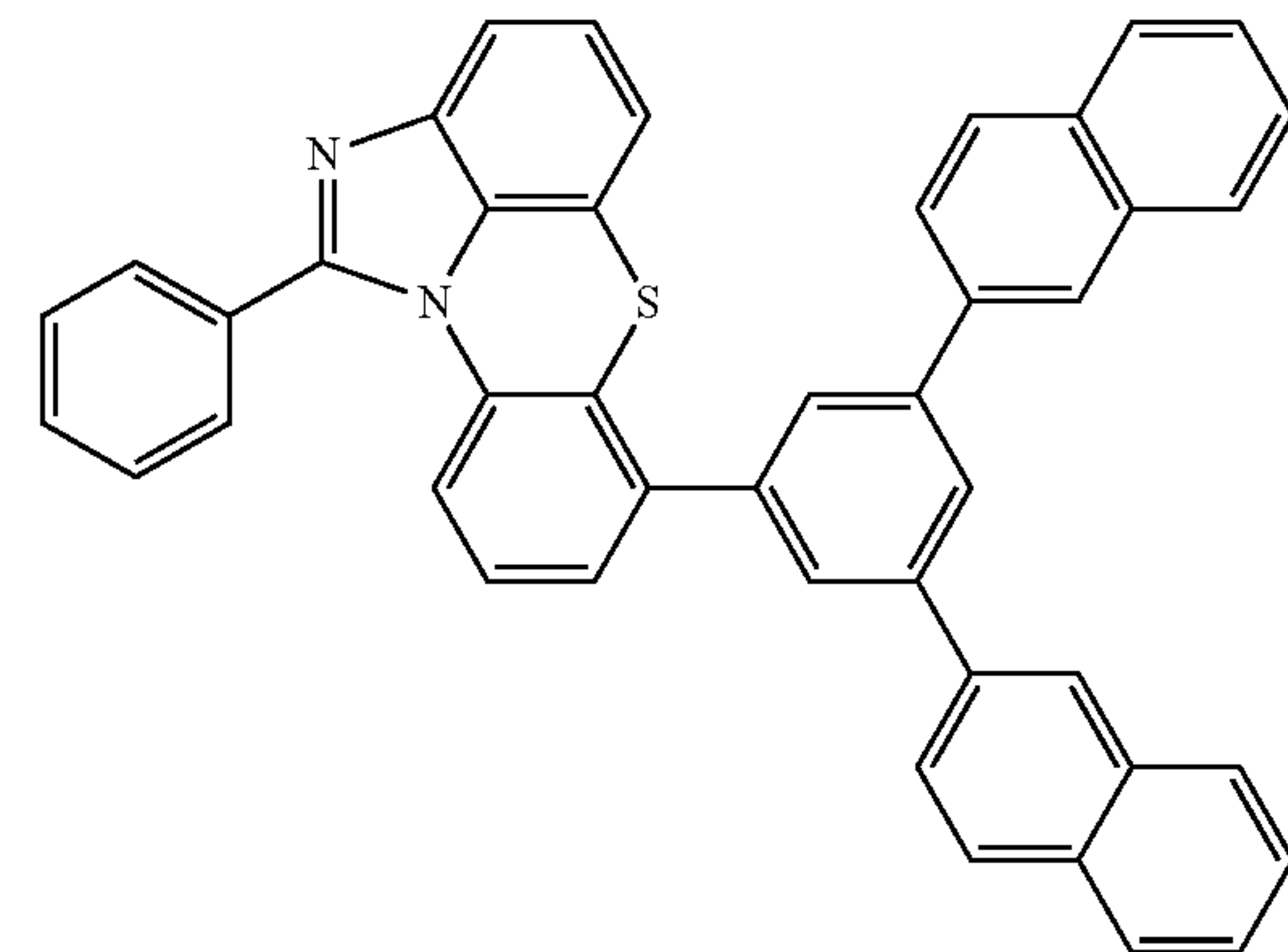
[Chemical Formula 2-2-43]
