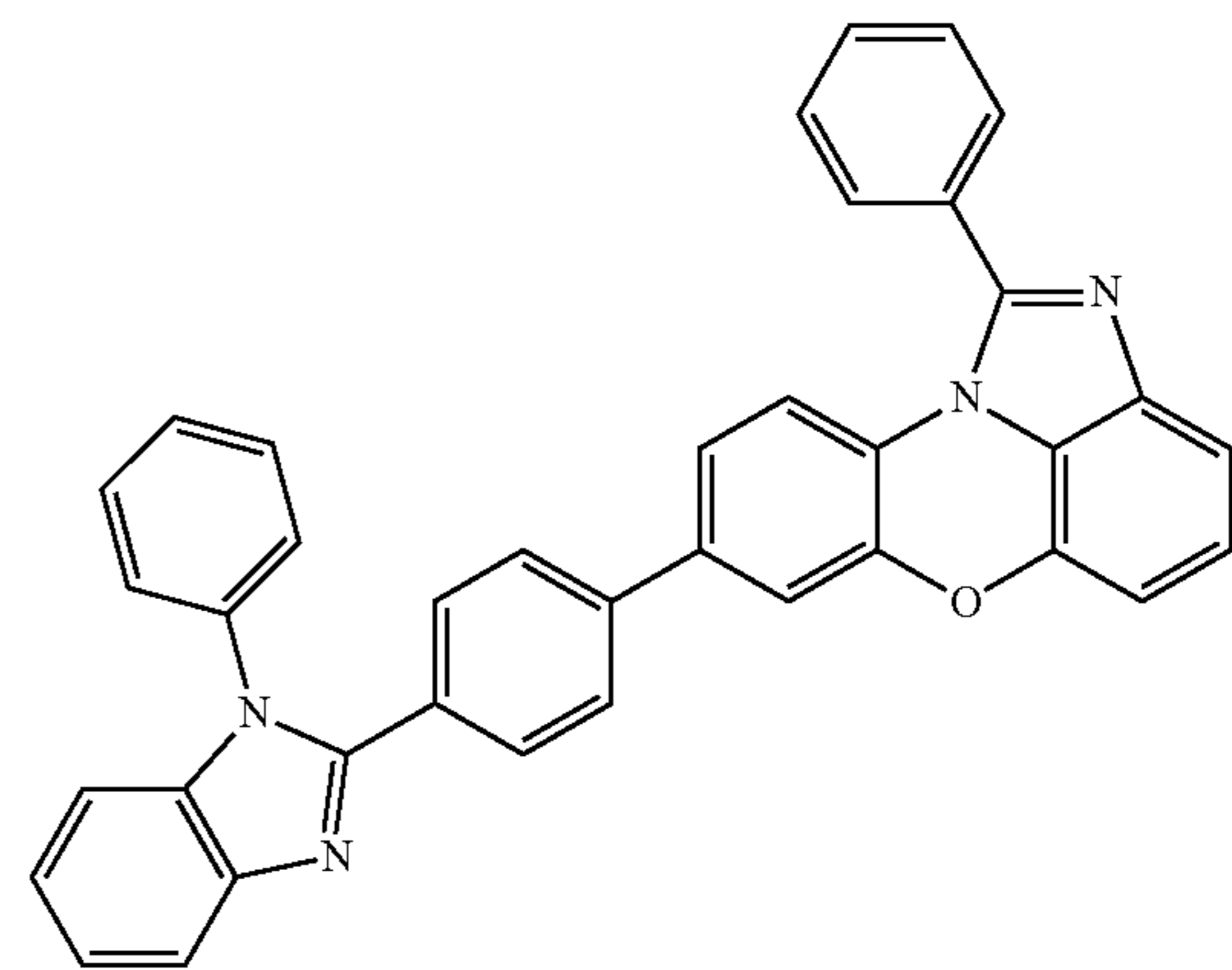
[Chemical Formula 1-4-45]
