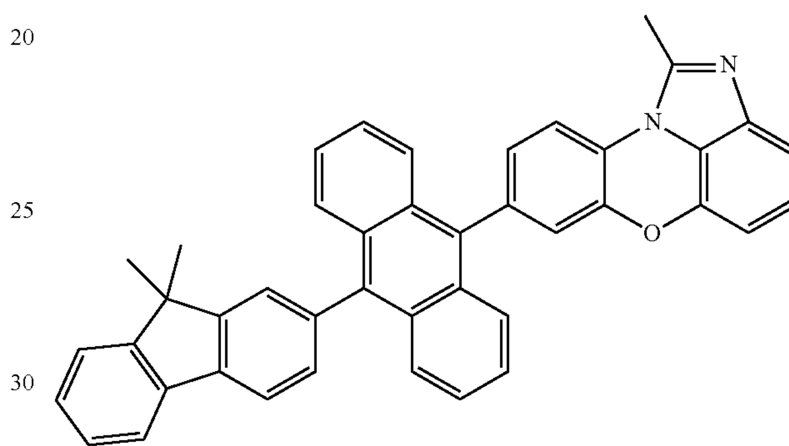
[Chemical Formula 1-2-6]
