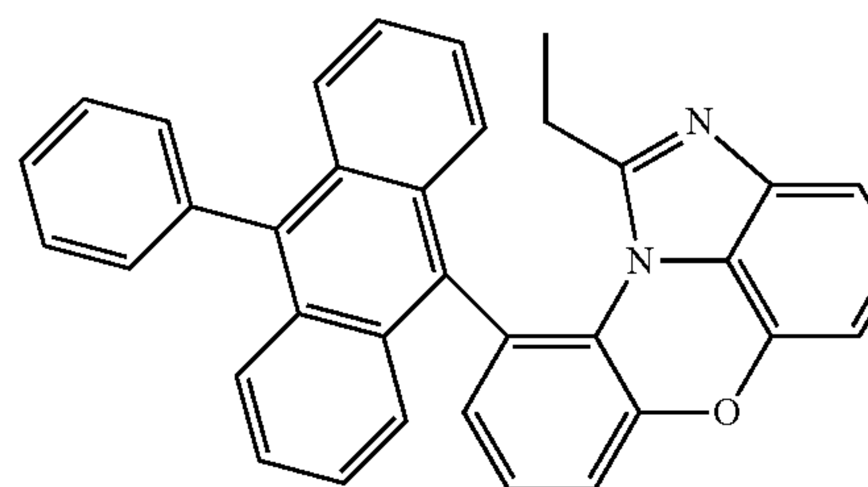
[Chemical Formula 1-8-2]
