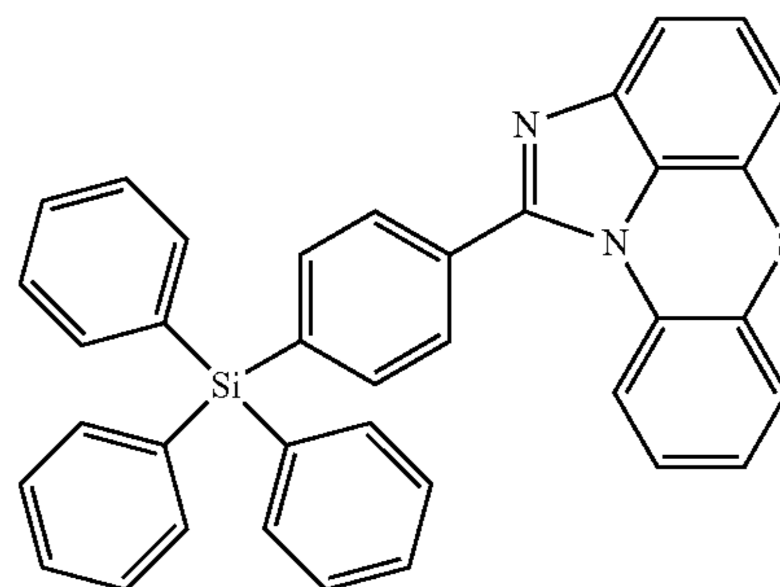
[Chemical Formula 2-1-9]
