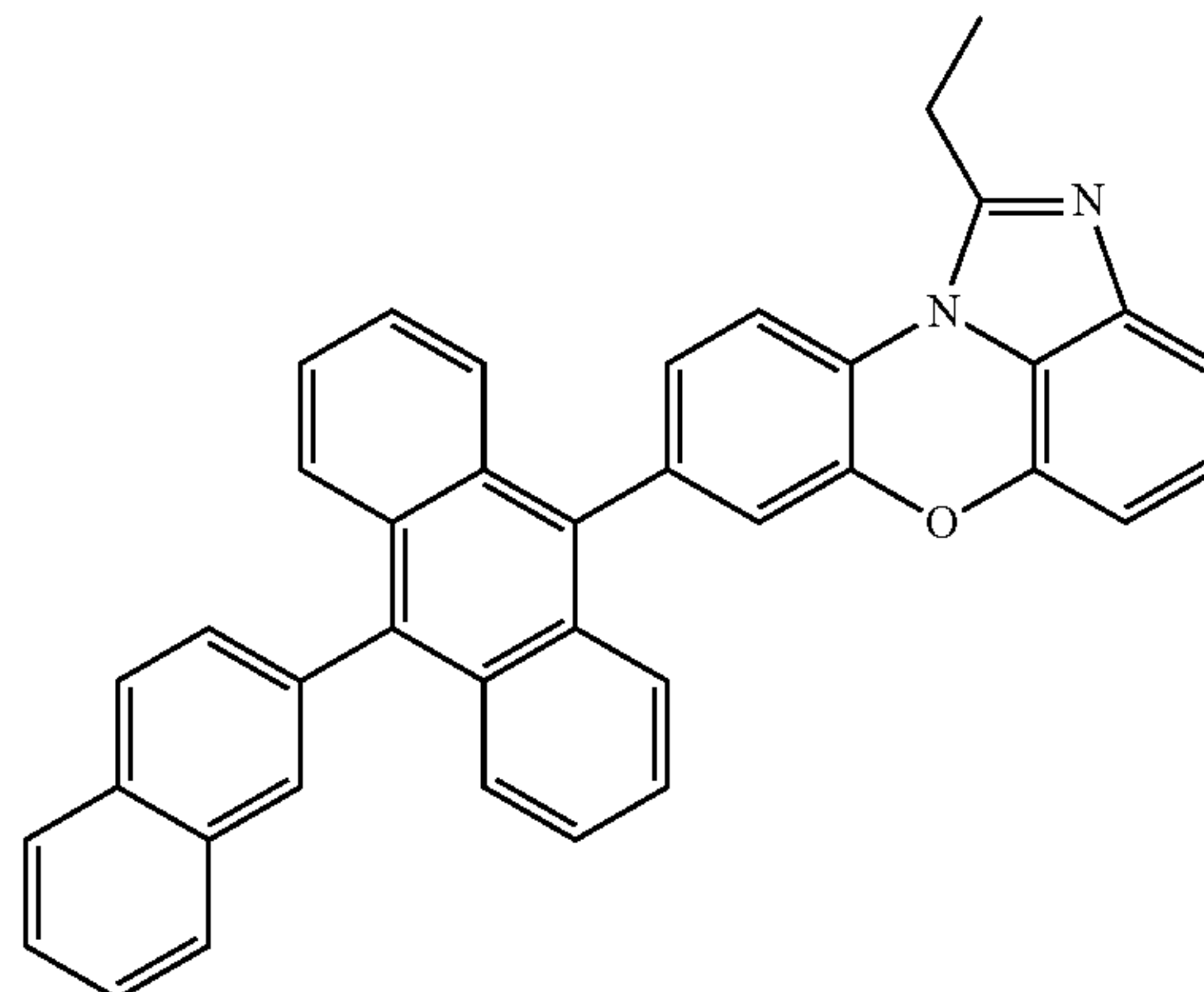
[Chemical Formula 1-3-2]
