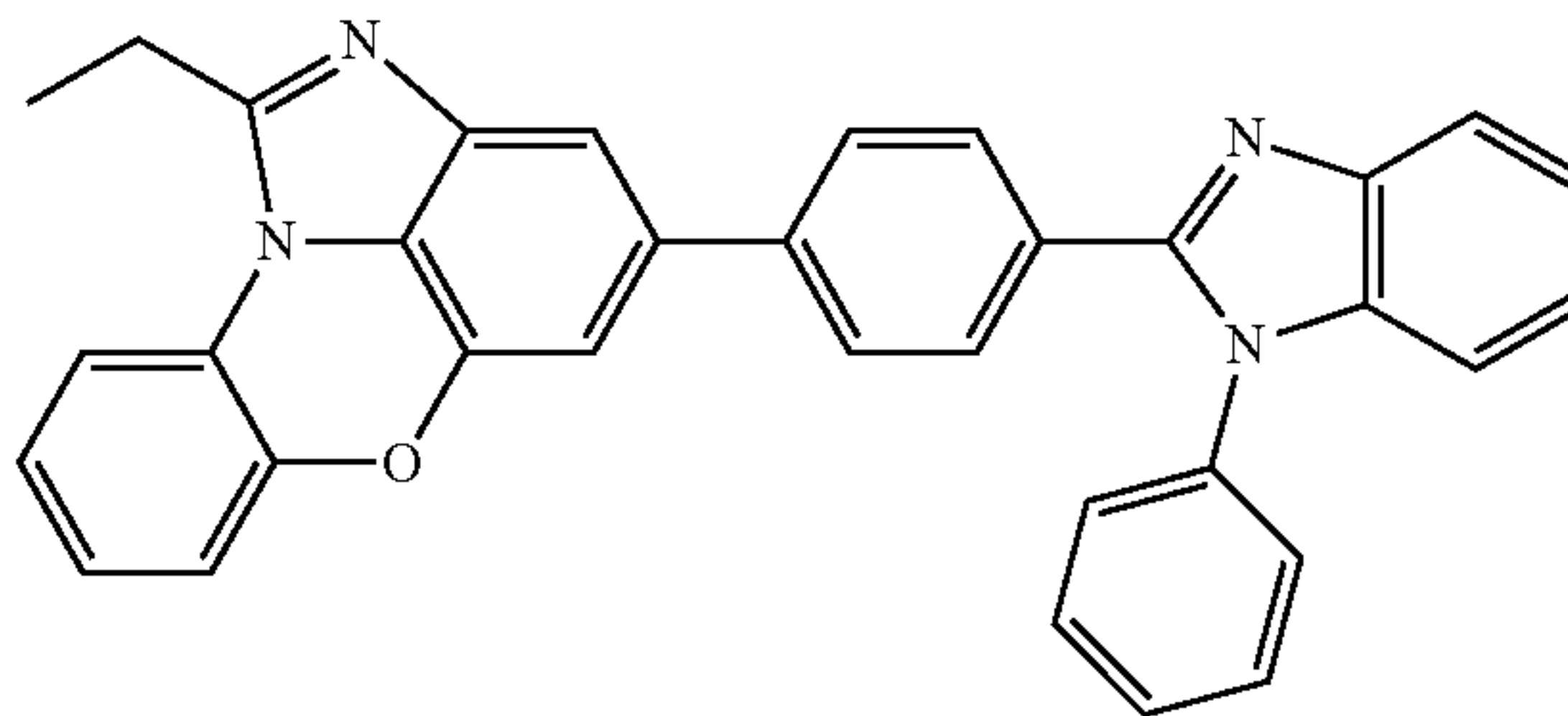
[Chemical Formula 1-10-9]
