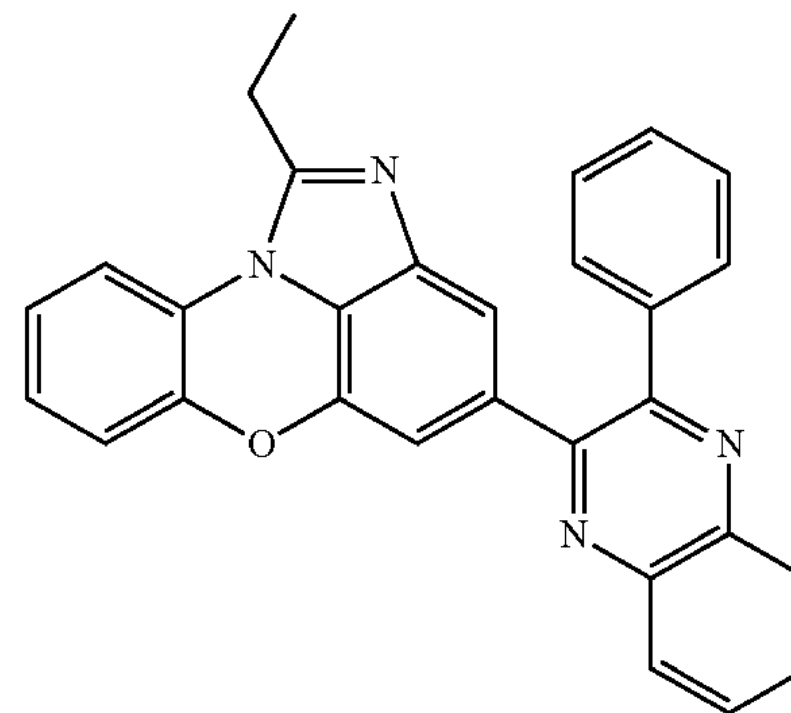
[Chemical Formula 1-10-13]
