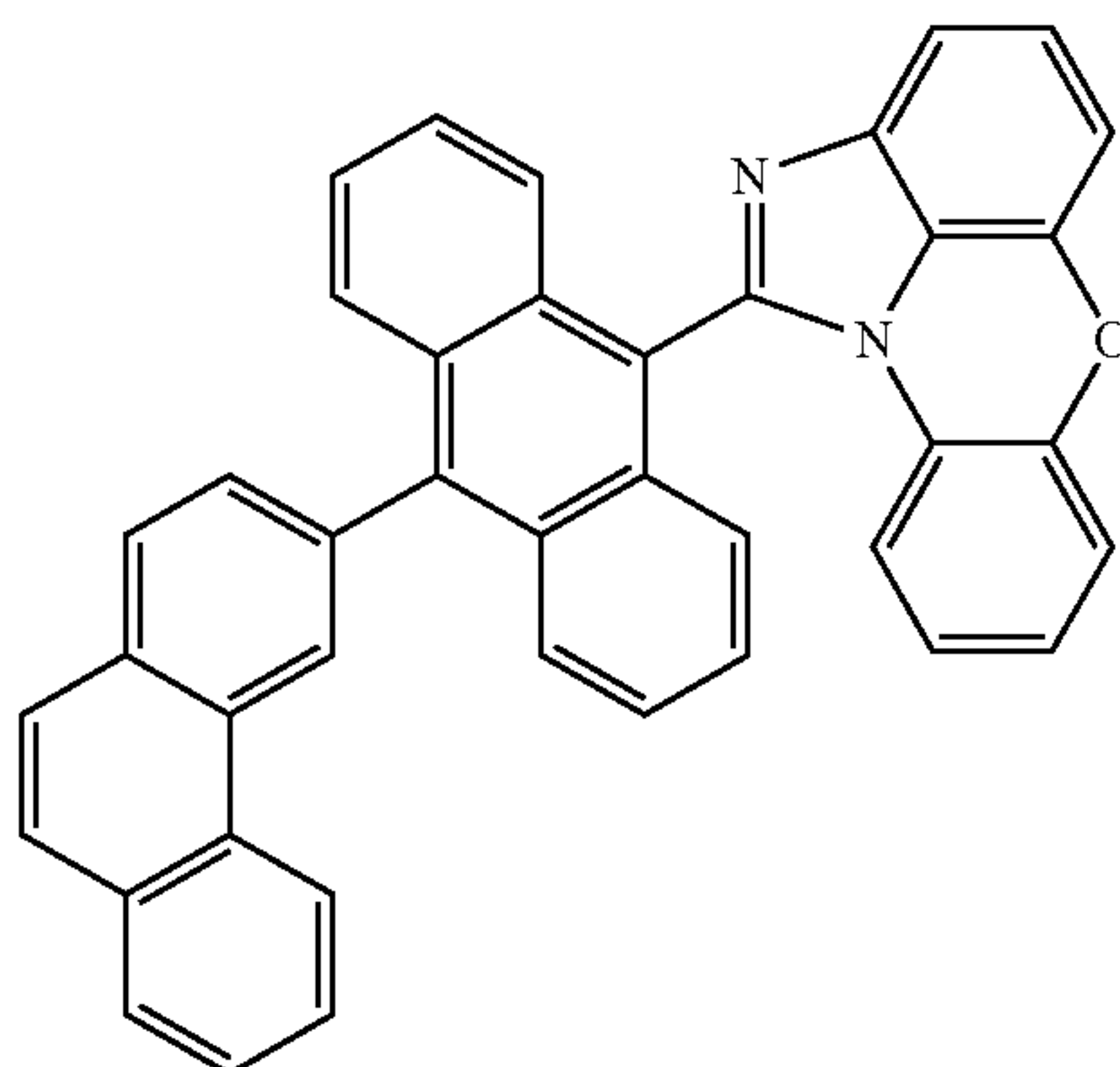
[Chemical Formula 1-1-16]
