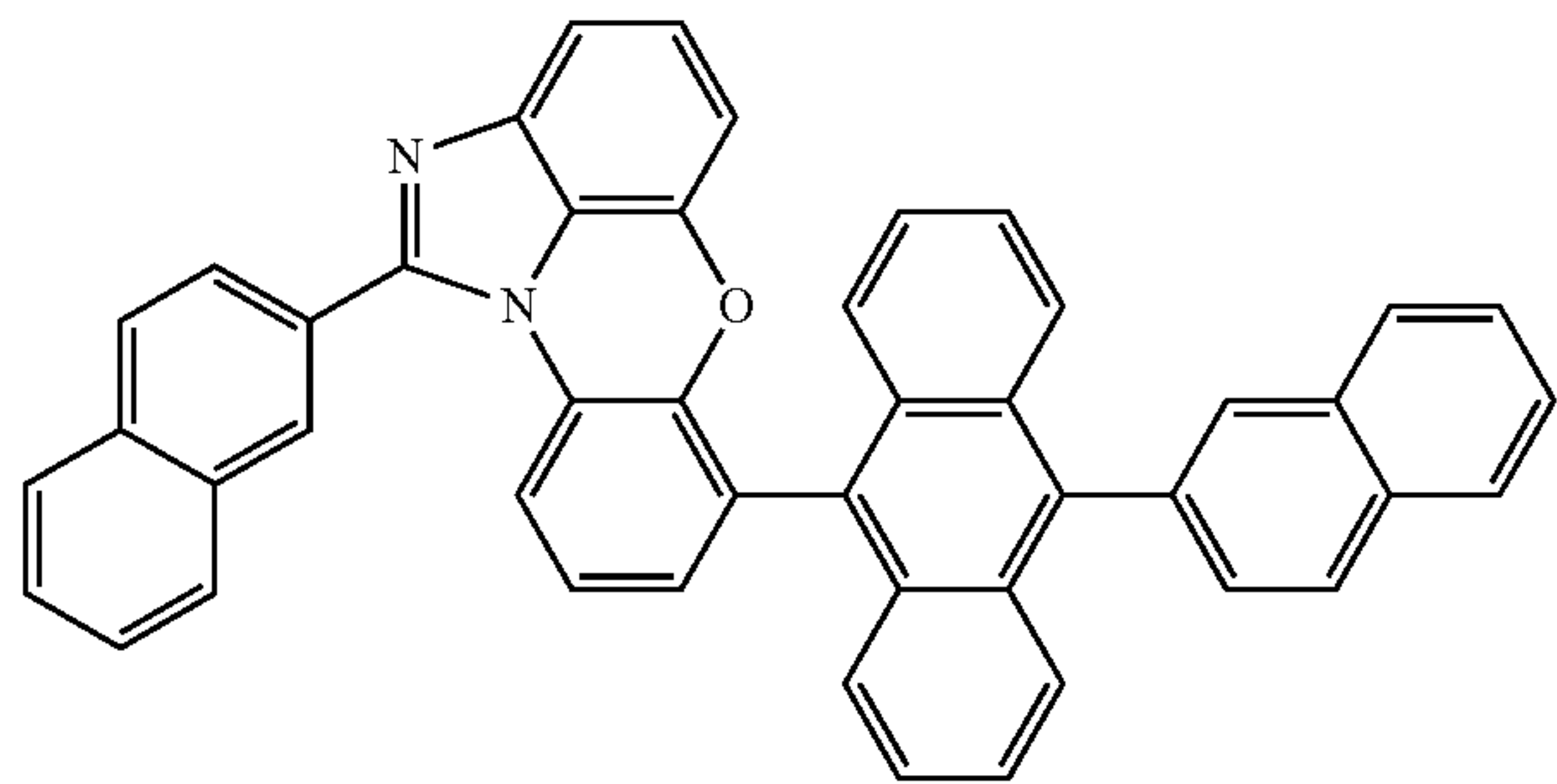
[Chemical Formula 1-6-3]
