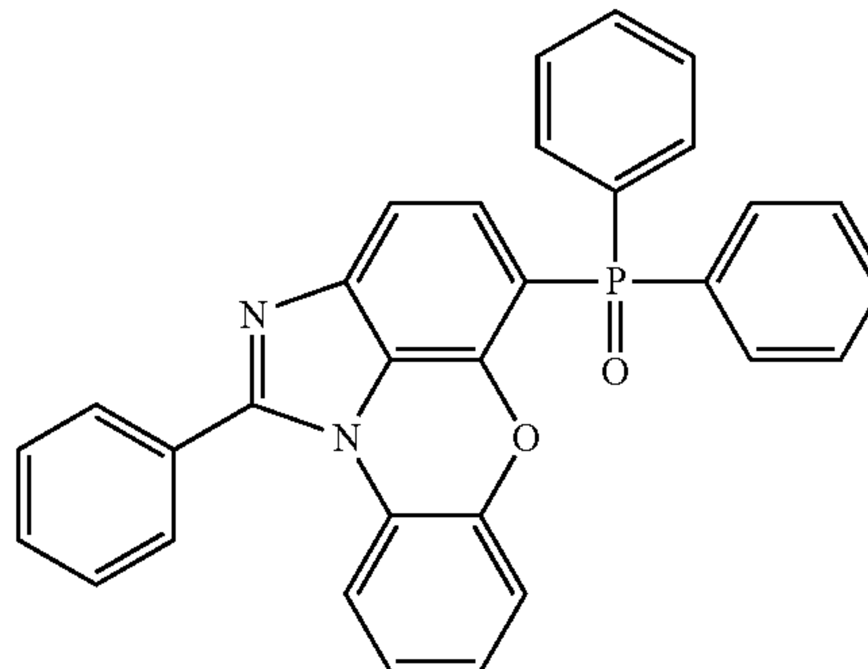
[Chemical Formula 1-5-6]
