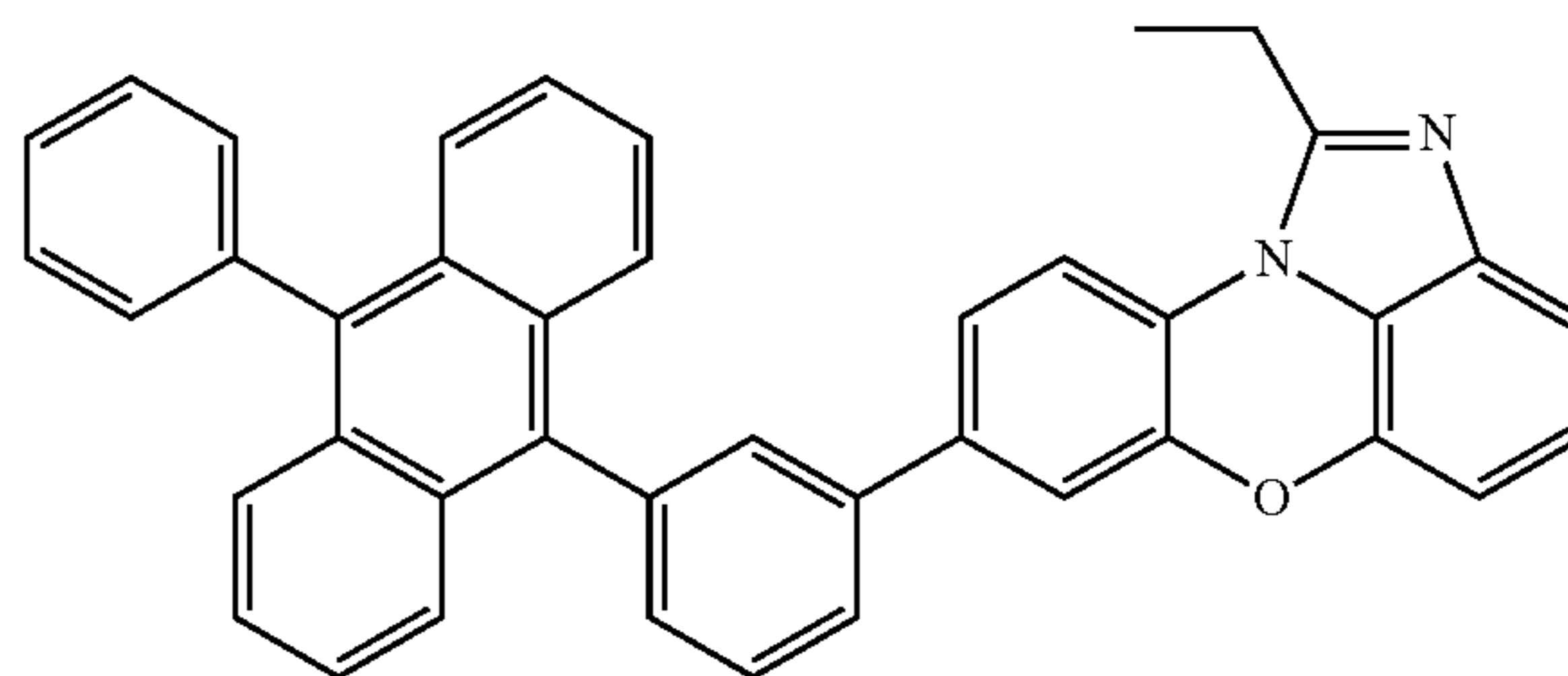
[Chemical Formula 1-3-19]
