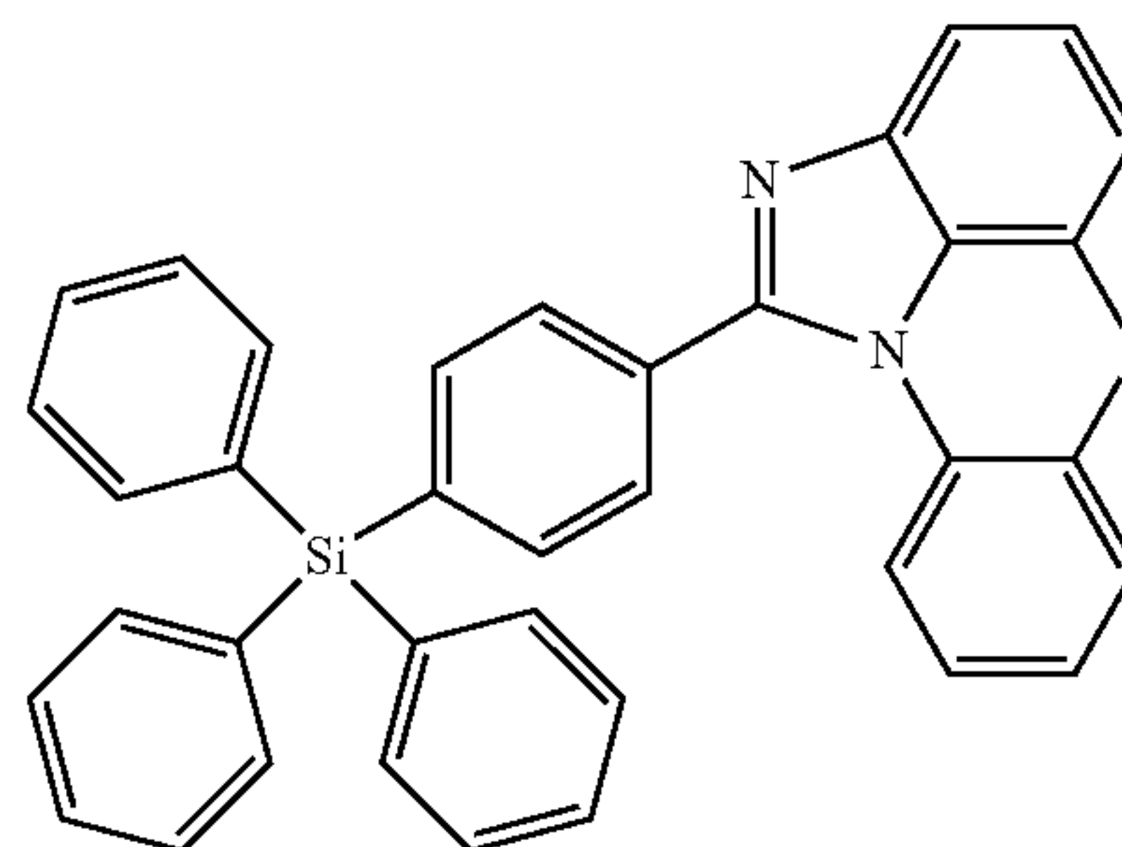
[Chemical Formula 2-1-9]
