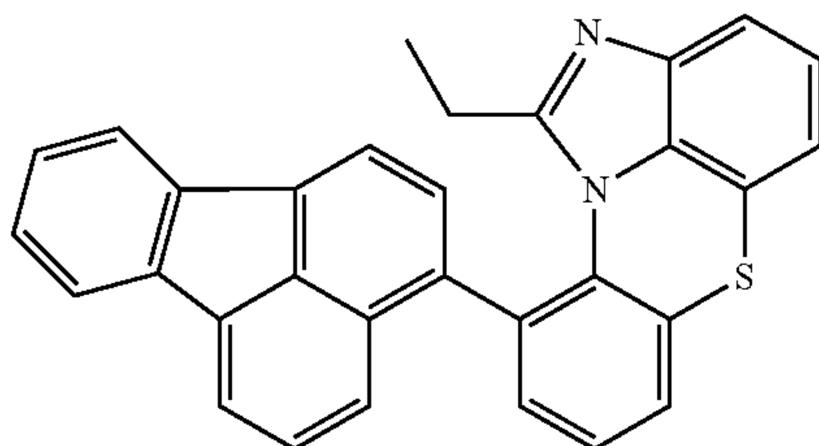
[Chemical Formula 2-3-31]
