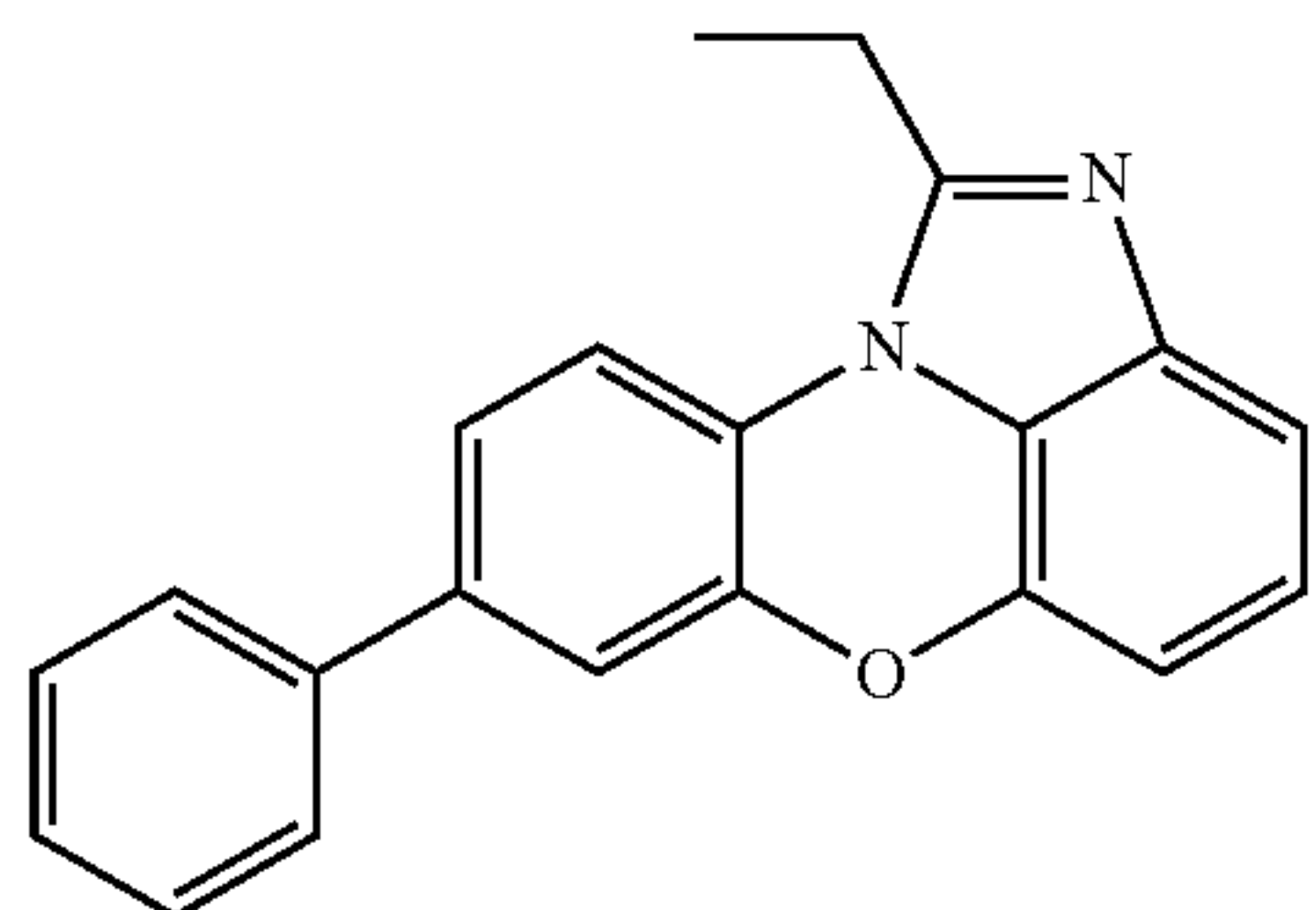
[Chemical Formula 1-3-38]
