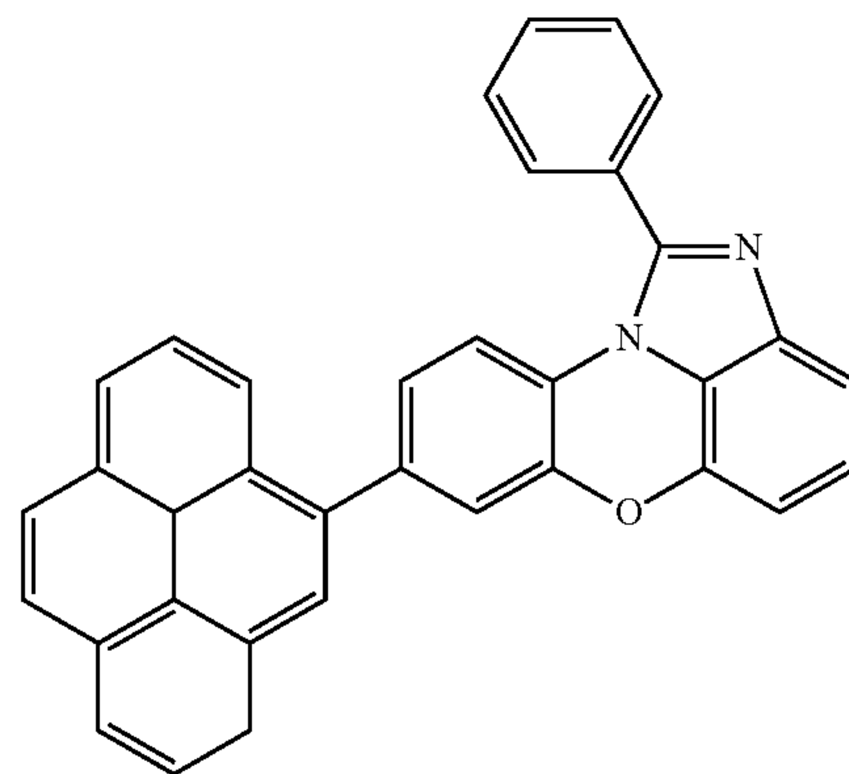
[Chemical Formula 1-4-28]
