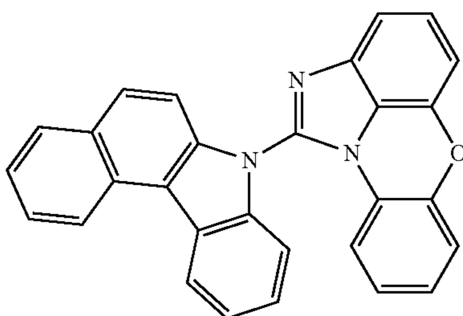
[Chemical Formula 1-1-60]
