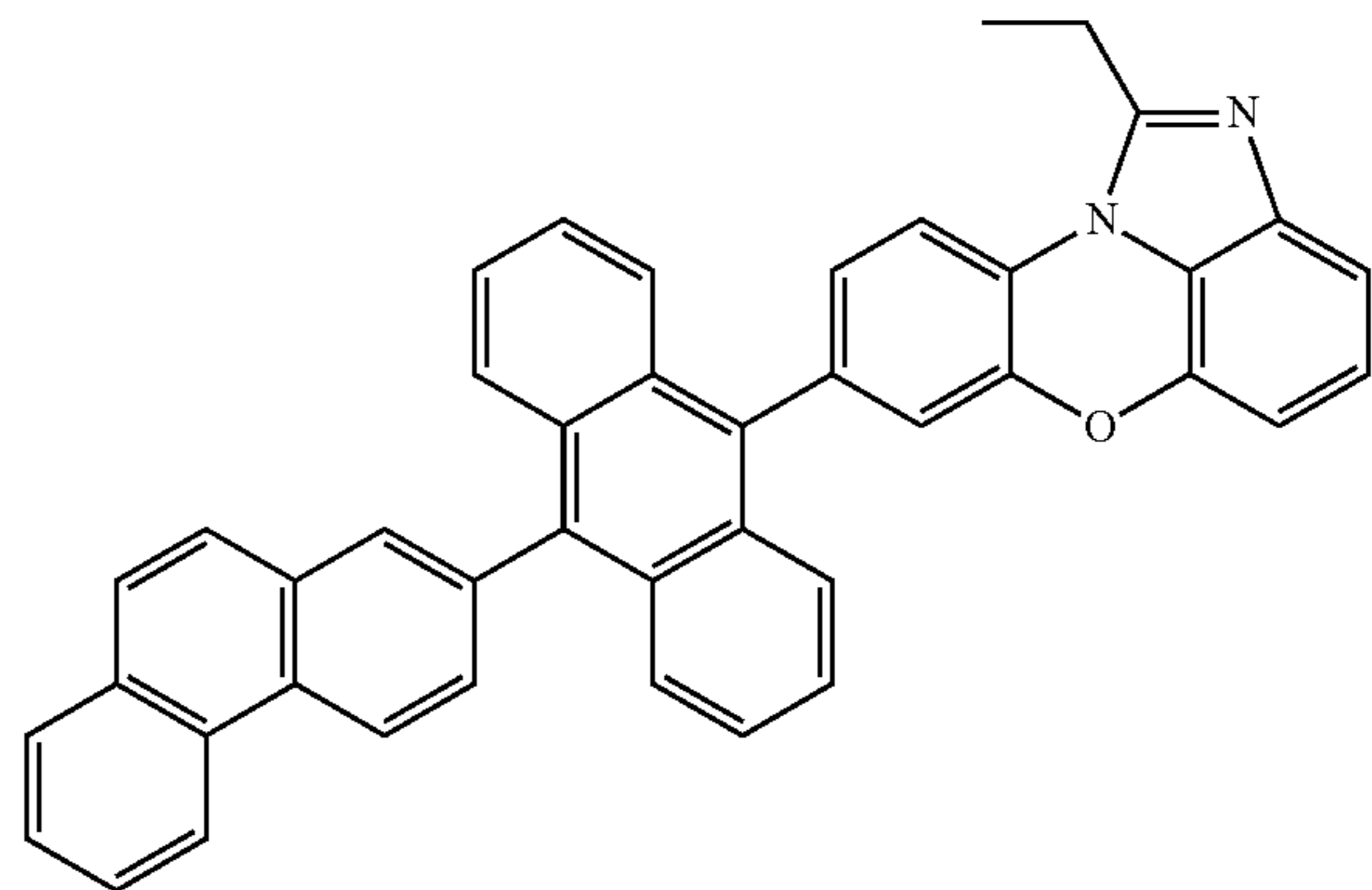
[Chemical Formula 1-3-9]
