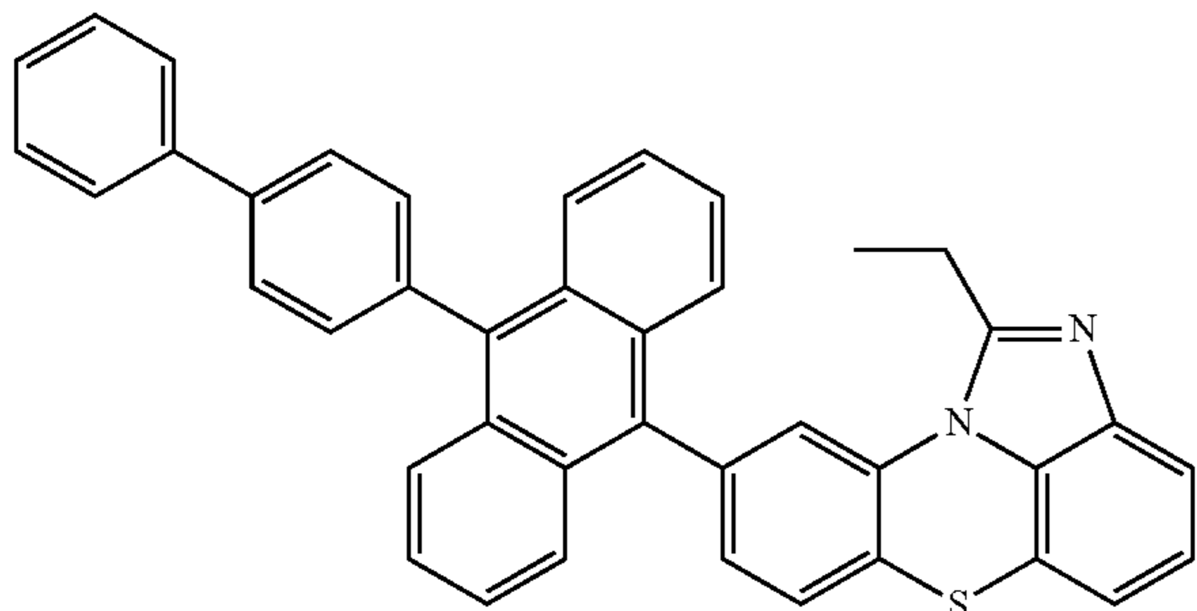
[Chemical Formula 2-3-4]
