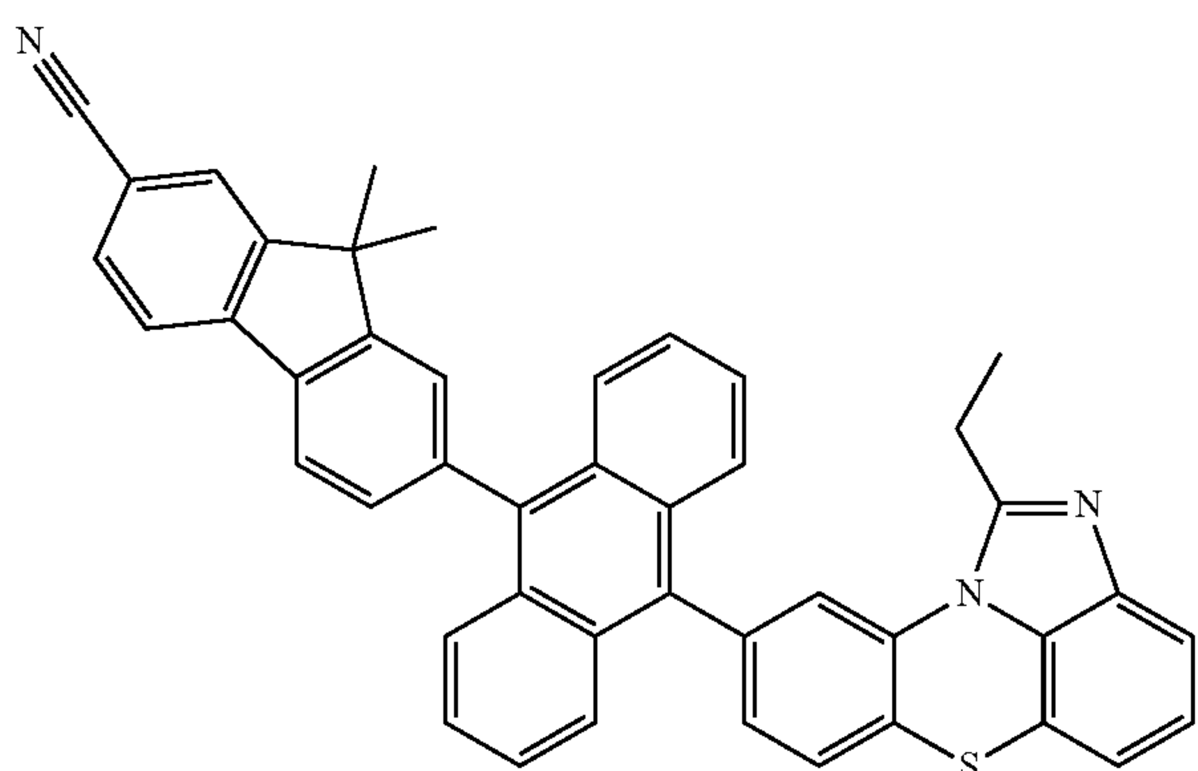
[Chemical Formula 2-3-15]
