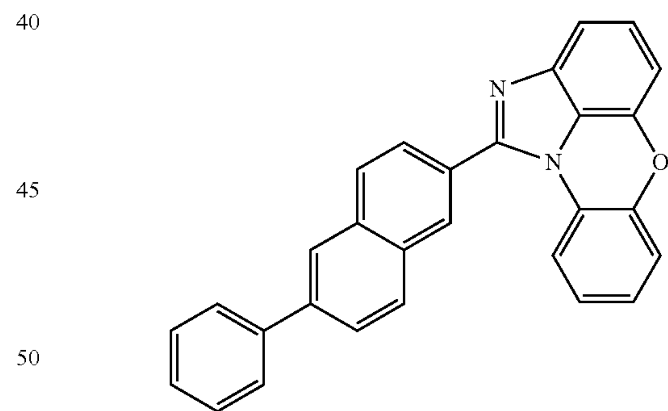
[Chemical Formula 1-1-35]
