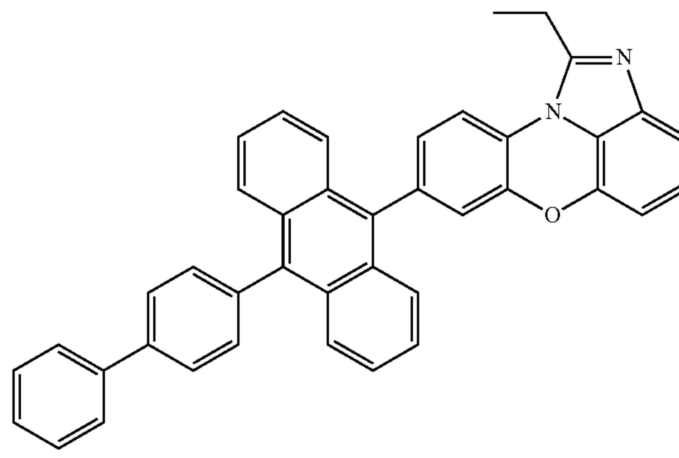
[Chemical Formula 1-3-4]
