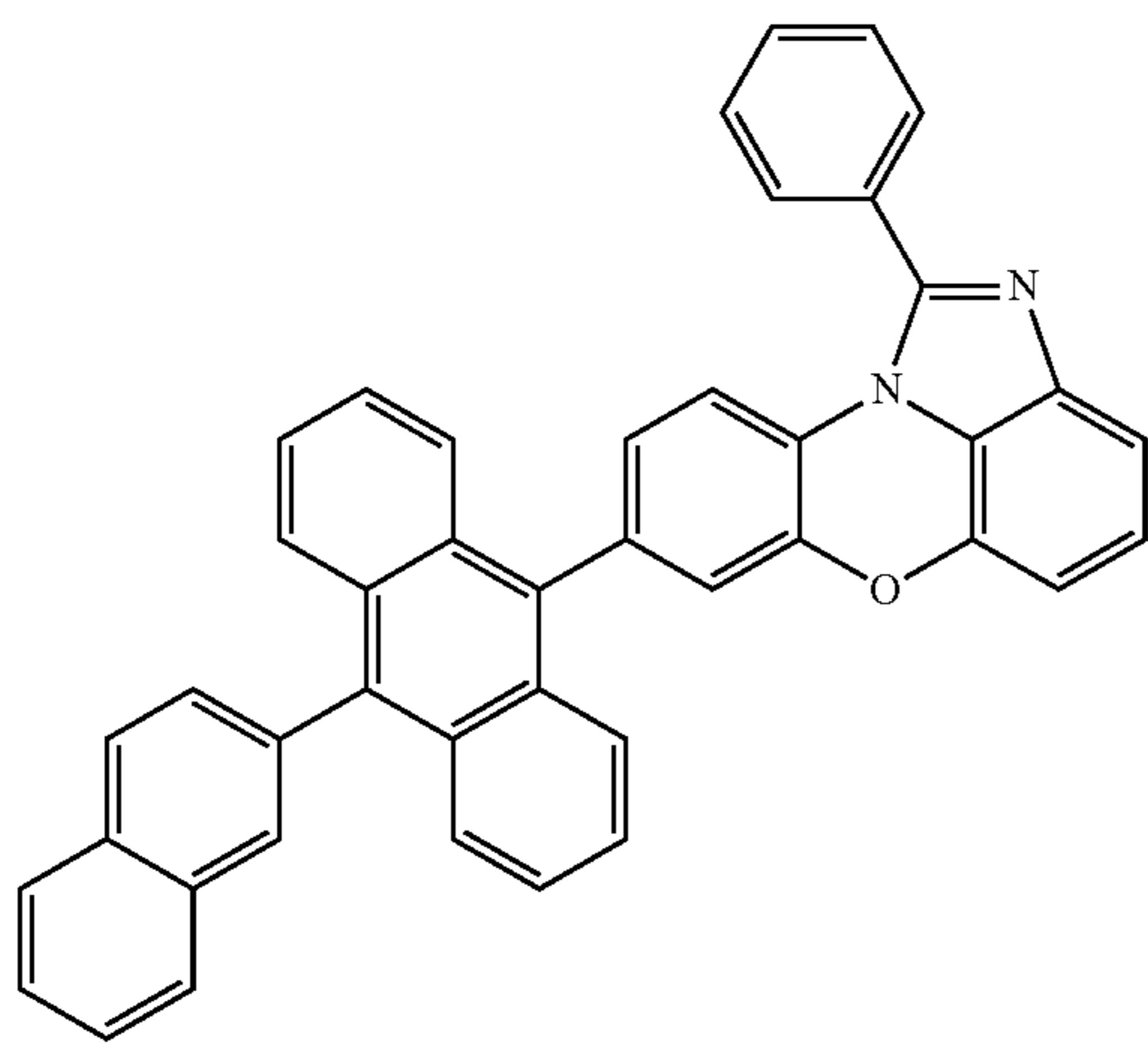
[Chemical Formula 1-4-2]
