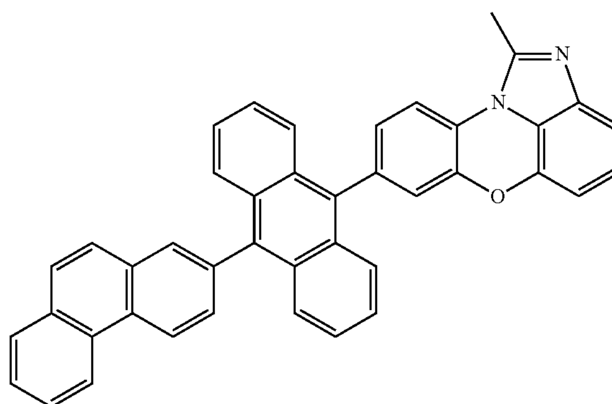
[Chemical Formula 1-2-9]
