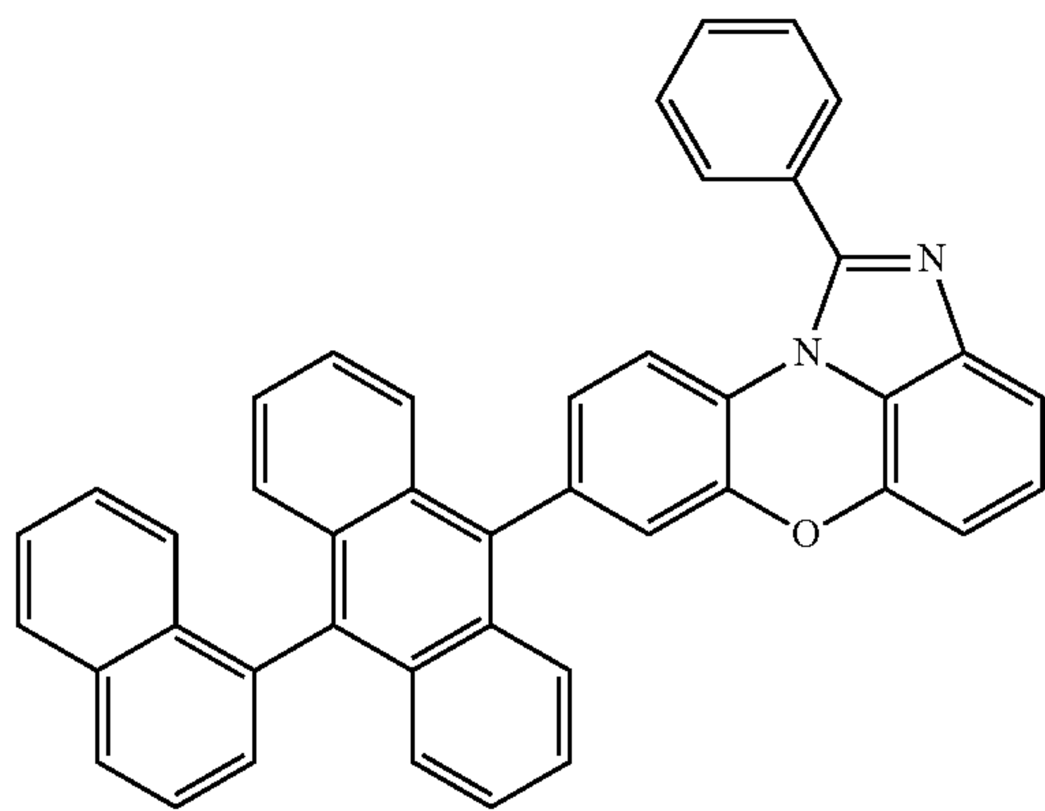
[Chemical Formula 1-4-3]
