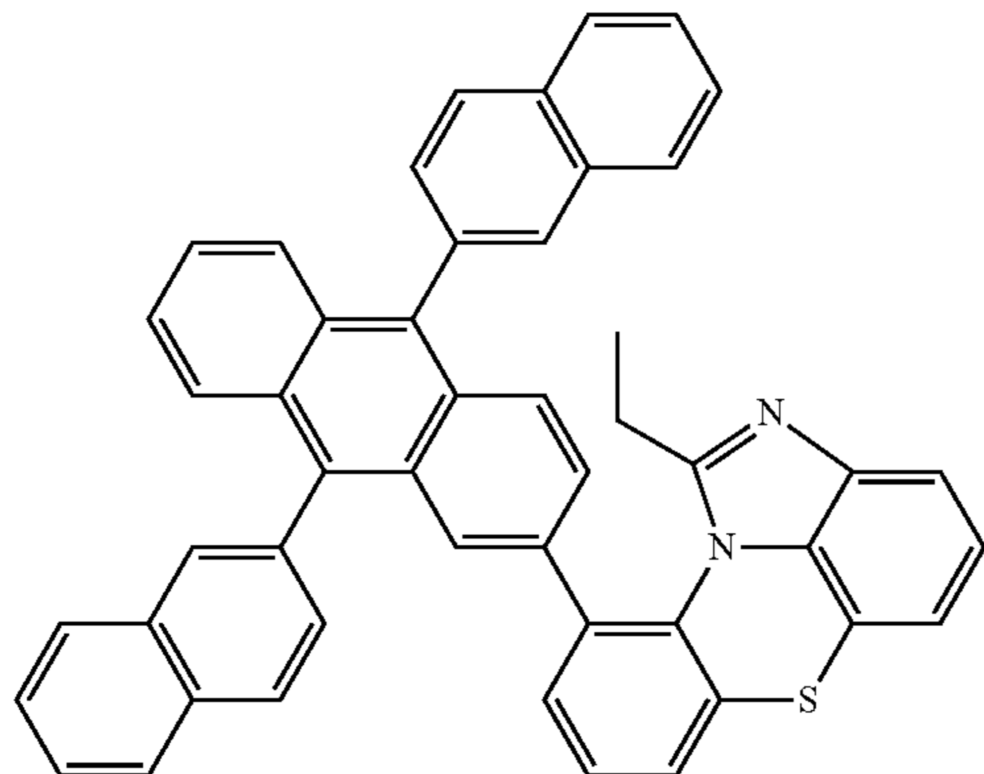
[Chemical Formula 2-3-21]
