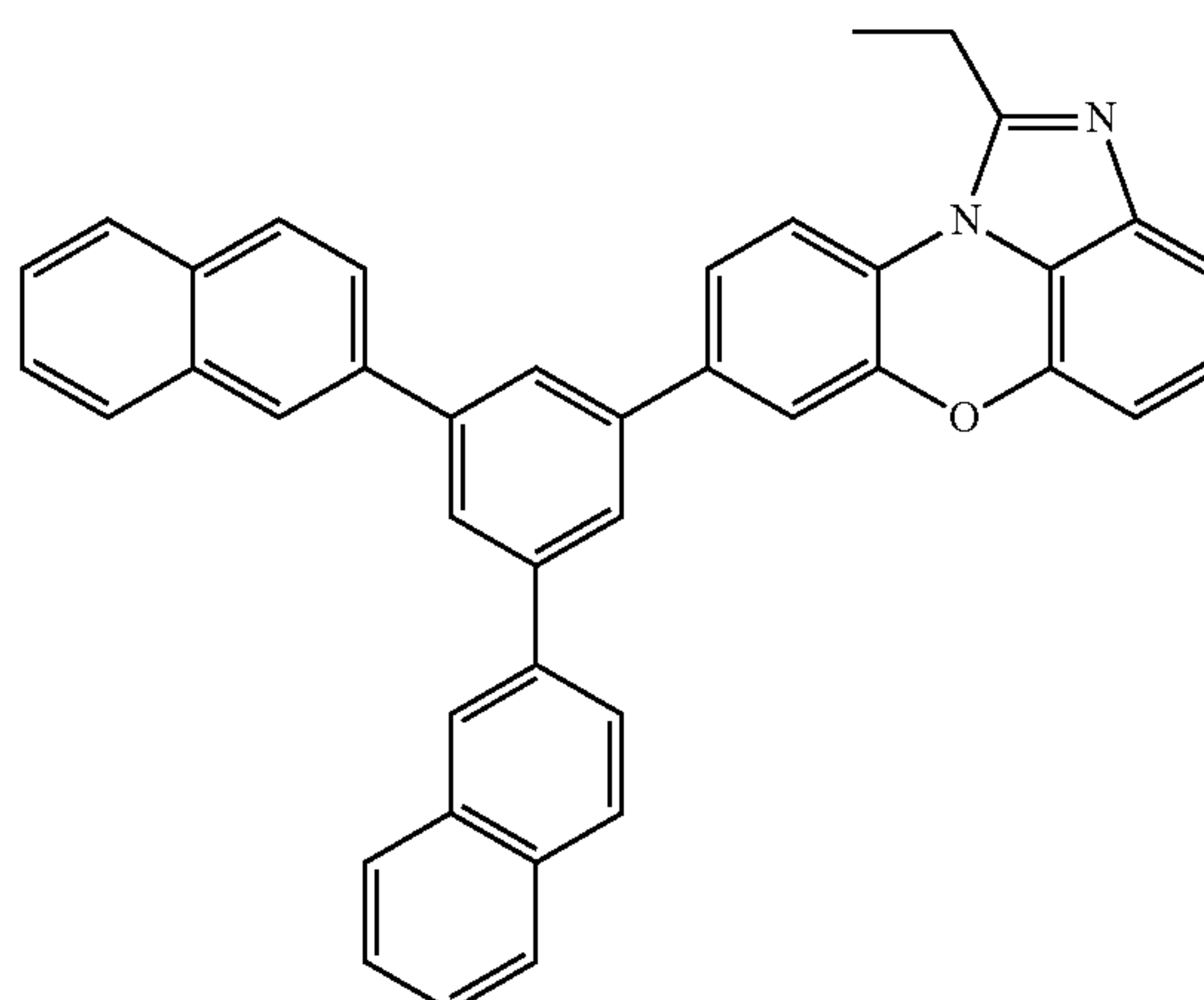
[Chemical Formula 1-3-43]
