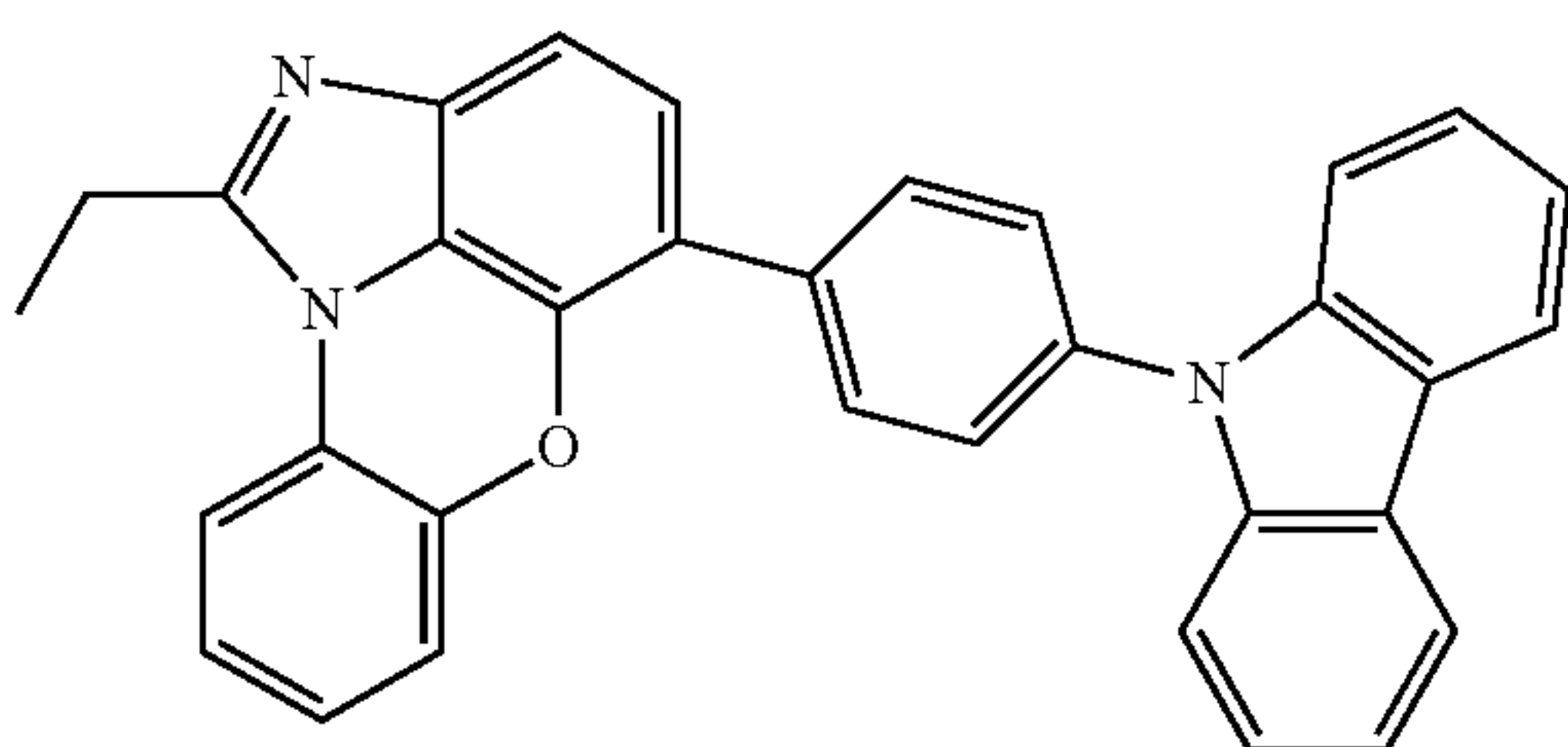
[Chemical Formula 1-9-6]
