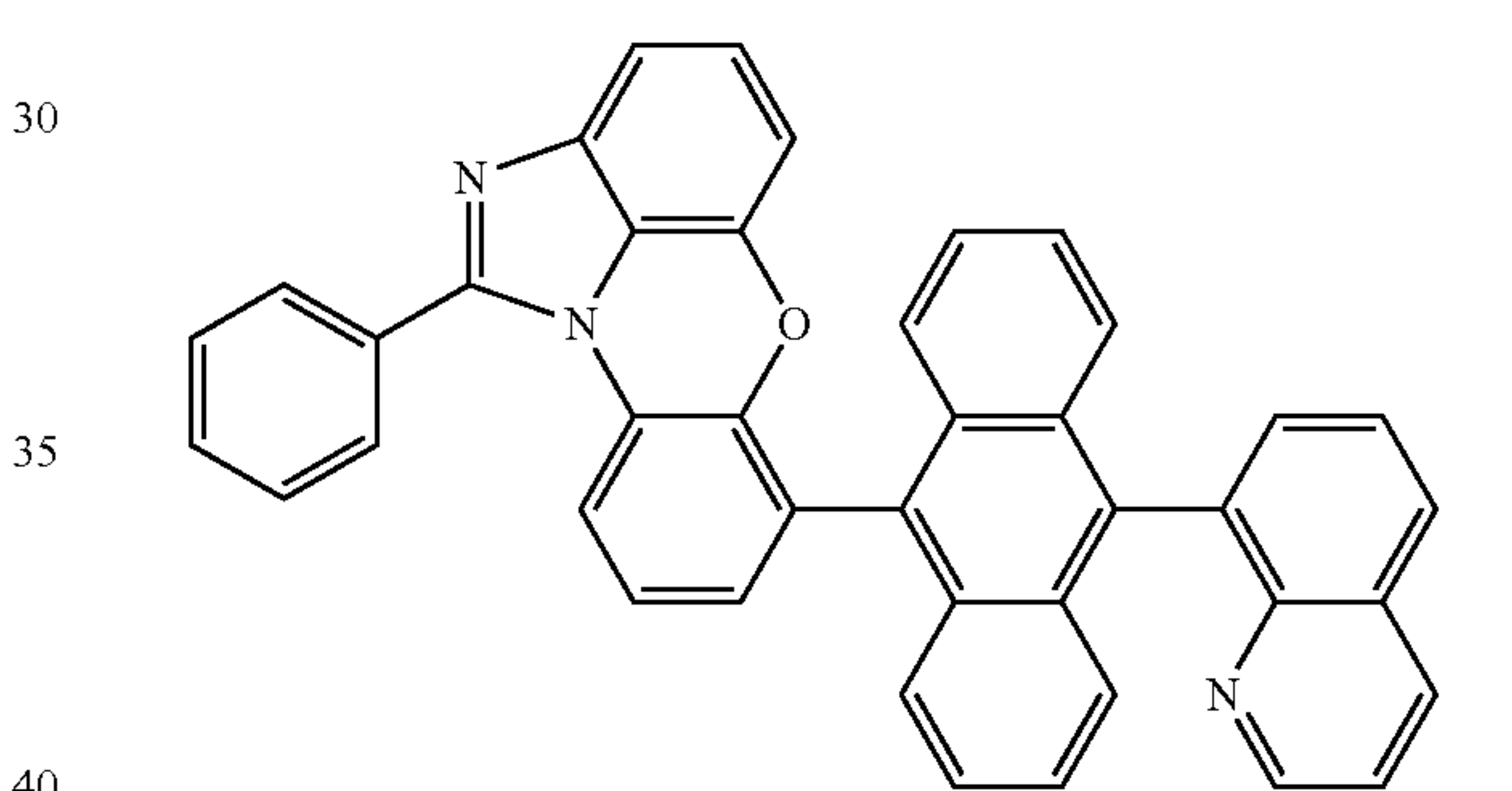
[Chemical Formula 1-6-12]
