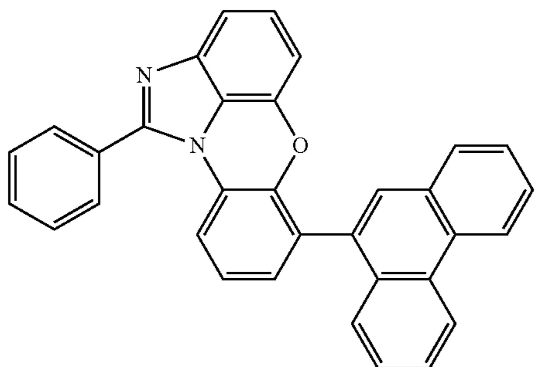
[Chemical Formula 1-6-32]
