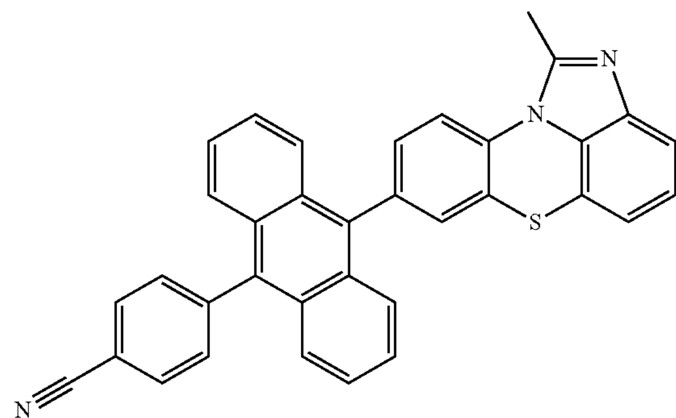
[Chemical Formula 2-2-12]
