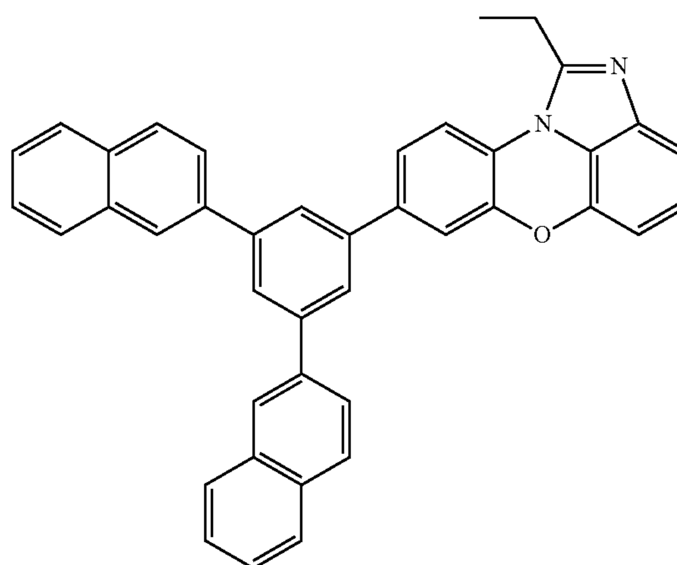
[Chemical Formula 1-3-43]
