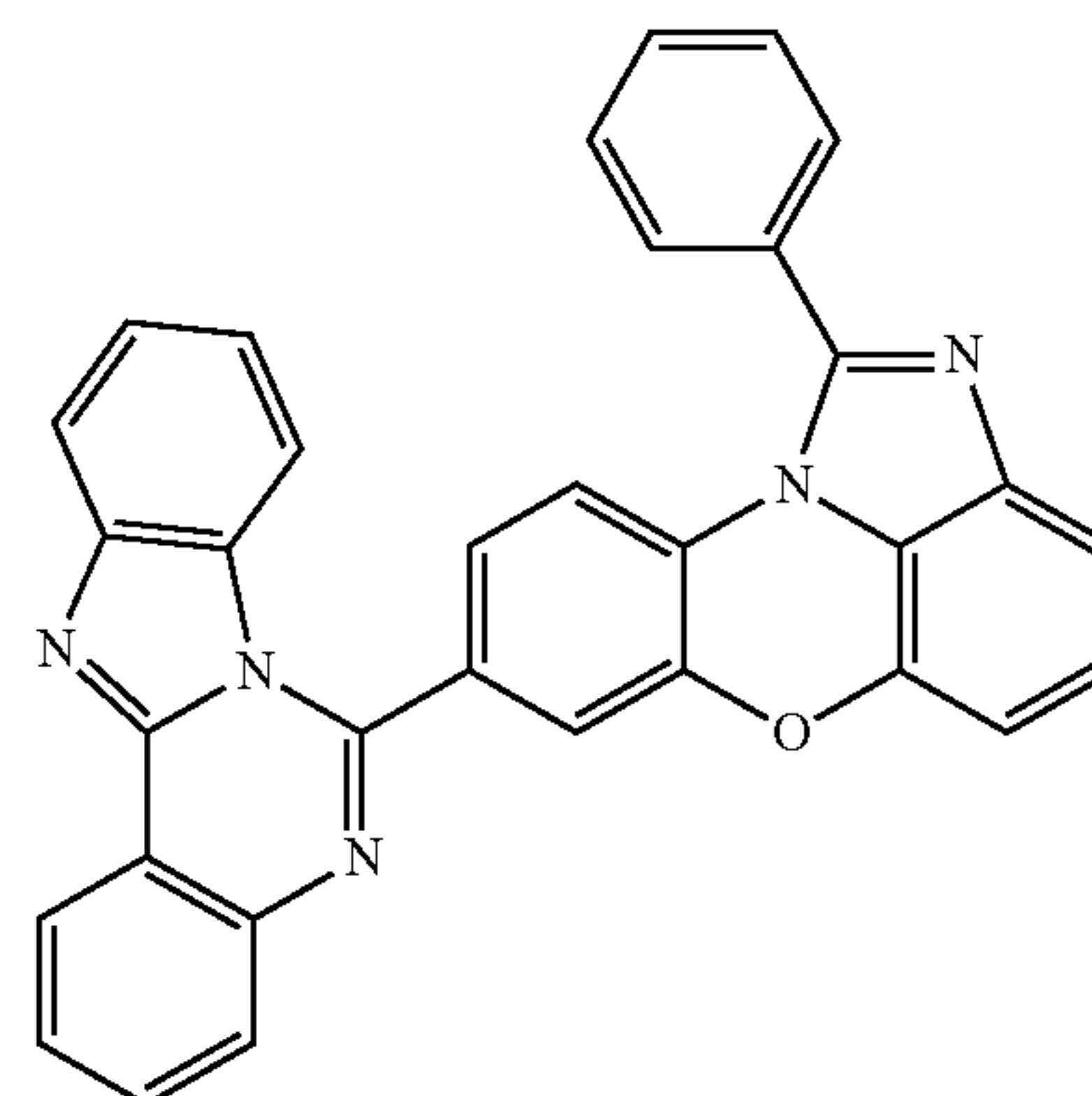
[Chemical Formula 1-4-53]
