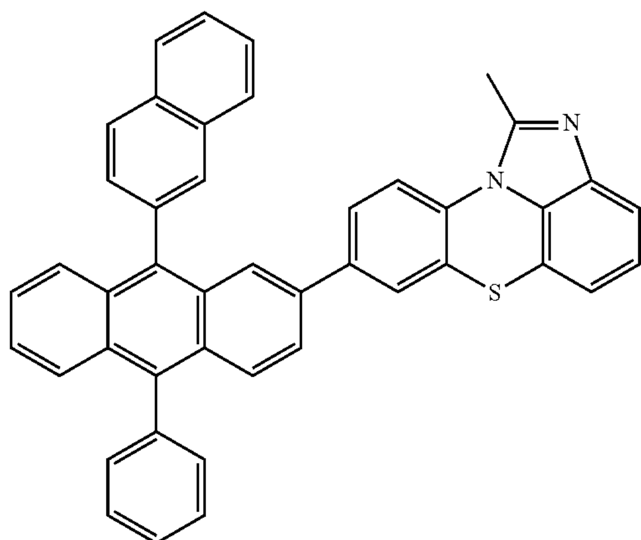
[Chemical Formula 2-2-23]
