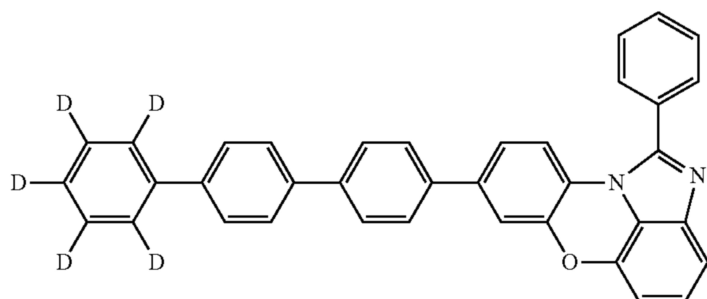
[Chemical Formula 1-4-52]
