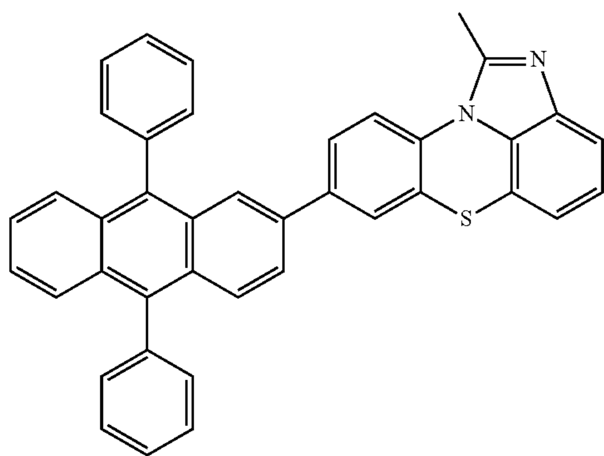
[Chemical Formula 2-2-20]
