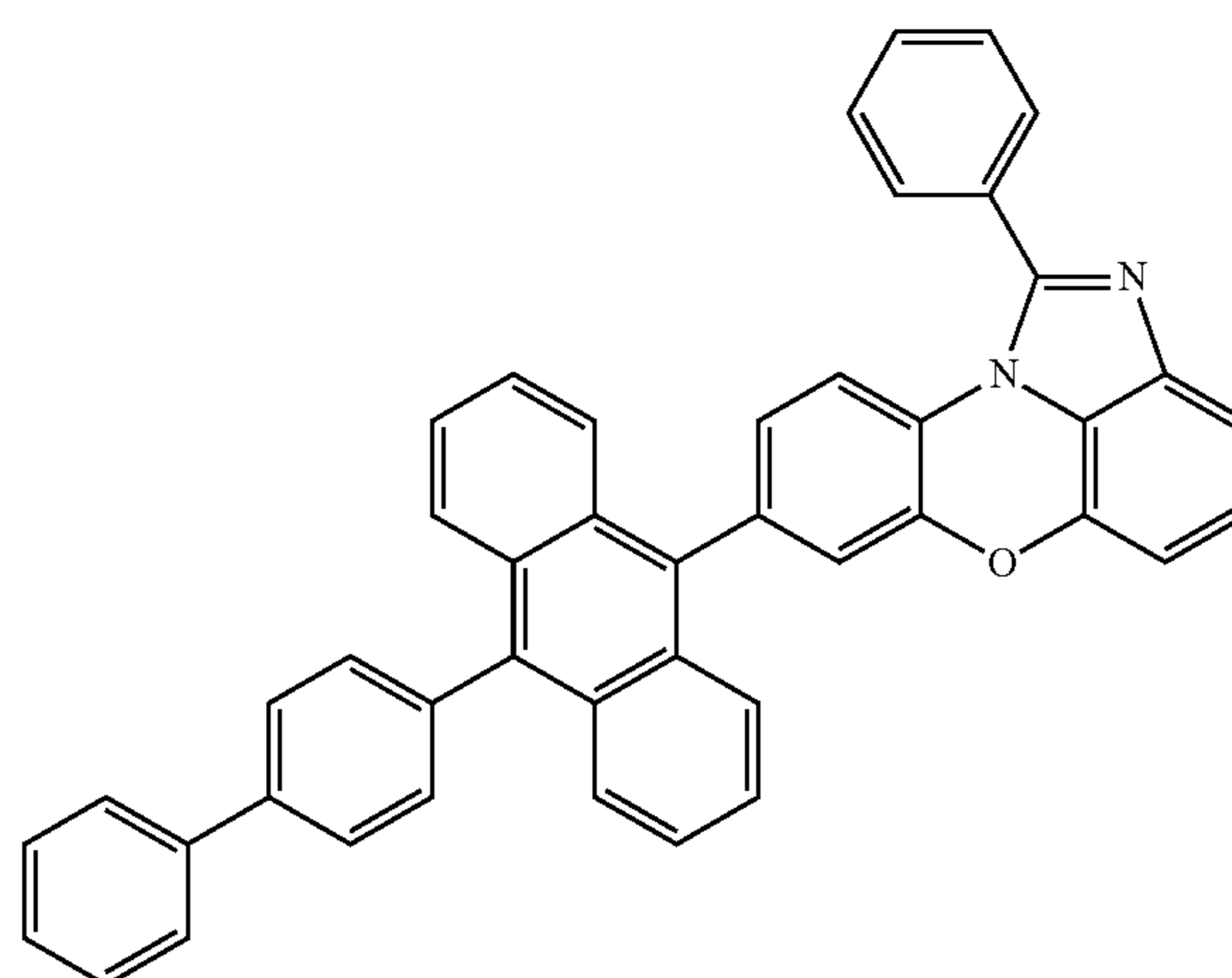
[Chemical Formula 1-4-4]
