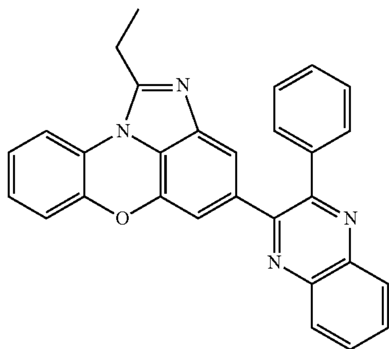
[Chemical Formula 1-10-13]
