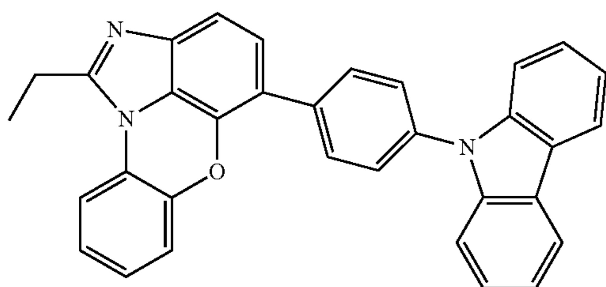
[Chemical Formula 1-9-6]
