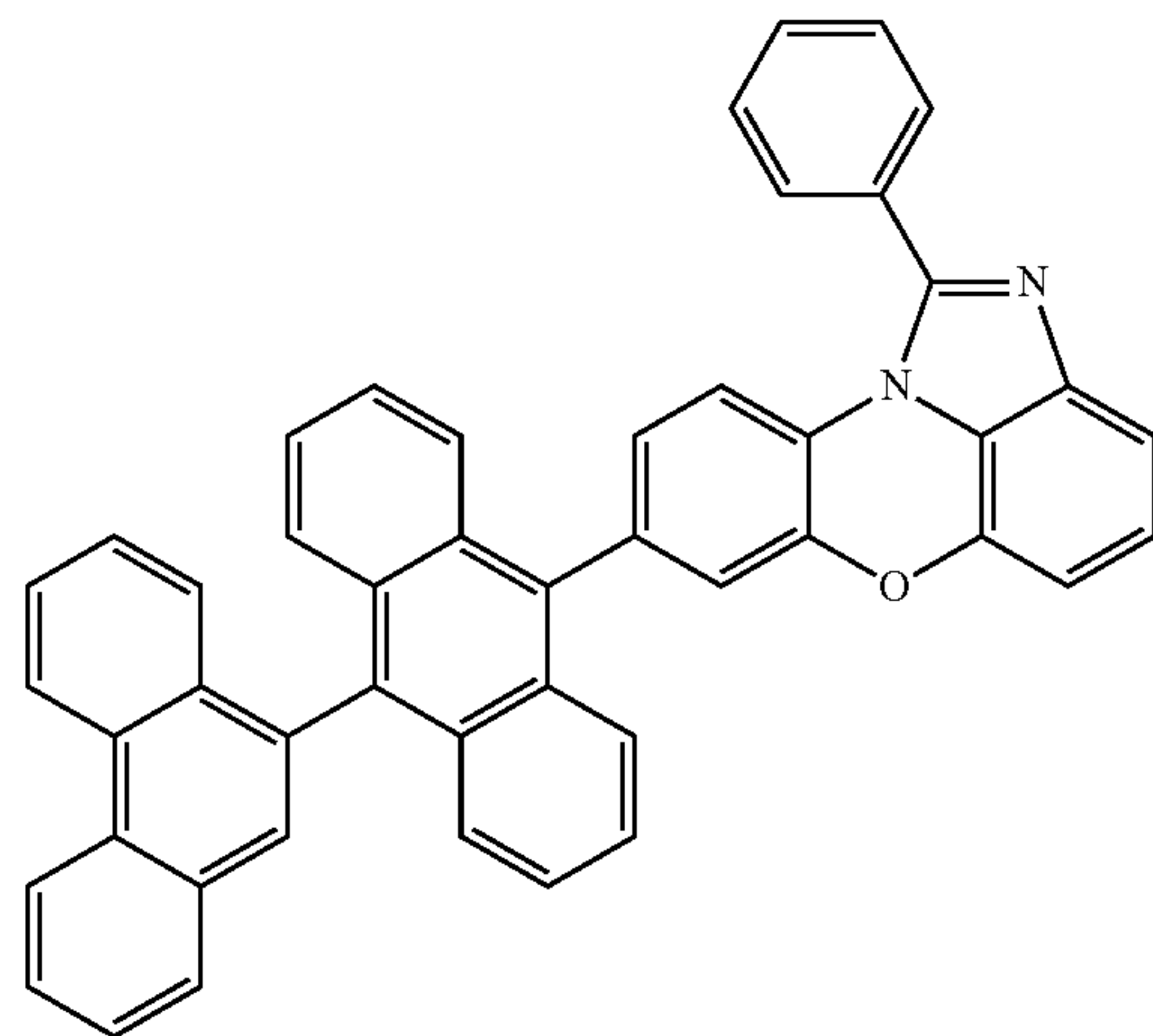
[Chemical Formula 1-4-7]
