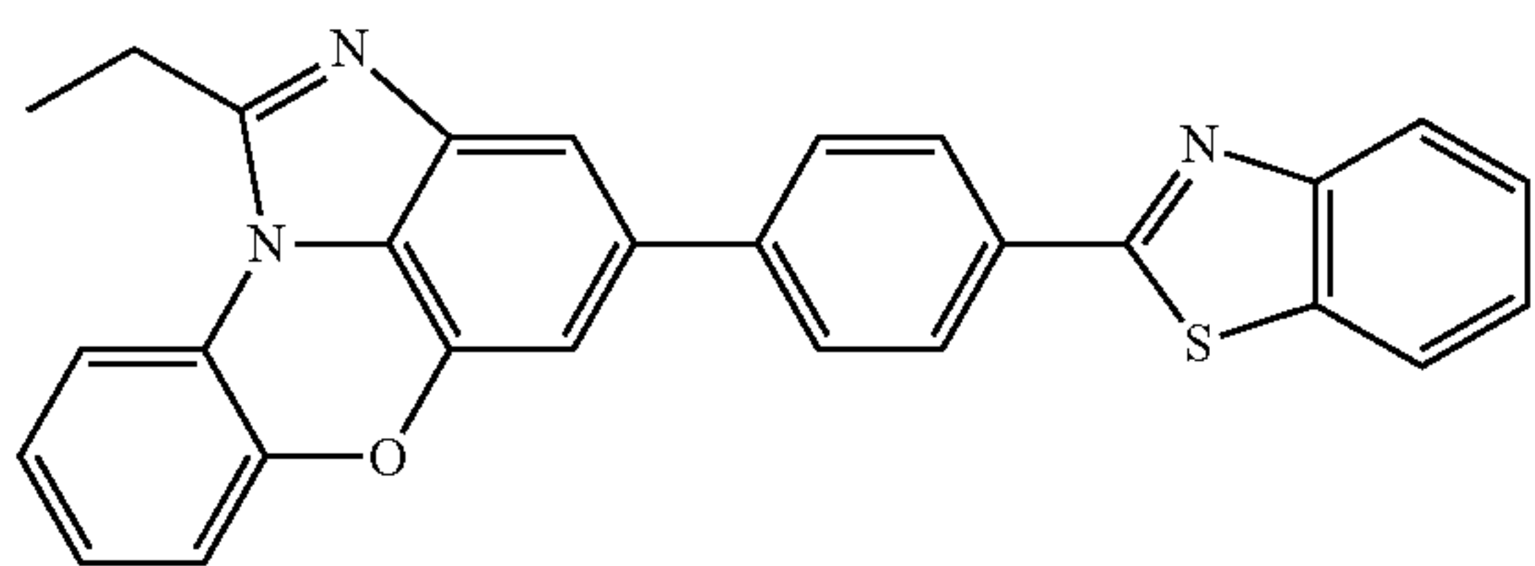
[Chemical Formula 1-10-10]
