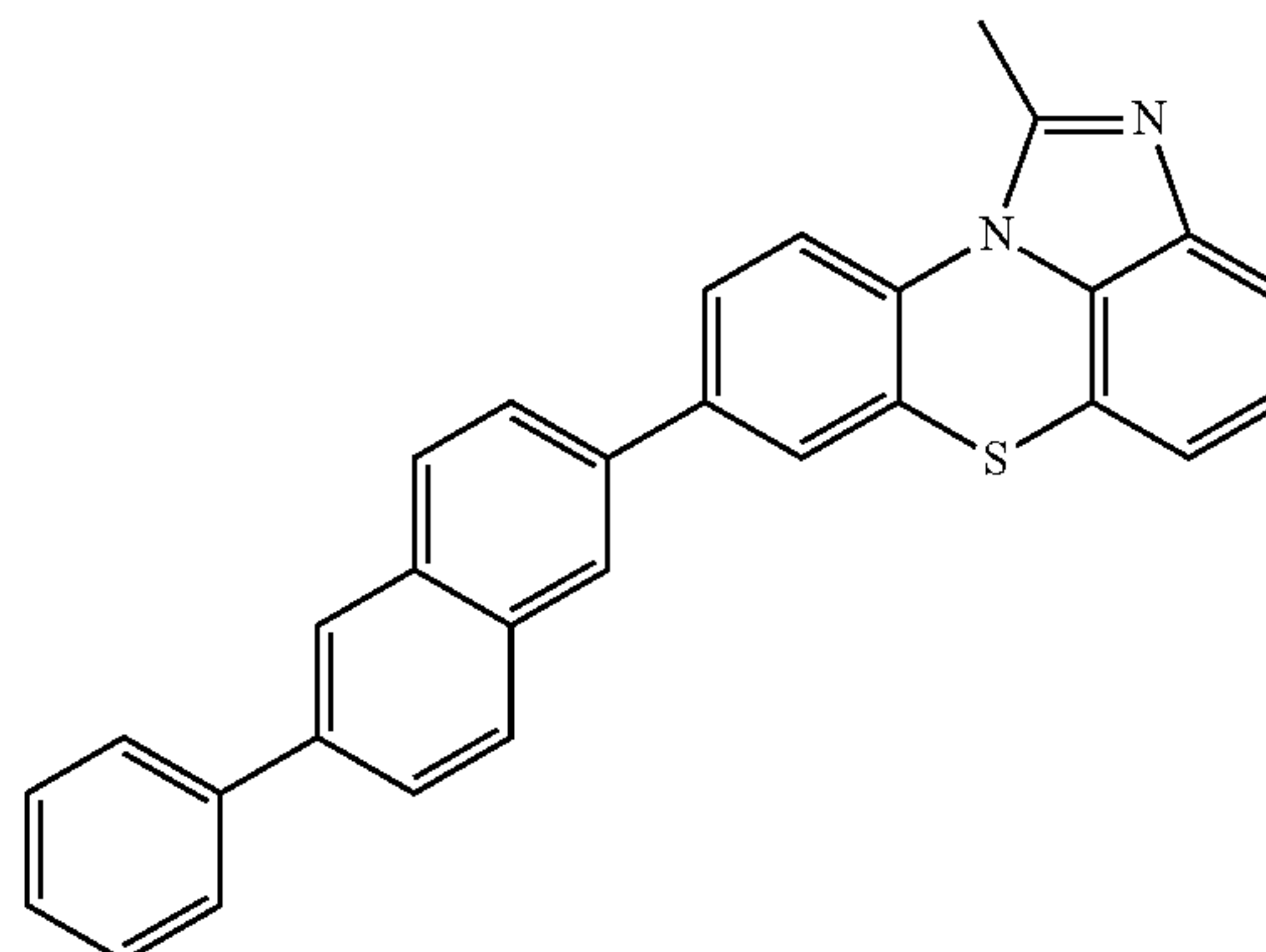
[Chemical Formula 2-2-27]
