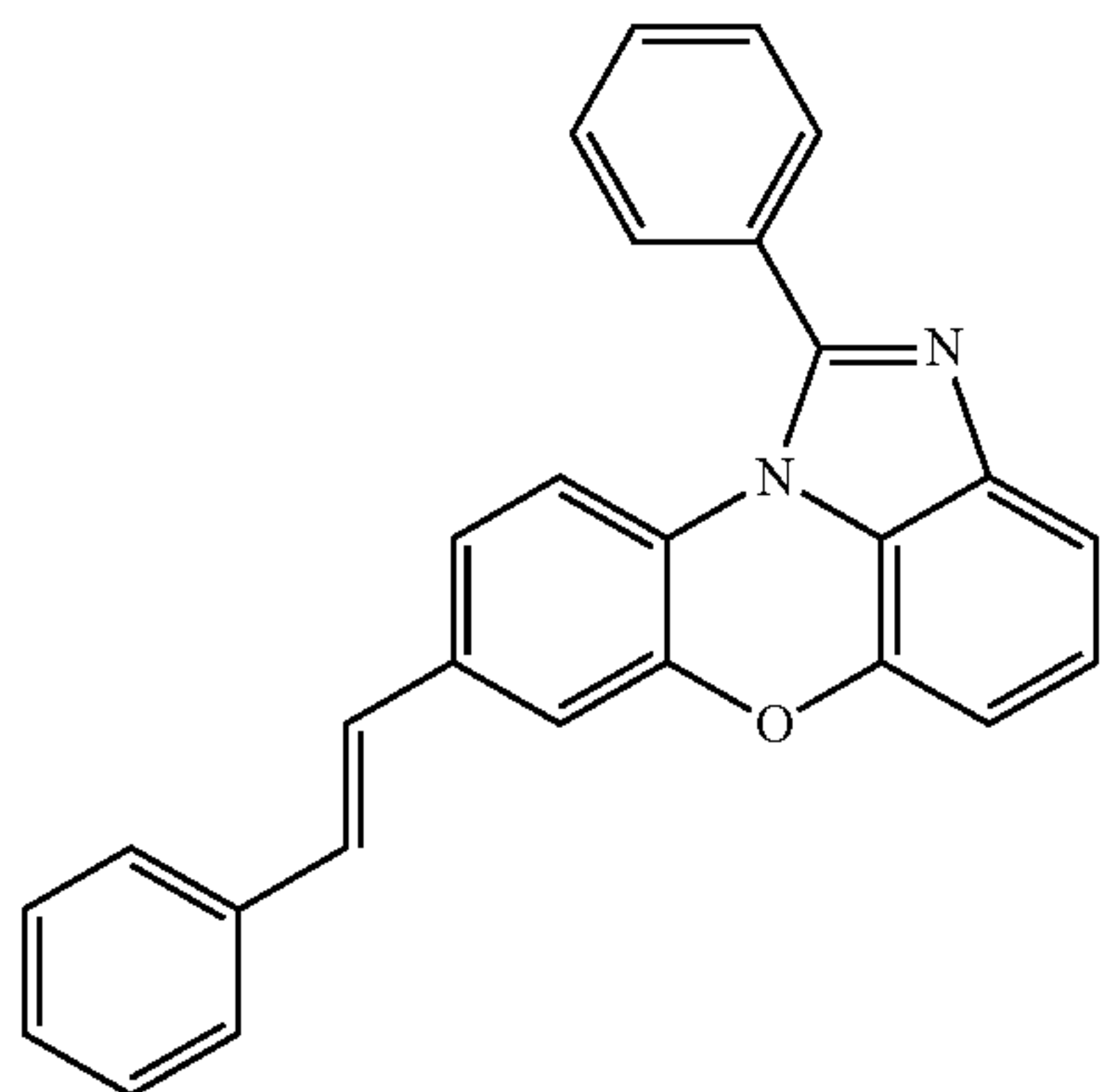
[Chemical Formula 1-4-54]
