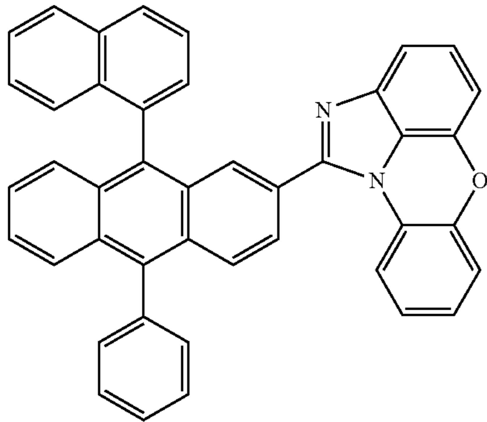
[Chemical Formula 1-1-30] 5
