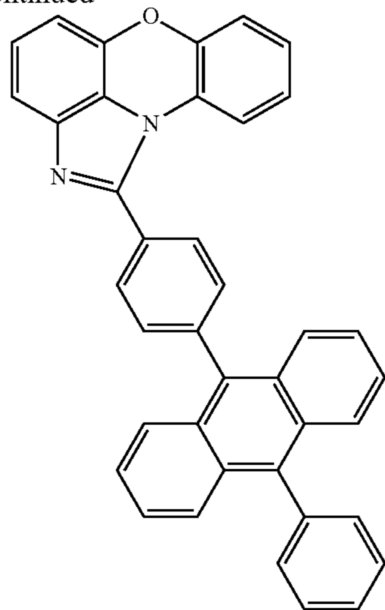
[Chemical Formula 1-1-25]
