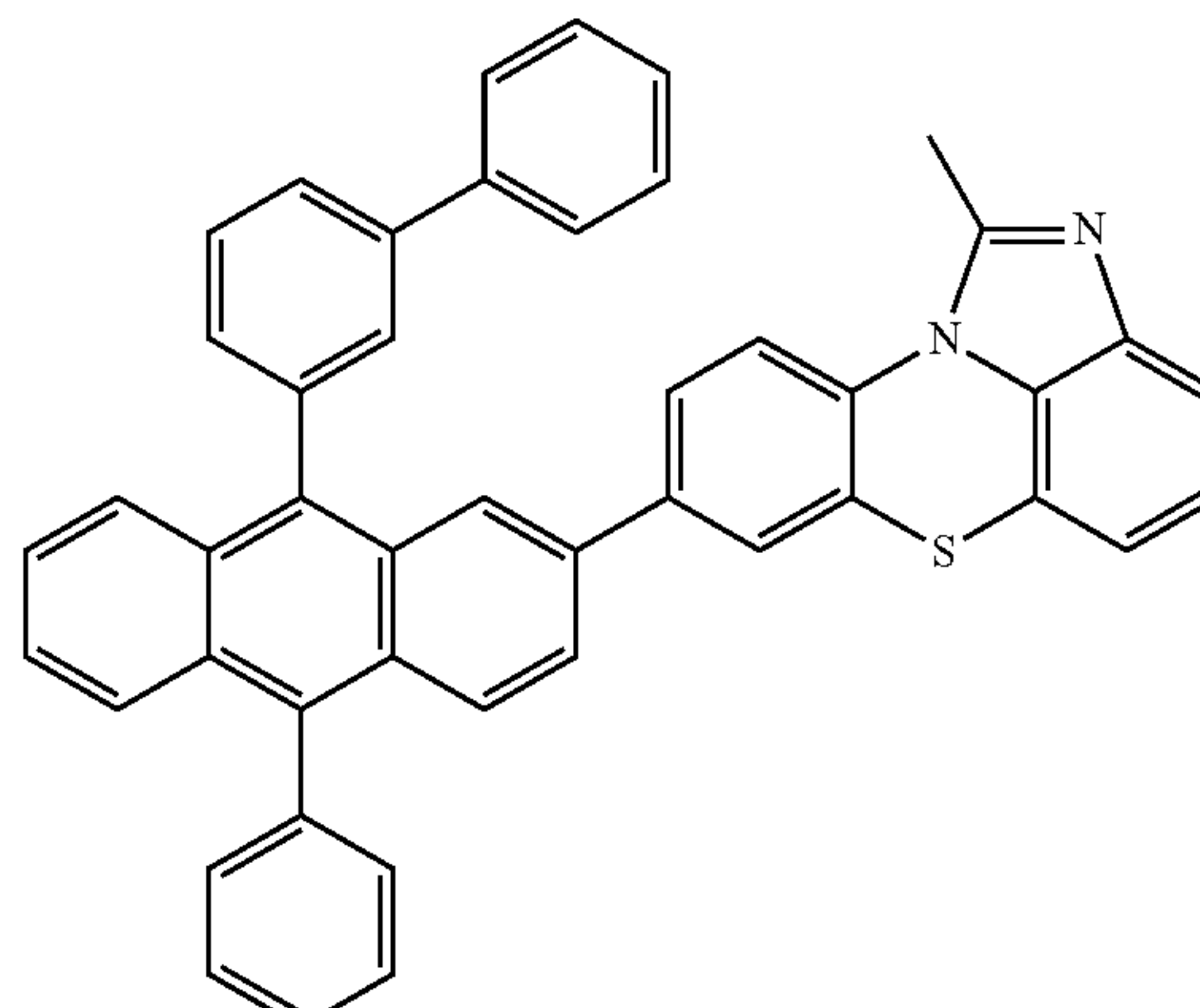
[Chemical Formula 2-2-25]
