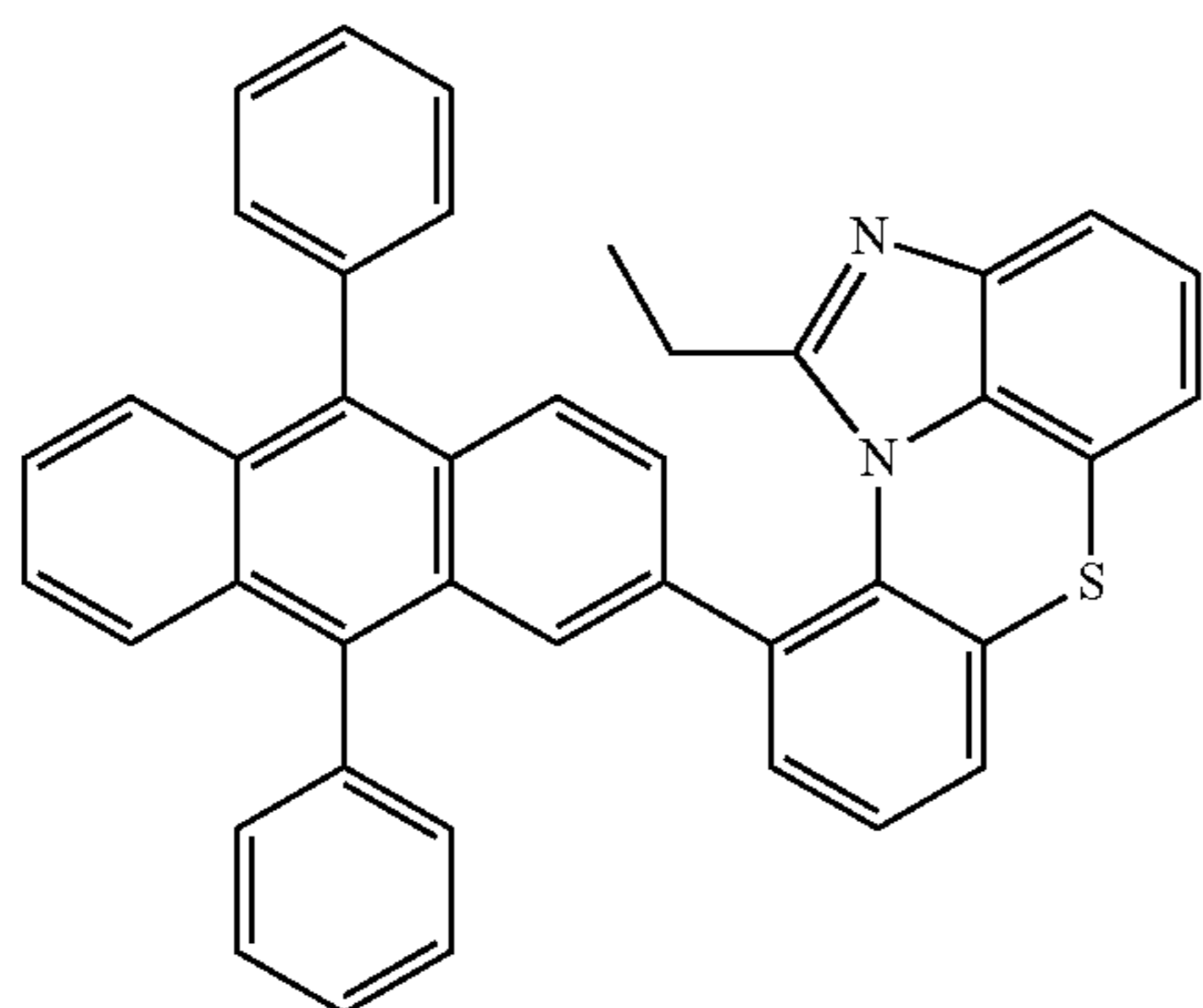
[Chemical Formula 2-3-20]
