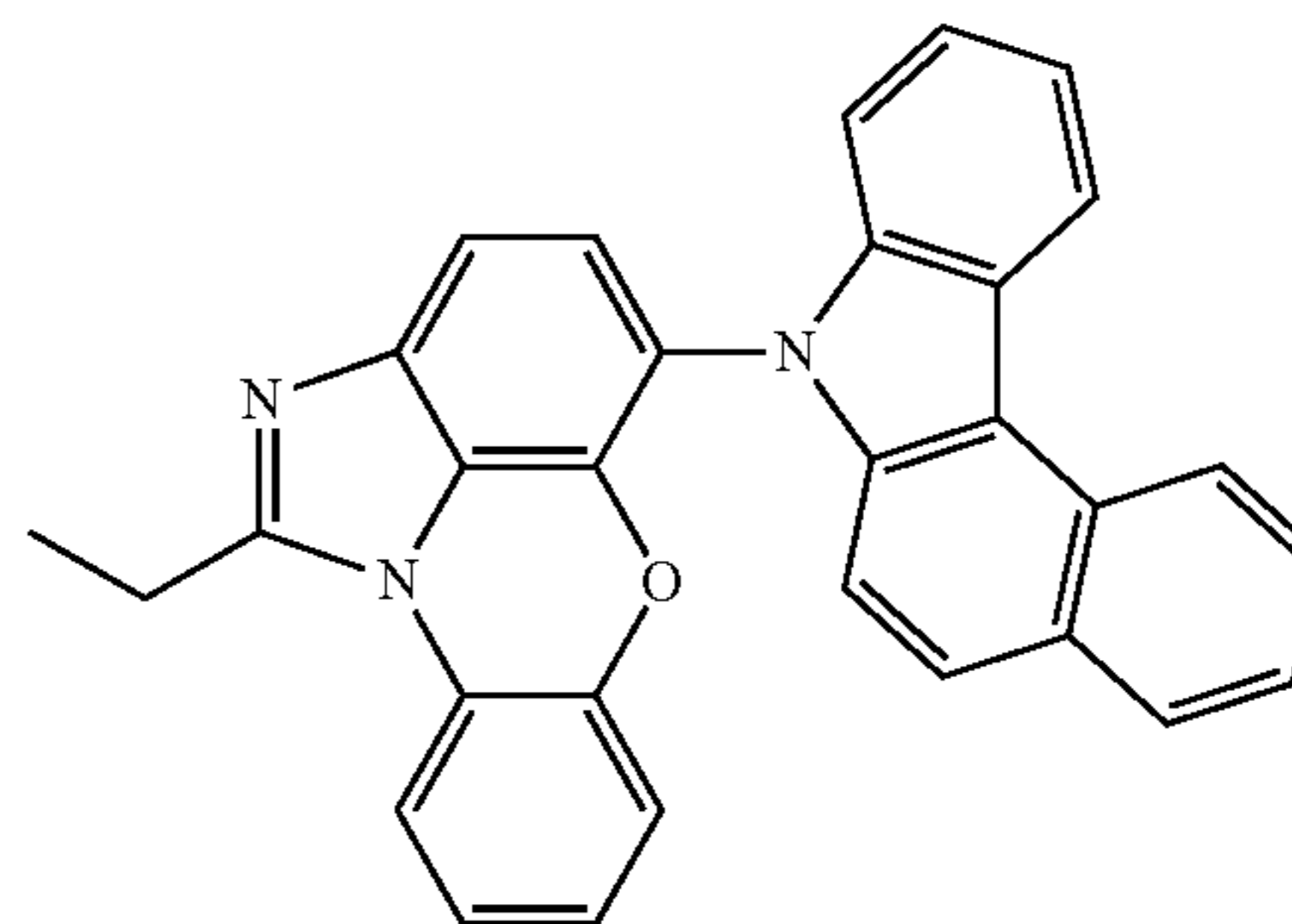
[Chemical Formula 1-9-15]
