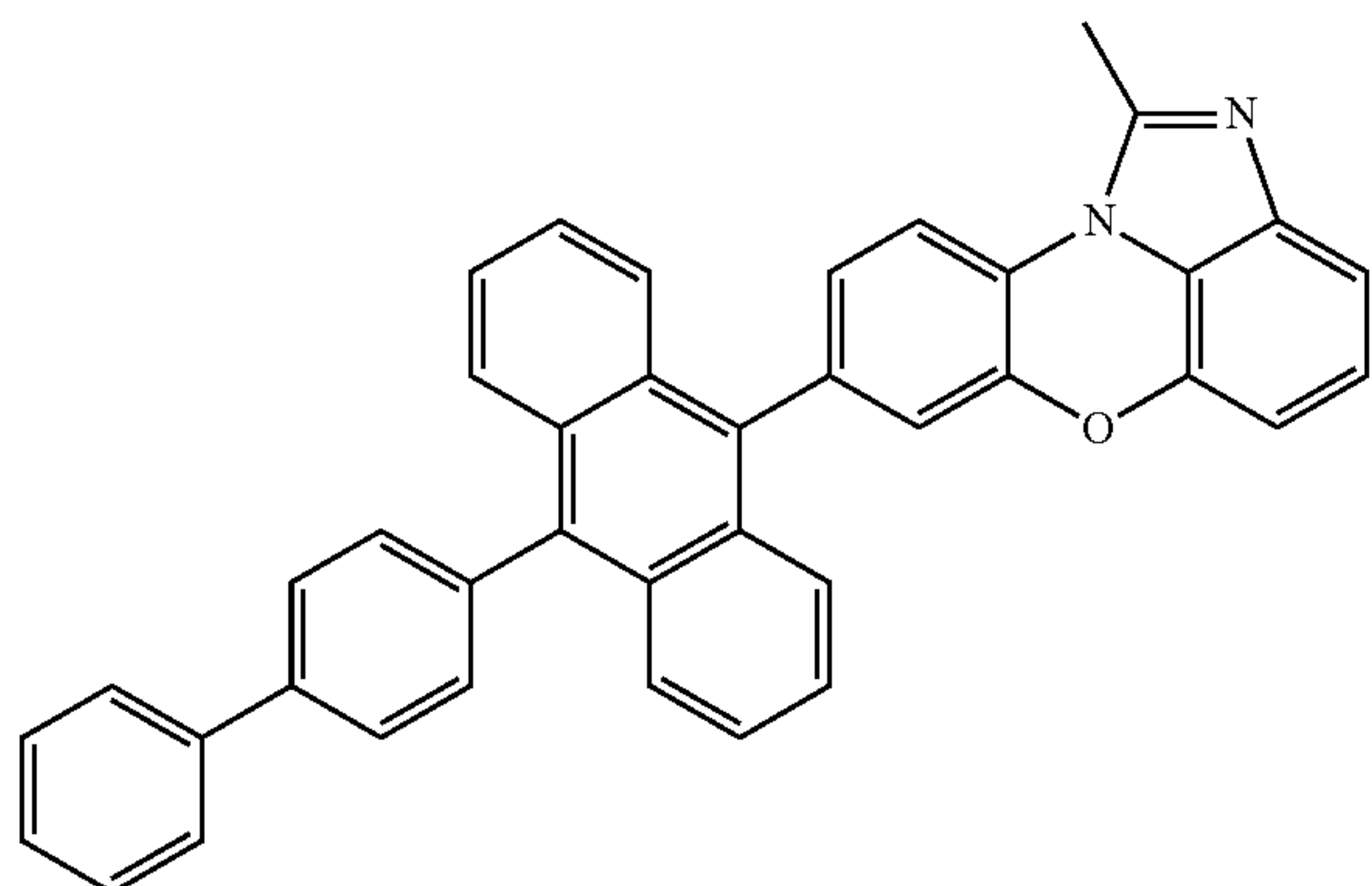
[Chemical Formula 1-2-5]
