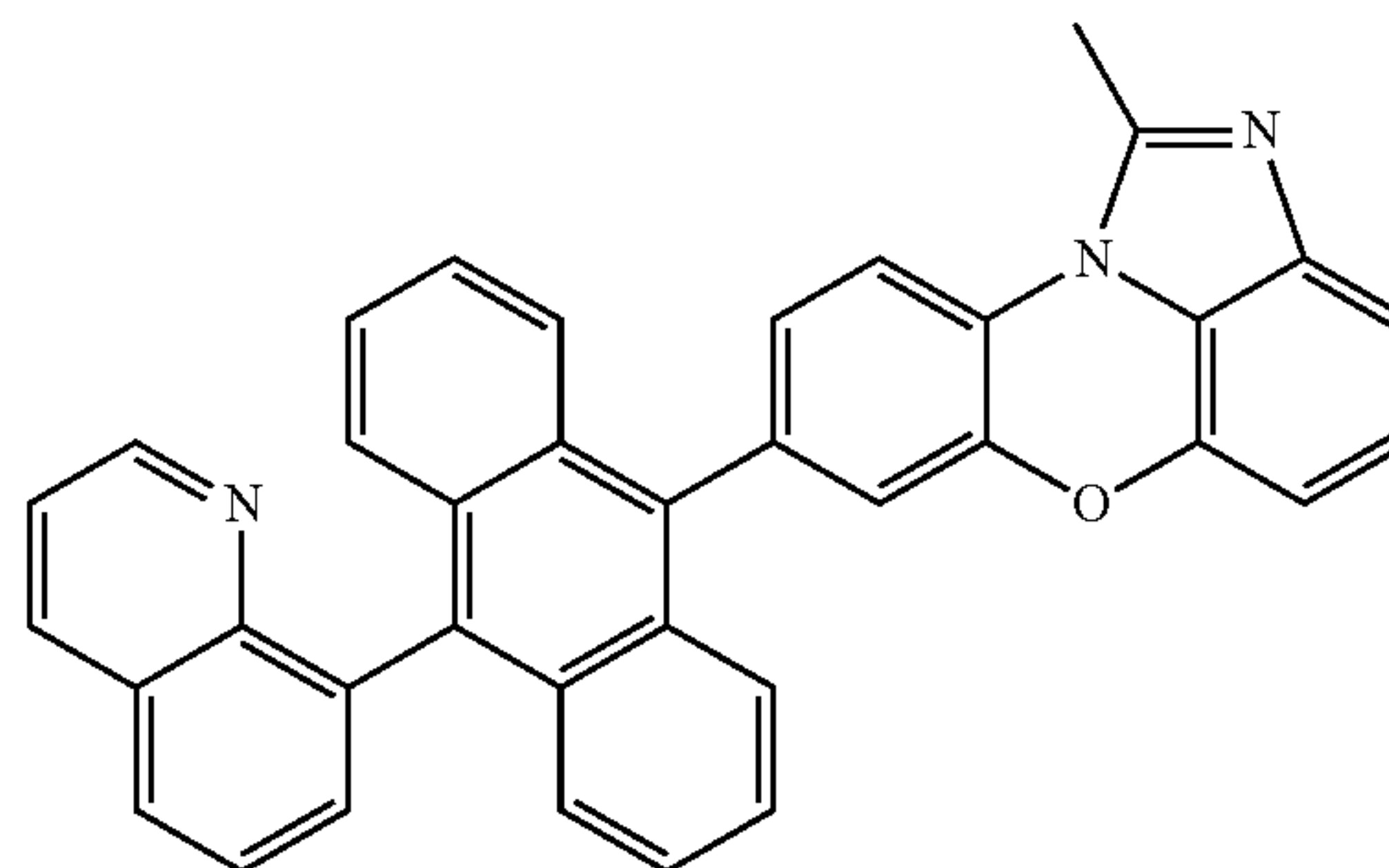
[Chemical Formula 1-2-11]
