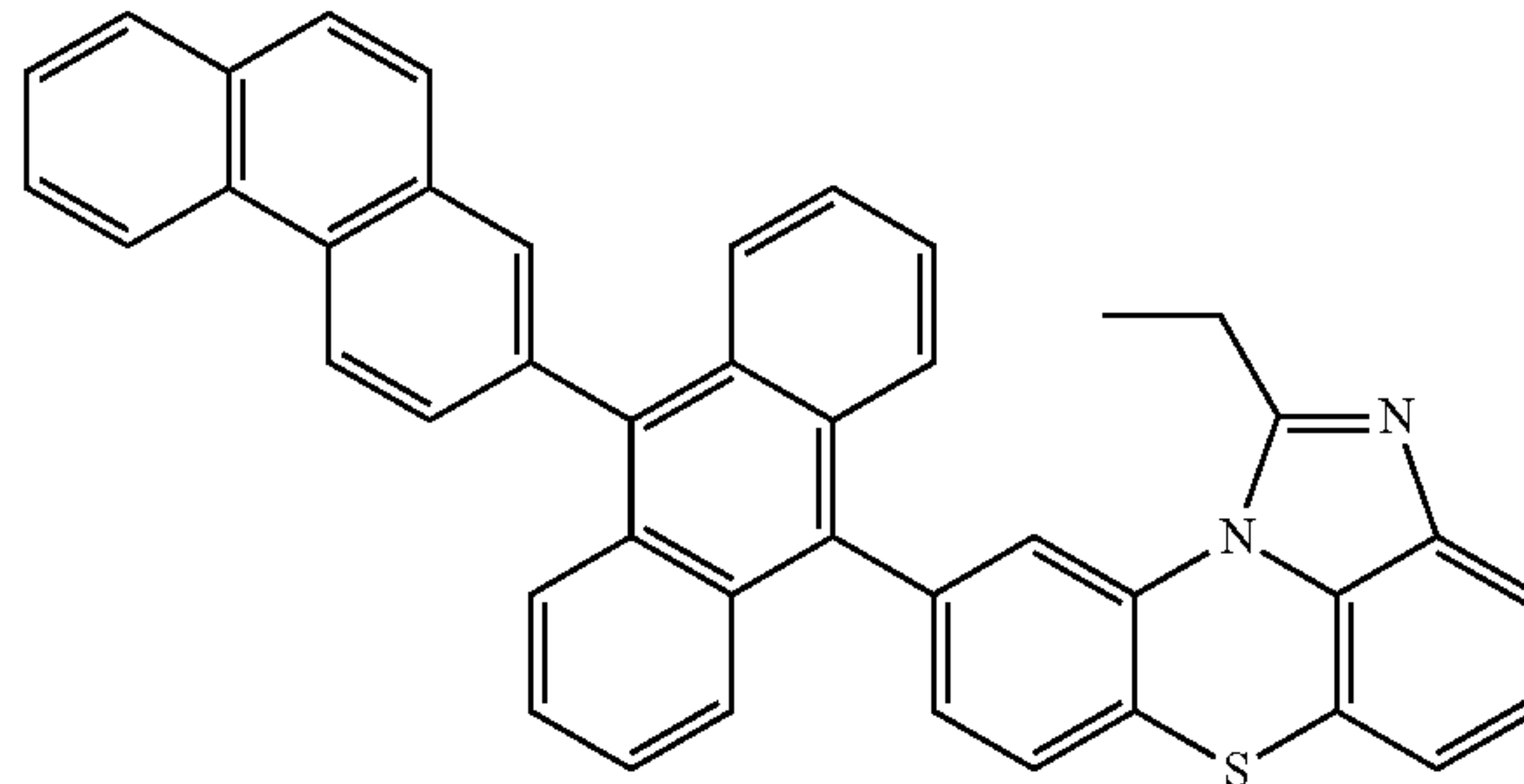
[Chemical Formula 2-3-9]
