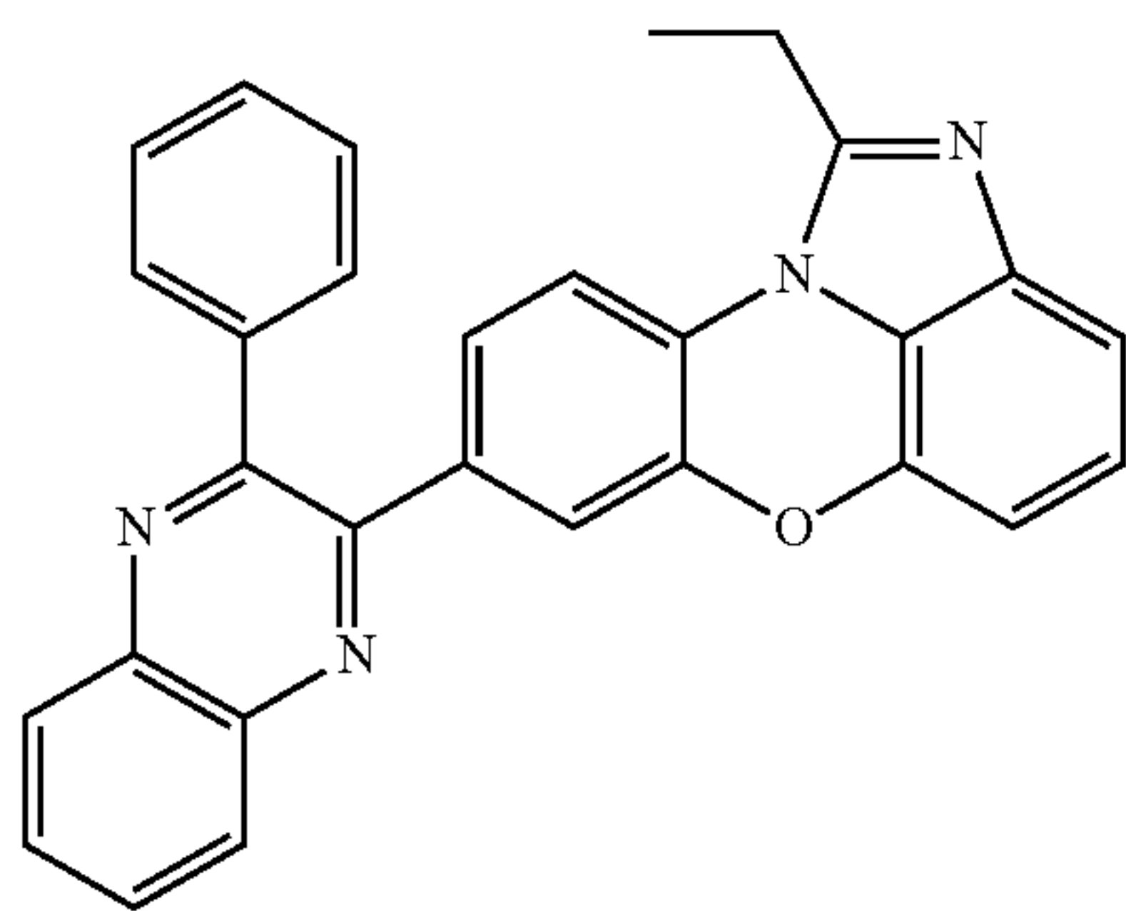
[Chemical Formula 1-3-49]
