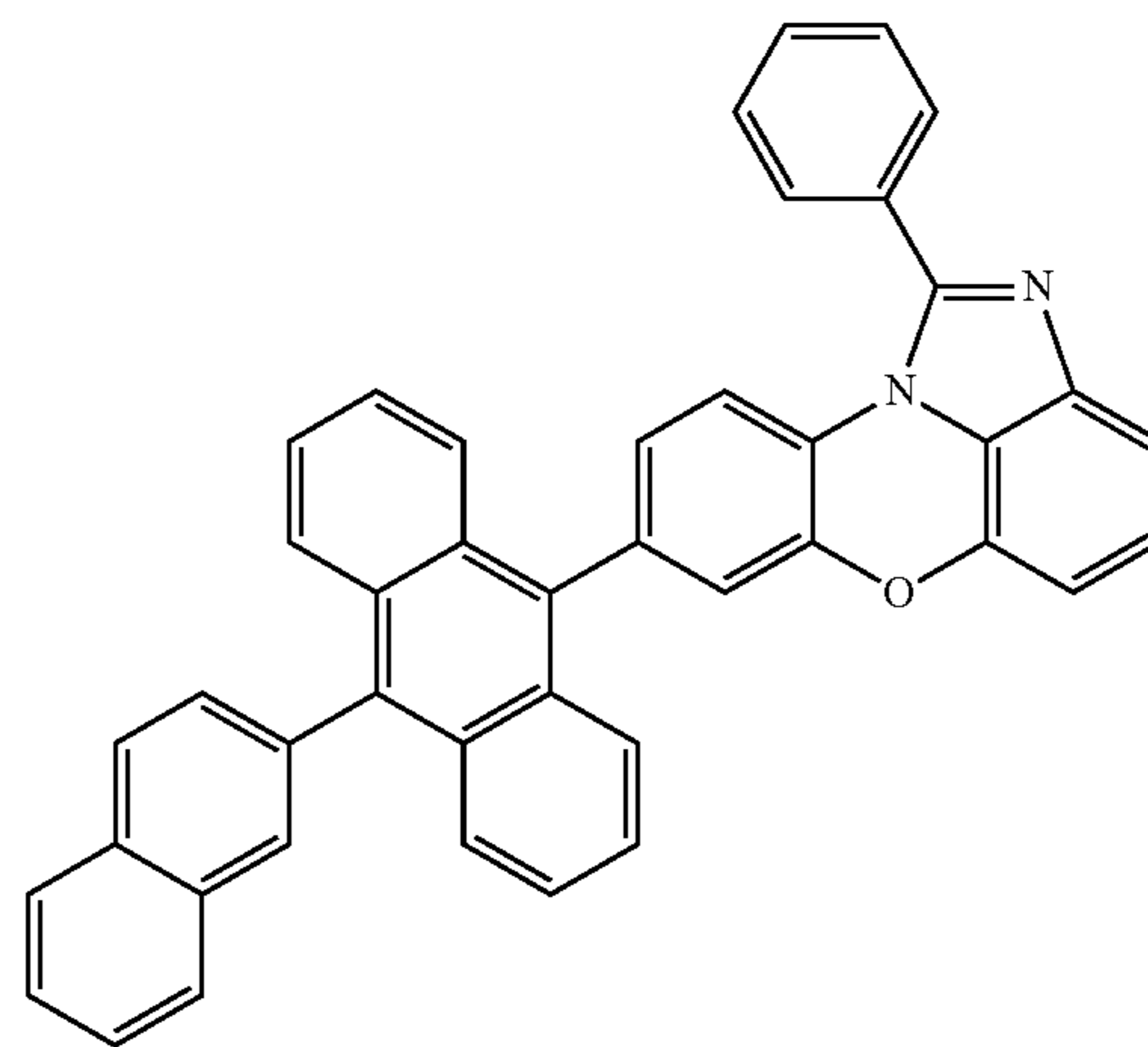
[Chemical Formula 1-4-2]
