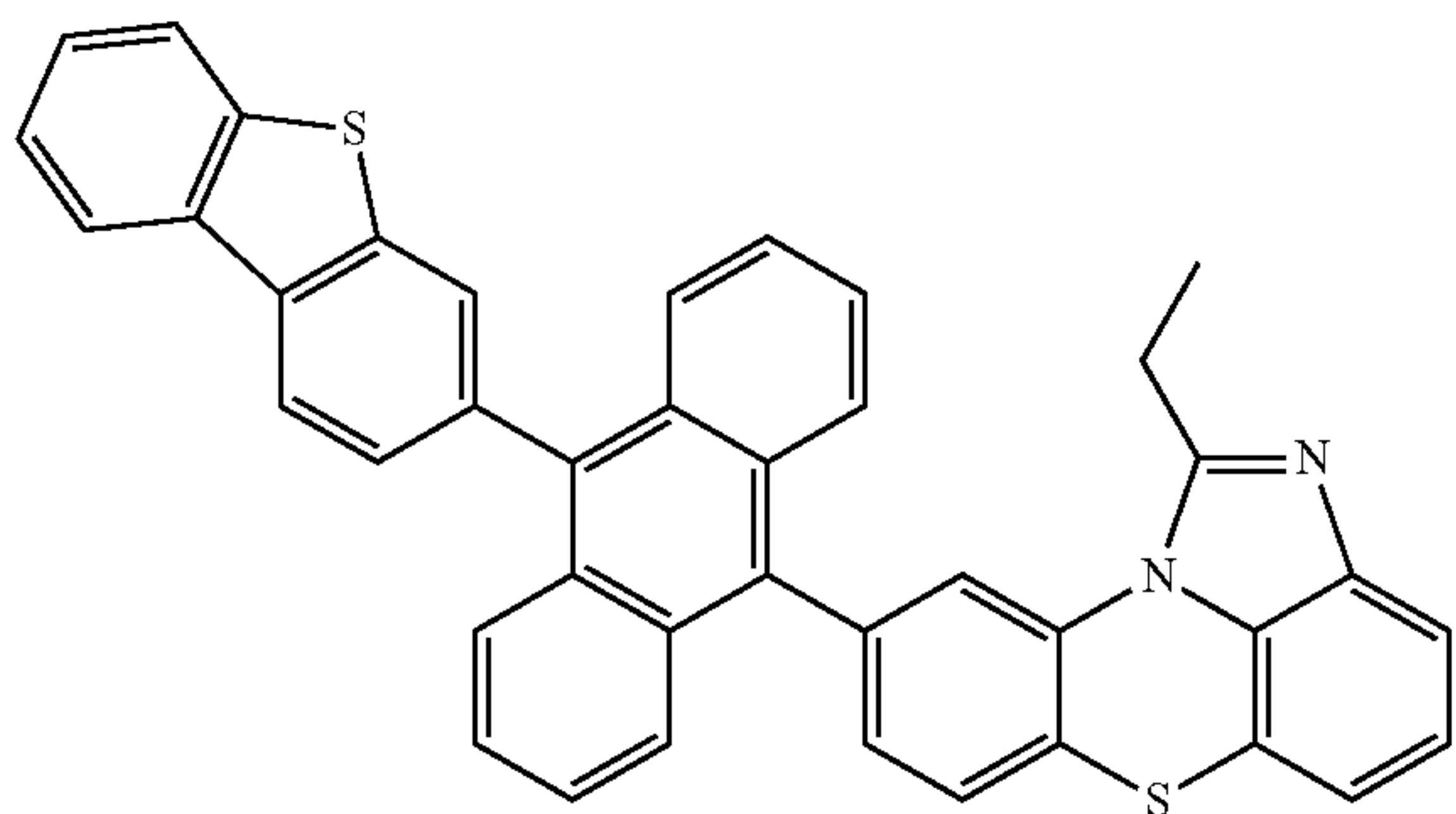
[Chemical Formula 2-3-14]
