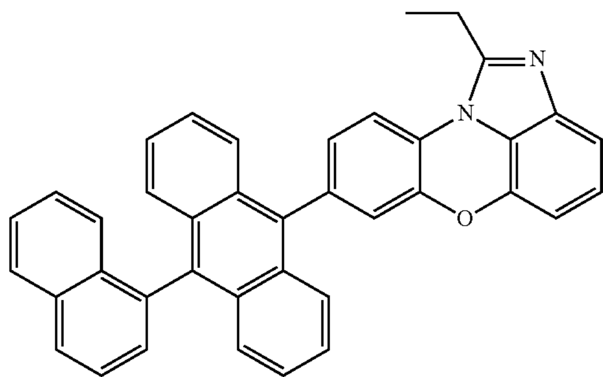
[Chemical Formula 1-3-3]
