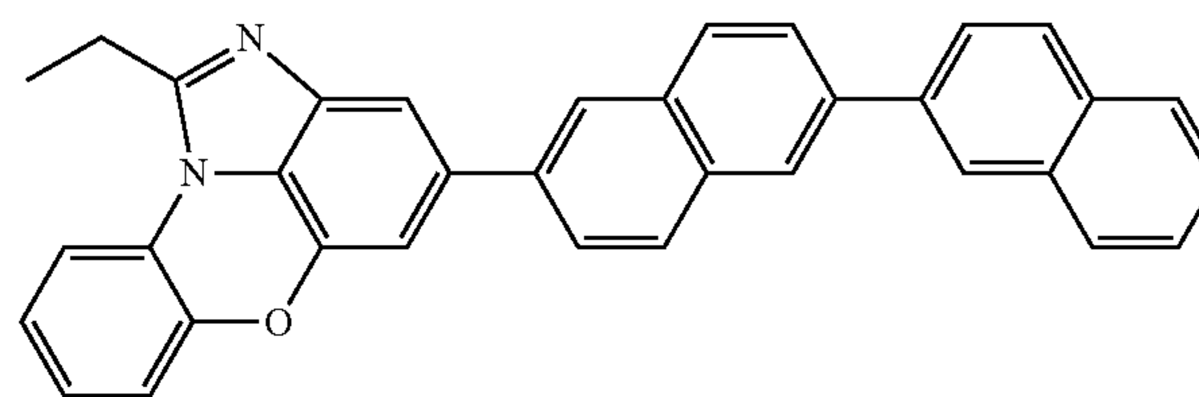
[Chemical Formula 1-10-8]
