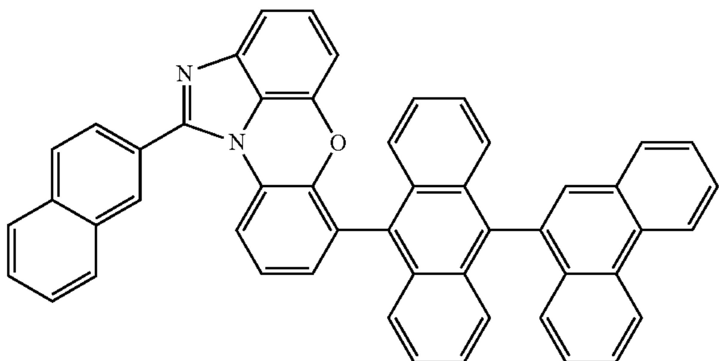
[Chemical Formula 1-6-8]
