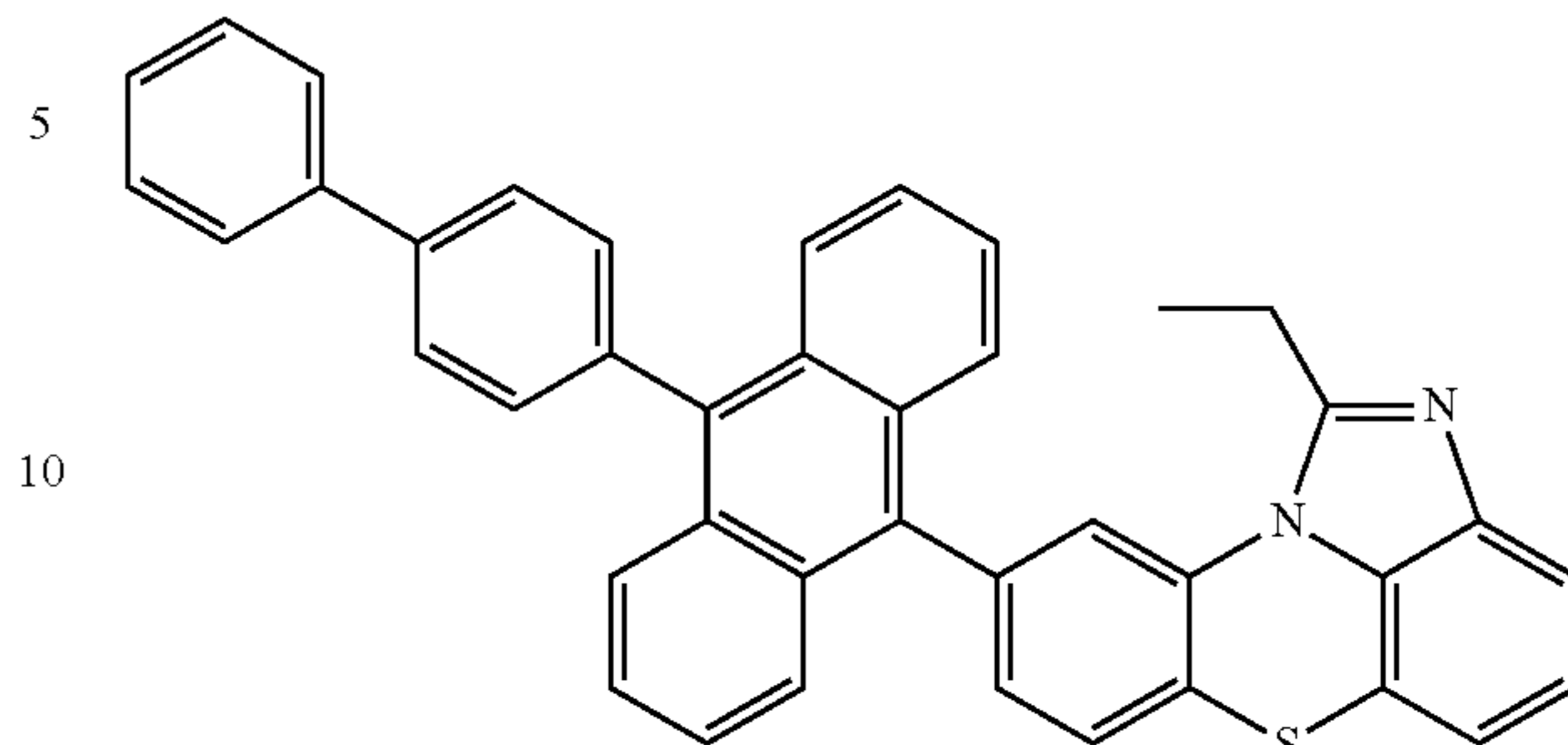
[Chemical Formula 2-3-4]
