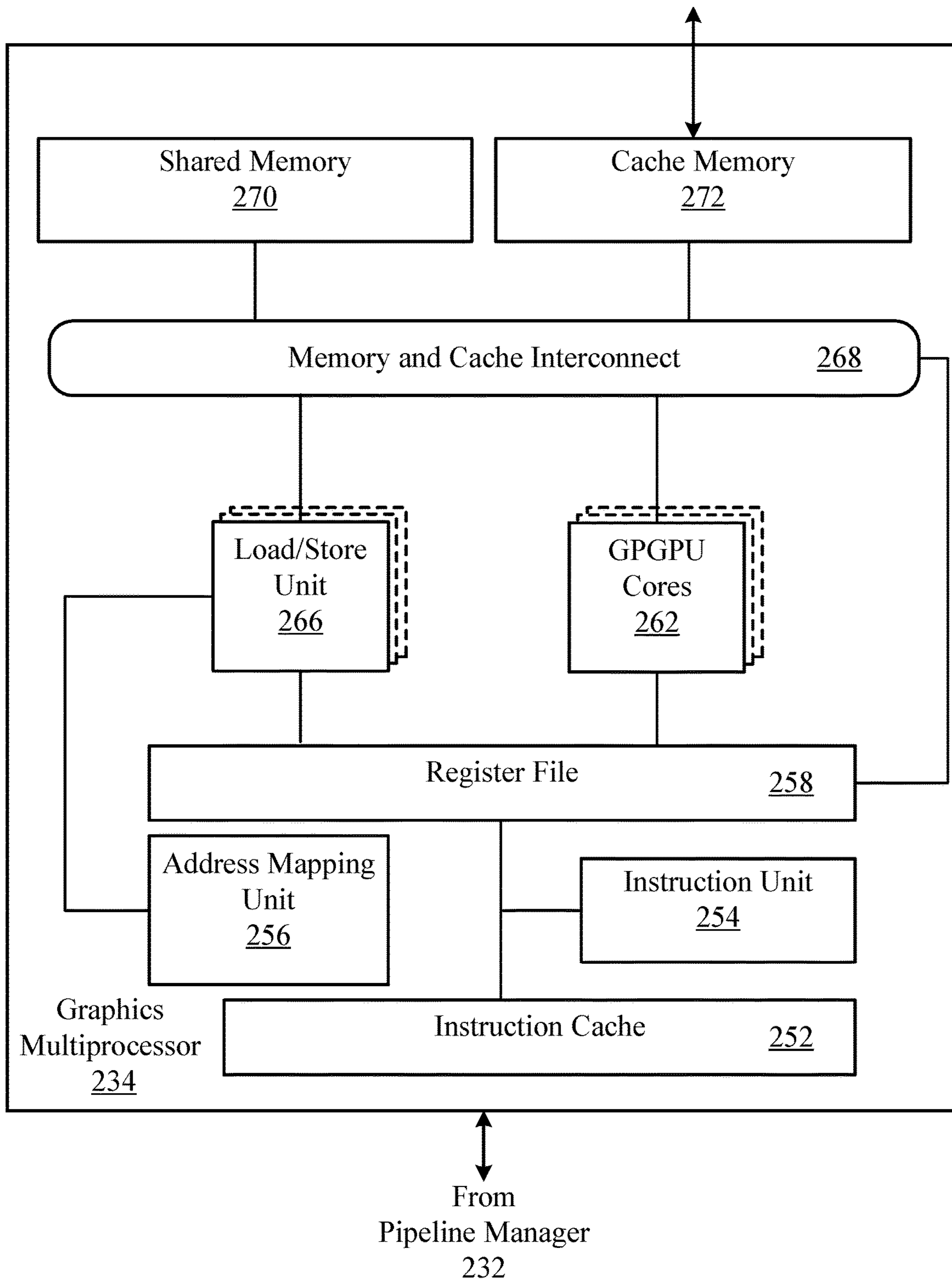
FIG. 2D
