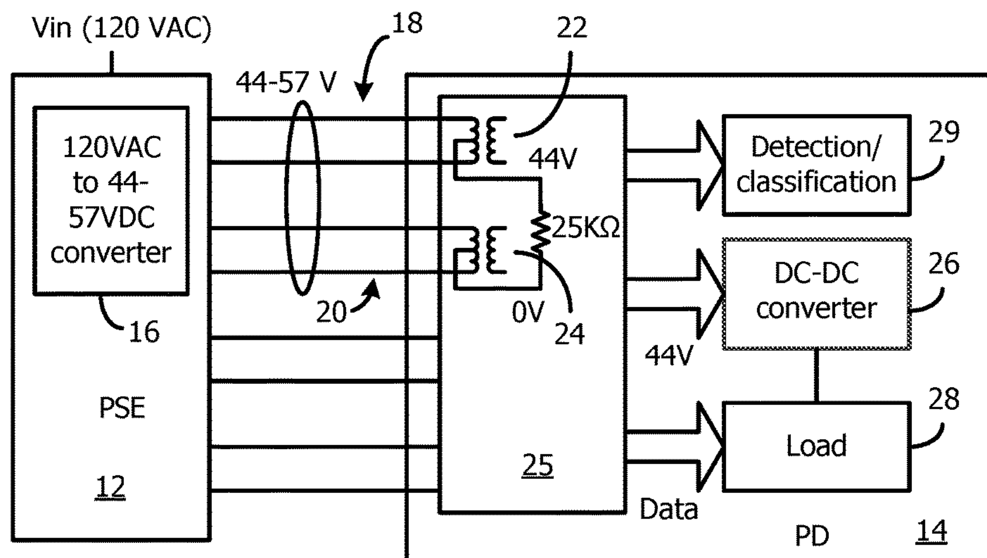
Fig. 1 (prior art)
