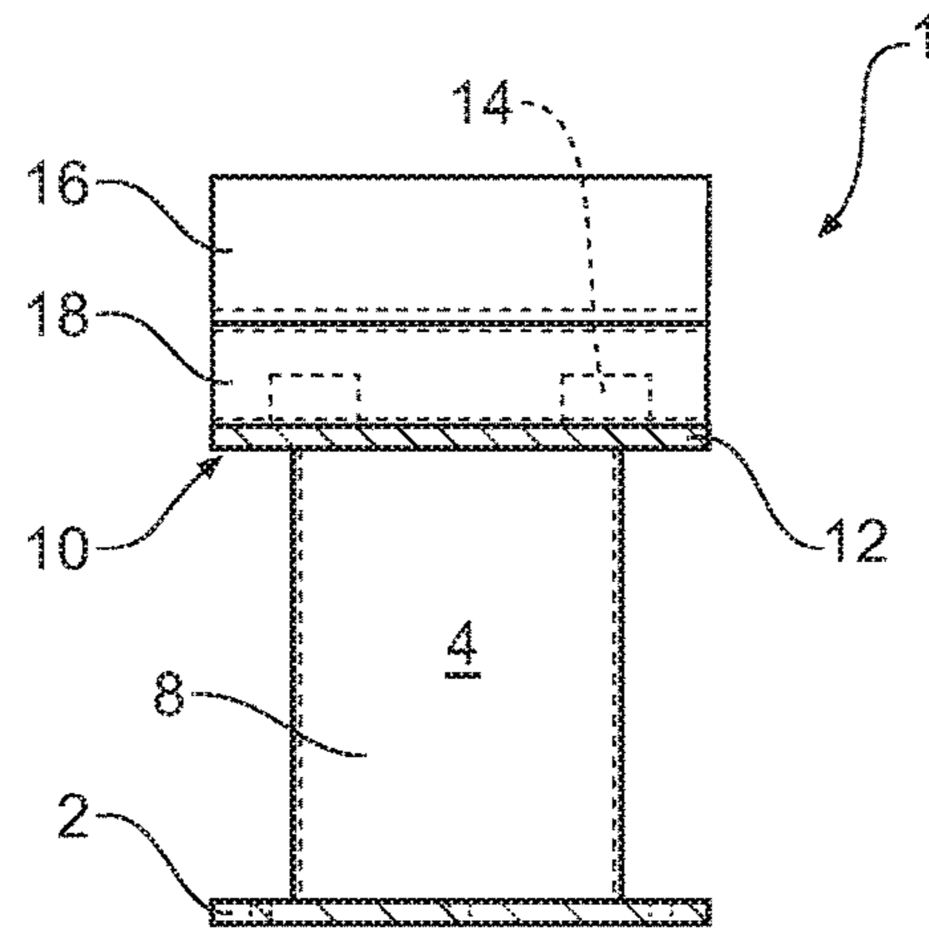
Figure 2 Section B-B
