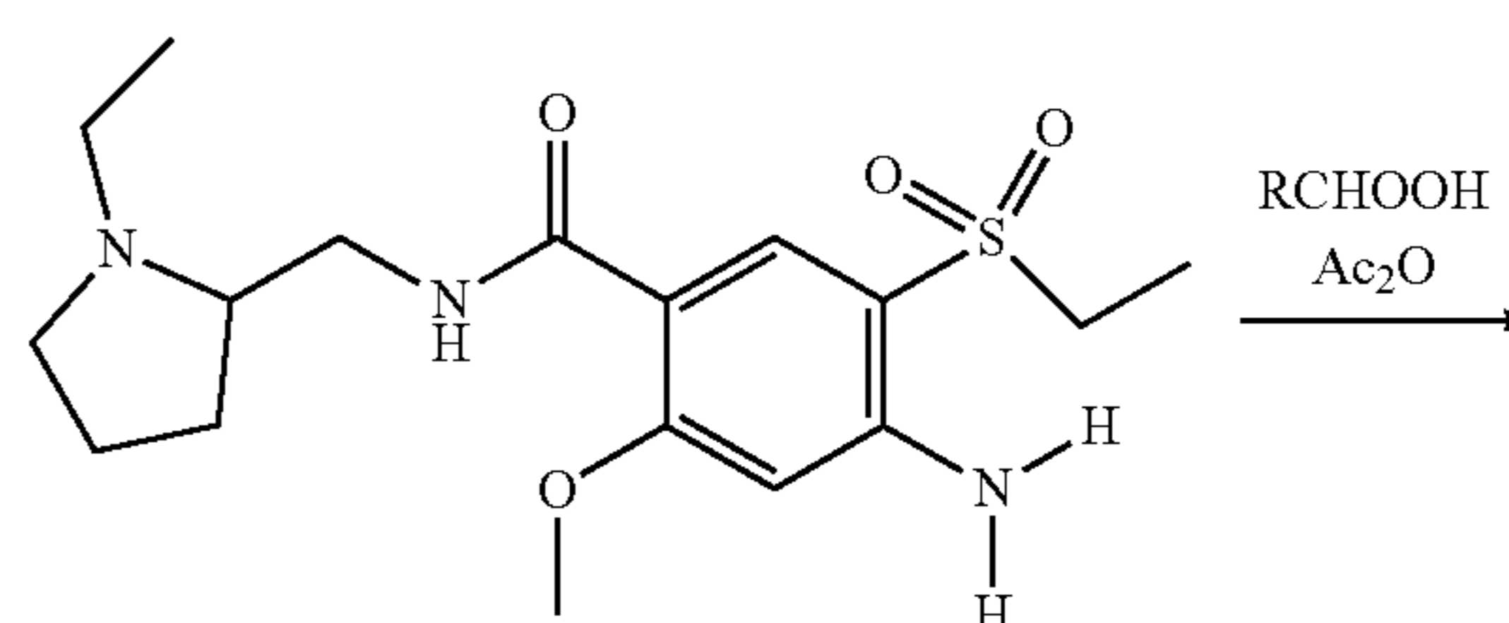
Scheme 1. Preparation of Amisulpride Derivatives
