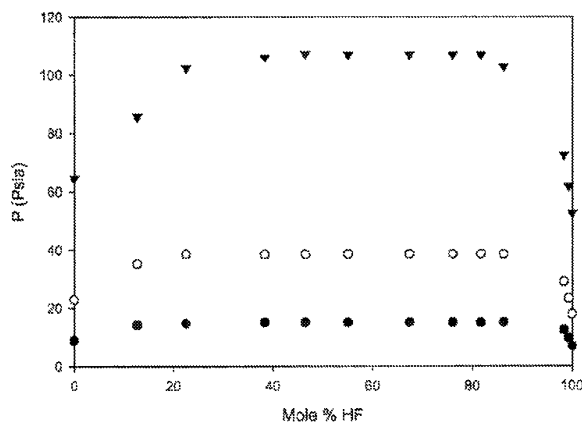
FIGURE 1: P-T-X of 1233xf/HF system
