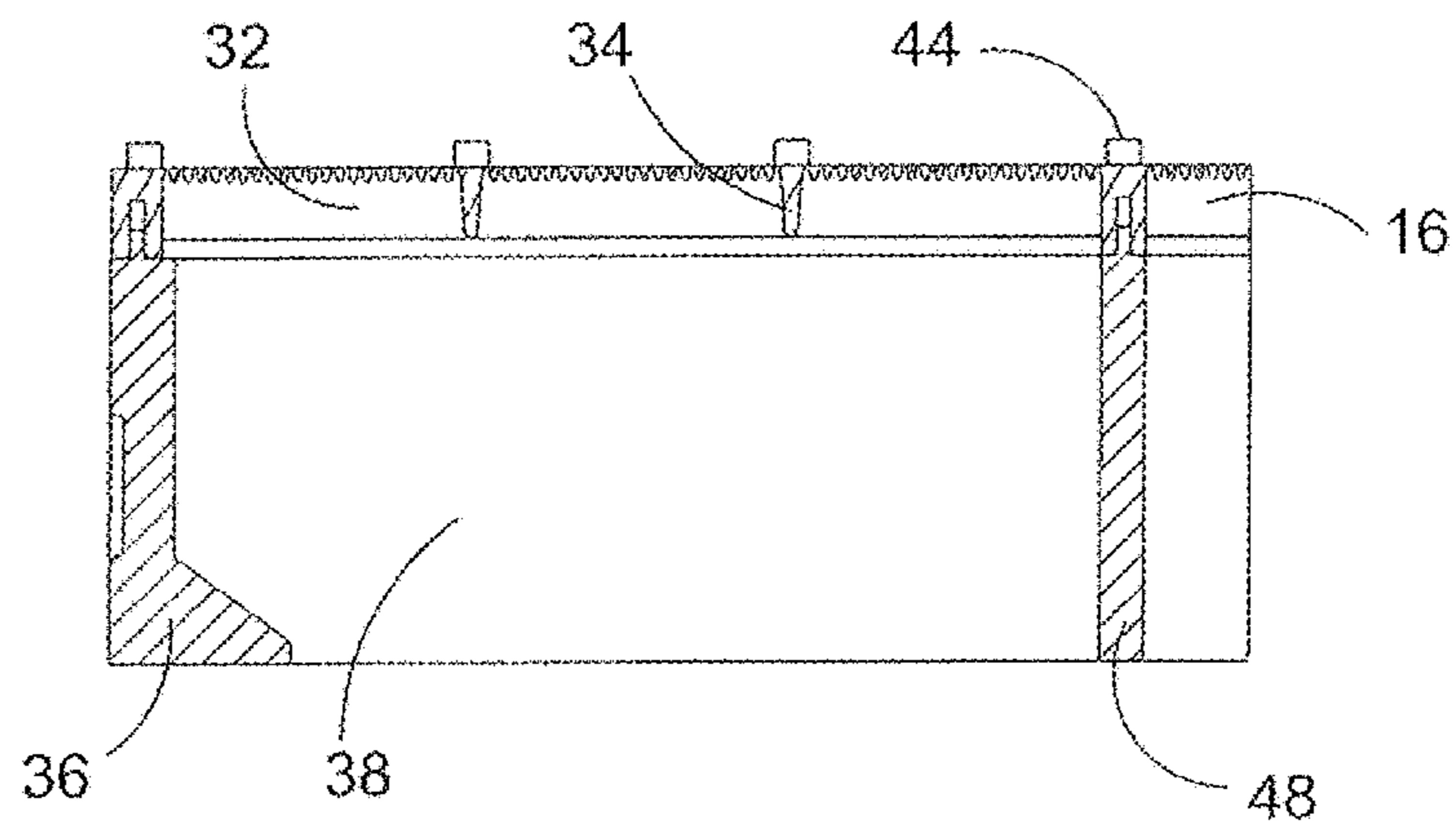
SECTION B-B
