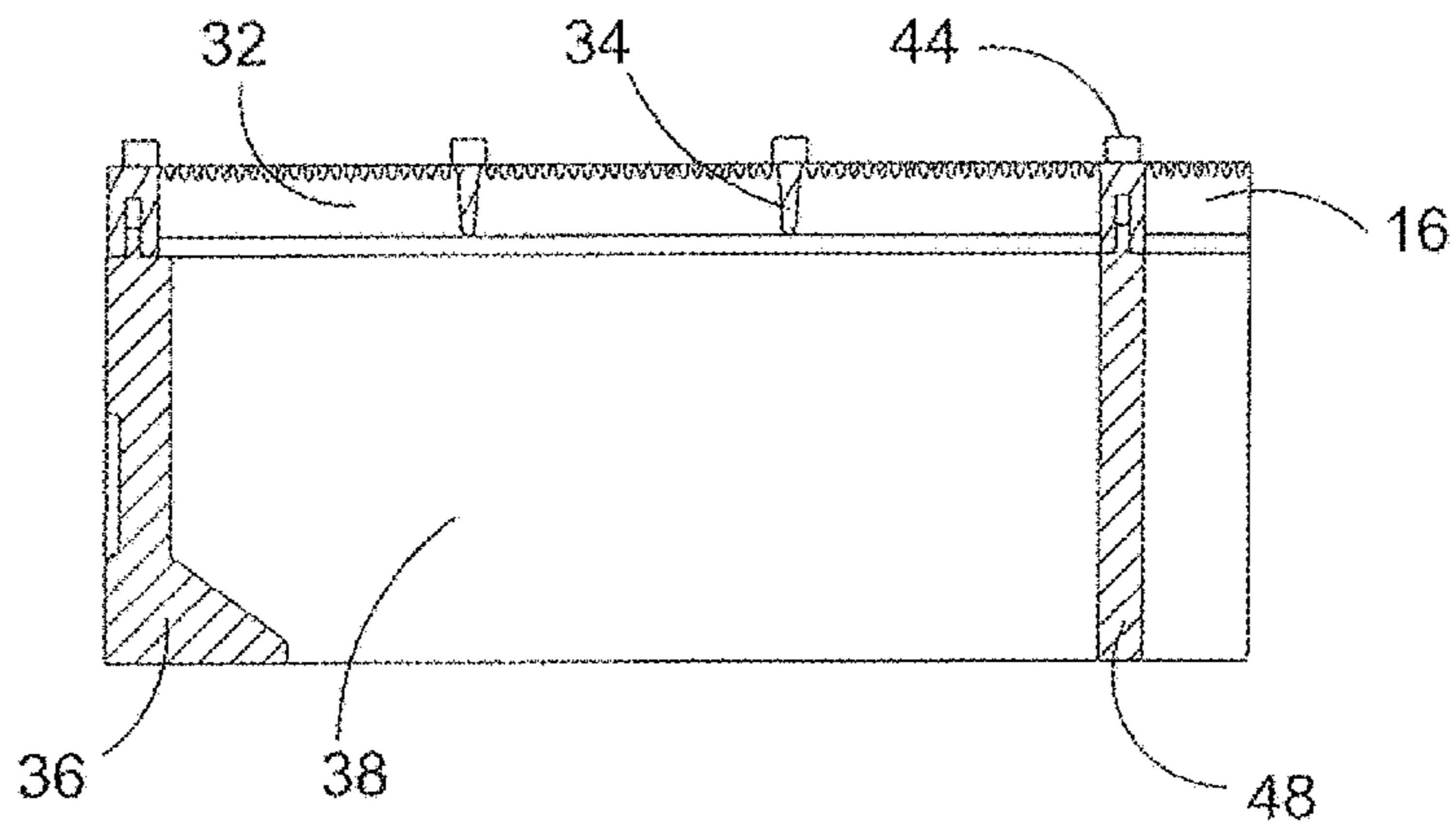
SECTION B-B
