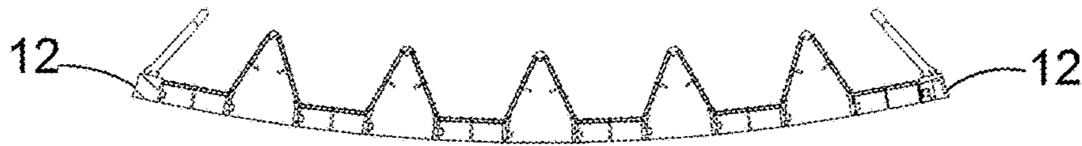
SECTION C-C FIG.25A
