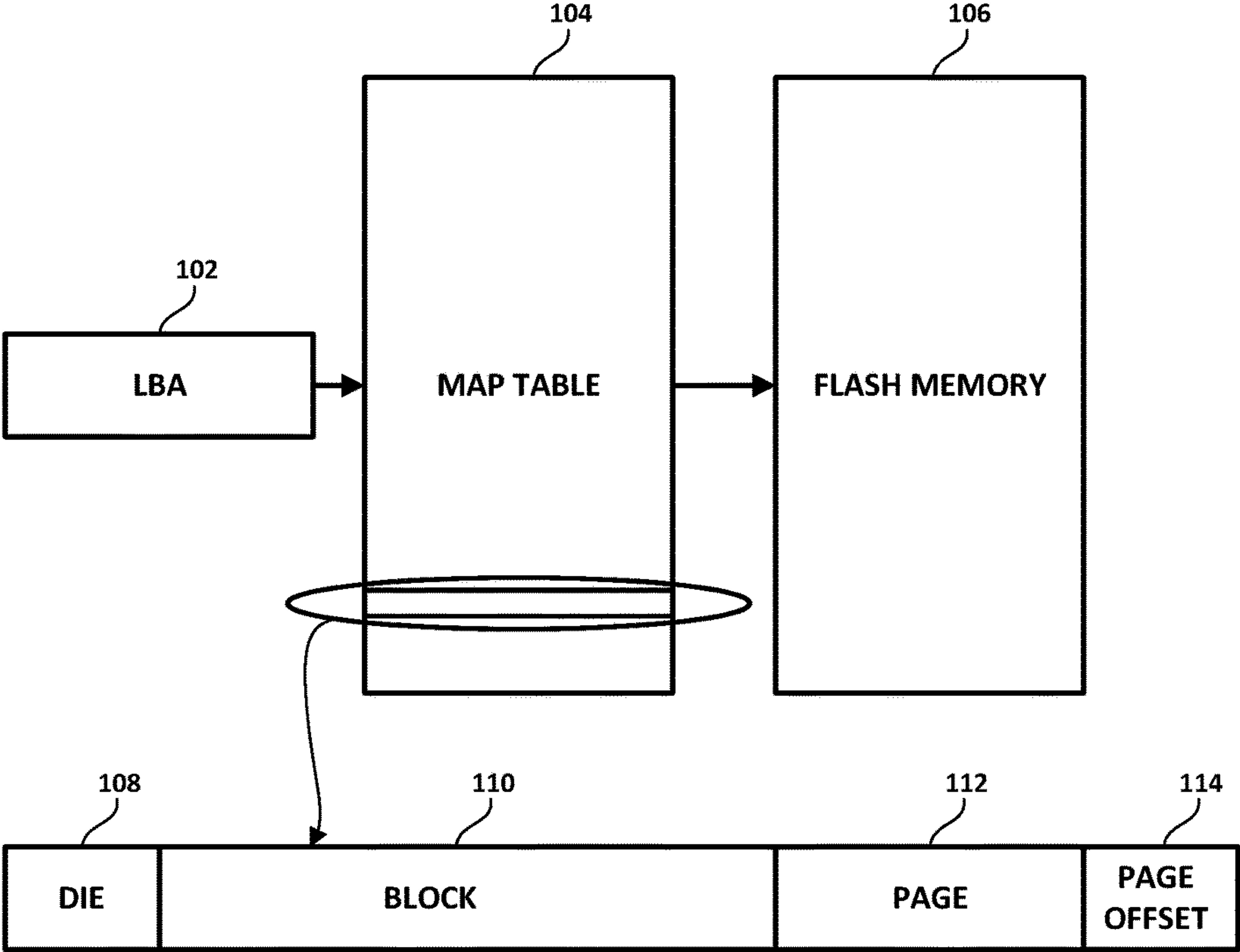
FIG. 1 (Prior Art)
