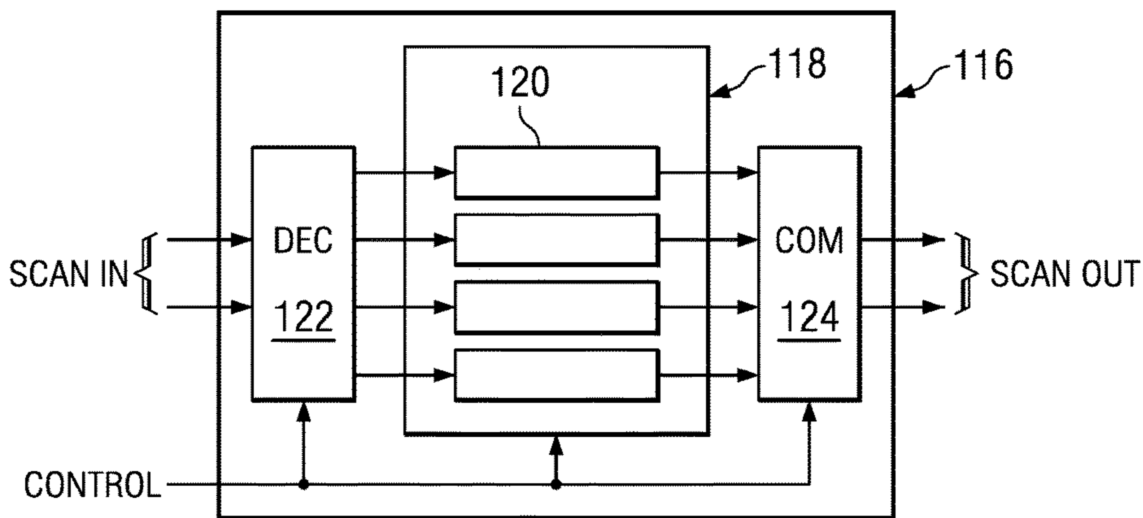
FIG. 1C (PRIOR ART)
