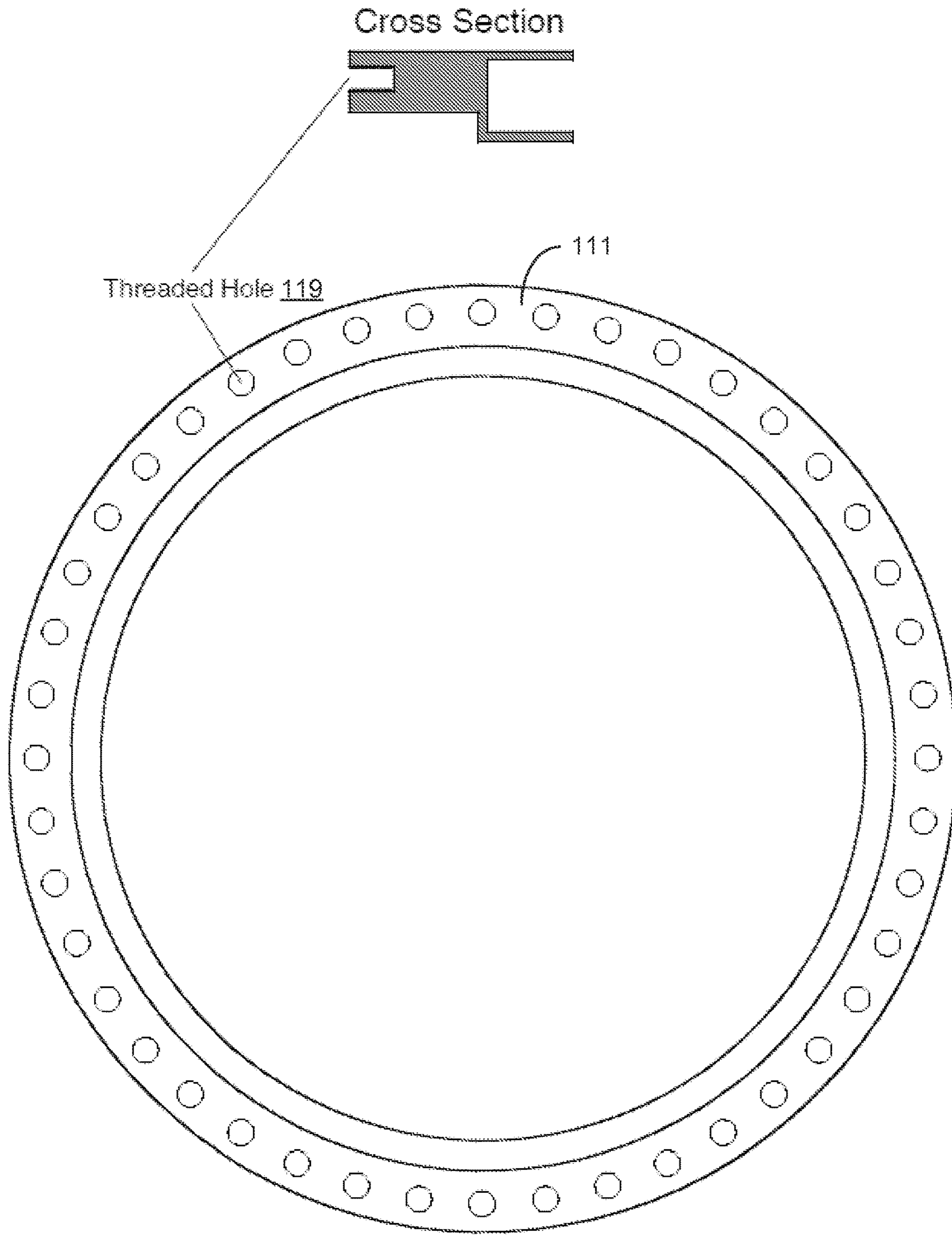
Front View
