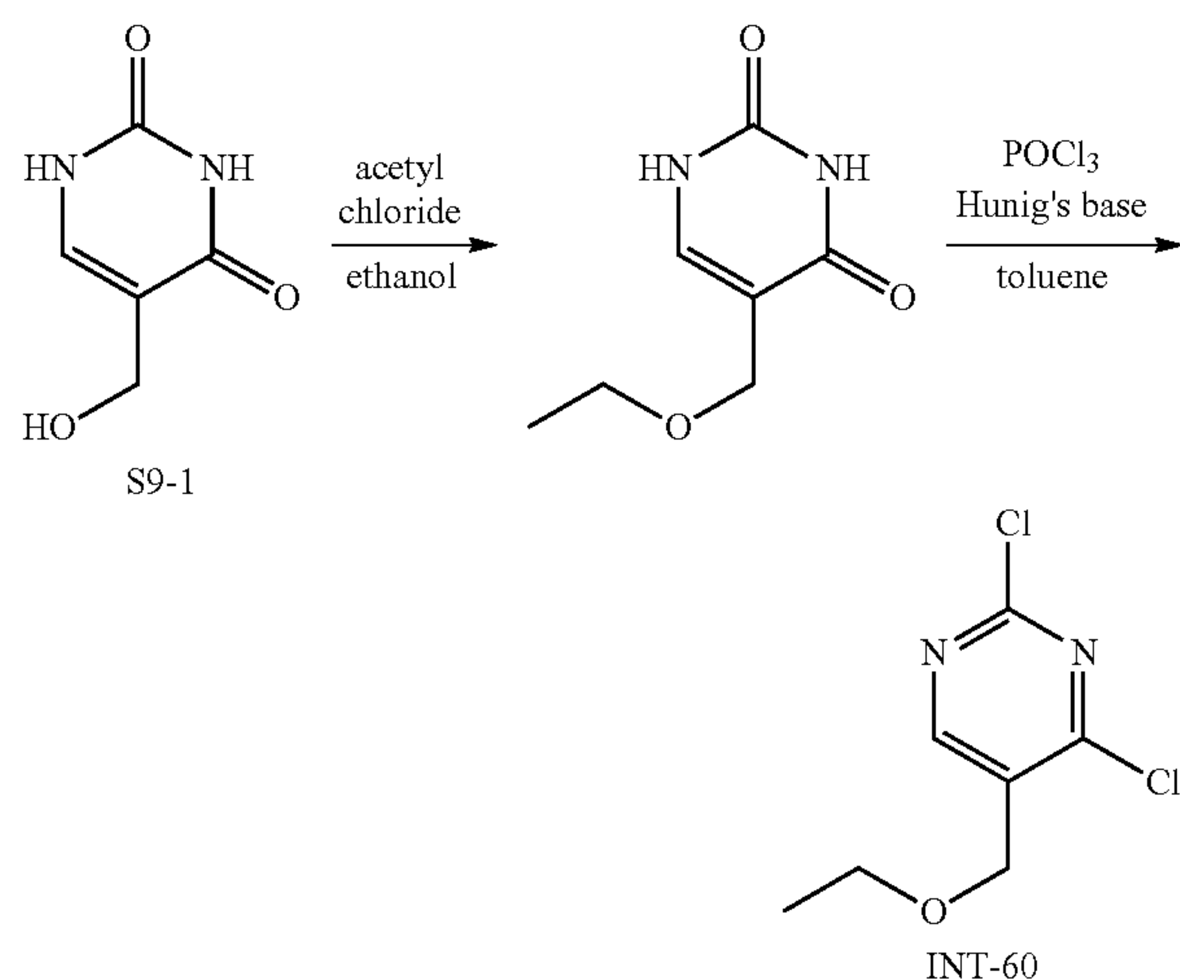
Alternative Synthesis of 2,4-Dichloro-5-(ethoxymethyl)pyrimidine (INT-60): Method B
