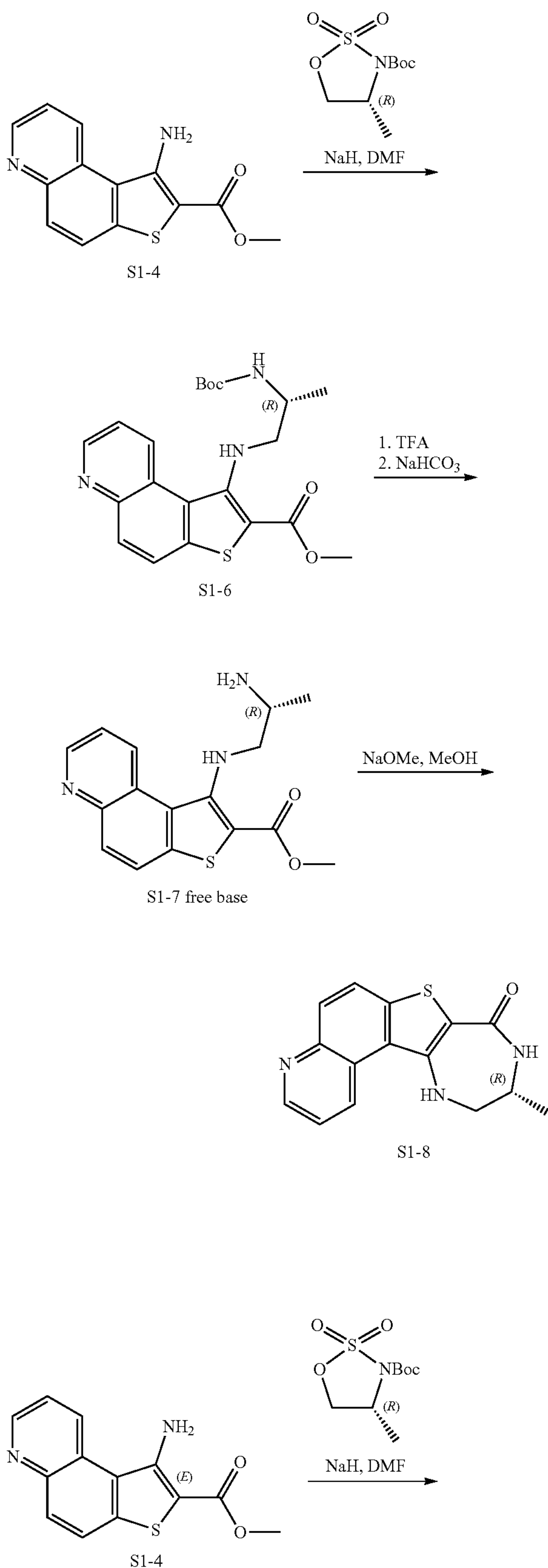
Scheme 1B: Alternative Synthesis of S1-8
