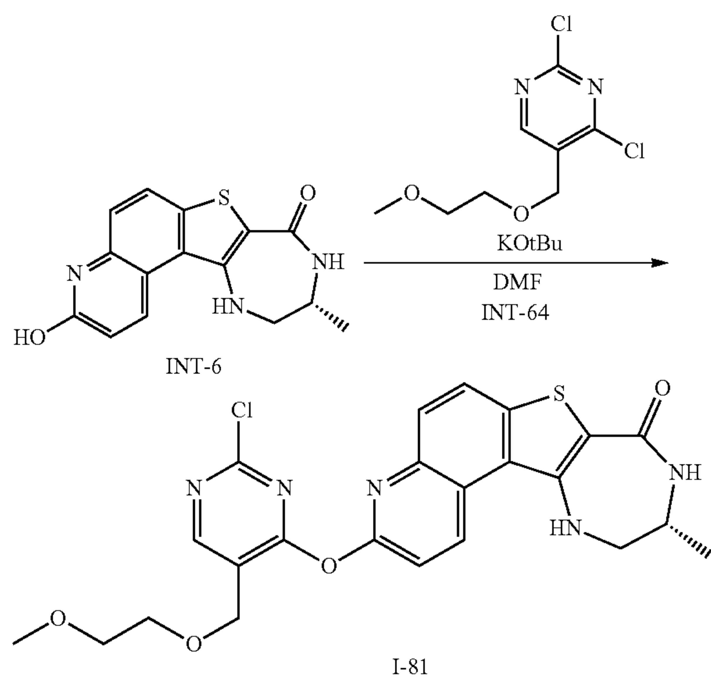
Synthesis of (R)-3-((2-chloro-5-((2-methoxyethoxy)methyl)pyrimidin-4-yl)oxy)-10-methyl-9,10,11,12-tetrahydro-8H-[1,4]diazepino[5',6':4,5]thieno[3,2-f]quinolin-8-one (81)
