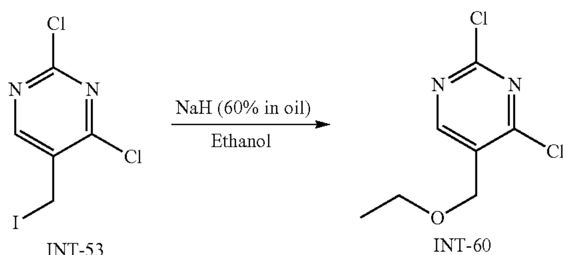
2,4-Dichloro-5-(ethoxymethyl)pyrimidine (INT-60): Method A
