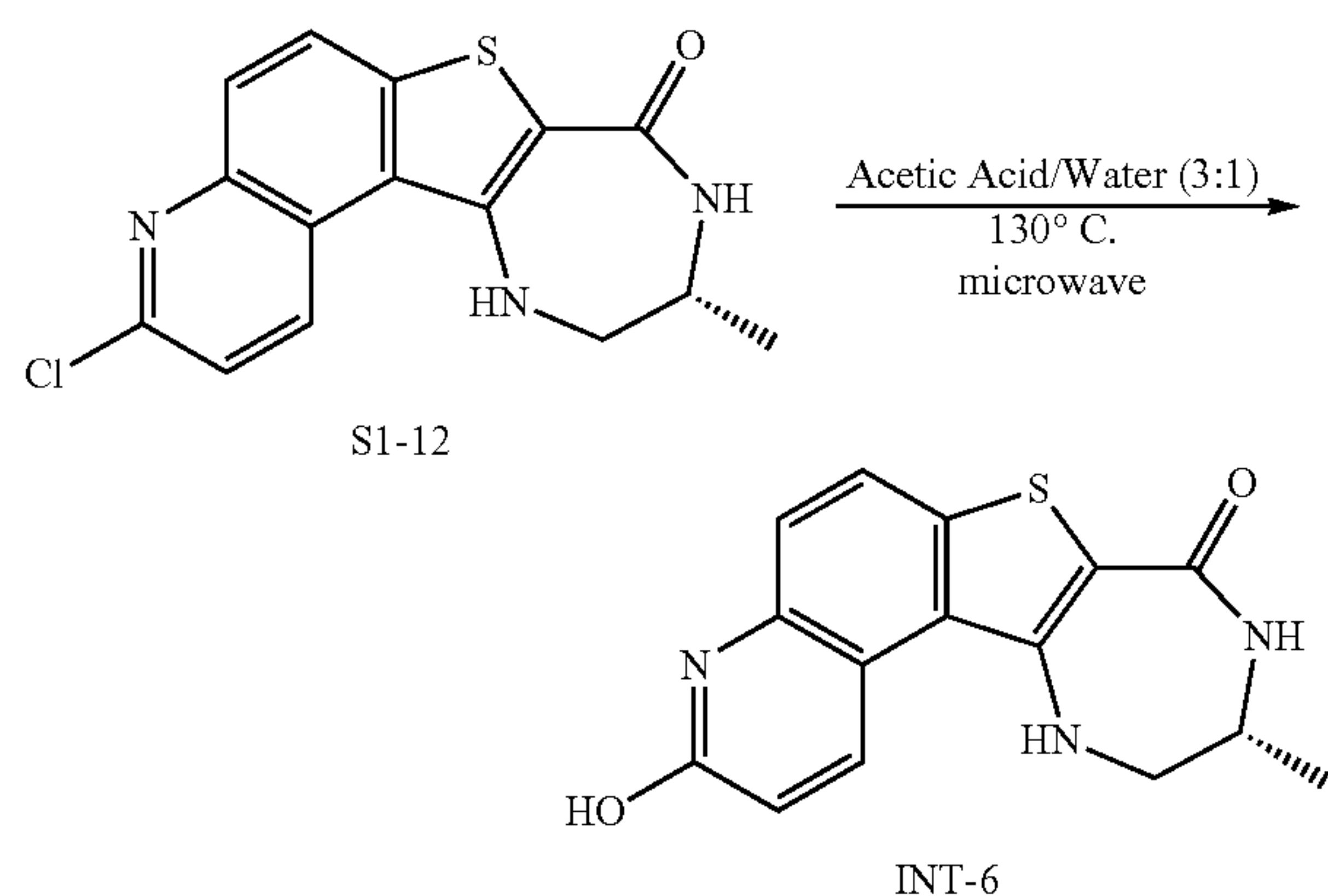
Synthesis of (R)-3-hydroxy-10-methyl-9,10,11,12-tetrahydro-SH-[1,4]diazepino-[5',6':4,5]thieno[3,2-f]quinolin-8-one (INT-6)
