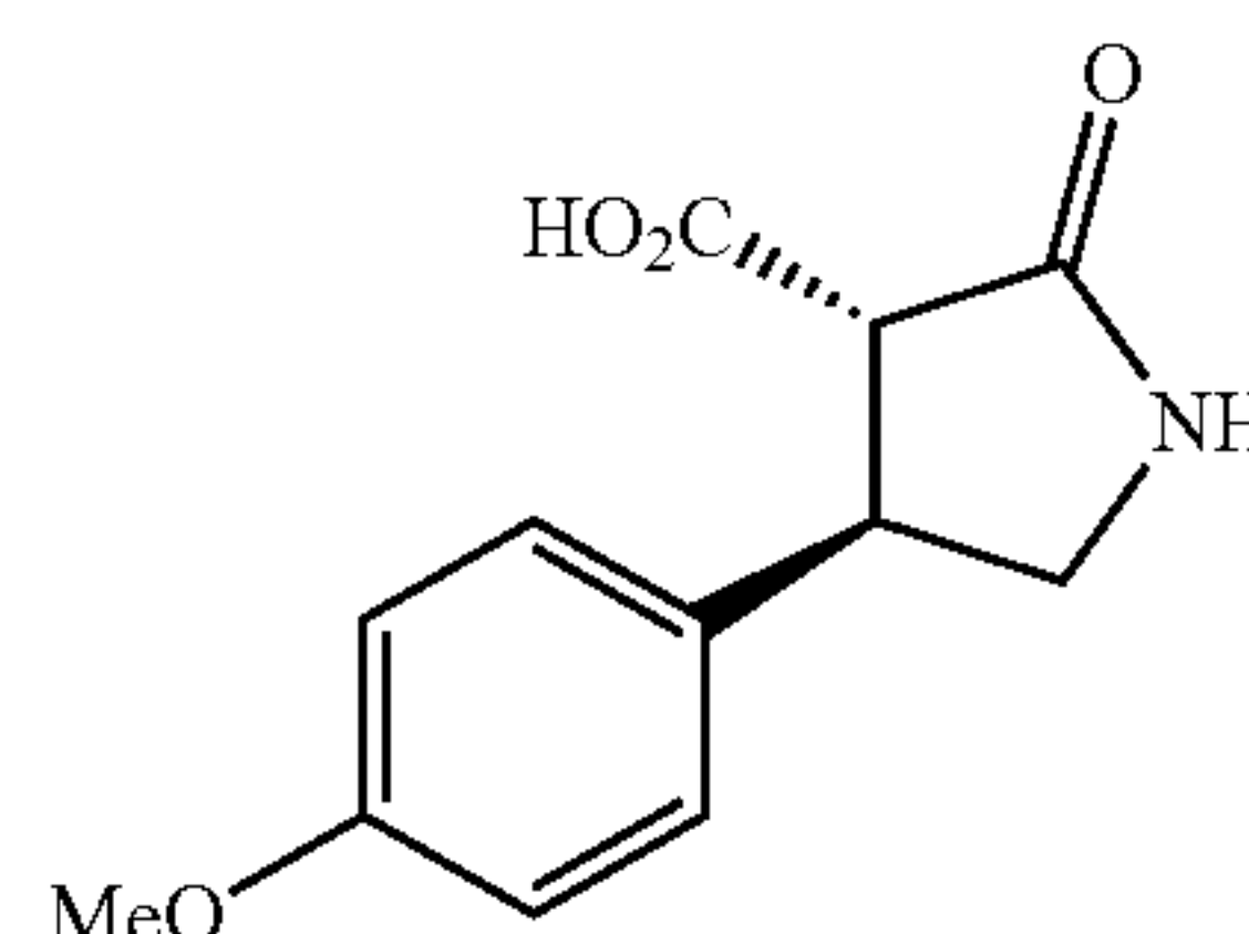
(-)-(3S*,4R*)-4-(4-Methoxyphenyl)-2-oxopyrrolidine-3-carboxylic acid
