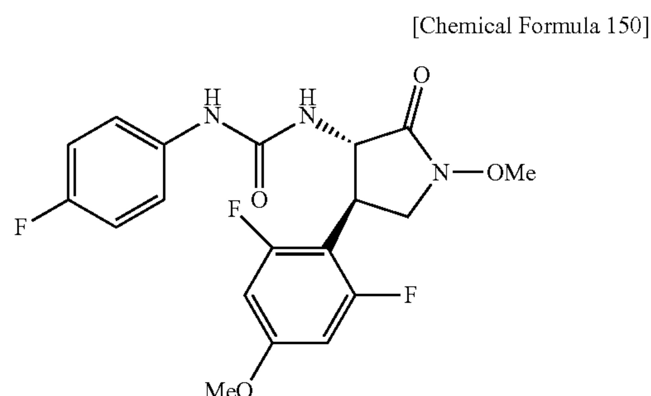
(-)-1-[(3S*,4R*)-4-(2,6-Difluoro-4-methoxyphenyl)-1-methoxy-2-oxopyrrolidin-3-yl]-3-(4-fluorophenyl)urea
