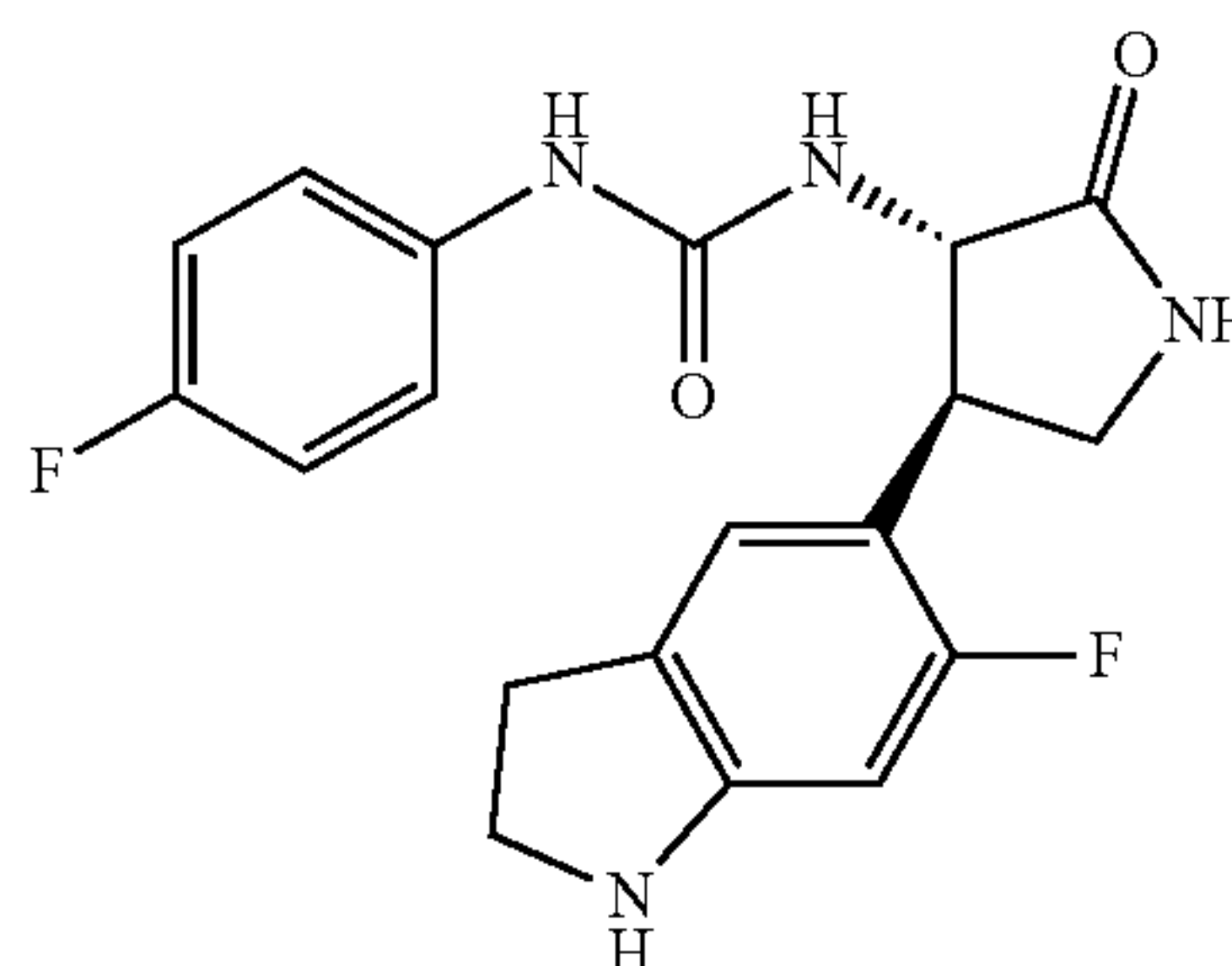
(−)-1-[(3S*,4R*)-4-(6-Fluoroindolin-5-yl)-2-oxopyrrolidin-3-yl]-3-(4-fluorophenyl)urea
