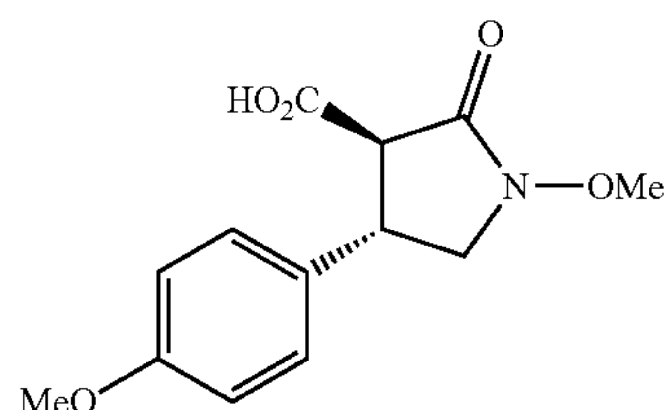
(3R*,4S*)-1-Methoxy-4-(4-methoxyphenyl)-2-oxopyrrolidine-3-carboxylic acid
