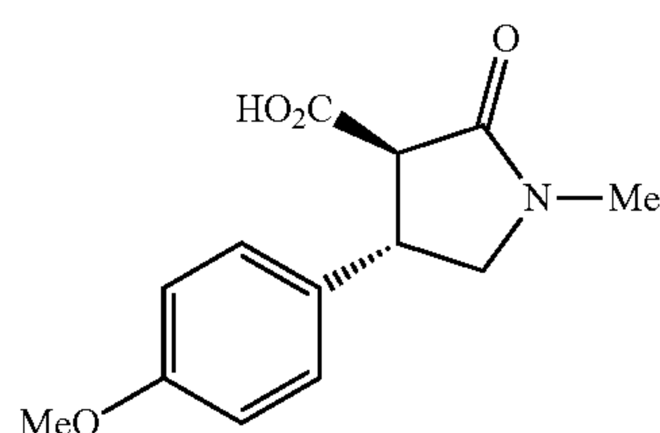
(3R*,4S*)-4-(4-Methoxyphenyl)-1-methyl-2-oxopyrrolidine-3-carboxylic acid
