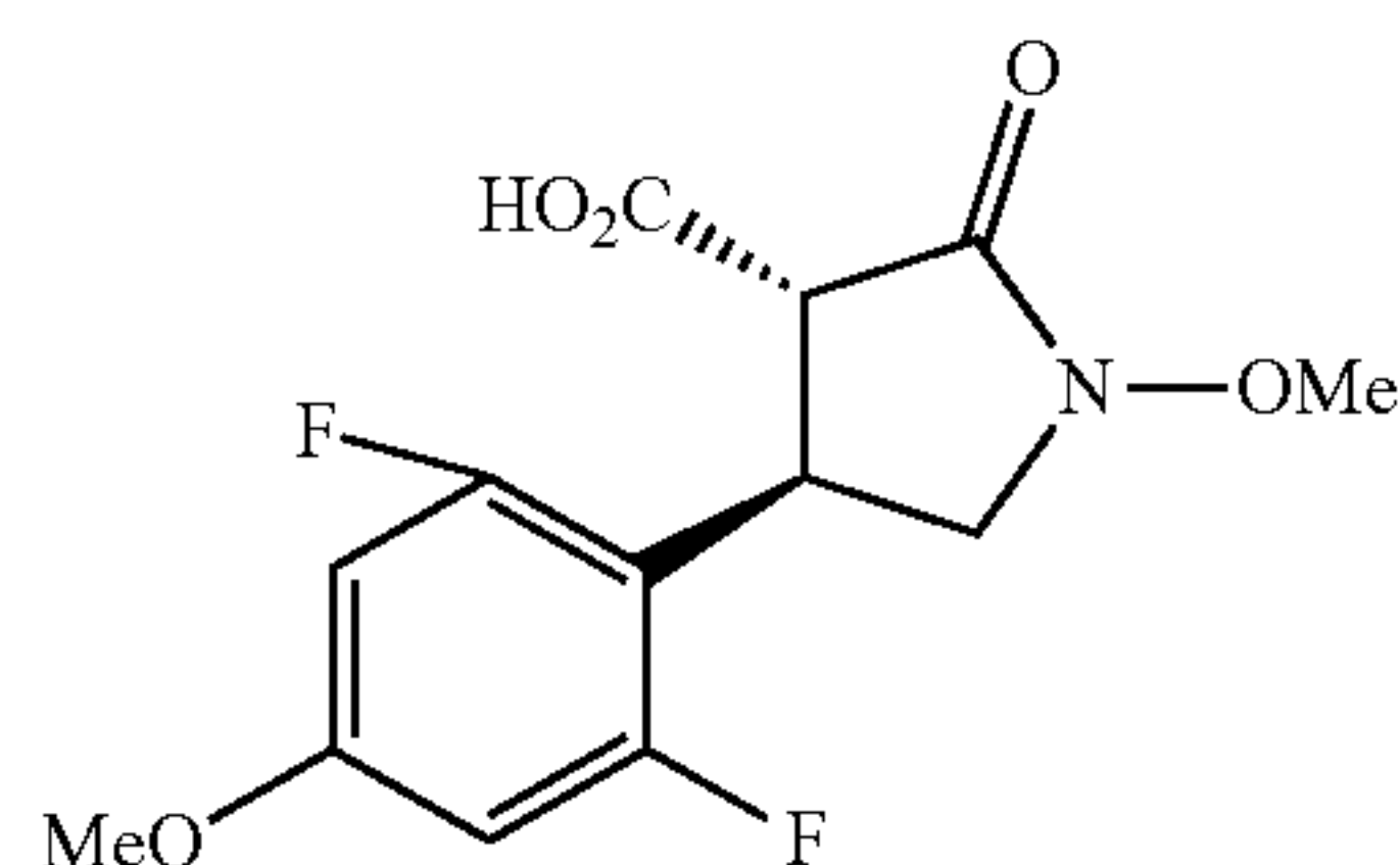
(3S*,4R*)-4-(2,6-Difluoro-4-methoxyphenyl)-1-methoxy-2-oxopyrrolidine-3-carboxylic acid
