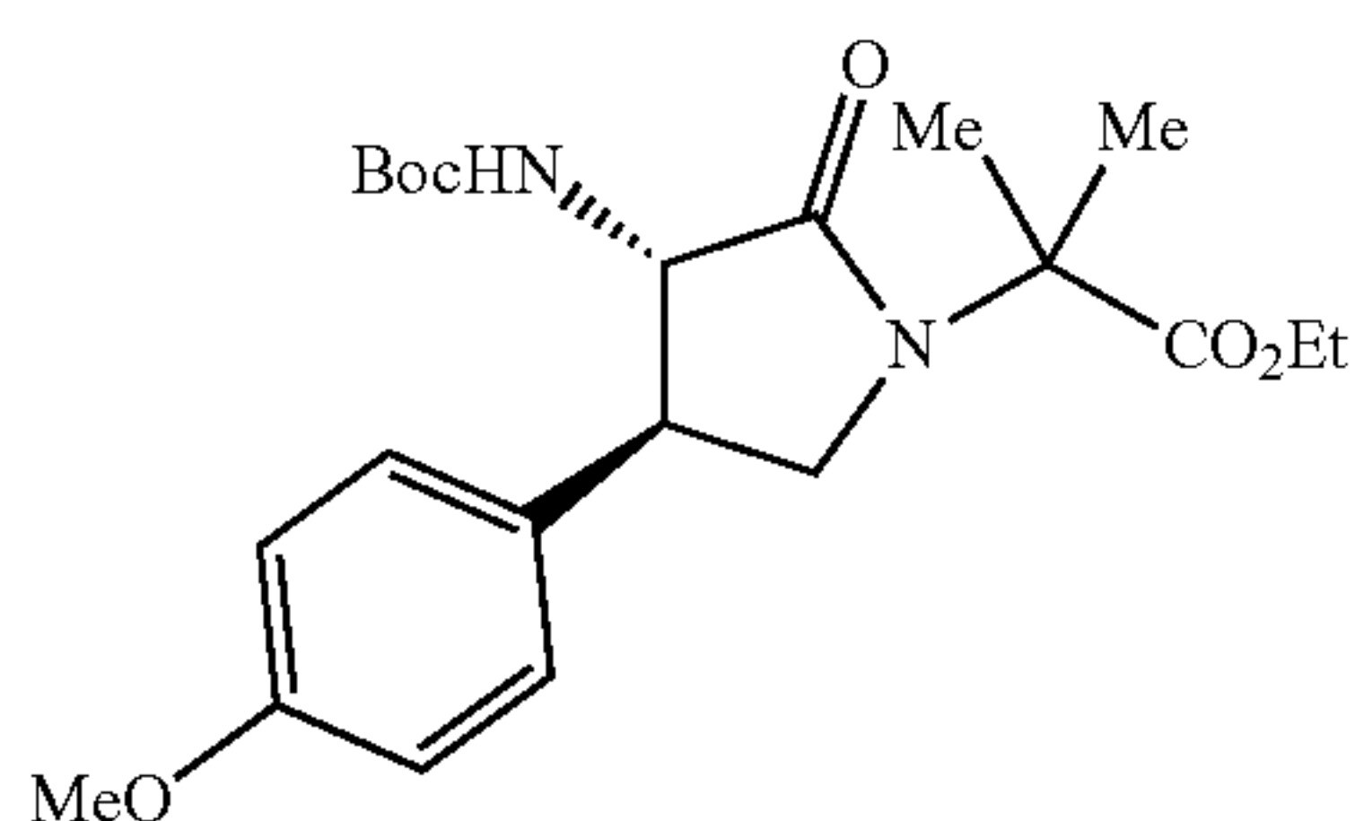
2-[(3S*,4R*)-3-[(tert-butoxycarbonyl)amino]-4-(4-methoxyphenyl)-2-oxopyrrolidin-1-yl]-2-methylpropanoic acid ethyl ester
