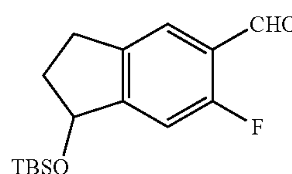
1-[(tert-Butyldimethylsilyl)oxy]-6-fluoro-2,3-dihydro-1H-indene-5-carbaldehyde
