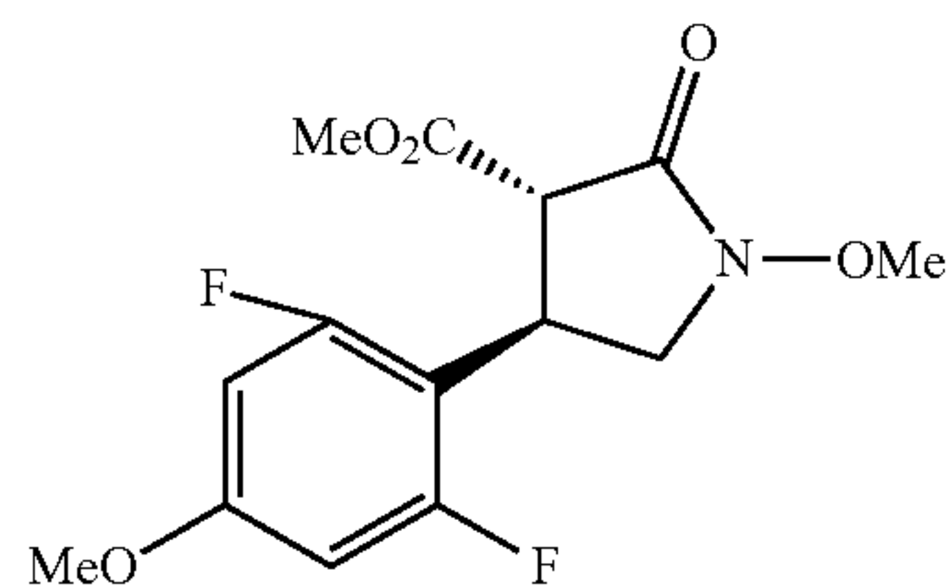
(3S*,4R*)-4-(2,6-Difluoro-4-methoxyphenyl)-1-methoxy-2-oxopyrrolidine-3-carboxylic acid methyl ester
