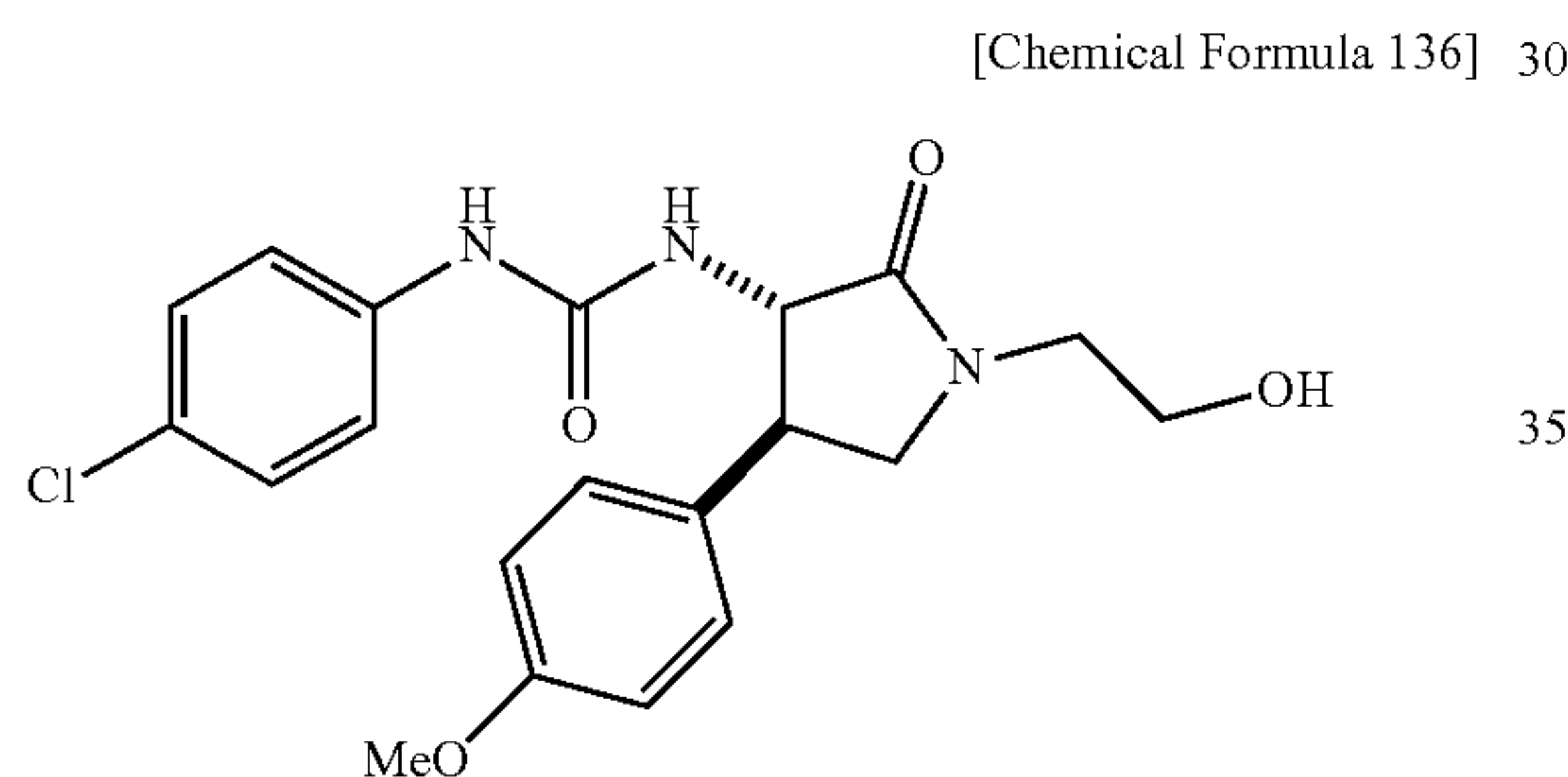
Isomer A (-)-trans
