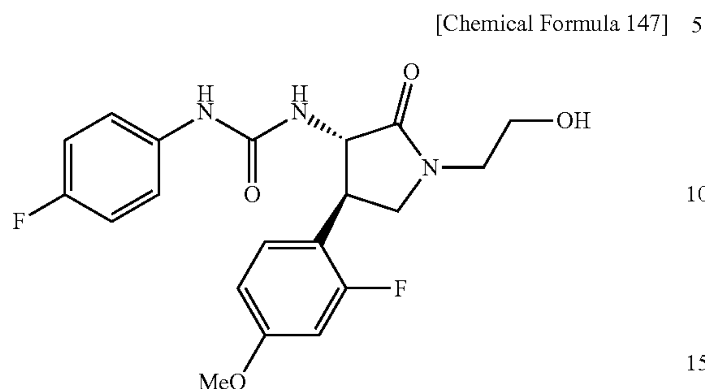
(-)-1-[(3S*,4R*)-4-(2-Fluoro-4-methoxyphenyl)-1-(2-hydroxyethyl)-2-oxopyrrolidin-3-yl]-3-(4-fluorophenyl)urea
