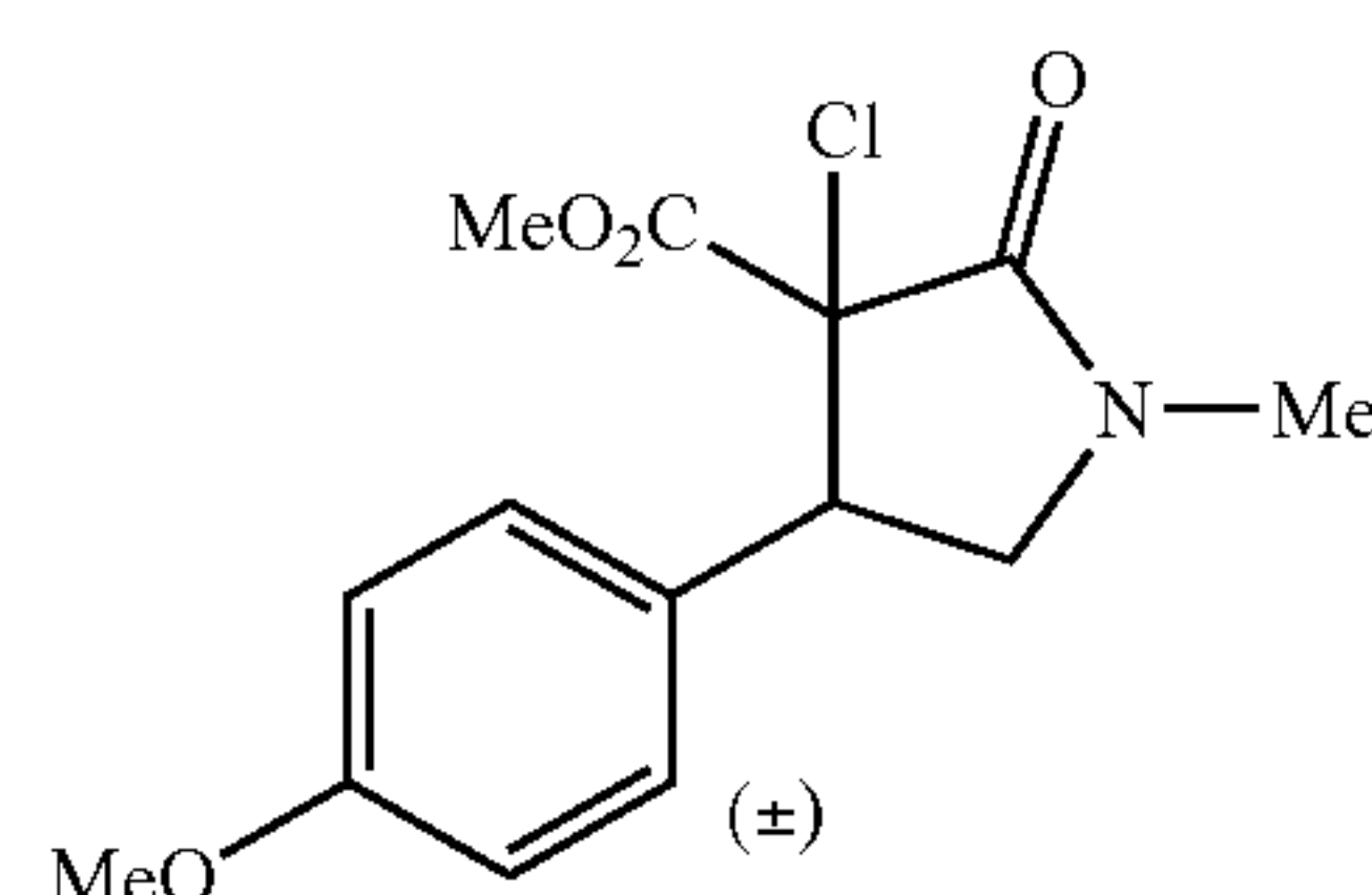
(±)-3-Chloro-4-(4-methoxyphenyl)-1-methyl-2-oxopyrrolidine-3-carboxylic acid methyl ester
