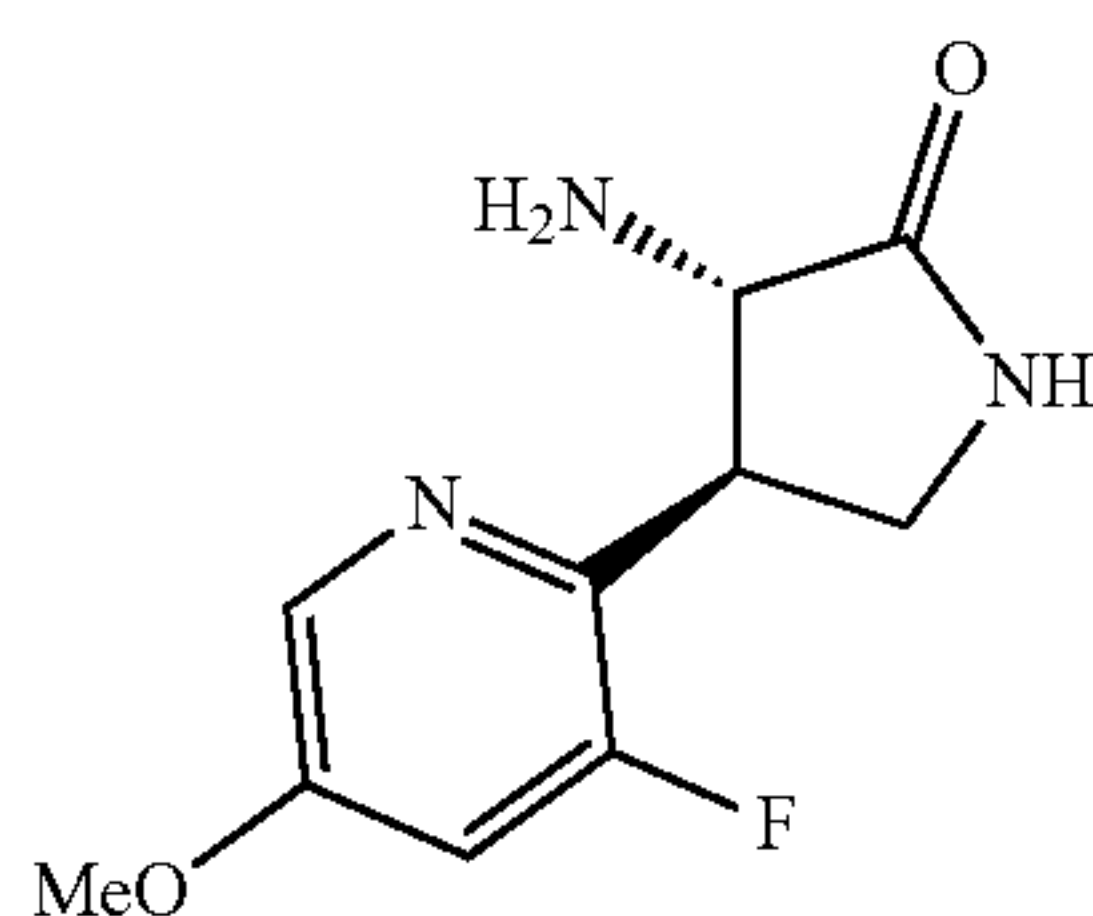
(3S*,4R*)-3-Amino-4-(3-fluoro-5-methoxypyridin-2-yl)pyrrolidin-2-one
