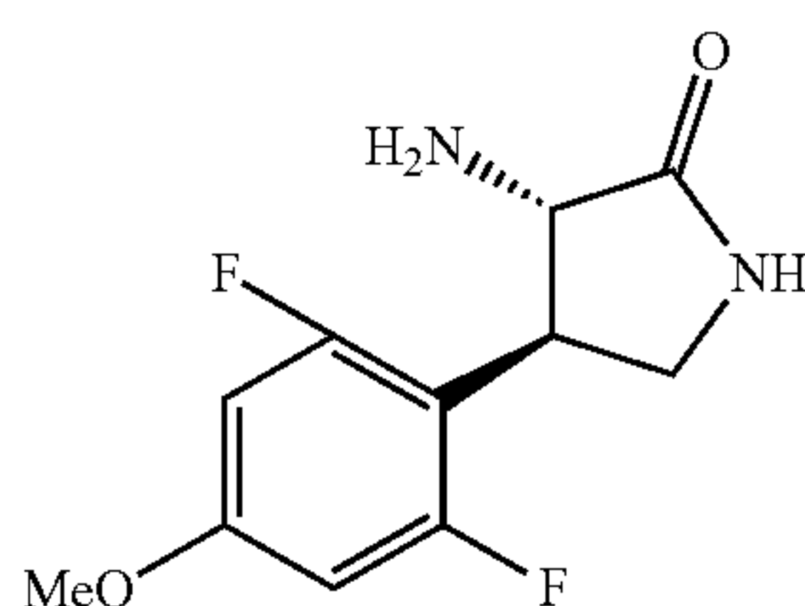
(-)-(3S*,4R*)-3-Amino-4-(2,6-difluoro-4-methoxyphenyl)pyrrolidin-2-one
