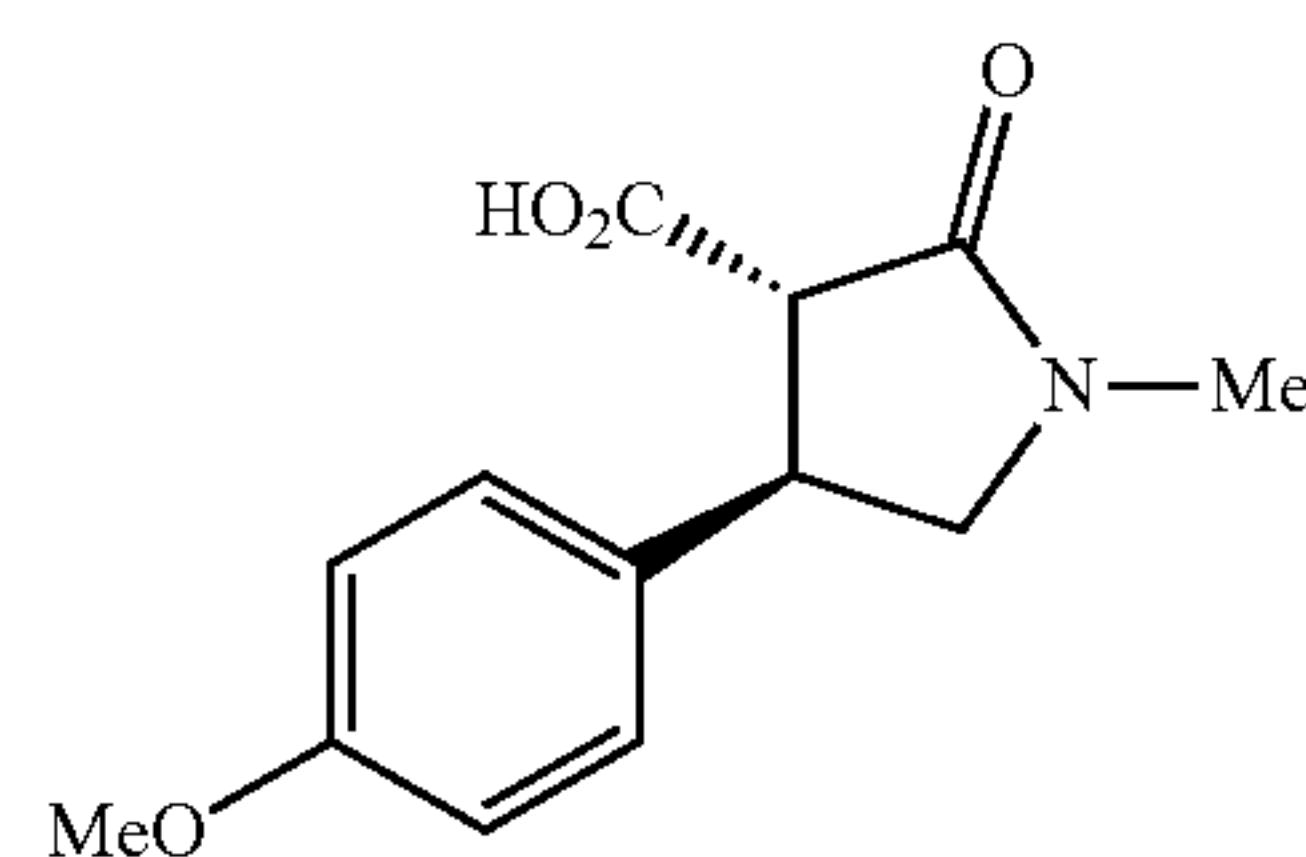
(3S*,4R*)-4-(4-Methoxyphenyl)-1-methyl-2-oxopyrrolidine-3-carboxylic acid
