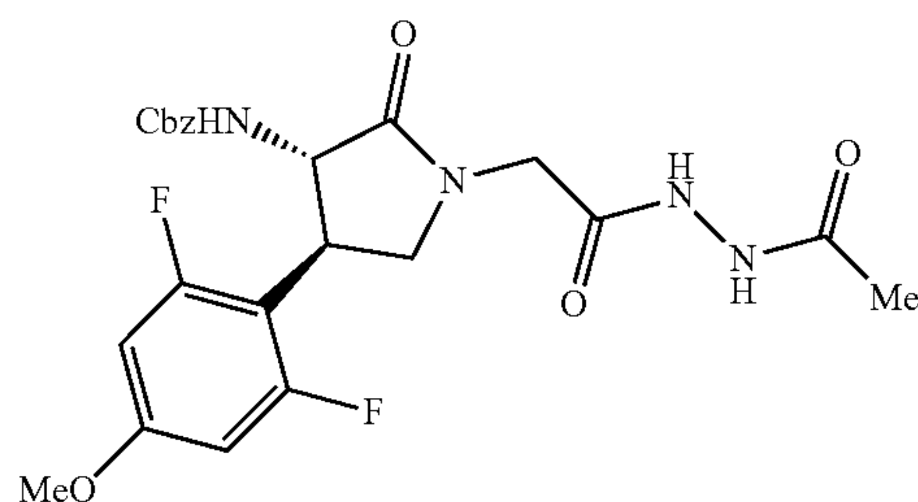
((3S*,4R*)-1-[2-(2-[(Acetylhydrazinyl)-2-oxoethyl]-4-(2,6-difluoro-4-methoxyphenyl)-2-oxopyrrolidin-3-yl)carbamic acid benzyl ester
