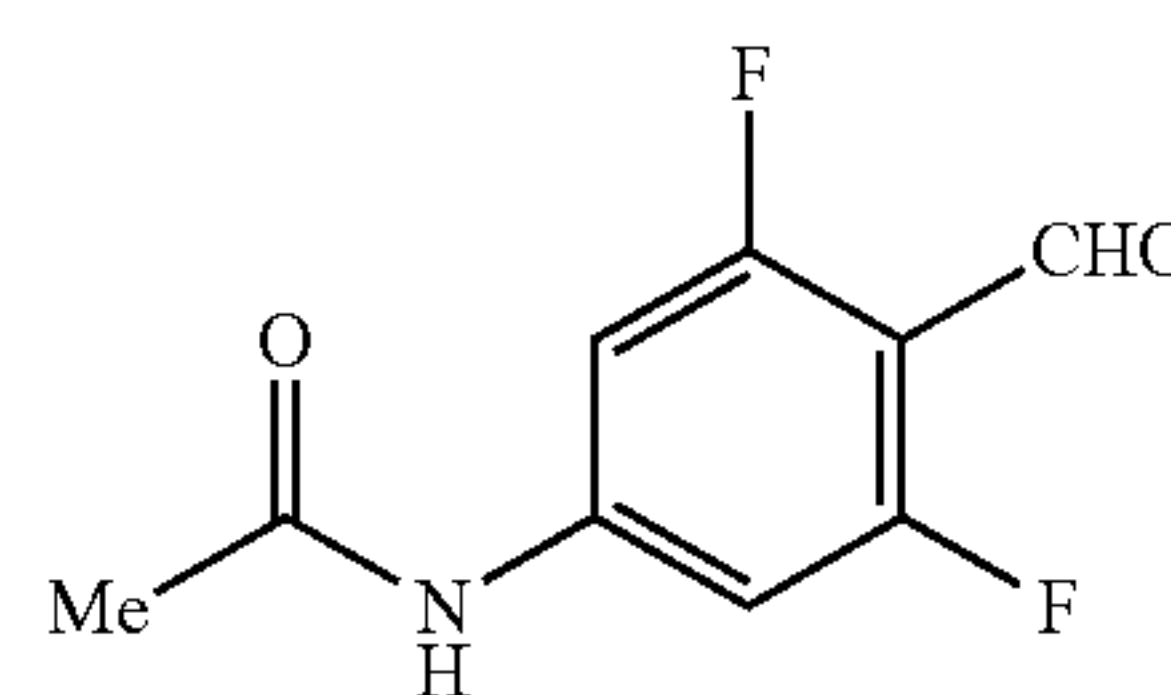
N-(3,5-Difluoro-4-formylphenyl) acetamide
