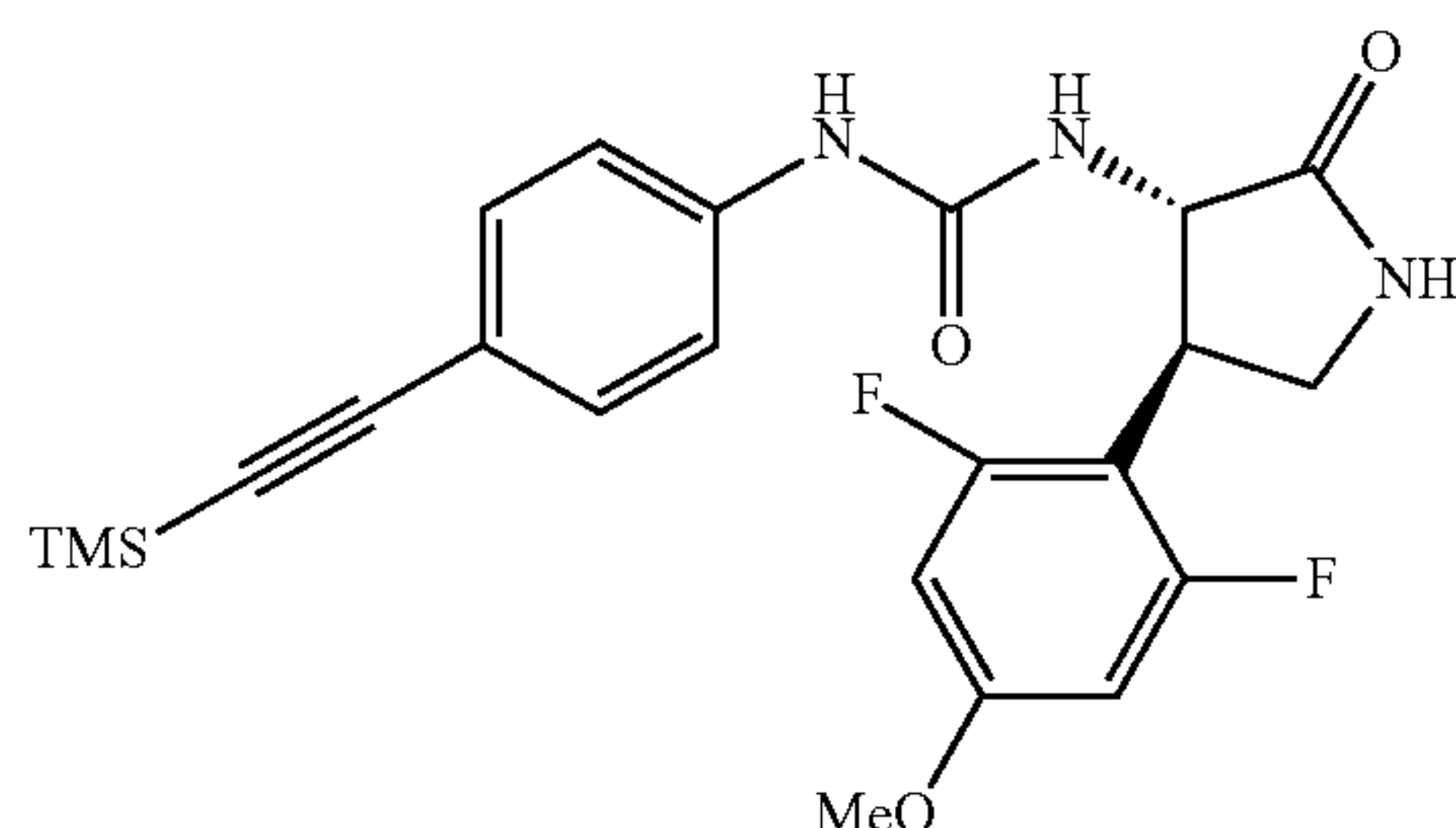
1-[(3S*,4R*)-4-(2,6-Difluoro-4-methoxyphenyl)-2-oxopyrrolidin-3-yl]-3-{4-[(trimethylsilyl)ethynyl]phenyl}urea
