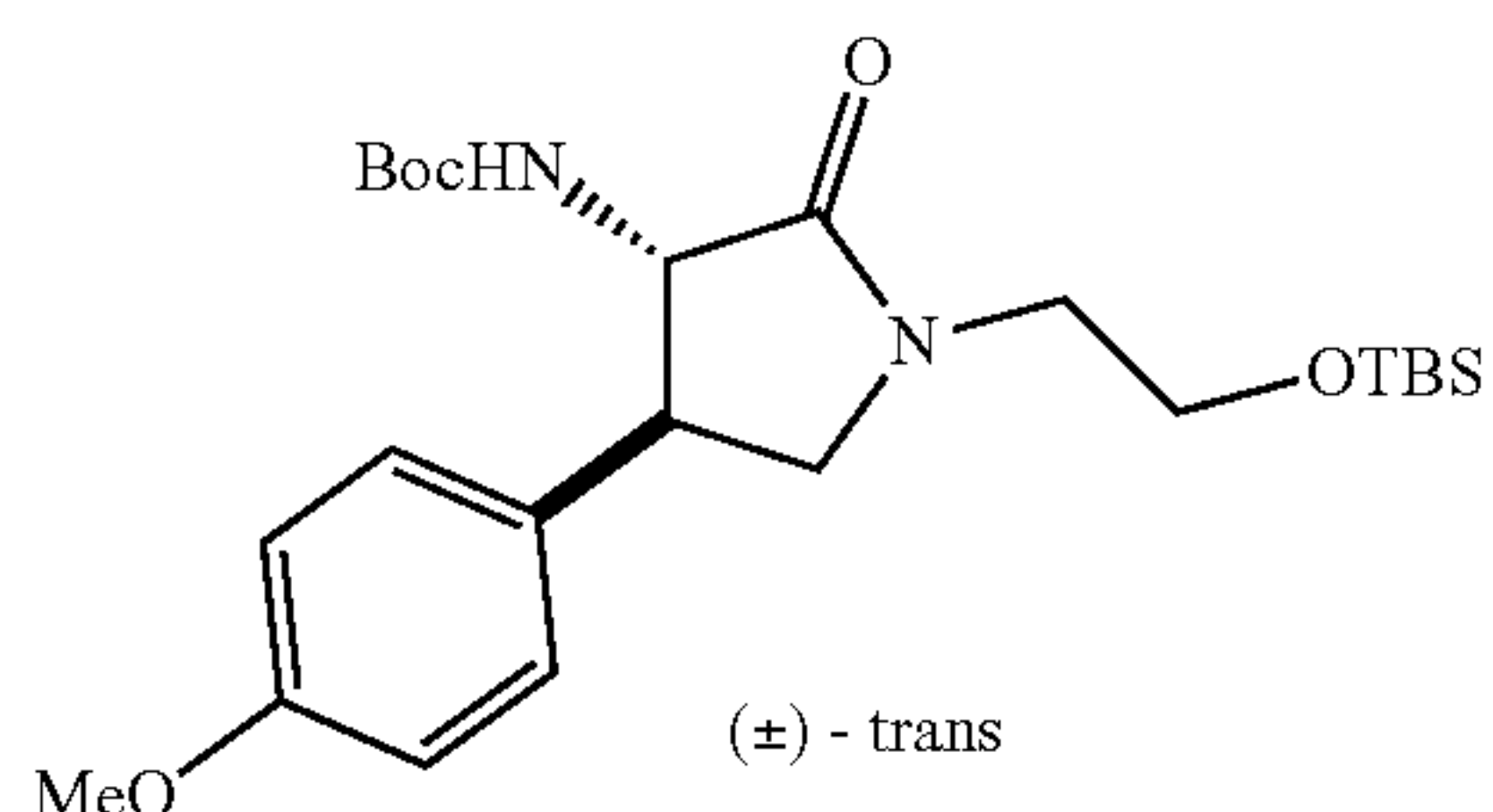
(±)-trans-({1-[2-[(tert-butyl)dimethylsilyl]oxy]ethyl}-4-(4-methoxyphenyl)-2-oxopyrrolidin-3-yl)carbamate
