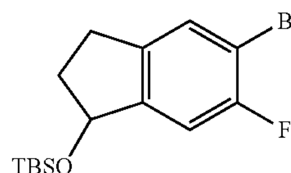
[(5-Bromo-6-fluoro-2,3-dihydro-1H-inden-1-yl)oxy] (tert-butyl)dimethylsilane
