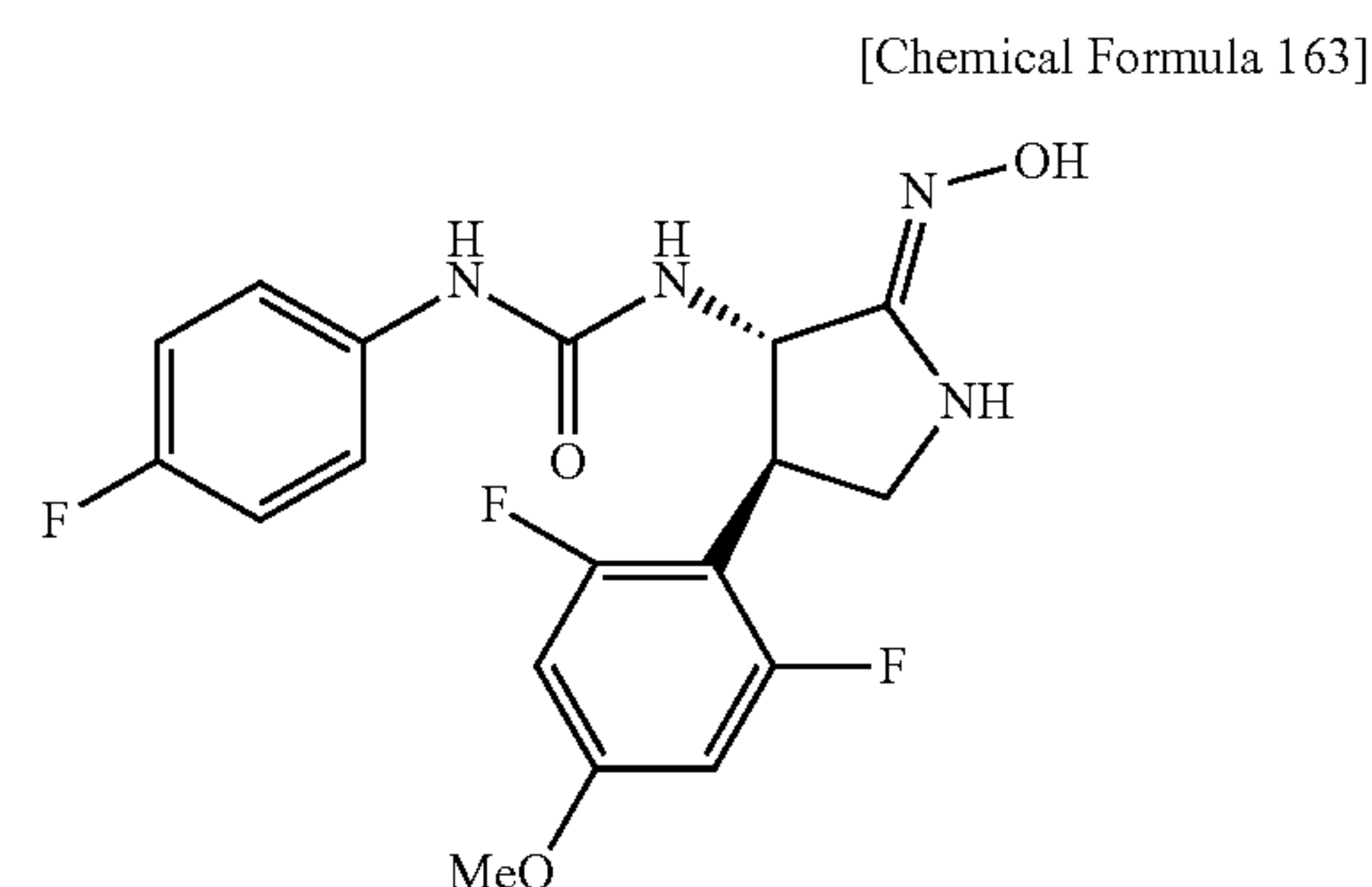
(-)-1-((3S*,4R*,Z)-2-(2,6-Difluoro-4-methoxyphenyl)-4-(hydroxyimino)pyrrolidin-3-yl)-3-(4-fluorophenyl)urea
