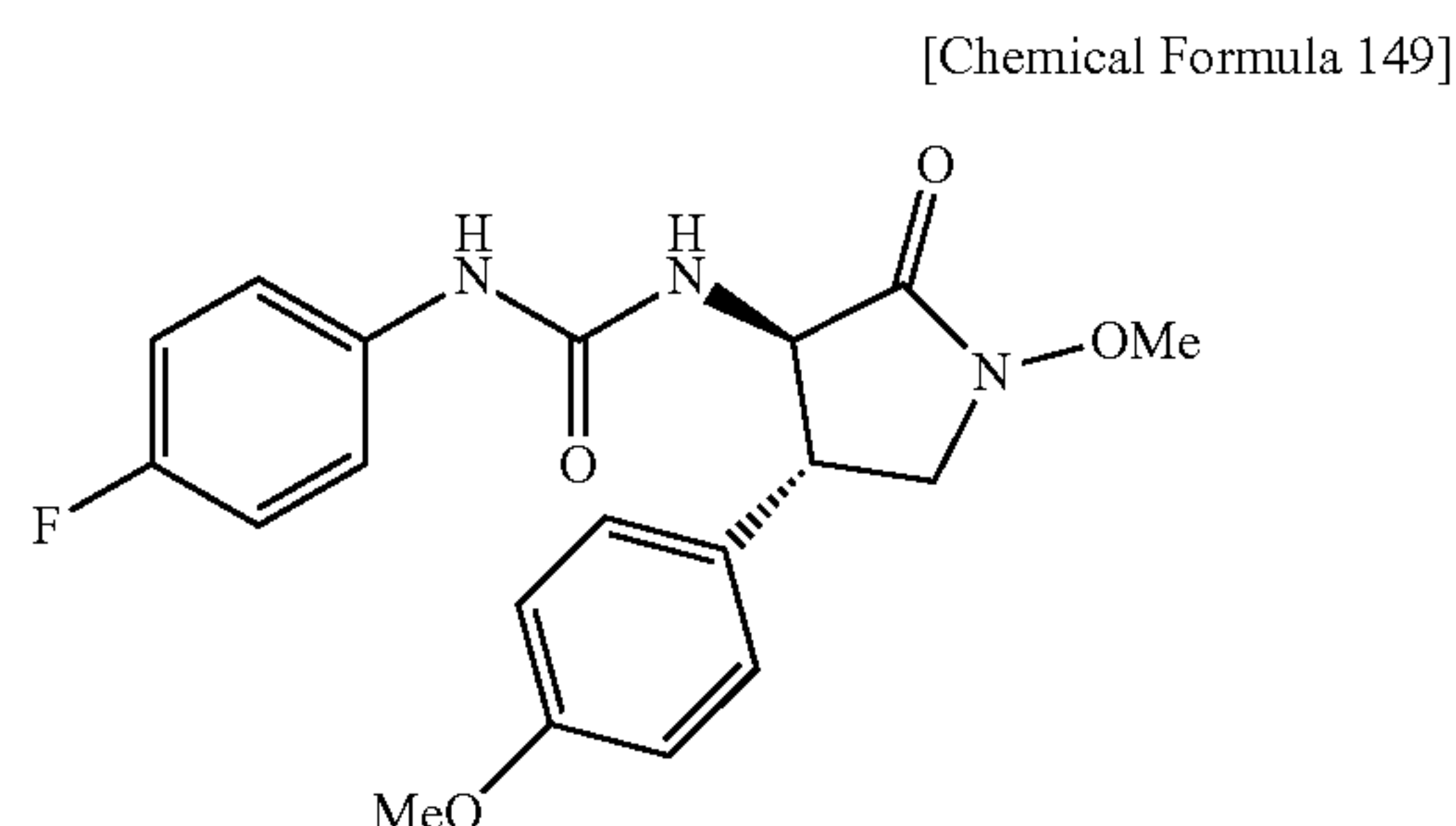
(+)-1-(4-Fluorophenyl)-3-[(3R*,4S*)-1-methoxy-4-(4-methoxyphenyl)-2-oxopyrrolidin-3-yl]urea
