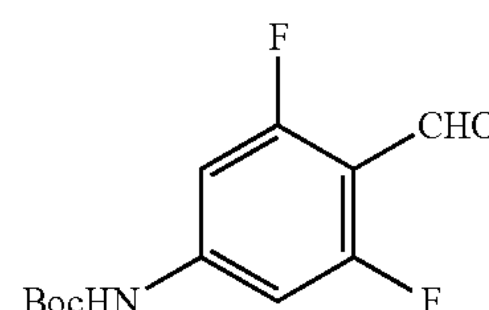
(3,5-Difluoro-4-formylphenyl)carbamic acid tert-butyl ester
