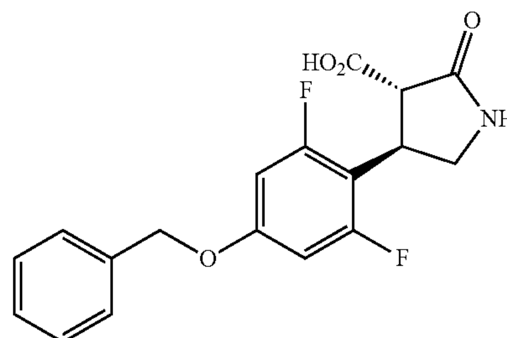
(3S*,4R*)-4-[4-(Benzyloxy)-2,6-difluorophenyl]-2-oxopyrrolidine-3-carboxylic acid
