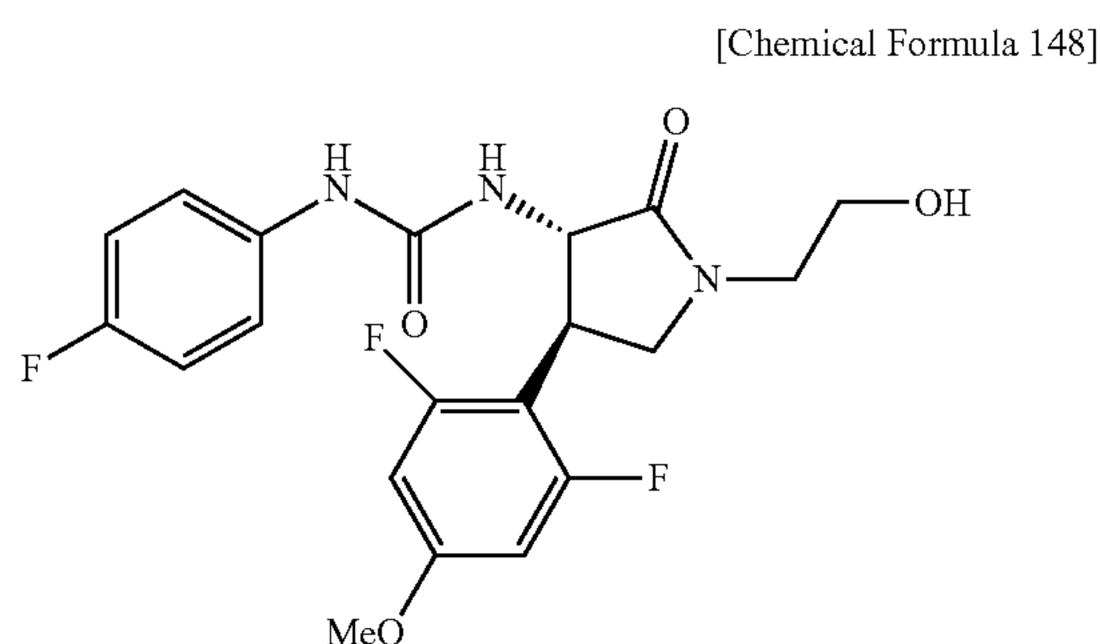
(-)-1-[(3S*,4R*)-4-(2,6-Difluoro-4-methoxyphenyl)-1-(2-hydroxyethyl)-2-oxopyrrolidin-3-yl]-3-(4-fluorophenyl)urea
