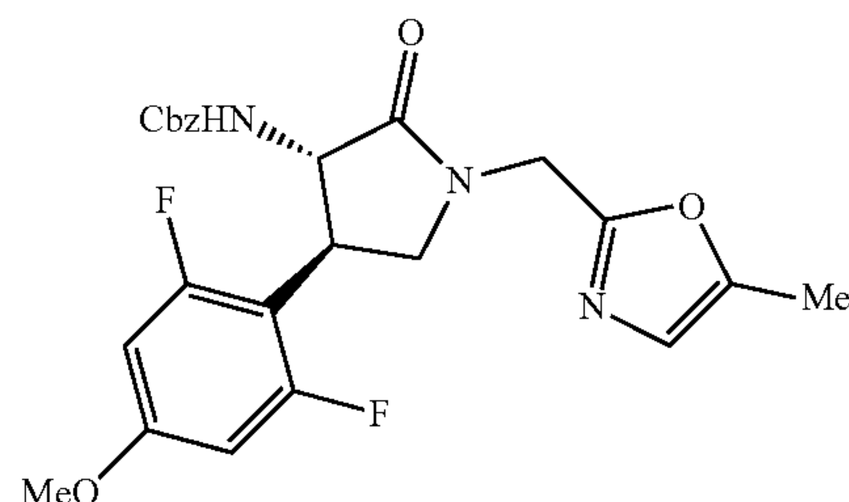
{(3S*,4R*)-4-(2,6-Difluoro-4-methoxyphenyl)-1-[(5-methyloxazol-2-yl)methyl]-2-oxopyrrolidin-3-yl}carbamic acid benzyl ester
