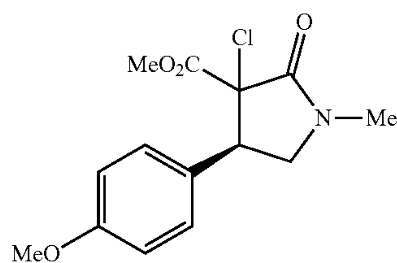
(4R*)-3-Chloro-4-(4-methoxyphenyl)-1-methyl-2-oxopyrrolidine-3-carboxylic acid methyl ester
