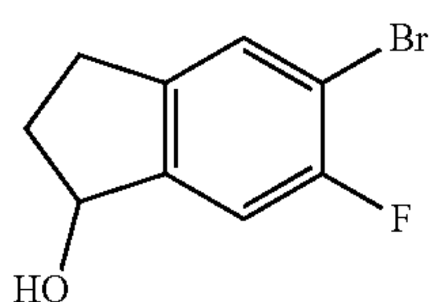
5-Bromo-6-fluoro-2,3-dihydro-1H-inden-1-ol
