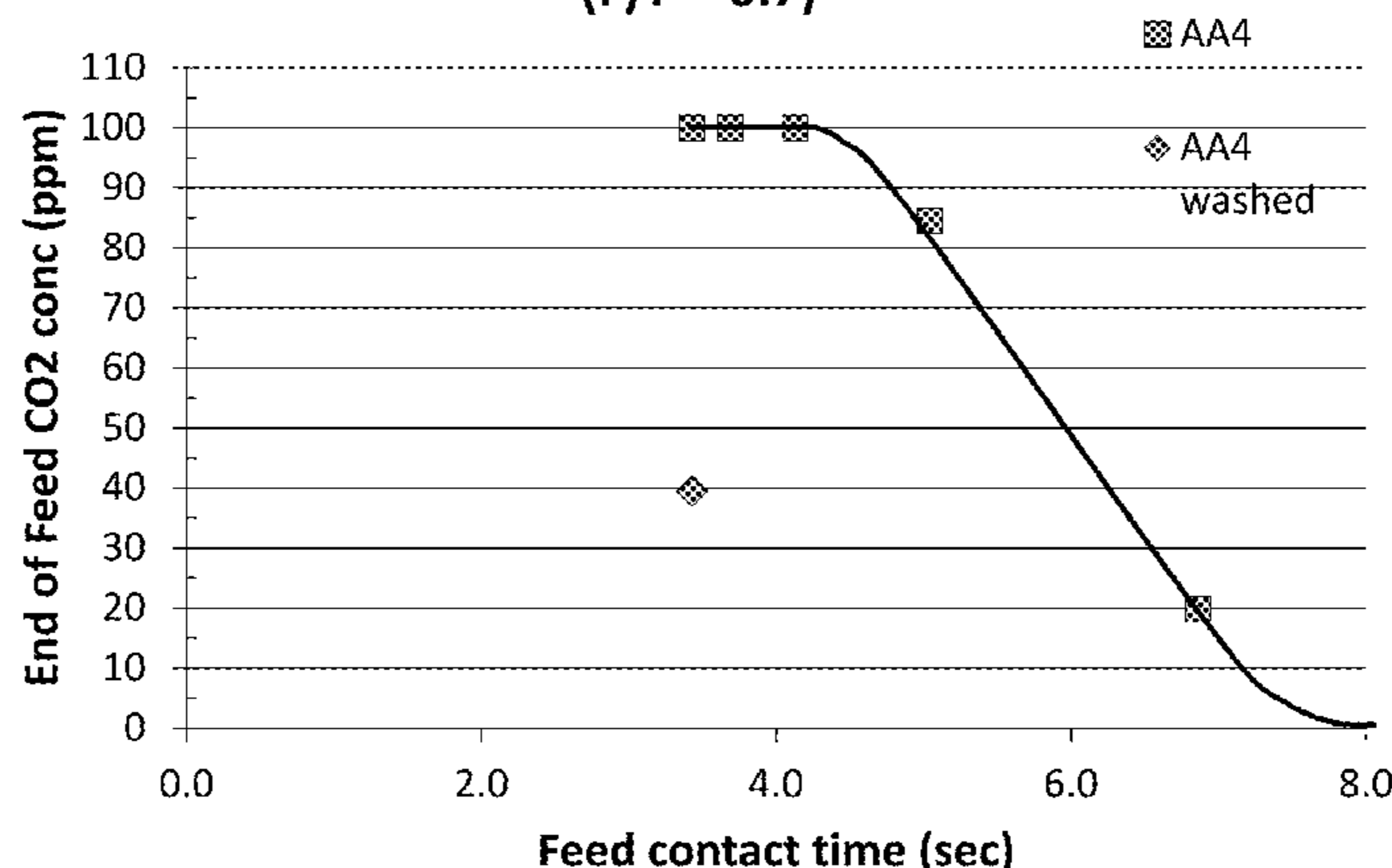
Alumina PSA vs. Contact time (P/F = 0.7)
