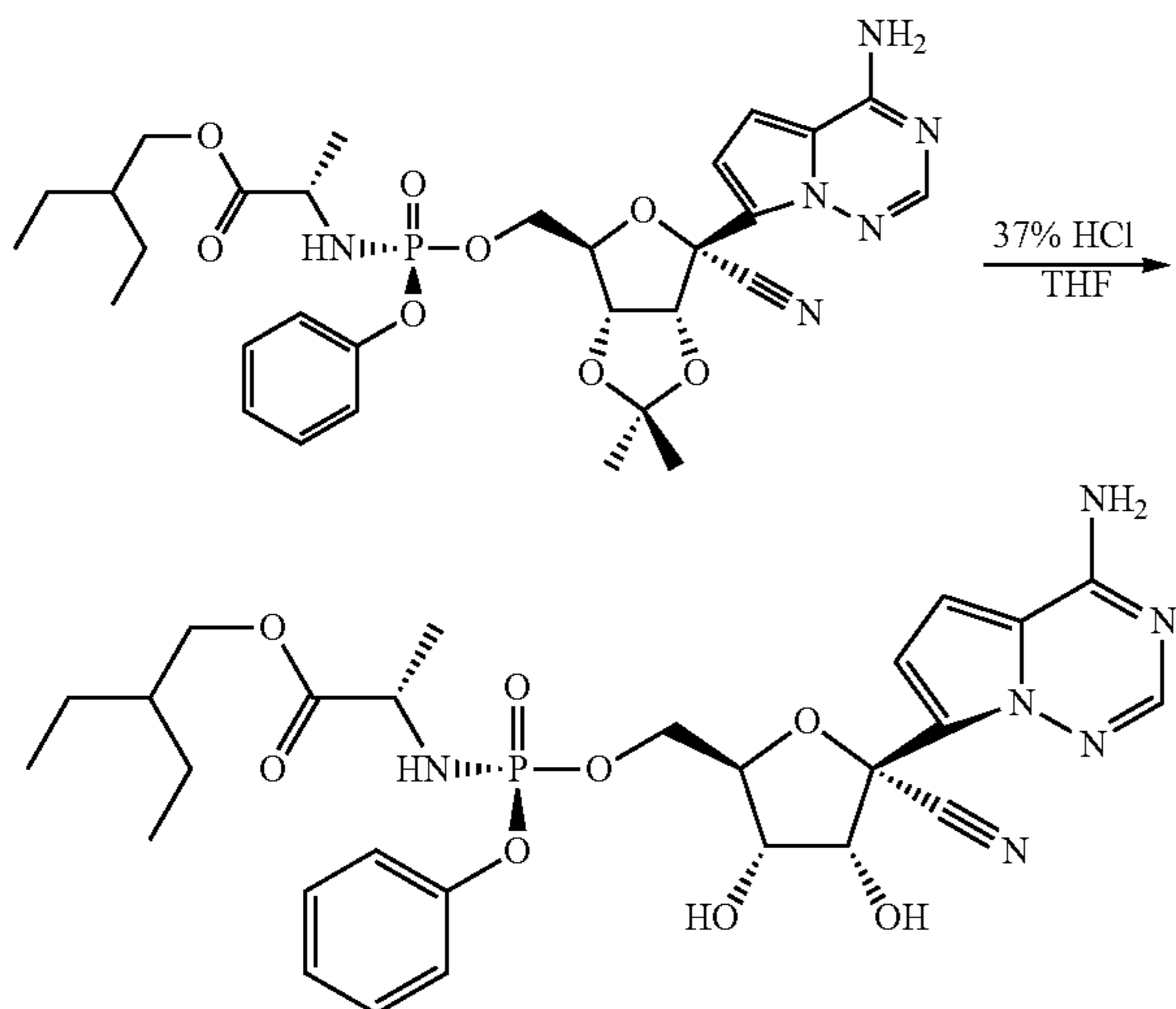
Compound 32
