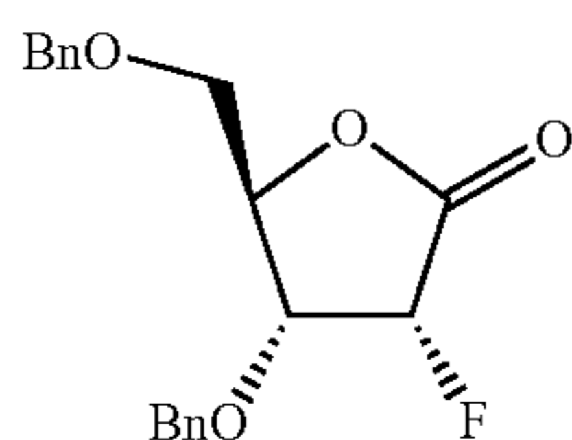
(3R,4R,5R)-4-(benzyloxy)-5-(benzyloxymethyl)-3-fluorodihydrofuran-2(3H)-one
