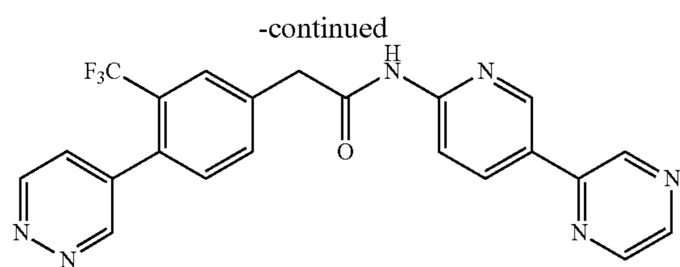
compound 118
