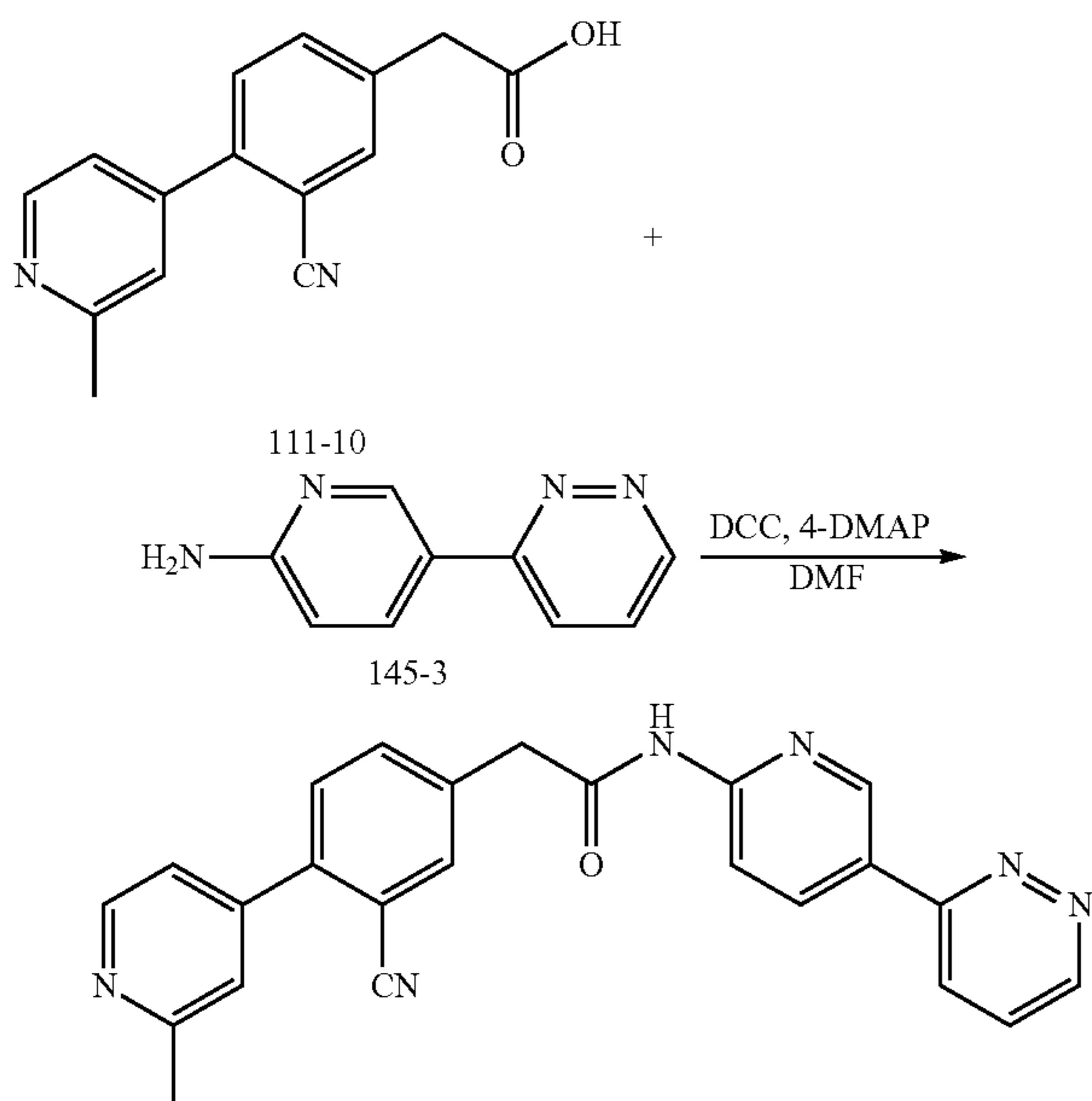
compound 181
