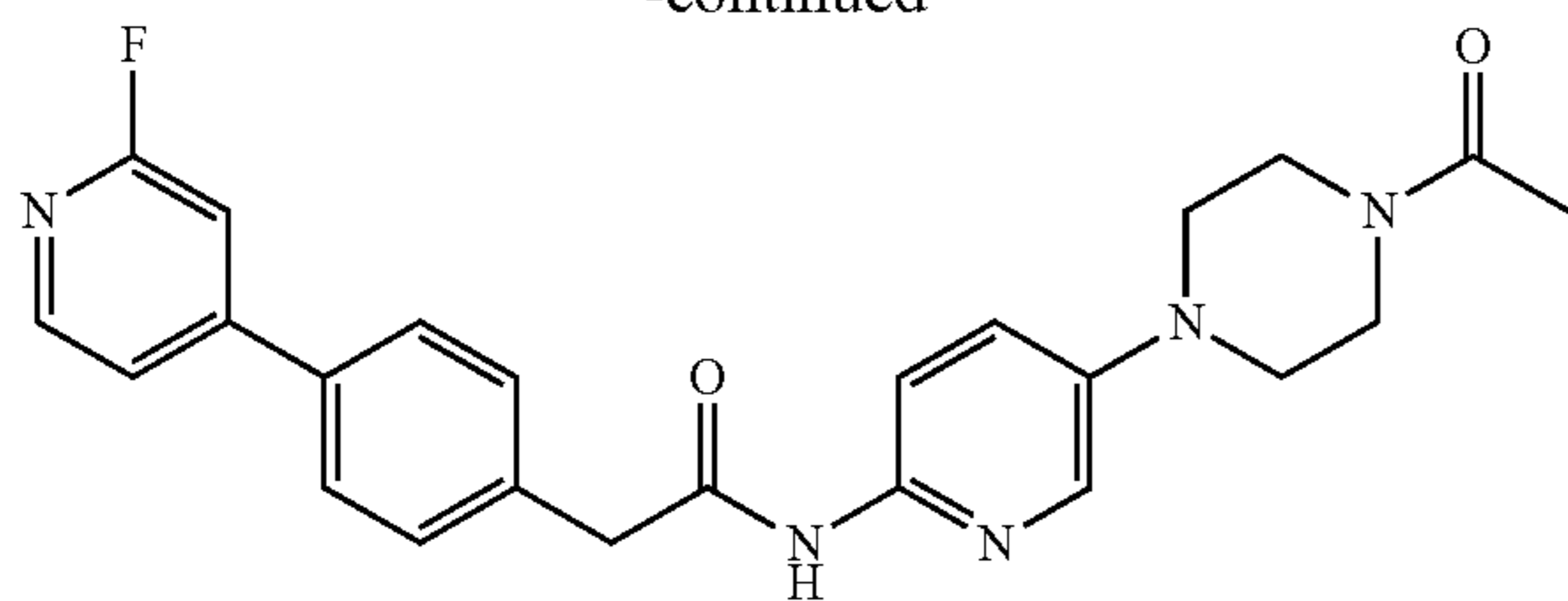
Compound 178
