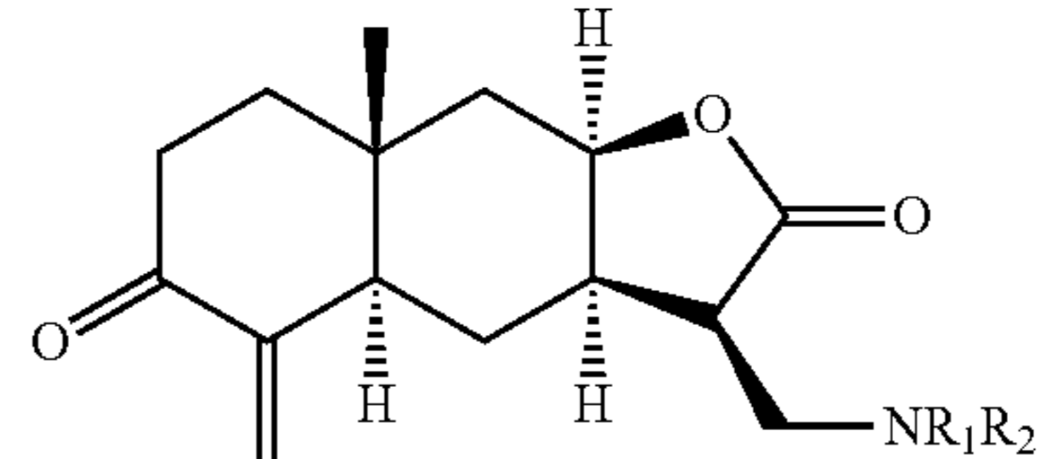
Amino-3-oxo-isoalantolactones
