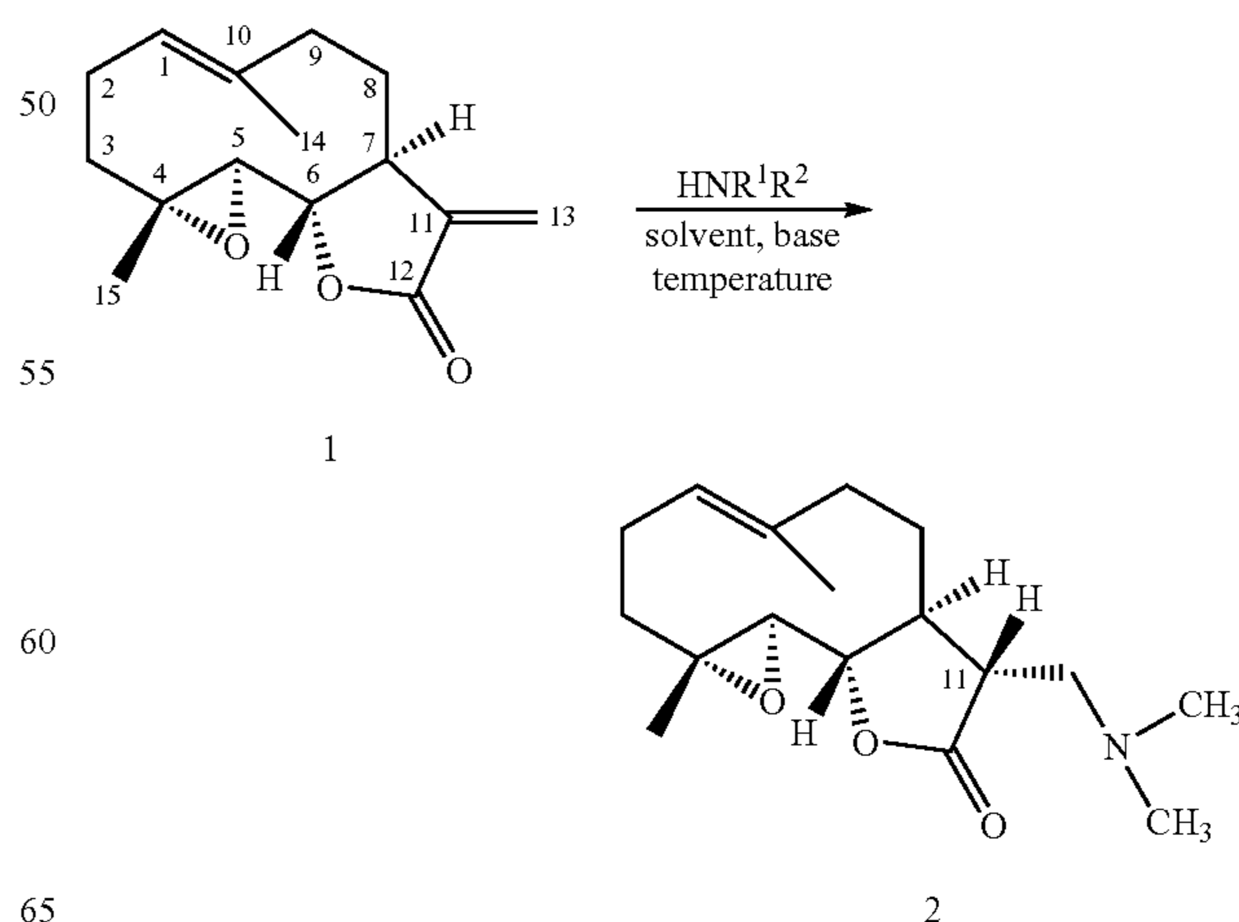
Scheme I
