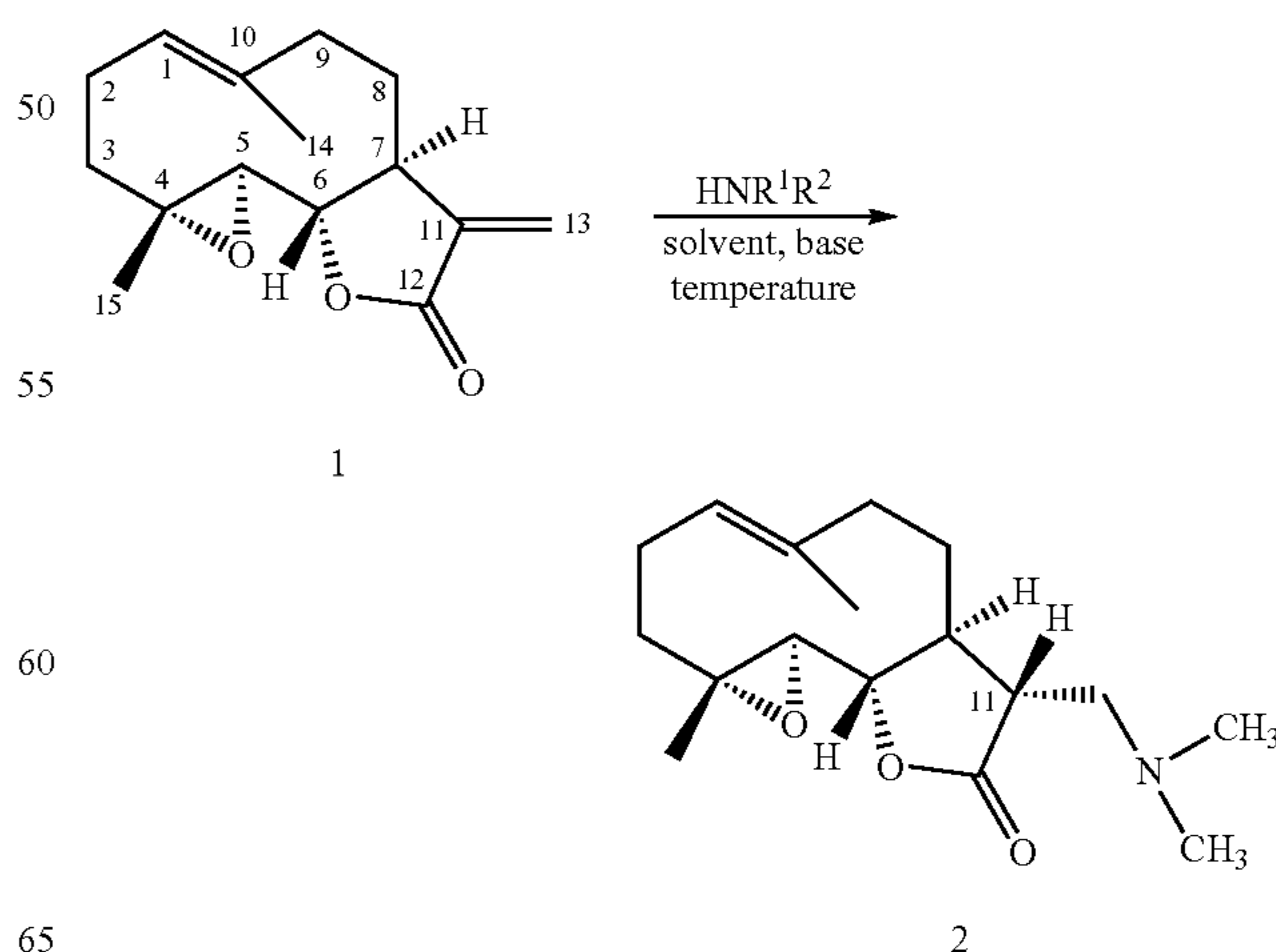
Scheme I
