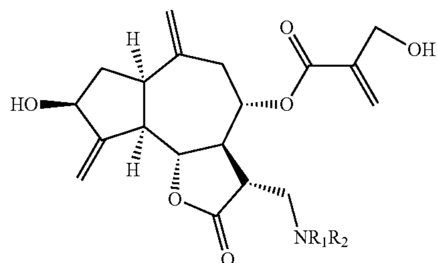
Aminocynarpicrins
