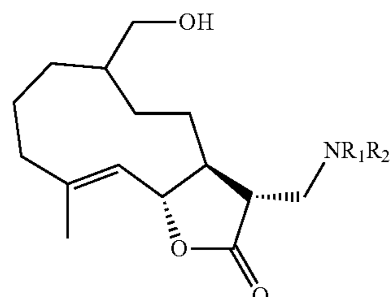
Aminosoulangianolides
