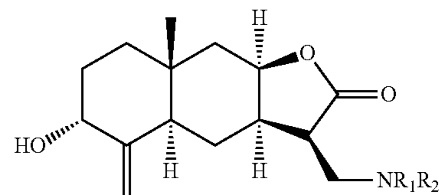
Aminoisotelekins
