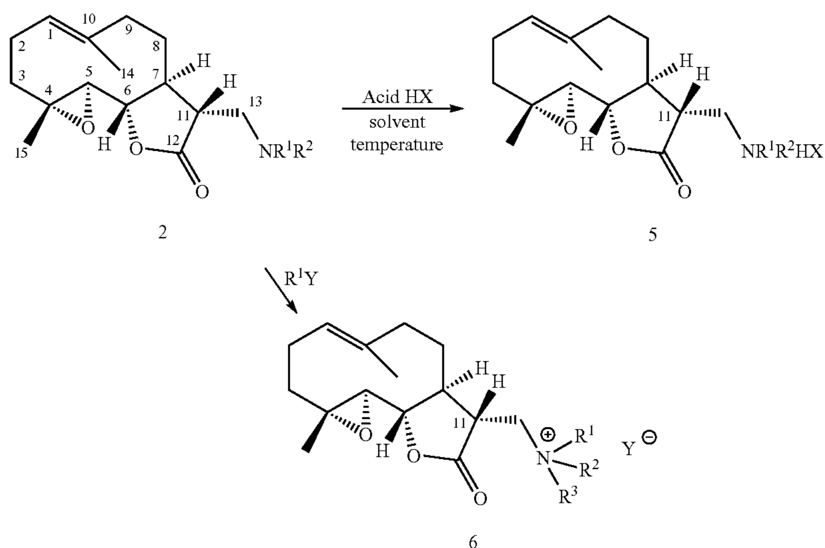
Scheme III
