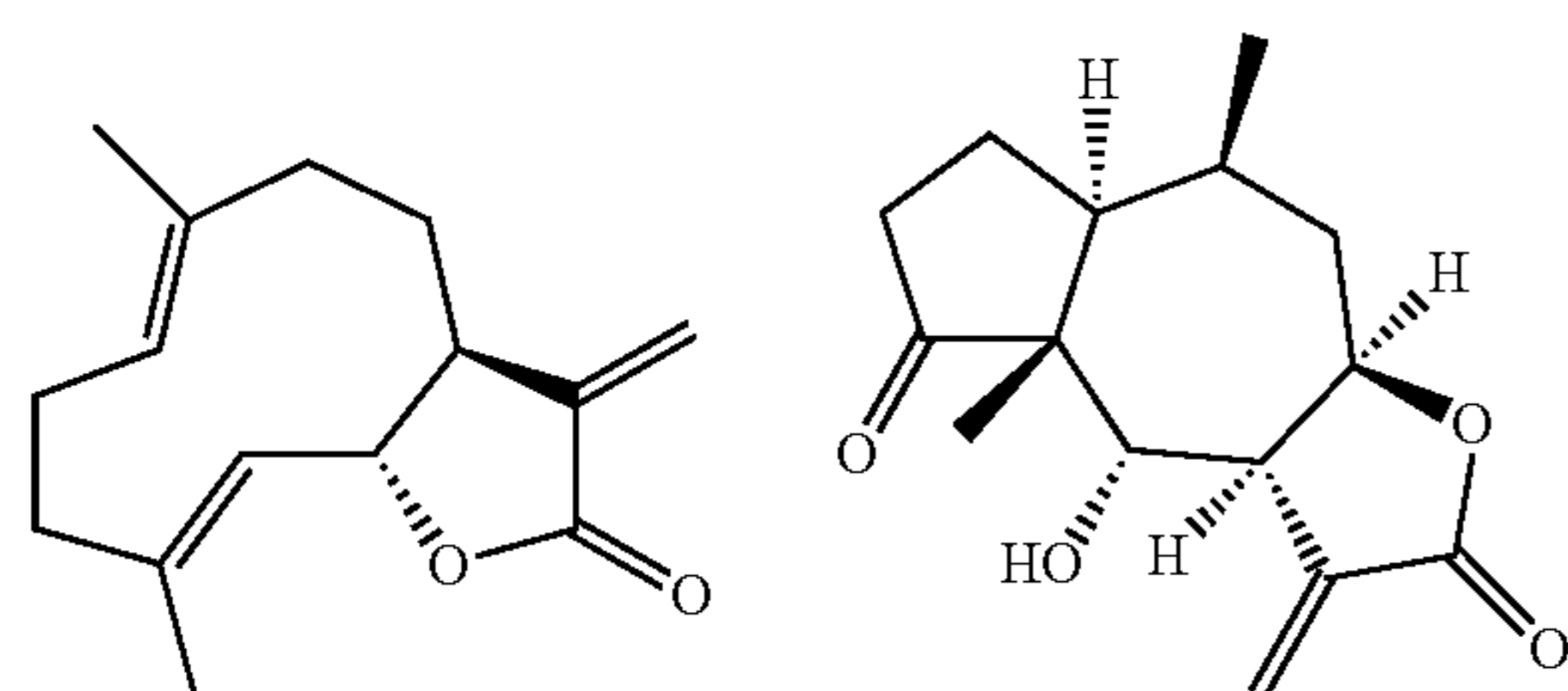
Costunolide
