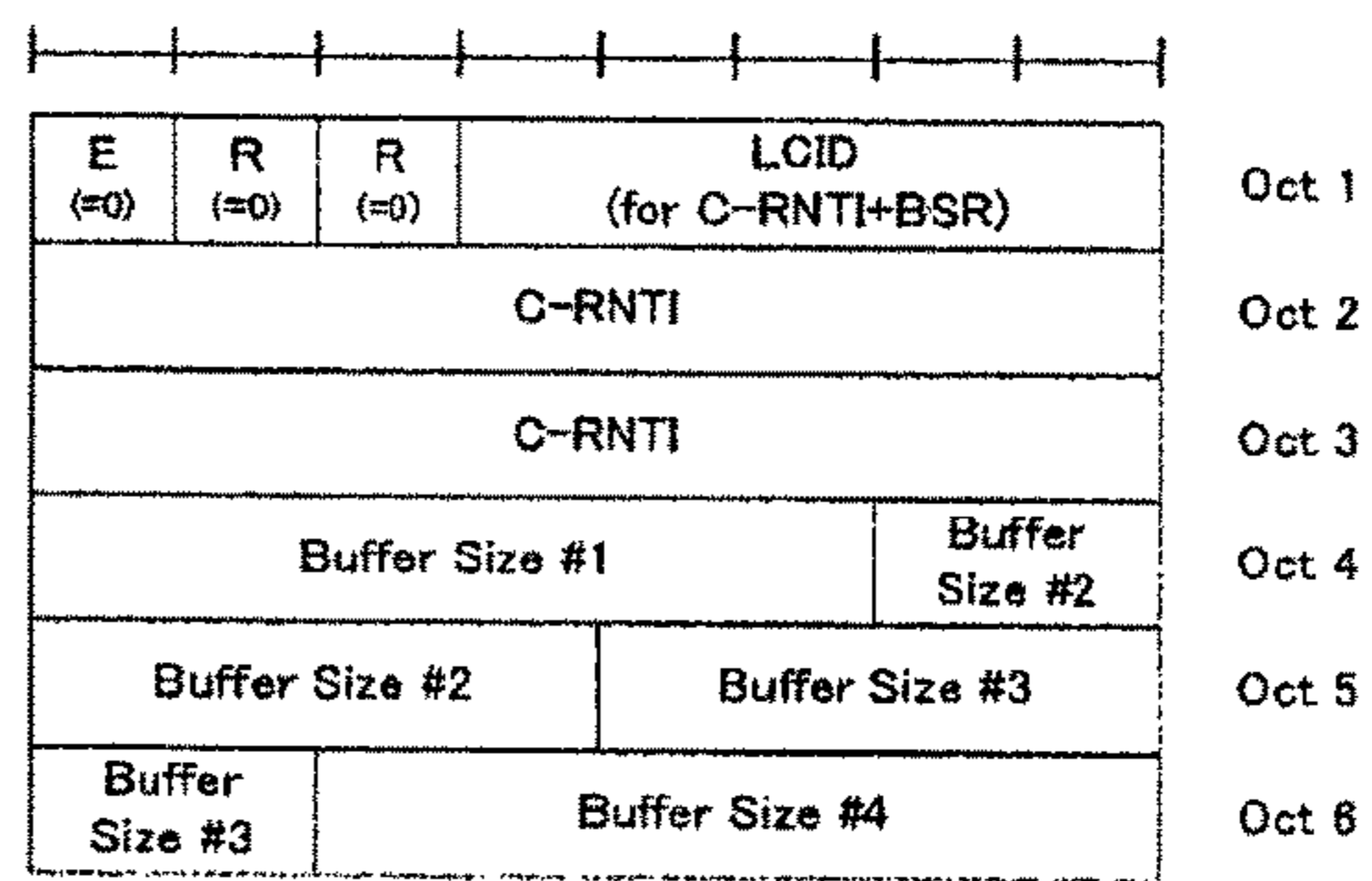
(d) C-RNTI + BSR e.g. for UL data resuming and handover (if BSR is prioritized)
