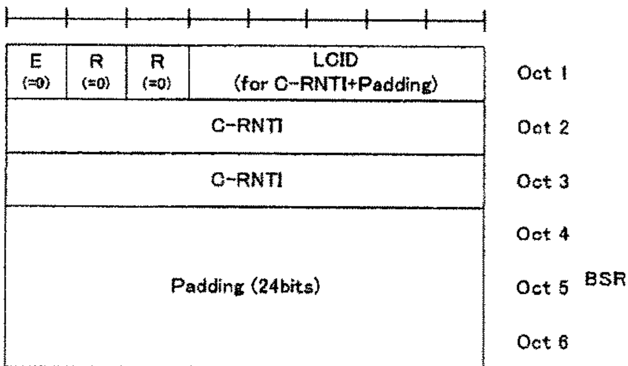
(c) Only C-RNTI
