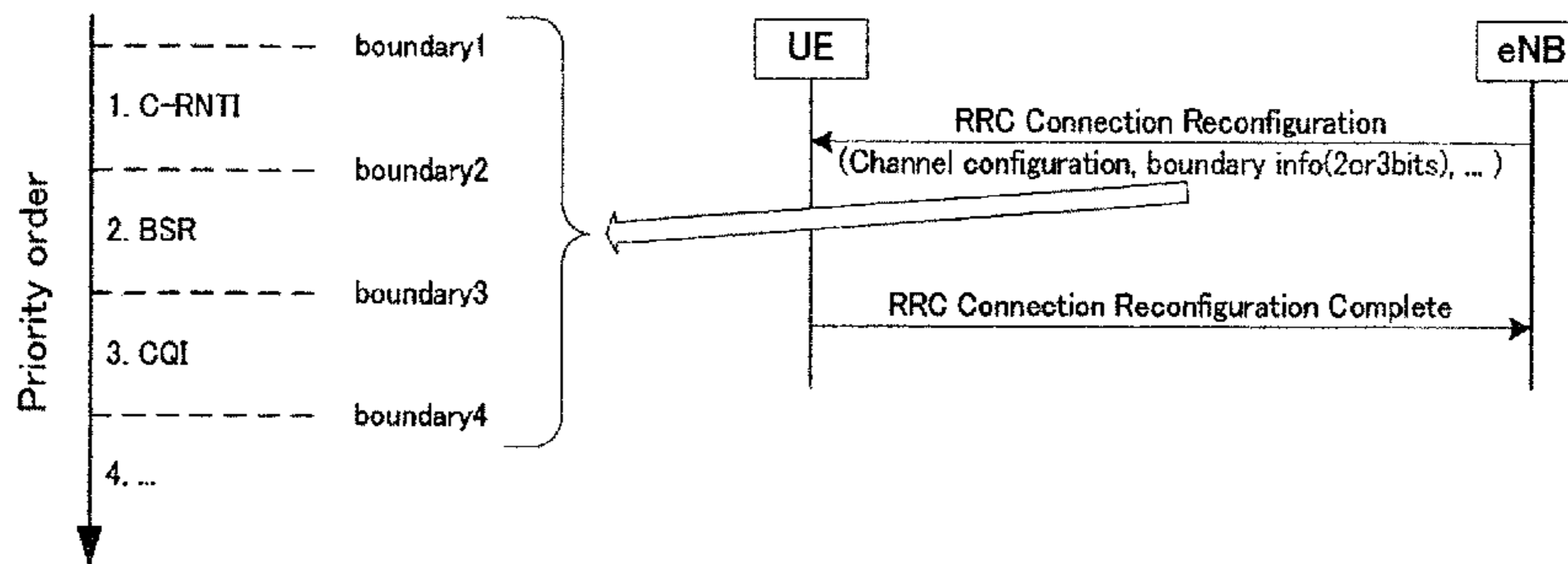
(a) priority order of MAC control elements
