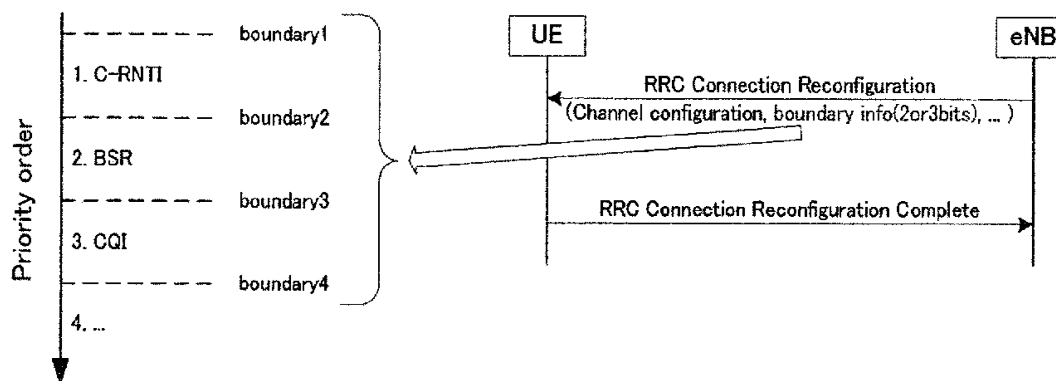
(a) priority order of MAC control elements
