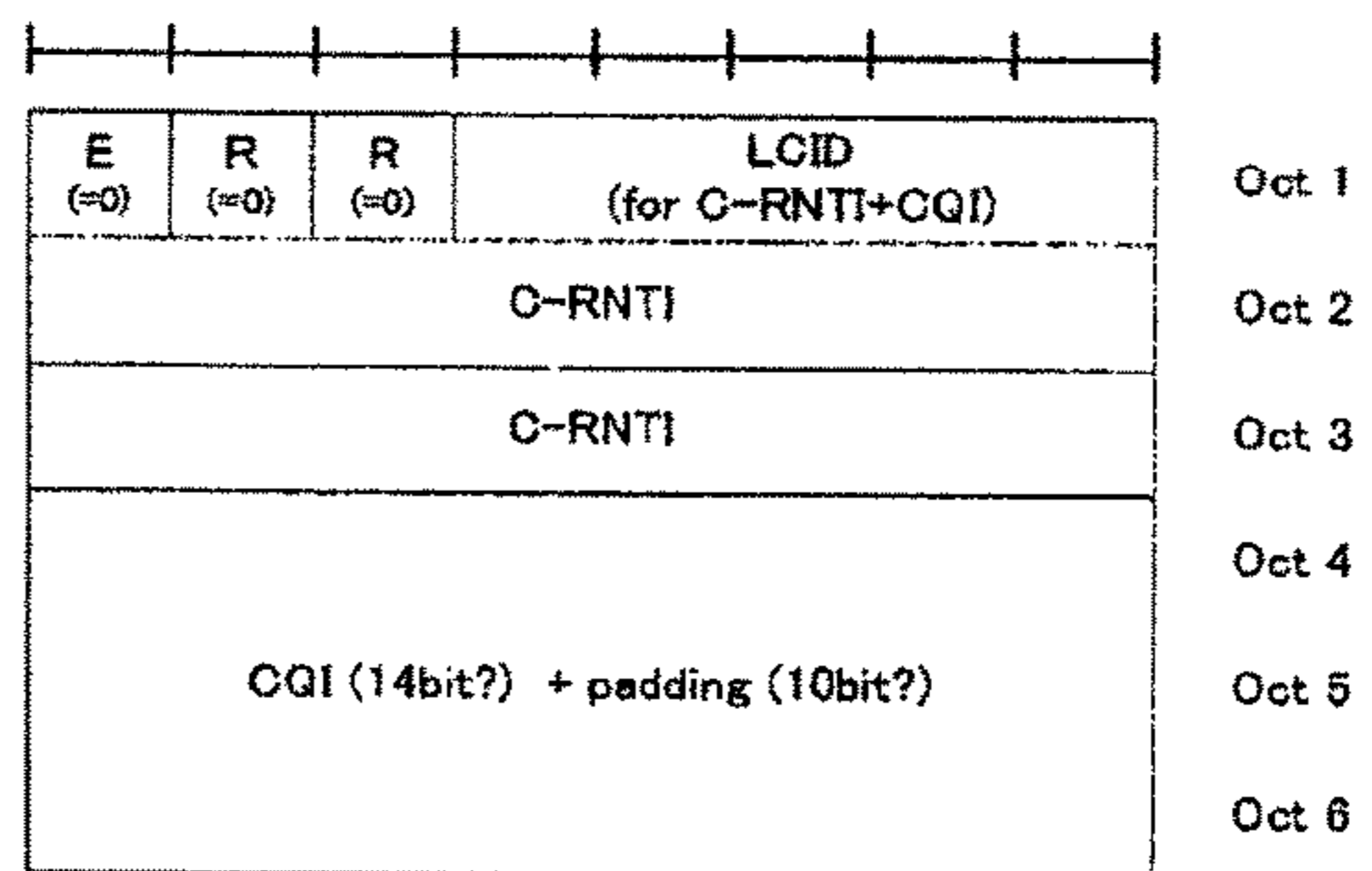
(f) C-RNTI + CQI e.g. for DL data resuming
