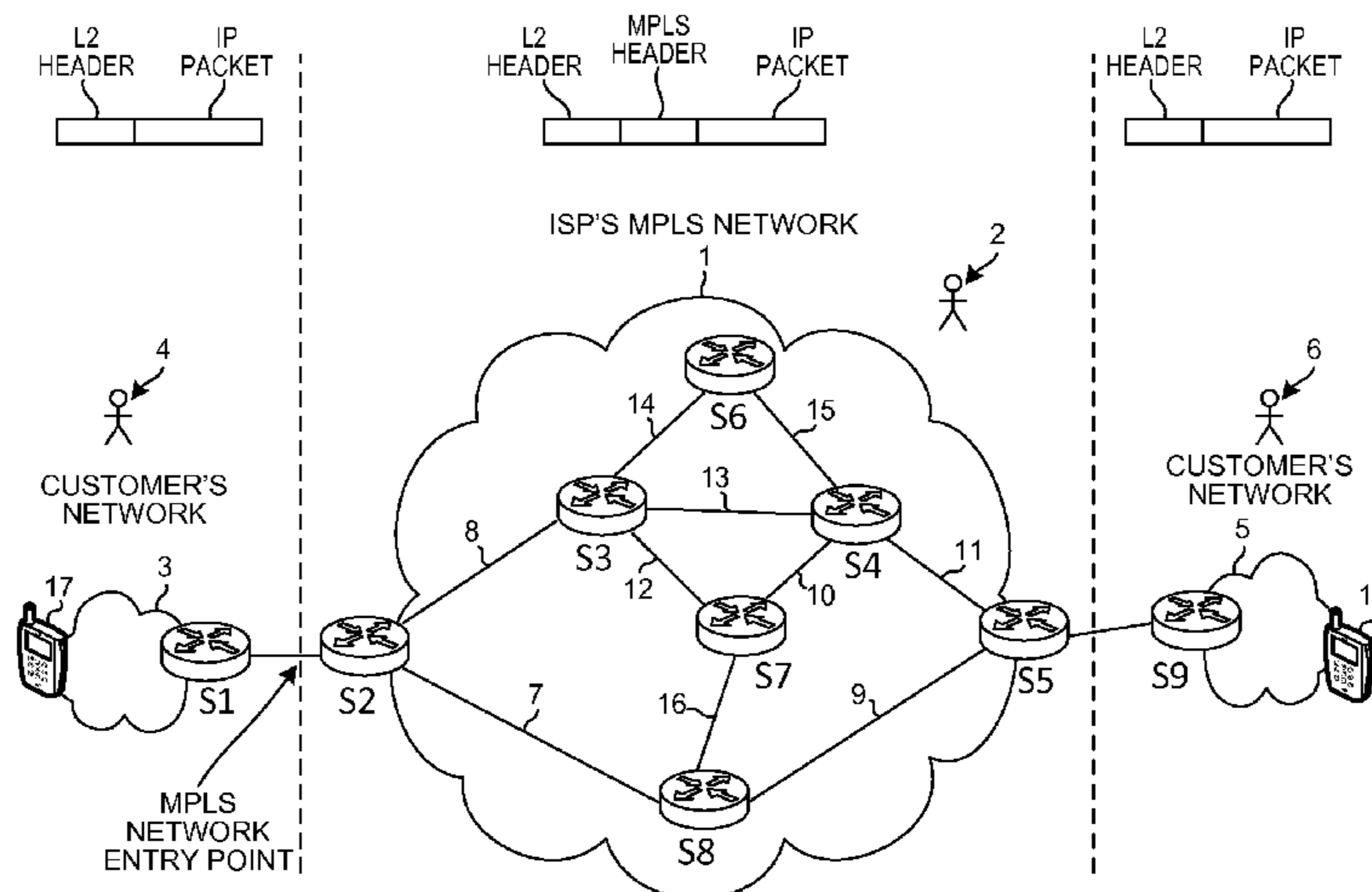
EXEMPLARY SYSTEM INVOLVING AN MPLS NETWORK
