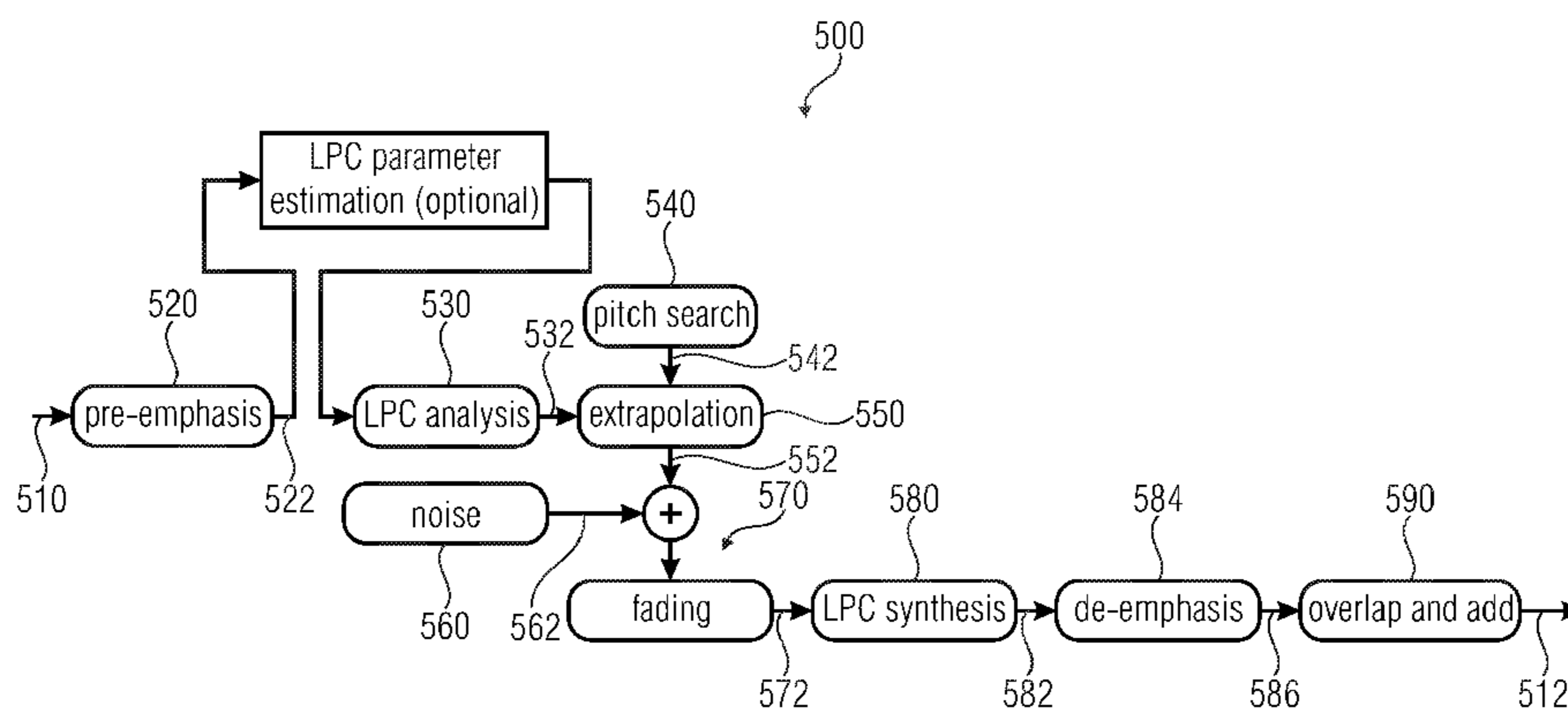
Time domain concealment overview for transform decoder
