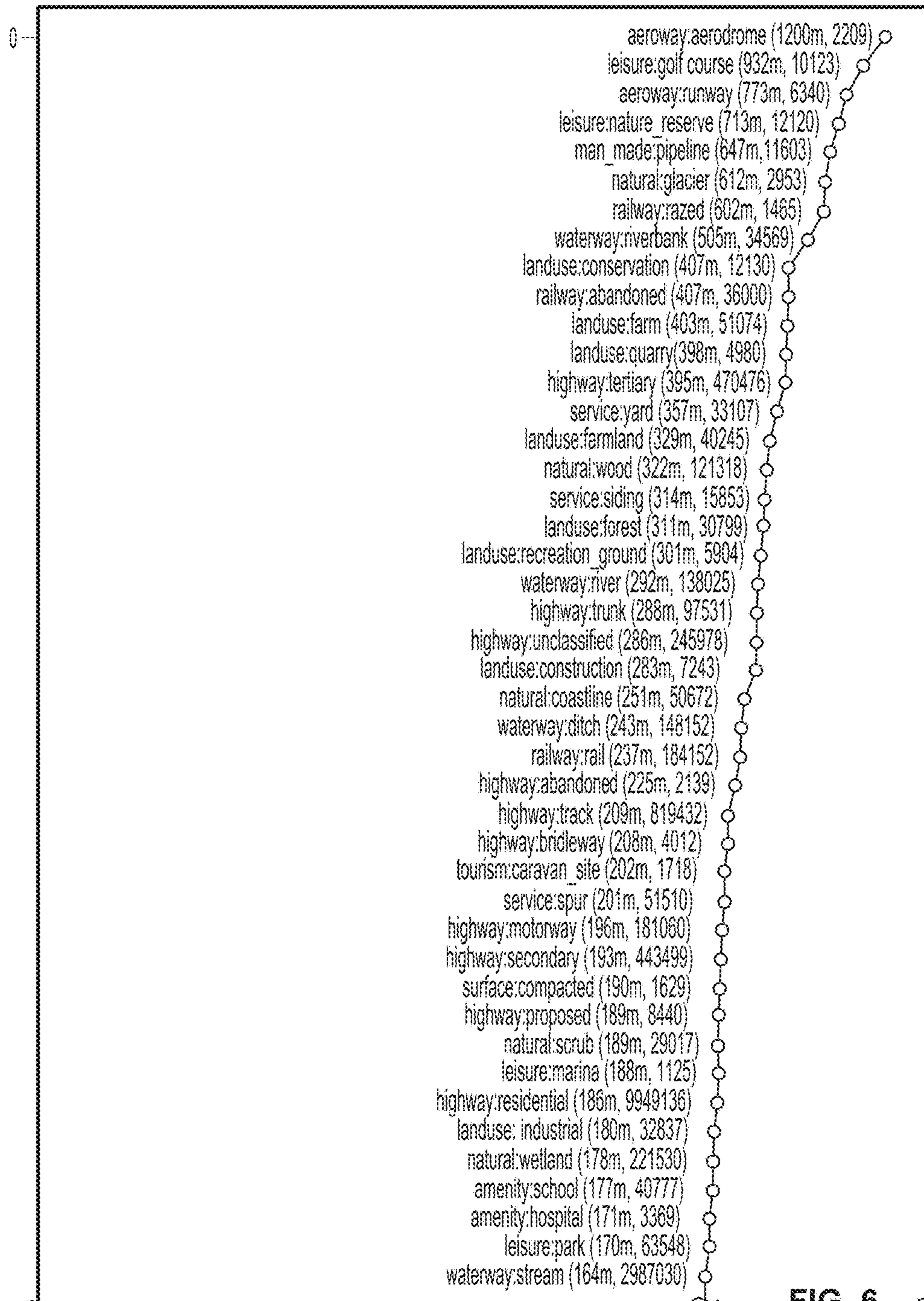
OSM "Ways" with >1000 instances in USA, [name (size, count)]
