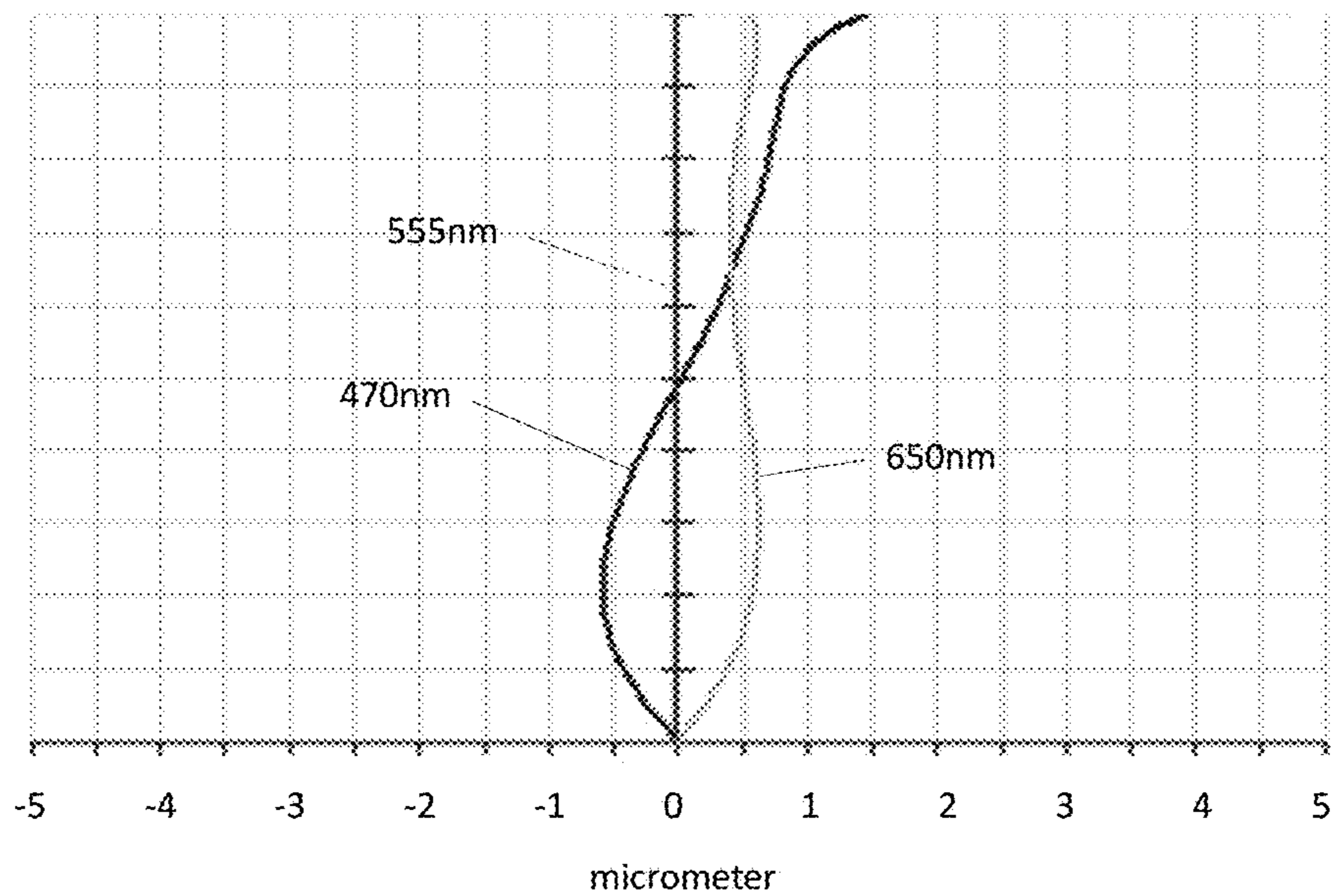
Lateral color
