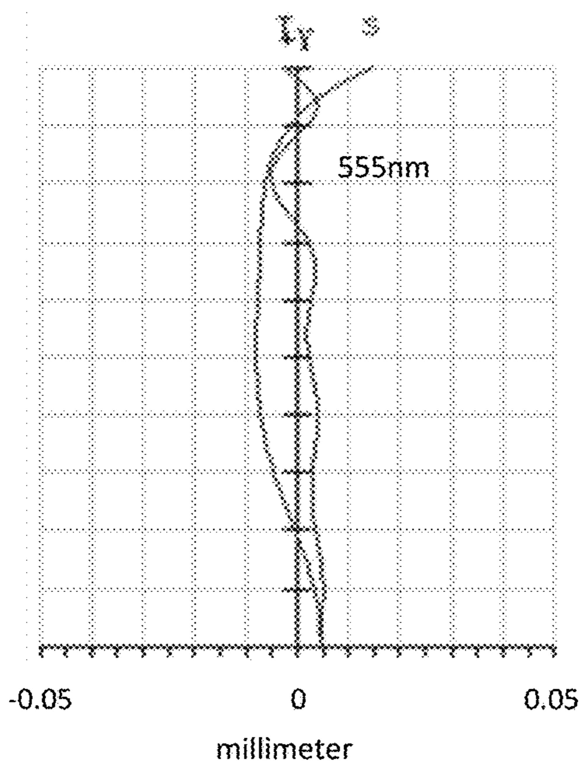
Field curvature
