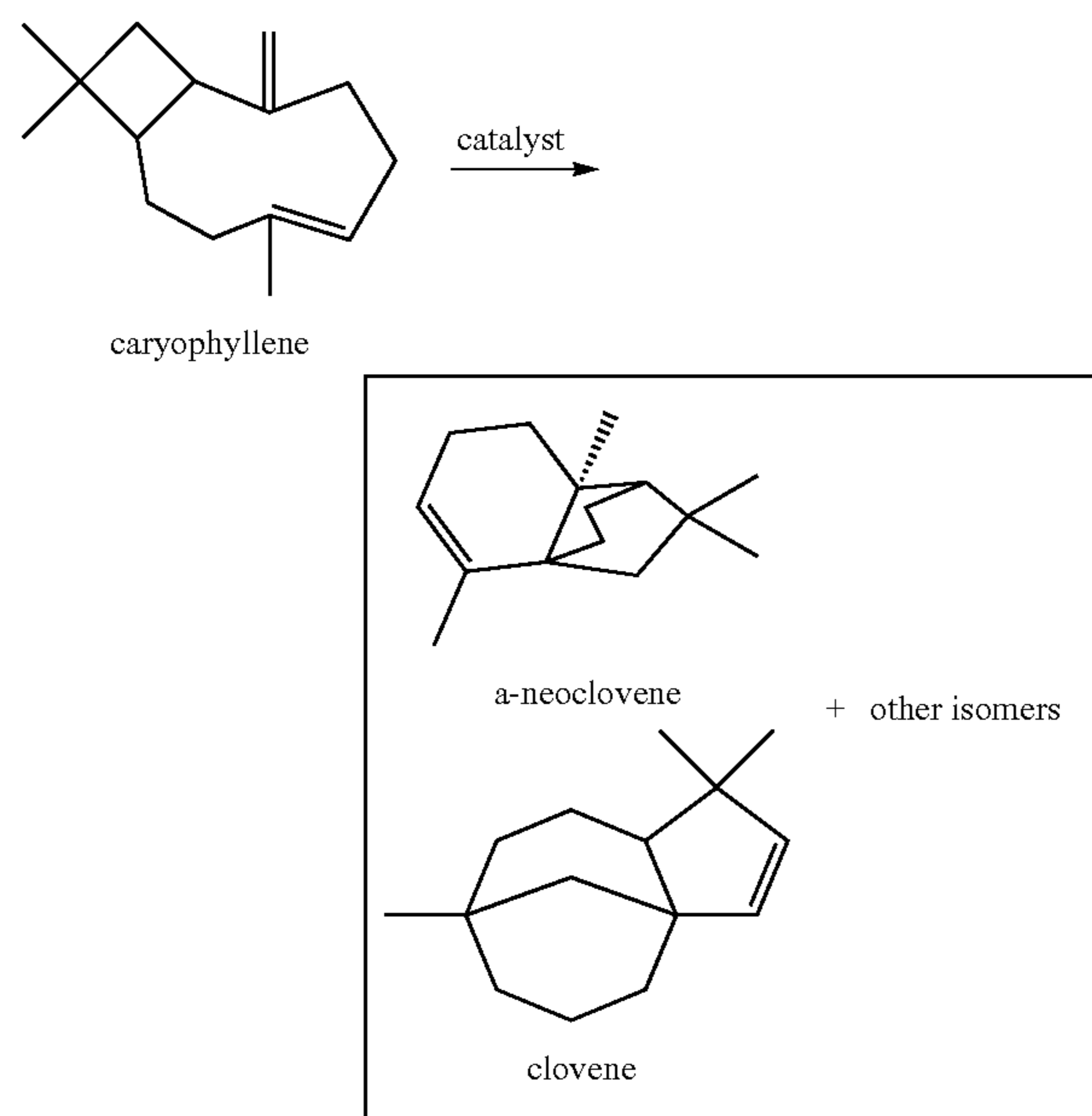
Scheme 2. Isomerization of caryophyllene with a heterogeneous acid catalyst.
