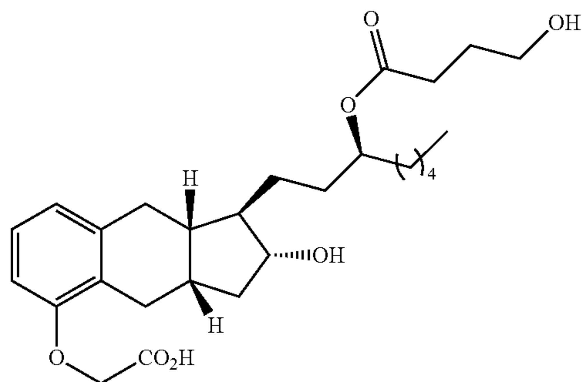
Compound Ib-18
