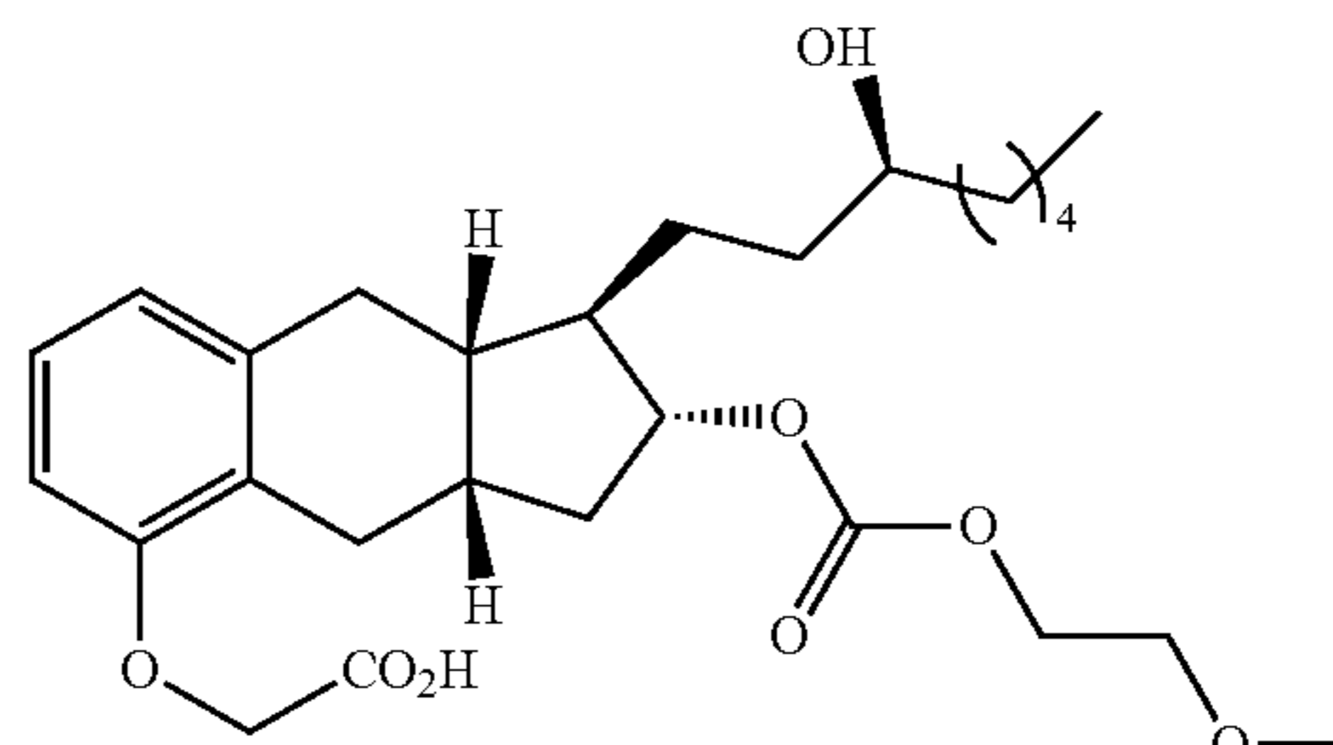
Compound Ib-1
