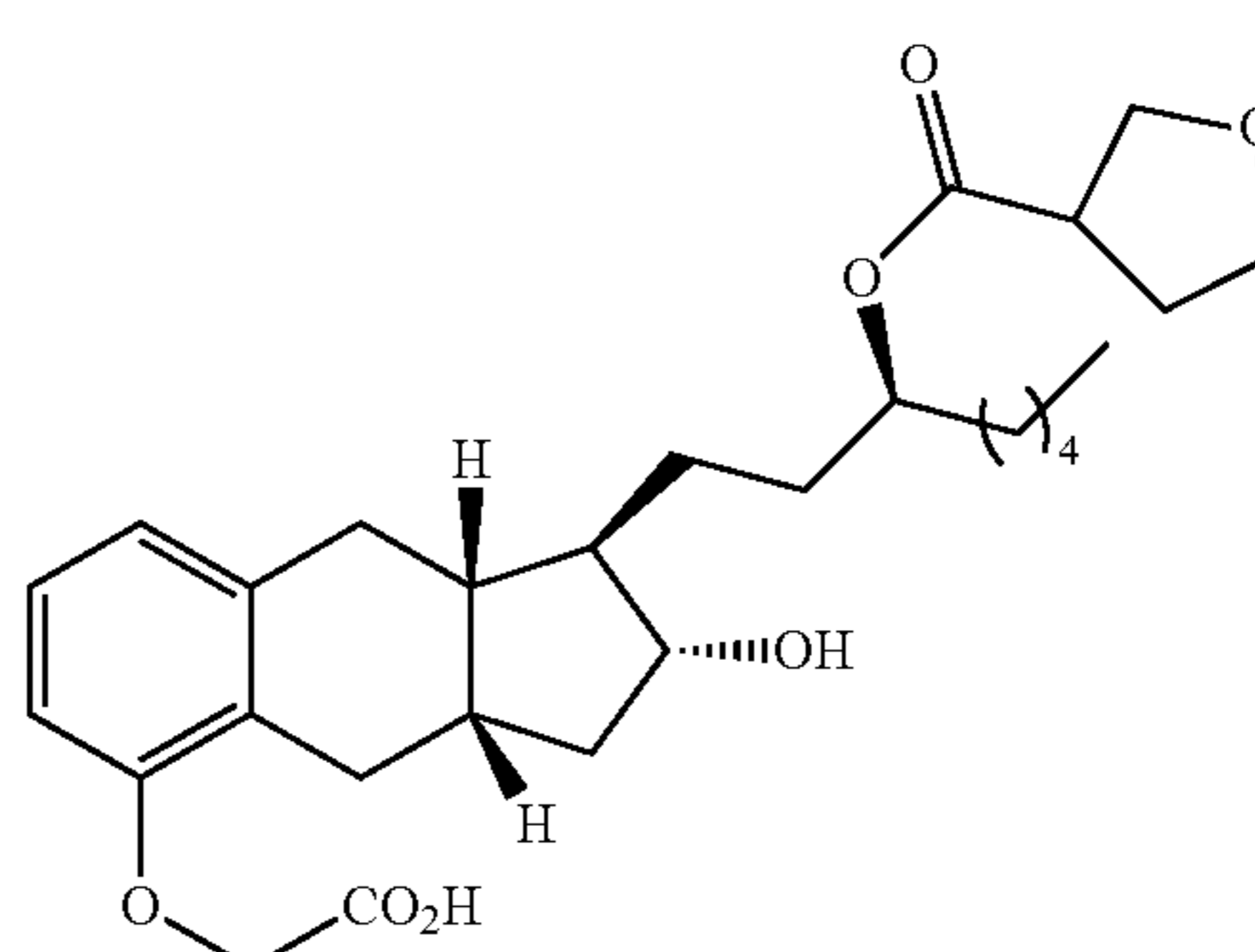
Compound Ib-33
