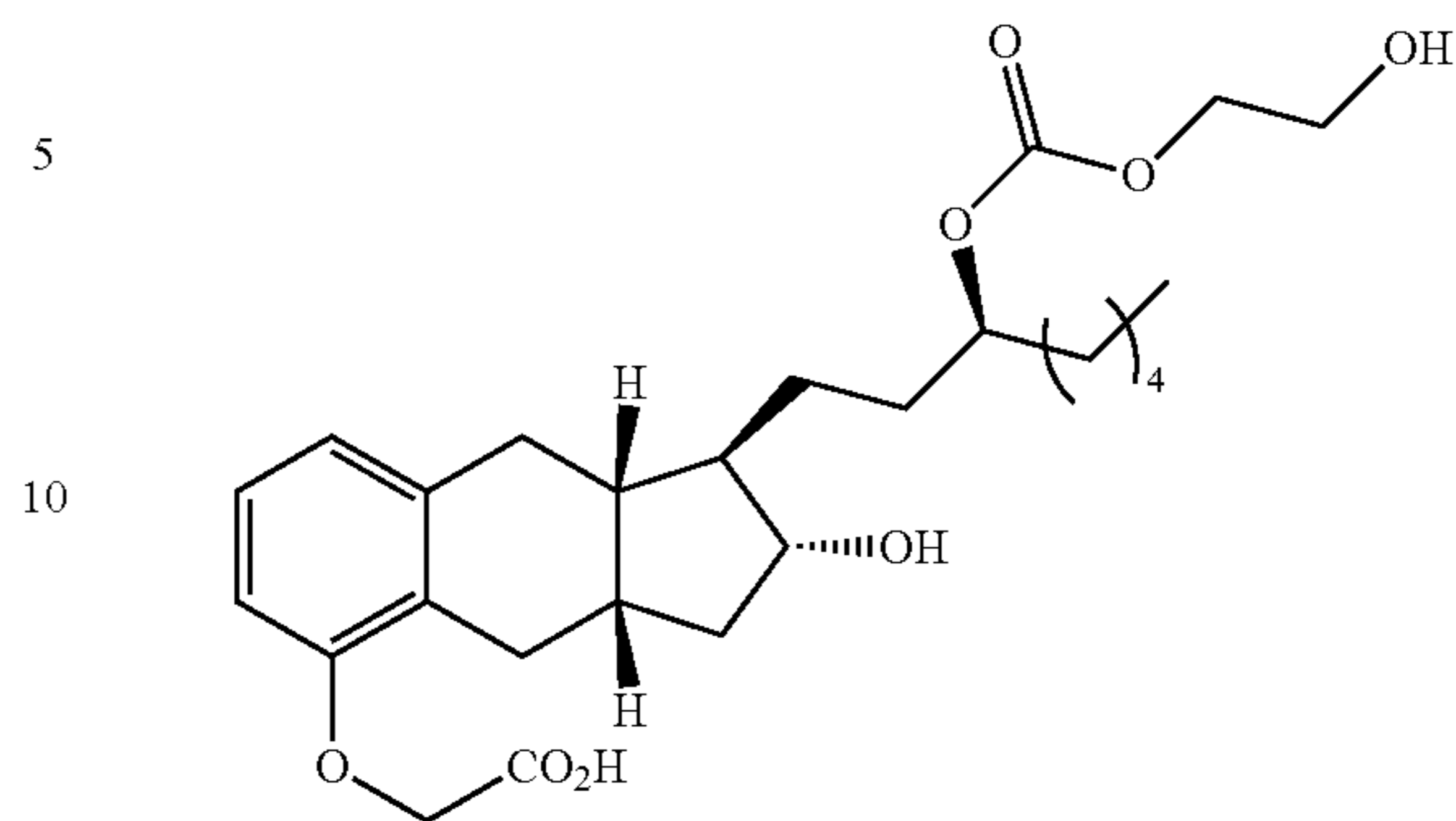
Compound Ib-15
