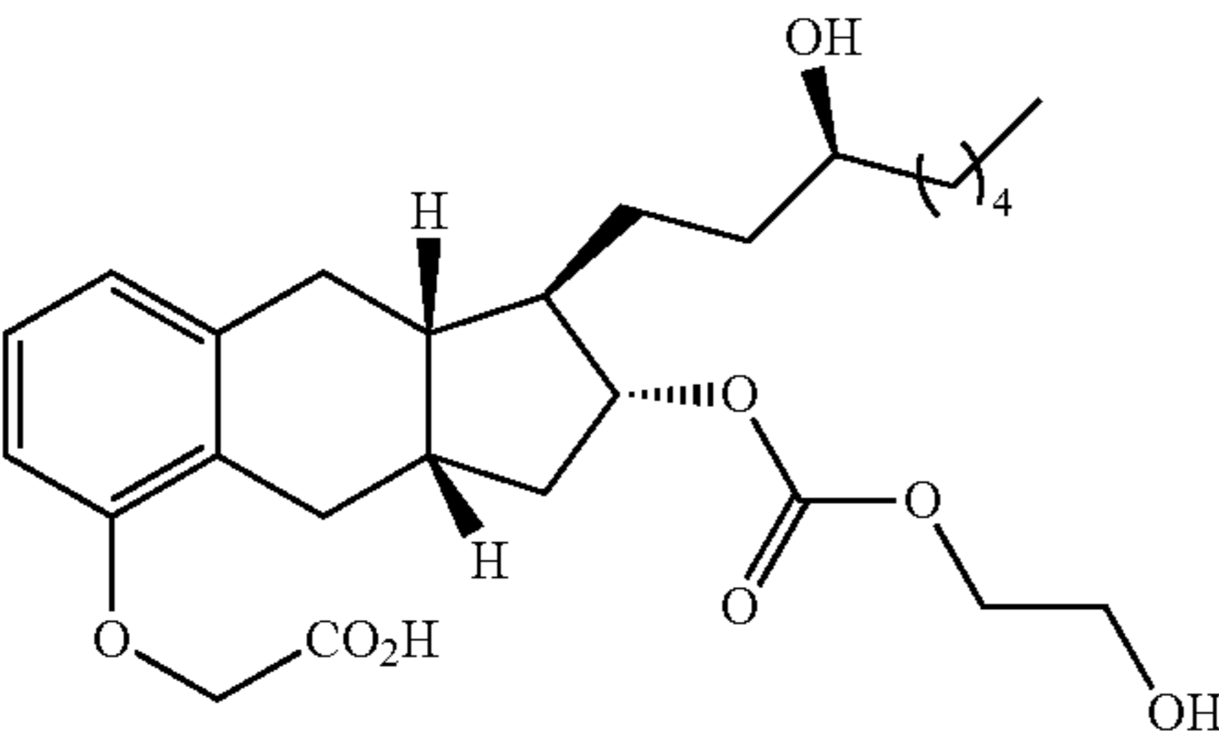
Compound Ia-14
