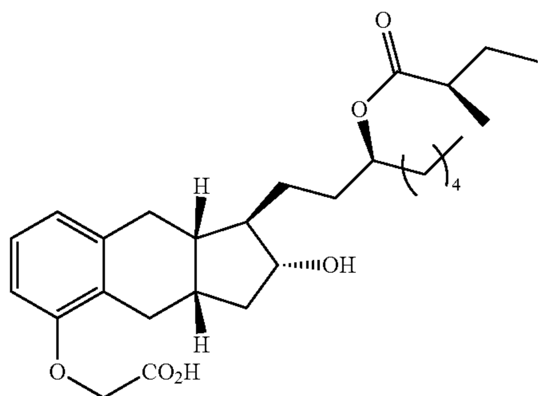
Compound Ib-28
