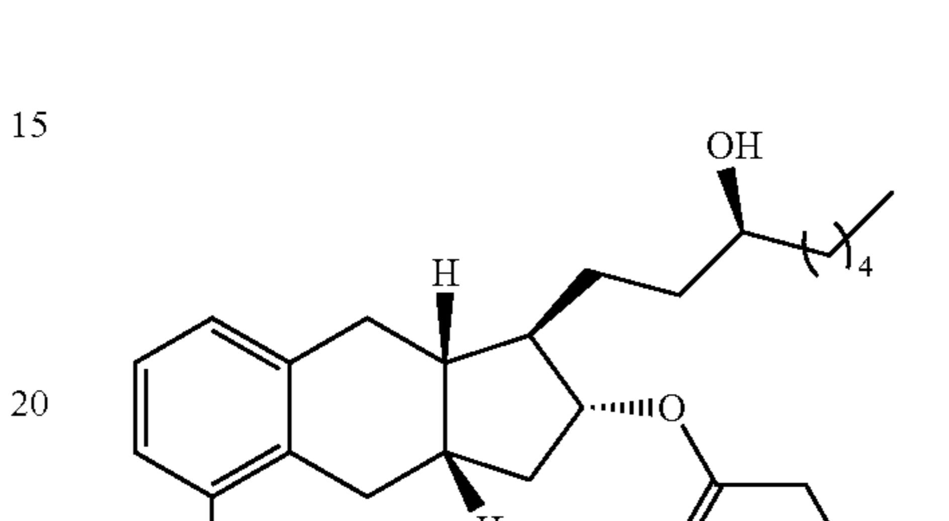
Compound 1a-9
