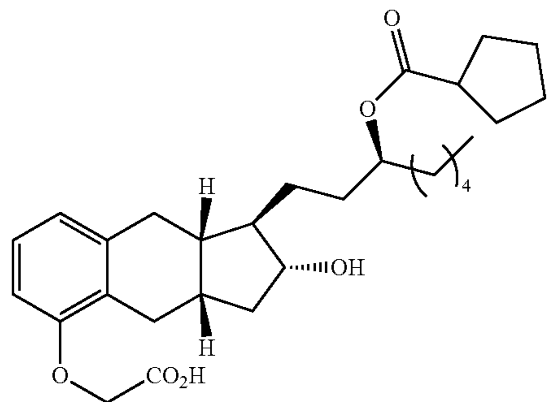
Compound Ib-30
