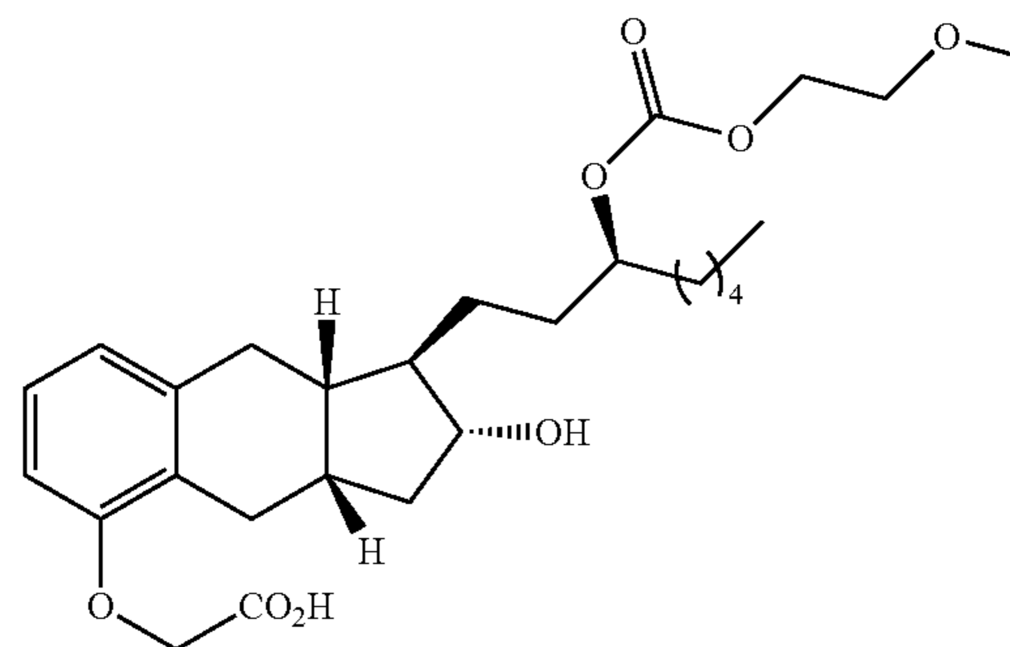
Compound Ib-15
