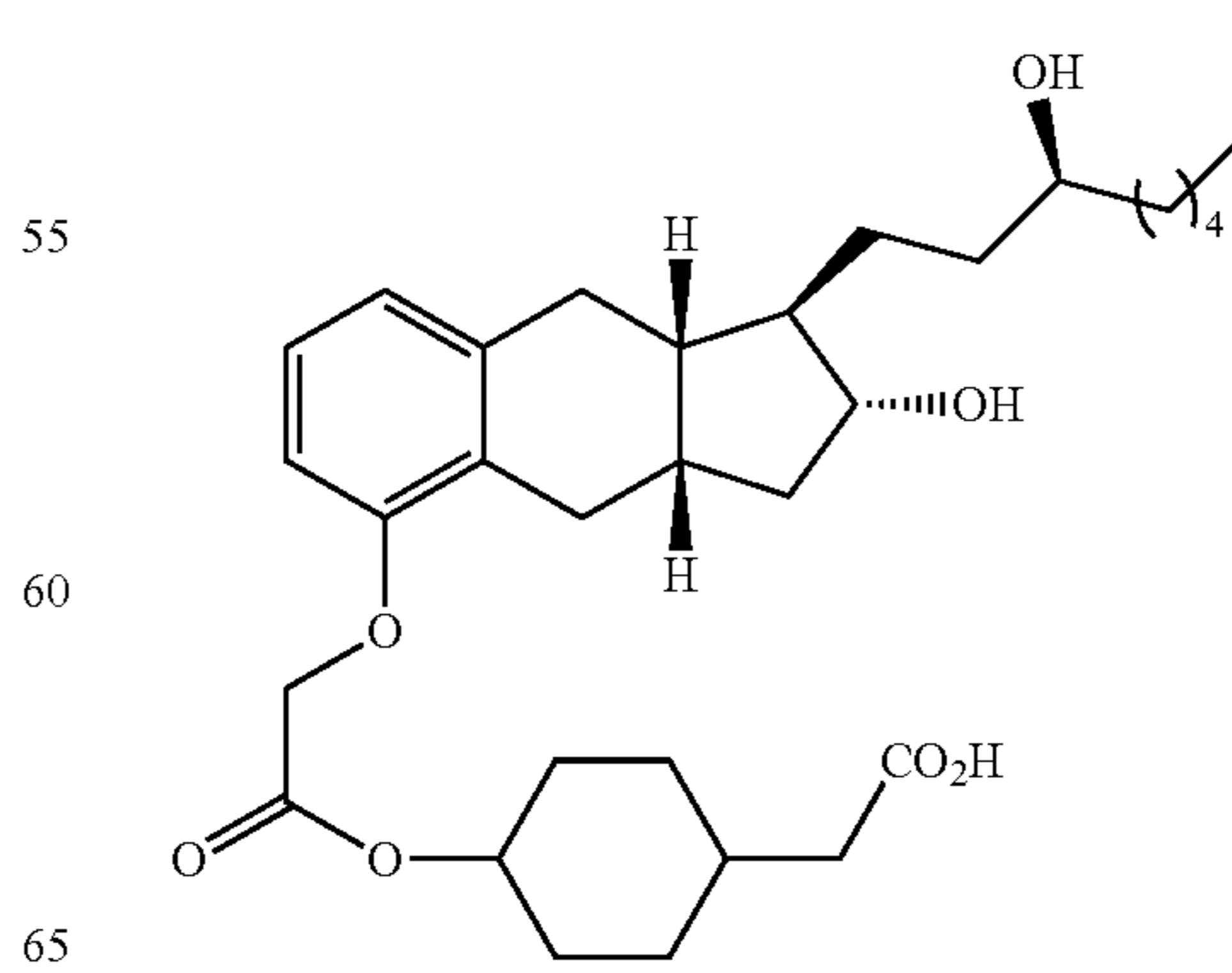
Compound II-21
