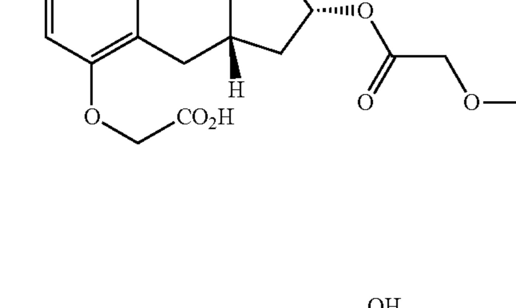
Compound Ia-21
