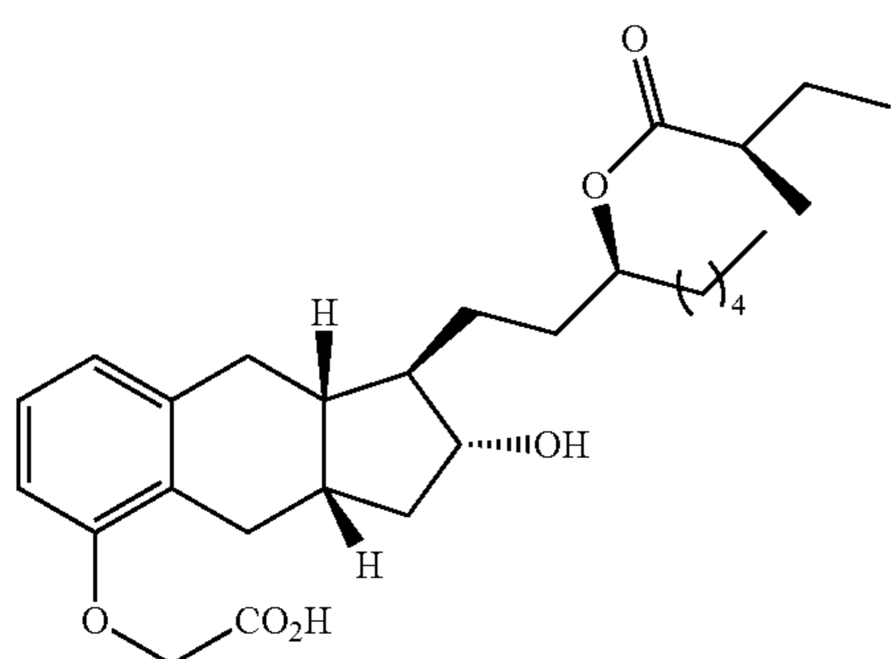
Compound Ib-28
