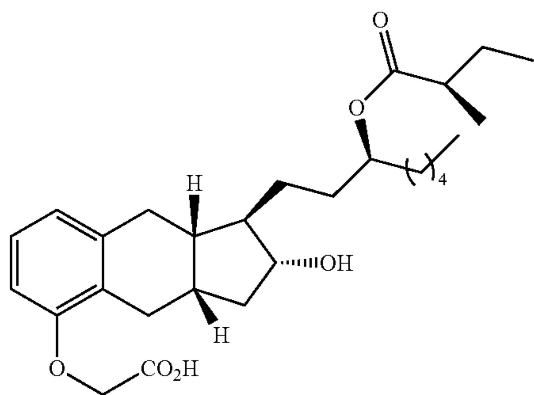
Compound Ib-28
