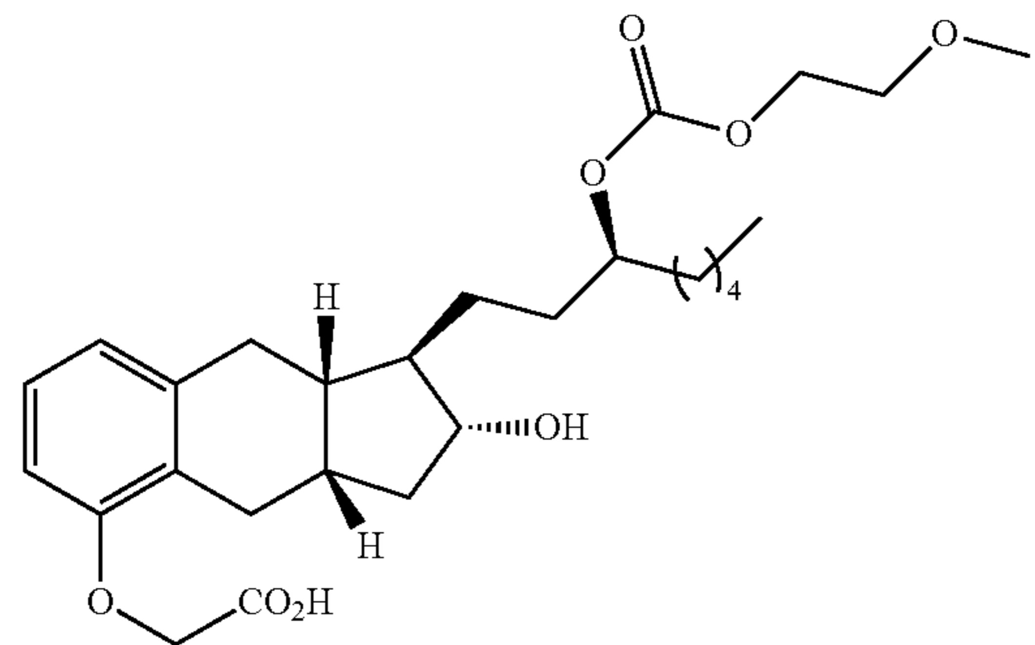
Compound Ib-15
