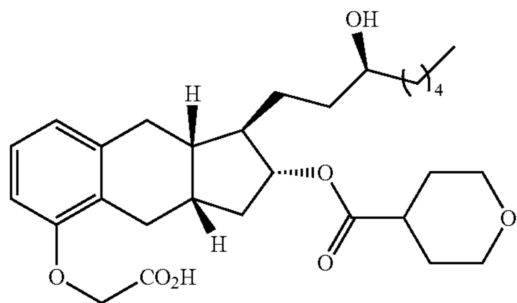
Compound Ia-10
