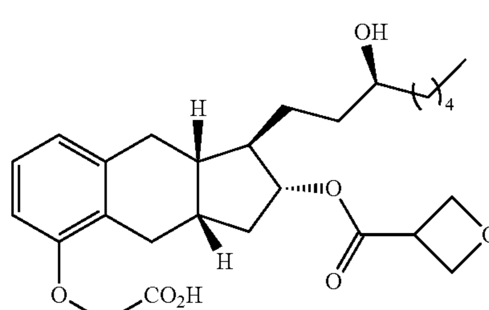
Compound Ia-32
