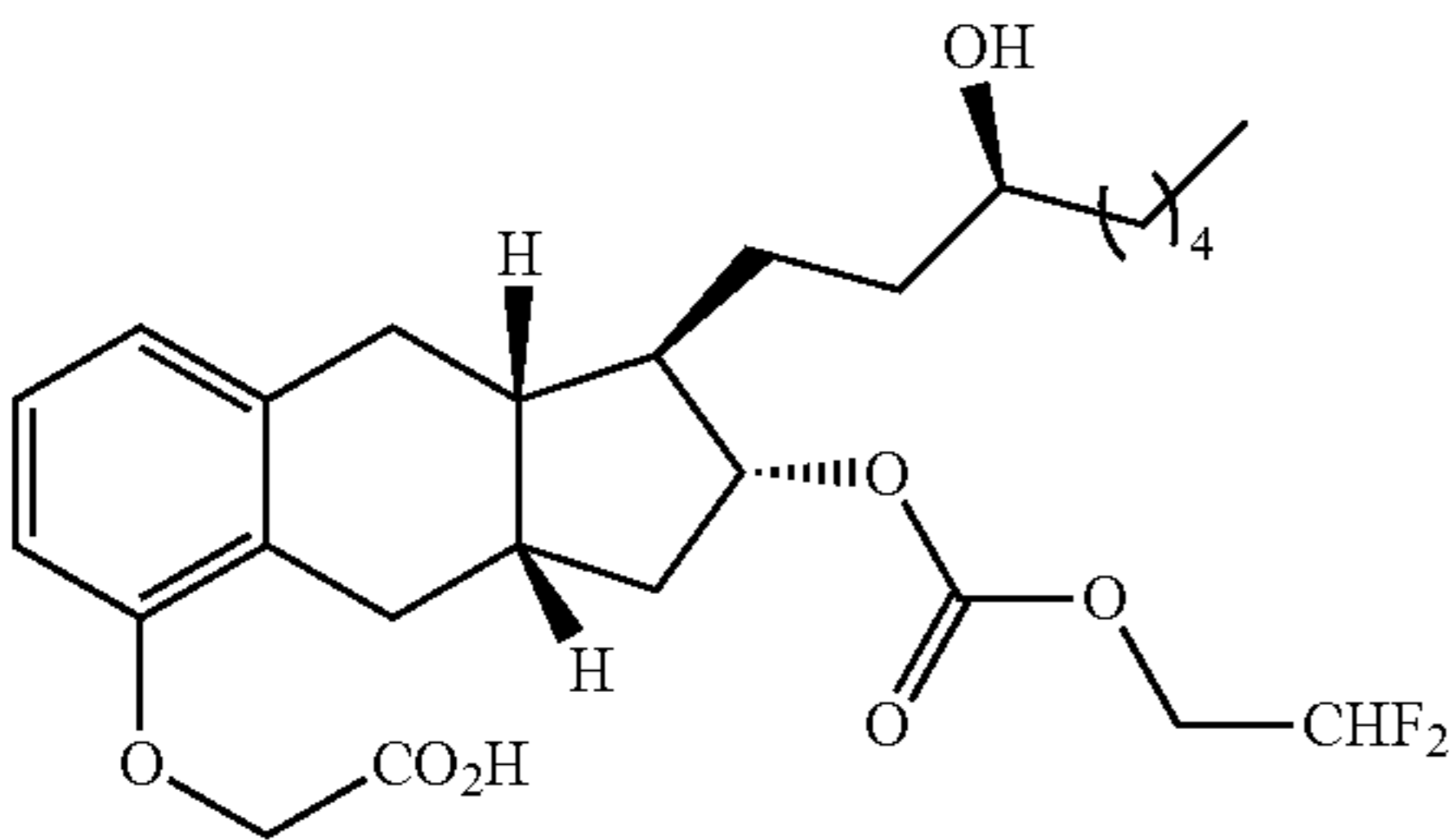
Compound Ia-14
