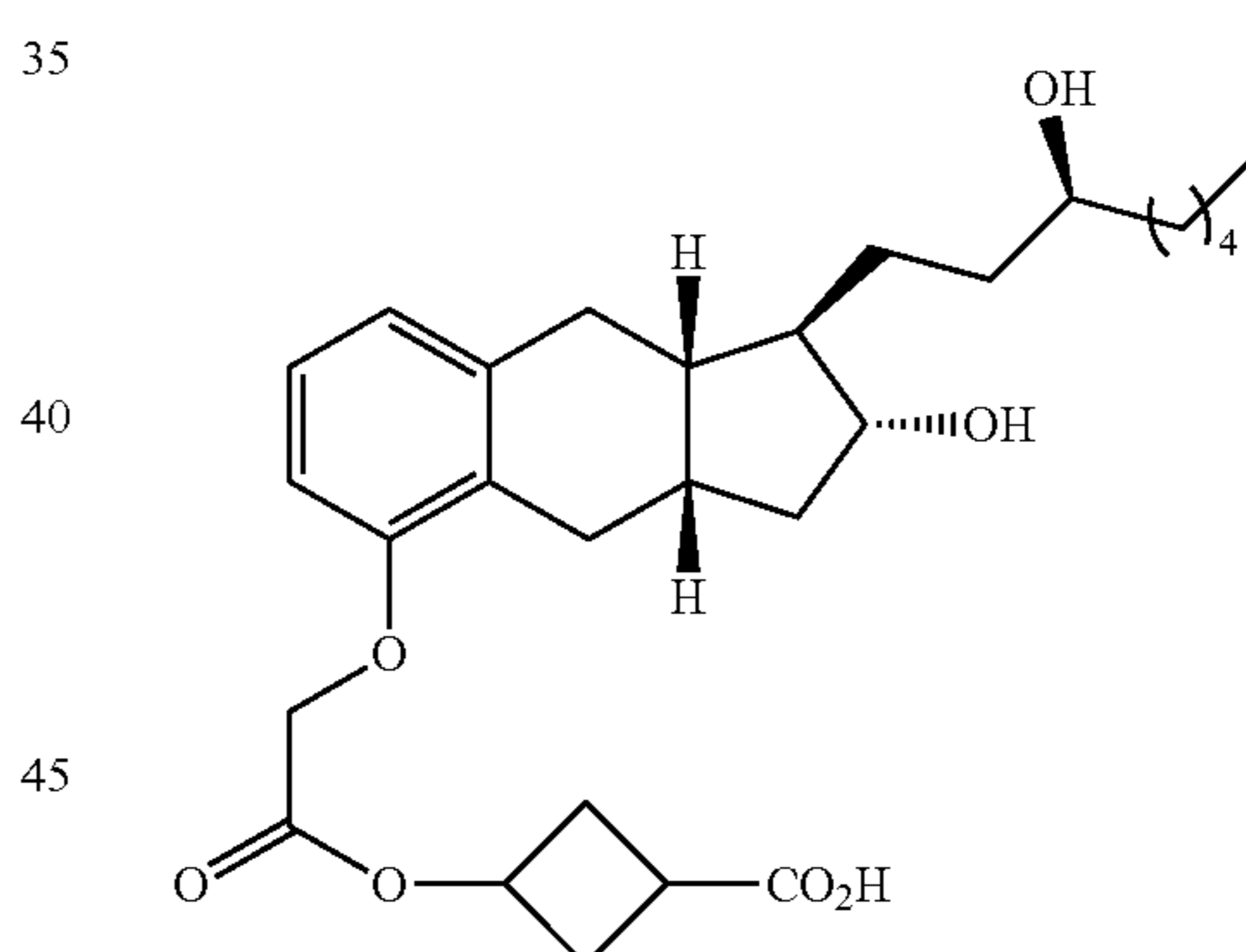
Compound II-20
