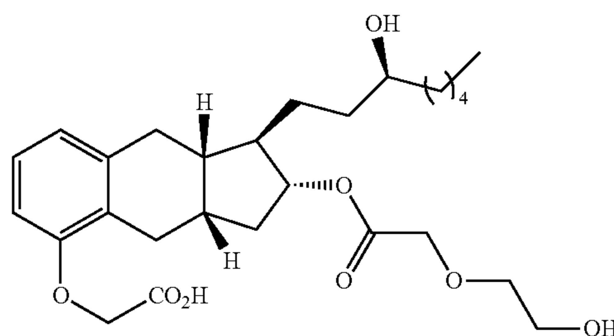
Compound Ia-20
