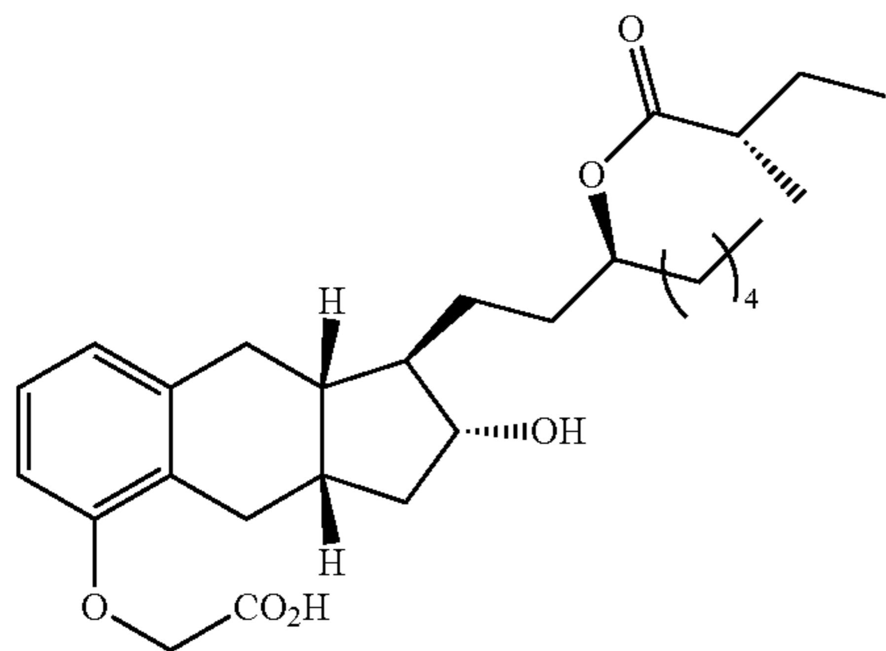
Compound Ib-27
