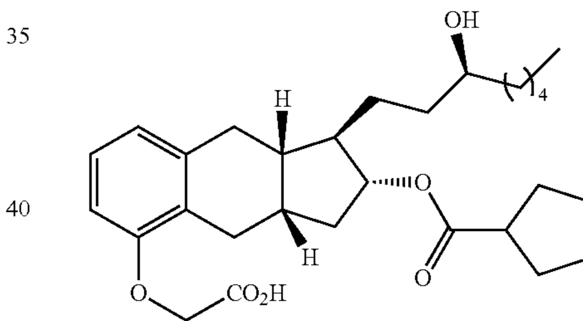
Compound Ia-24
