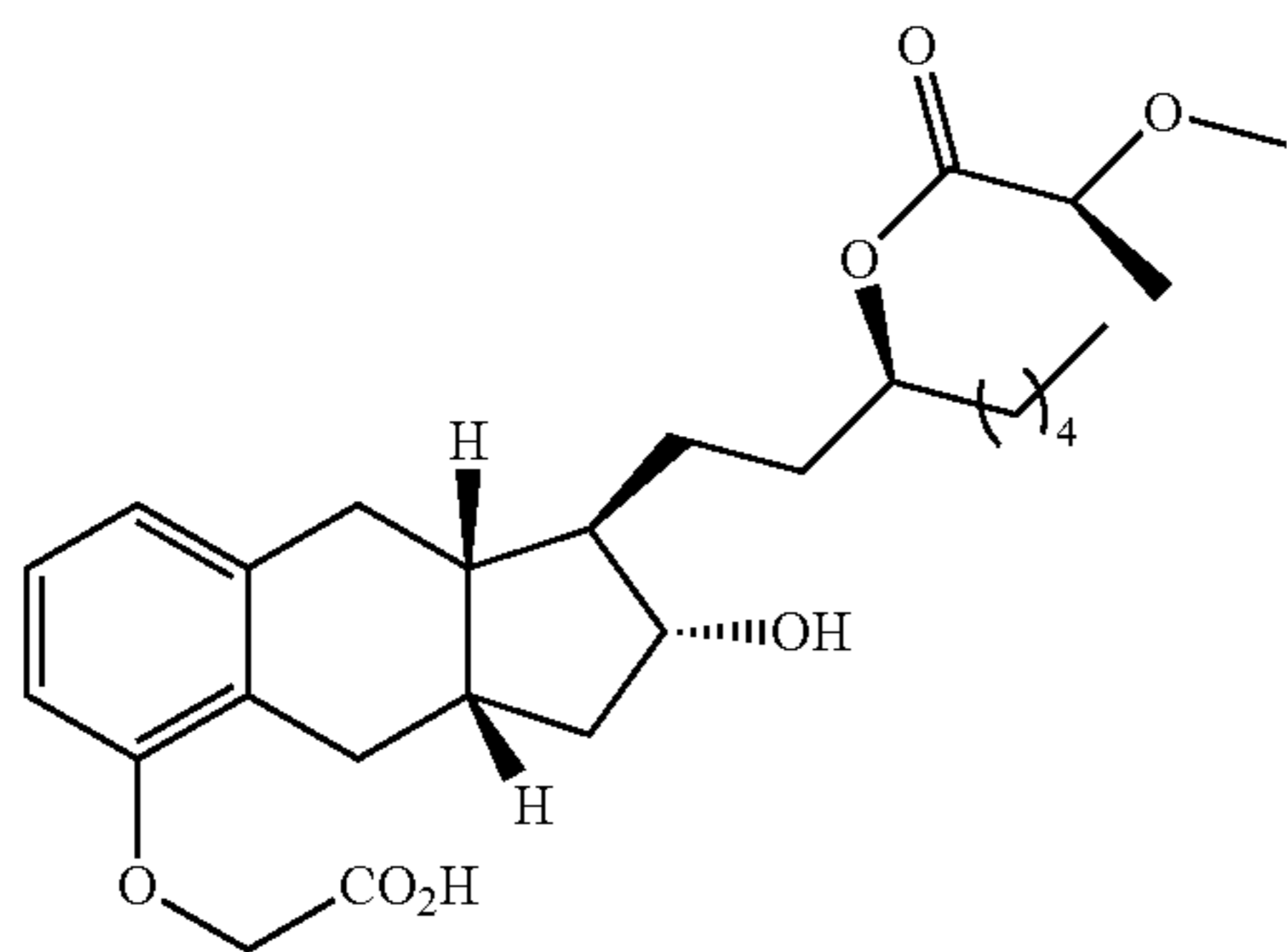
Compound Ib-26
