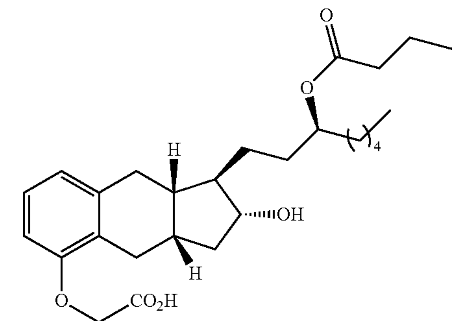
Compound Ib-3
