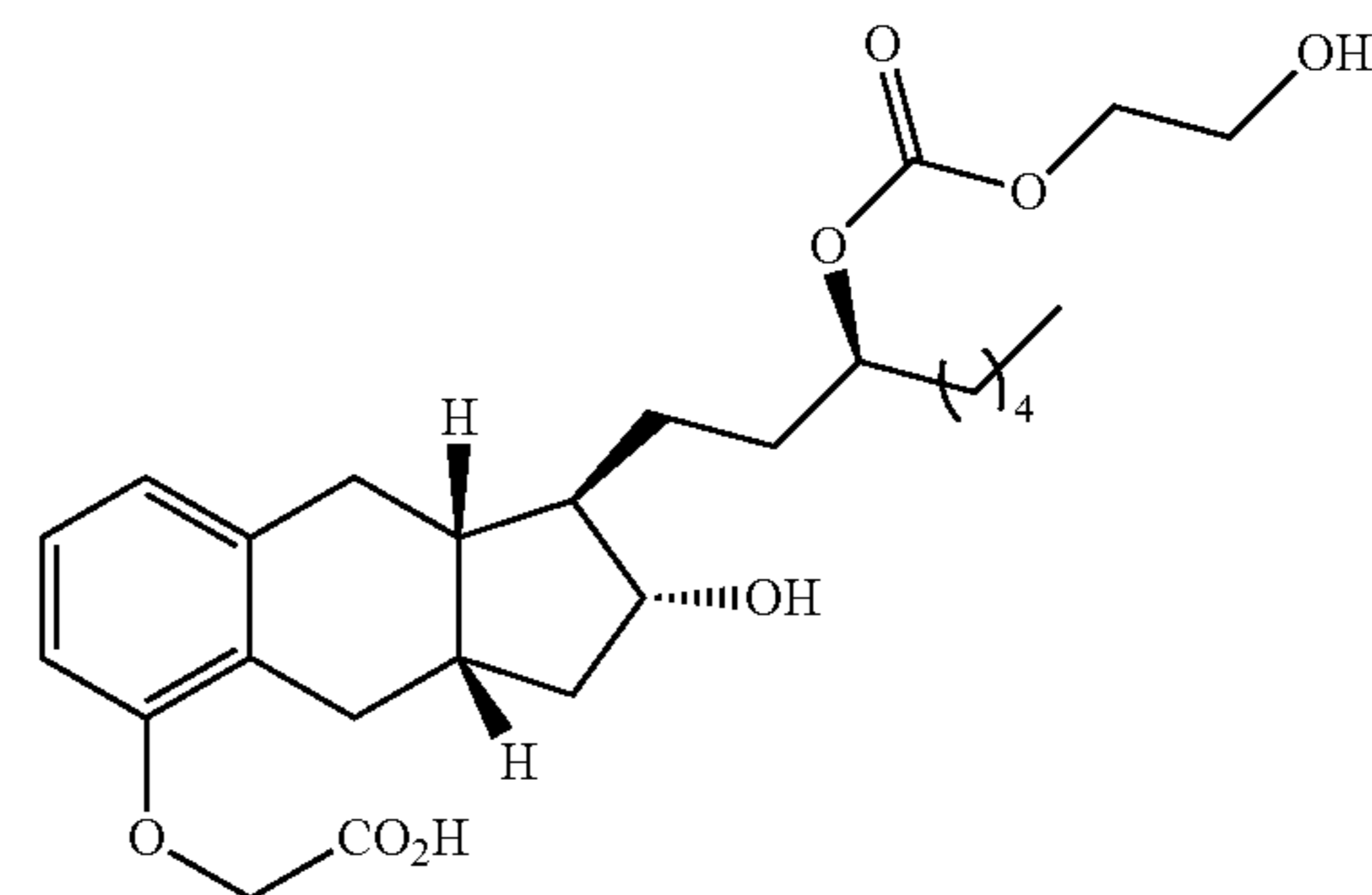
Compound Ib-15
