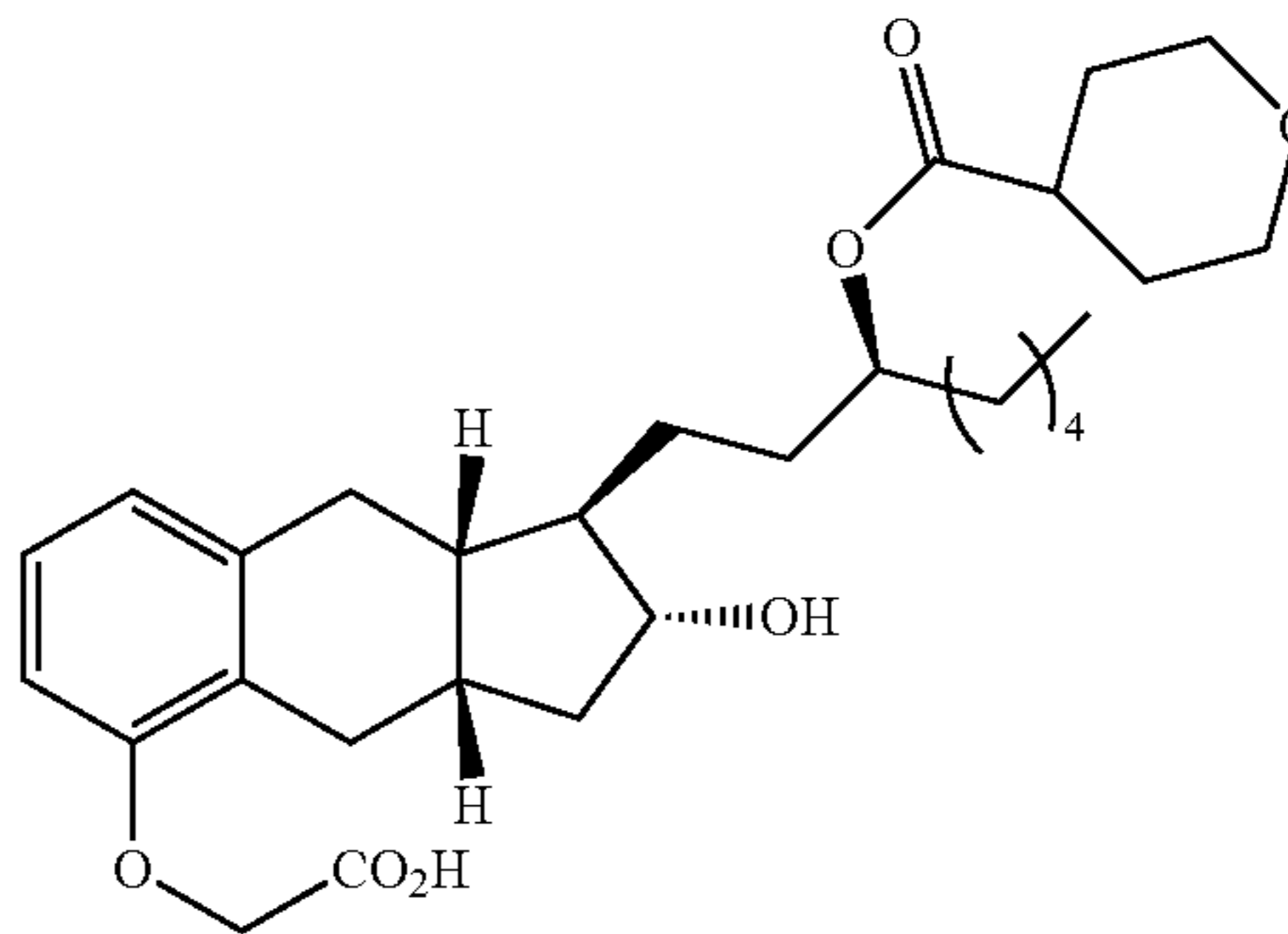
Compound Ib-34
