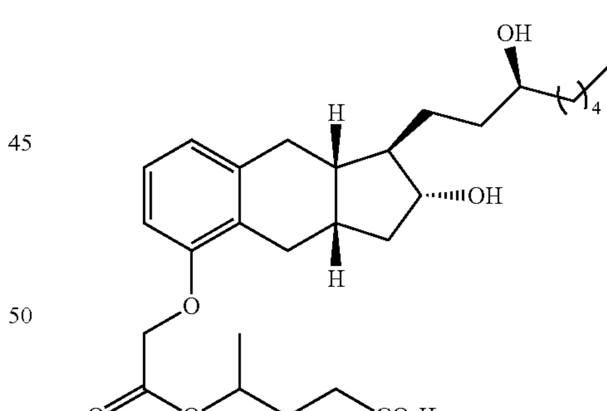
Compound II-6
