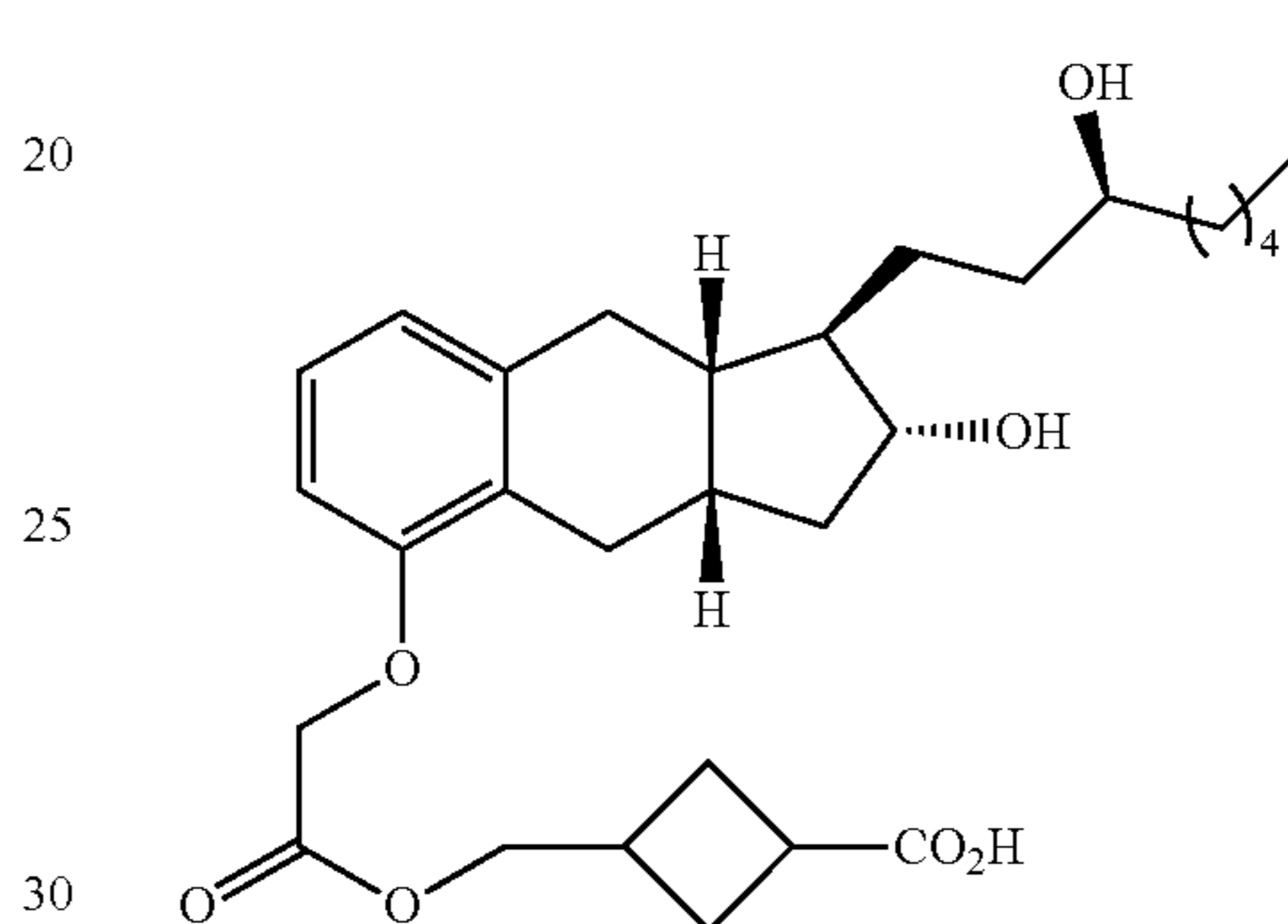
Compound II-19
