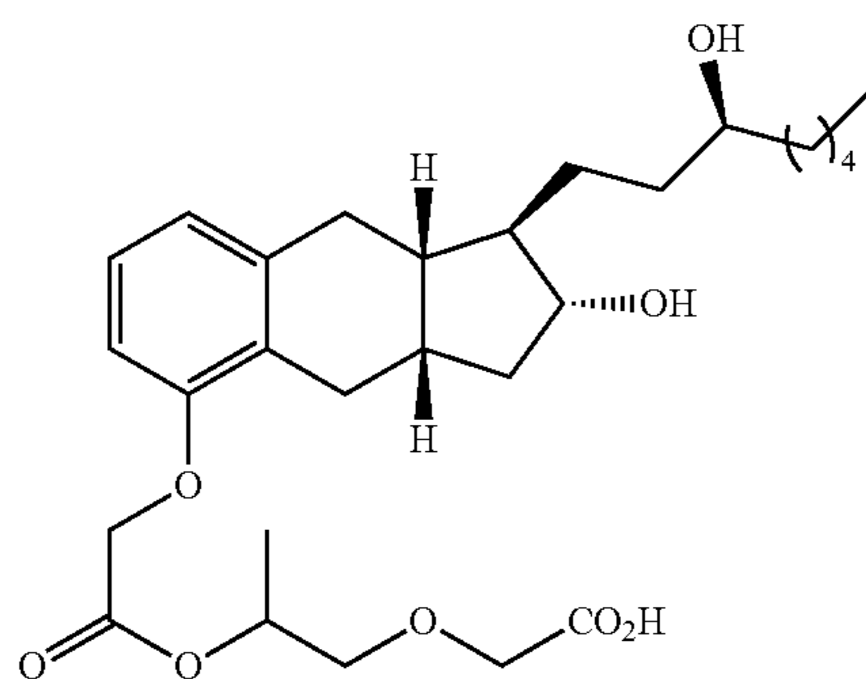
Compound II-9
