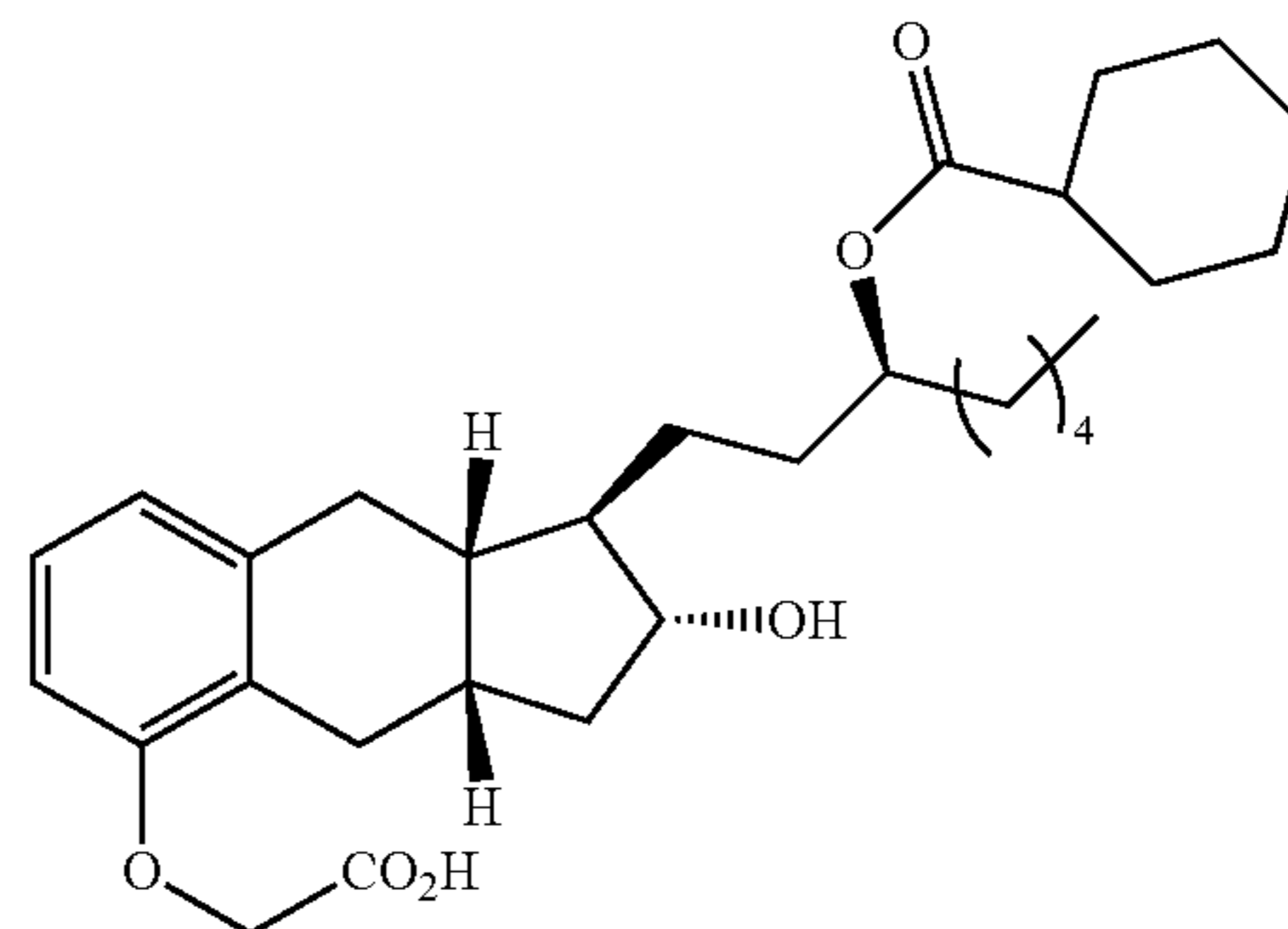
Compound Ib-31
