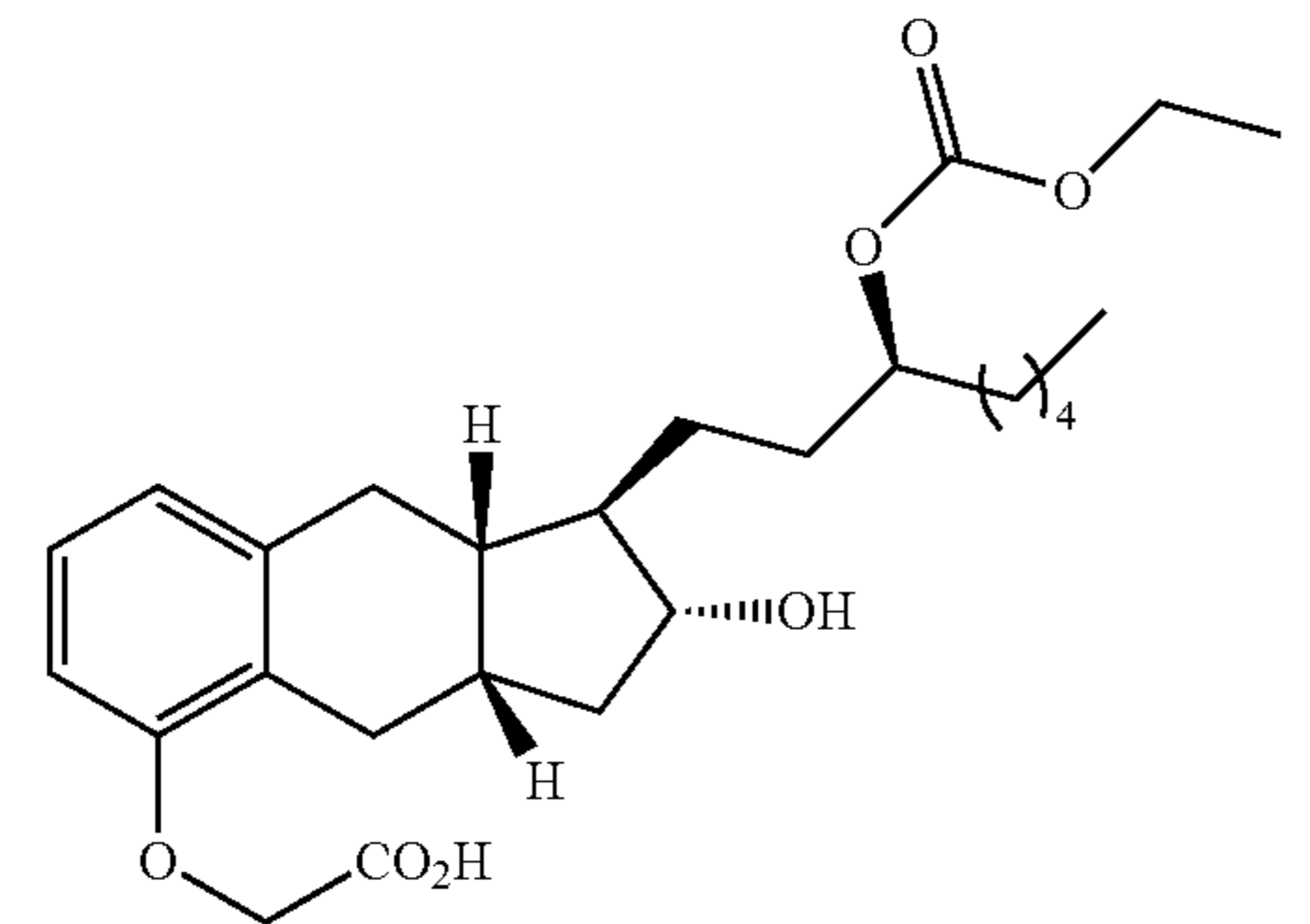
Compound Ib-11
