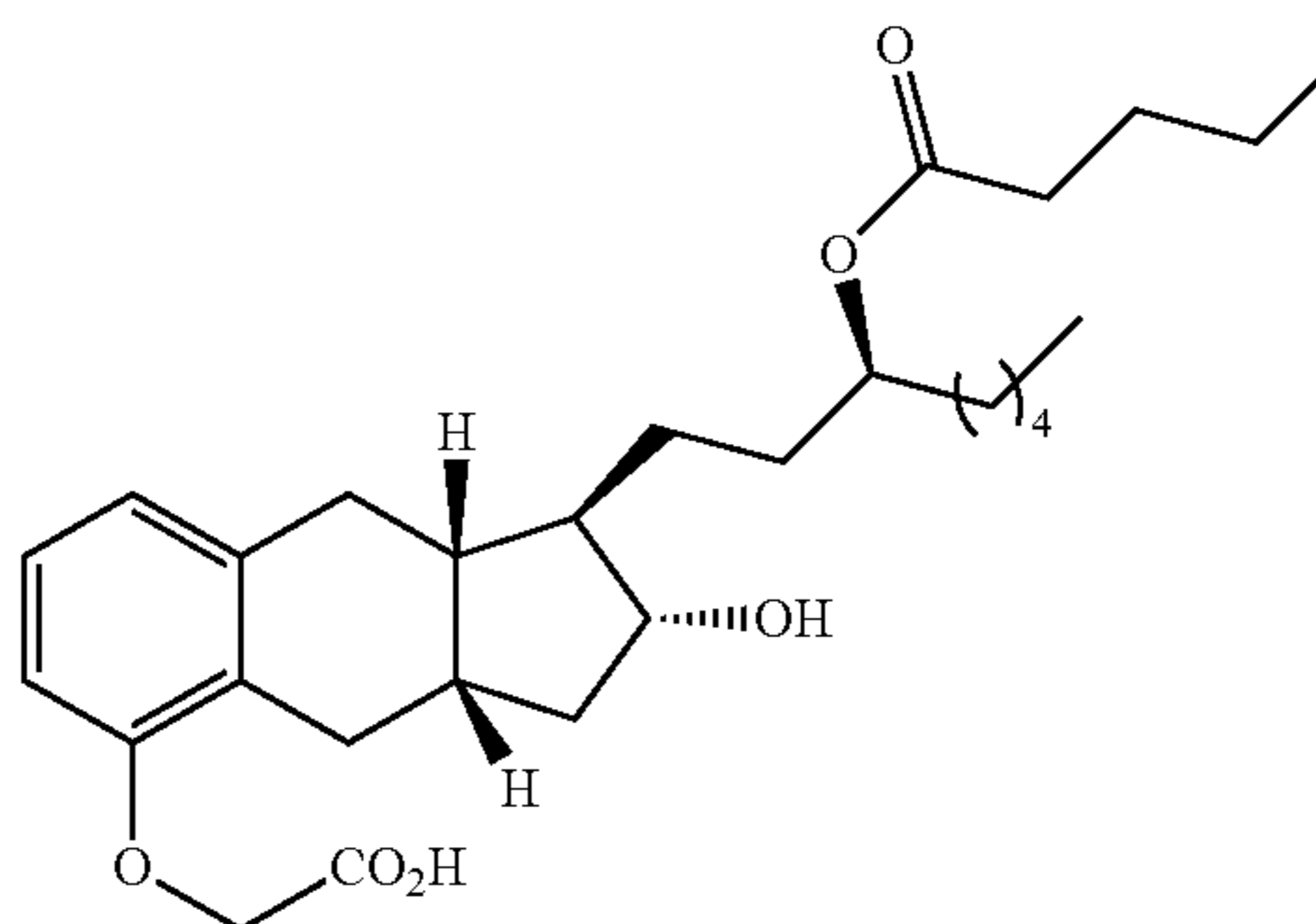
Compound Ib-16
