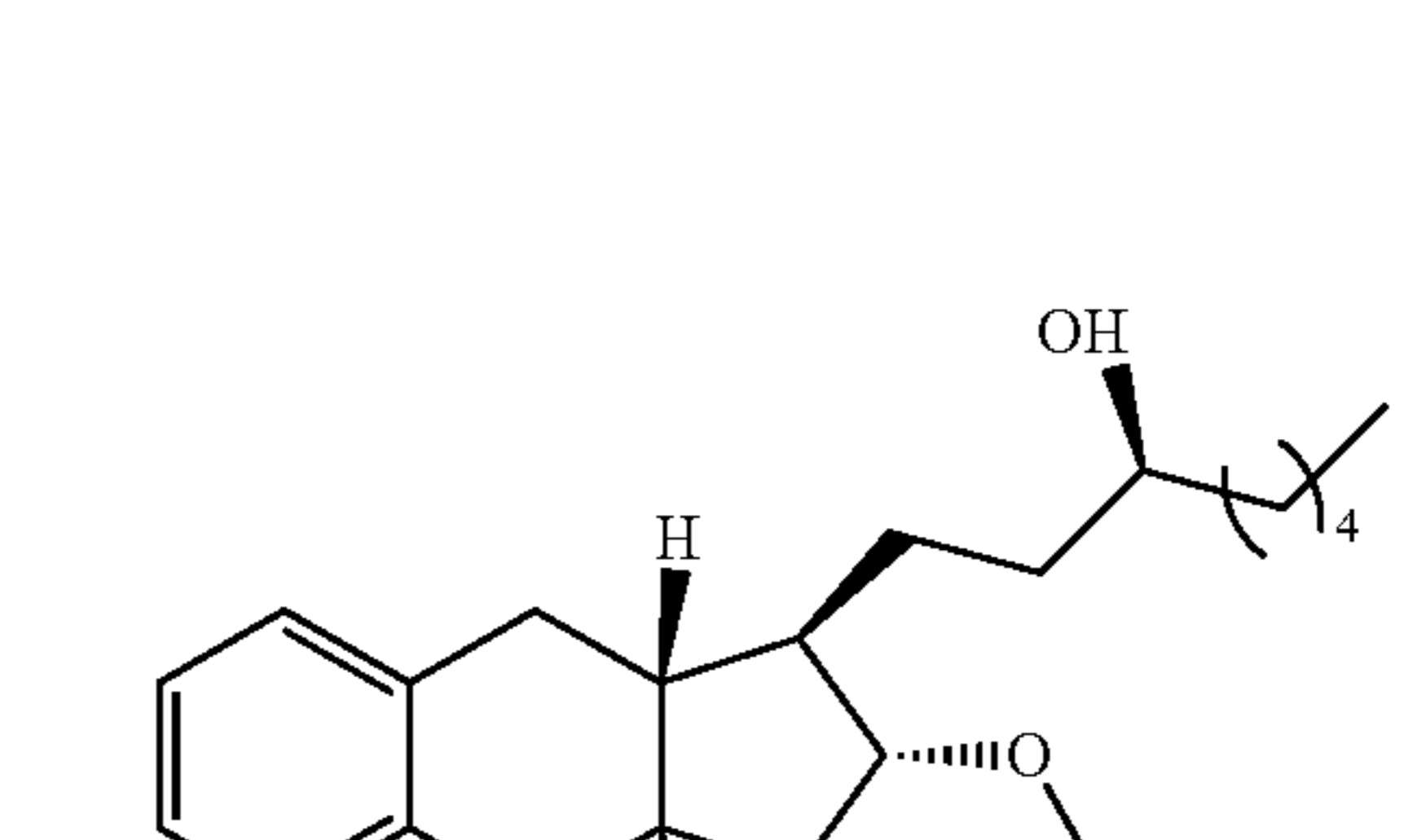
Compound Ia-19
