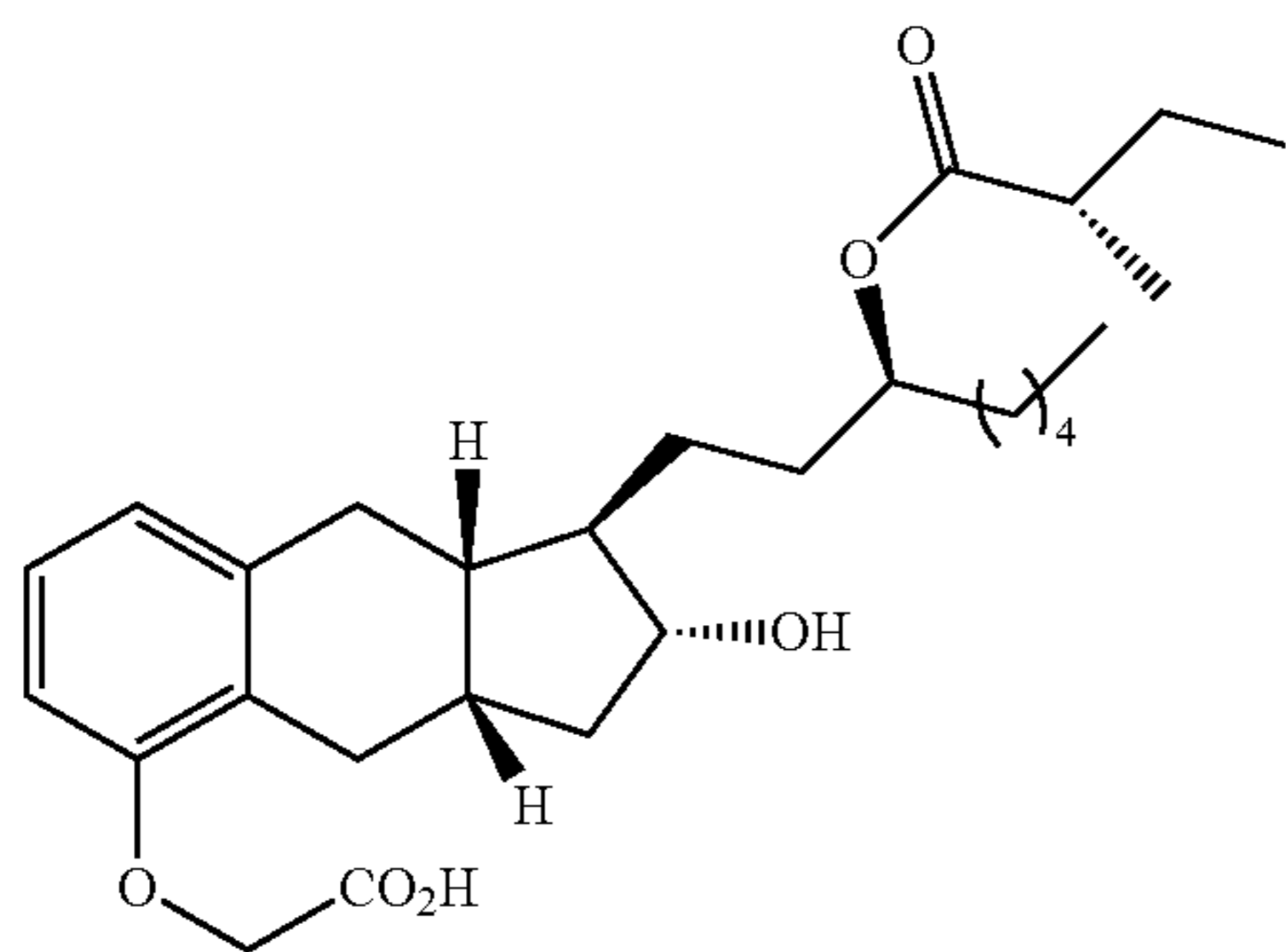
Compound Ib-27
