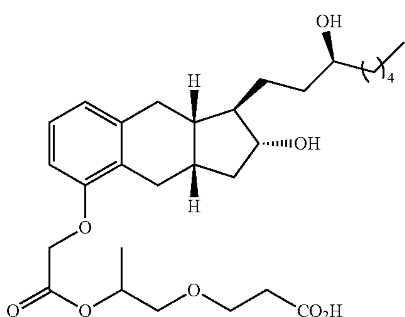
Compound II-16
