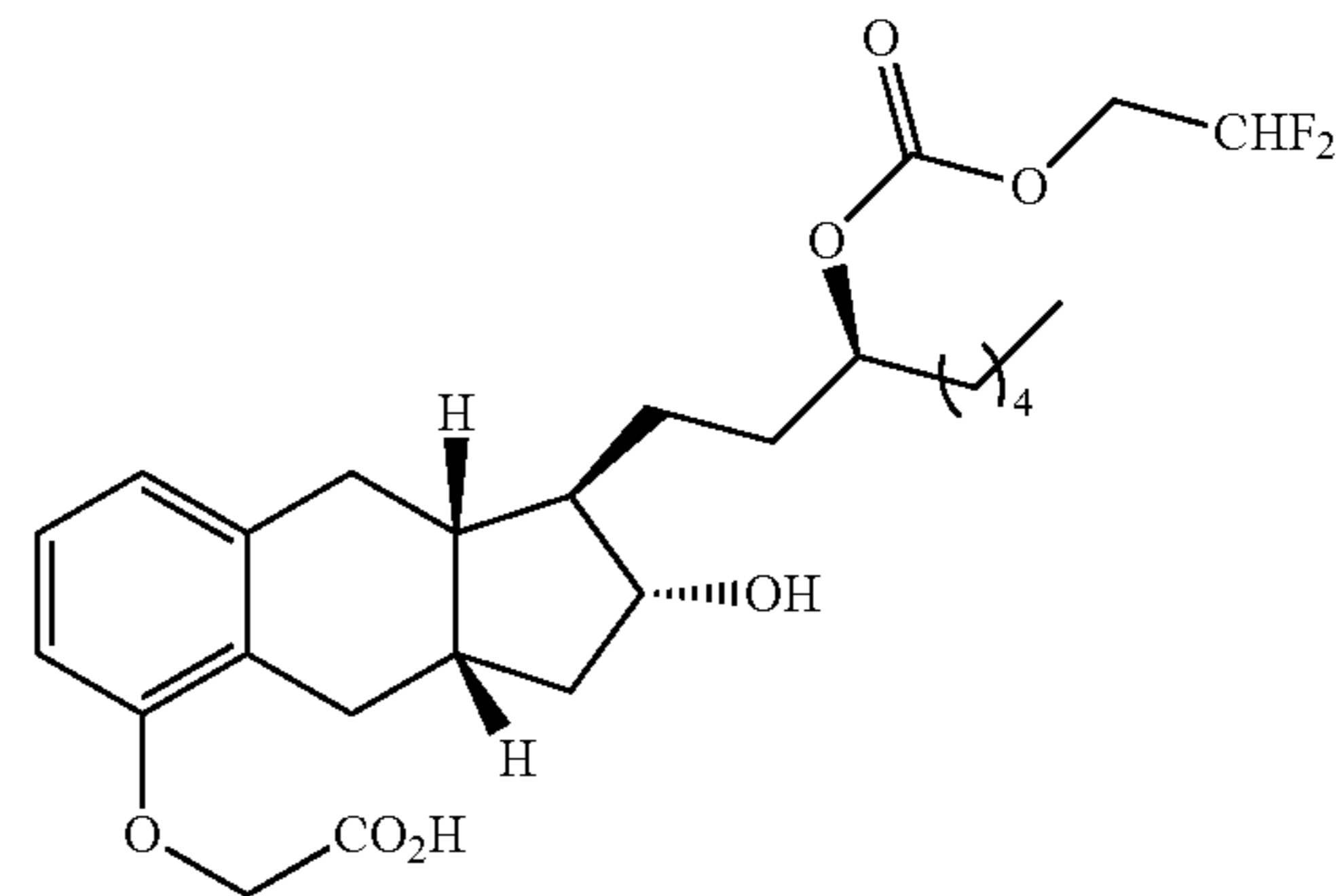
Compound Ib-14
