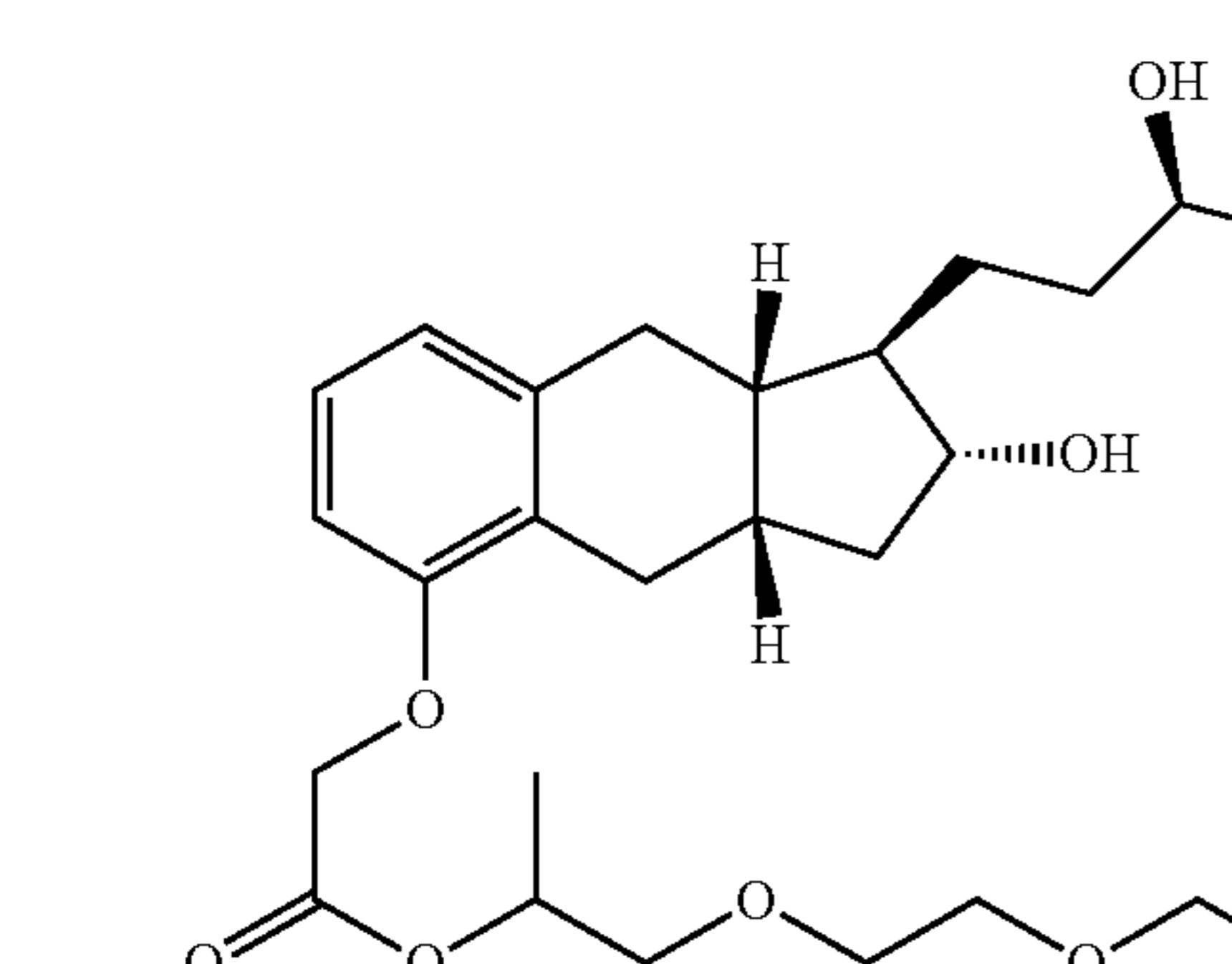
Compound II-18
