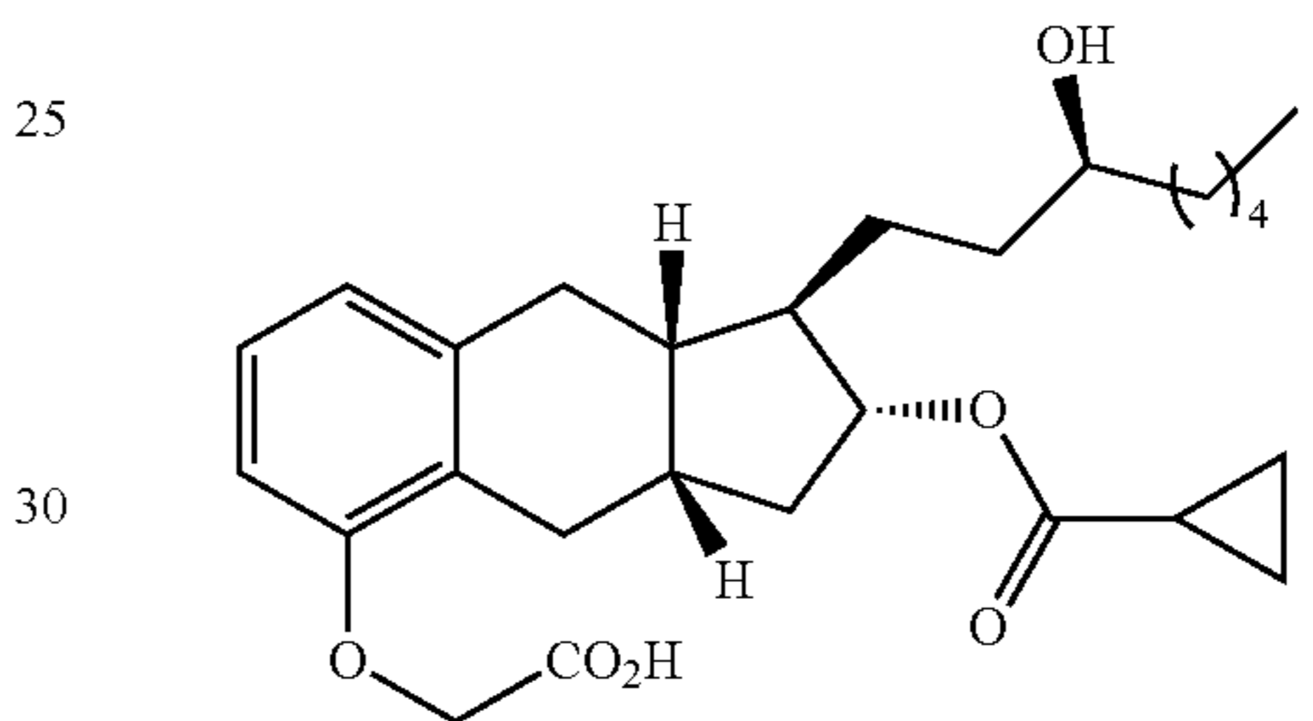
Compound Ia-23
