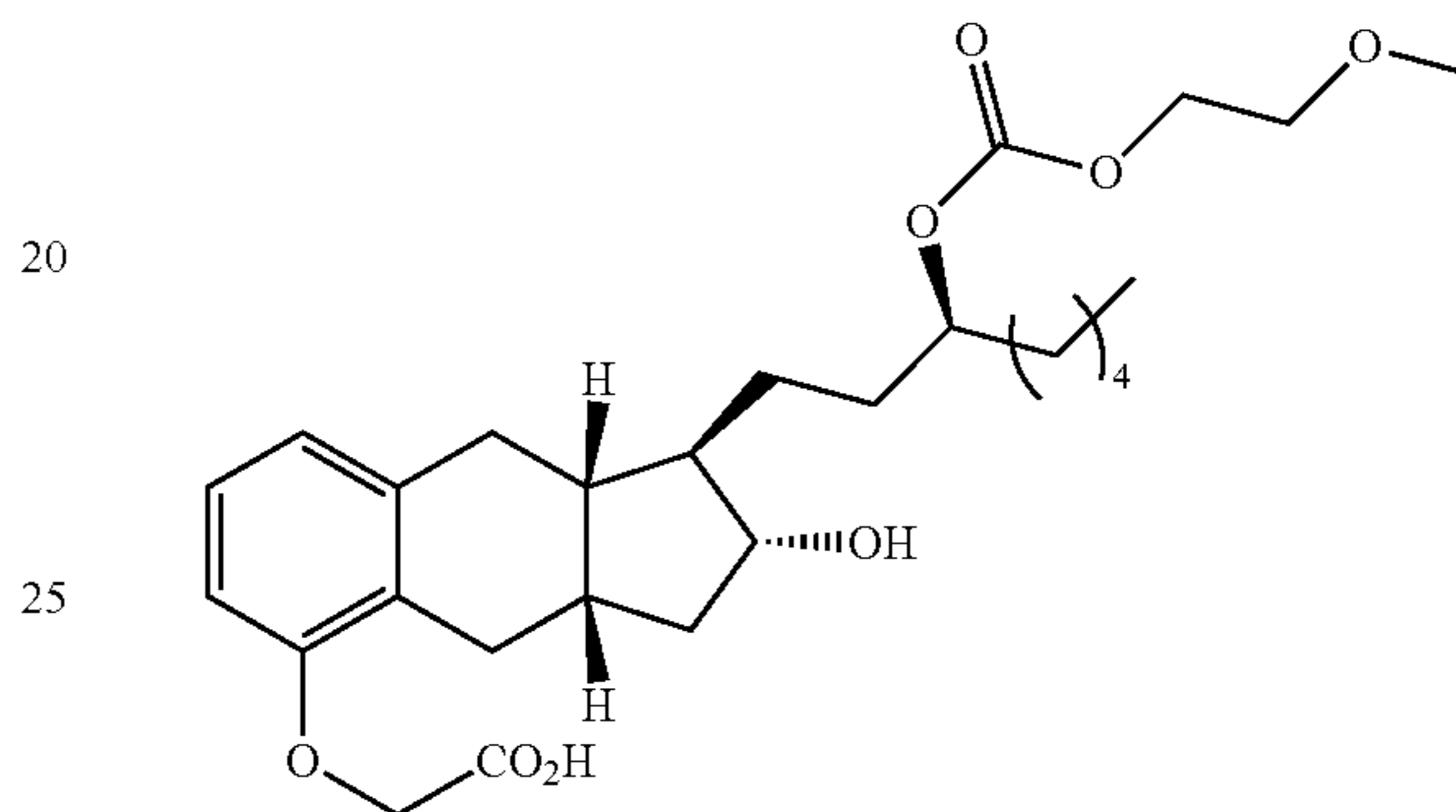
Compound Ib-15
