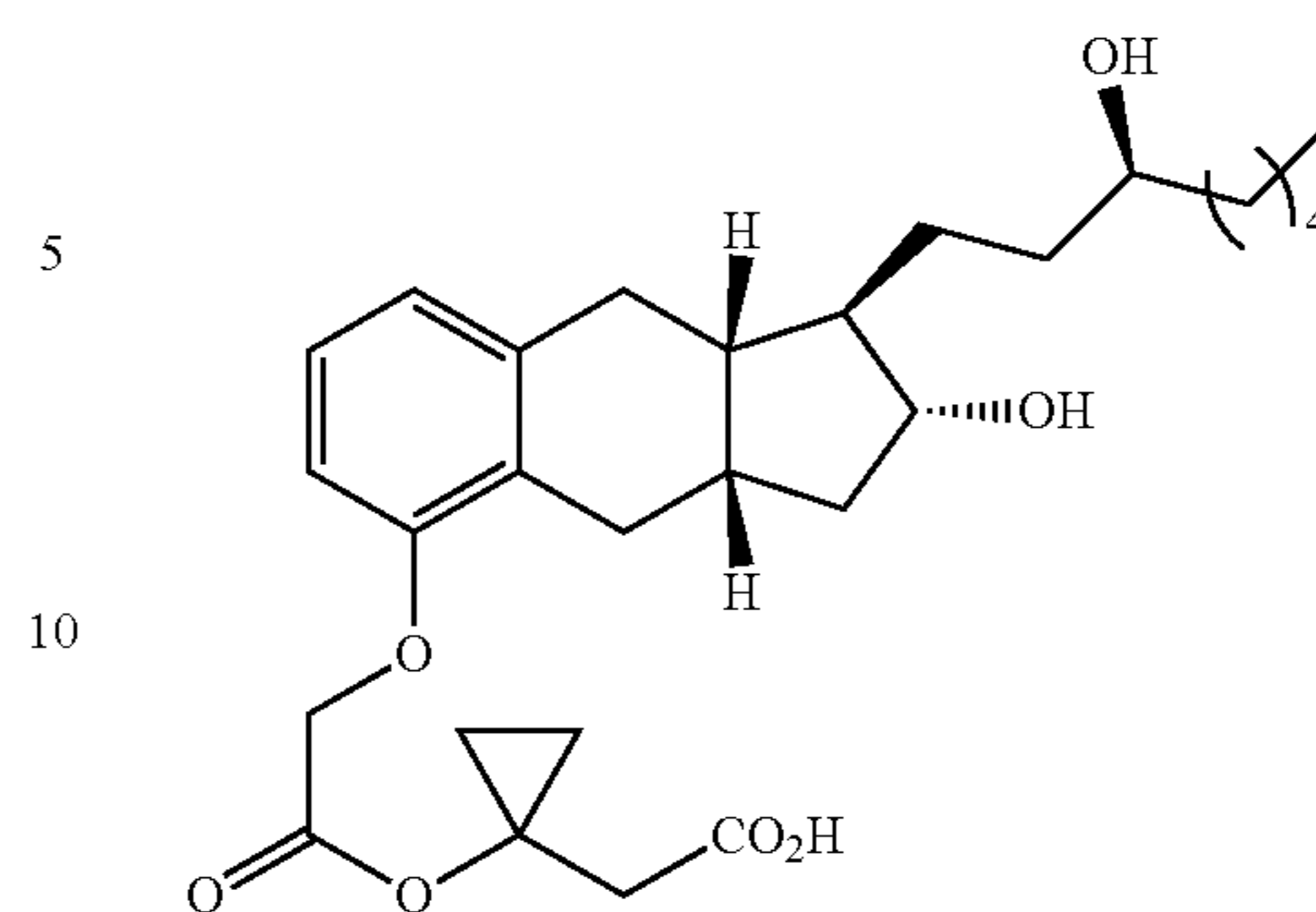
Compound II-24
