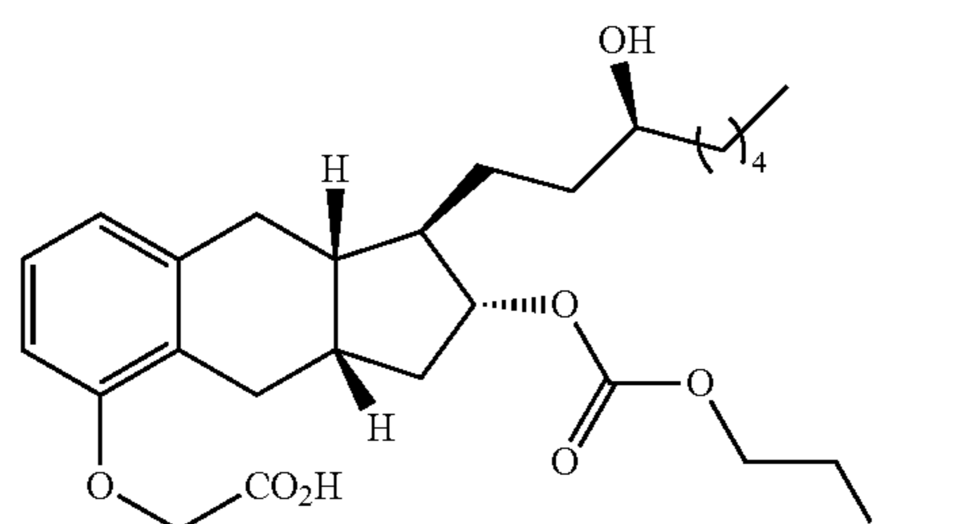
Compound Ib-1
