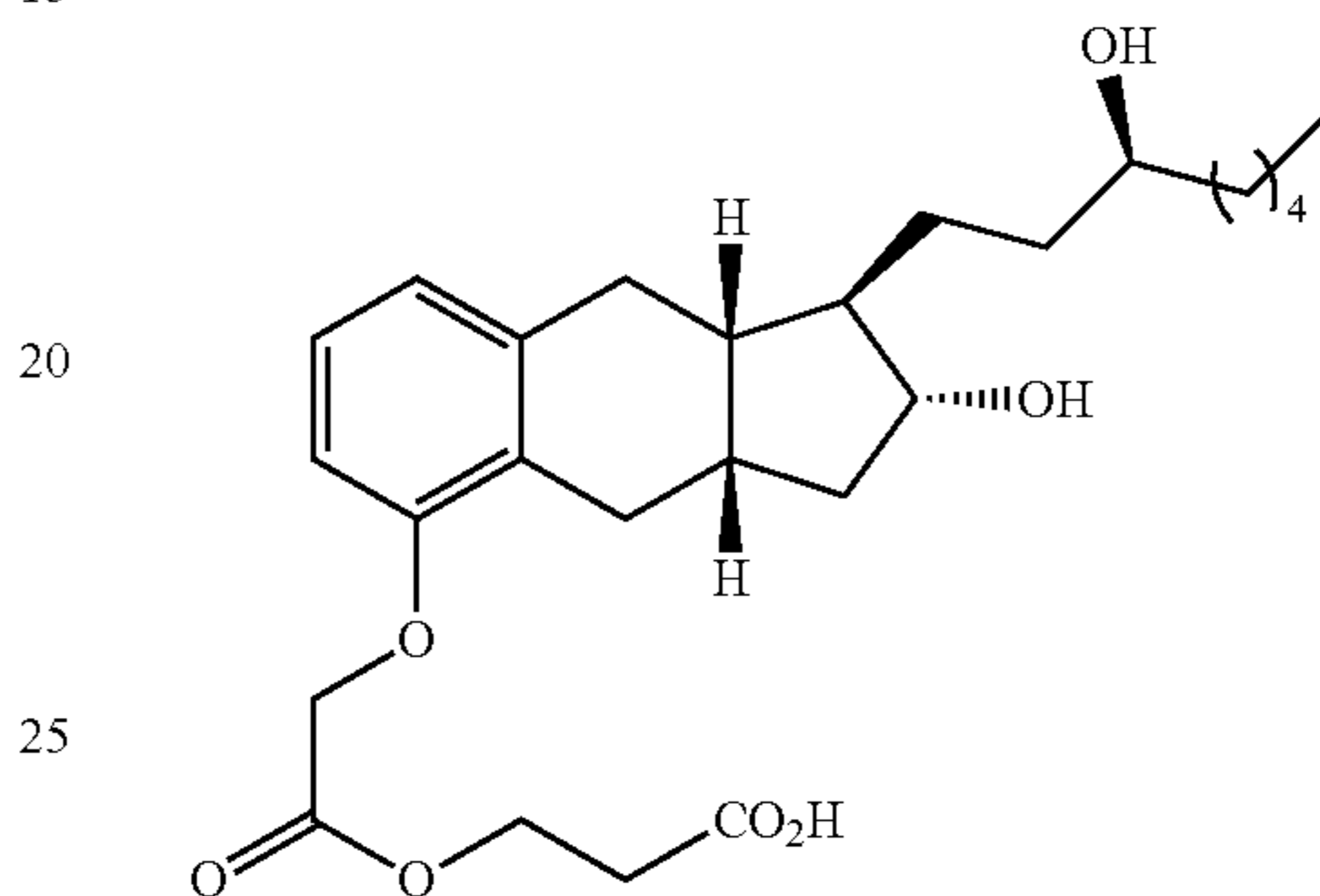
Compound II-15
