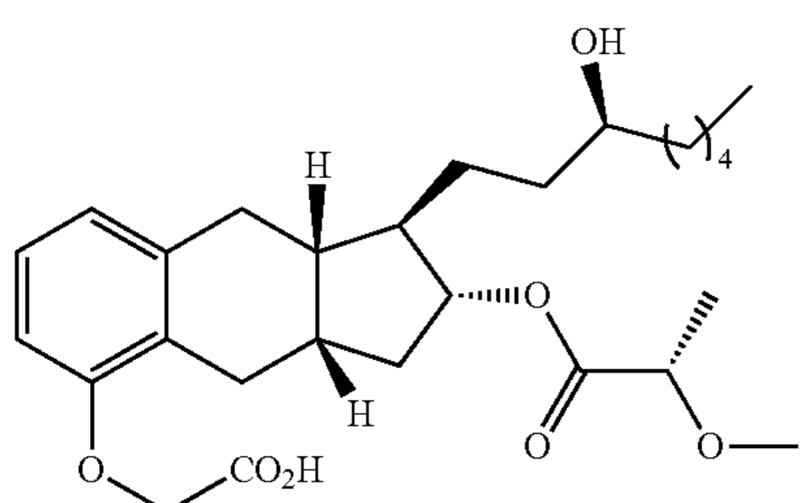
Compound Ia-26
