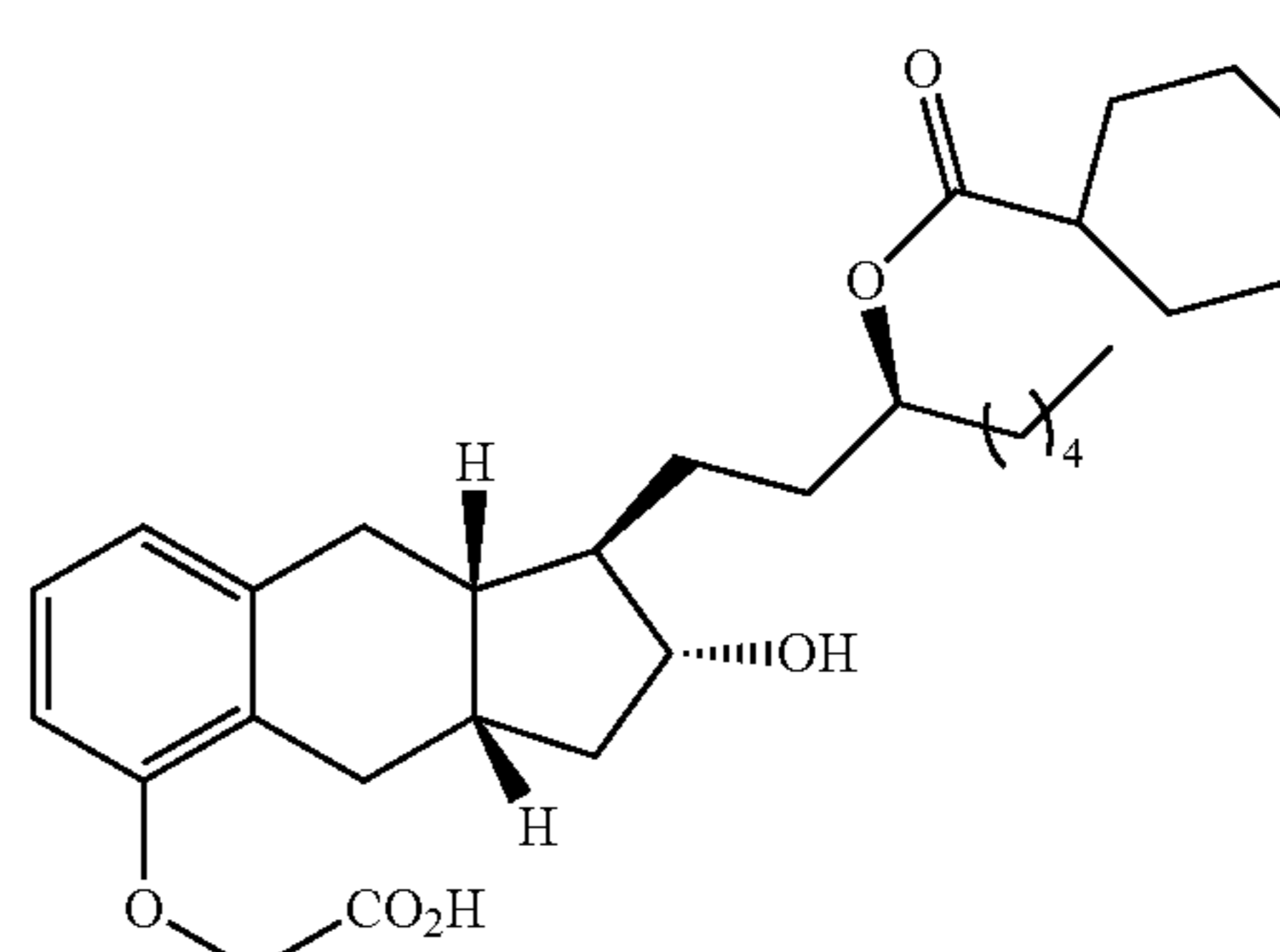
Compound Ib-31
