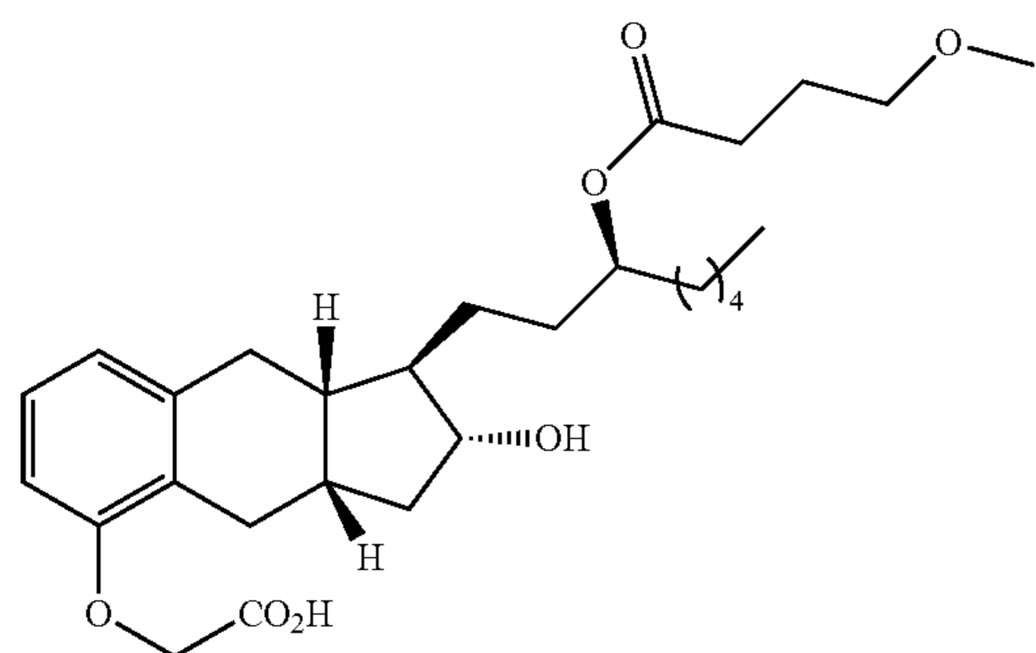
Compound Ib-19
