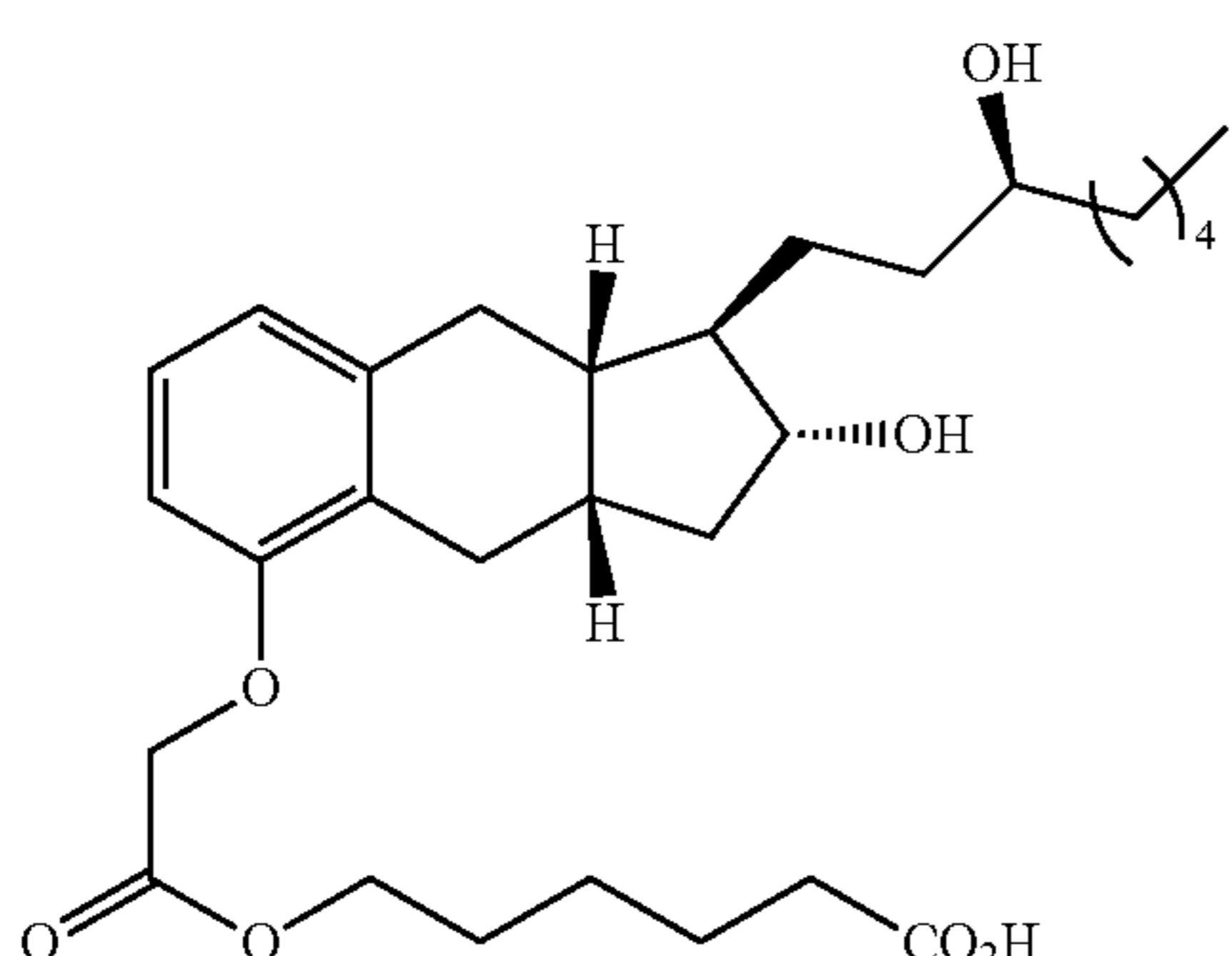
Compound II-9
