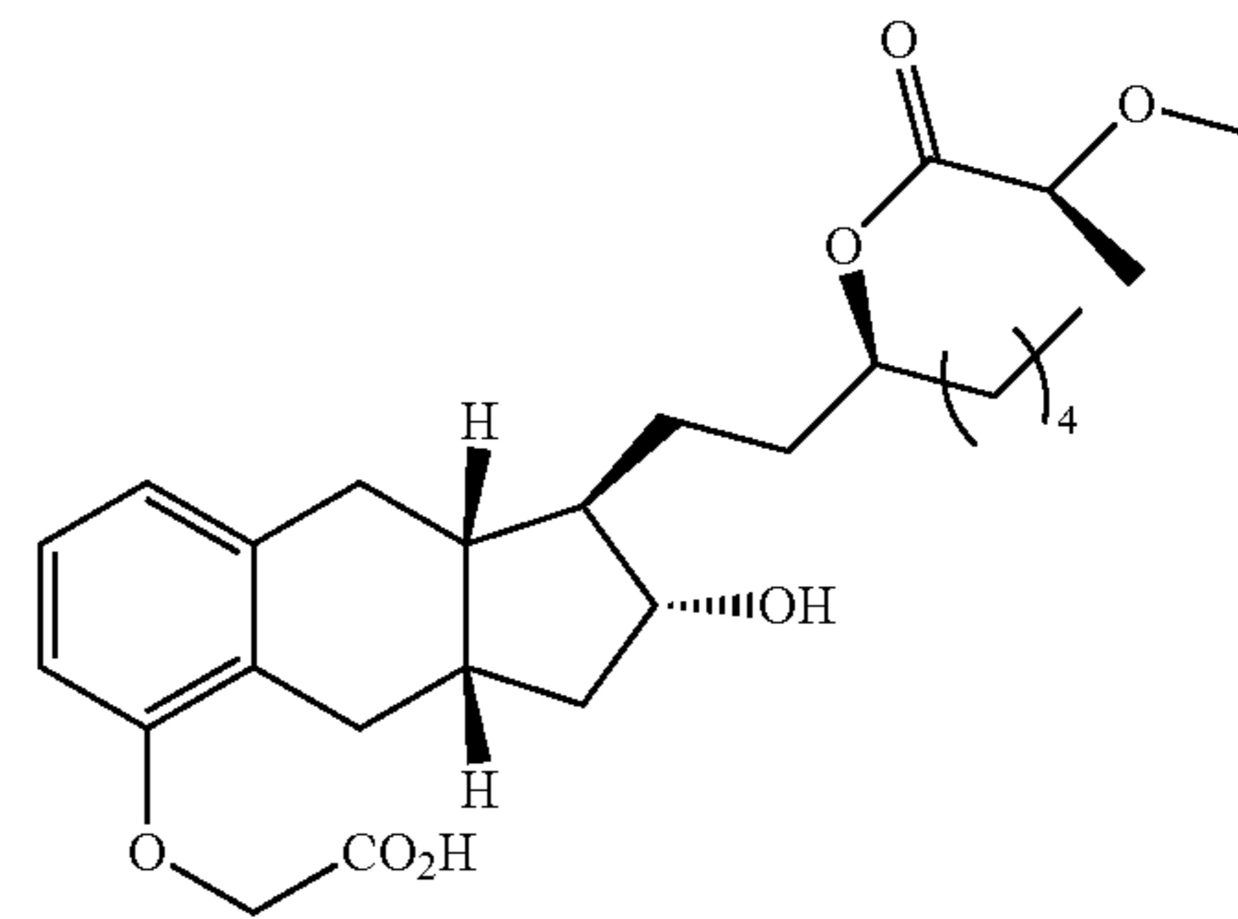
Compound Ib-26
