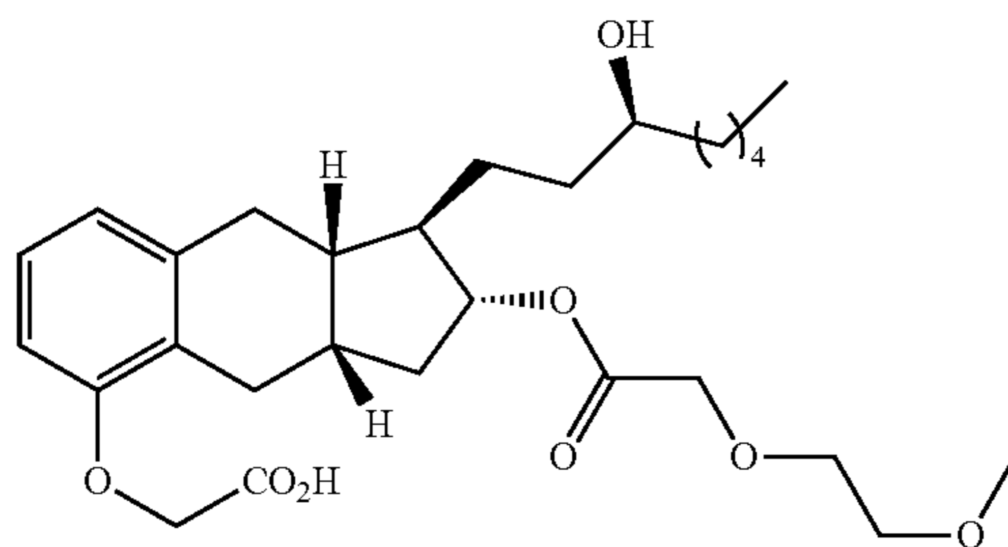
Compound Ia-21
