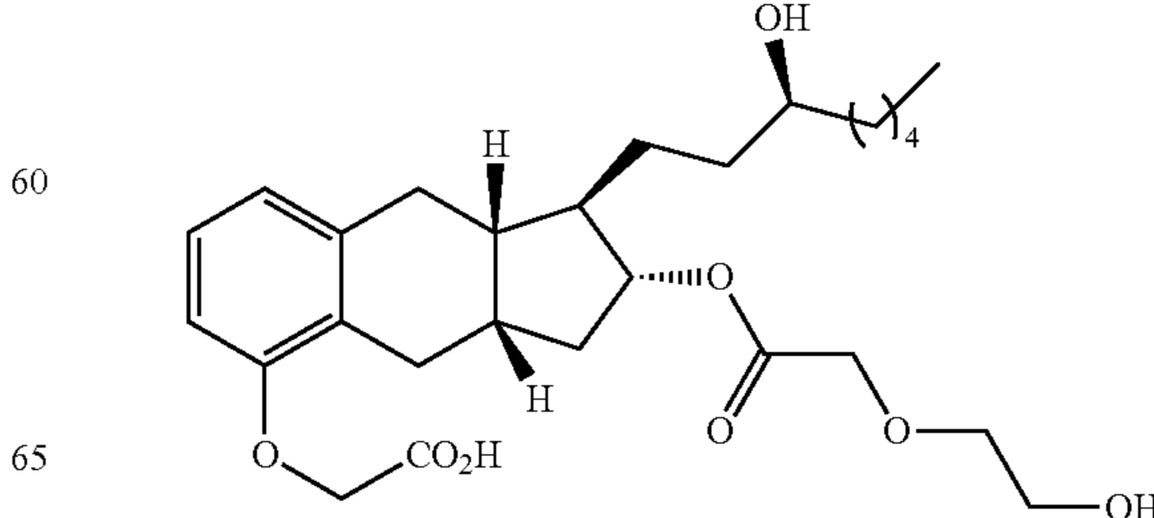
Compound 1a-20
