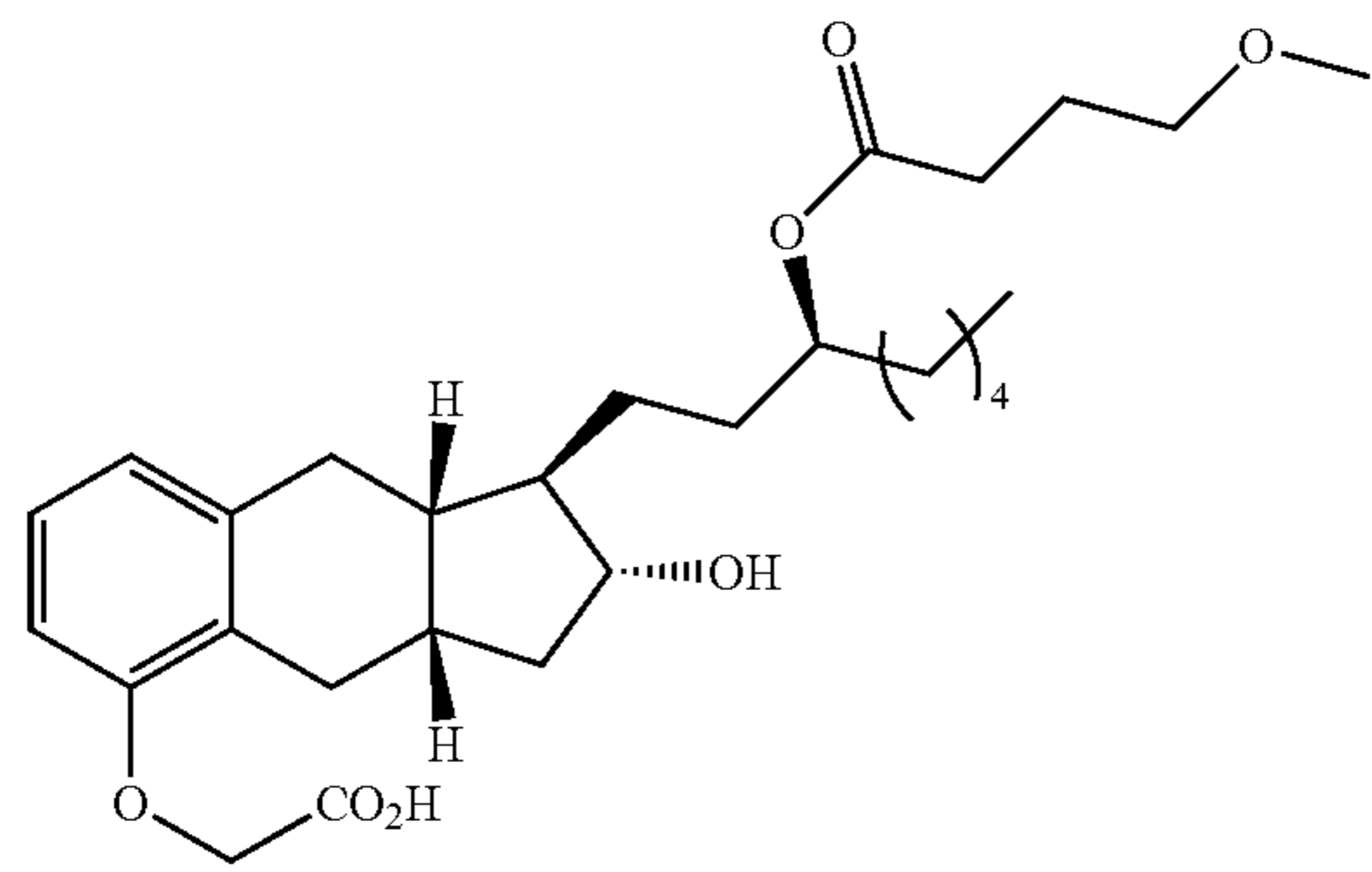
Compound Ib-19
