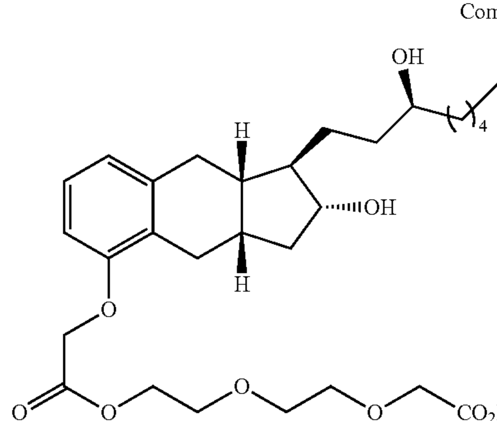
Compound II-17
