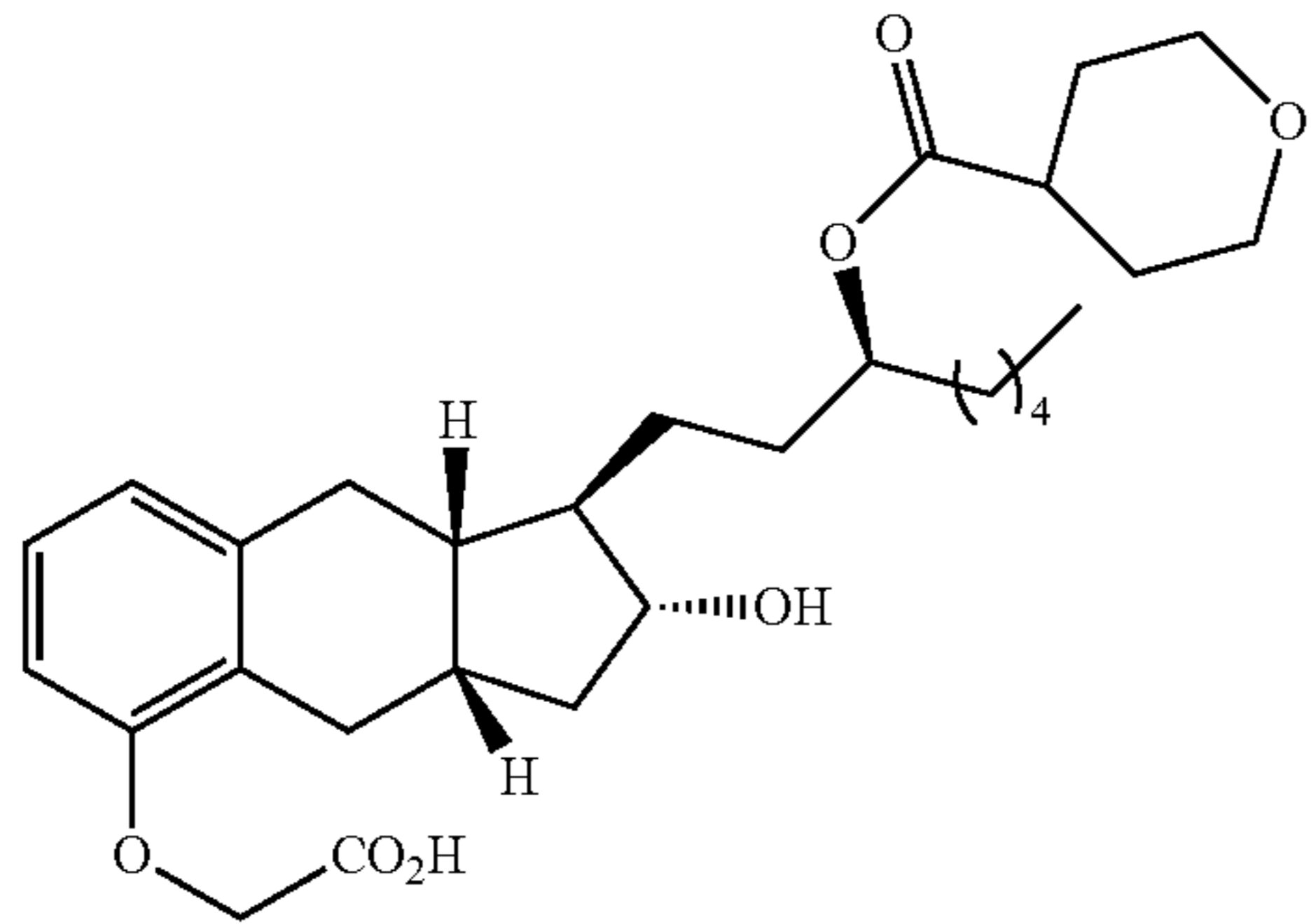
Compound Ib-34
