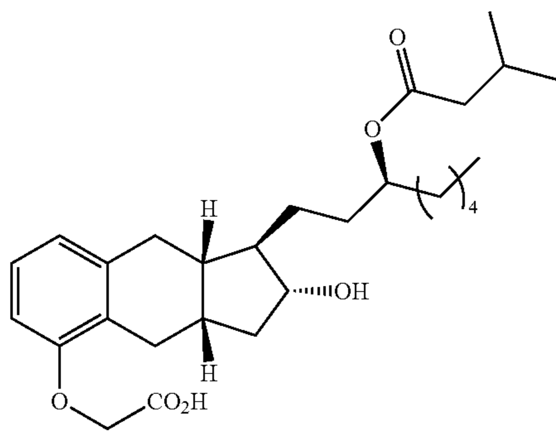
Compound Ib-4
