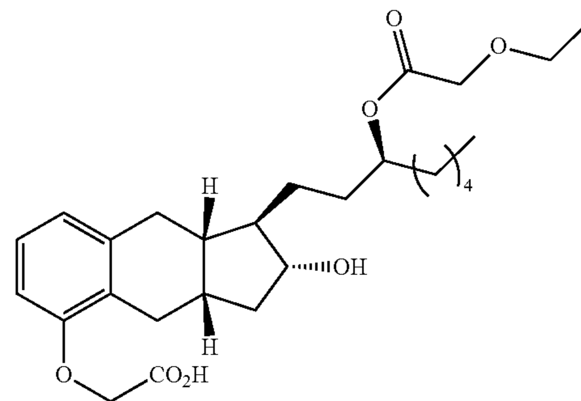
Compound Ib-9
