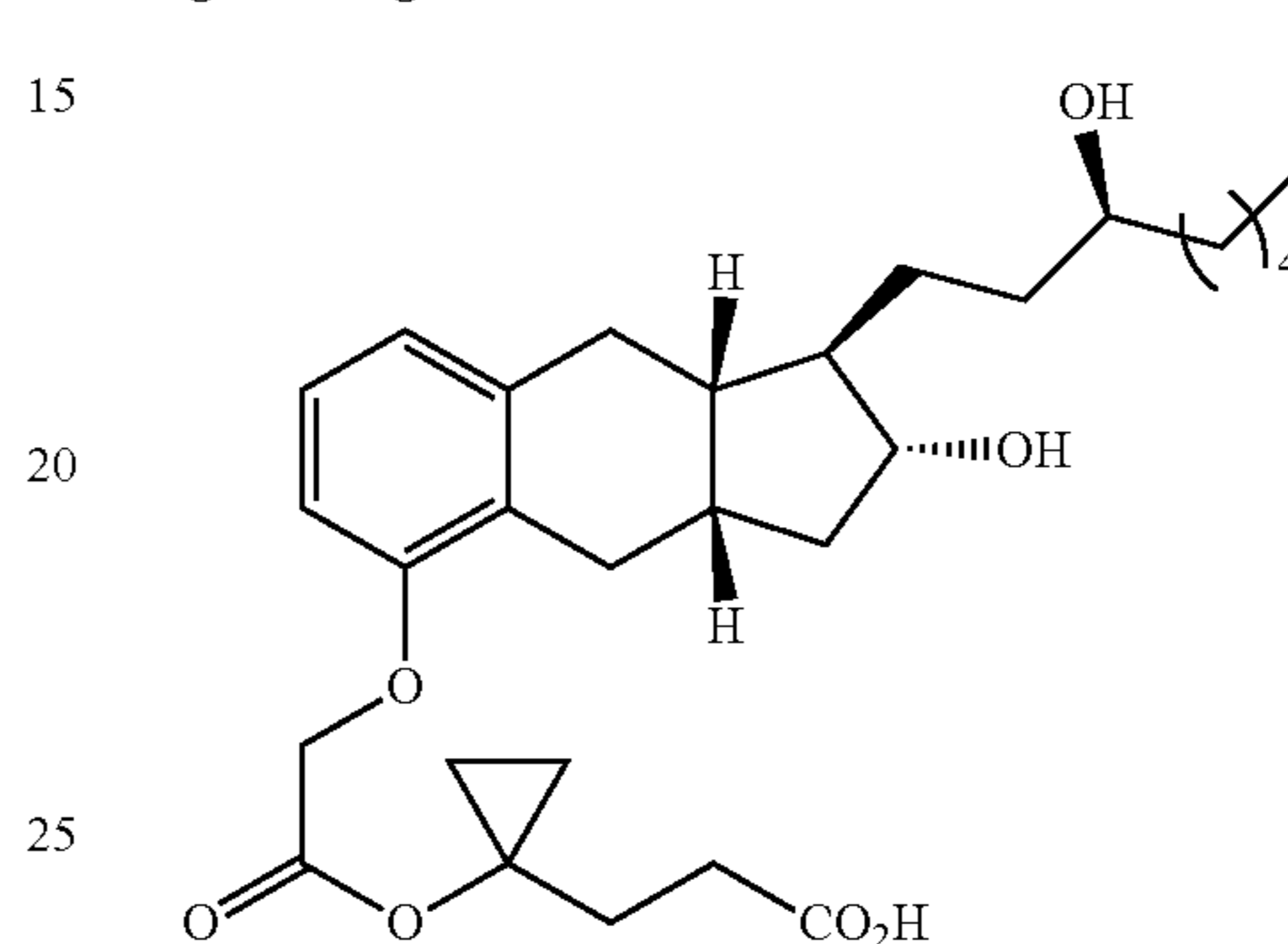
Compound II-25
