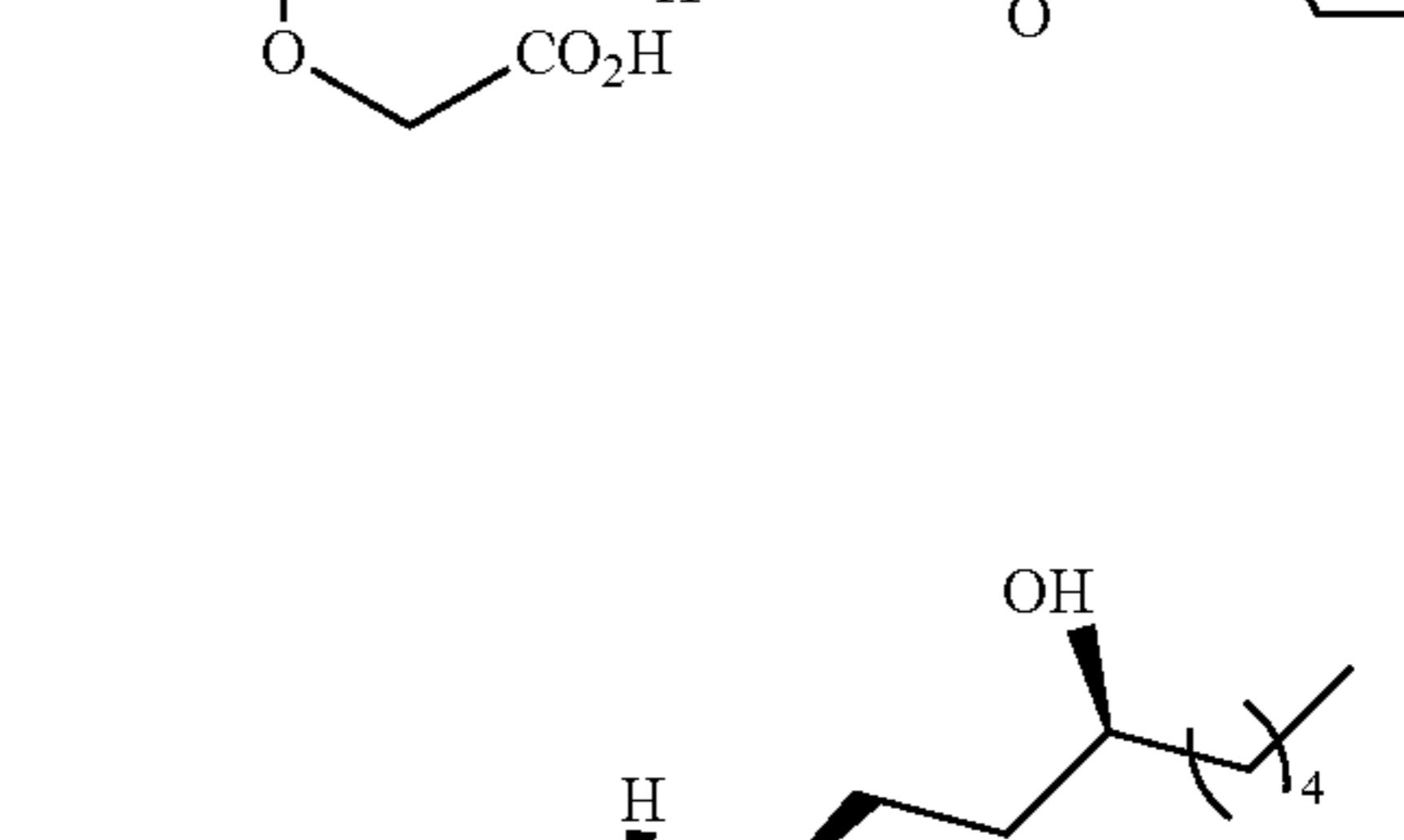
Compound Ia-20
