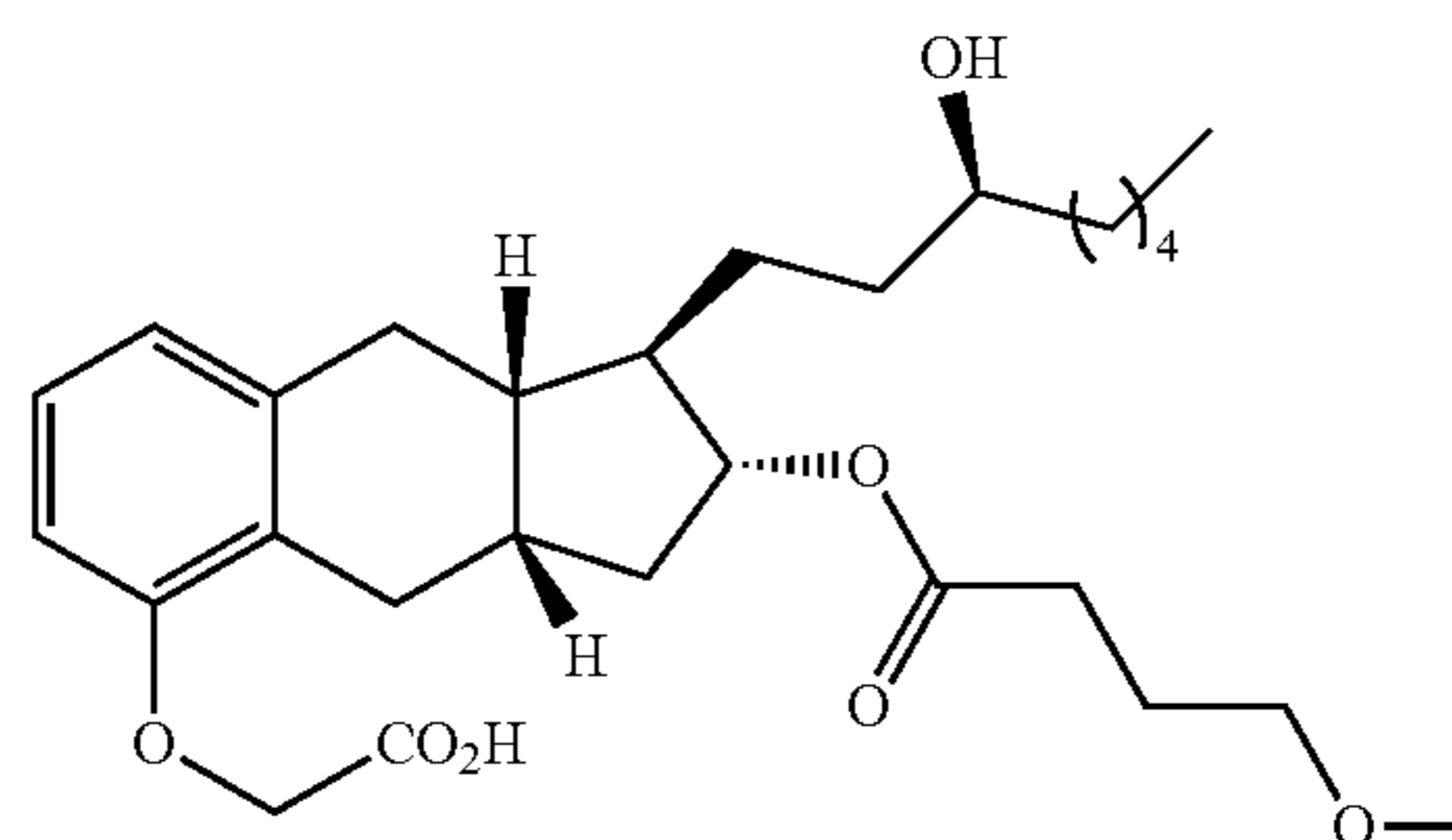
Compound Ia-19
