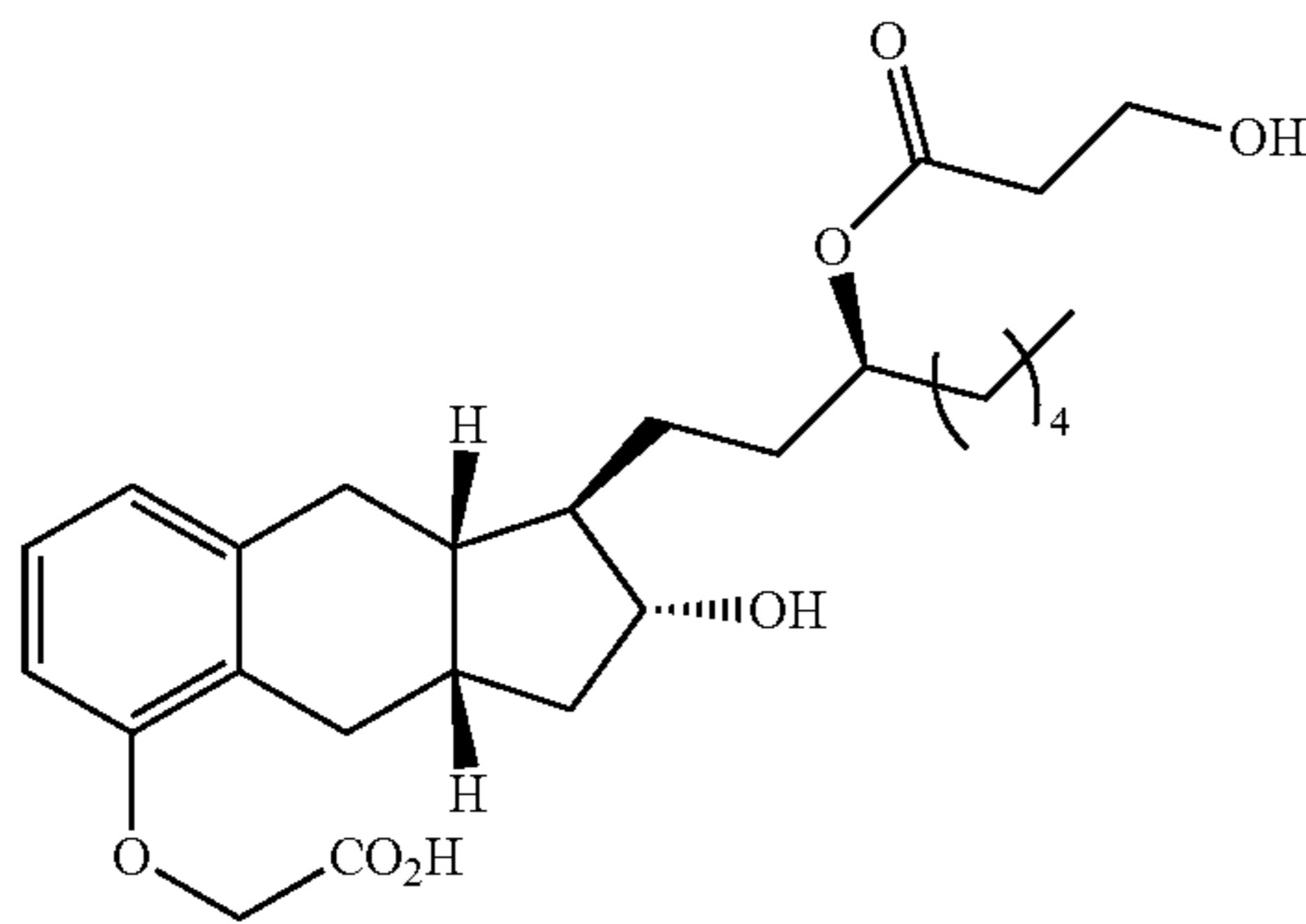
Compound Ib-5
