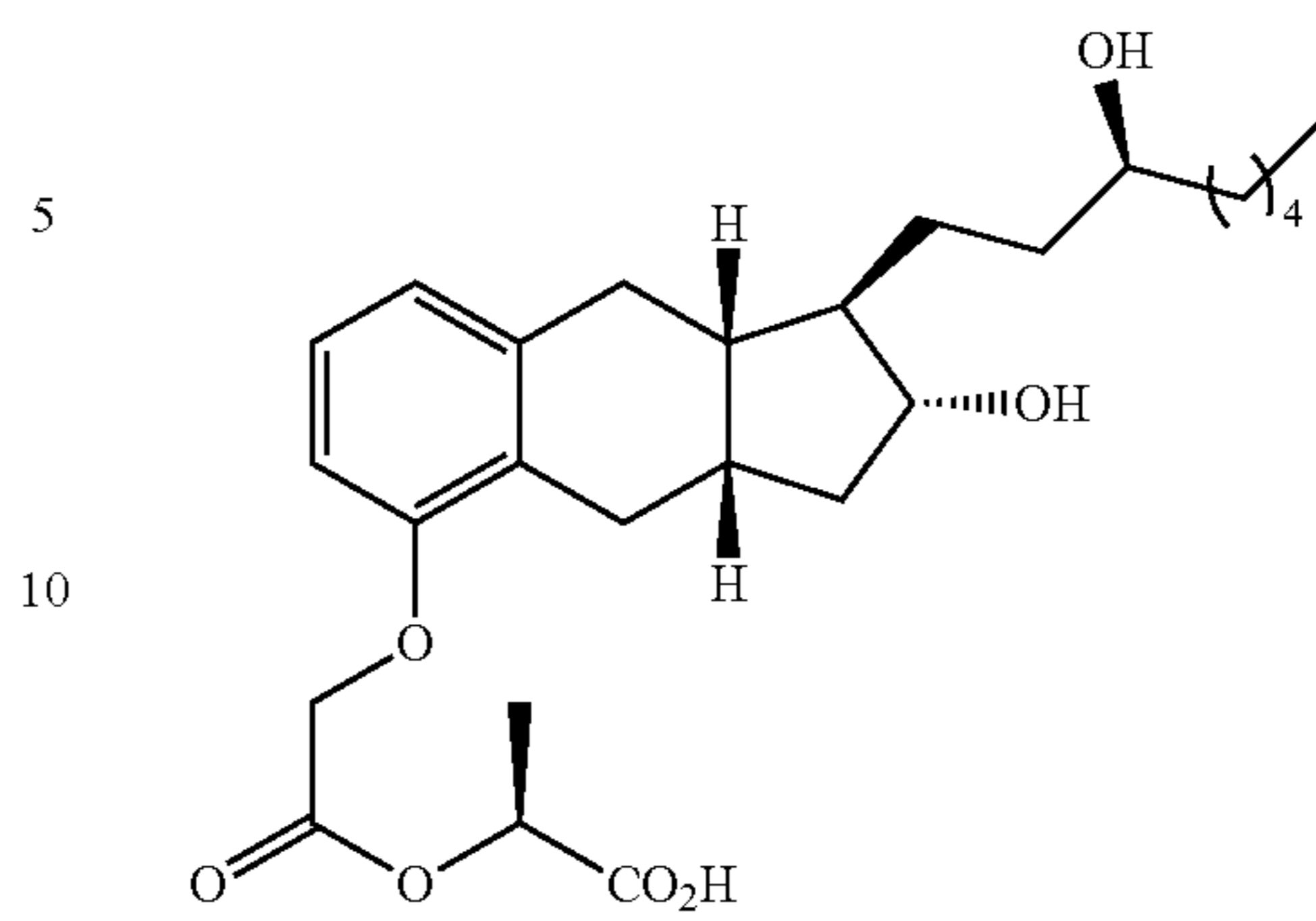
Compound II-13
