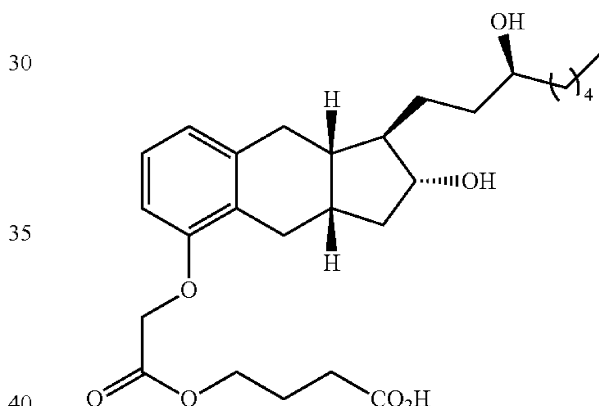
Compound II-1
