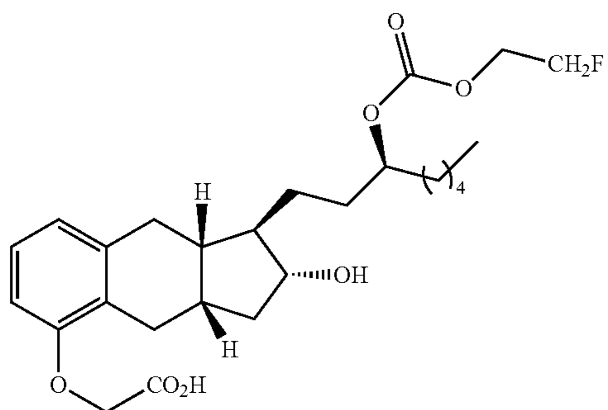
Compound Ib-12
