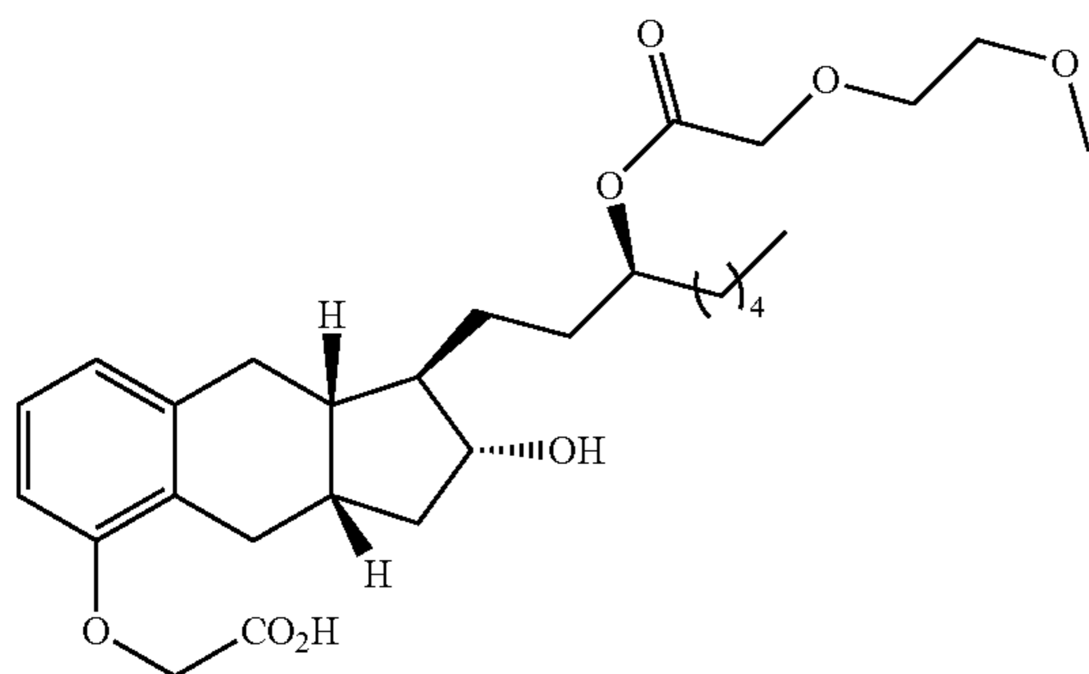
Compound Ib-21
