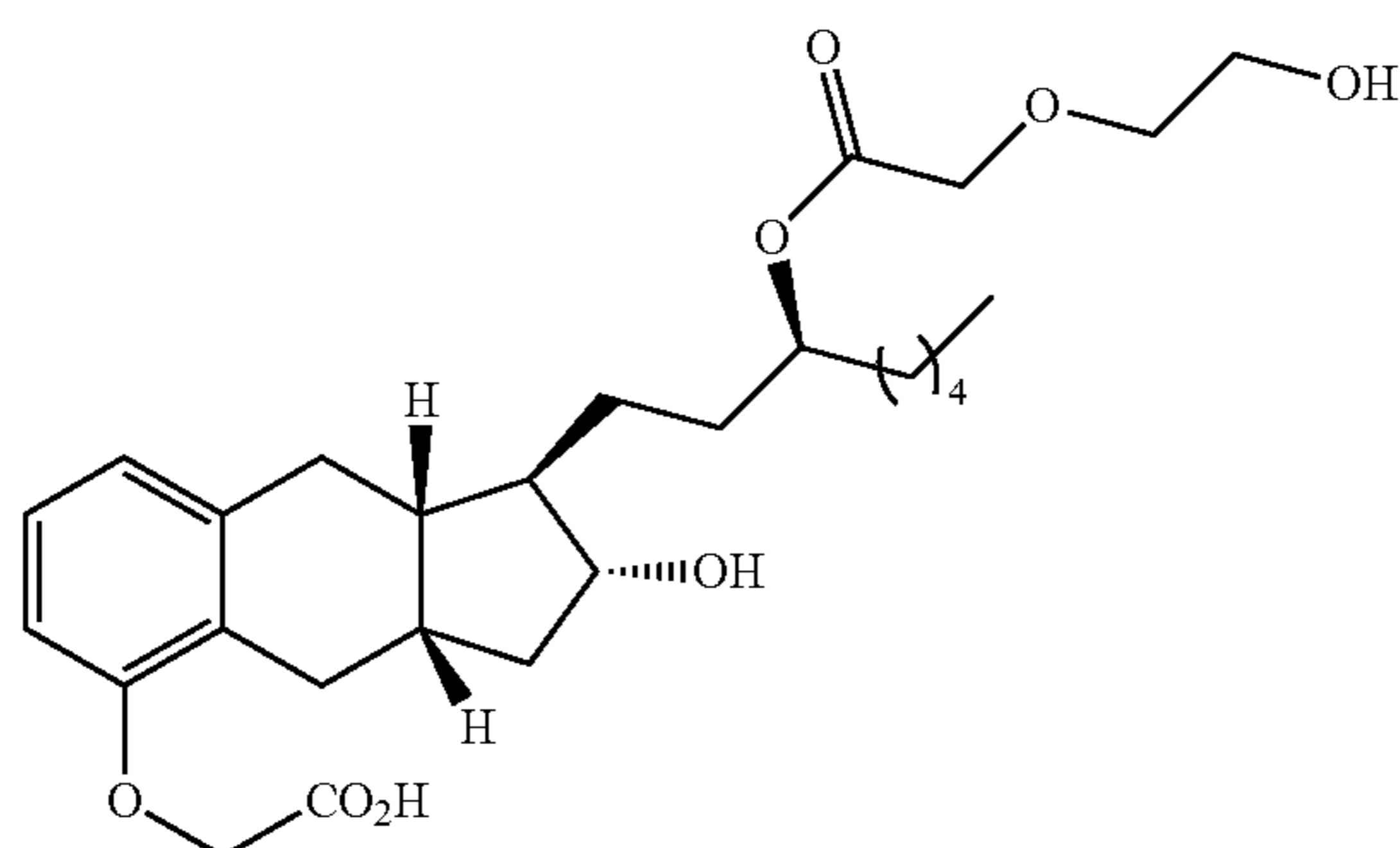
Compound Ib-20
