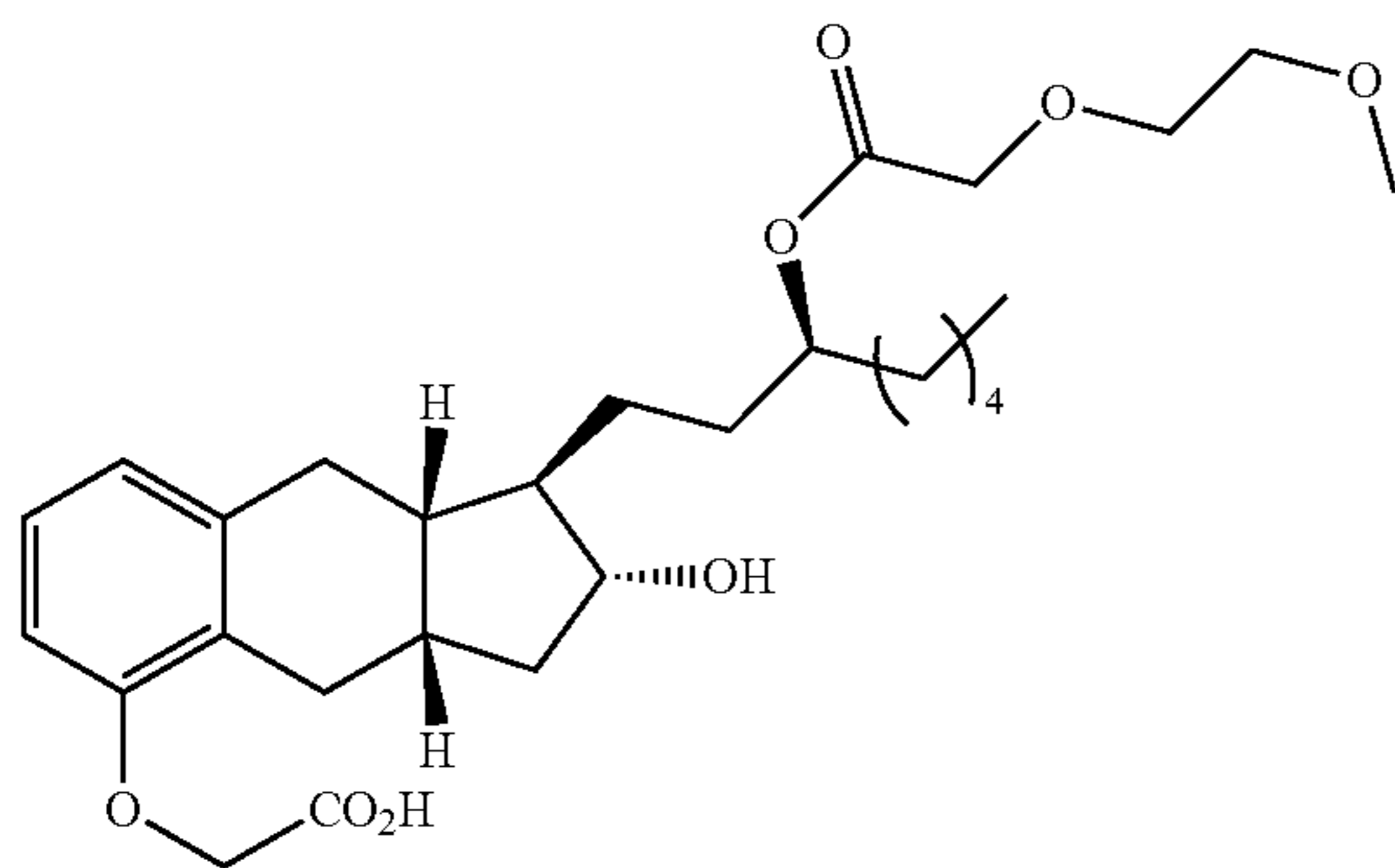
Compound Ib-21
