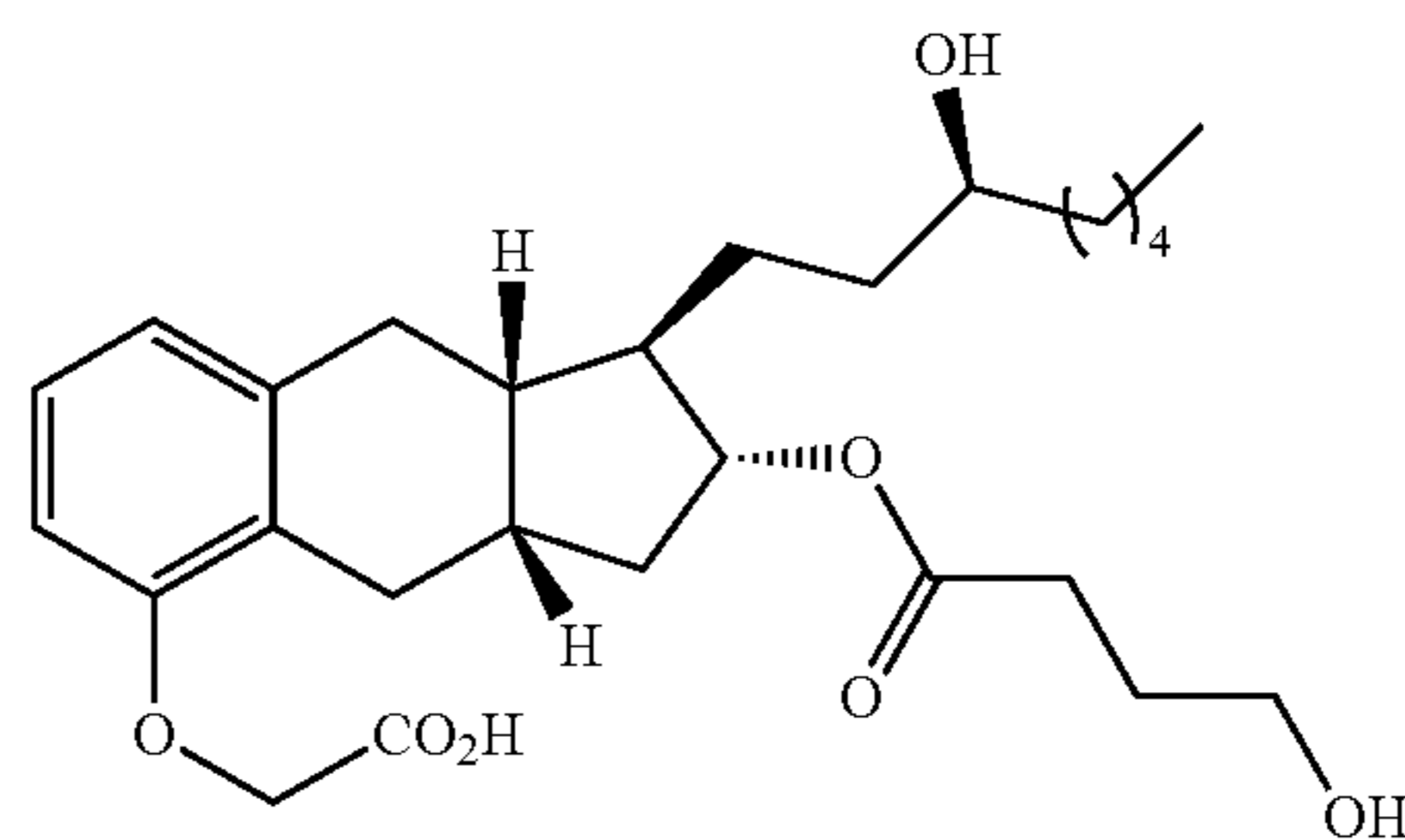
Compound Ia-18
