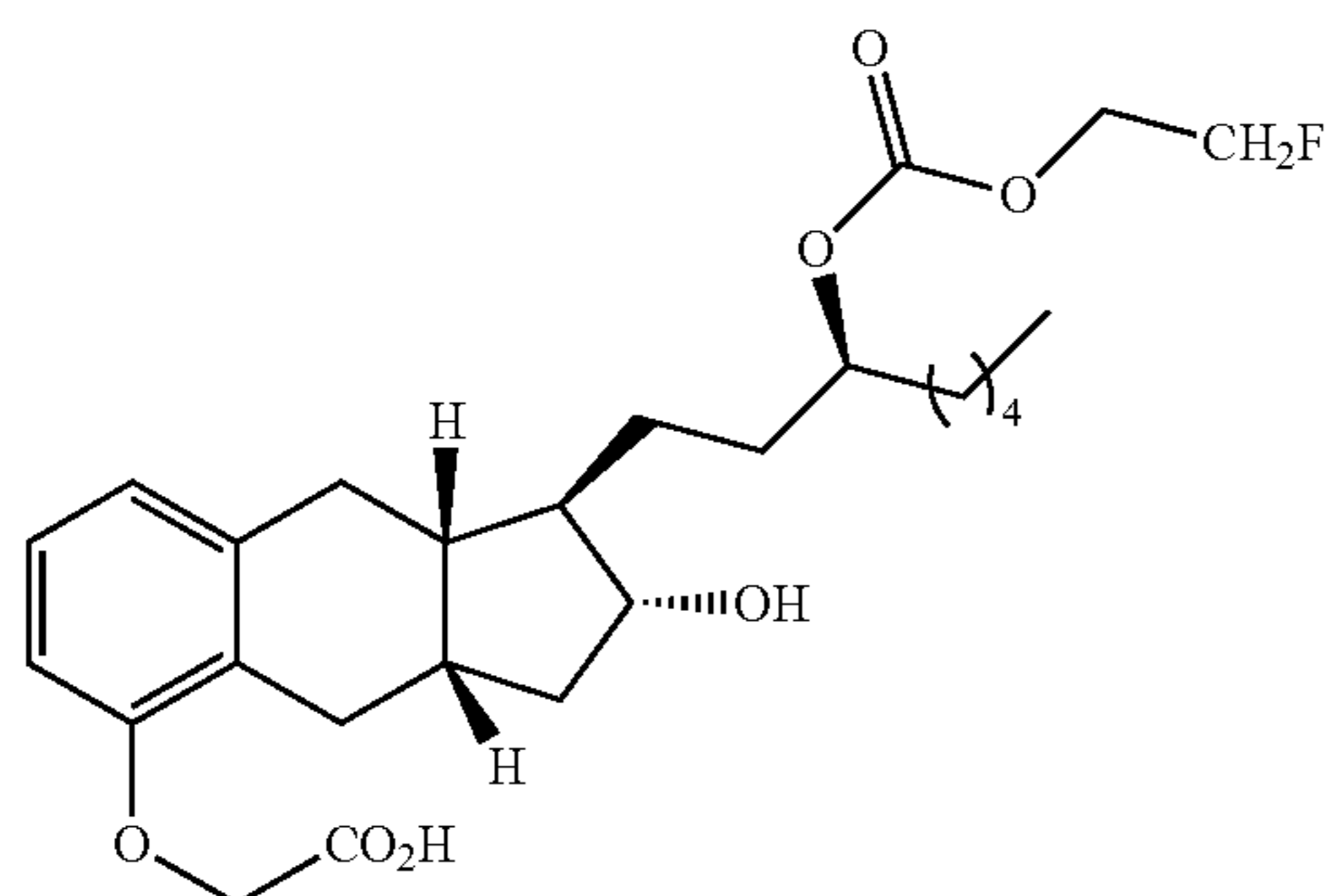
Compound Ib-12
