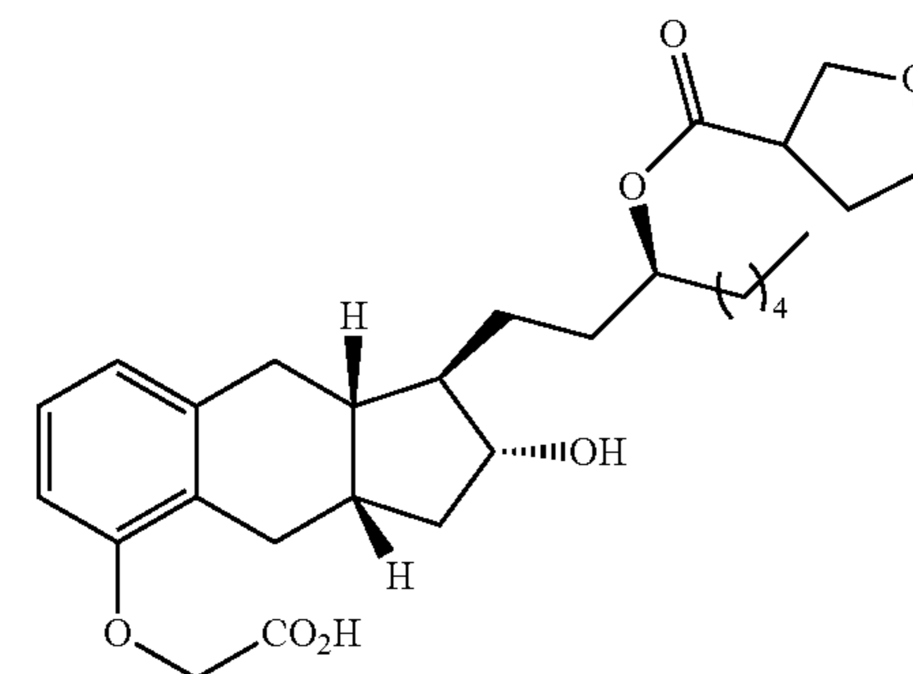
Compound Ib-33
