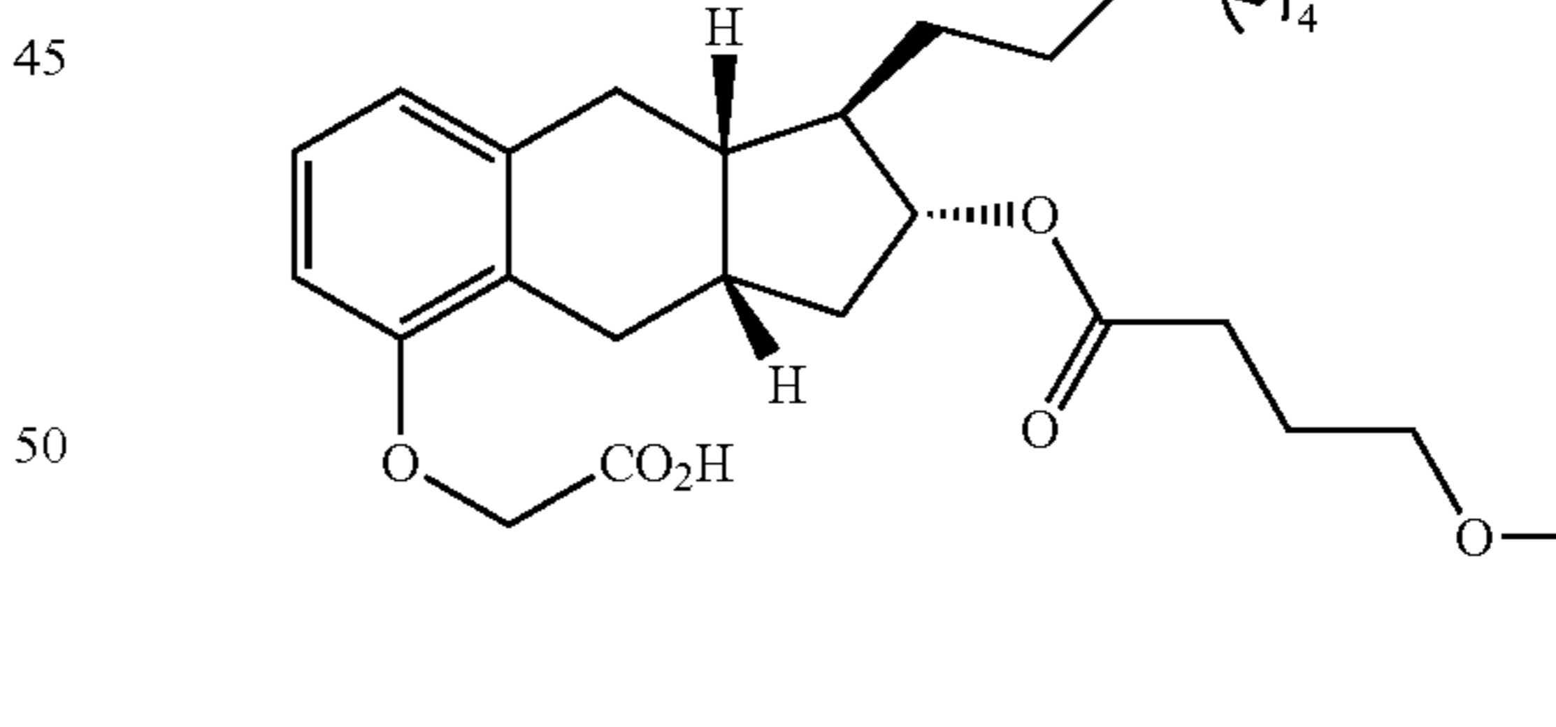
Compound 1a-20
