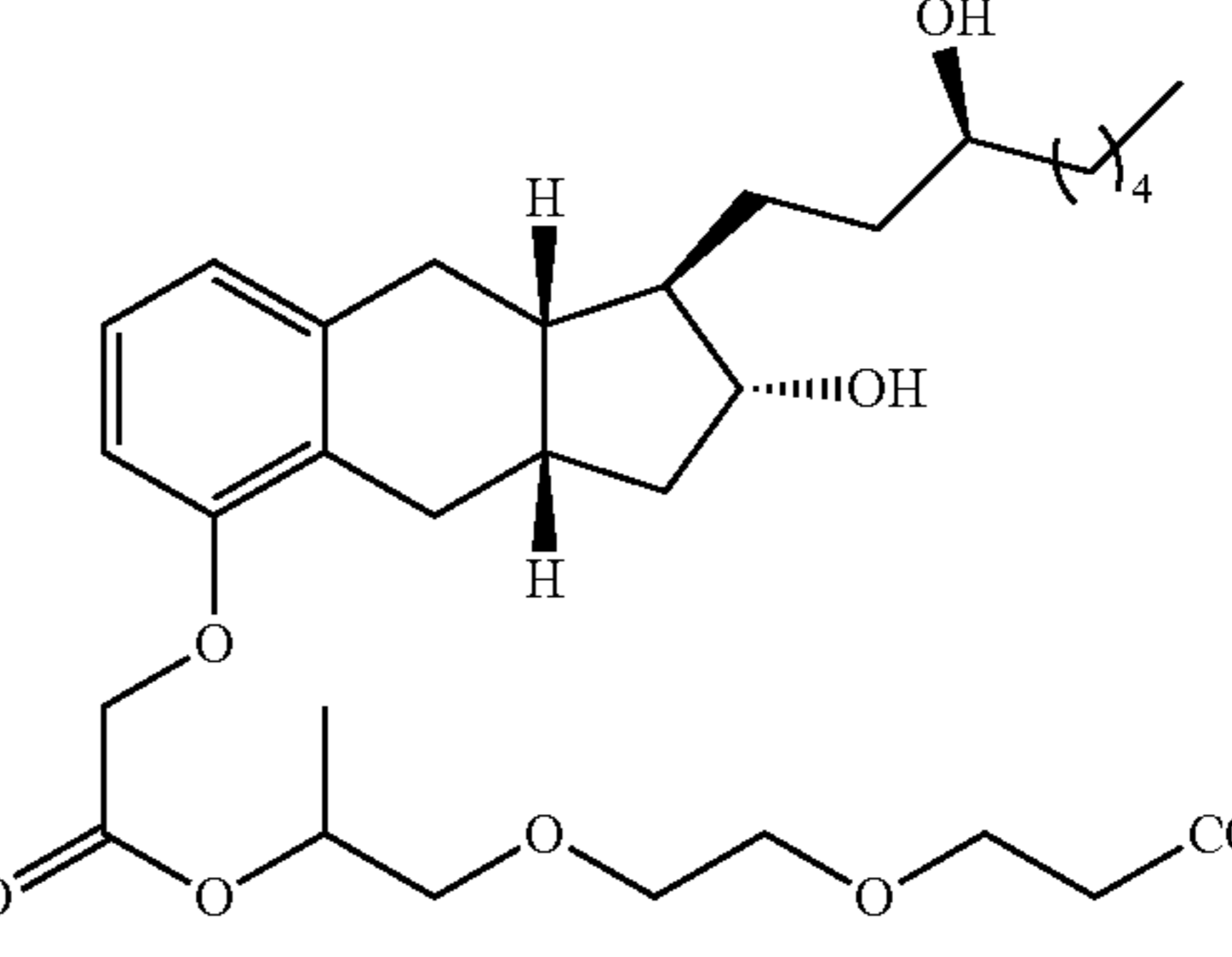
Compound II-20
