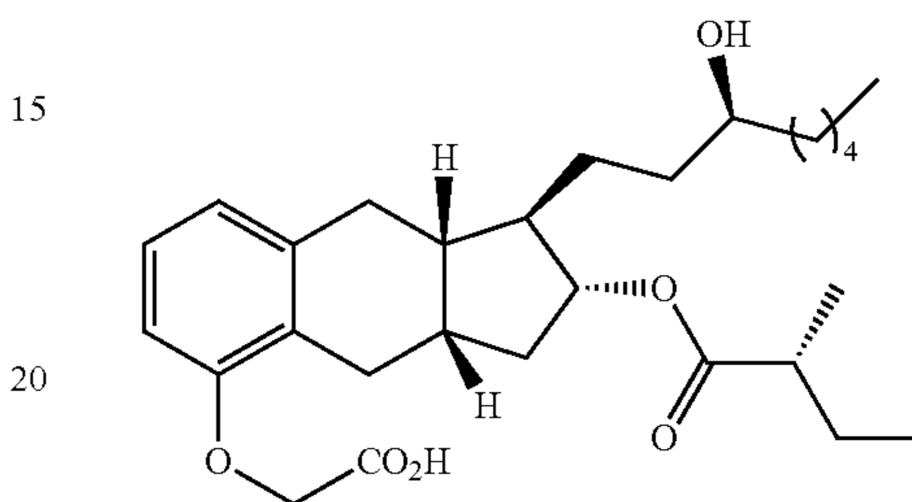
Compound Ia-22
