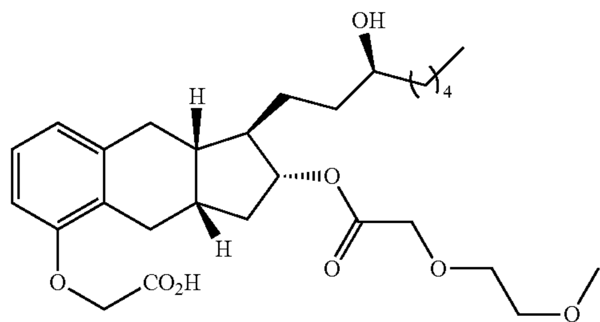
Compound Ia-22
