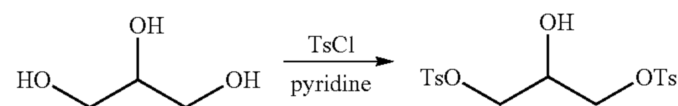
1,3-Bis(4-methylbenzenesulfonate) propanetriol
