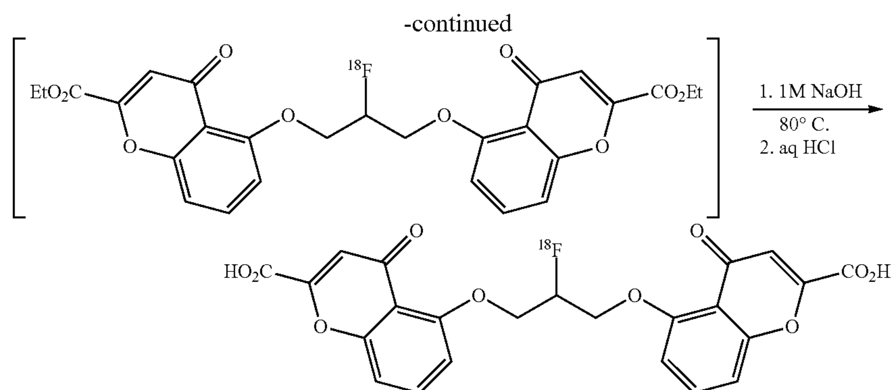
5,5'-(2-[ 18 F]fluoropropane-1,3-diyl)bis(oxy)bis(4-oxo-4H-chromene-2-carboxylic acid)
