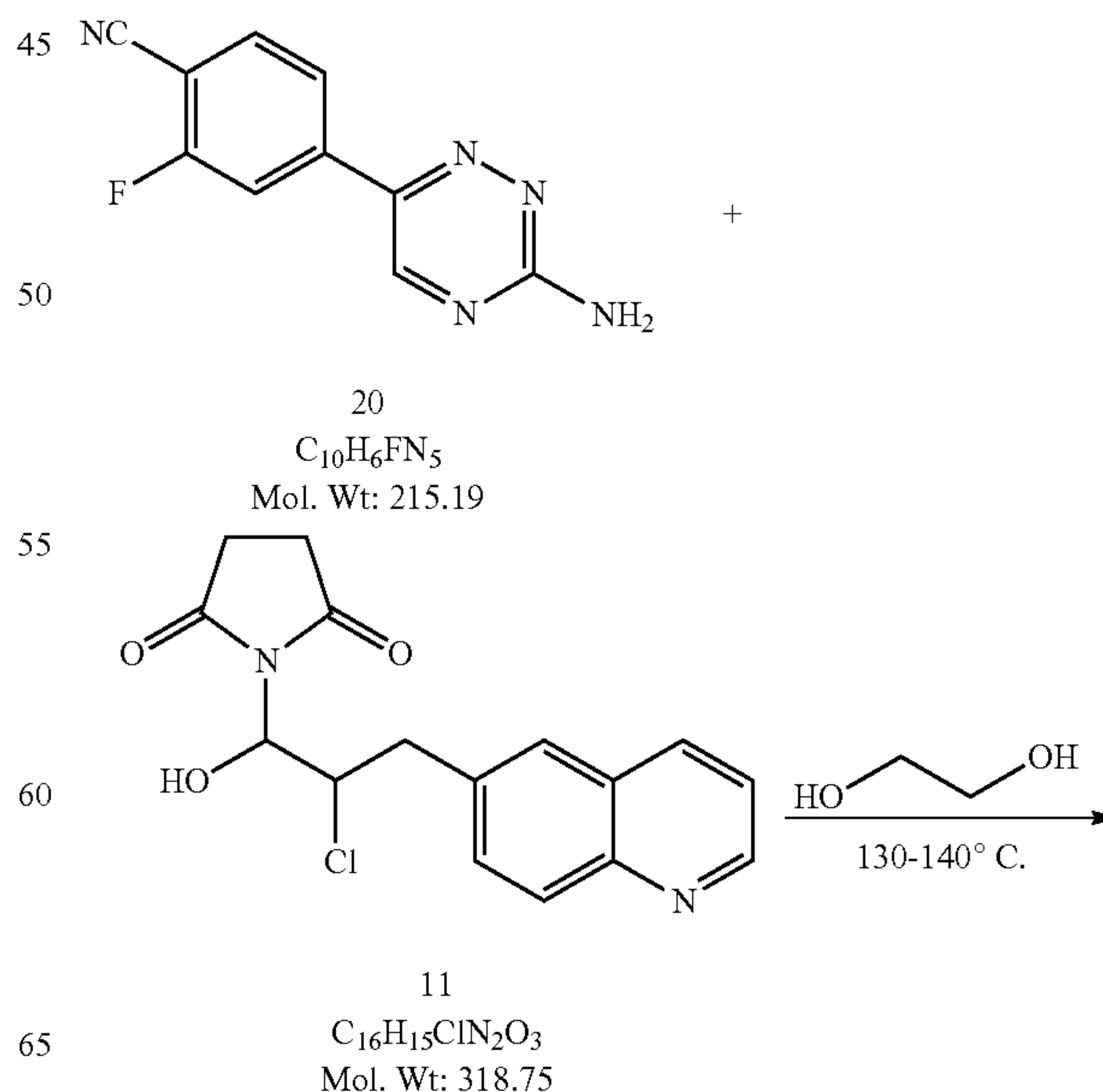
Scheme 5 (Example 26)
