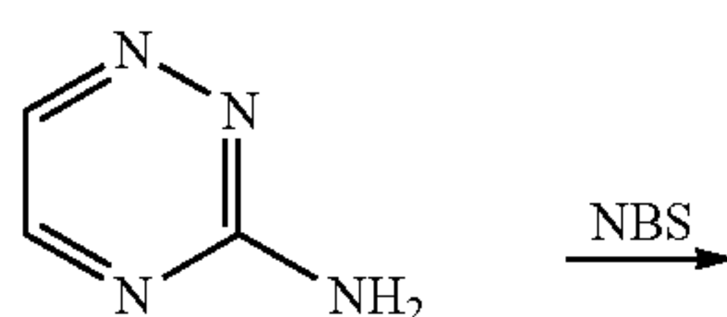
Scheme 4 (Examples 22-25)
