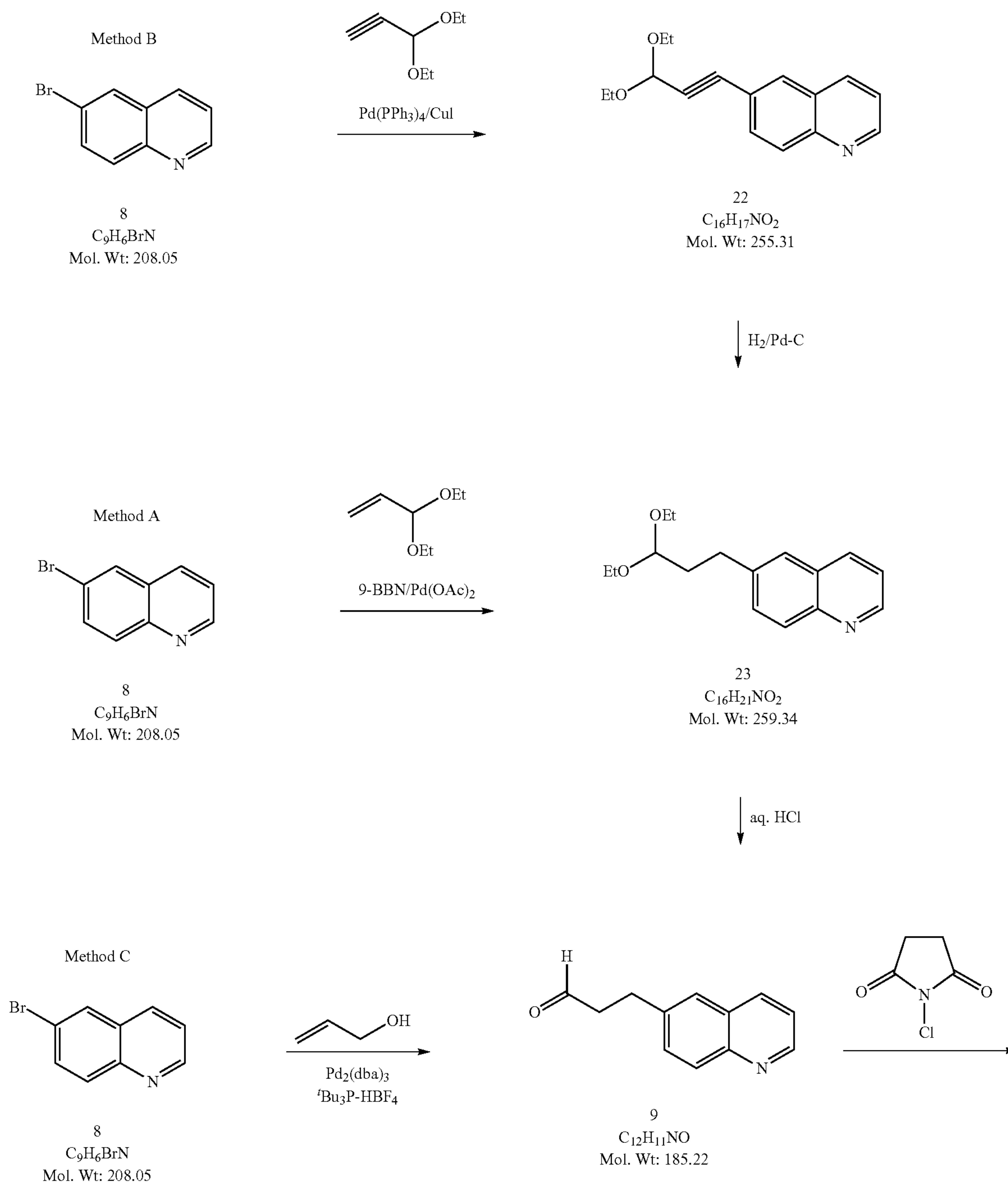
Scheme 2 (Examples 15-18)
