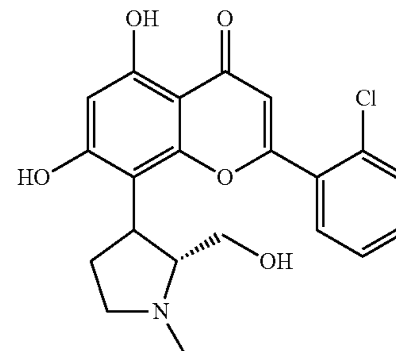
P276-00
