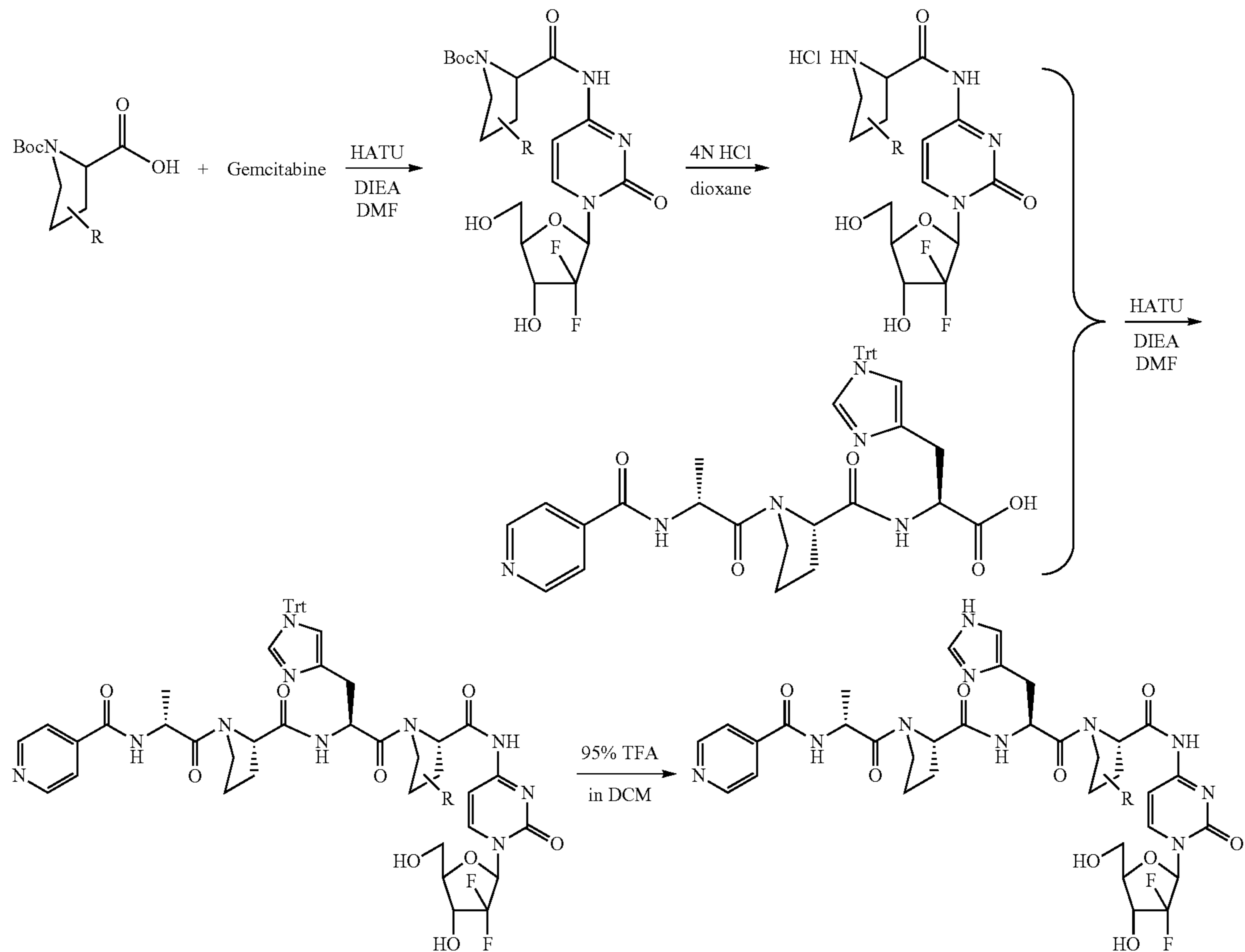
Scheme 1: General synthetic route to 4735 analogues
