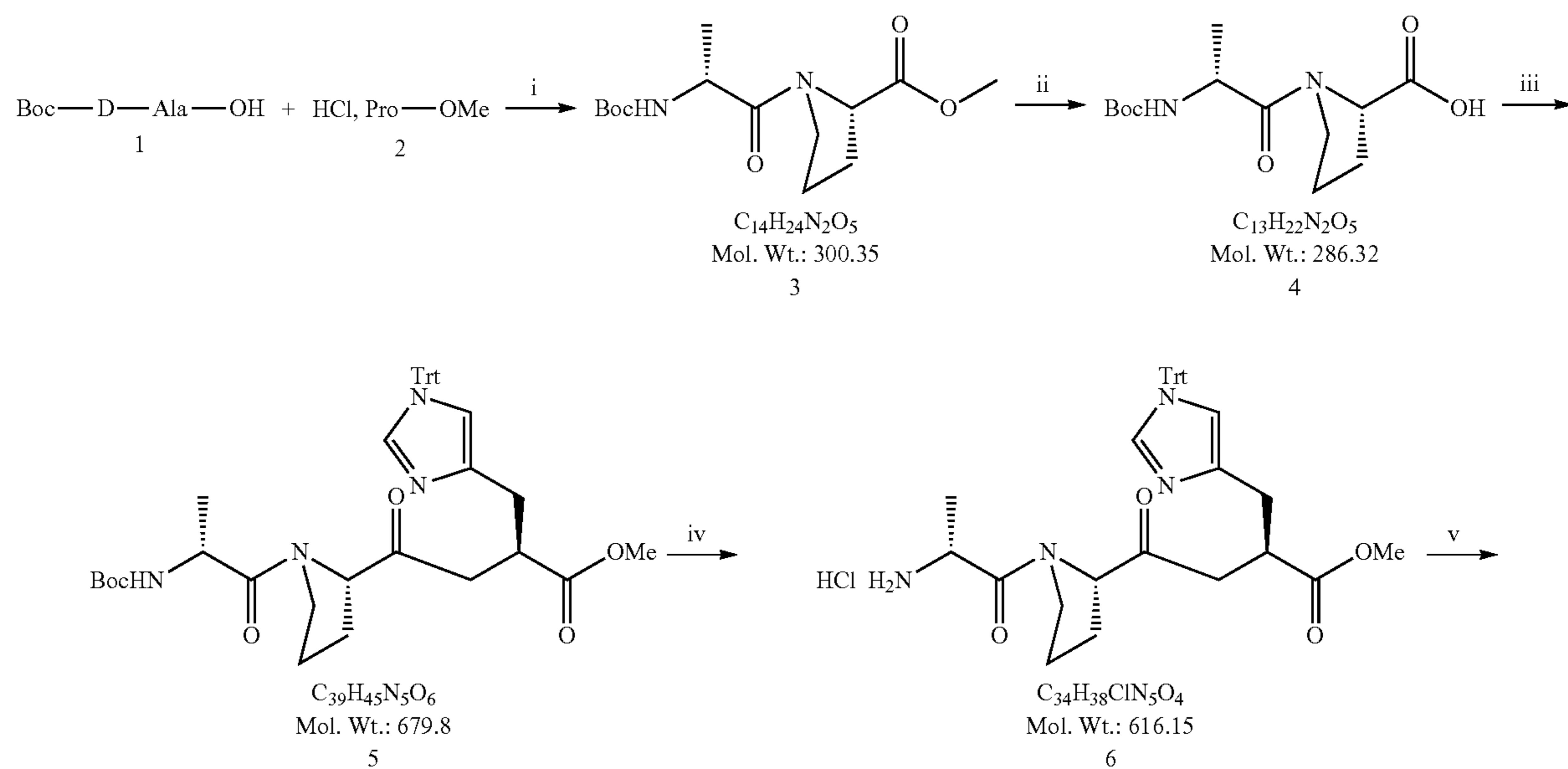
Scheme 2: Synthetic route to 4735D
