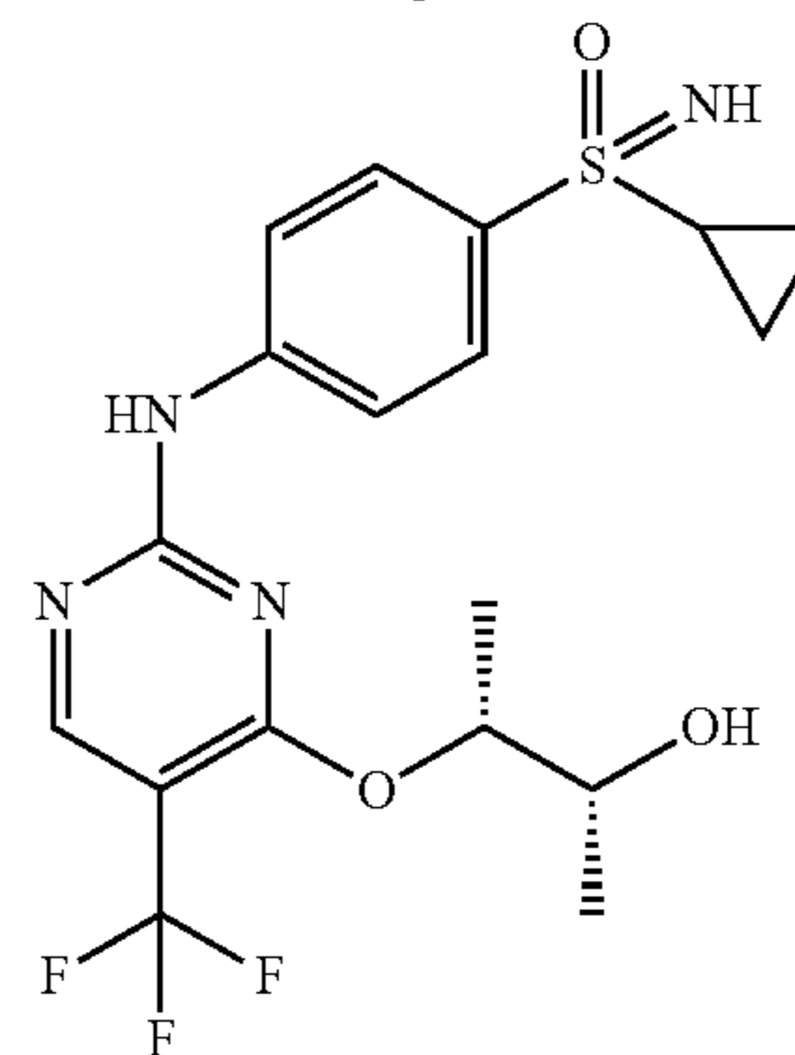
BAY1000394
