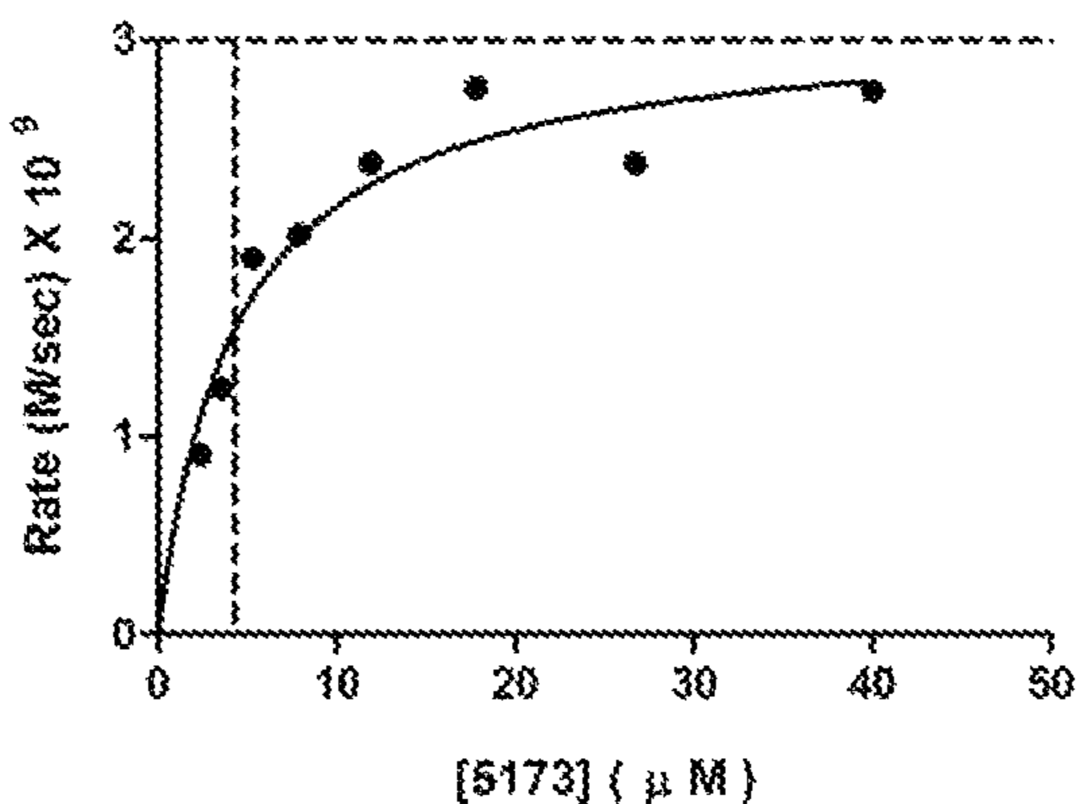
Kinetics of activation of ARI-5173 by FAP
