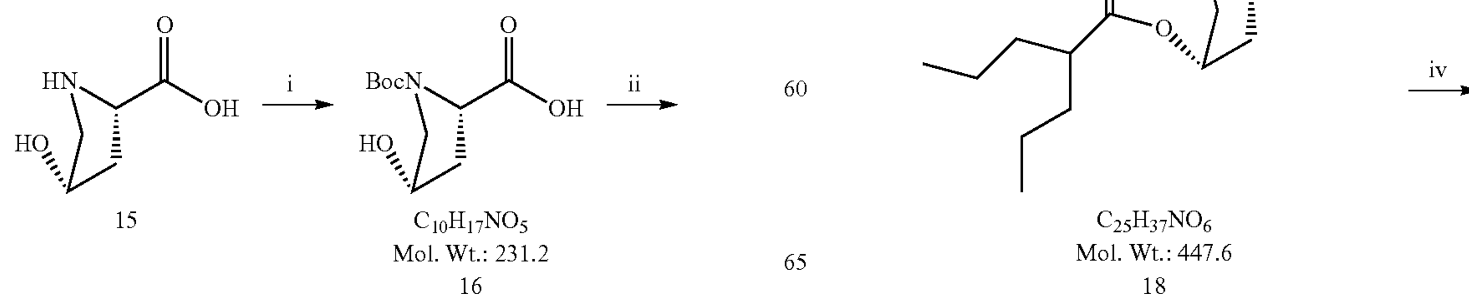
Scheme 3: Synthetic route to substituted Proline analogues
