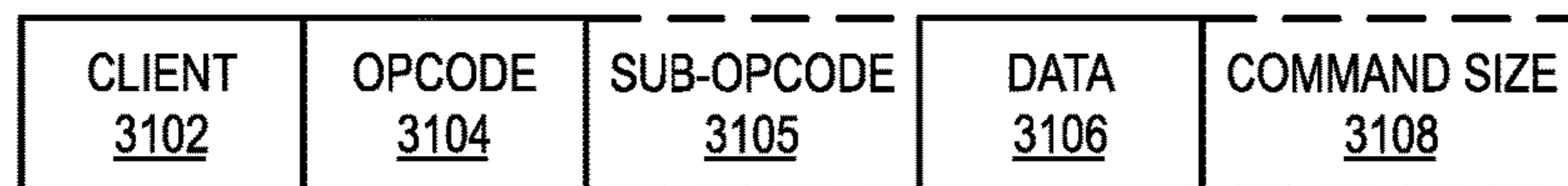
FIG. 31A GRAPHICS PROCESSOR COMMAND FORMAT 3100
