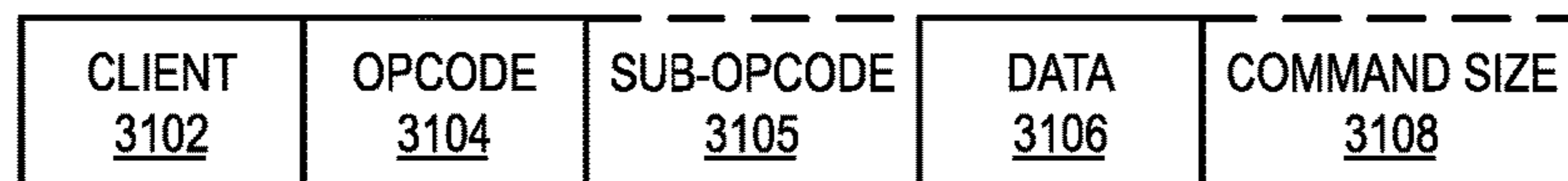
FIG. 31A GRAPHICS PROCESSOR COMMAND FORMAT 3100
