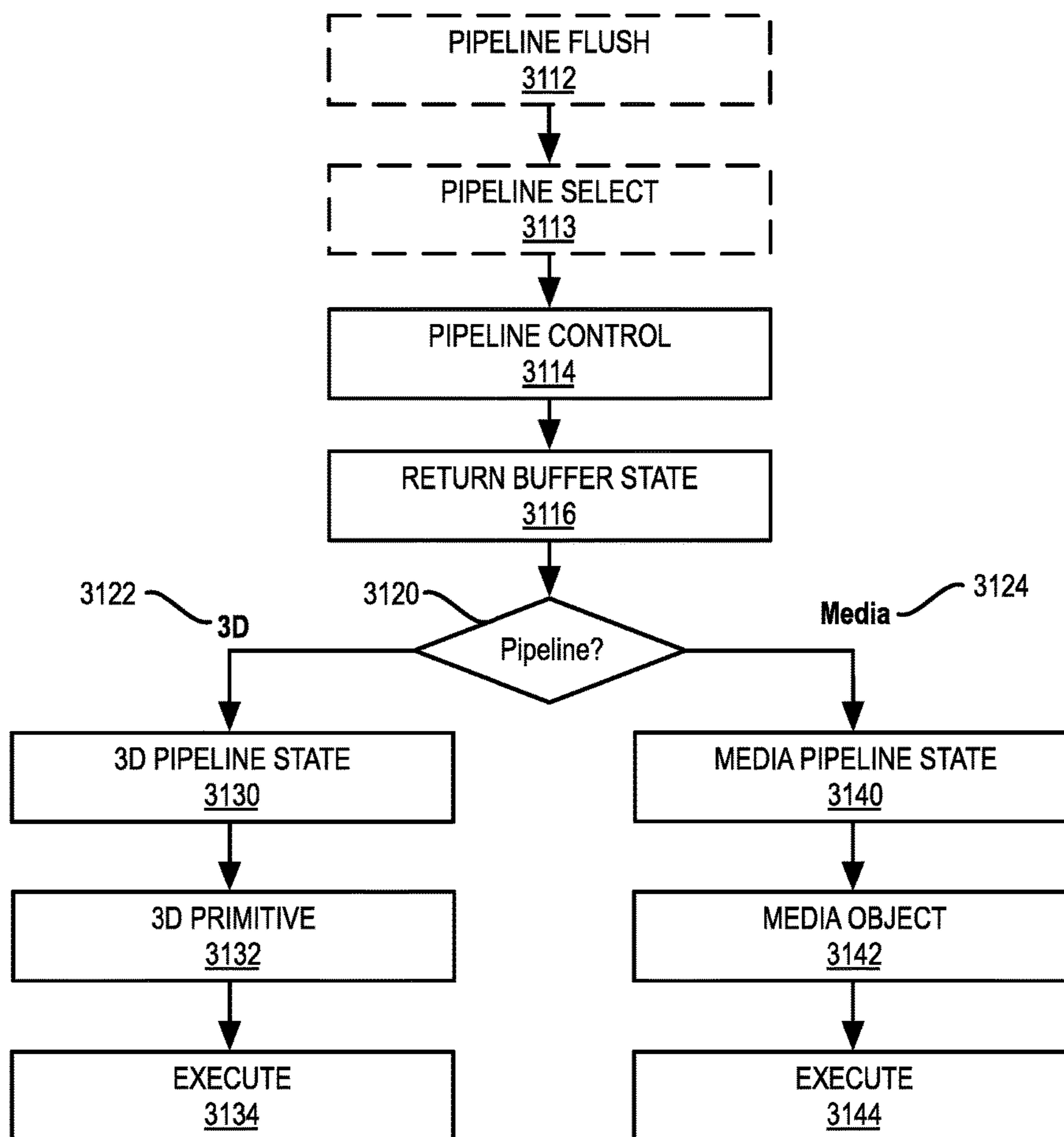
FIG. 31B GRAPHICS PROCESSOR COMMAND SEQUENCE 3110
