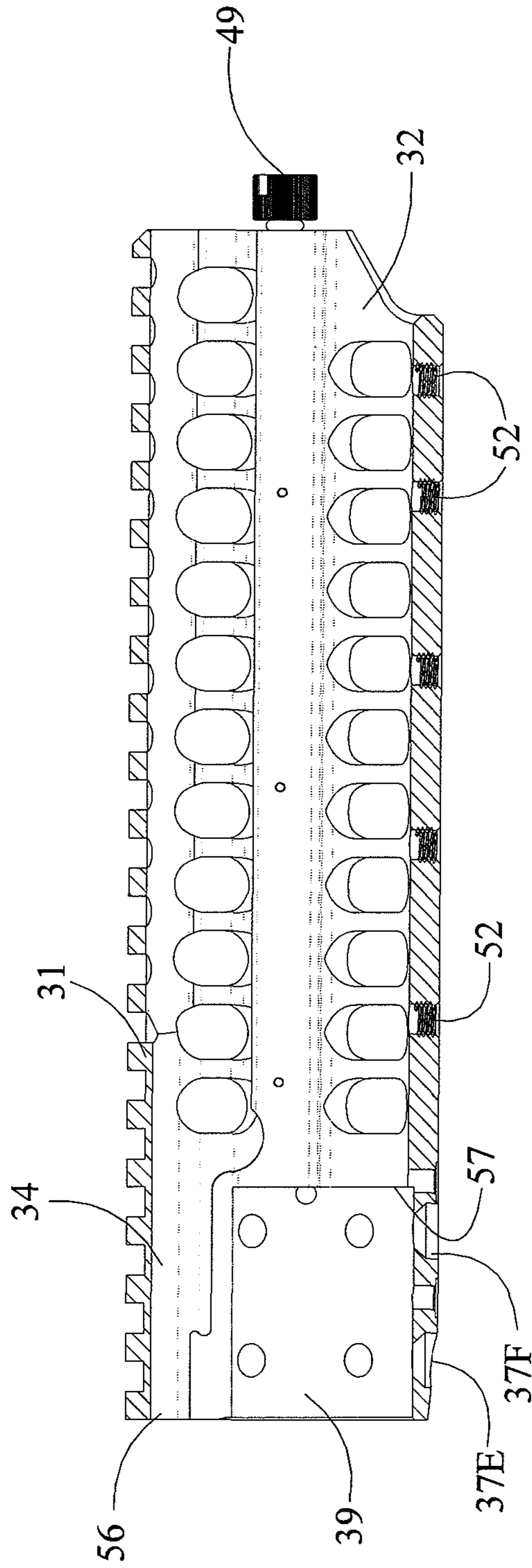
SECTION VIEW
