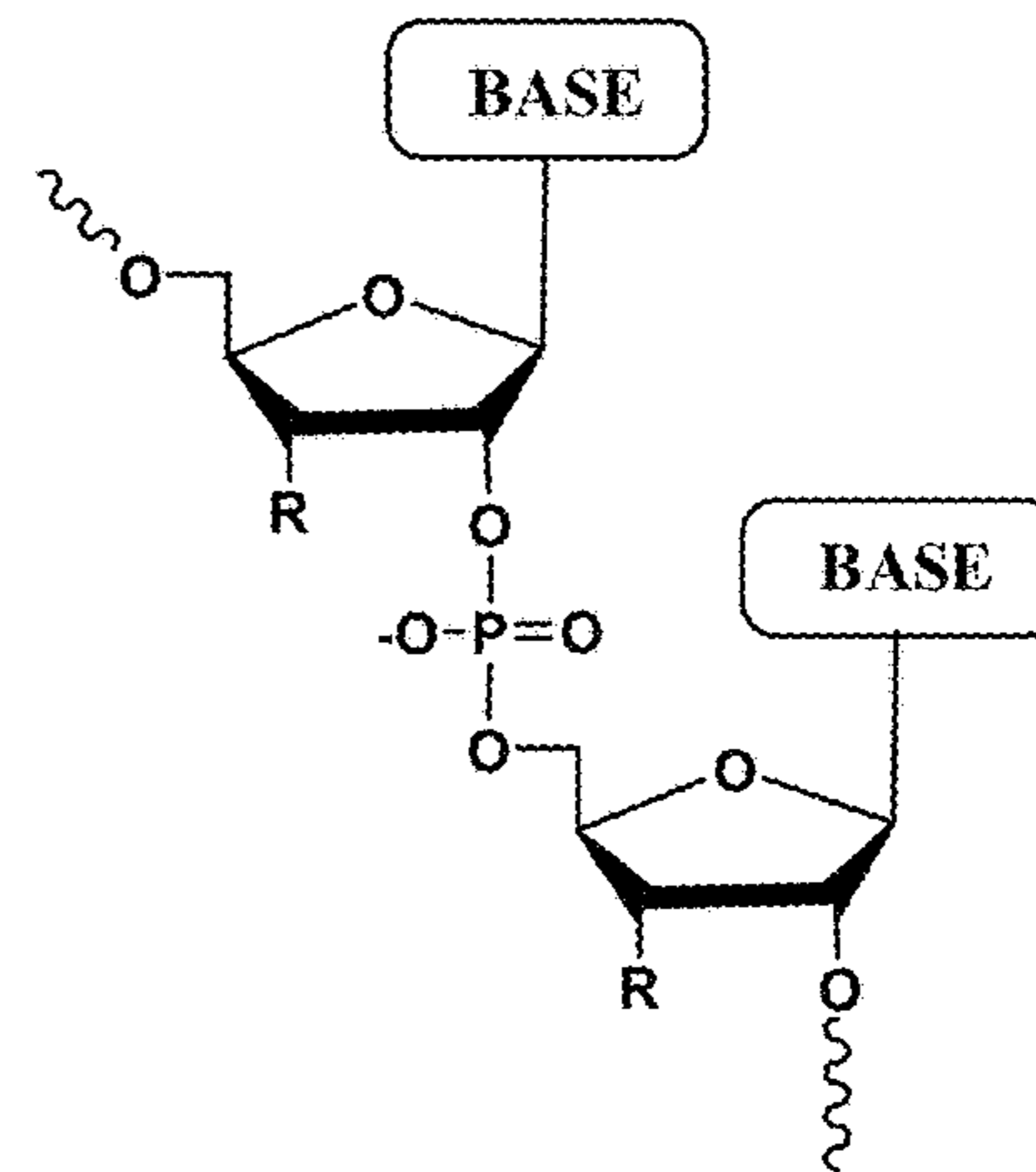
2', 5'-linked oligonucleotide
