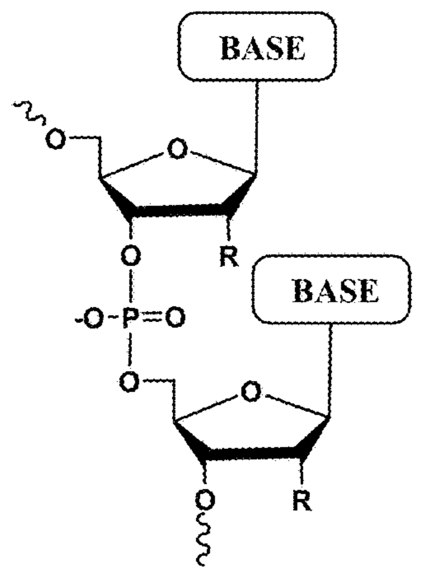
3', 5'-linked oligonucleotide
