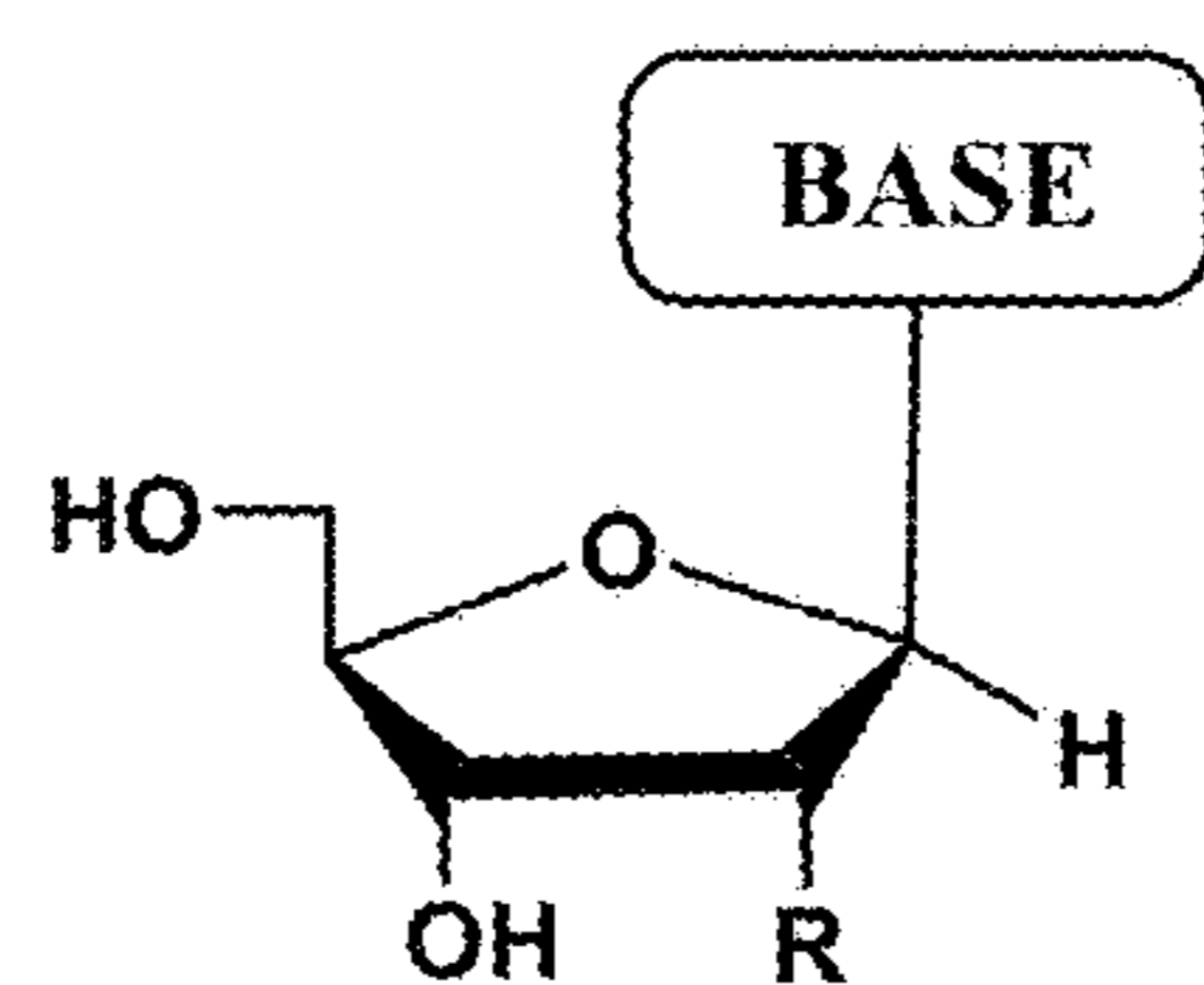
\beta -D-nucleoside
