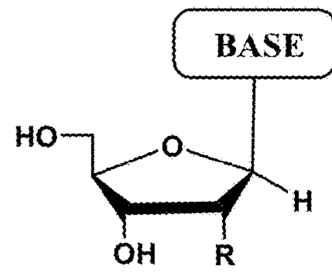
\beta -D-nucleoside
