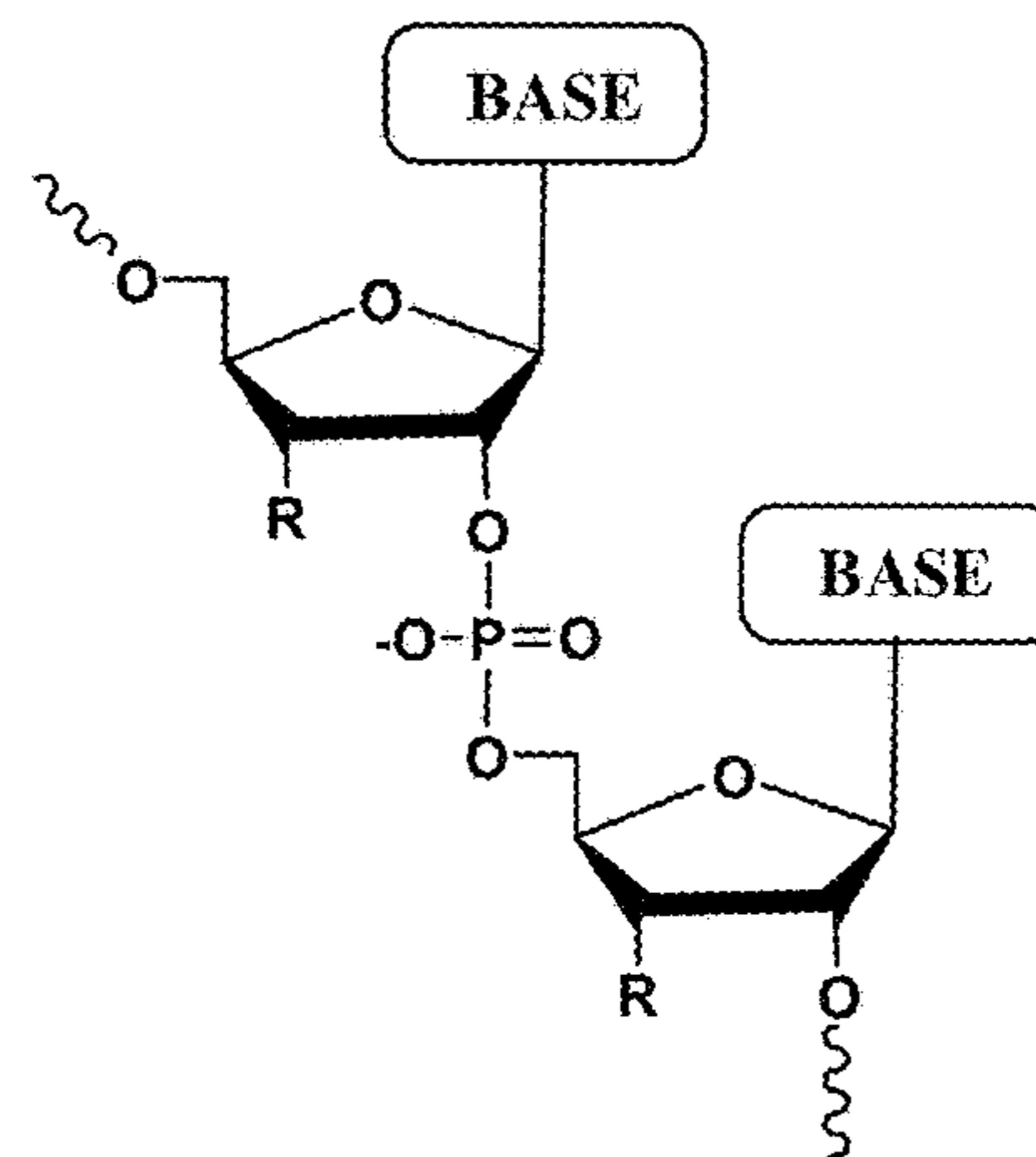
2', 5'-linked oligonucleotide
