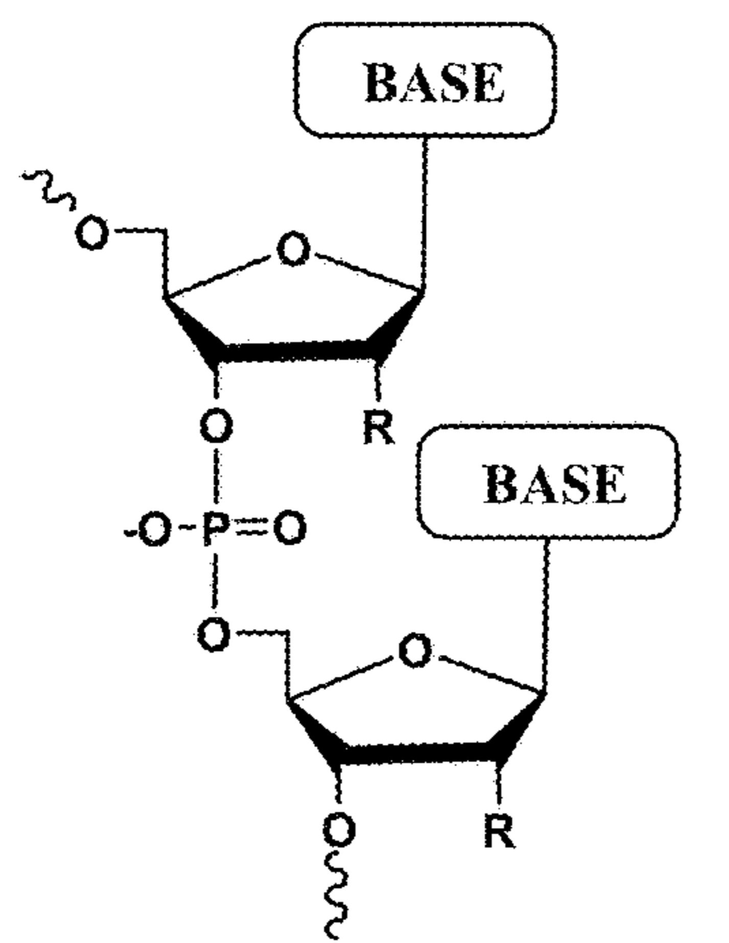
3', 5'-linked oligonucleotide
