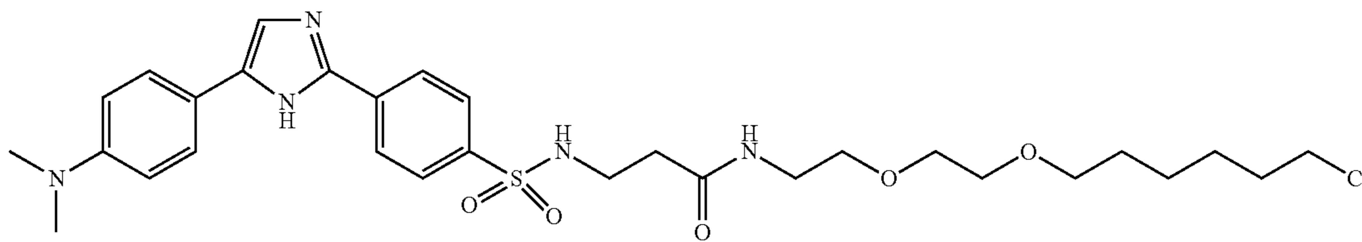
N-{2-[2-(6-Chlorohexyloxy)-ethoxy]-ethyl}-9'-chloro-roseminaphthofluorescein-5-(and -6)-amide
