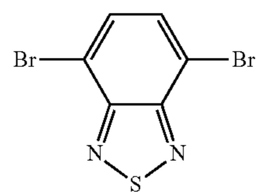
4,7-dibromobenzo[c]- 1,2,5-thiadiazole
