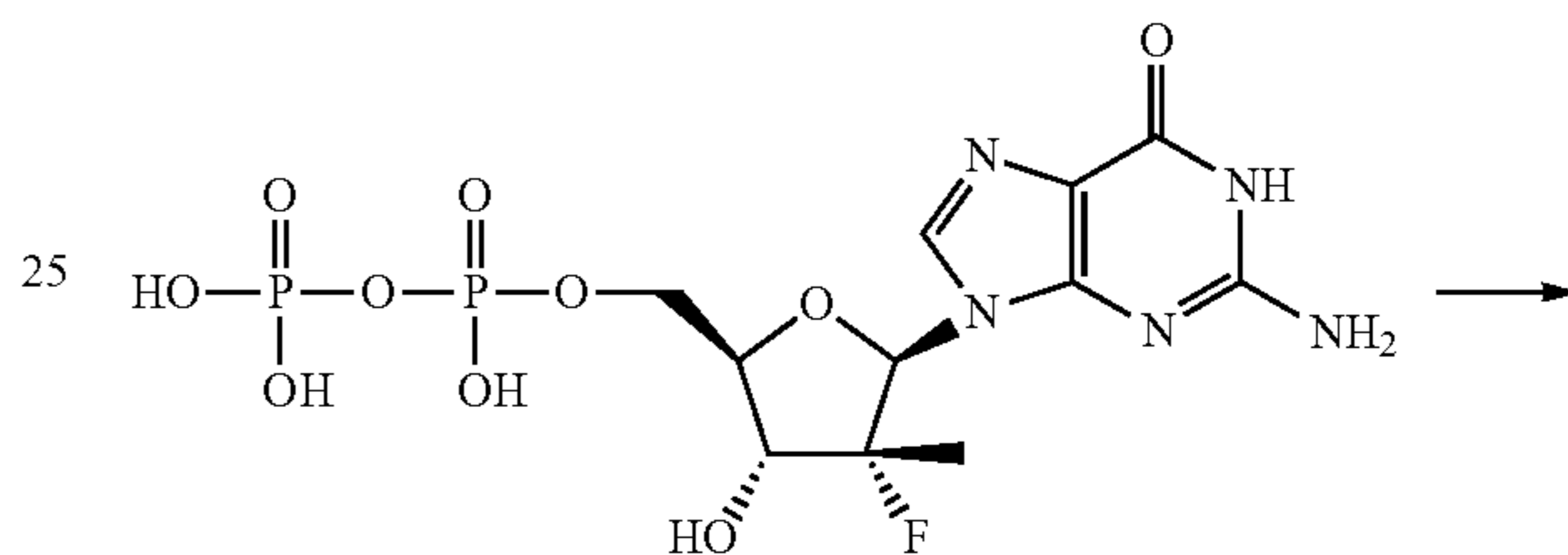
Formula VII
