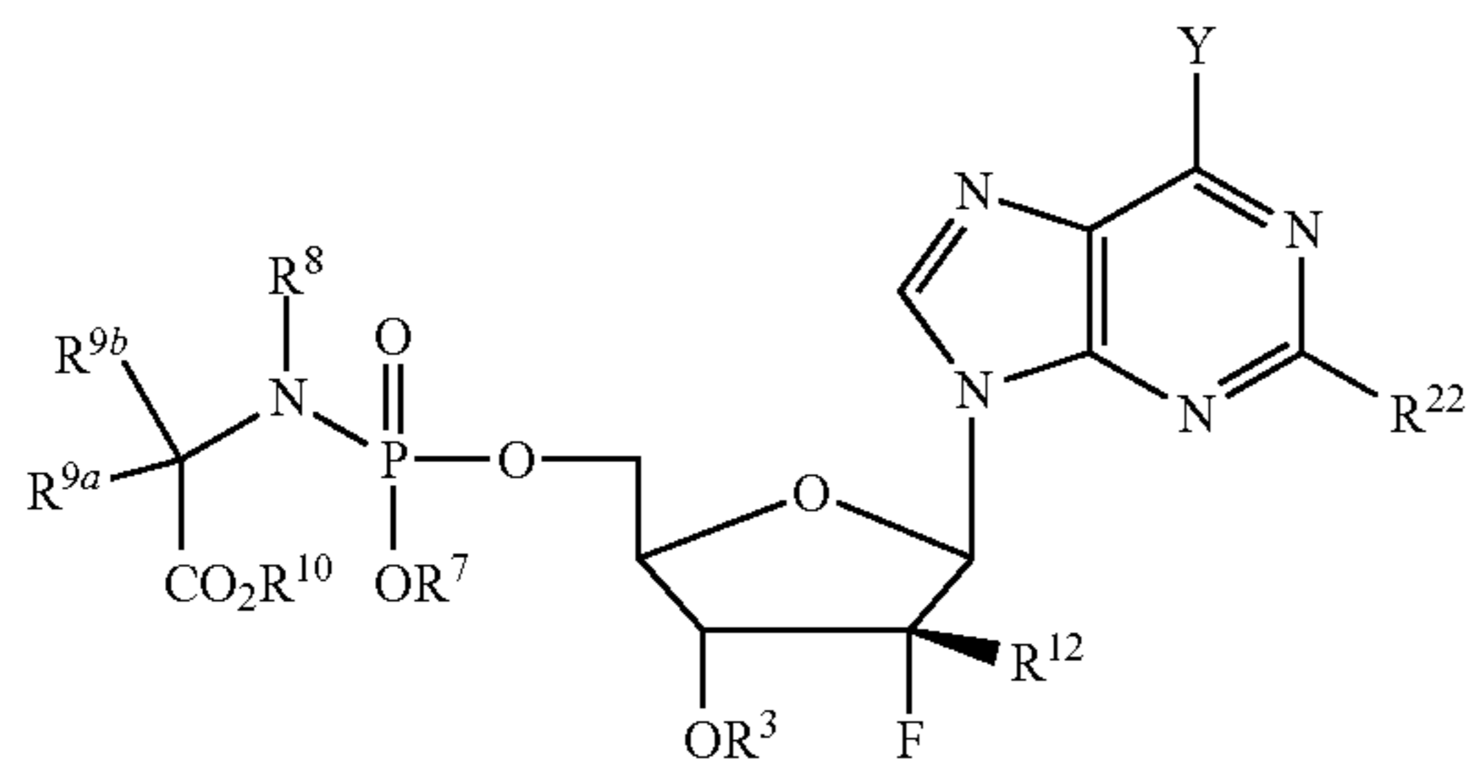
Formula III
