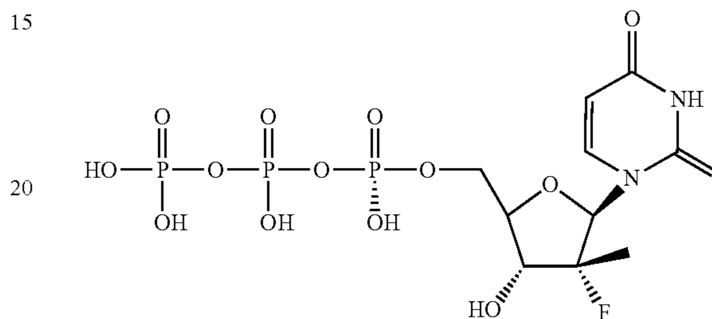
2'-Deoxy-2'- \alpha -fluoro- \beta -C-methyluridine-5'-triphosphate
