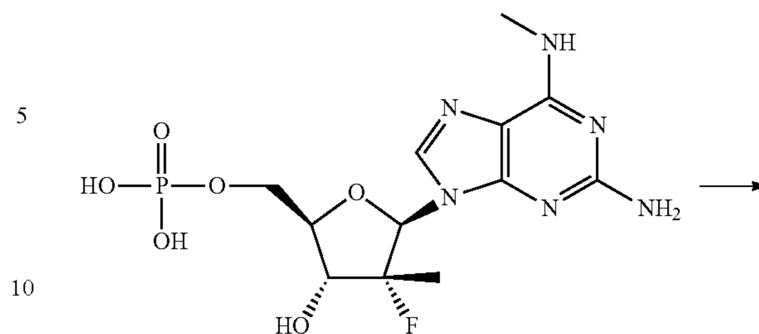
Formula VI
