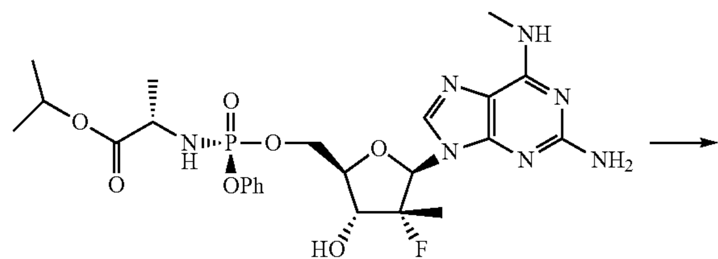
Scheme 1
