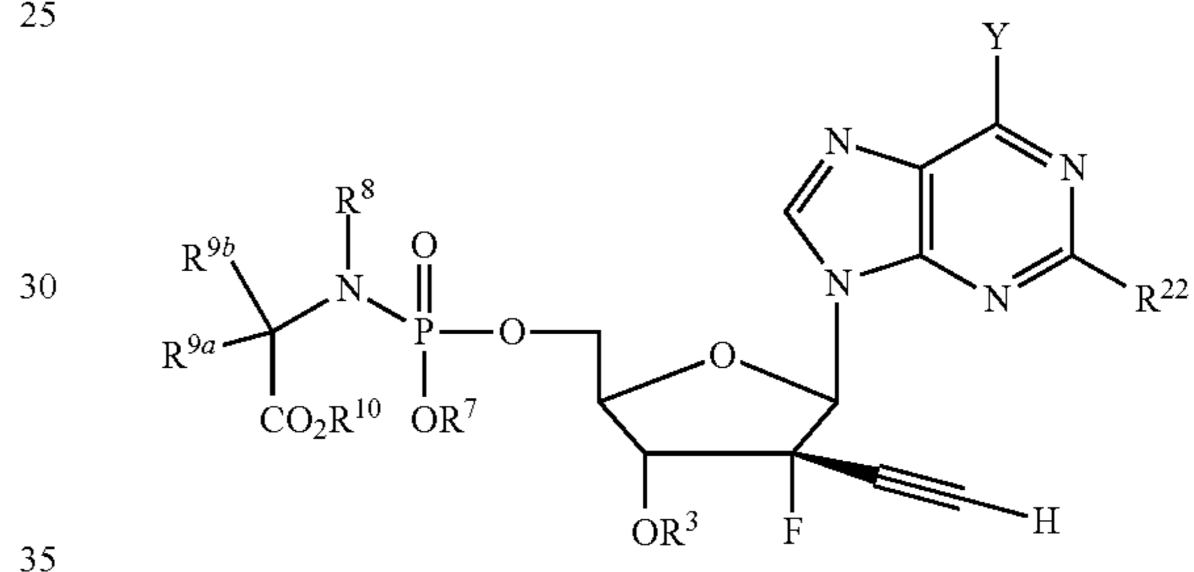
Formula V
