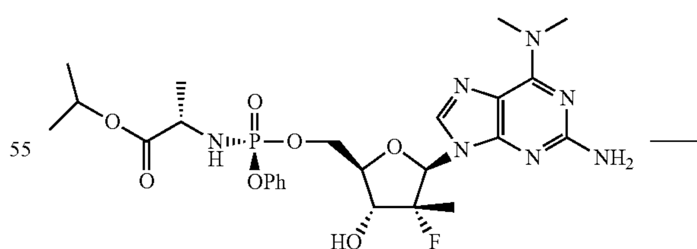
Scheme 2
