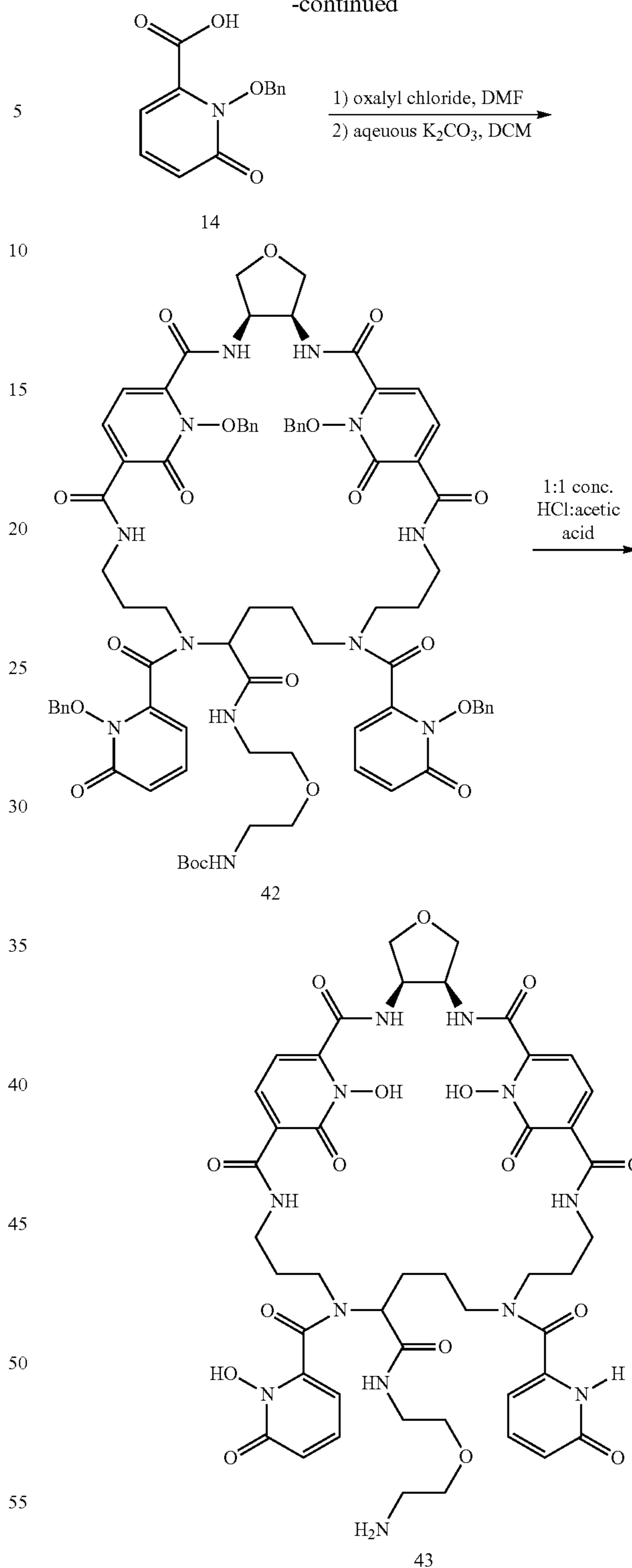
Synthesis of exemplary bifunctional chelator 43.
