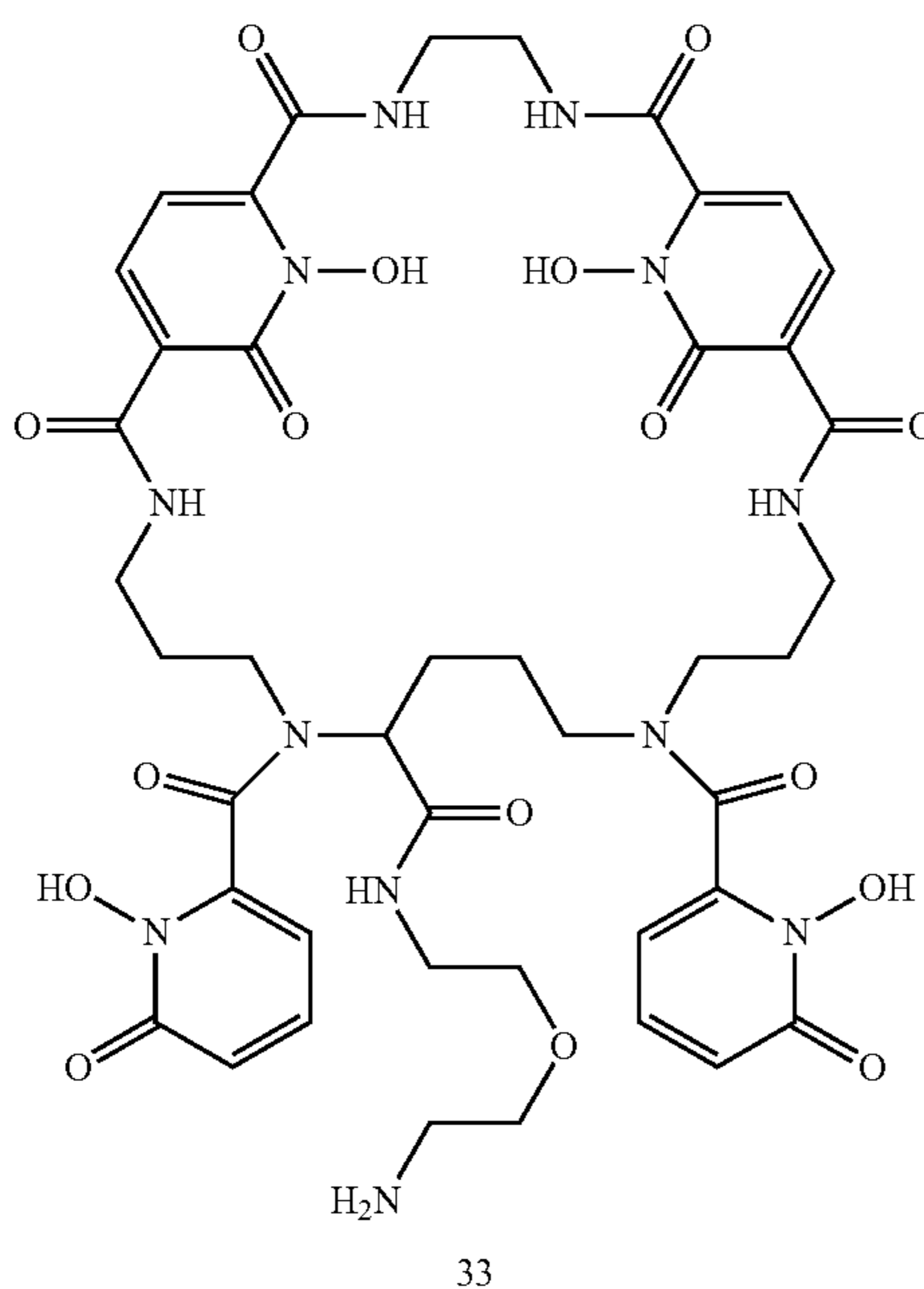
Synthetic scheme of exemplary bifunctional chelator 33.
