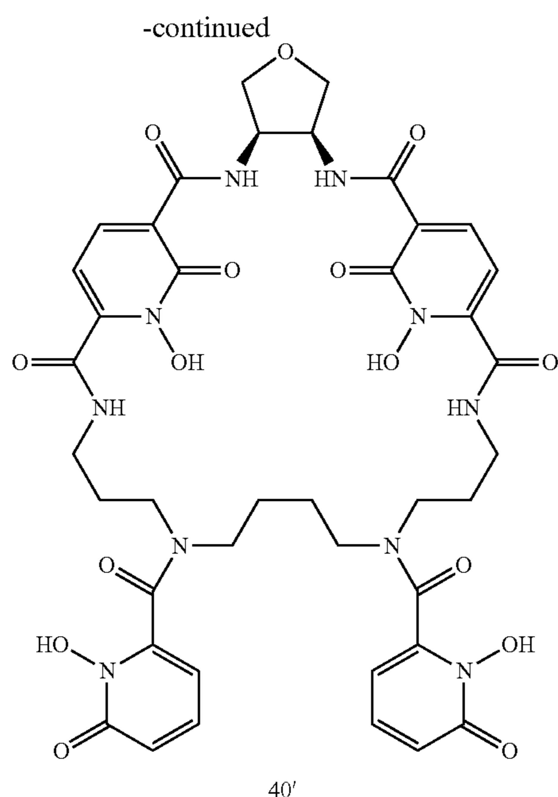
Synthetic scheme for parent compound 40'
