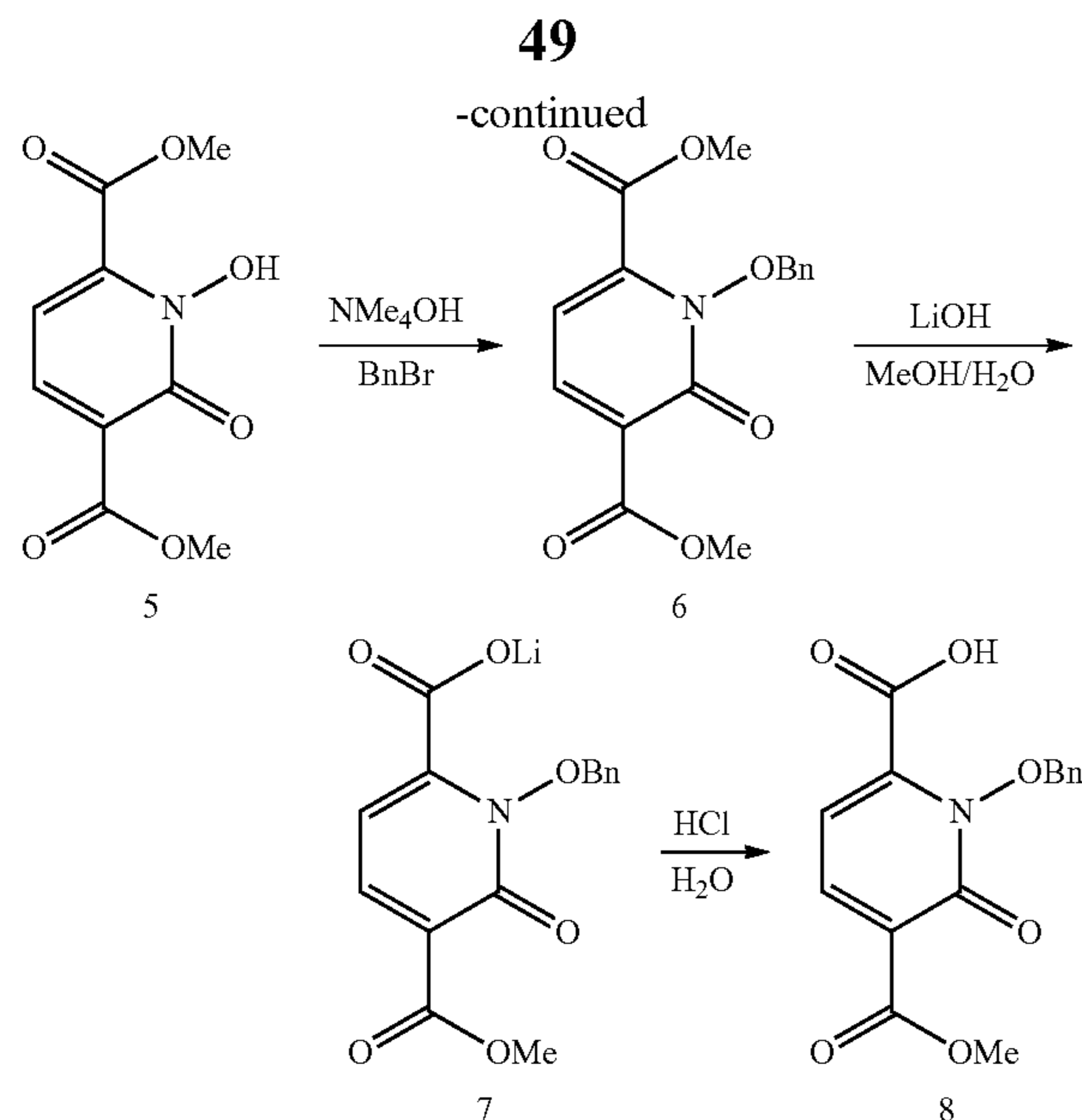
Synthetic scheme of bridging 1,2-HOPO intermediate 8.
