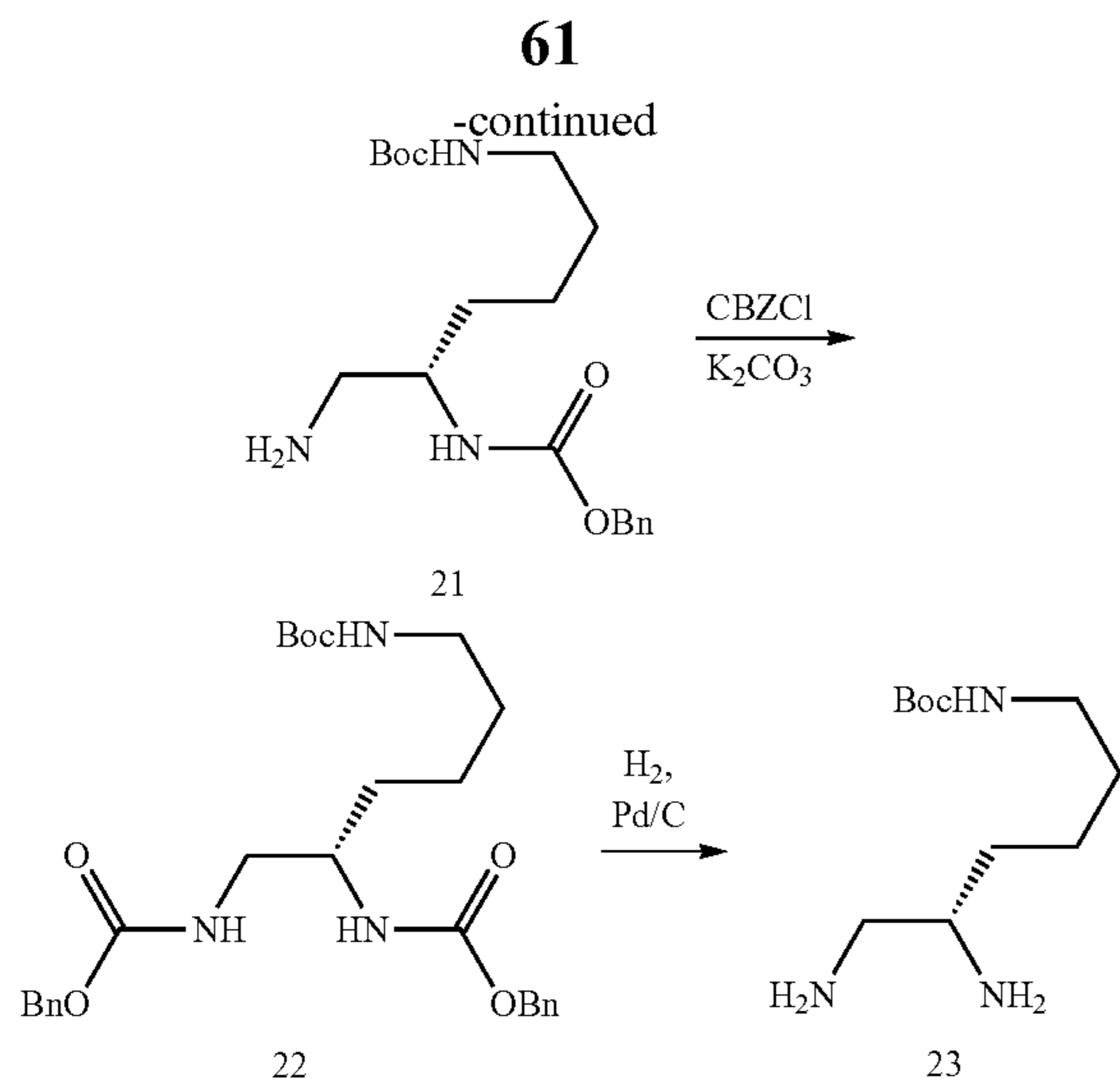
Synthetic scheme of exemplary scaffold amine 23.
