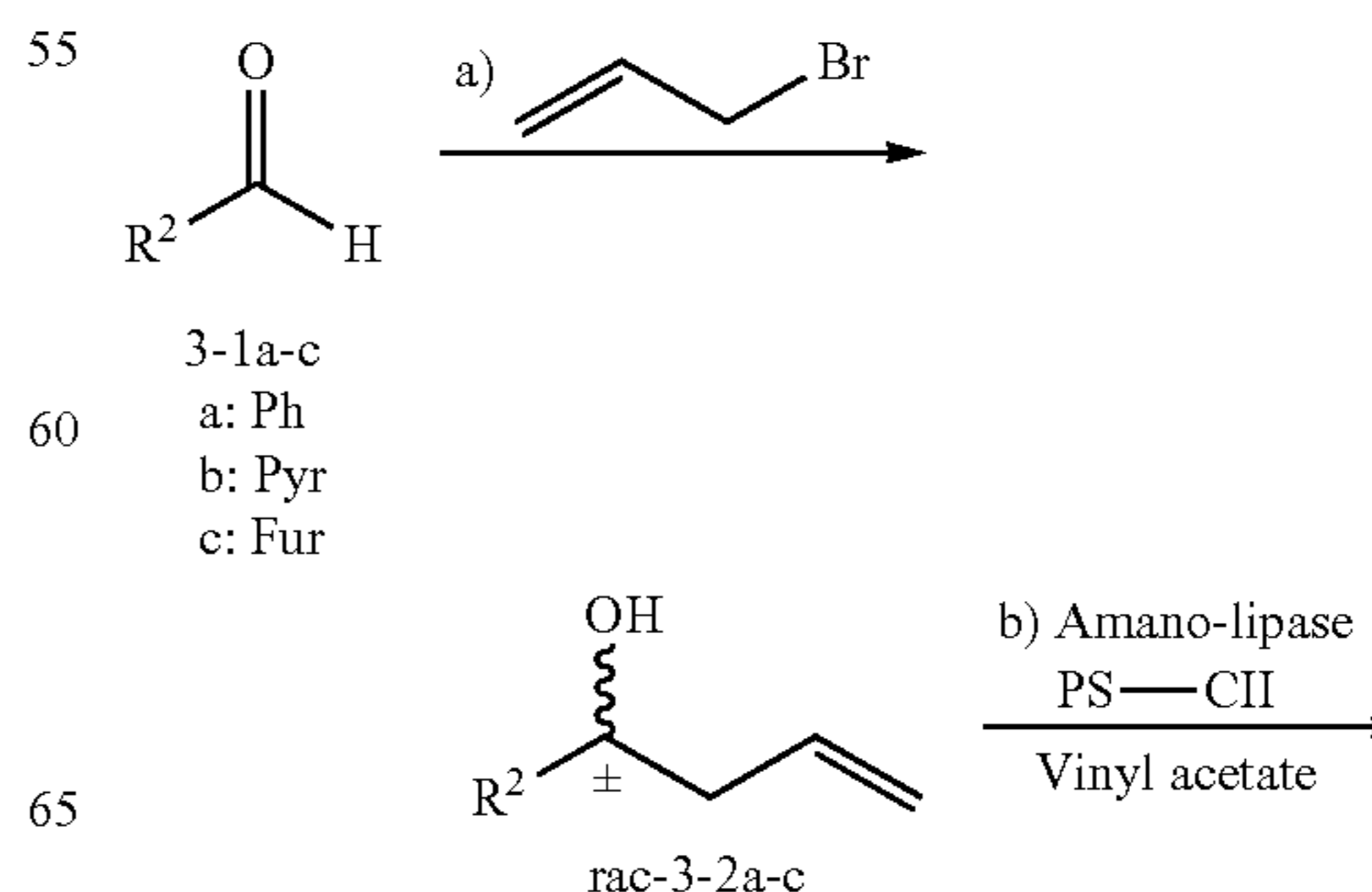
Scheme 3: Synthesis of chiral alcohols 3a-c using enzymatic resolution
