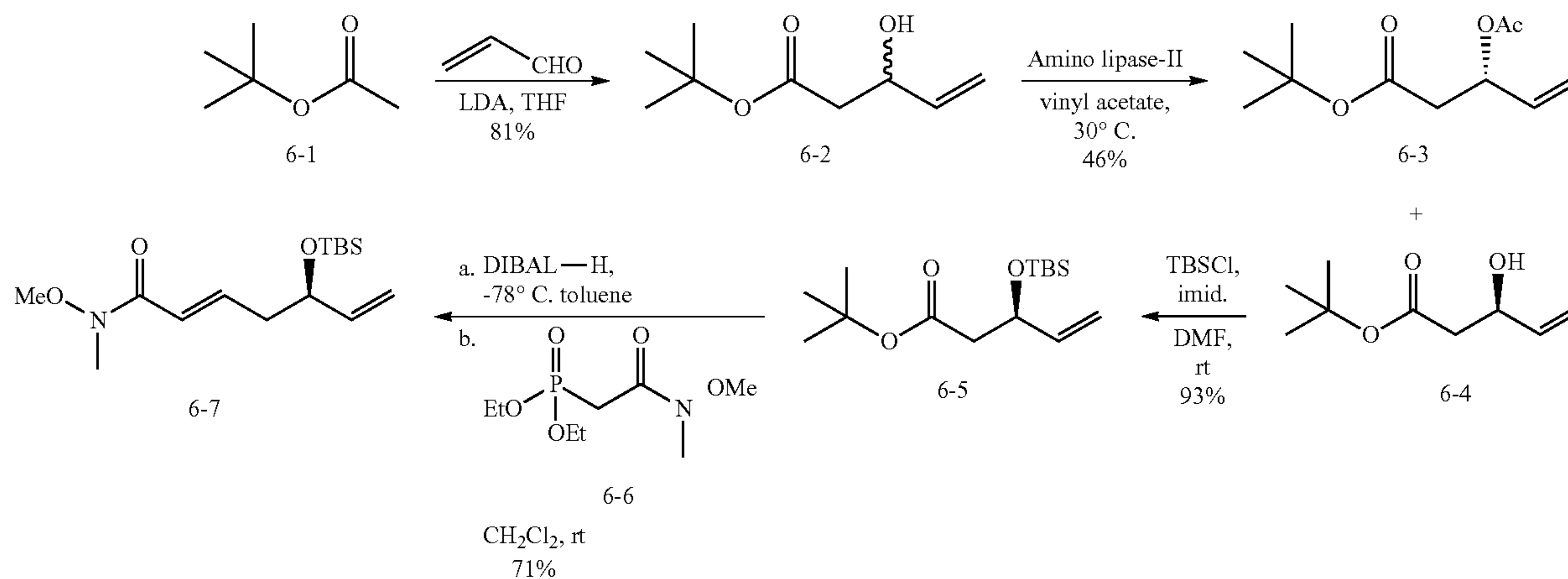
Scheme 6: Synthesis of hydroxy-substituted Weinreb amides
