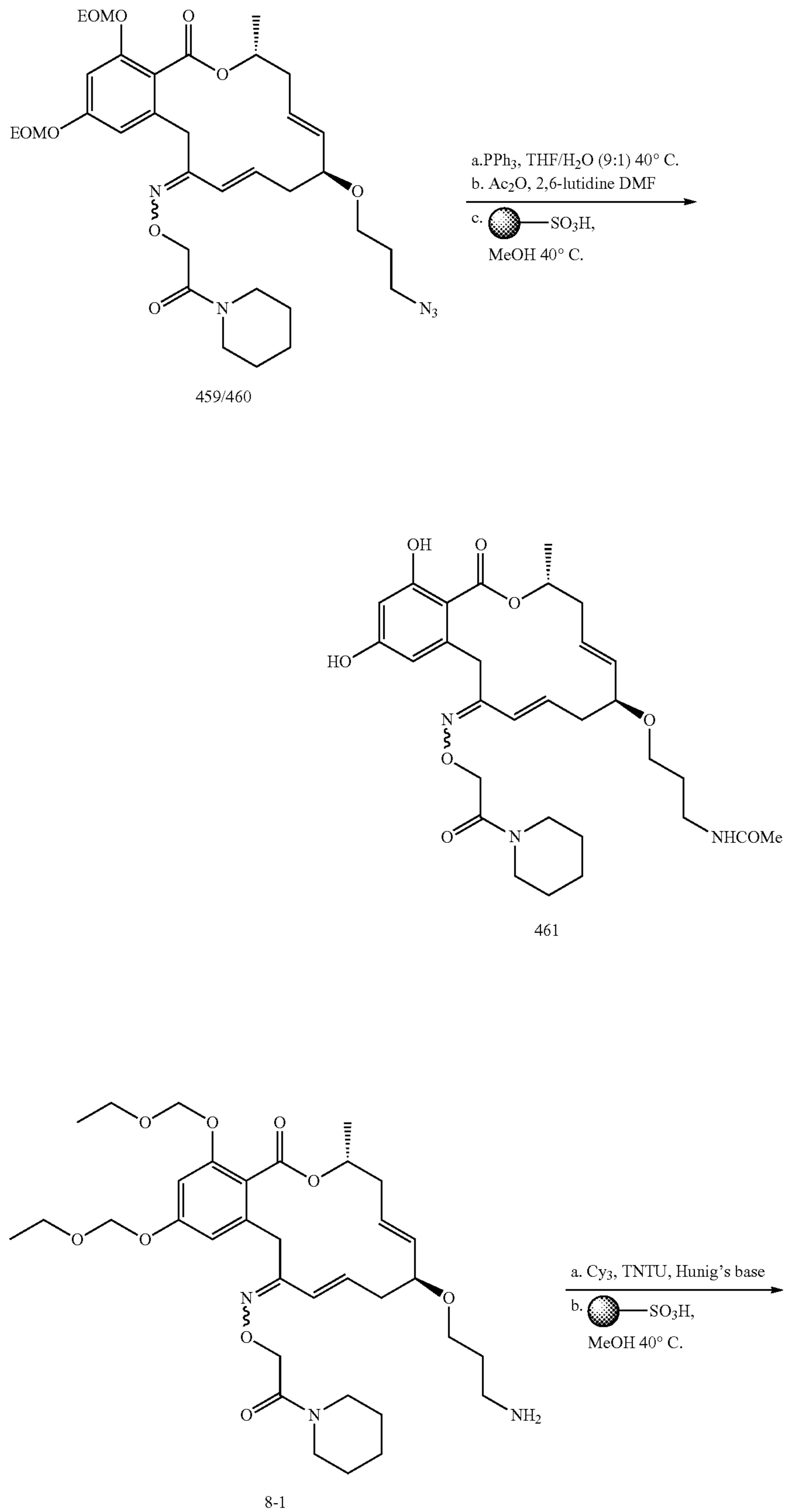
Scheme 8: Derivatization of amino-substituted macrocycles
