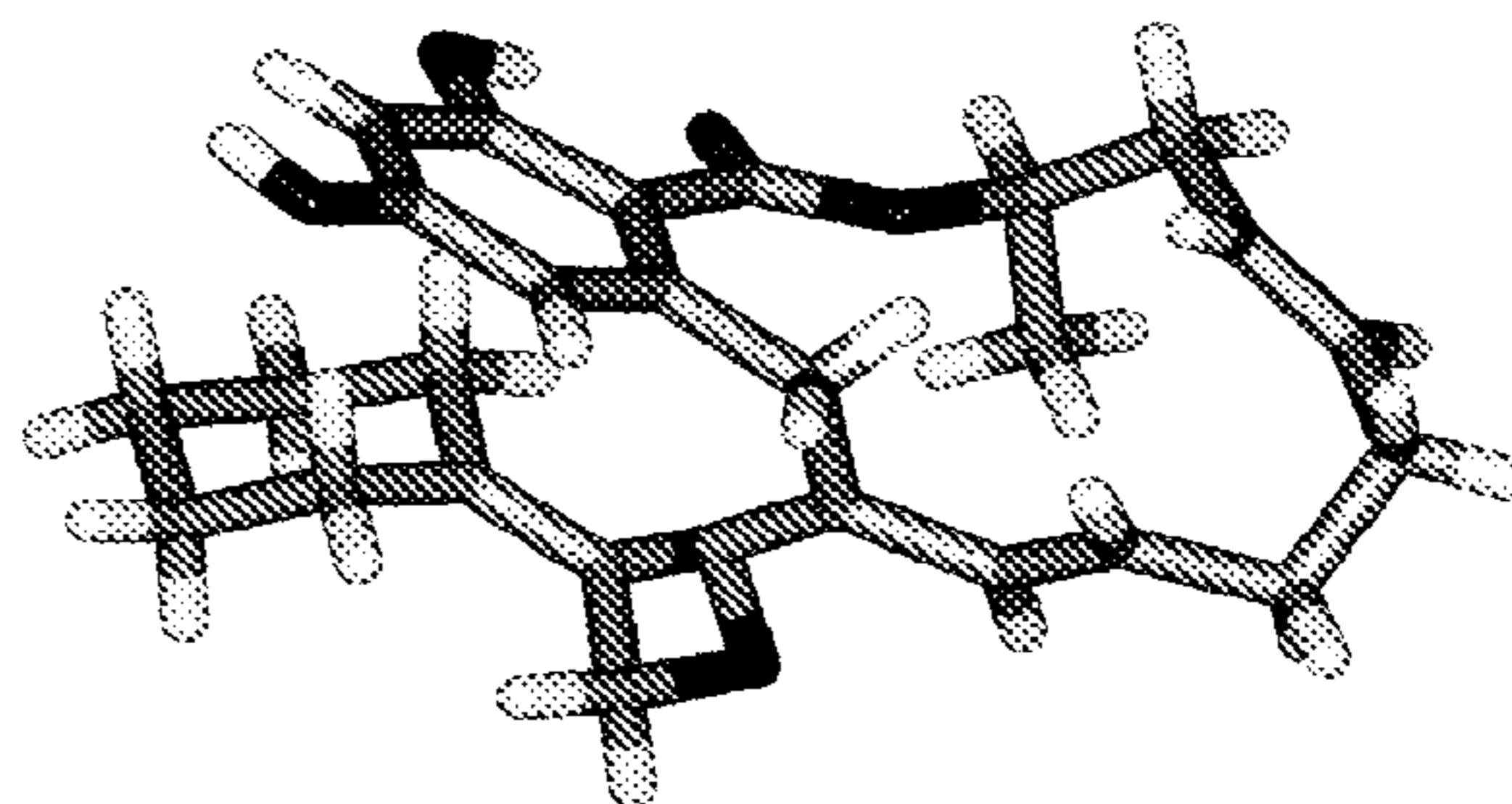
Wire-frame representation of the Z-isomer of compound 13c
