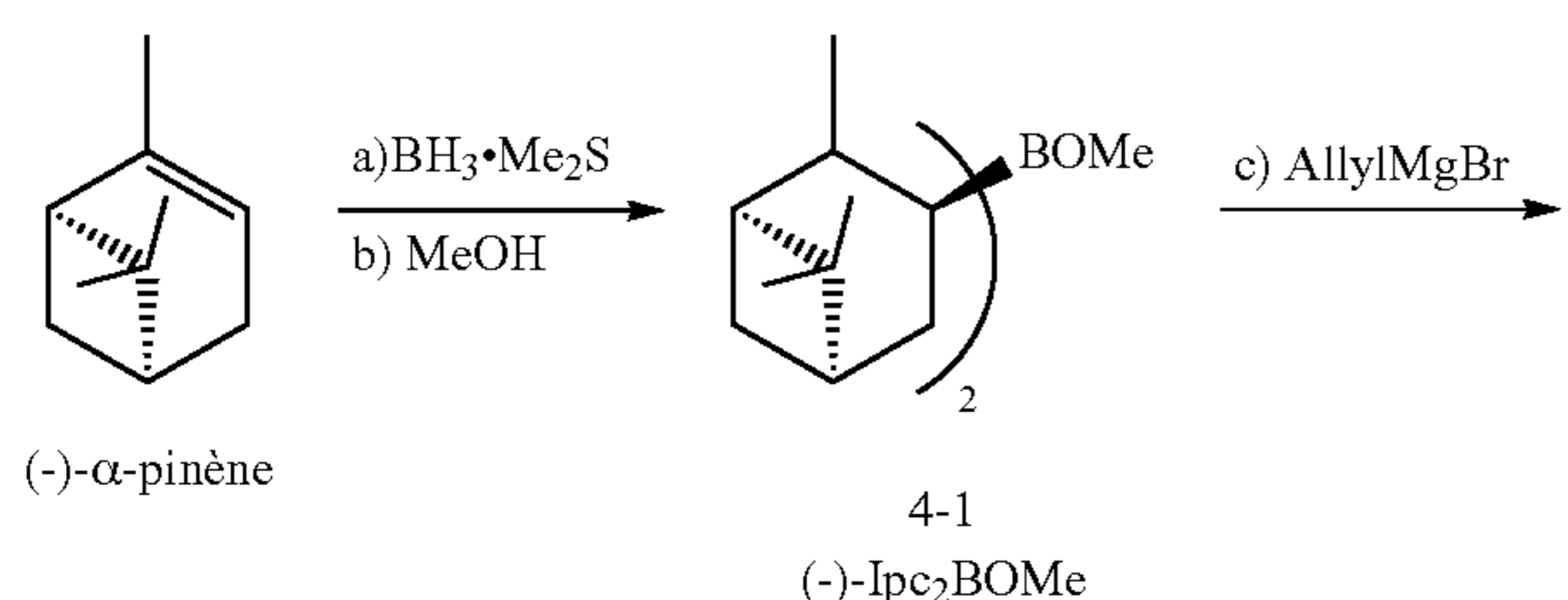
Scheme 4: Synthesis of chiral alcohols 4-3d-f using Brown allylation
