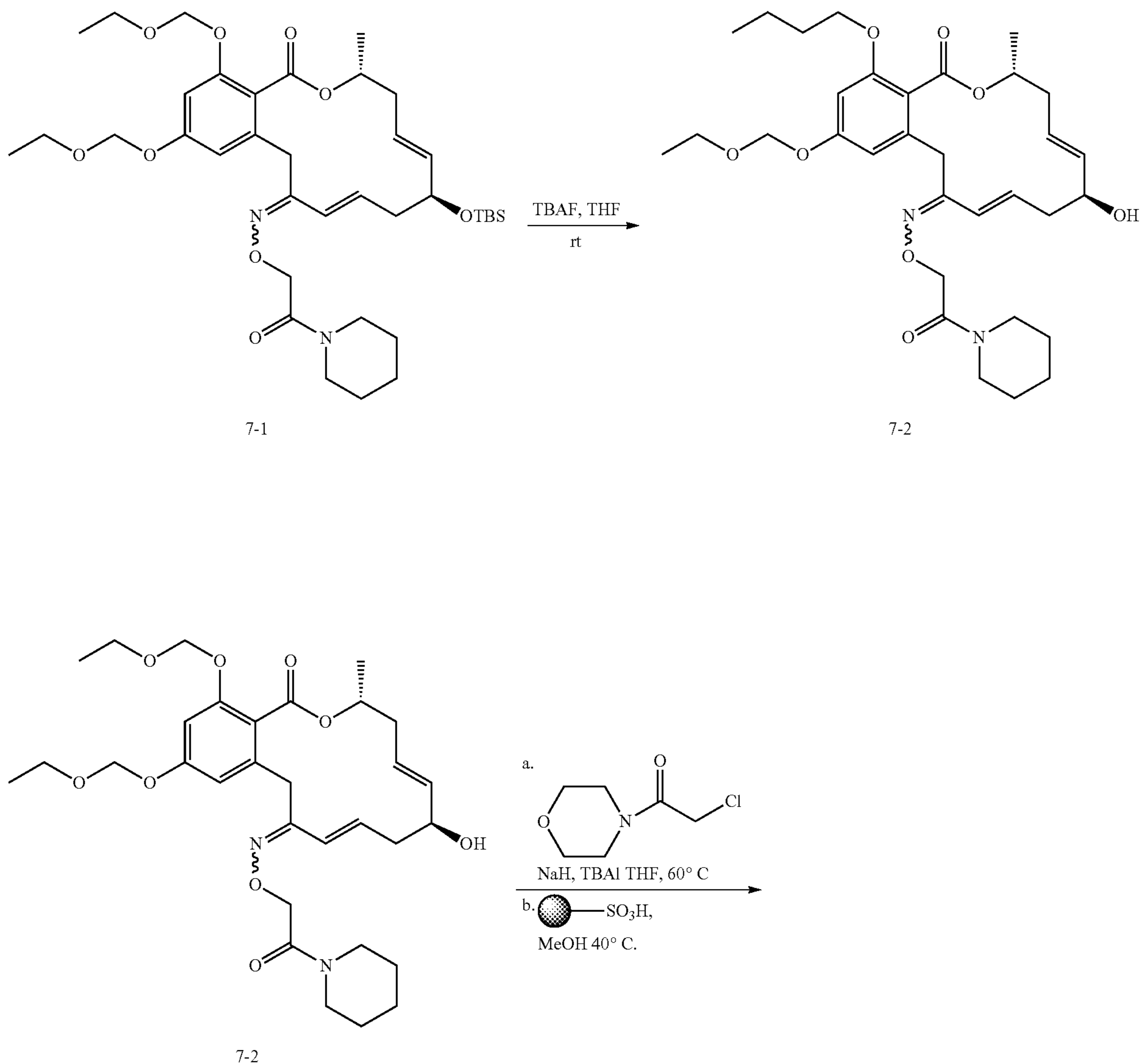
Scheme 7: Derivatives of hydroxy-substituted macrocycles
