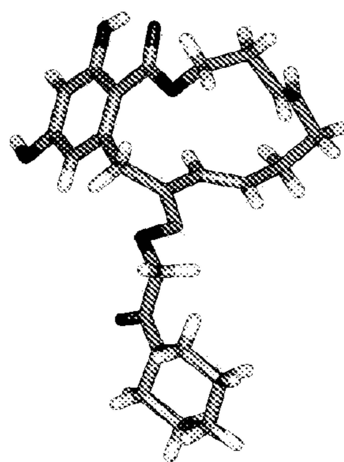
Wire-frame representation of crystal structure of compound 13b
