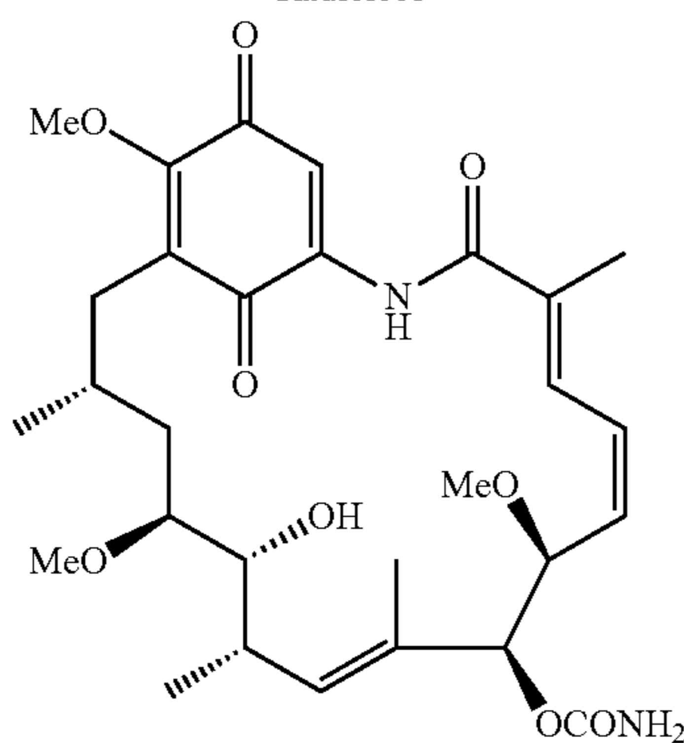
Geldanamycin
