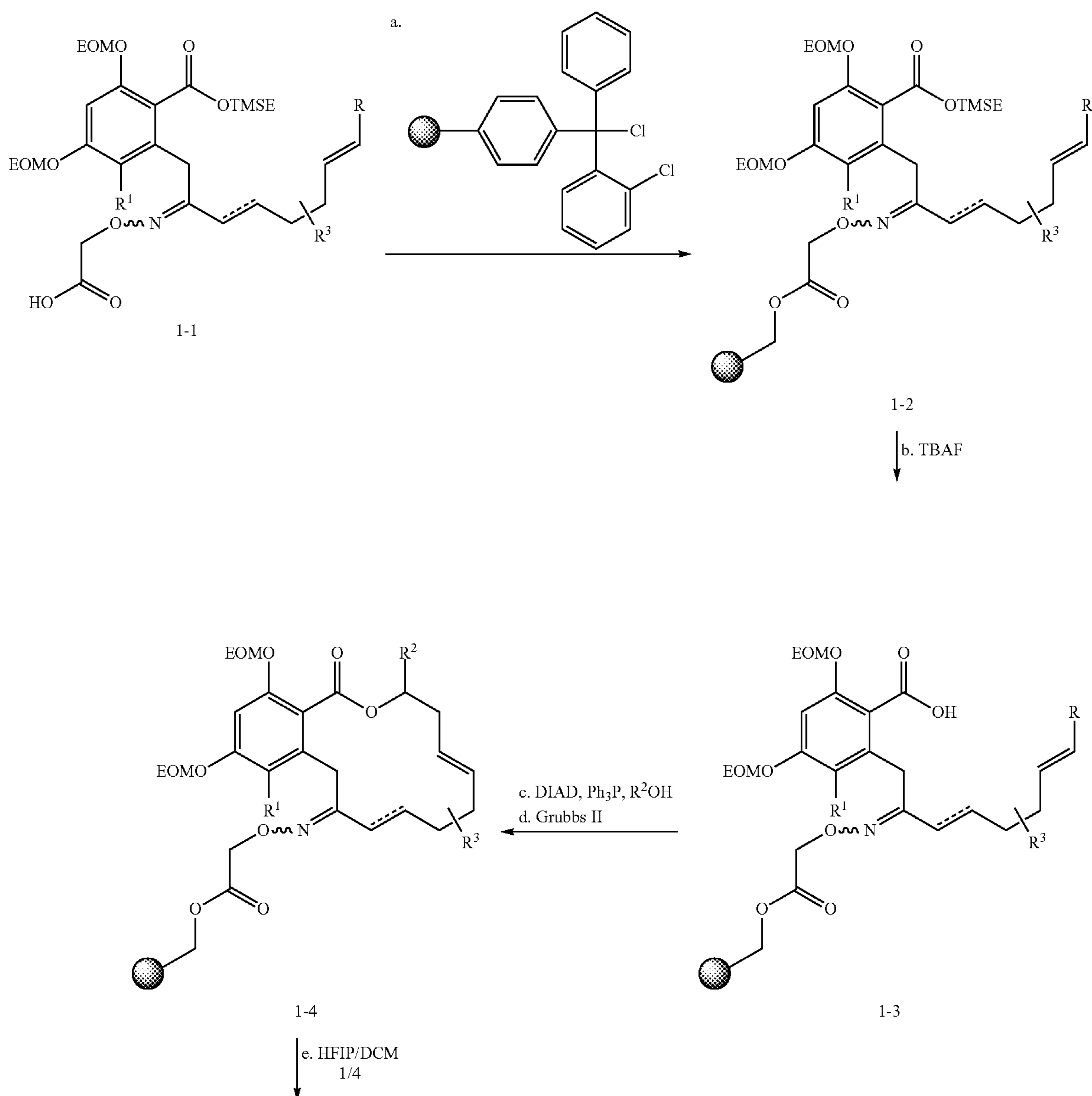
Scheme 1
