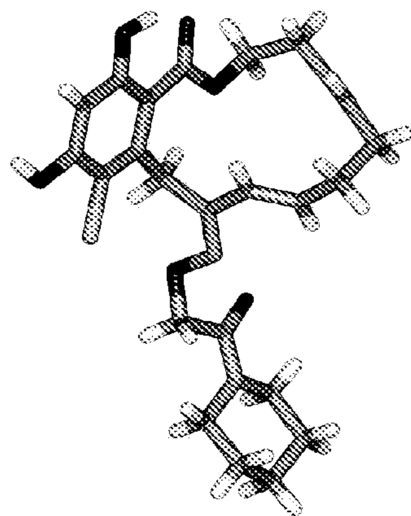
Wire-frame representation of crystal structure of compound 13a
