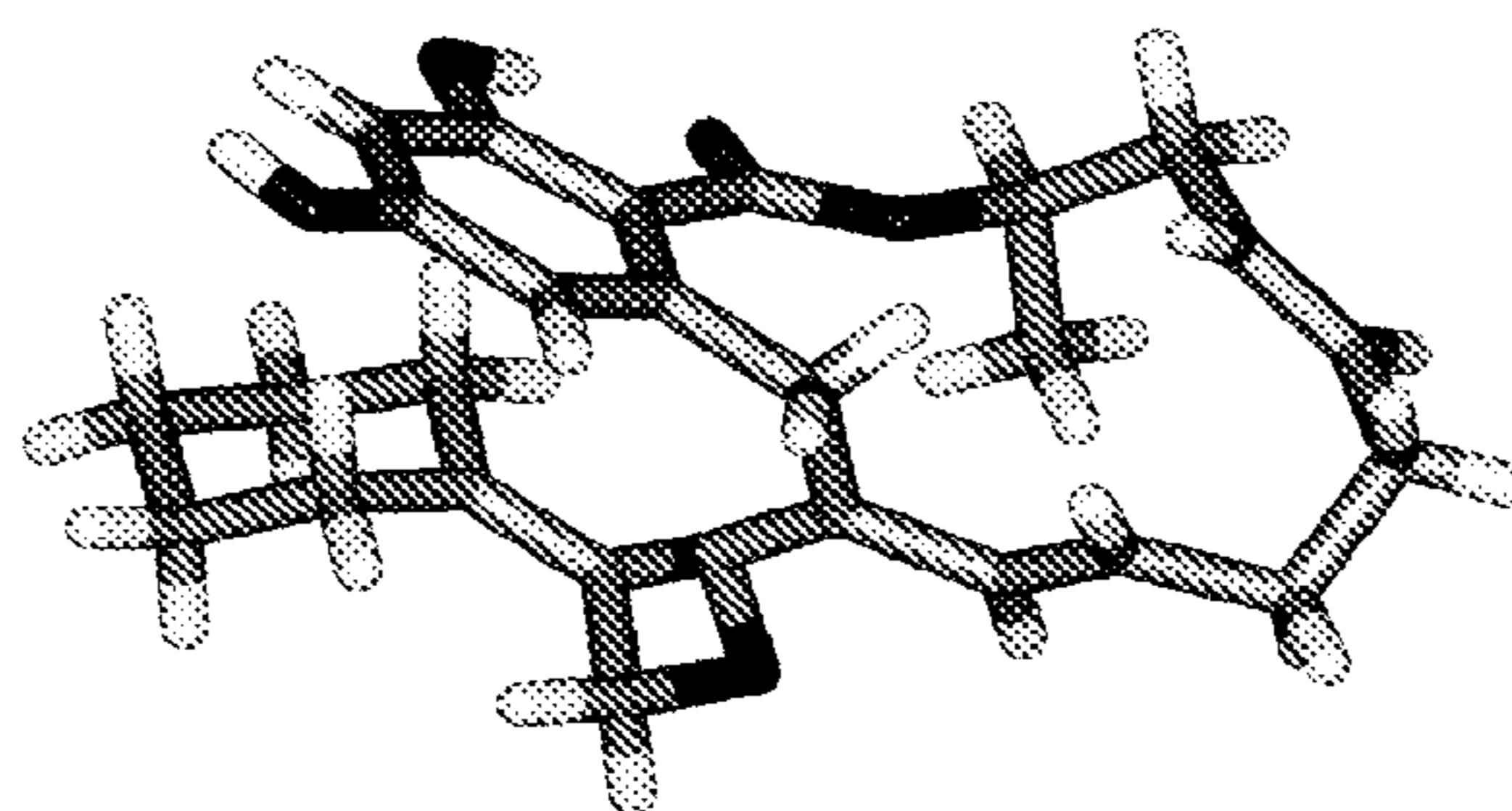
Wire-frame representation of the Z-isomer of compound 13c
