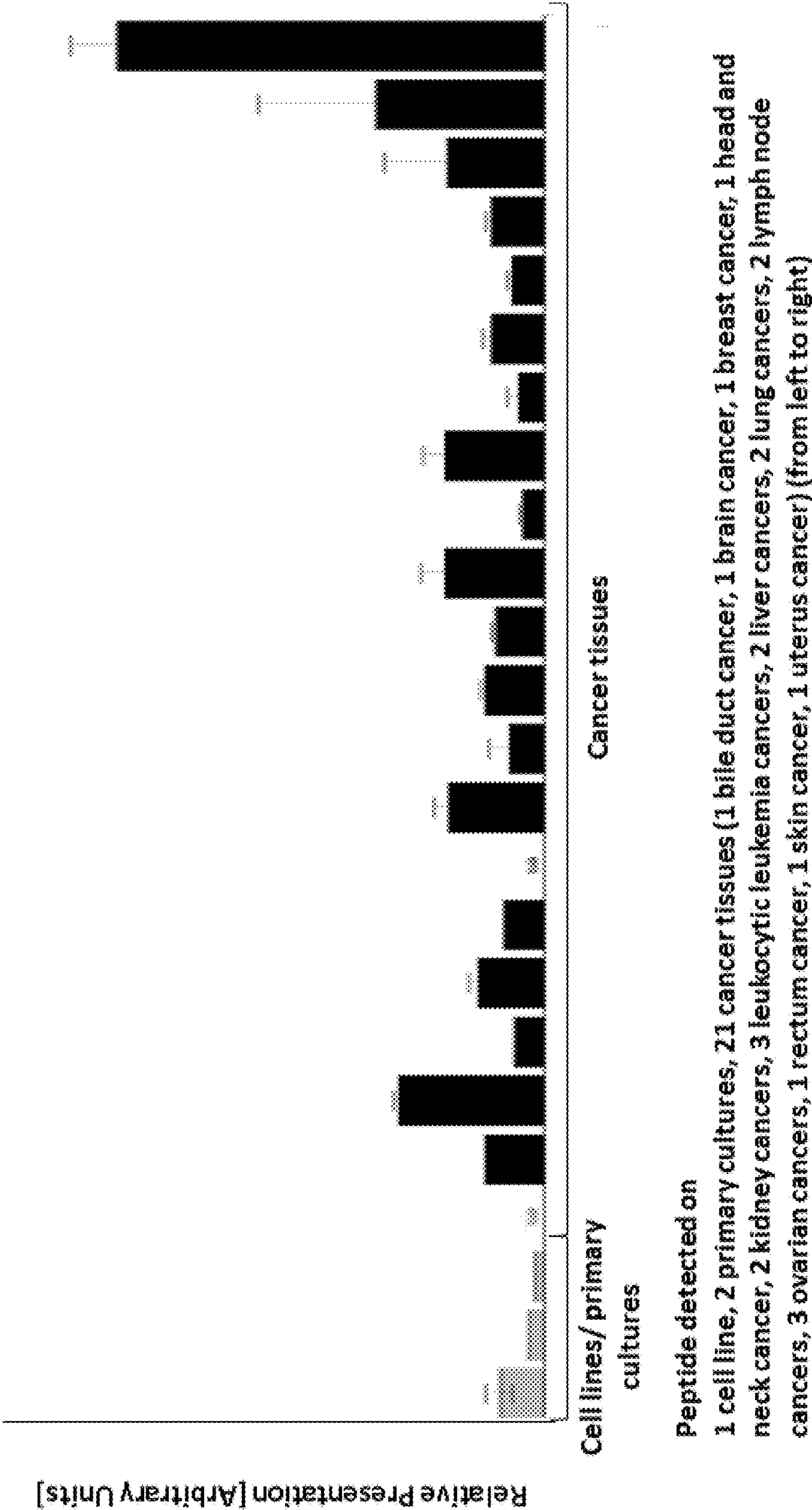
Figure 1G Peptide: GLDQQFAGLDL (A*02) SEQ ID NO: 68
