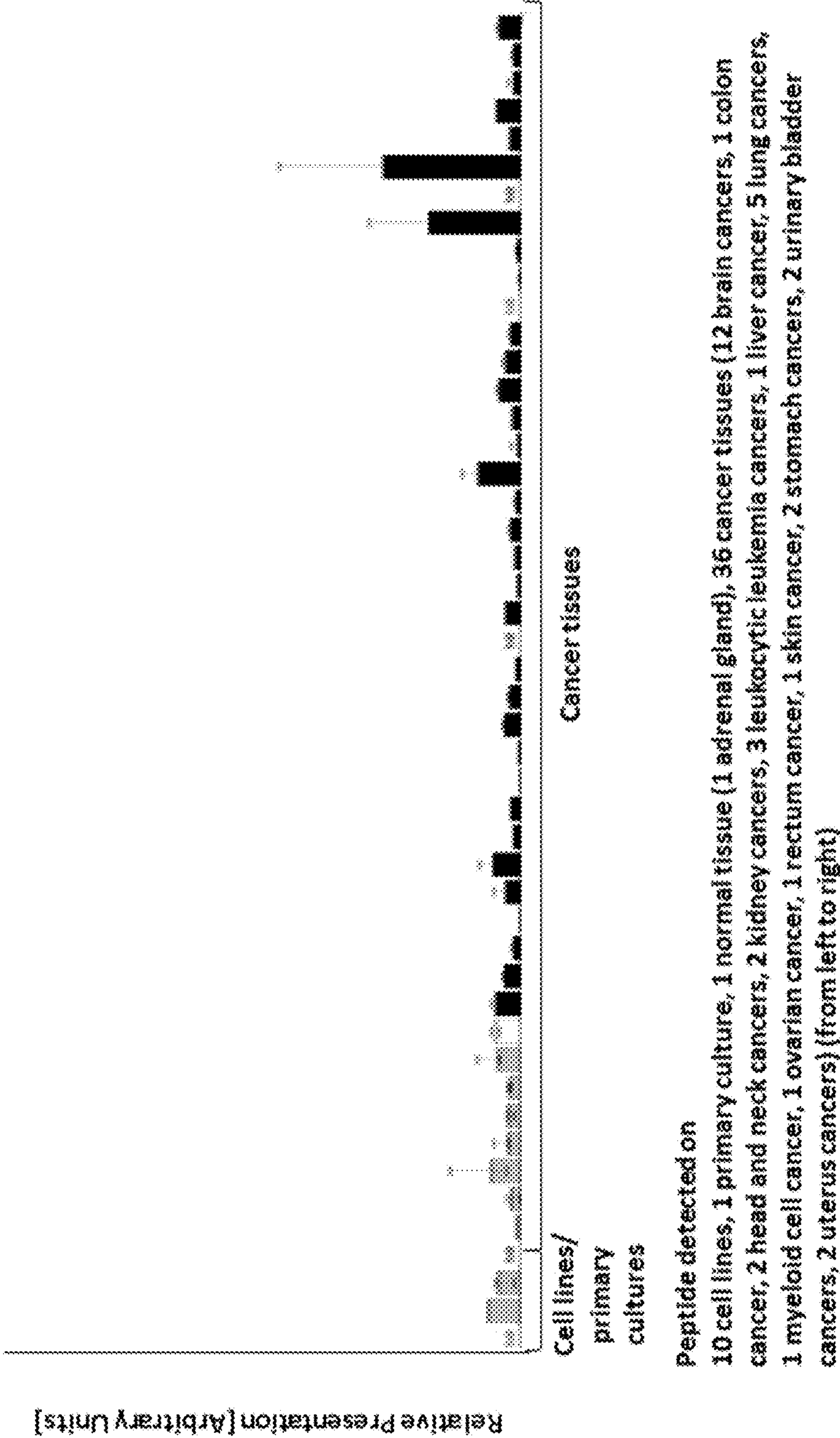
Figure 1M Peptide: SVHKGFAFV (A*02) SEQ ID NO: 164
