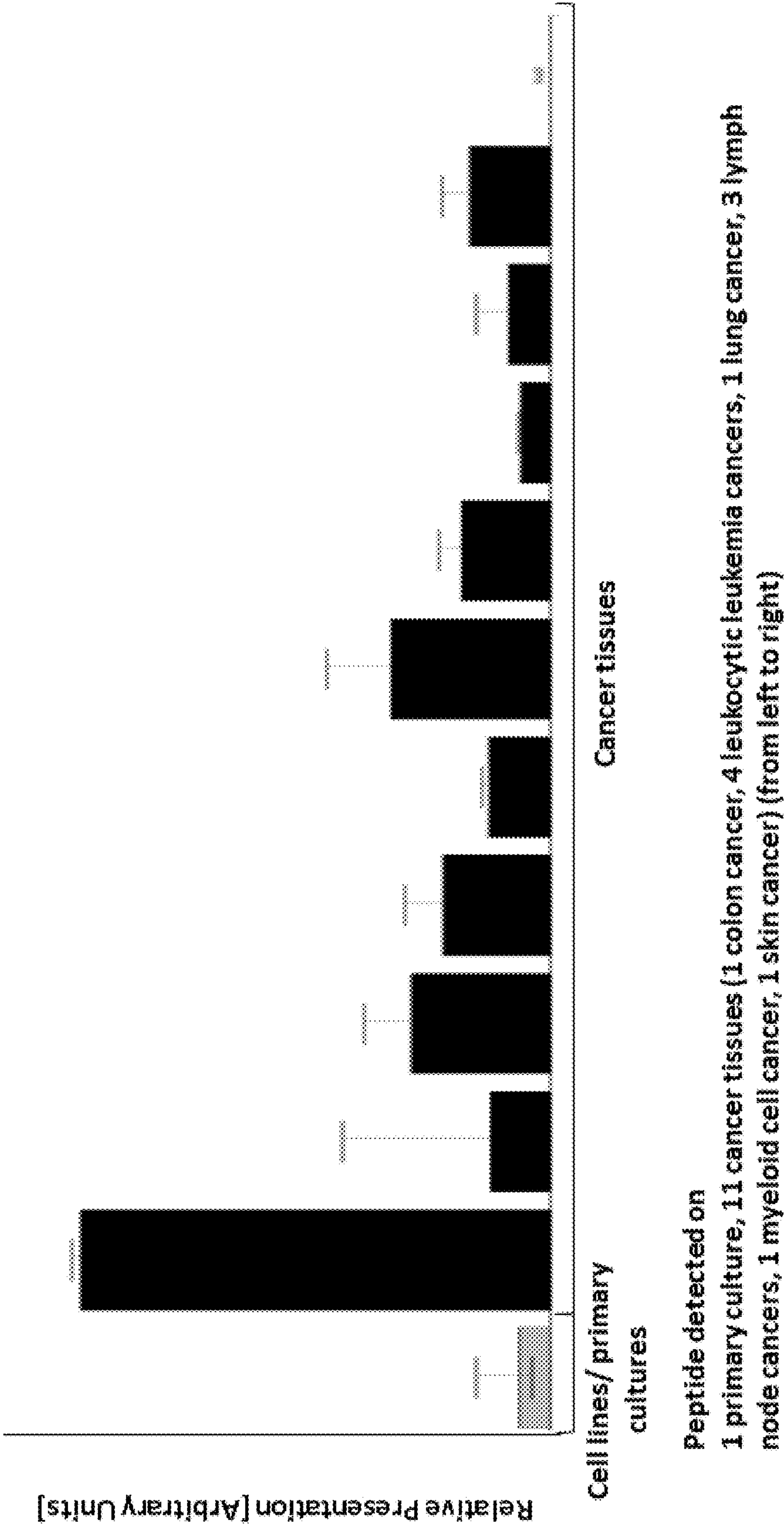
Figure 11 Peptide: SILETVATL (A*02) SEQ ID NO: 147
