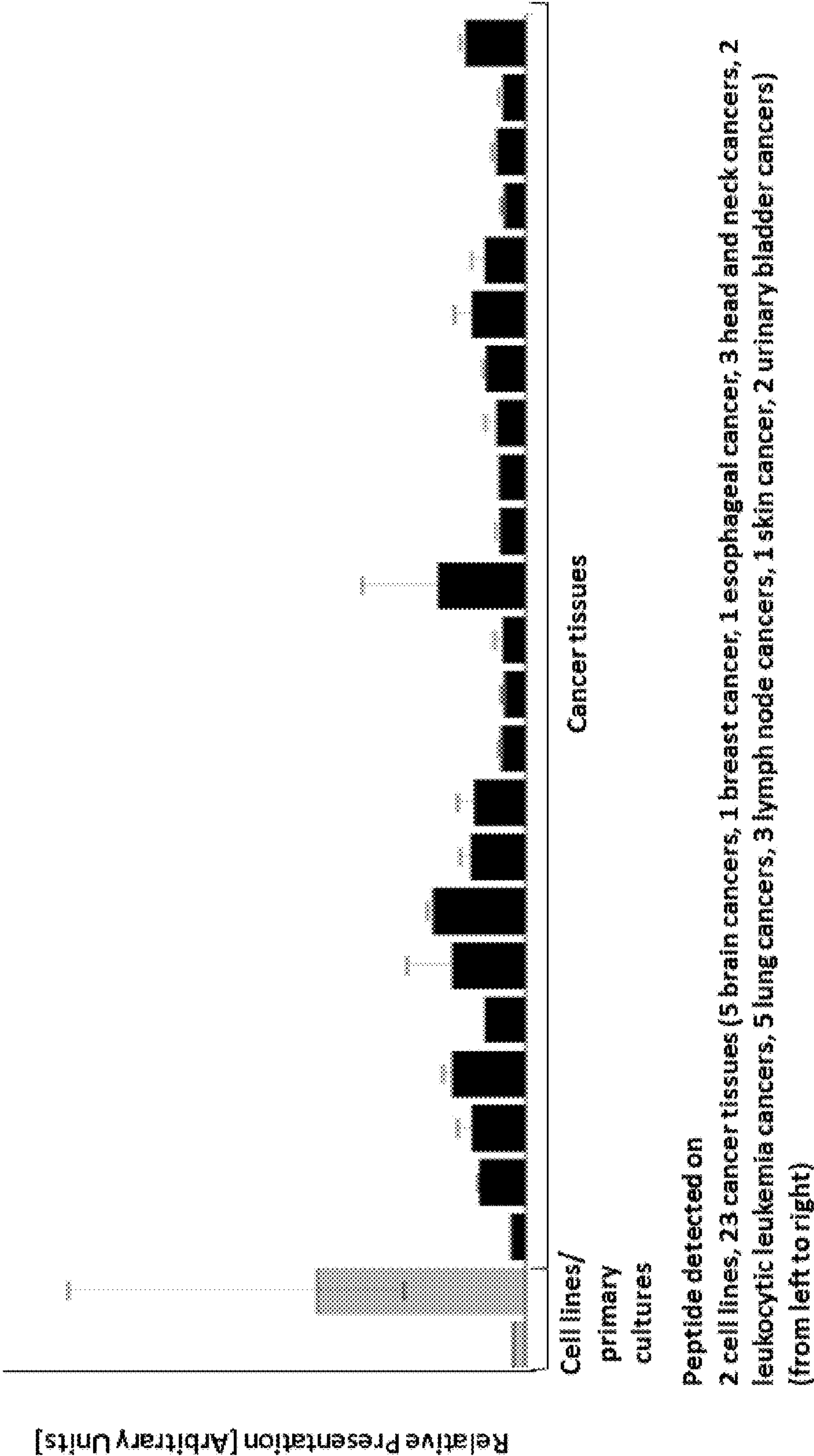
Figure 1L Peptide: SLQEEKLIYV (A*02) SEQ ID NO: 159
