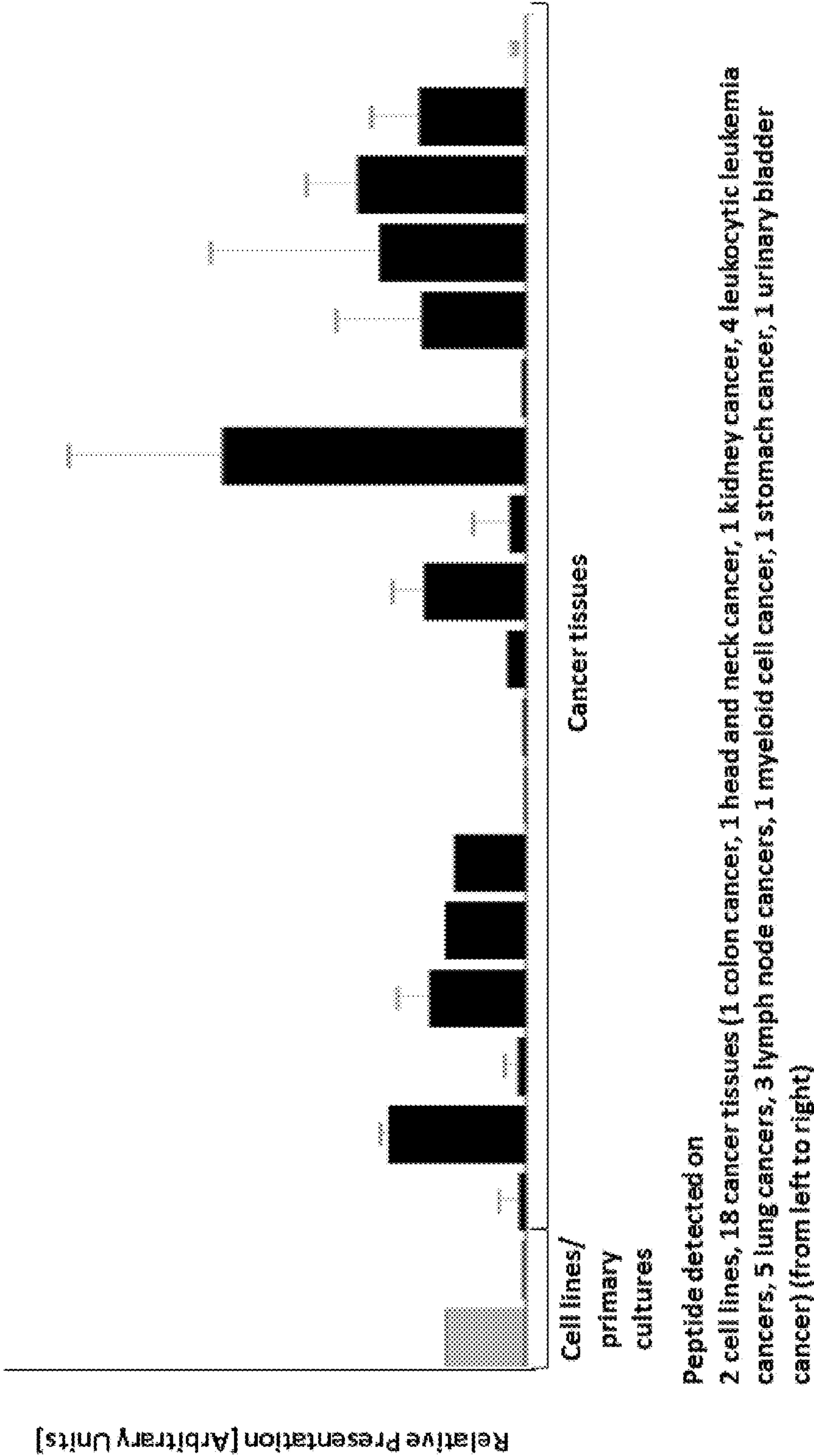
Figure 1P Peptide: YIQEYLTLL (A*02) SEQ ID NO: 192
