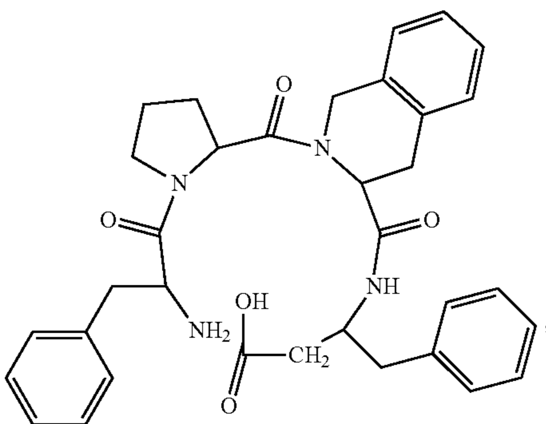
(H-Phe-Pro-Tic-β 3 hoPhe-OH)
