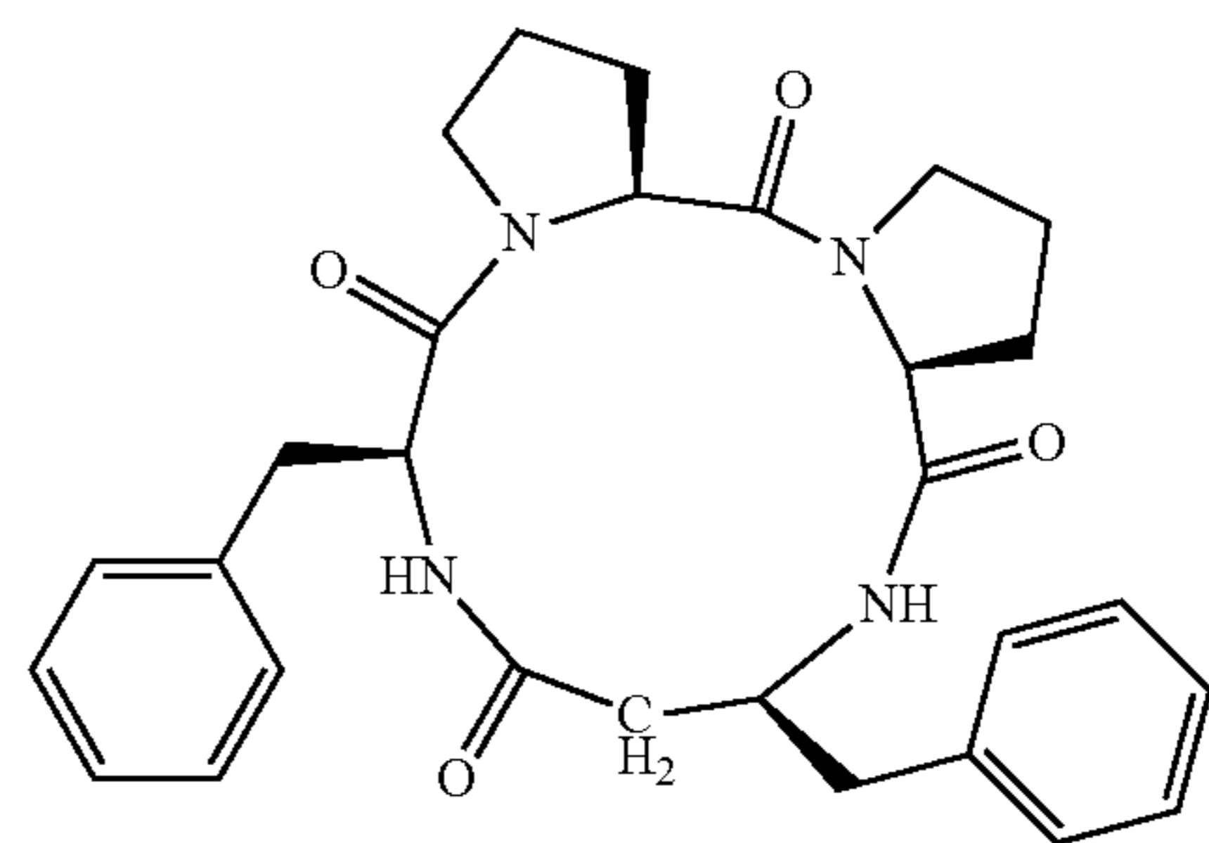
((cyclo(-L-Pro-L-Pro-L-β³hoPhe-L-Phe-)))
