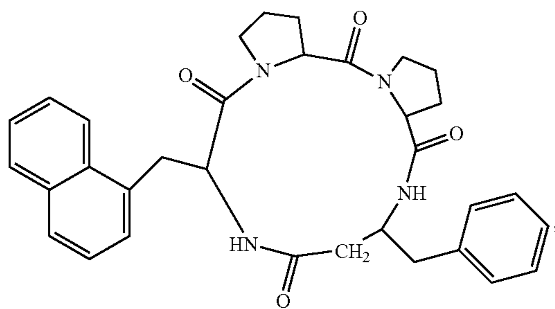
(cyclo(-Pro-Pro-β³hoPhe-1Nal))
