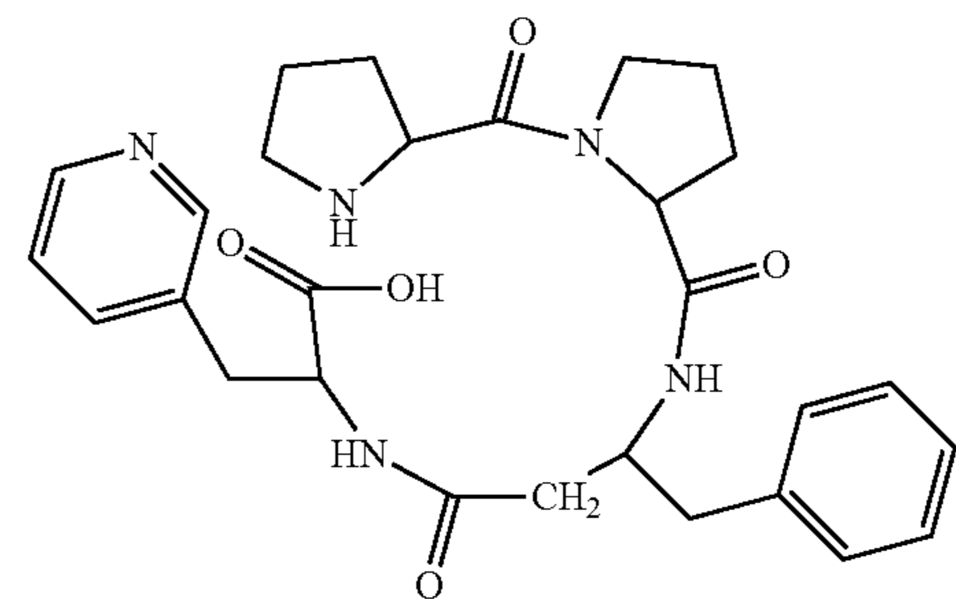
(H-Pro-Pro-β 3 hoPhe-Pal-OH)
