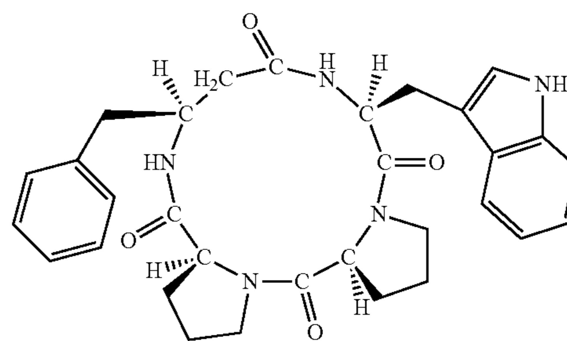
(cyclo(-L-Pro-L-Pro-L-β 3 HoPhe-L-Trp-))
