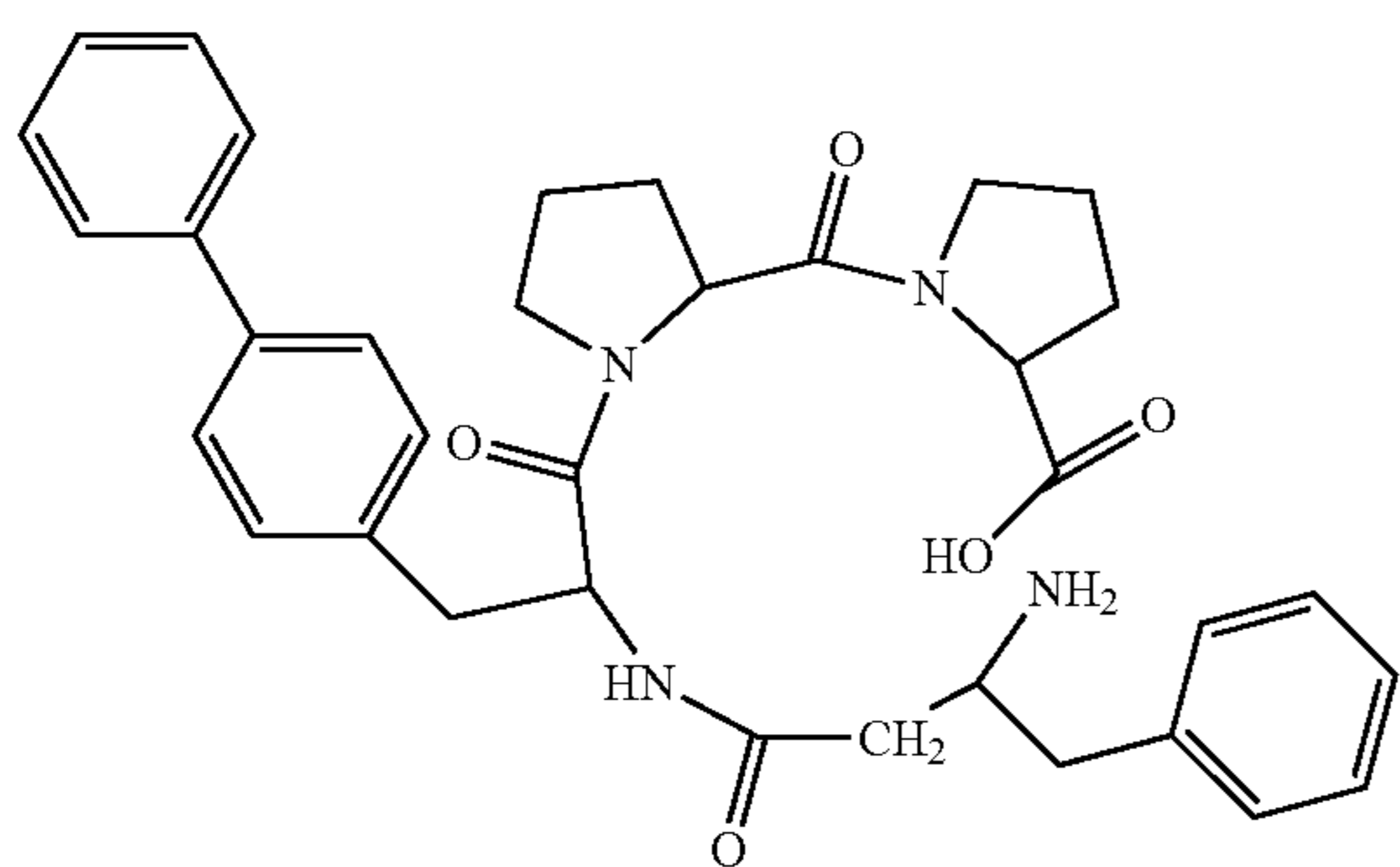
(H-β³hoPhe-Bip-Pro-Pro-OH)
