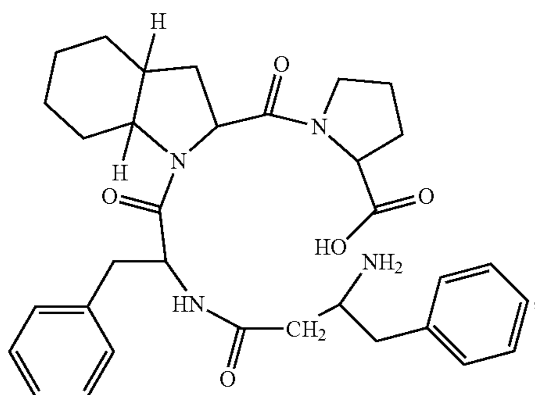
(H-β 3 hoPhe-Phe-Oic-Pro-OH)
