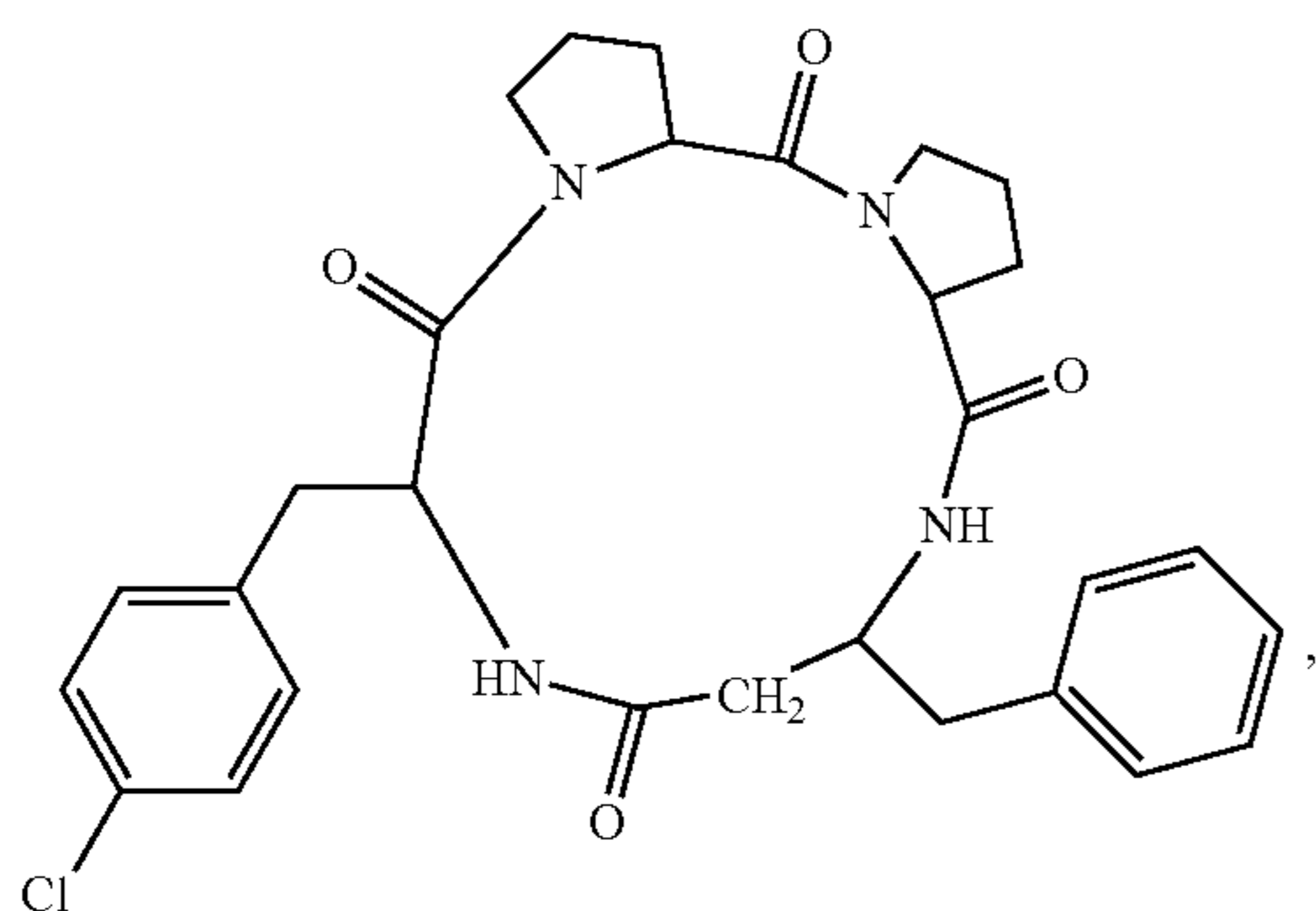
(cyclo(-Pro-Pro-β 3 hoPhe-Phe(4Cl)))
