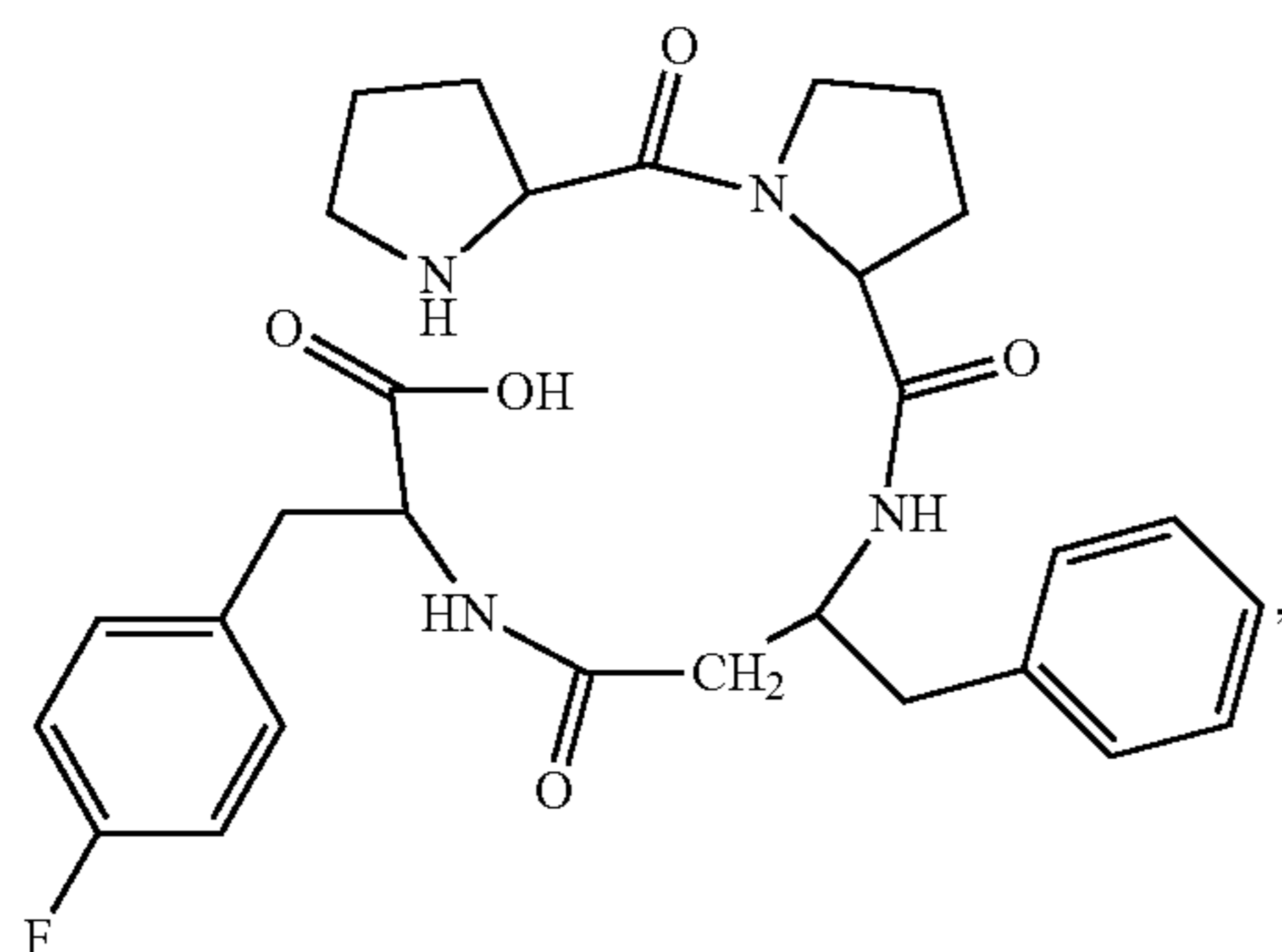
(H-Pro-Pro-β 3 hoPhe-Phe(4F)-OH)
