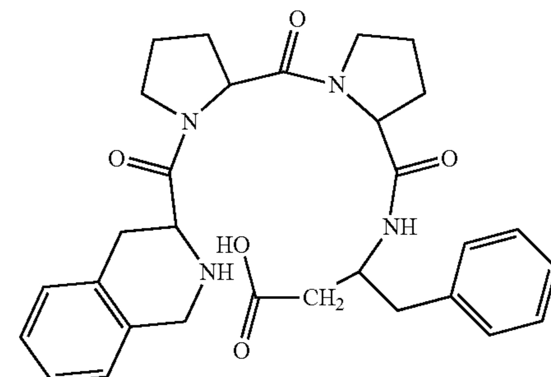
(H-Tic-Pro-Pro-β 3 hoPhe-OH)
