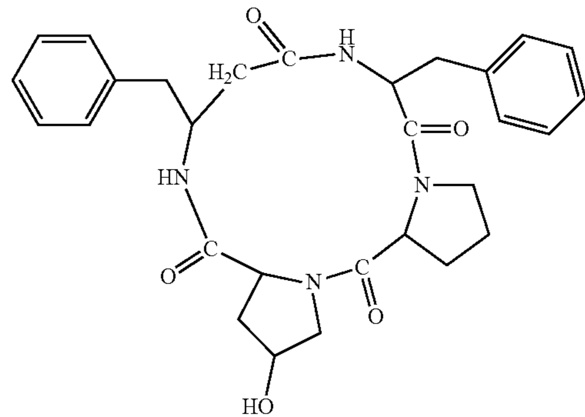
(cyclo(-Pro-Hyp-β³hoPhe-Phe-))
