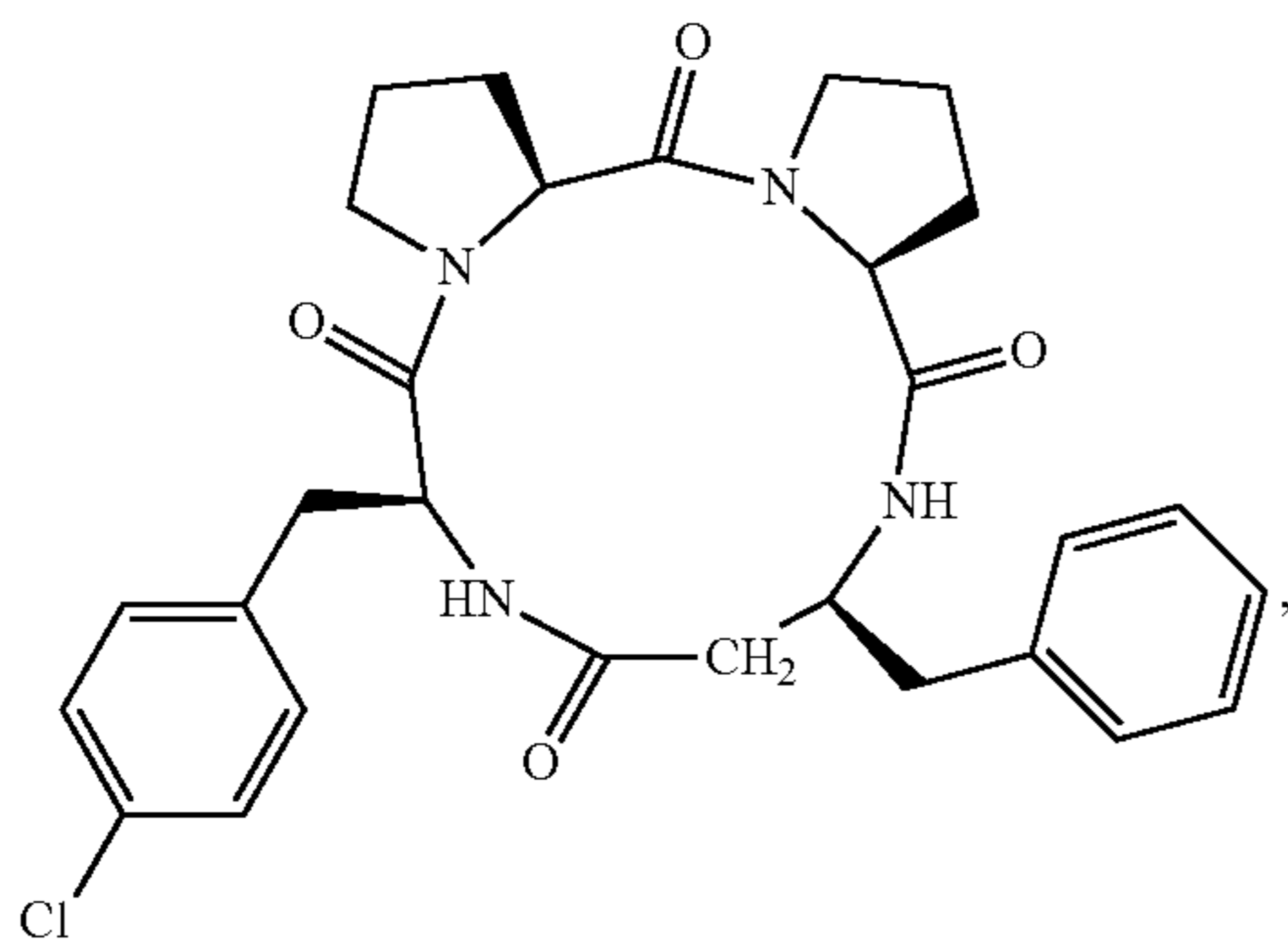
(cyclo(-L-Pro-L-Pro-L-β³hoPhe-L-Phe(4Cl)))
