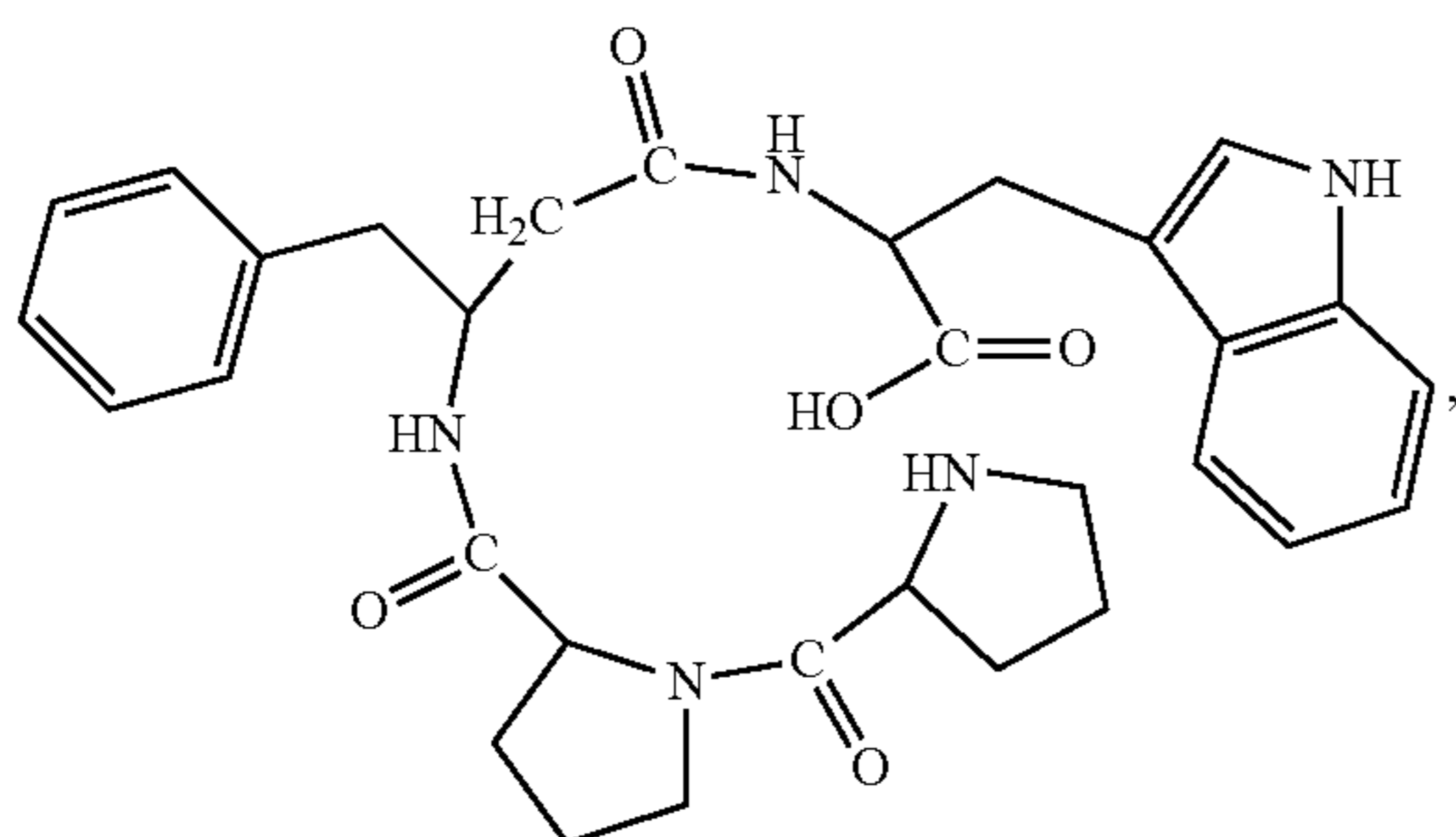
(H-Pro-Pro-β 3 hoPhe-Trp-OH)
