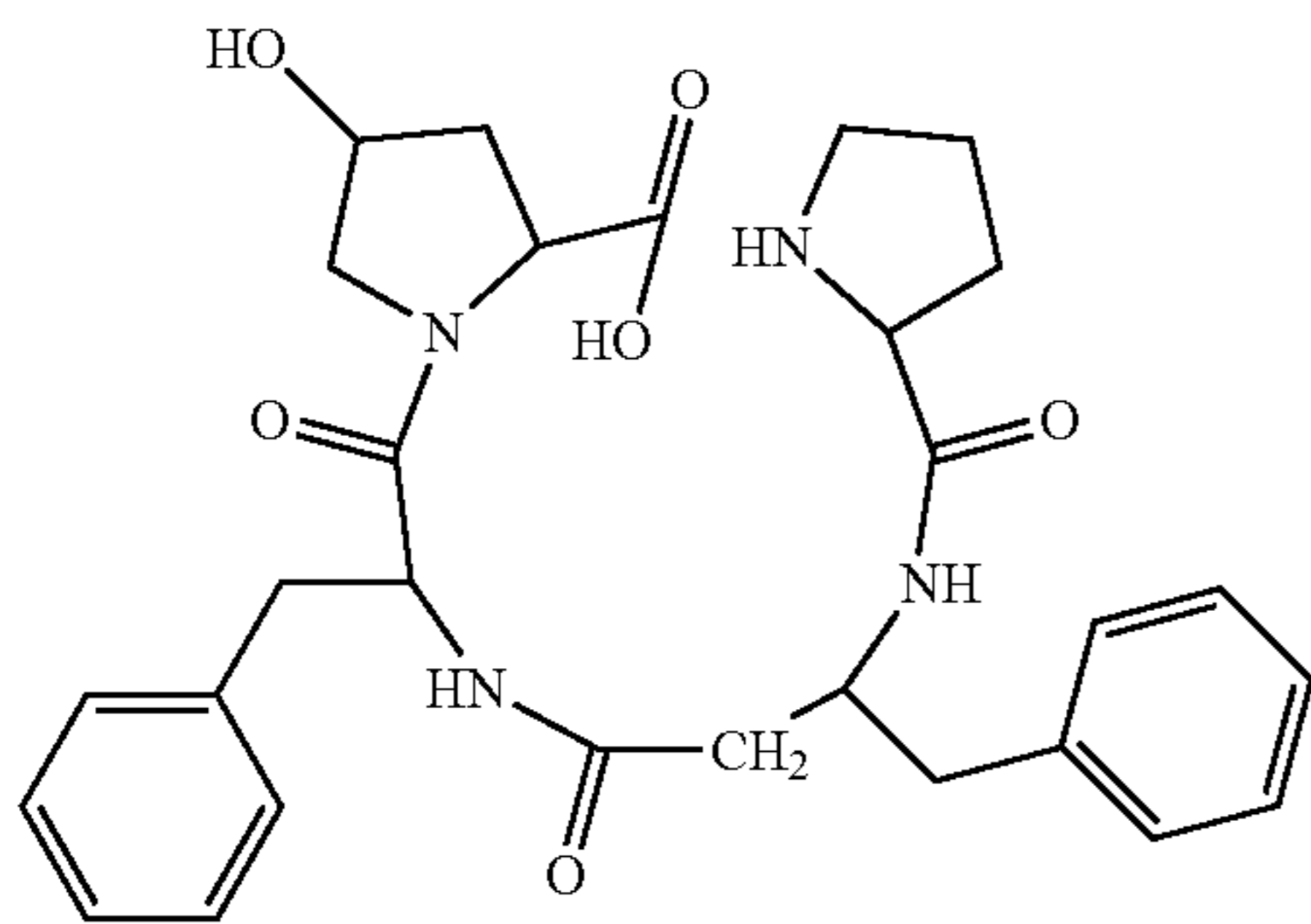
(H-Pro-β³hoPhe-Phe-Hyp-OH)
