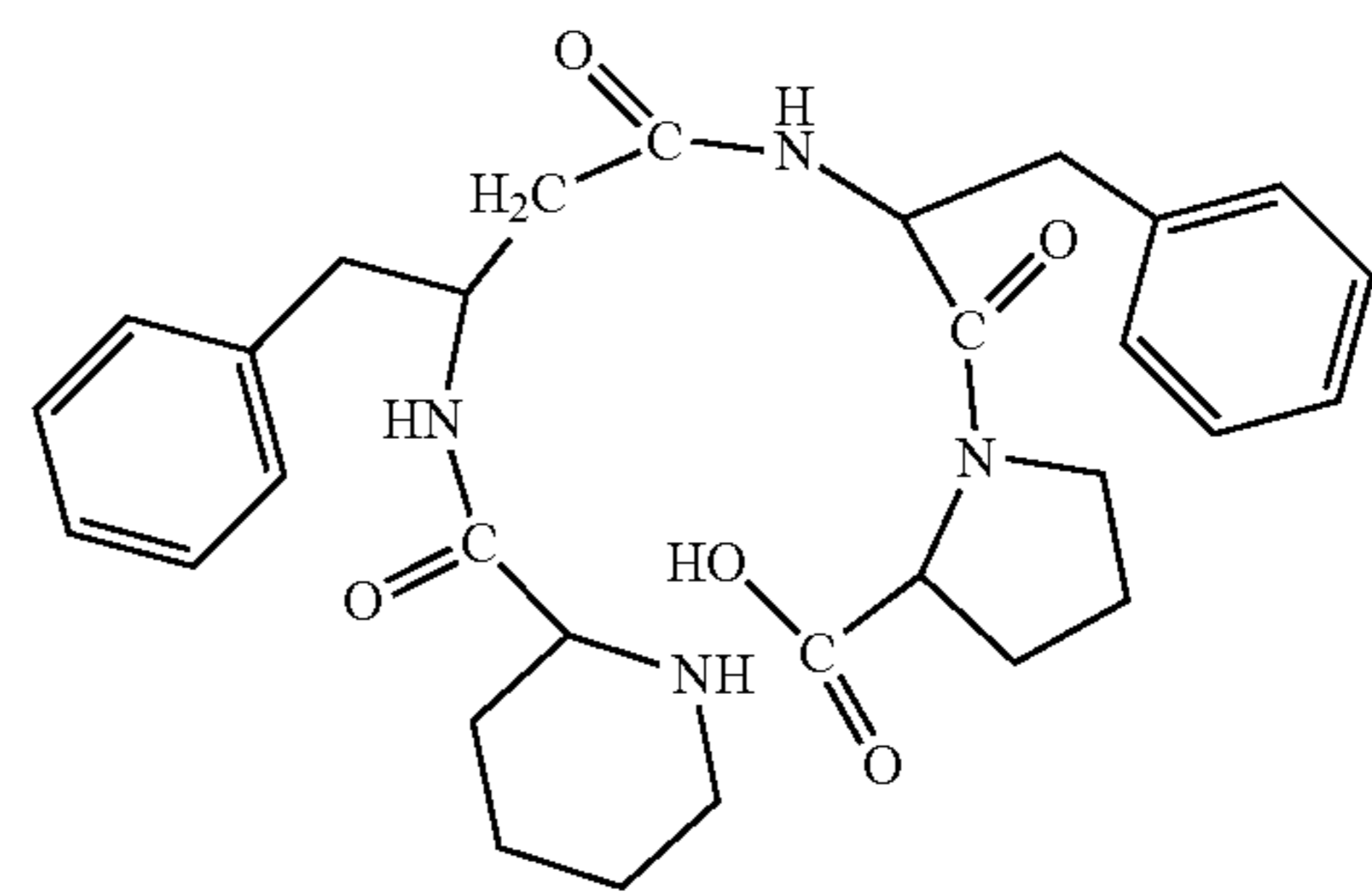
(H-Pip-β 3 hoPhe-Pre-Pro-OH)
