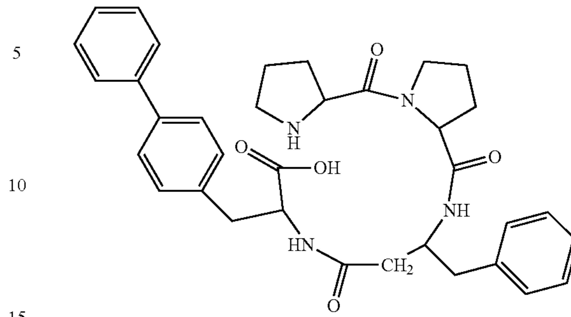
(H-Pro-Pro-β³hoPhe-Bip-OH)
