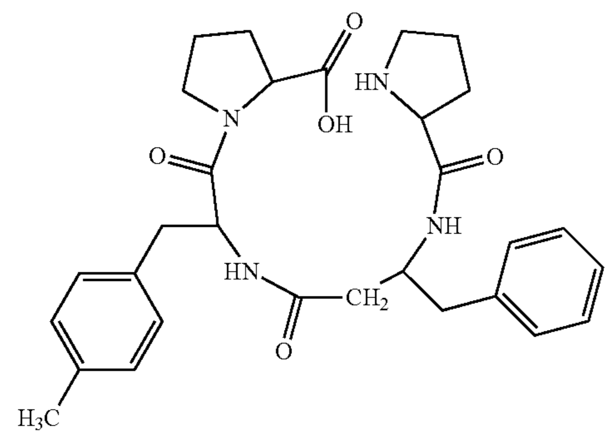
(H-Pro-β 3 hoPhe-Phe(4Me)-Pro-OH)
