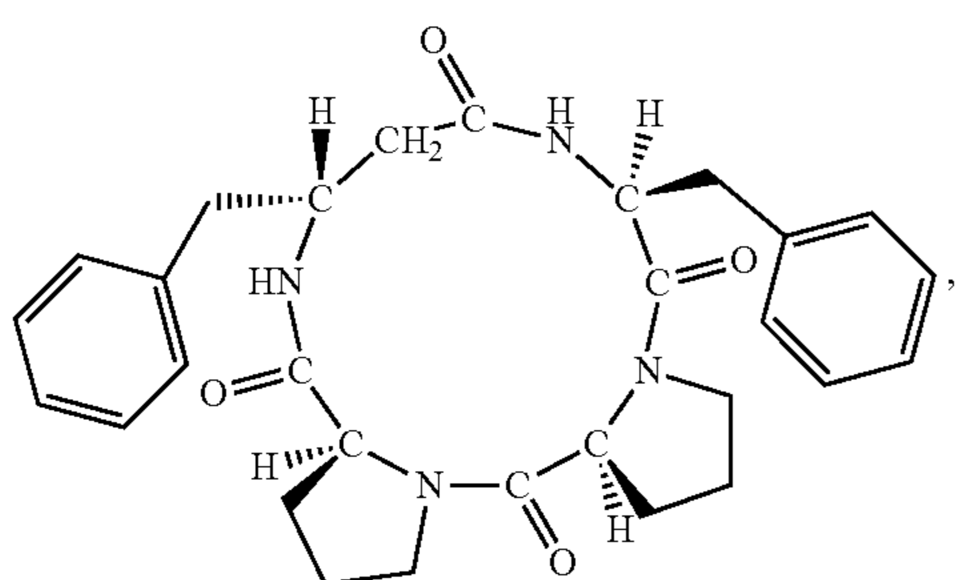
(cyclo(-L-Pro-L-Pro-D-β 3 HoPhe-L-Phe-))
