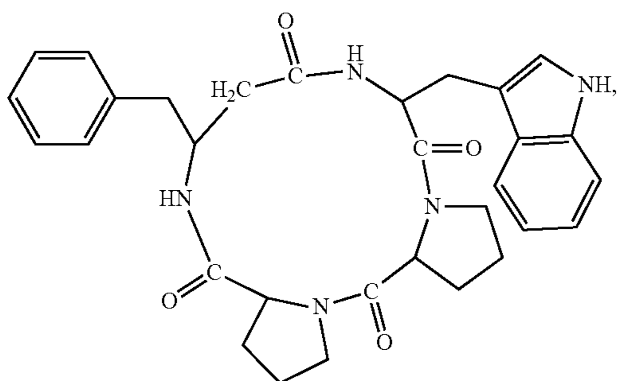
(cyclo(-Pro-Pro-β³hoPhe-Trp-))
