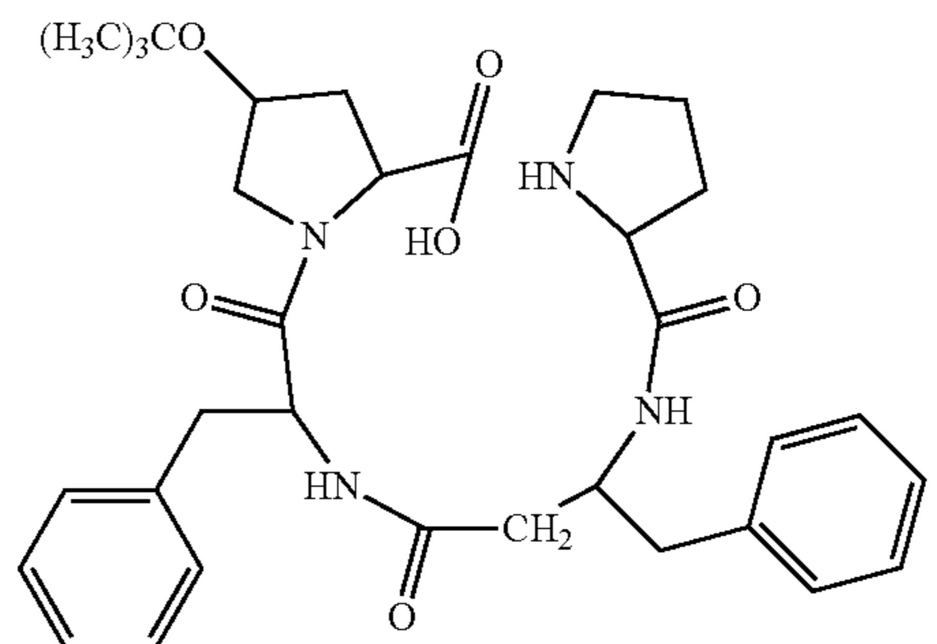
(H-Pro-β 3 hoPhe-Phe-Hyp(tBu)-OH)
