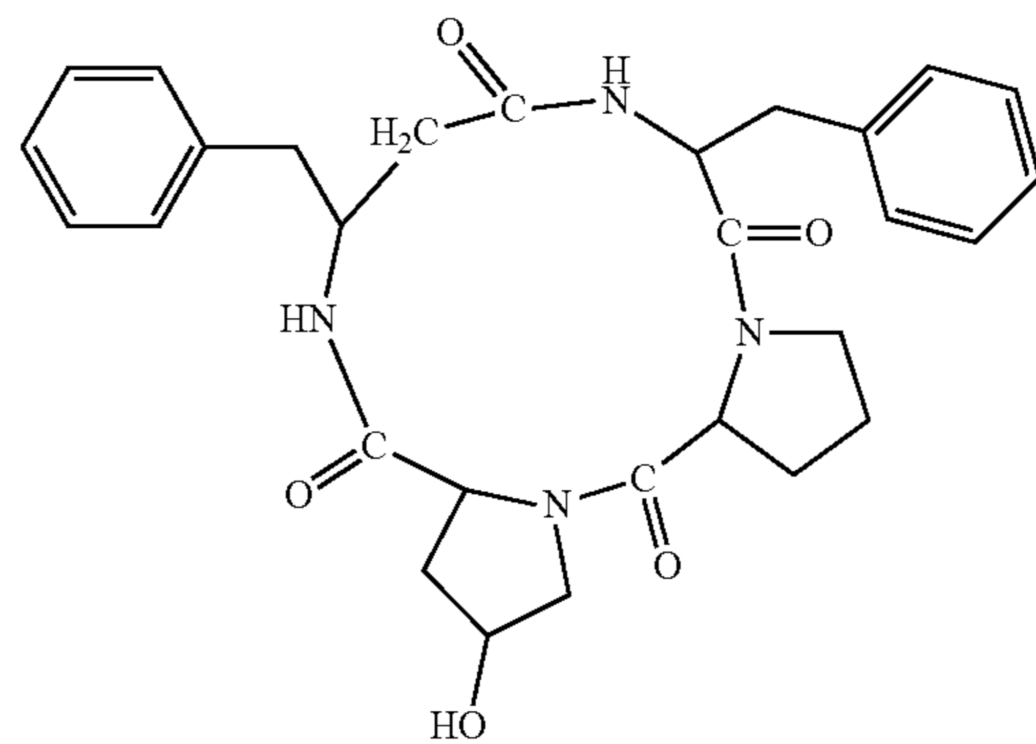
(cyclo(-Pro-Hyp-β 3 hoPhe-Phe-))
