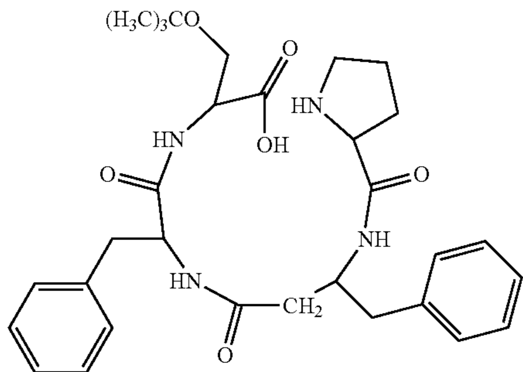
(H-Pro-β³hoPhe-Phe-Ser(tBu)-OH)
