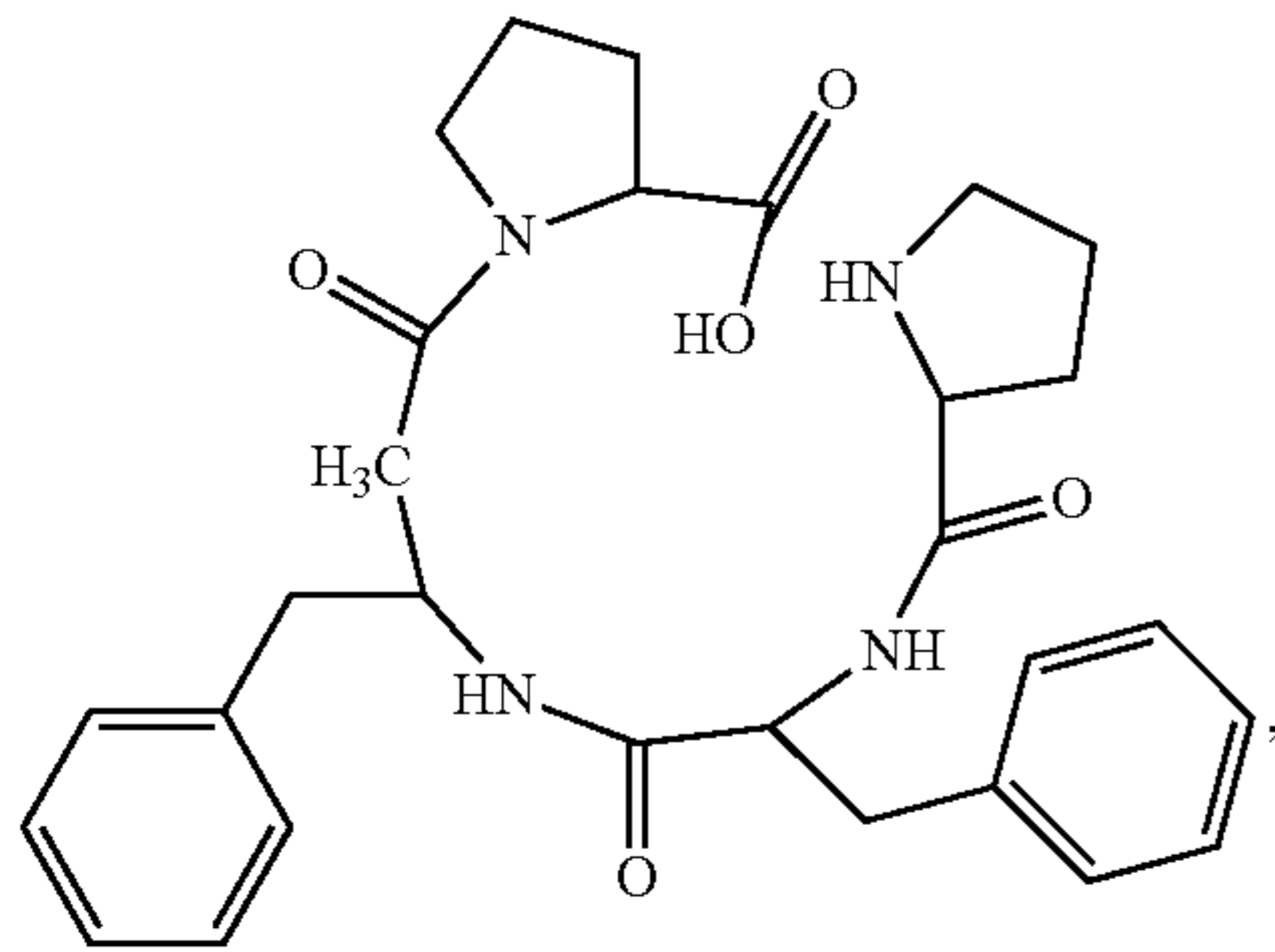
(H-Pro-Pro-Phe-β 3 hoPhe-OH)
