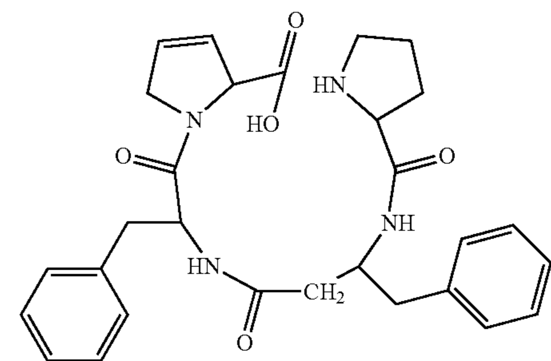
(H-Pro-β³hoPhe-Phe-ΔPro-OH)
