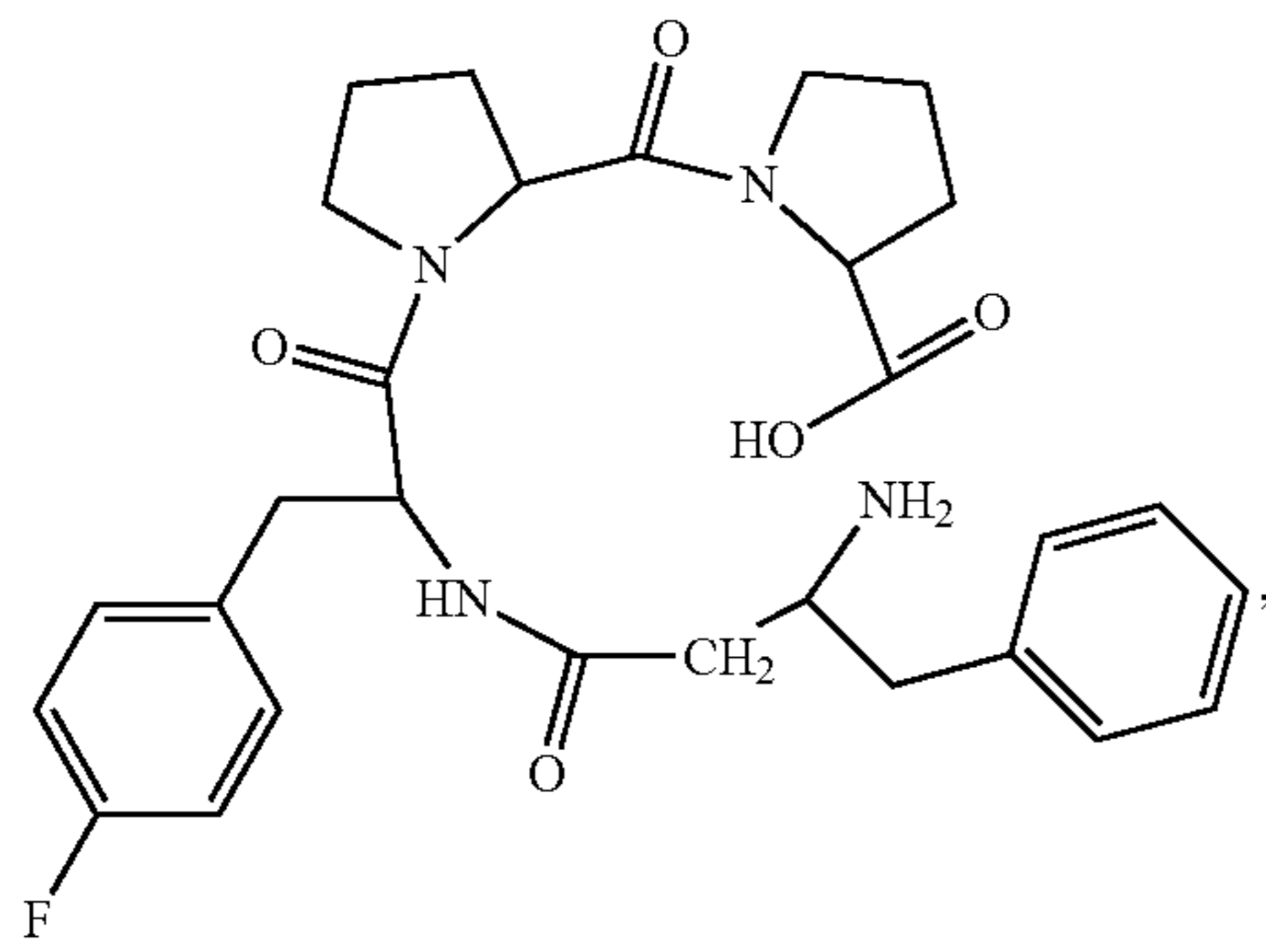
(H-β 3 hoPhe-Phe(4F)-Pro-Pro-OH)
