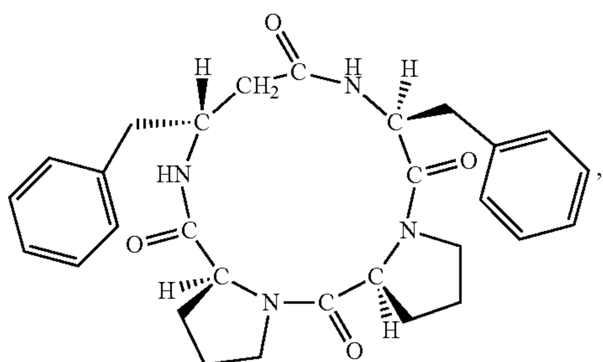
(cyclo(-L-Pro-L-Pro-D-β 3 HoPhe-L-Phe-))
