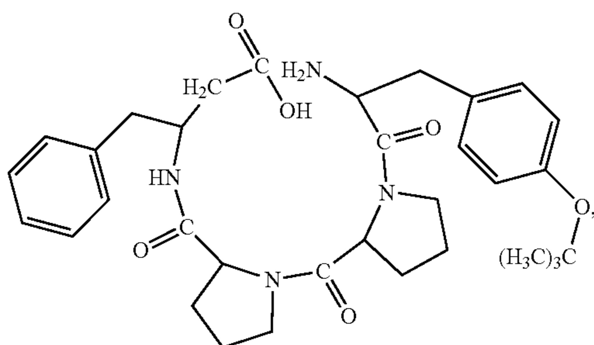
(H-Tyr(t-Bu)-Pro-Pro-β 3 hoPhe-OH)
