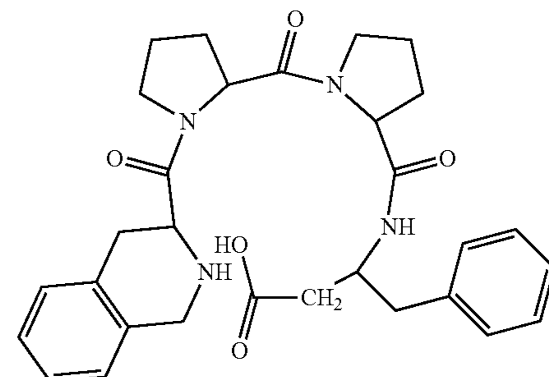
(H-Tic-Pro-Pro-β 3 hoPhe-OH)
