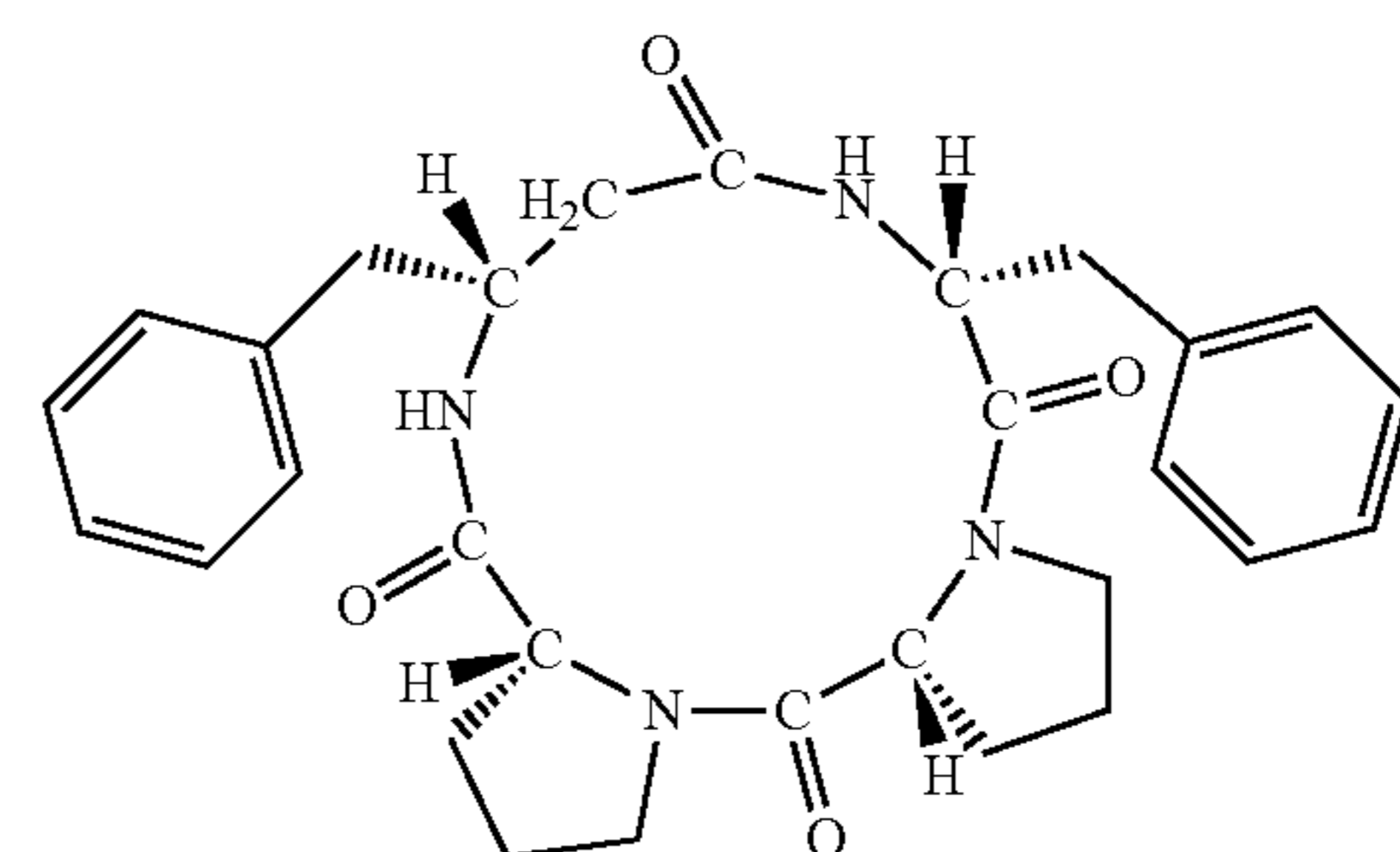
(cyclo(-D-Pro-D-Pro-D-β 3 HoPhe-D-Phe-))
