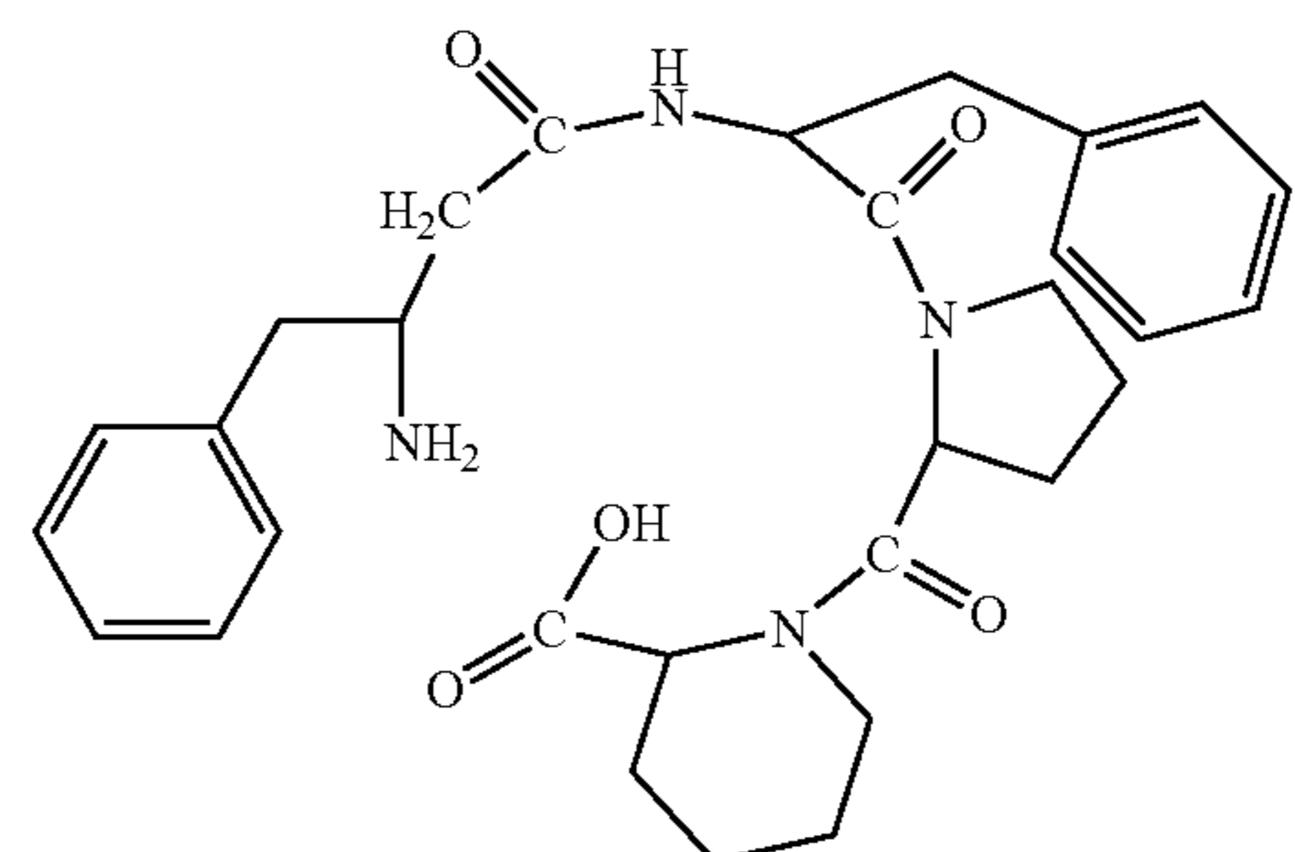
(H-β 3 hoPhe-Phe-Pro-Pip-OH)
