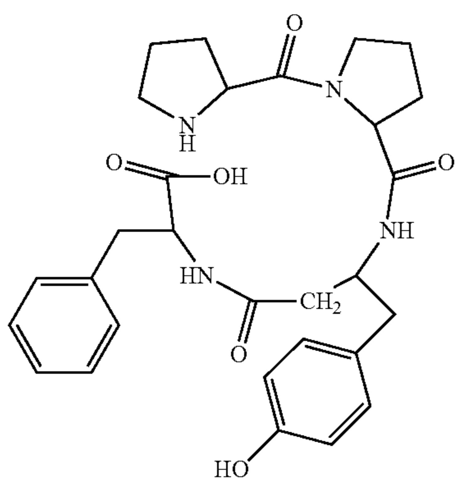
(H-Pro-Pro-β³hoTyr-Phe-OH)
