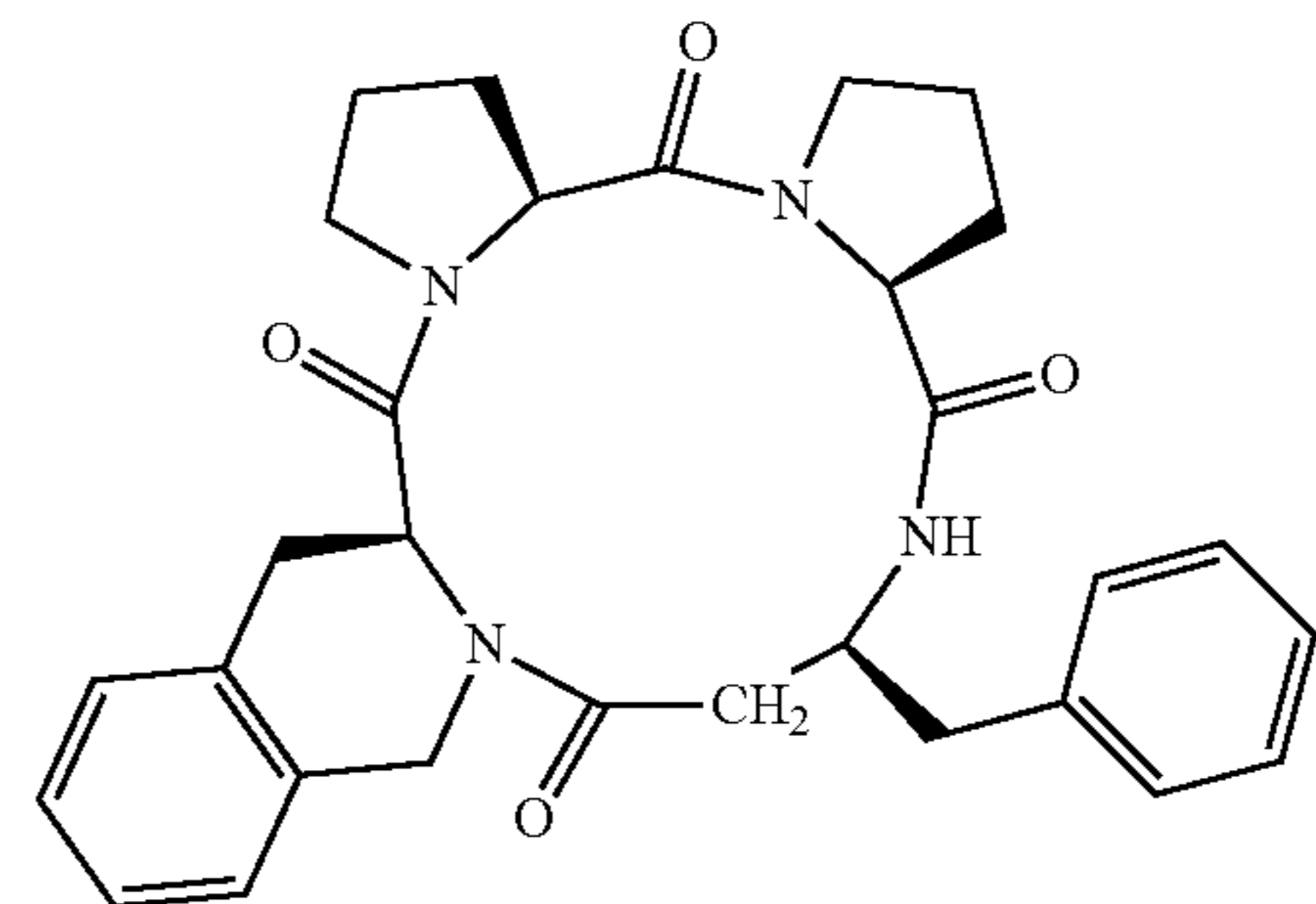
(cyclo(-L-Pro-L-Pro-L-β³hoPhe-L-Tic))
