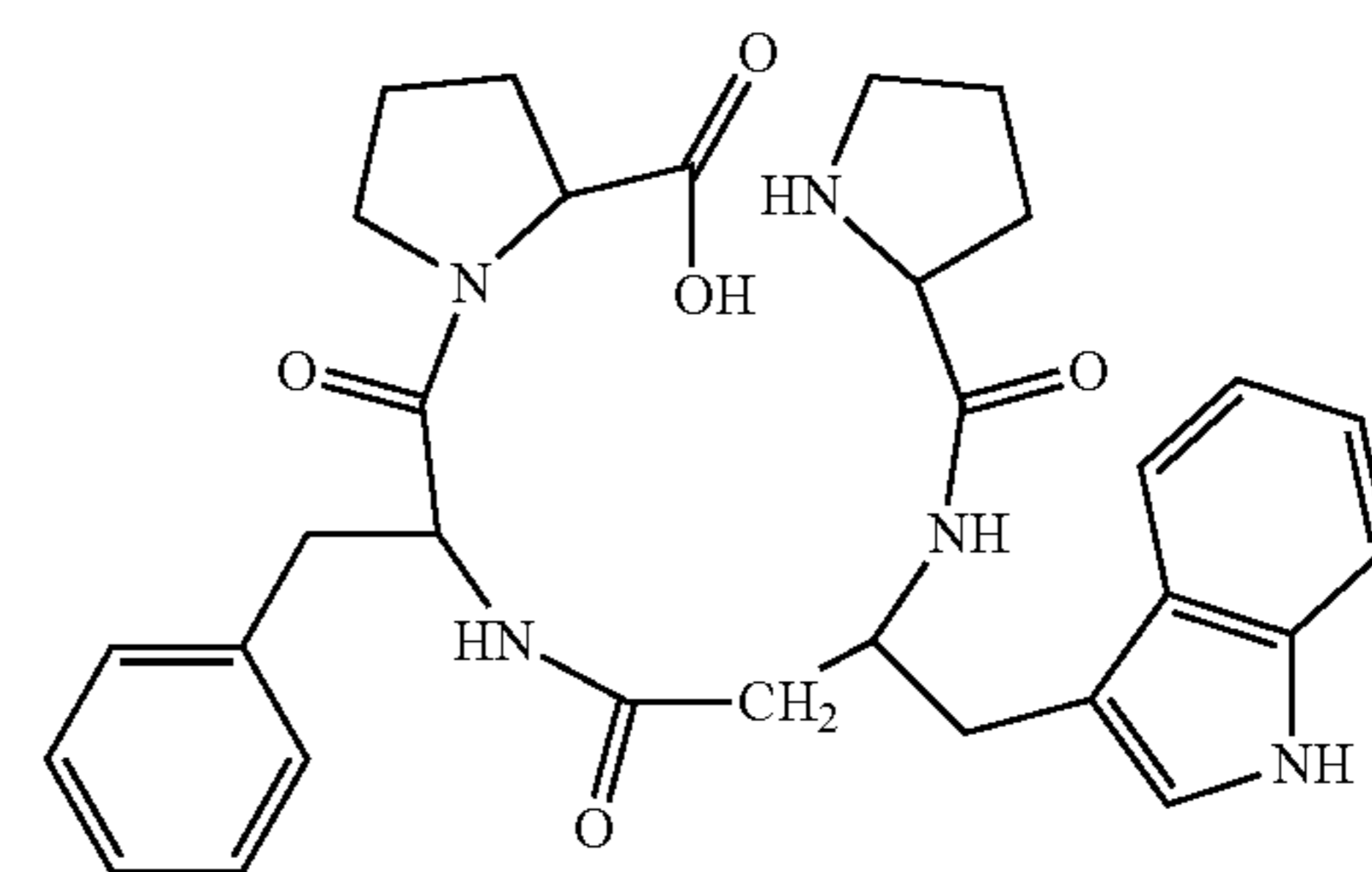
(H-Pro-β 3 hoTrp-Phe-Pro-OH)
