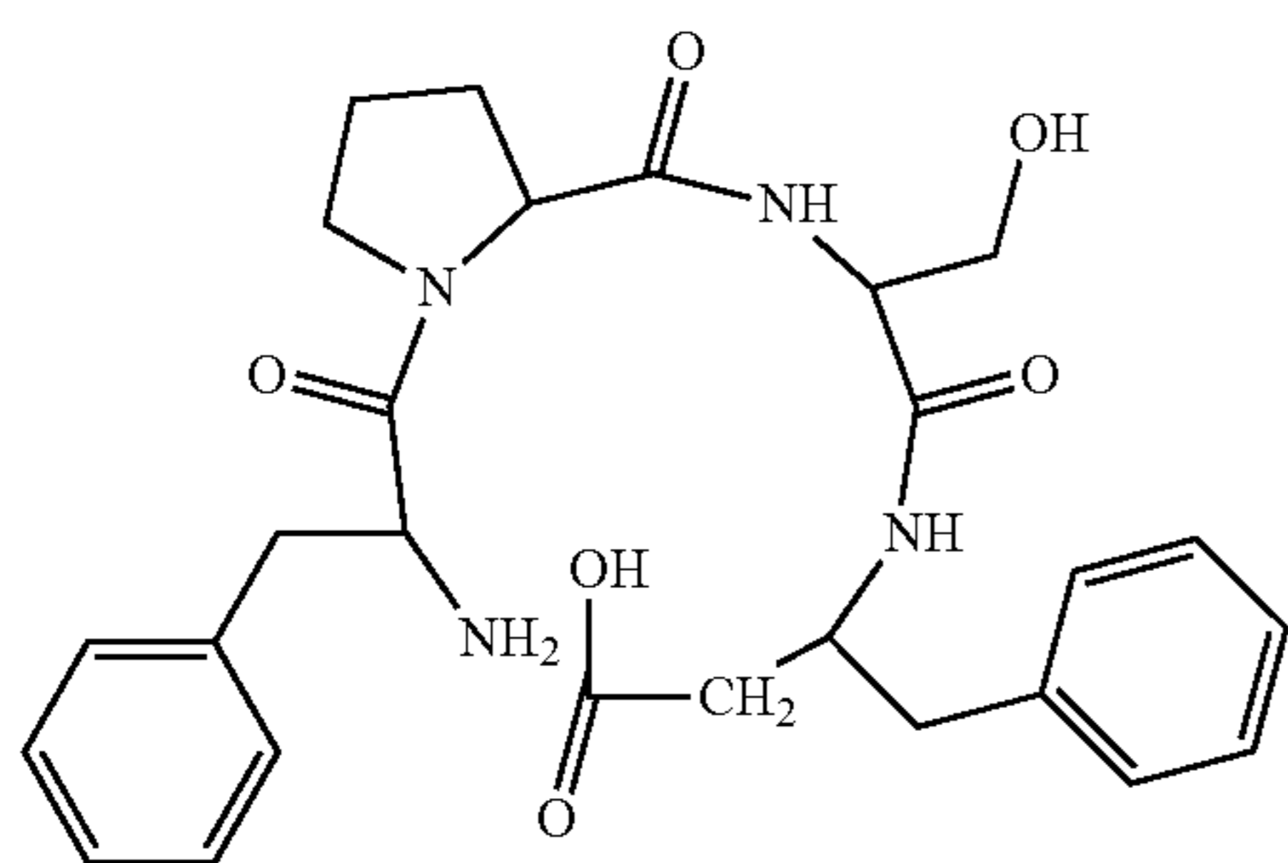
(H-Phe-Pro-Ser-β³hoPhe-OH)
