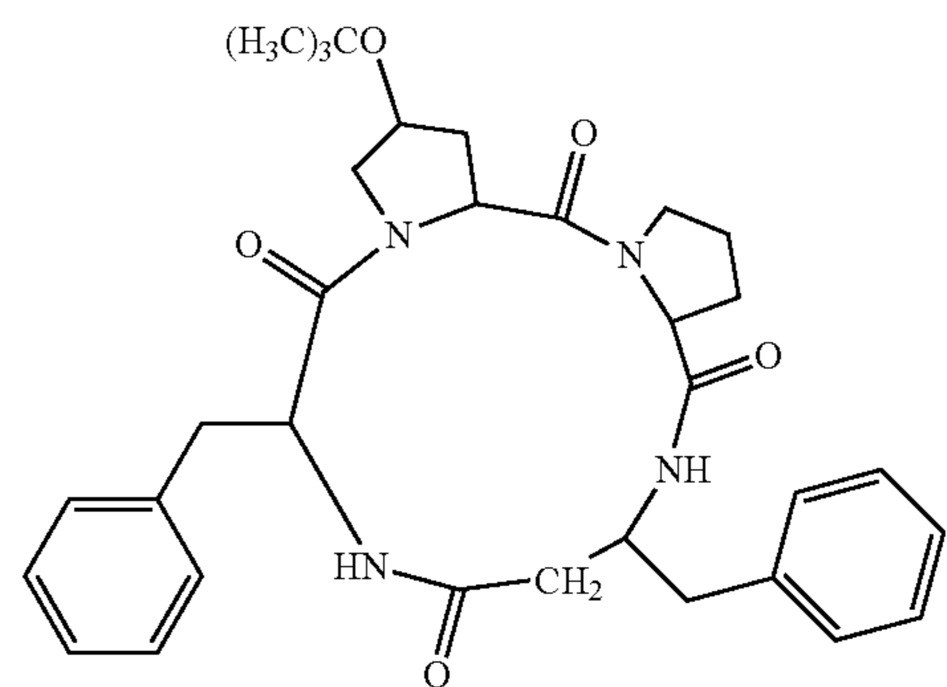
(cyclo(-Hyp(tBu)-Pro-β 3 hoPhe-Phe-))
