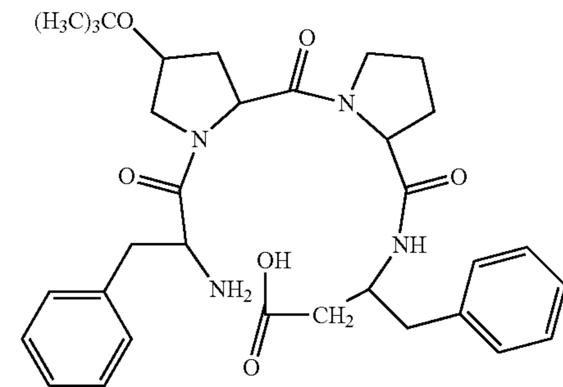
(H-Phe-Hyp(tBu)-Pro-β 3 hoPhe-OH)
