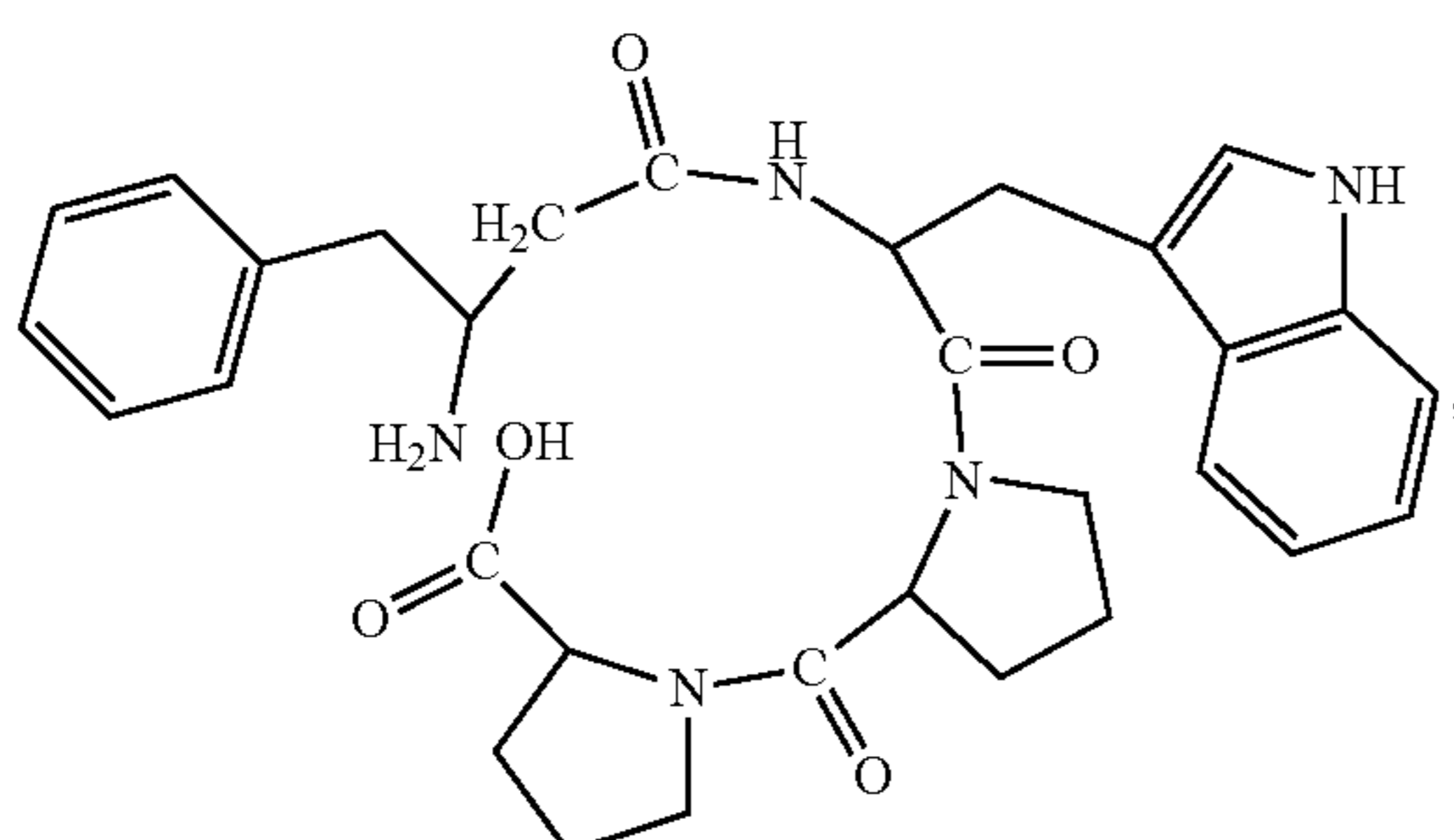
(H-β 3 hoPhe-Trp-Pro-Pro-OH)
