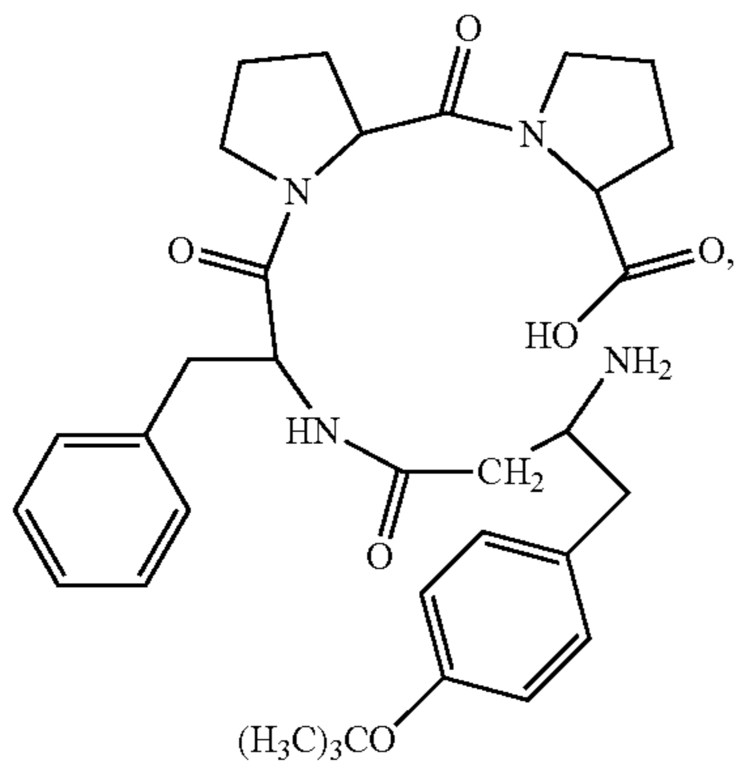
(H-β 3 hoTyr(tBu)-Phe-Pro-Pro-OH)
