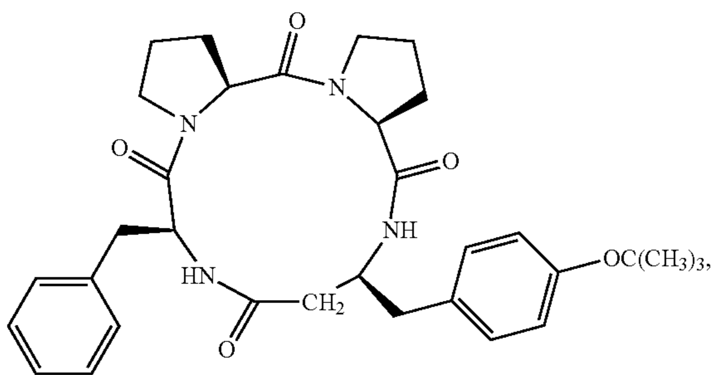
cyclo(-L-Pro-L-Pro-L-β³hoTyr(tBu)-L-Phe)
