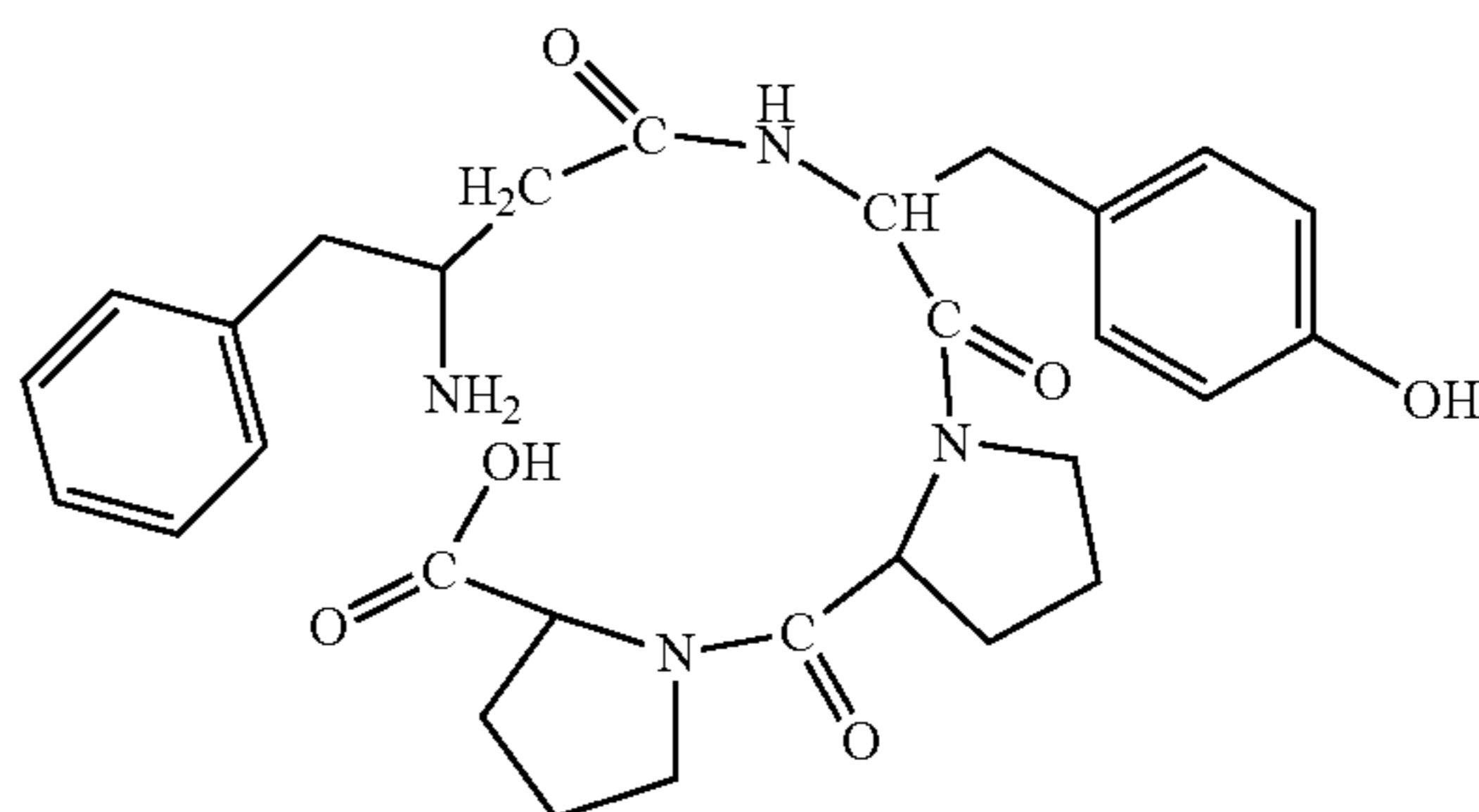
(H-β 3 hoPhe-Tyr-Pro-Pro-OH)
