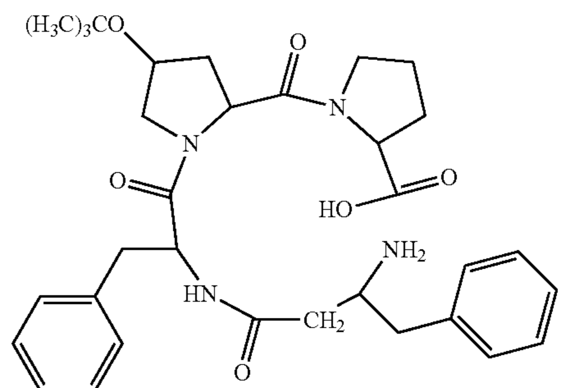
(H-β 3 hoPhe-Phe-Hyp(tBu)-Pro-OH)
