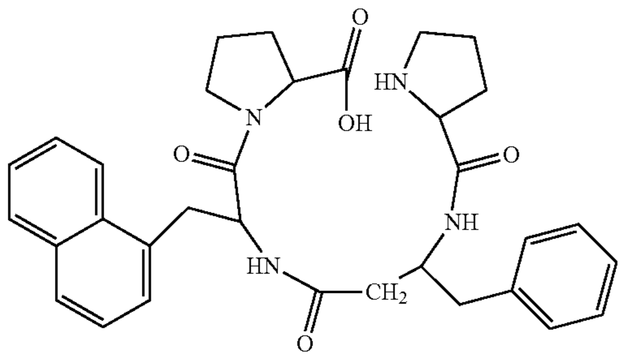
(H-Pro-β 3 hoPhe-1Nal-Pro-OH)
