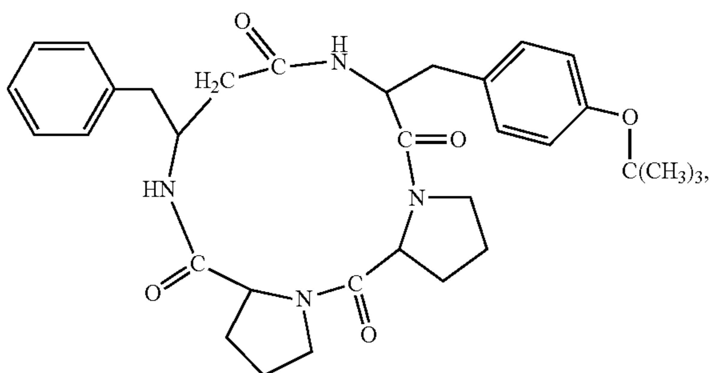
(cyclo(-Pro-Pro-β 3 hoPhe-Tyr(t-Bu-))
