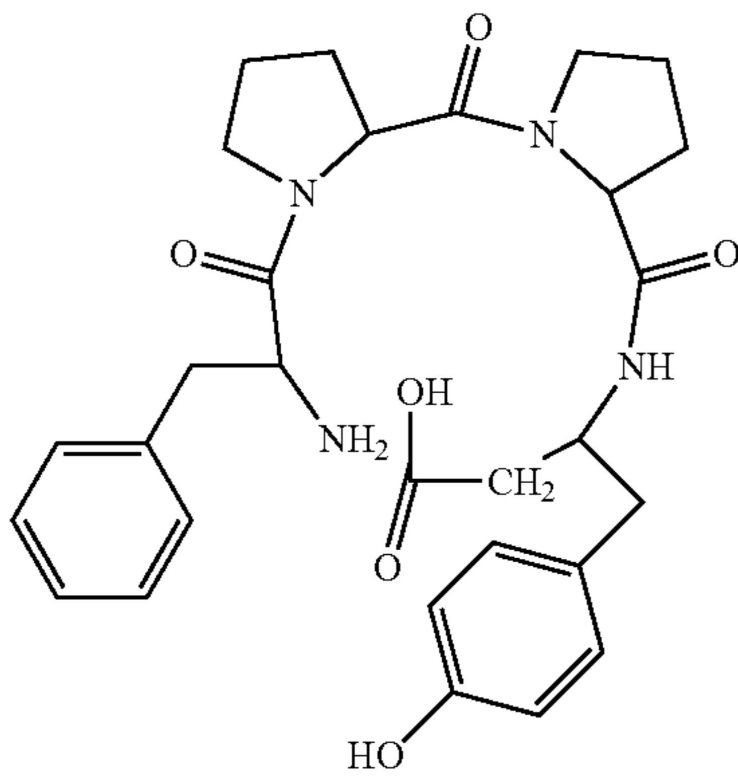
(H-Phe-Pro-Pro-β³hoTyr-OH)
