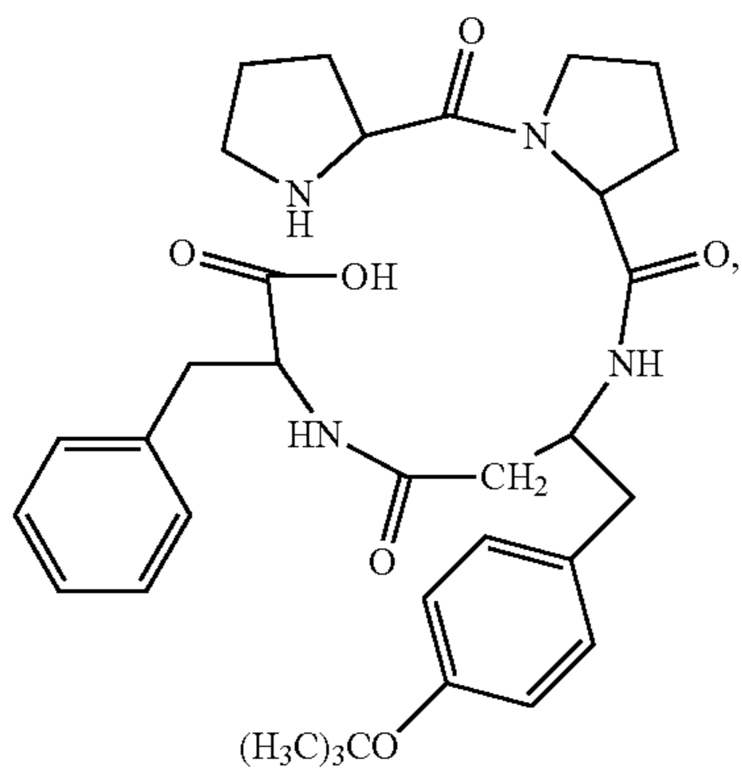
(H-Pro-Pro-β 3 hoTyr(tBu)-Phe-OH)
