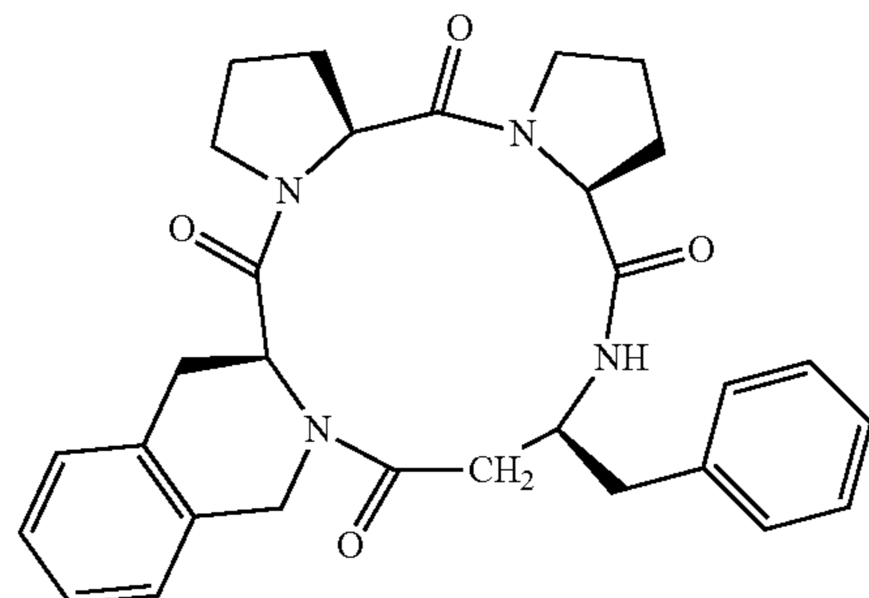
(cyclo(-L-Pro-L-Pro-L-β³hoPhe-L-Tic))
