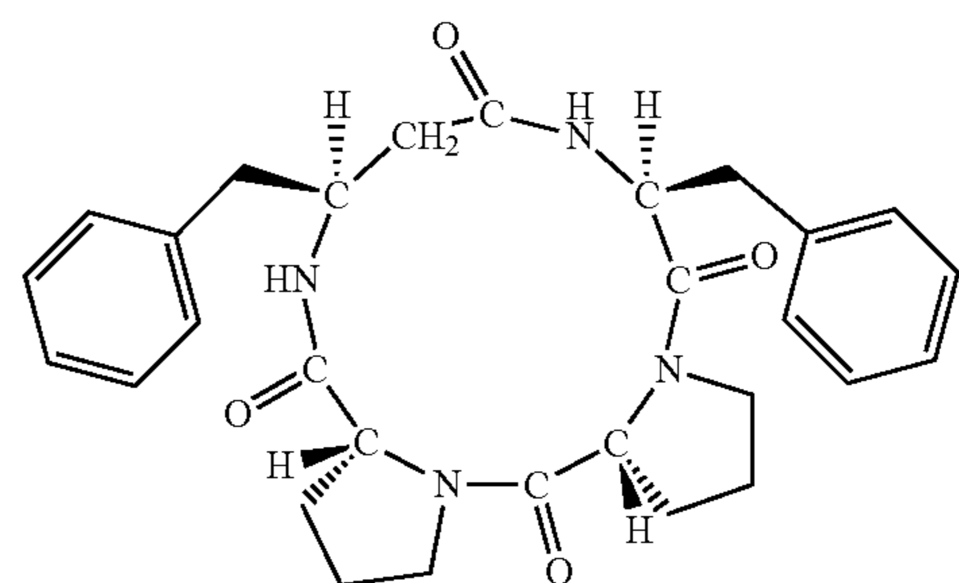
(cyclo(-D-Pro-D-Pro-L-β 3 HoPhe-L-Phe-))
