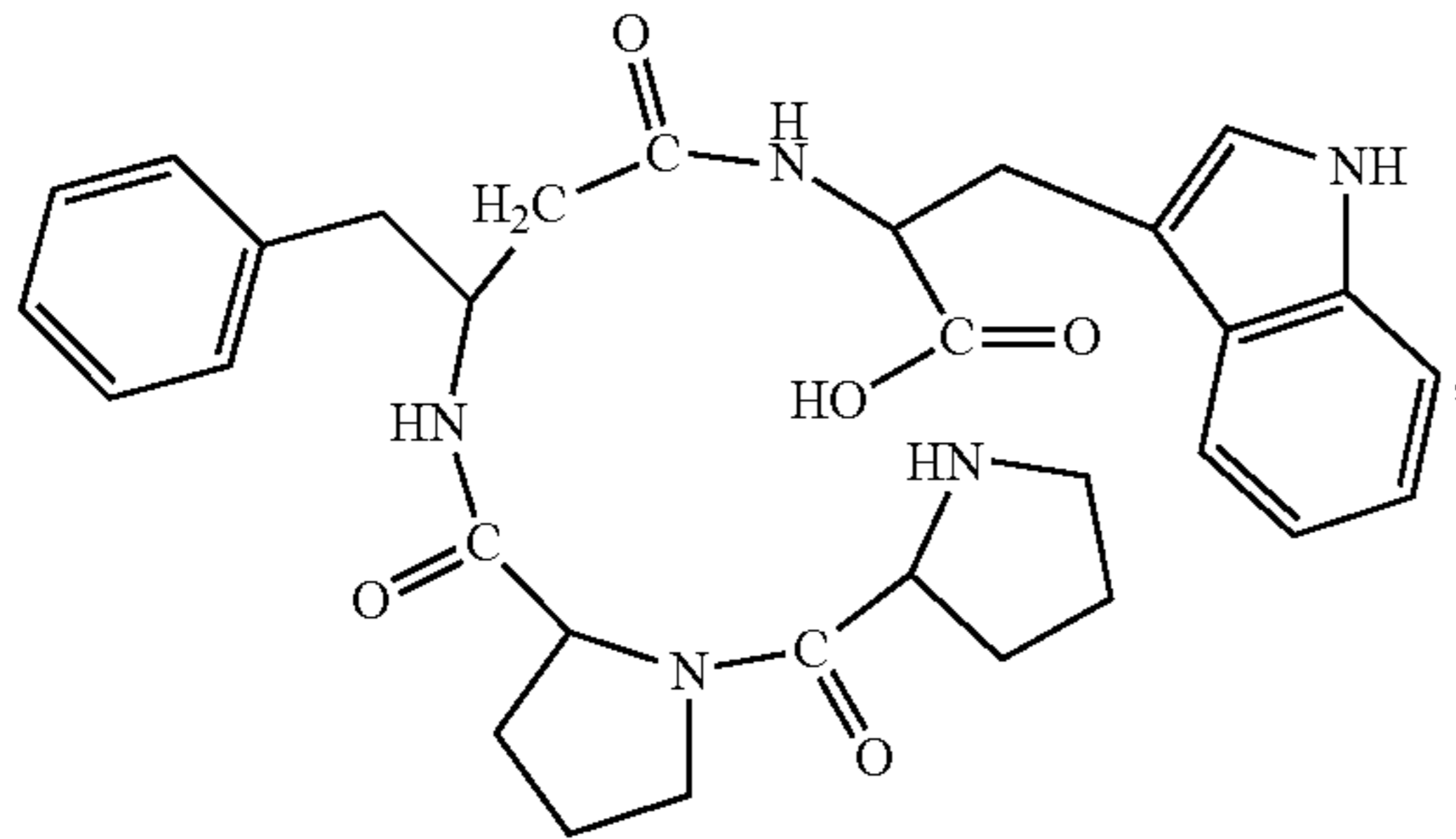
(H-Pro-Pro-β 3 hoPhe-Trp-OH)
