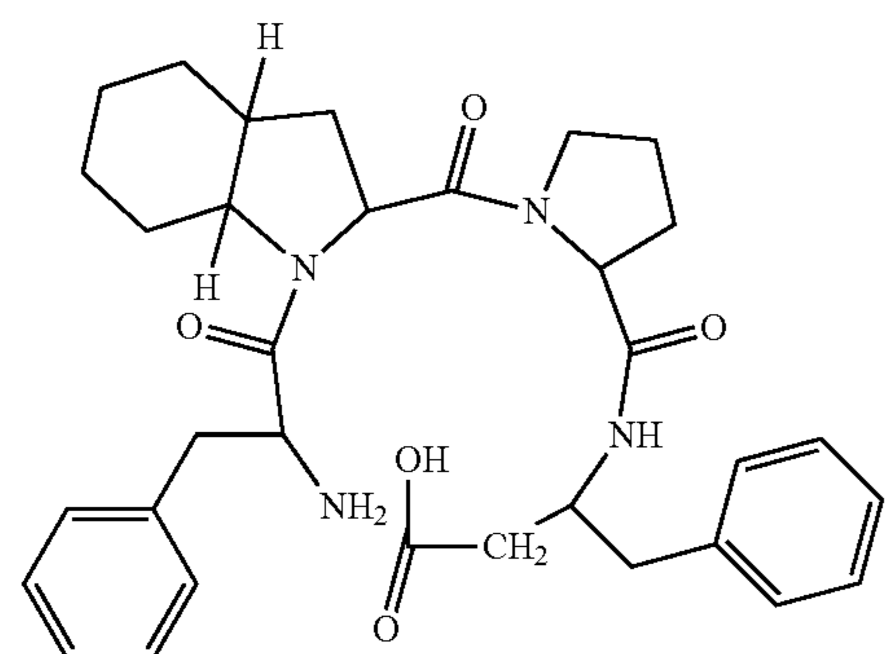
(H-Phe-Oic-Pro-β 3 hoPhe-OH)
