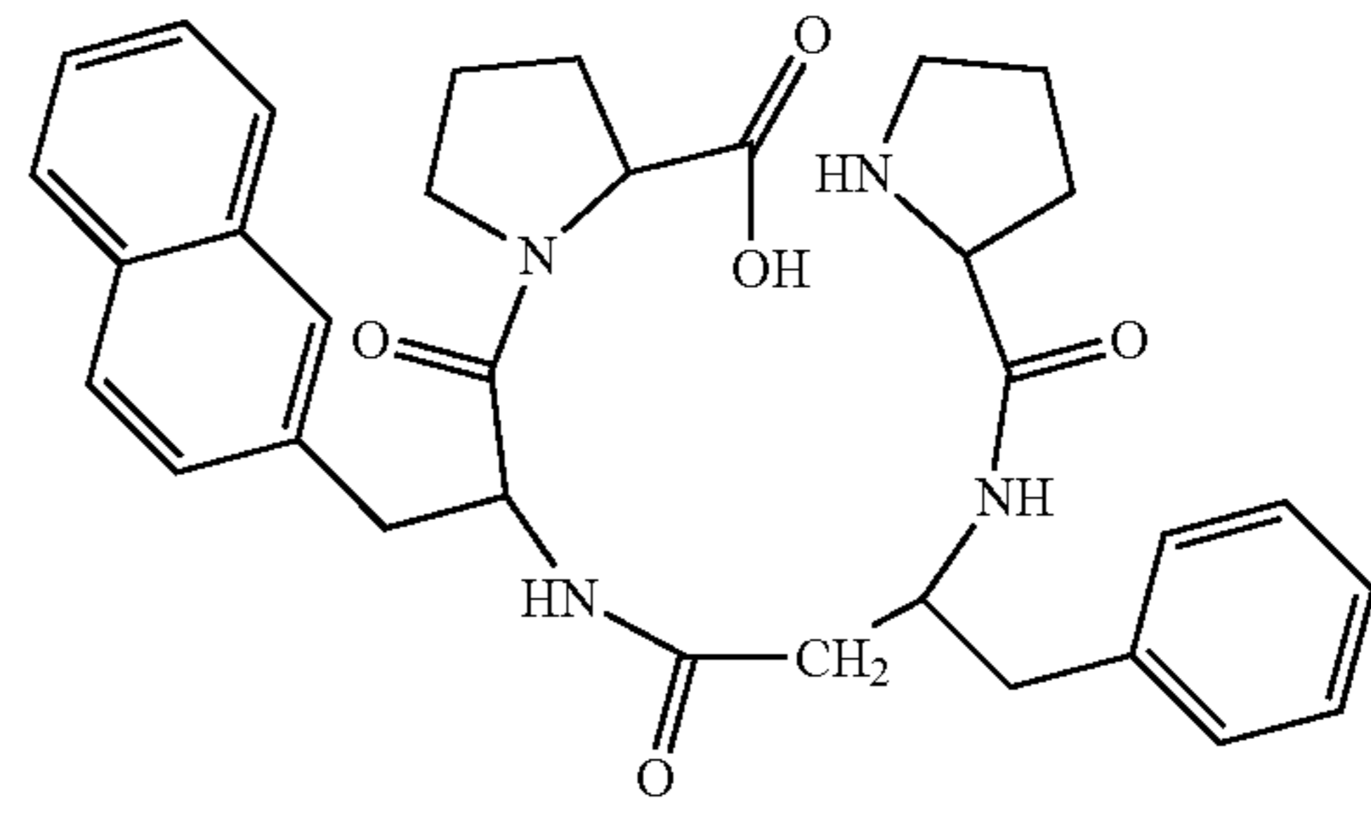
(H-Pro-β 3 hoPhe-2Nal-Pro-OH)
