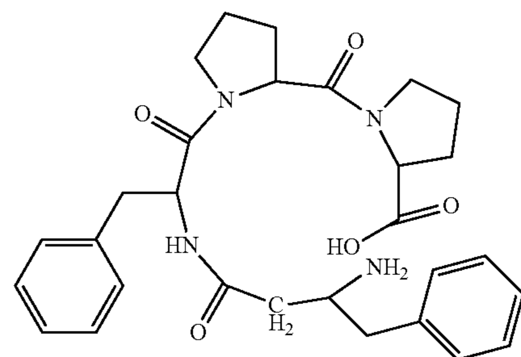
(H-β 3 hoPhe-Phe-Pro-Pro-OH)
