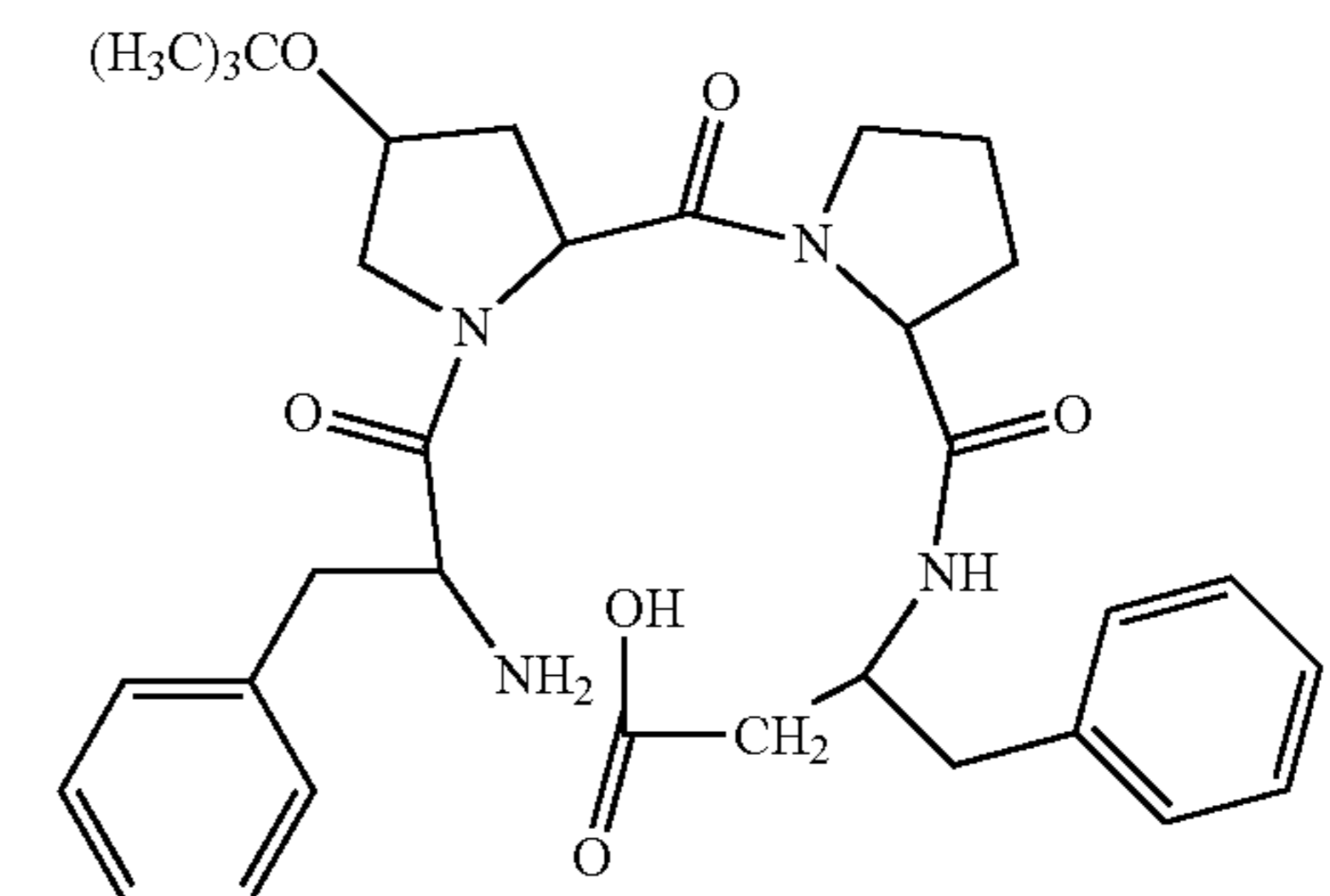
(H-Phe-Hyp(tBu)-Pro-β 3 hoPhe-OH)
