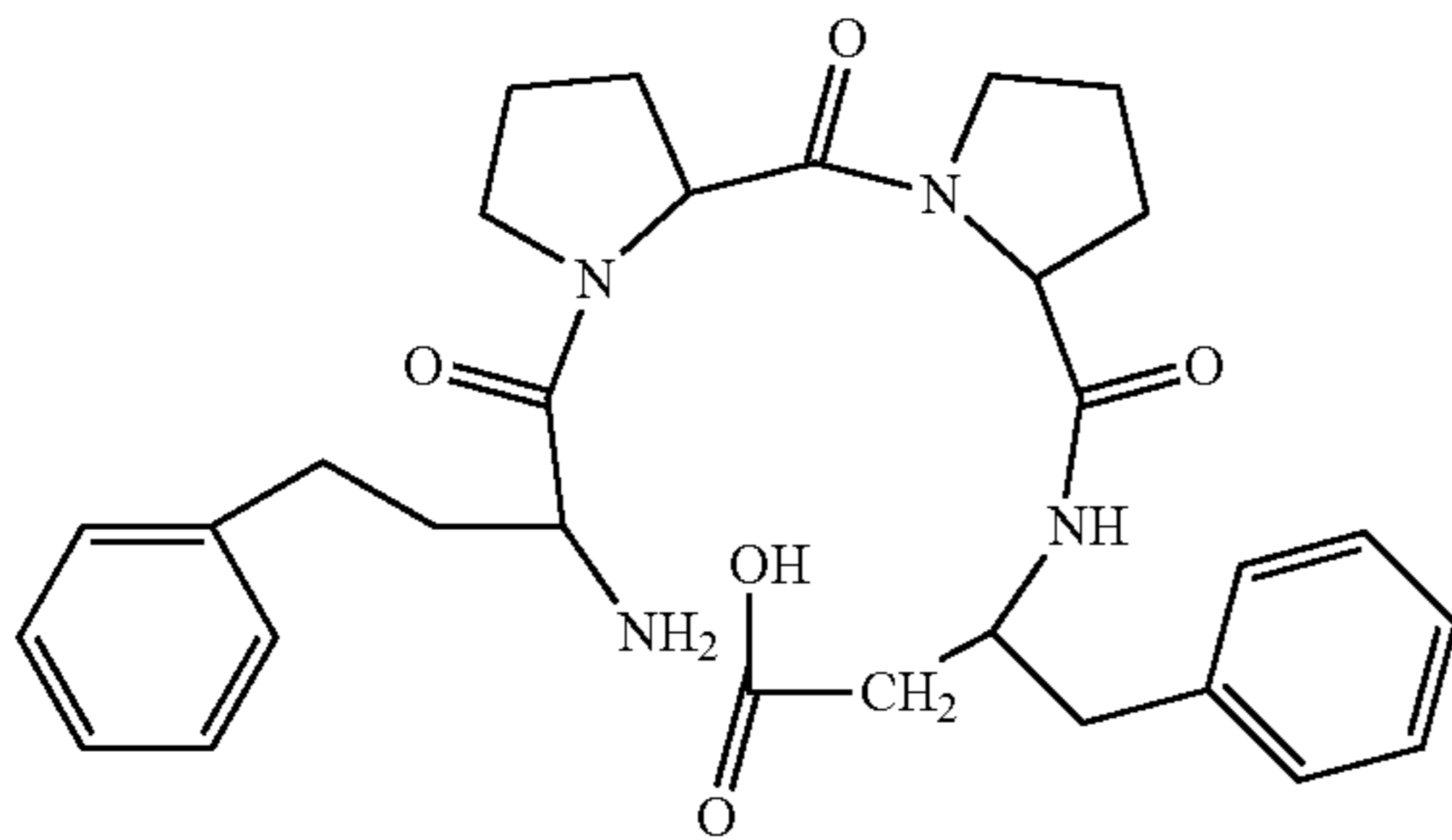
(H-hoPhe-Pro-Pro-β³hoPhe-OH)
