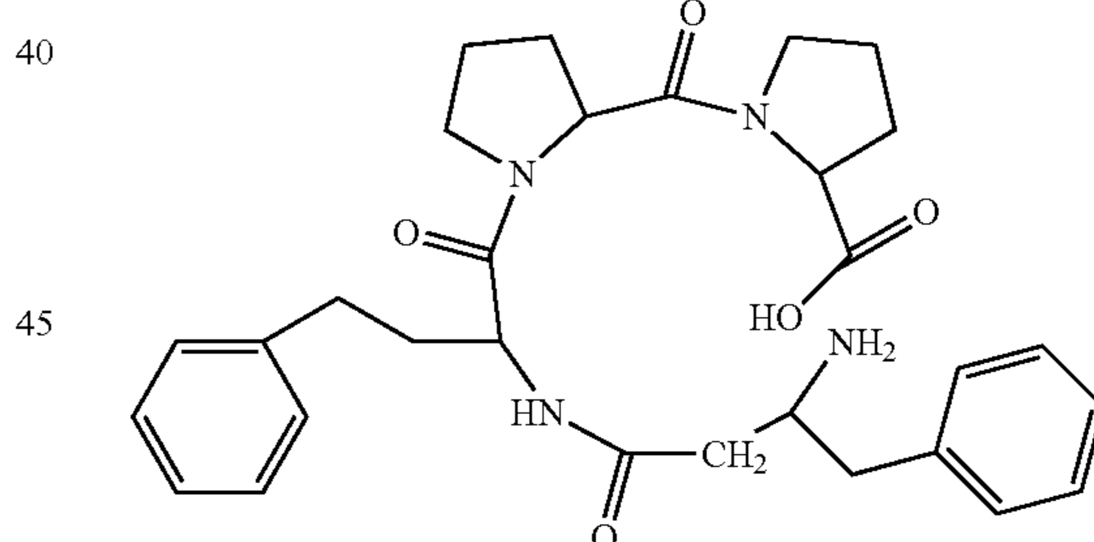
(H-β³hoPhe-hoPhe-Pro-Pro-OH)
