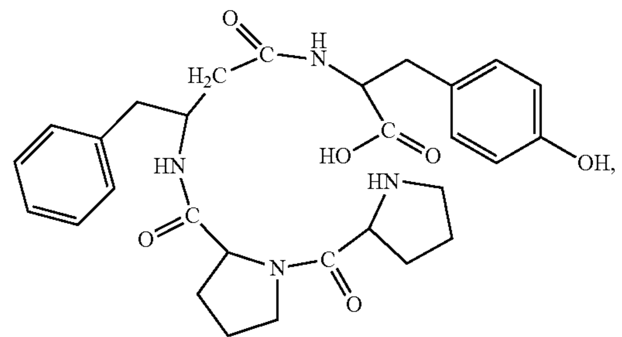
(H-Pro-Pro-β 3 hoPhe-Tyr-OH)
