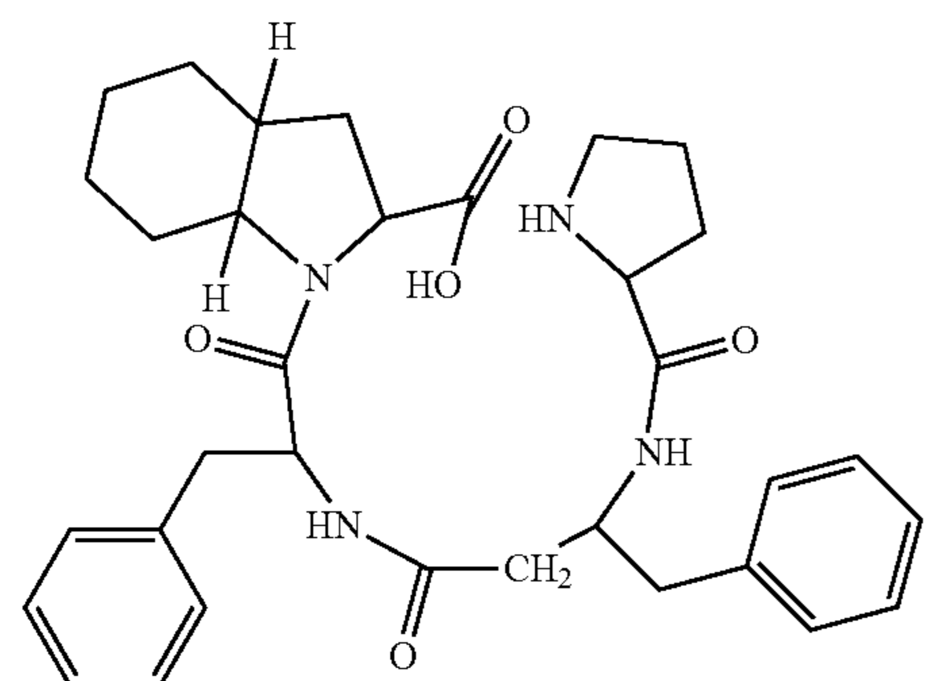
(H-Pro-β 3 hoPhe-Phe-Oic-OH)
