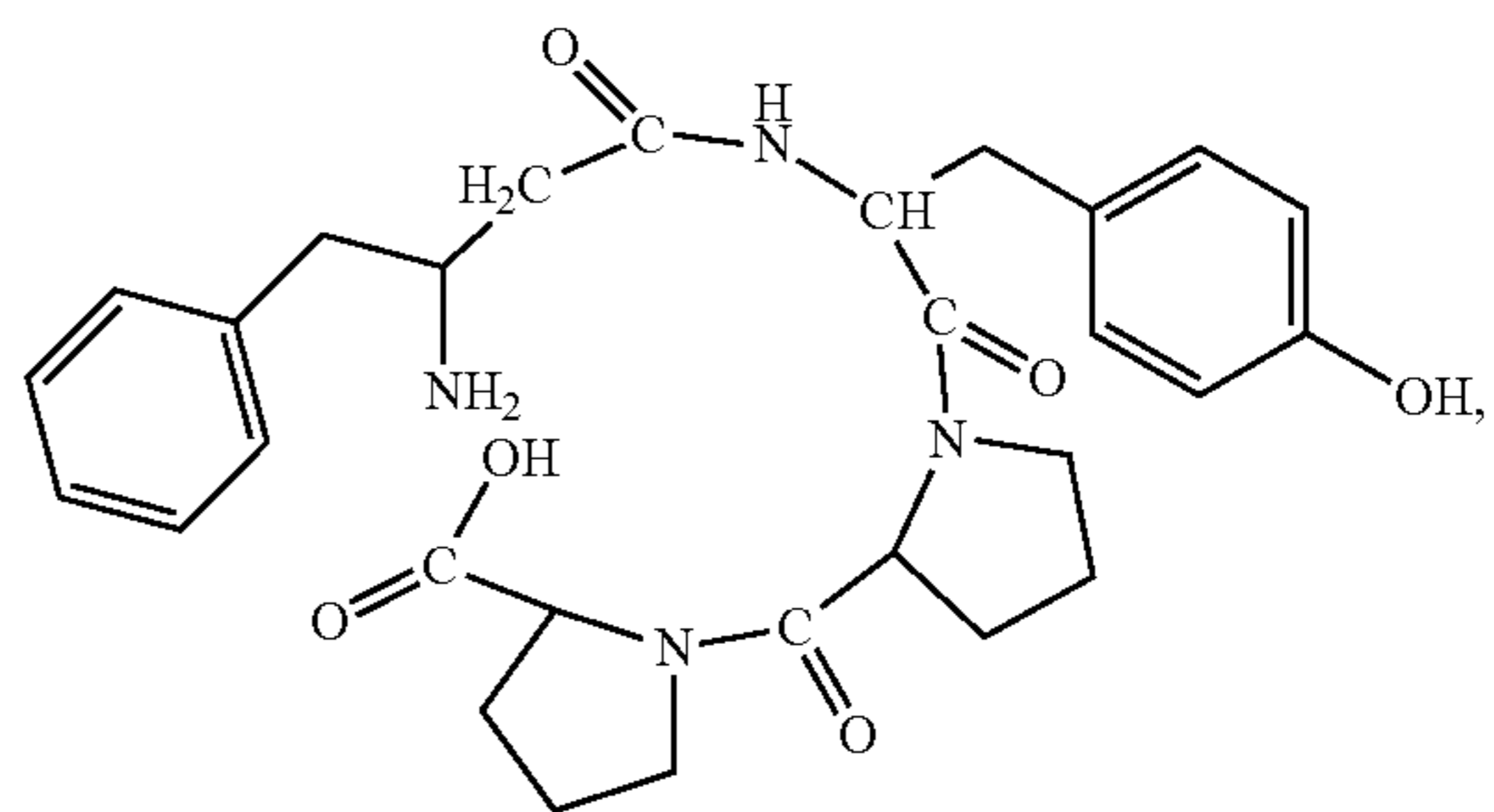
(H-β 3 hoPhe-Tyr-Pro-Pro-OH)
