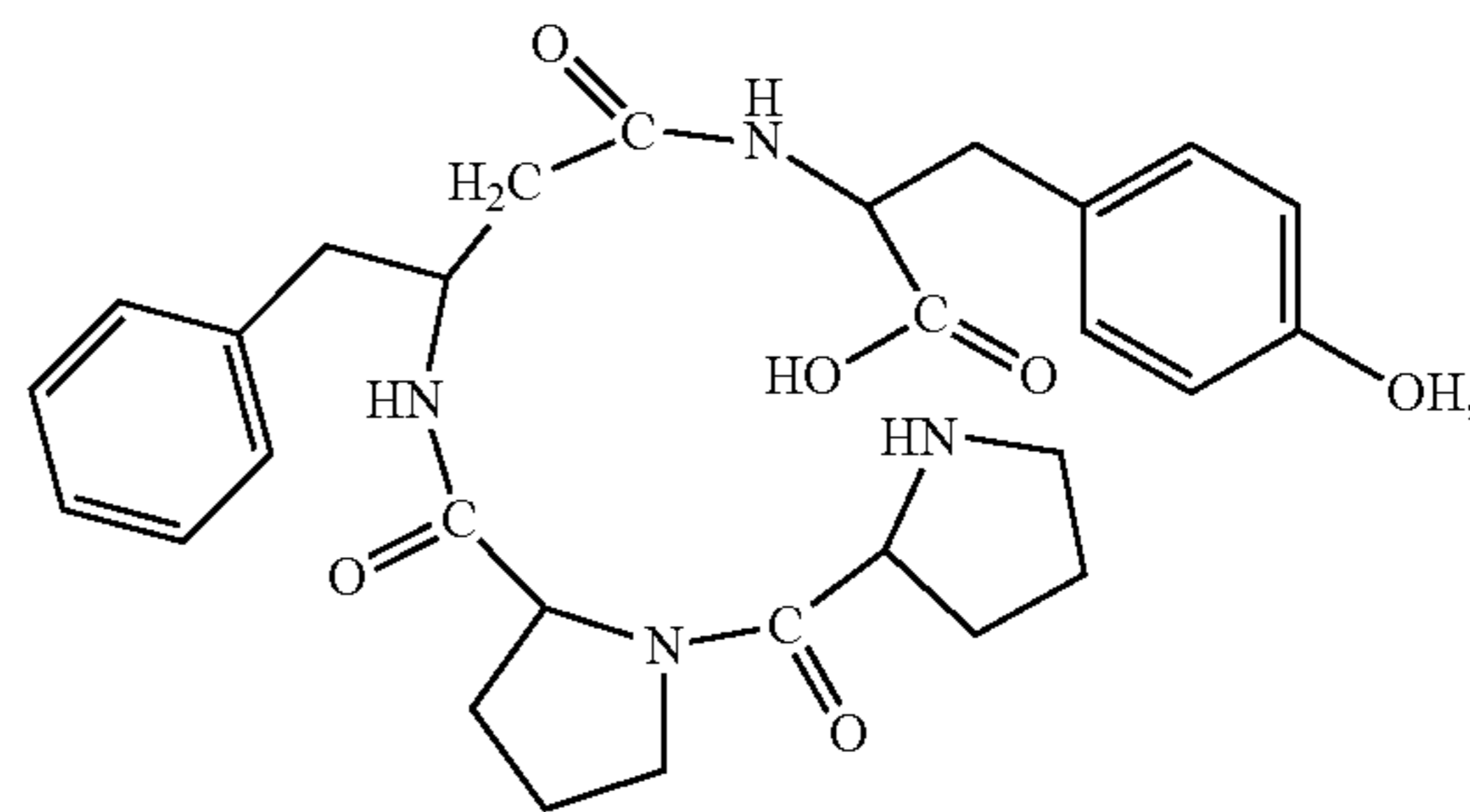
(H-Pro-Pro-β 3 hoPhe-Tyr-OH)
