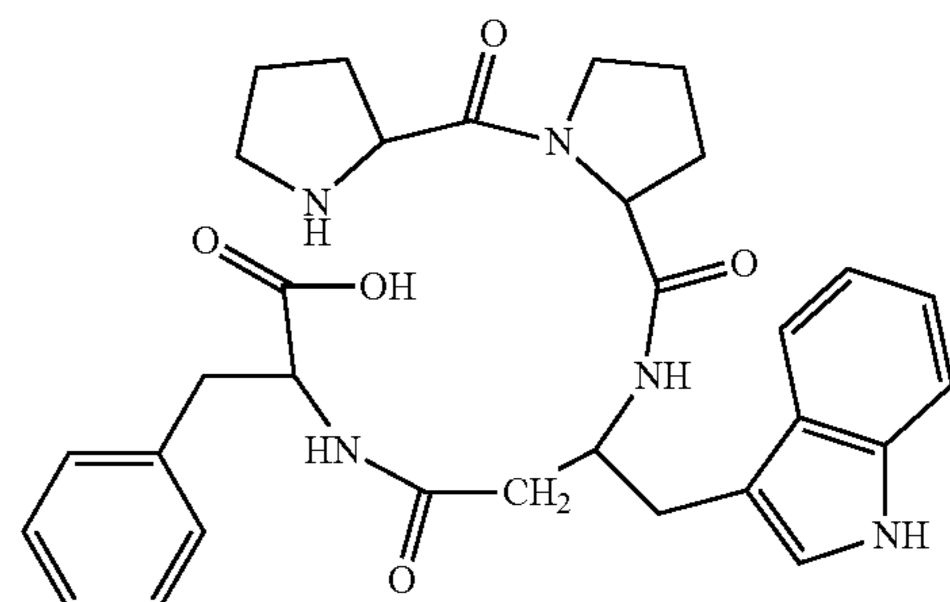
(H-Pro-Pro-β 3 hoTrp-Phe-OH)
