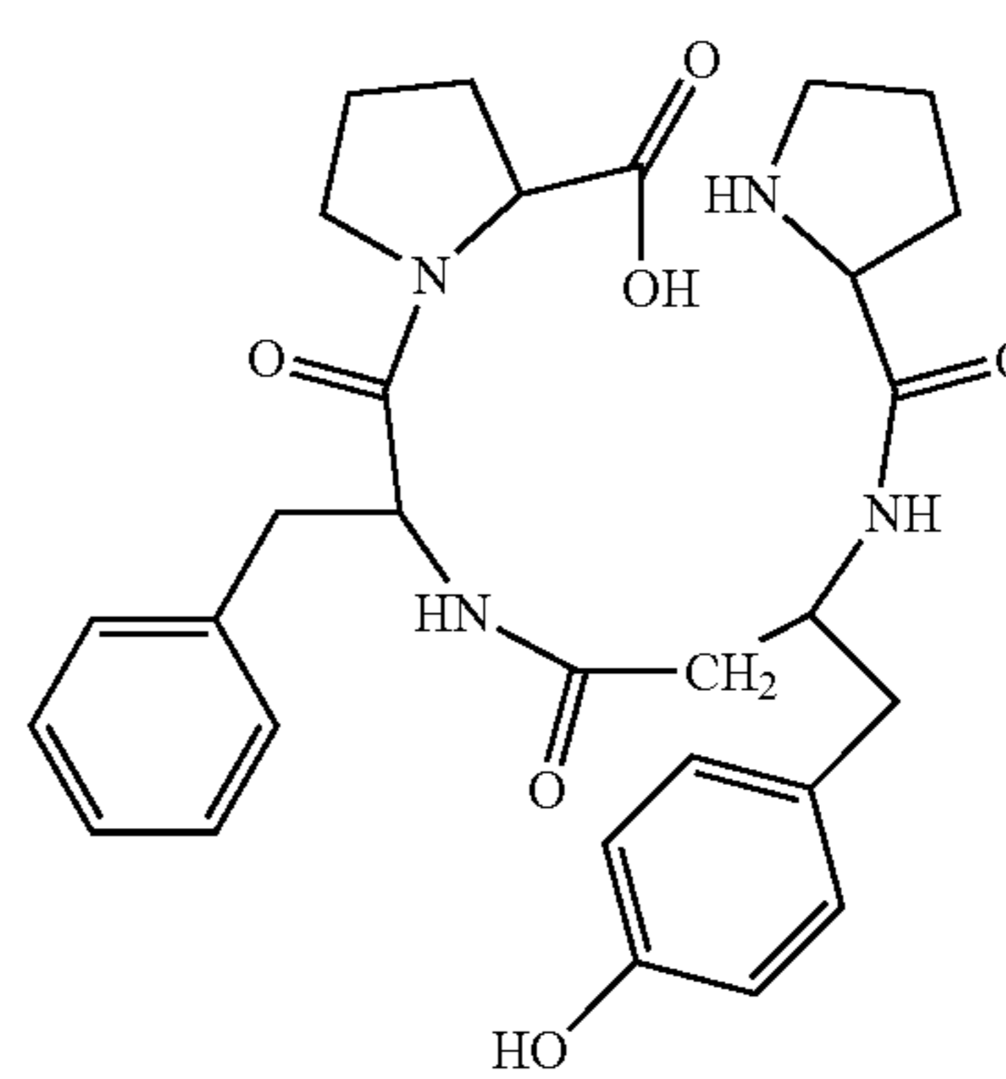
(H-Pro-β 3 hoTyr-Phe-Pro-OH)
