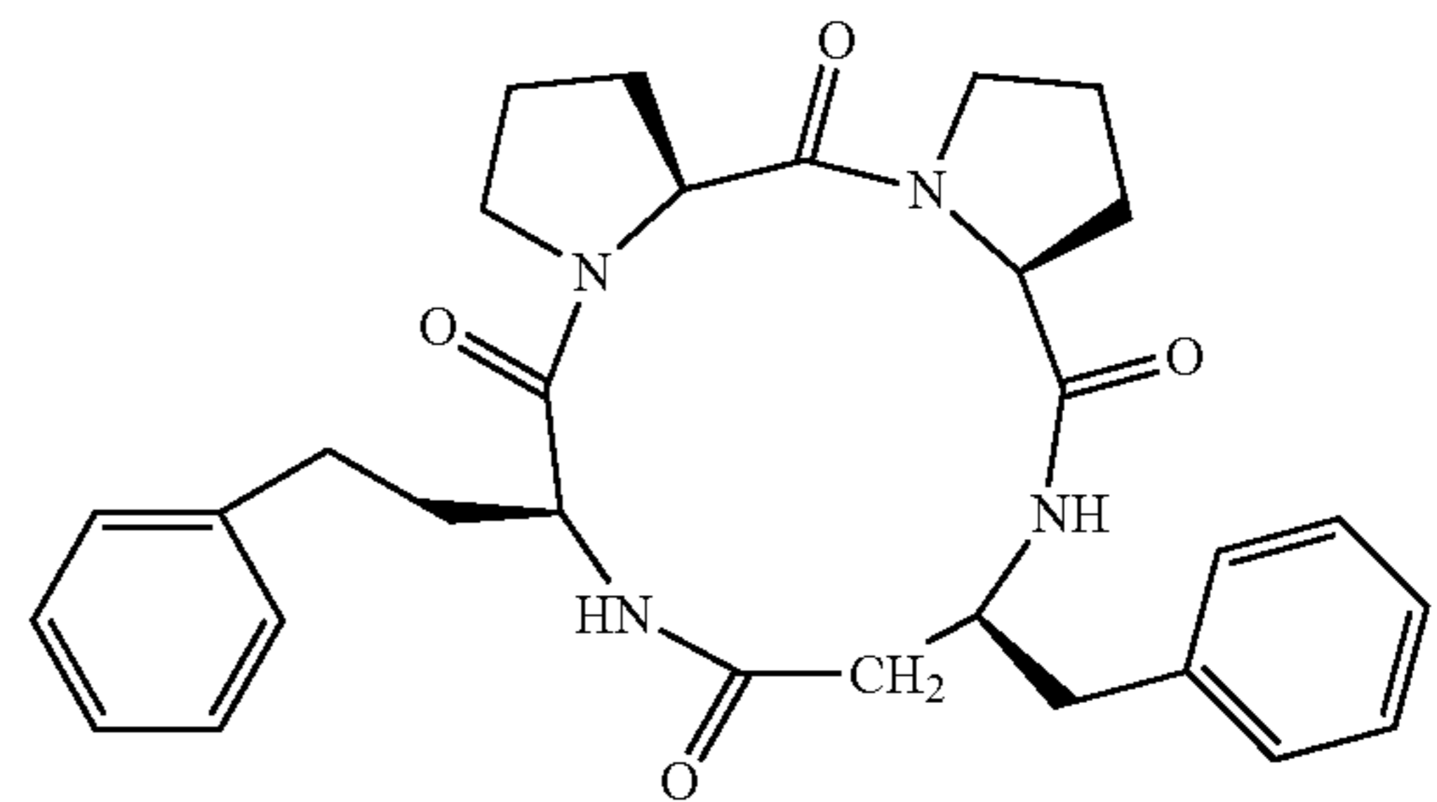
(cyclo(-L-Pro-L-Pro-L-β³hoPhe-L-hoPhe))
