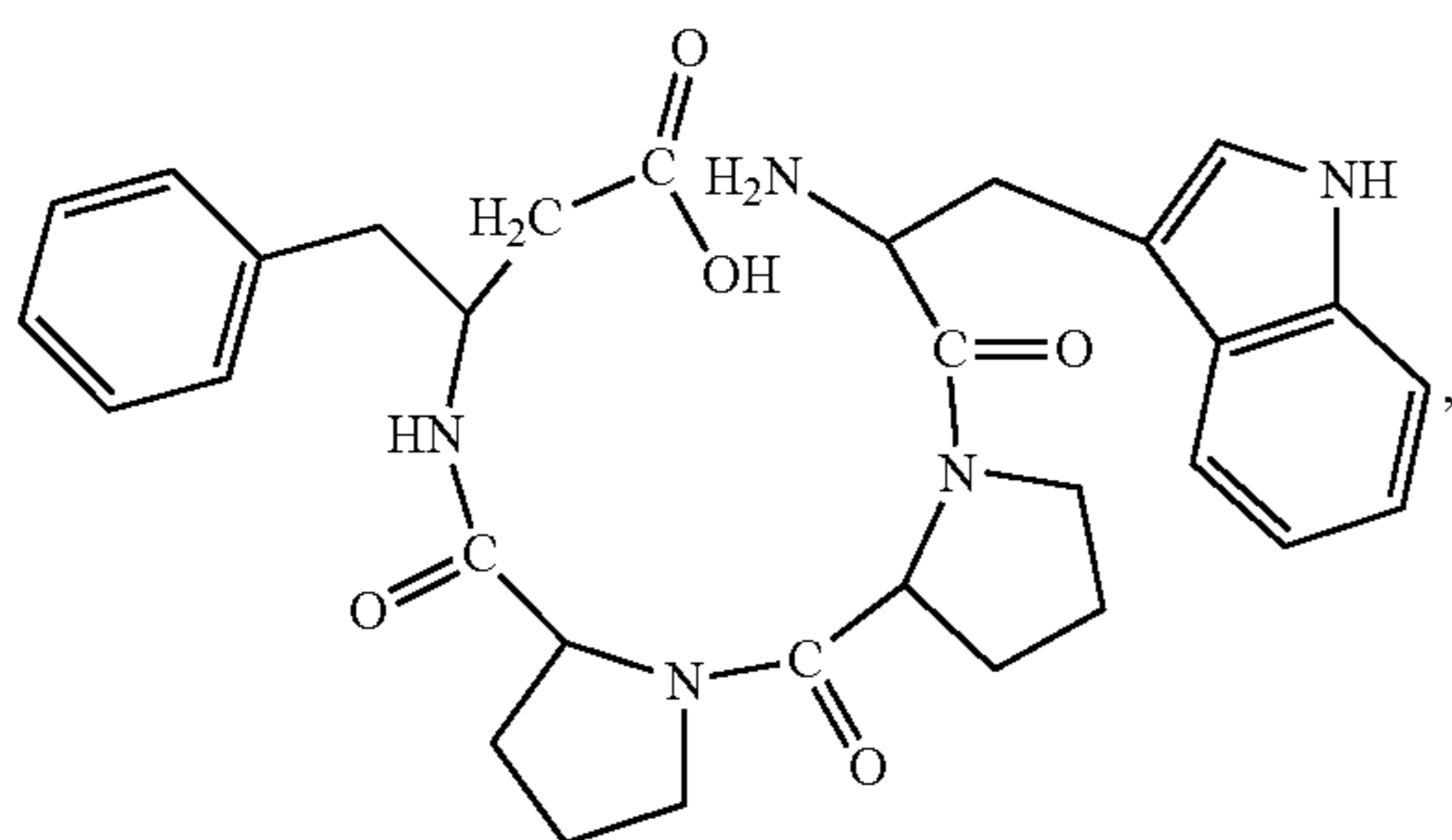
(H-Trp-Pro-Pro-β 3 hoPhe-OH)
