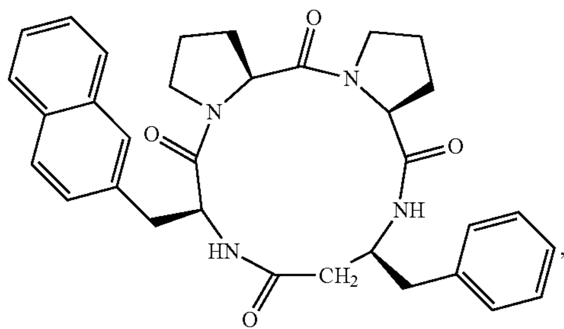
cyclo(-L-Pro-L-Pro-L-β³hoPhe-L-2Nal))
