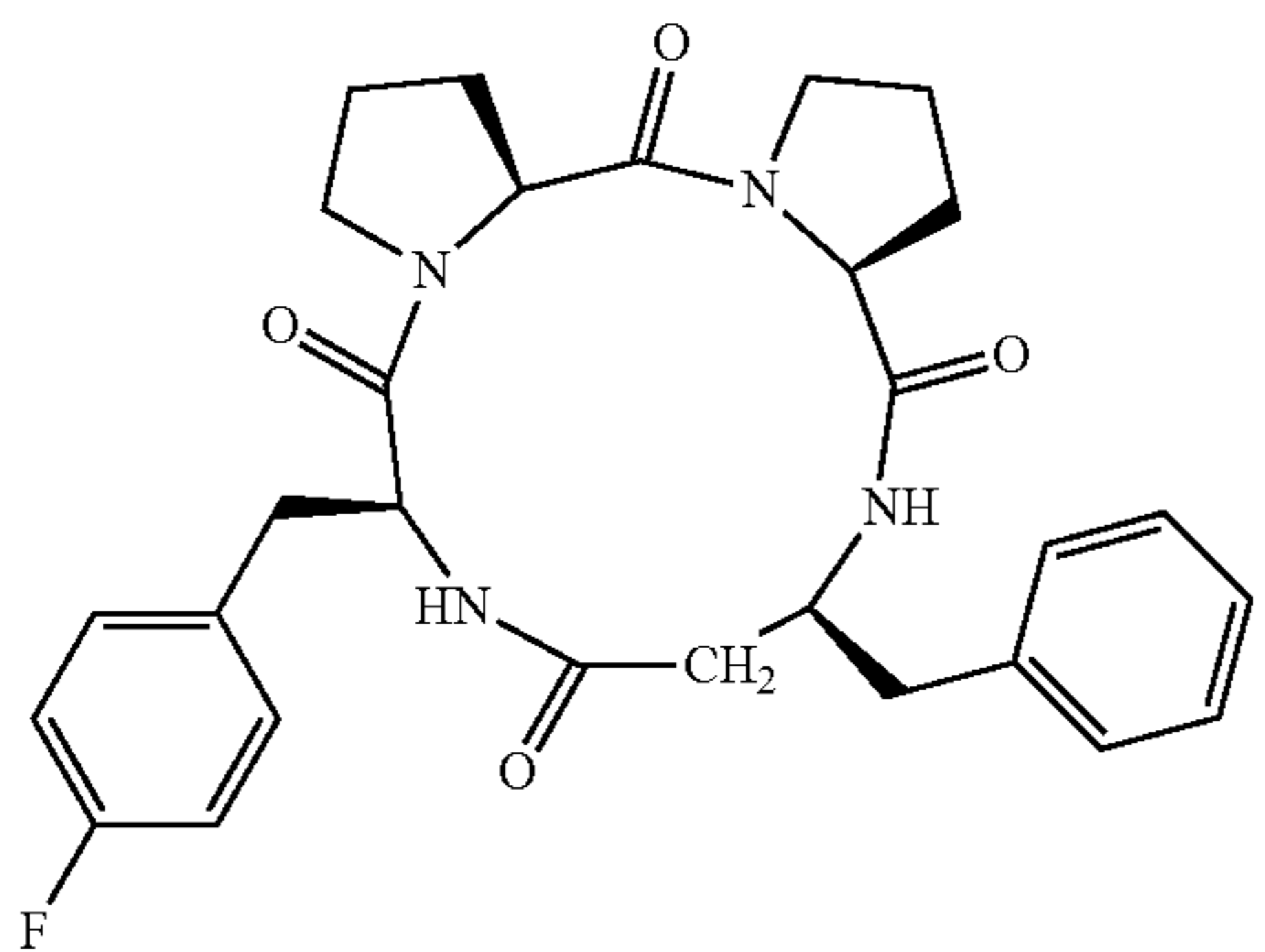
cyclo(-L-Pro-L-Pro-L-β³hoPhe-L-Phe(4F)))
