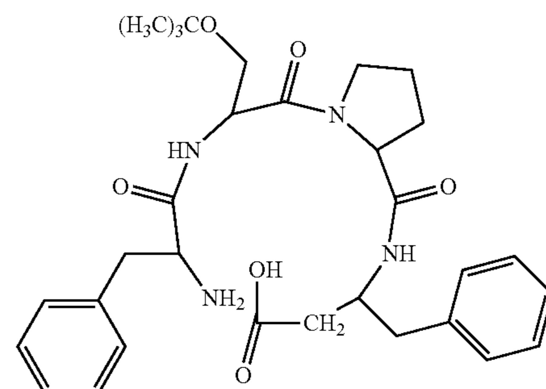
(H-Phe-Ser(tBu)-Pro-β³hoPhe-OH)
