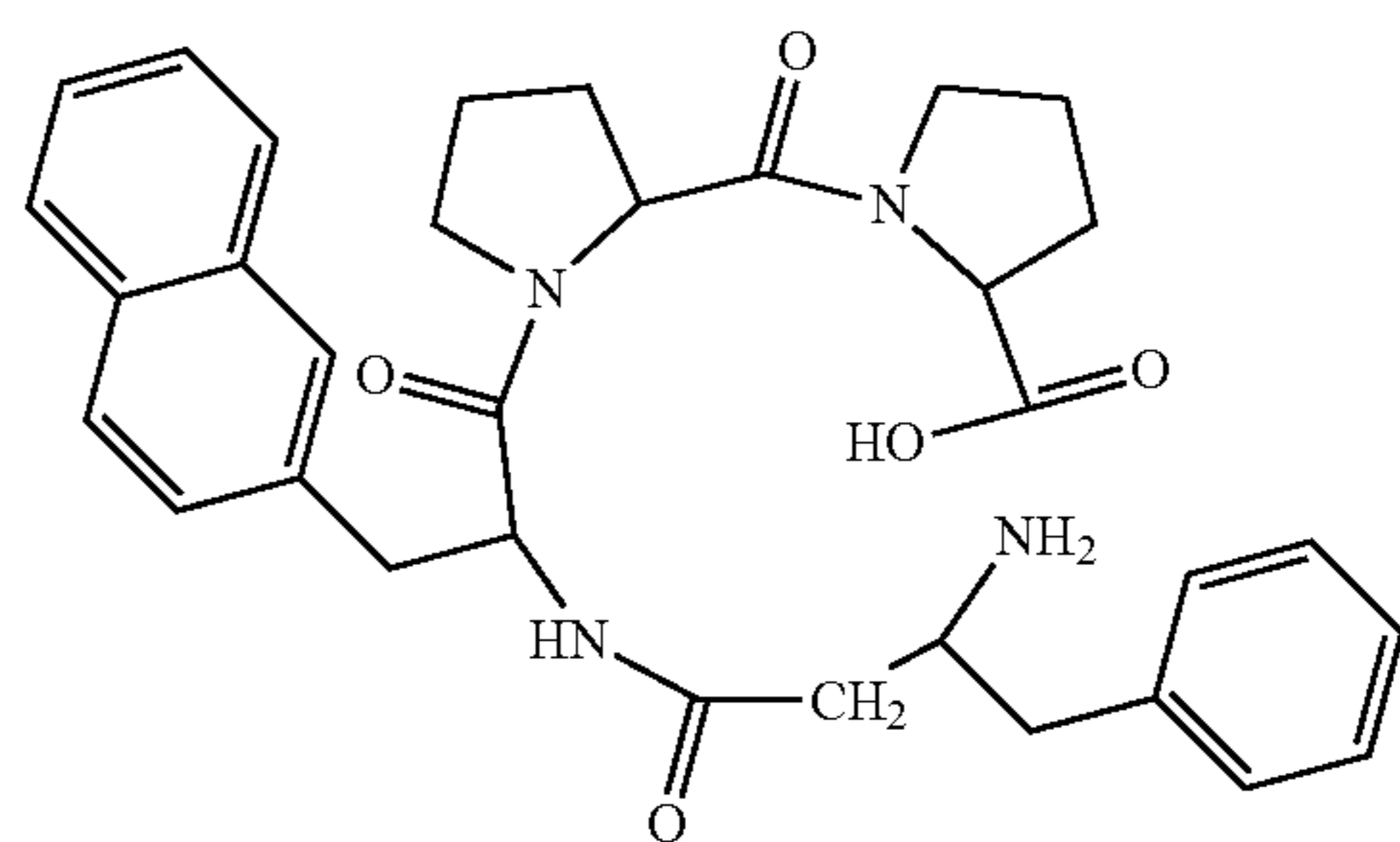
(H-β 3 hoPhe-2Nal-Pro-Pro-OH)
