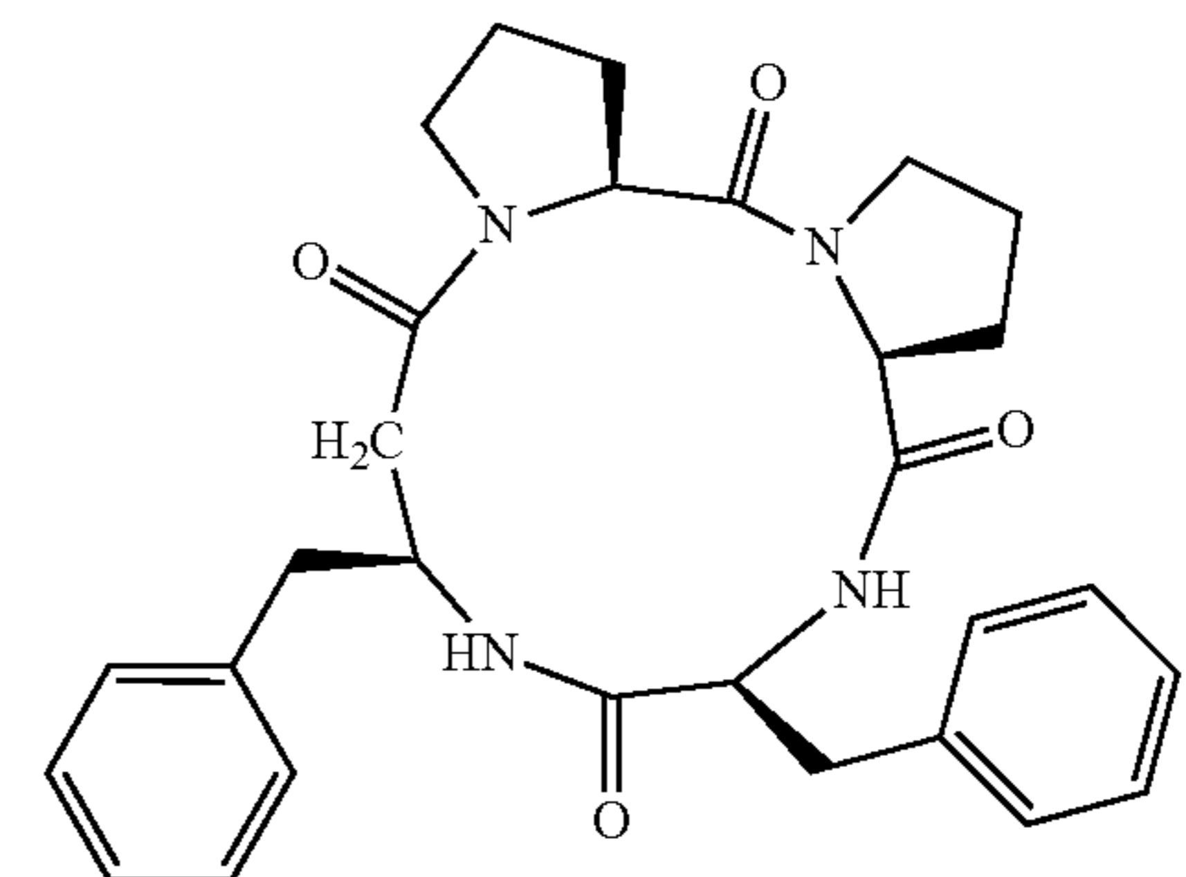
(cyclo(-L-Pro-L-Pro-L-Phe-LL-β 3 hoPhe-))
