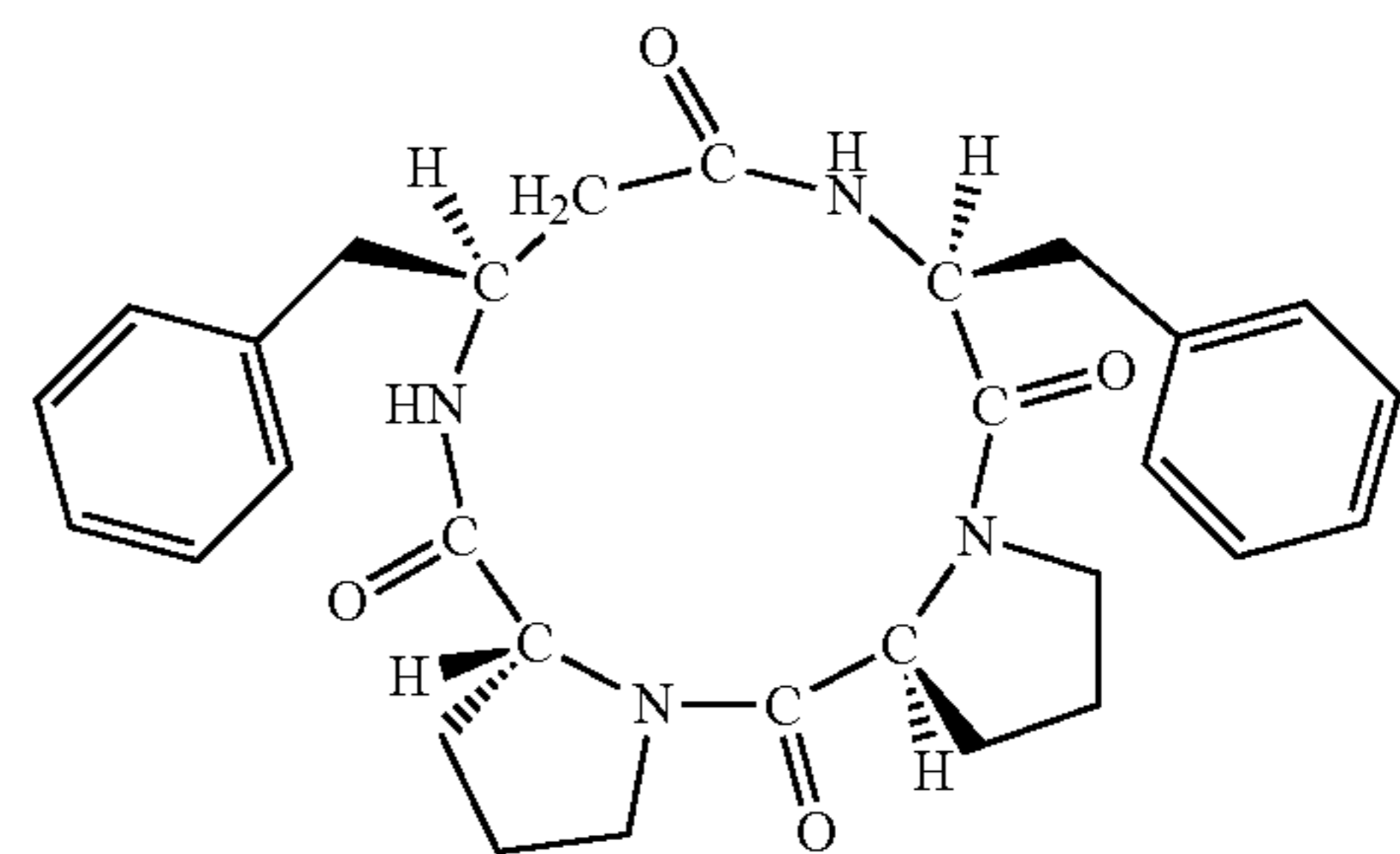
(cyclo(-L-Pro-D-Pro-L-β 3 HoPhe-L-Phe-))
