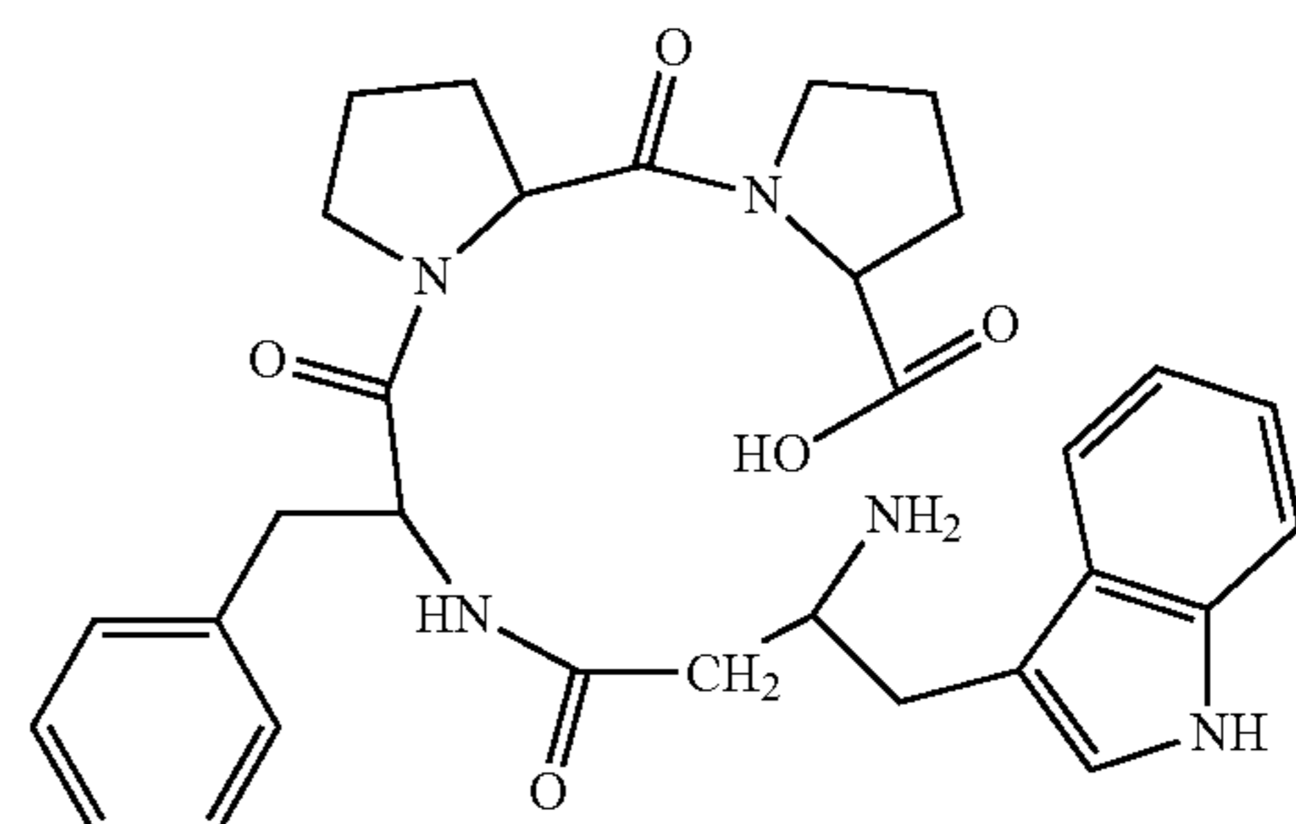
(H-β 3 hoTrp-Phe-Pro-Pro-OH)
