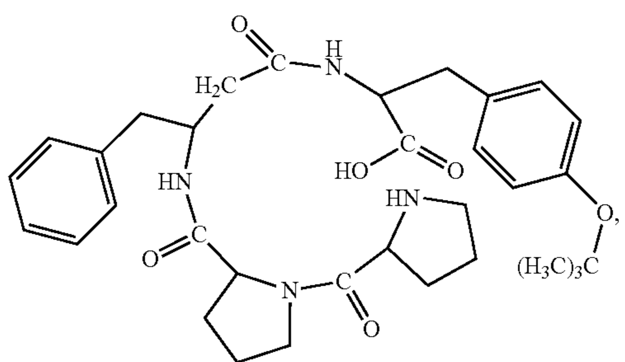
(H-Pro-Pro-β 3 hoPhe-Tyr(t-Bu)-OH)
