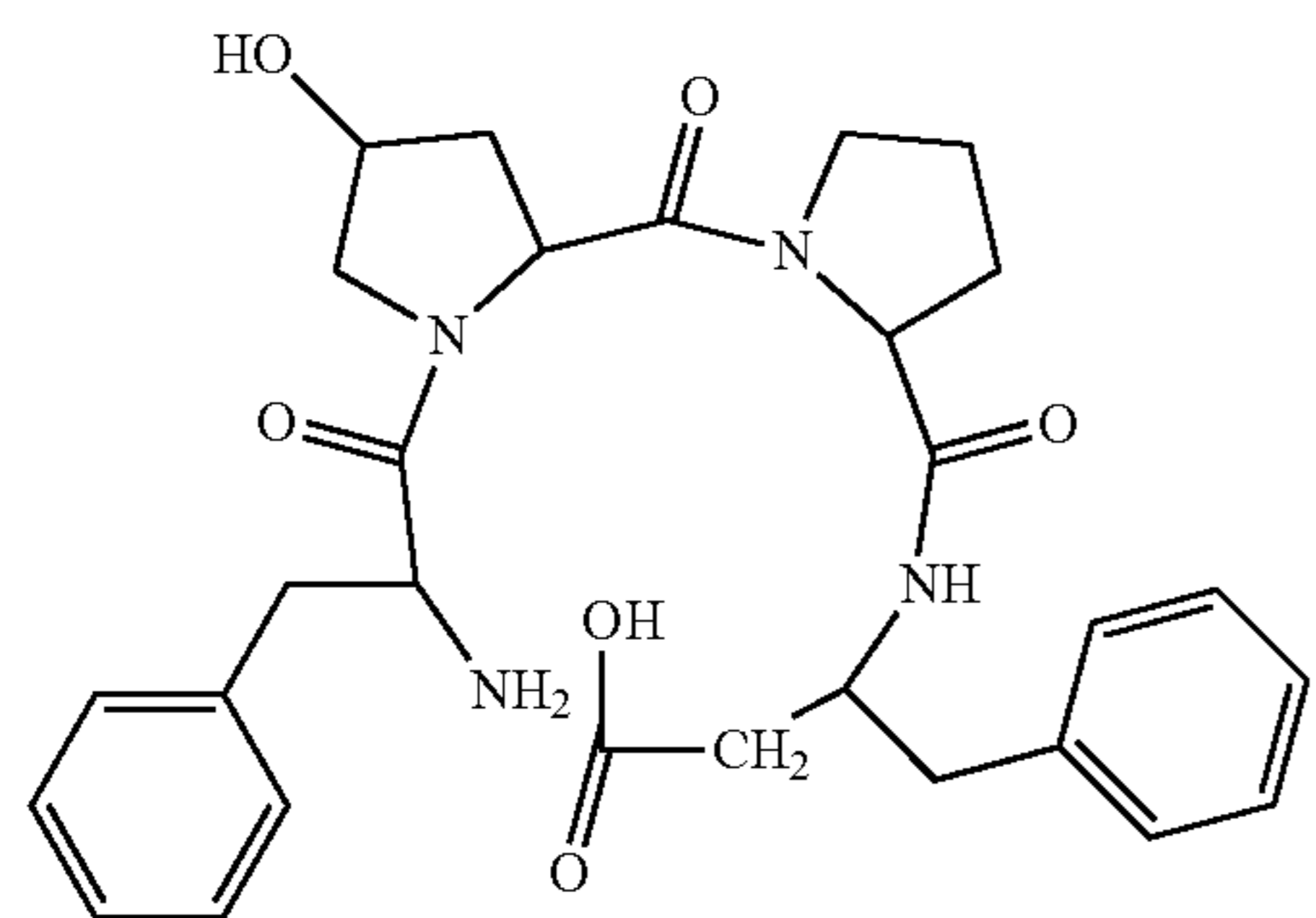
(H-Phe-Hyp-Pro-β³hoPhe-OH)
