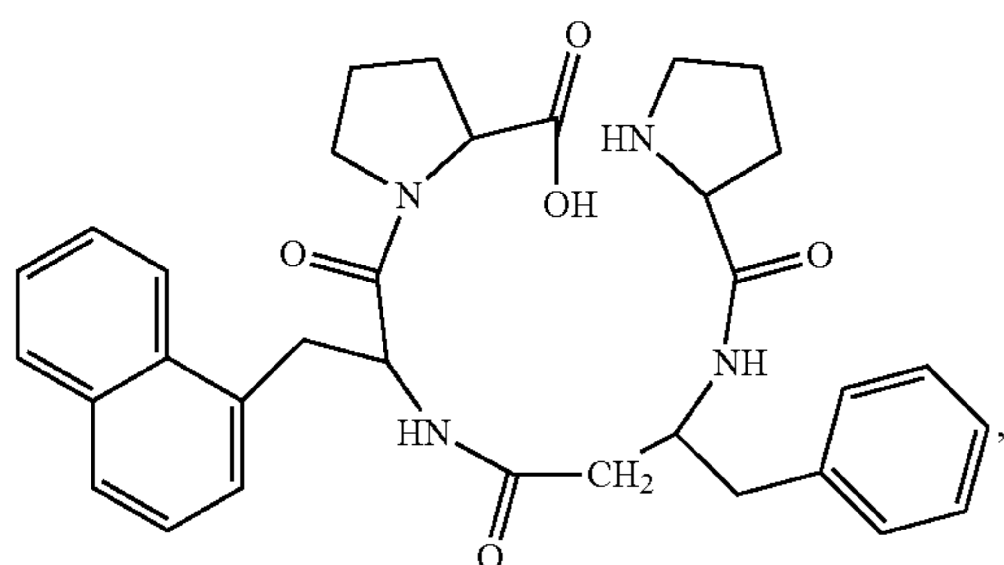
(H-Pro-β 3 hoPhe-1Nal-Pro-OH)
