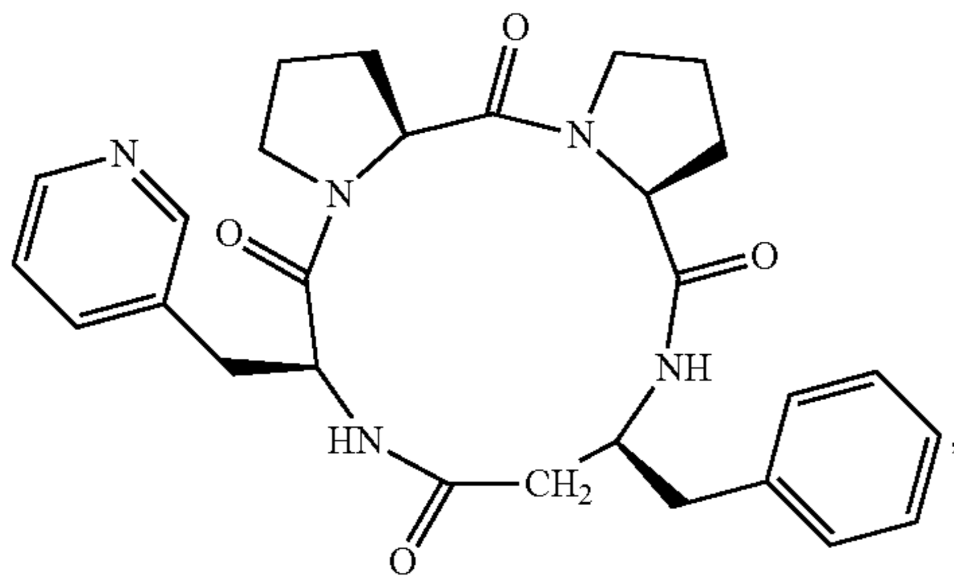
(cyclo(-L-Pro-L-Pro-L-β³hoPhe-L-3Pal))
