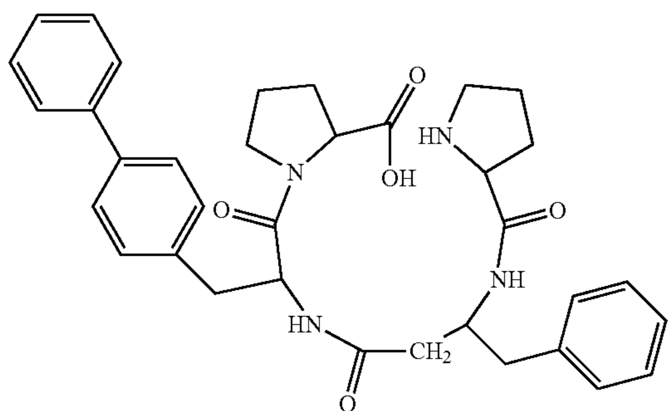
(H-Pro-β³hoPhe-Bip-Pro-OH)
