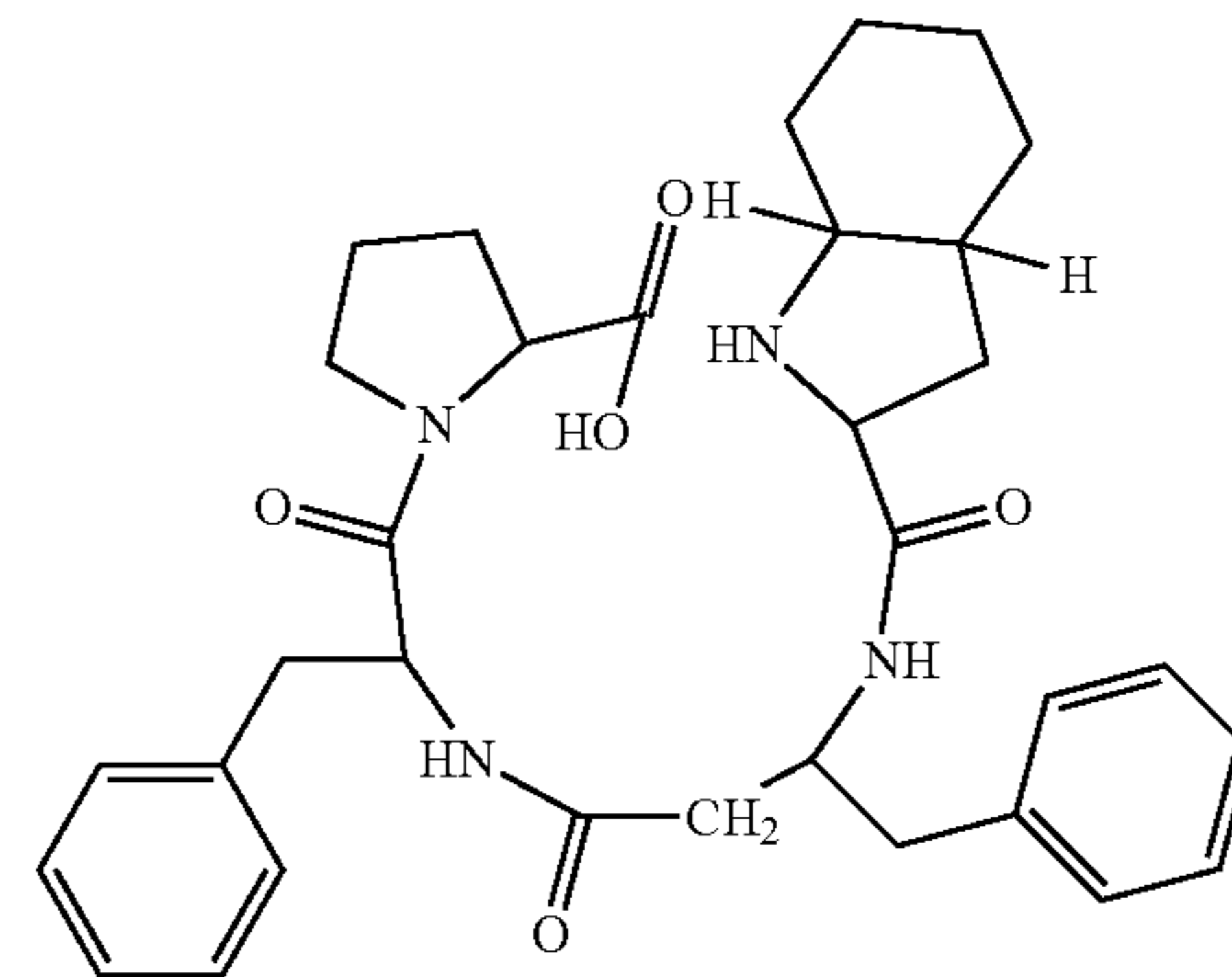
(H-Oic-β 3 hoPhe-Phe-Pro-OH)
