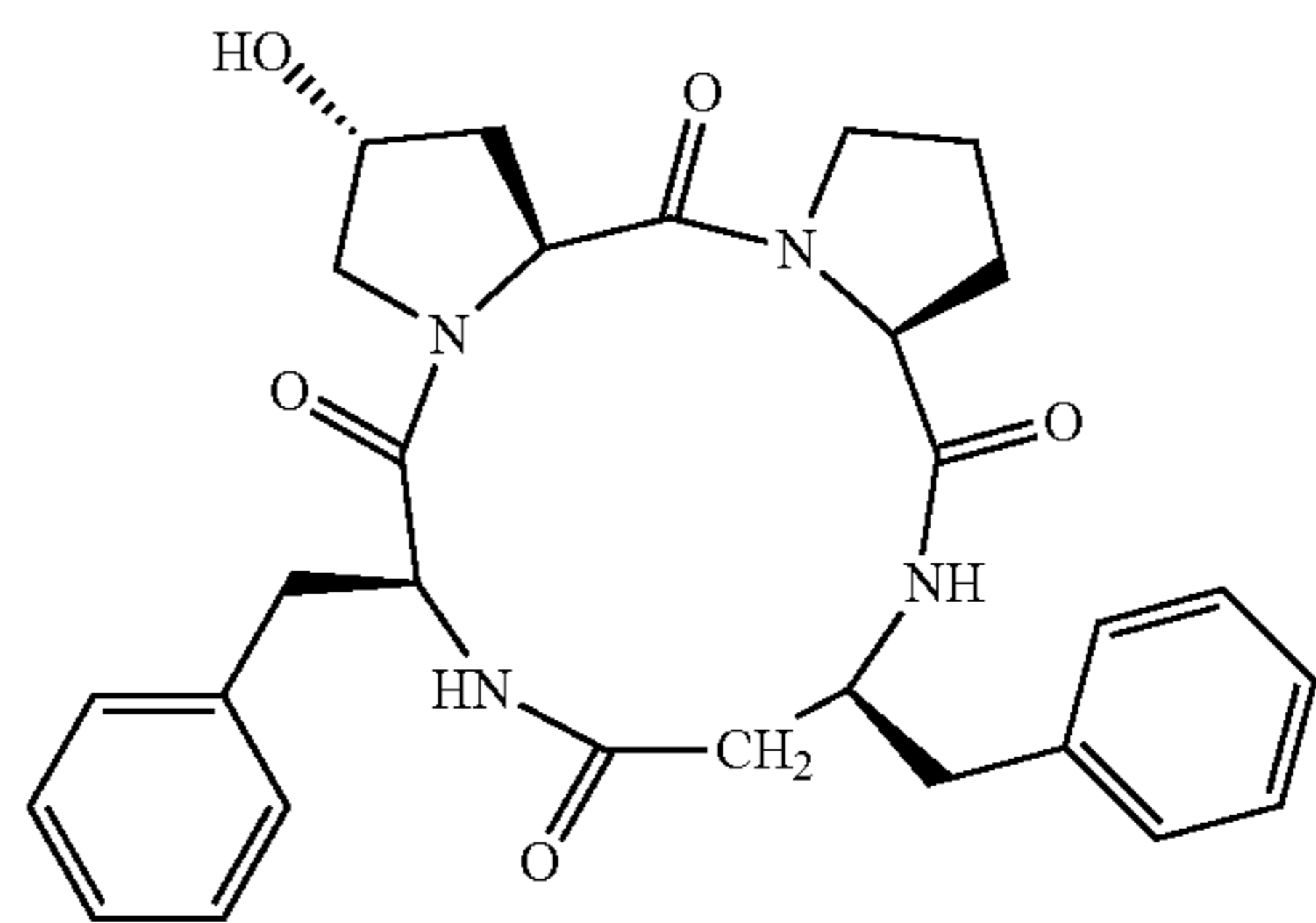
(cyclo(-L-Hyp-L-Pro-L-β 3 hoPhe-L-Phe-))
