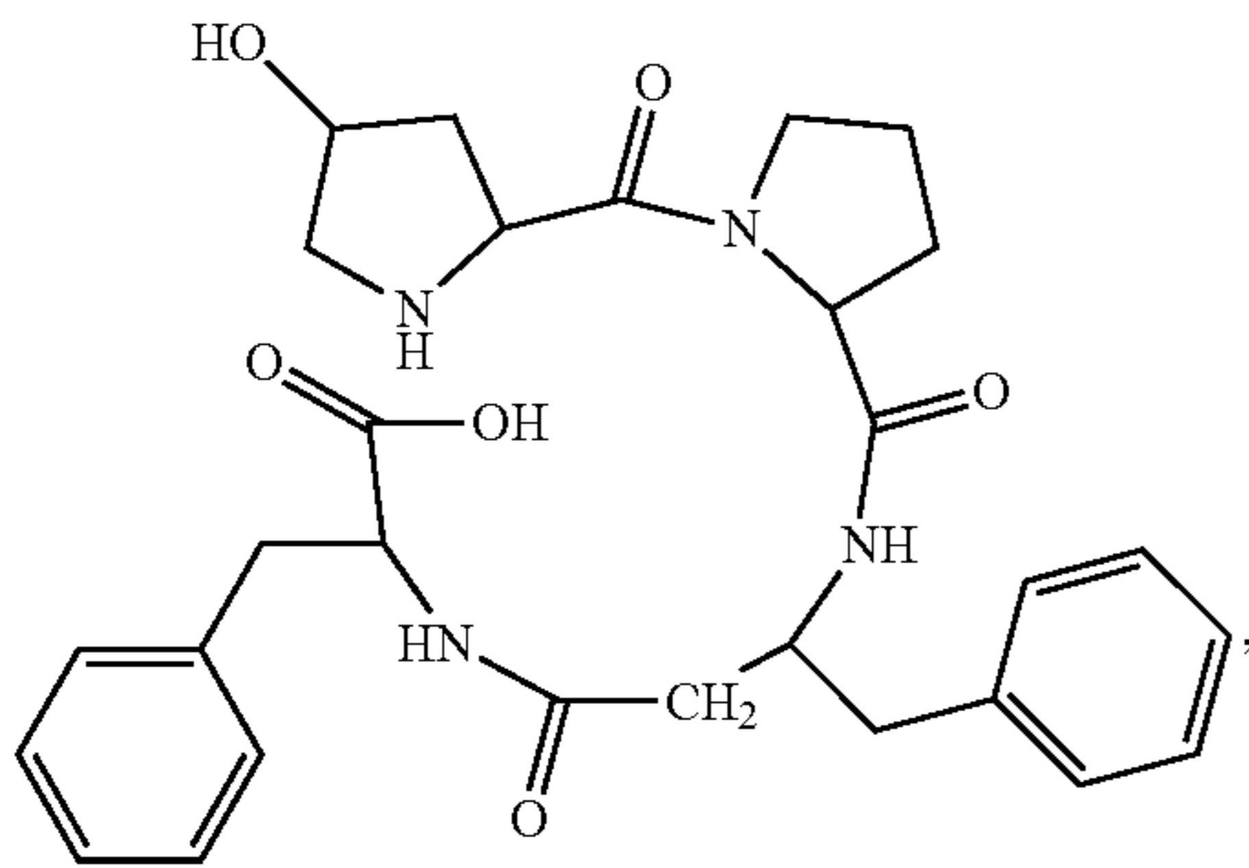
(H-Hyp-Pro-β³hoPhe-Phe-OH)
