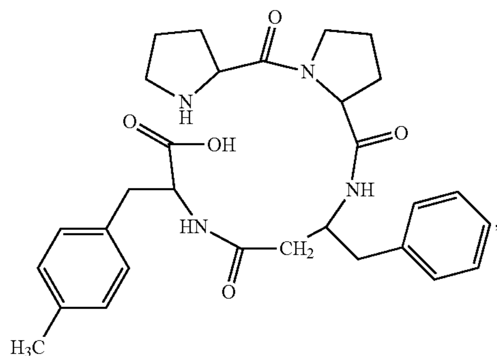
(H-Pro-Pro-β 3 hoPhe-Phe(4Me)-OH)
