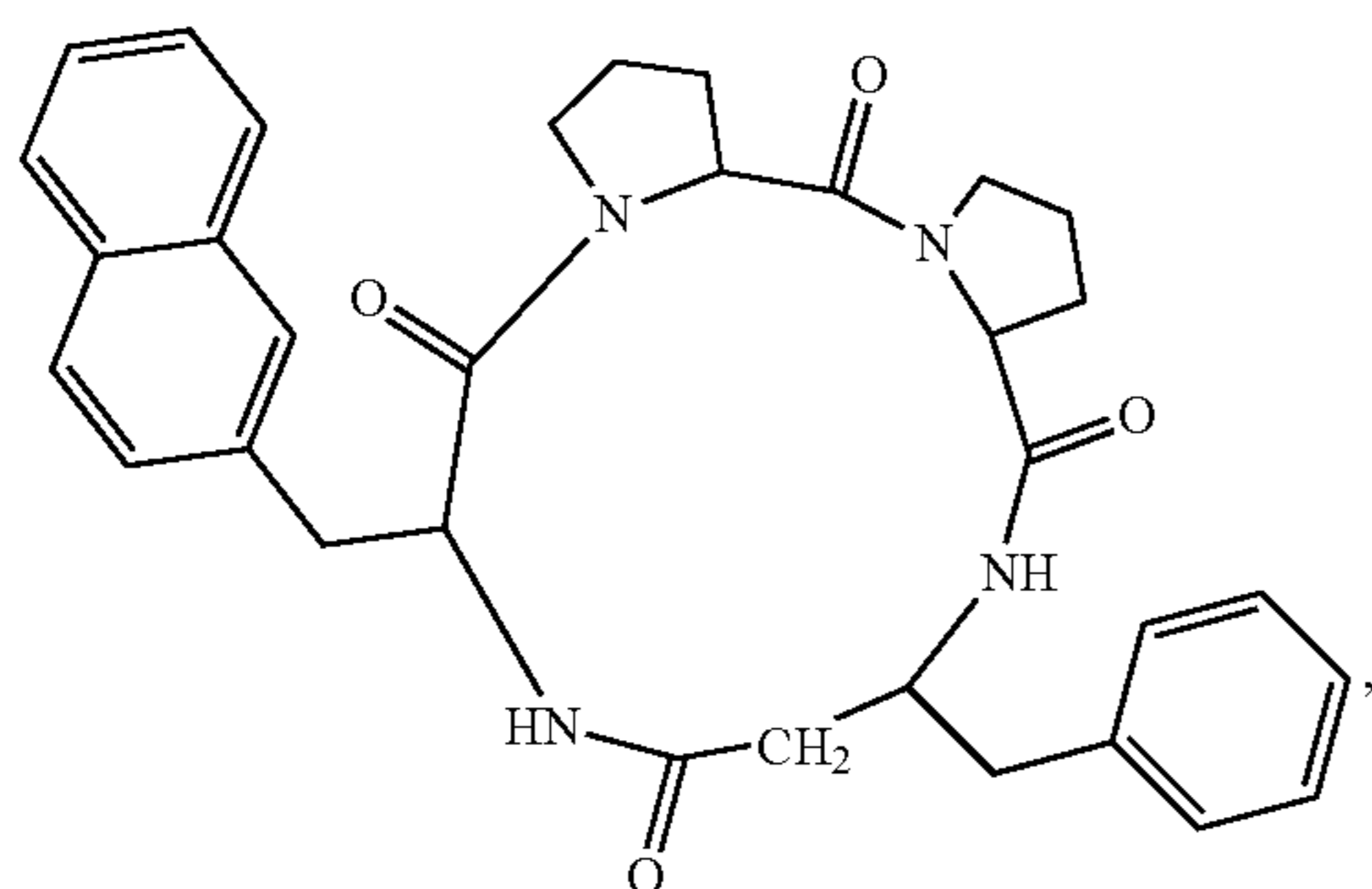
(cyclo(-Pro-Pro-β 3 hoPhe-2Nal))
