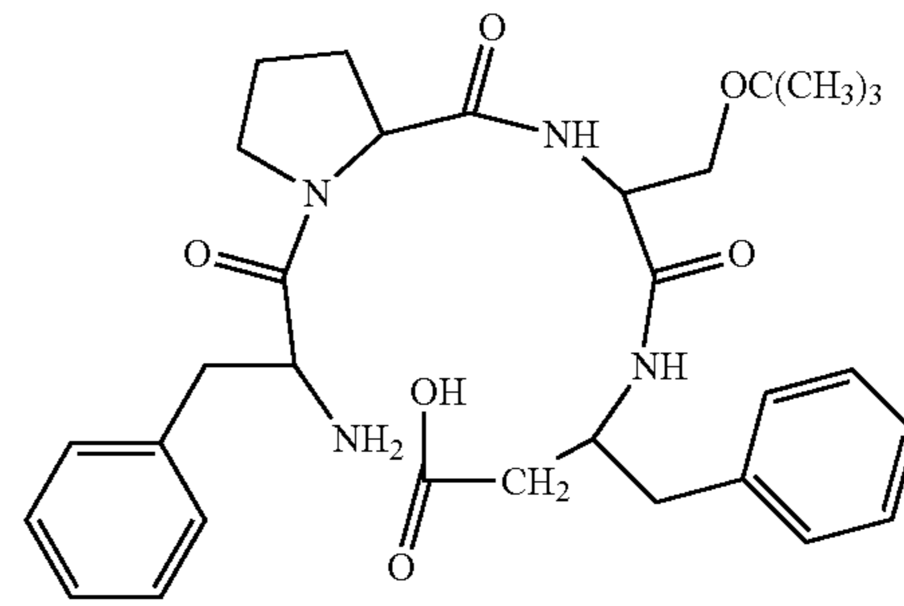
(H-Phe-Pro-Ser(tBu)-β³hoPhe-OH)
