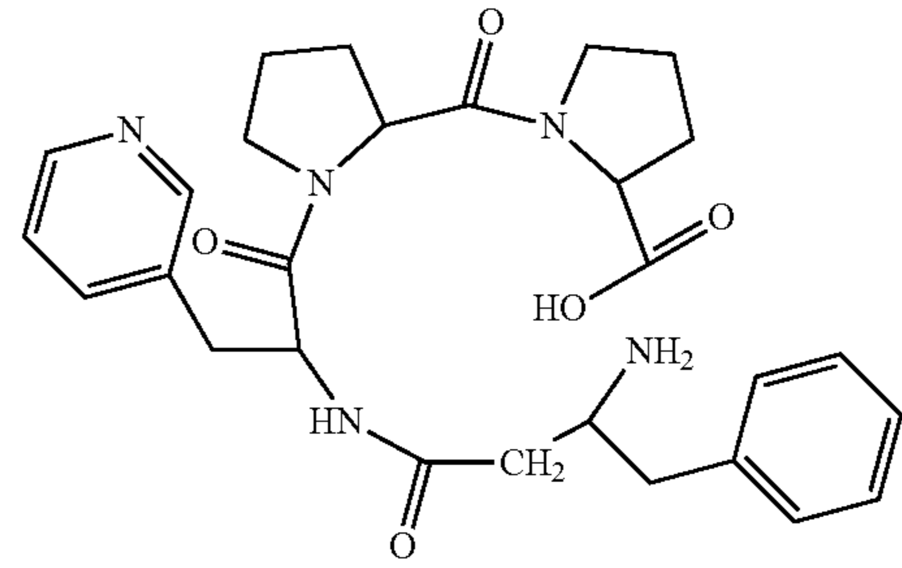
(H-β 3 hoPhe-Pal-Pro-Pro-OH)
