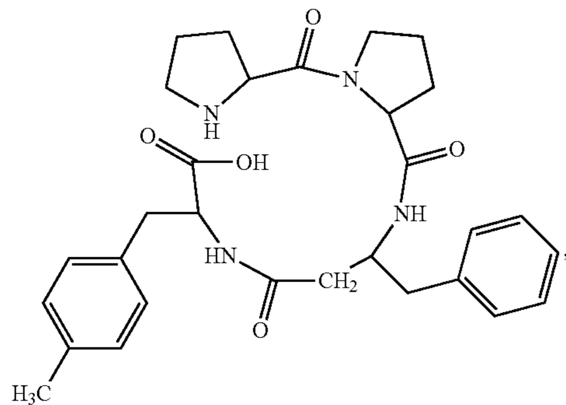
(H-Pro-Pro-β 3 hoPhe-Phe(4Me)-OH)
