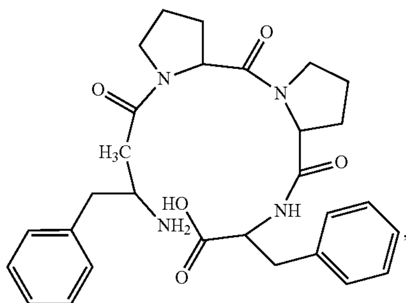
(H-β 3 hoPhe-Pro-Pro-Phe-OH)
