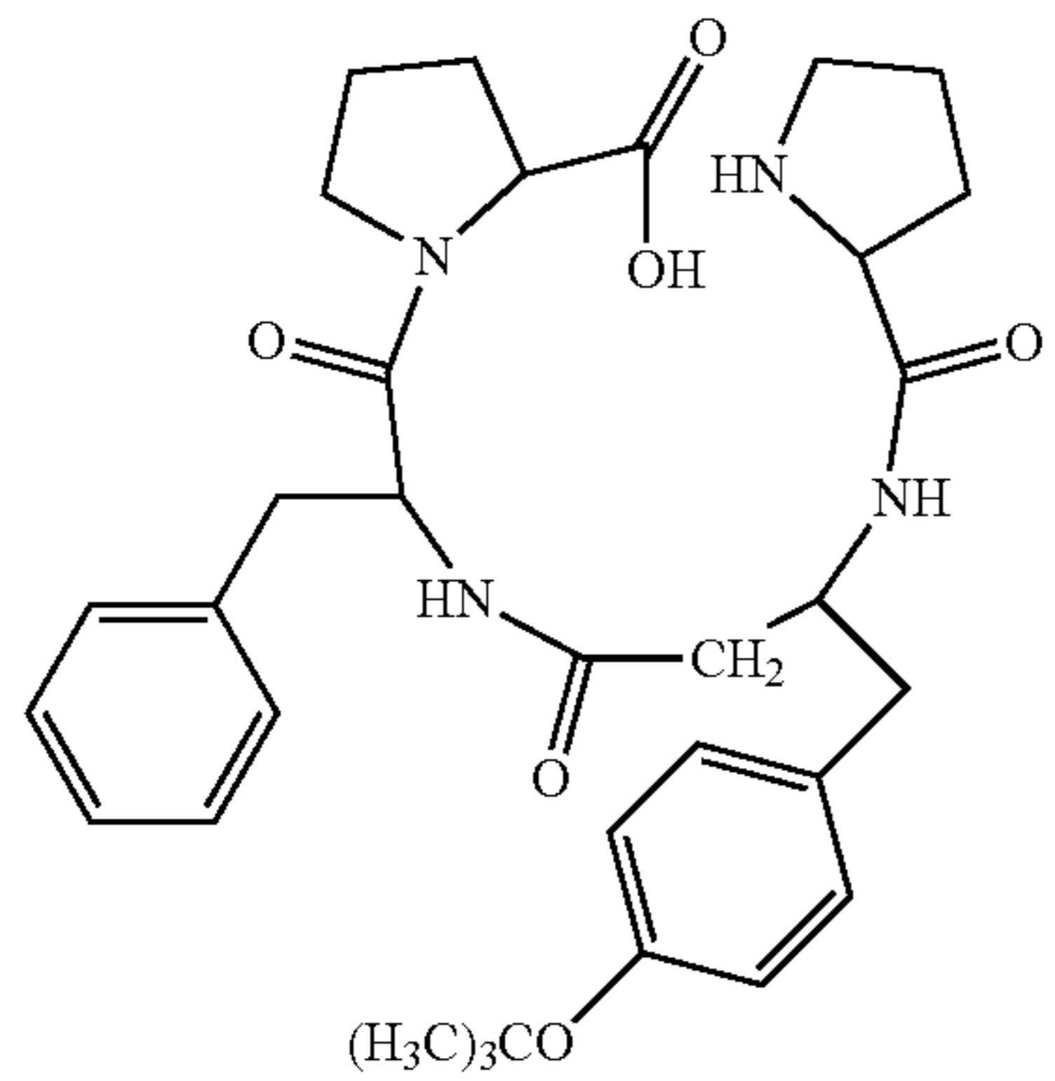
(H-Pro-β 3 hoTyr(tBu)-Pro-Pro-OH)
