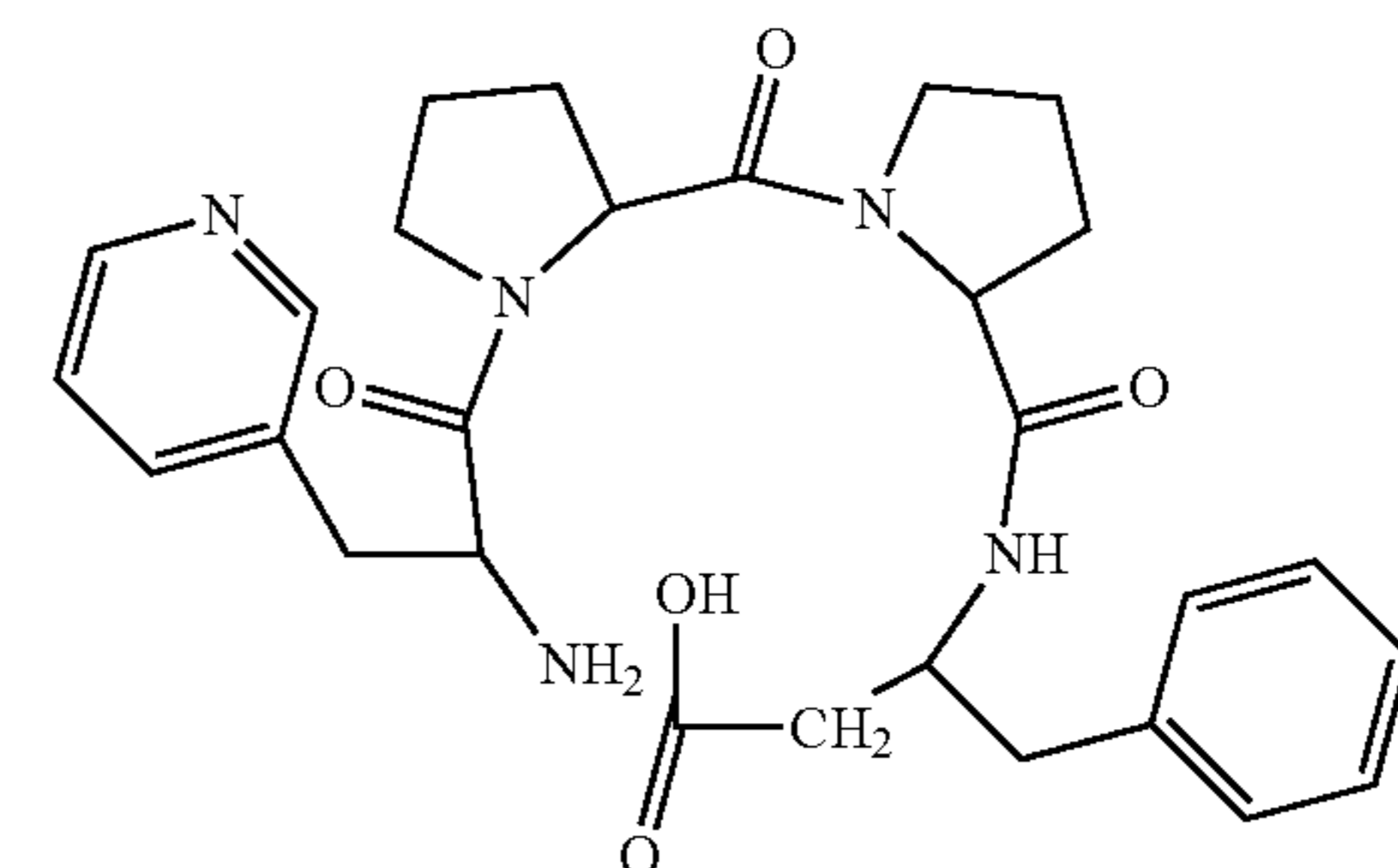
(H-Pal-Pro-Pro-β 3 hoPhe-OH)
