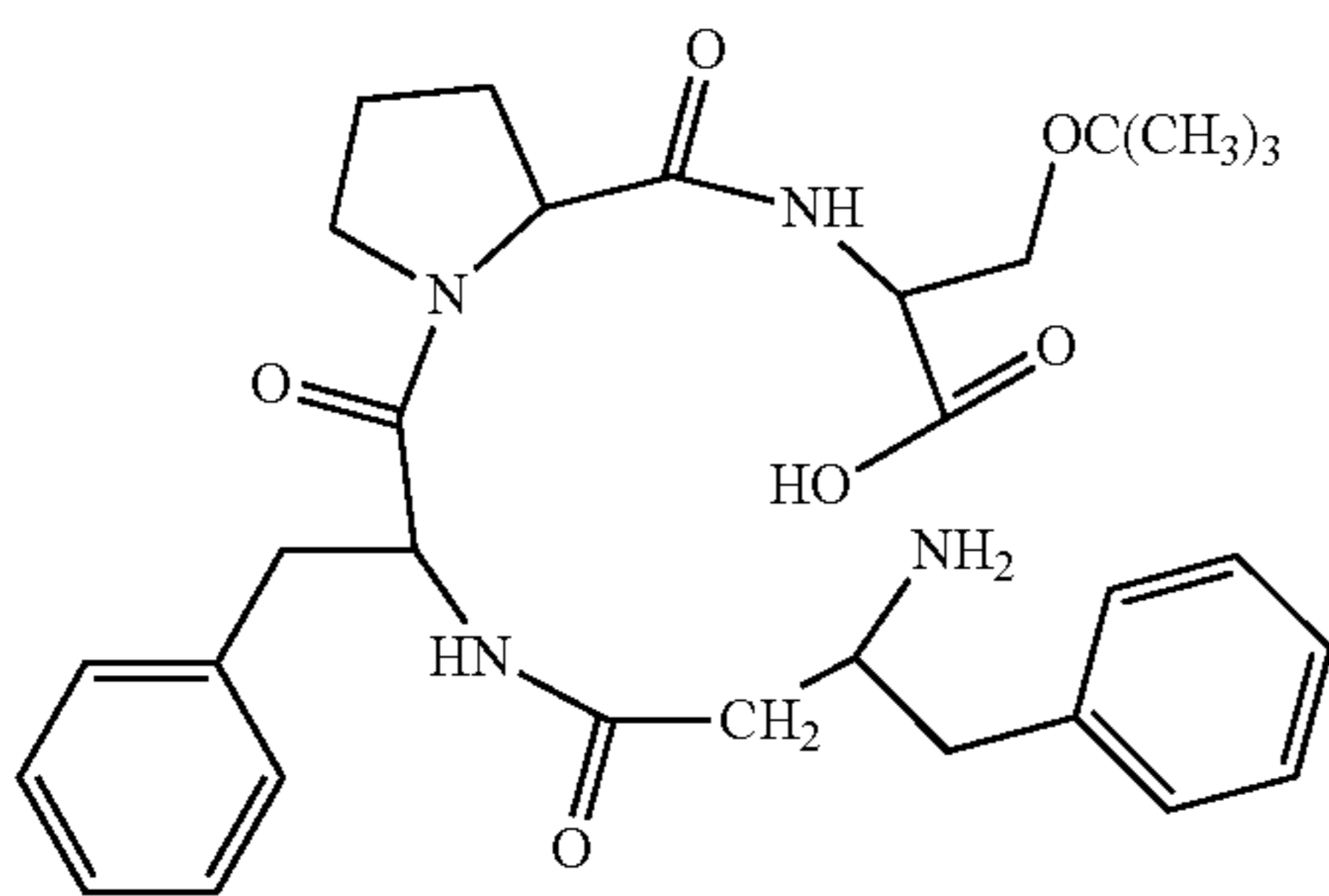
(H-β³hoPhe-Phe-Pro-Ser(tBu)-OH)
