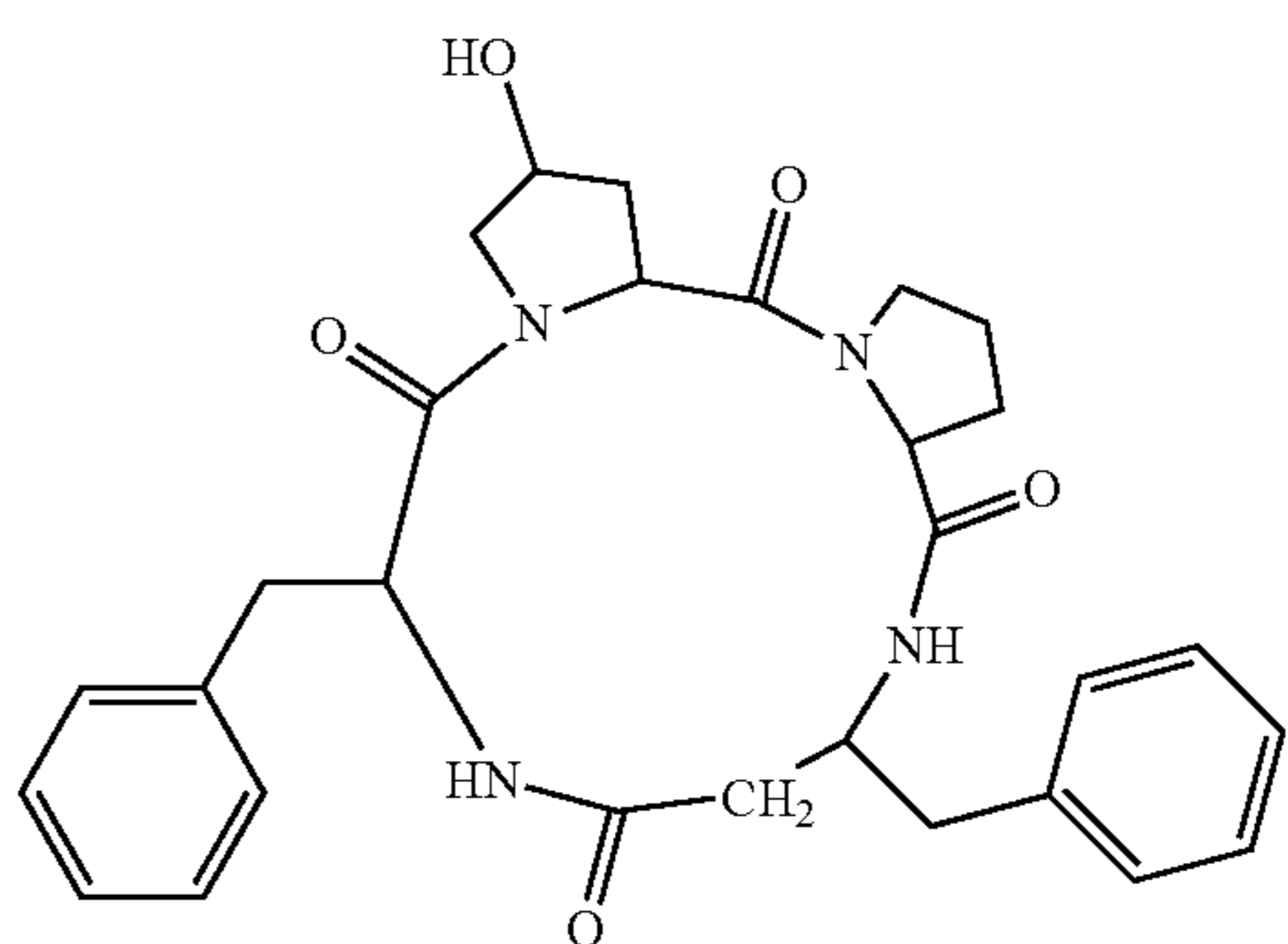
(cyclo(-Hyp-Pro-β³hoPhe-Phe-))
