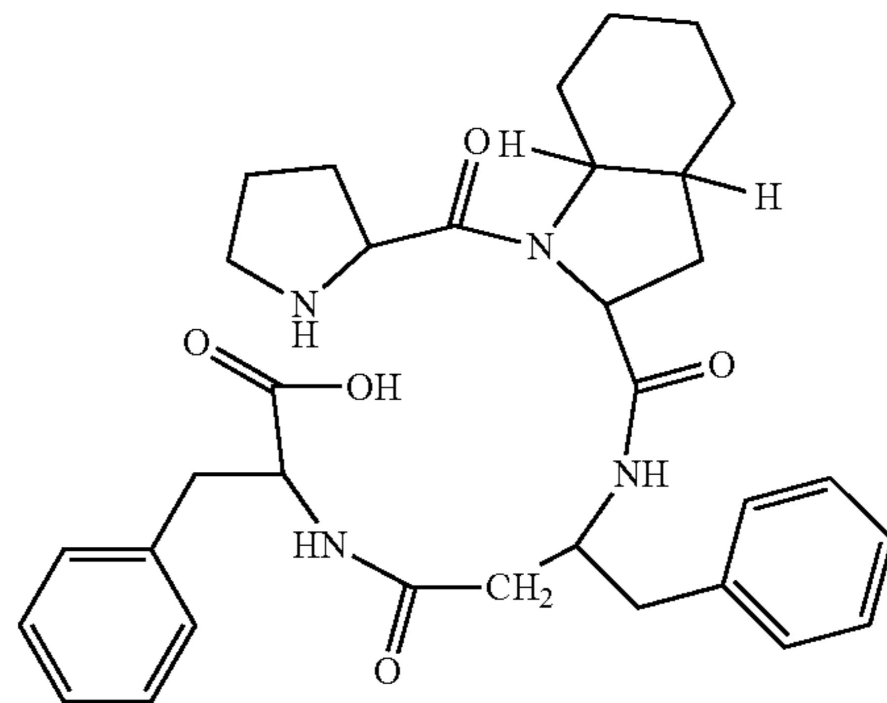
(H-Pro-Oic-β 3 hoPhe-Phe-OH)
