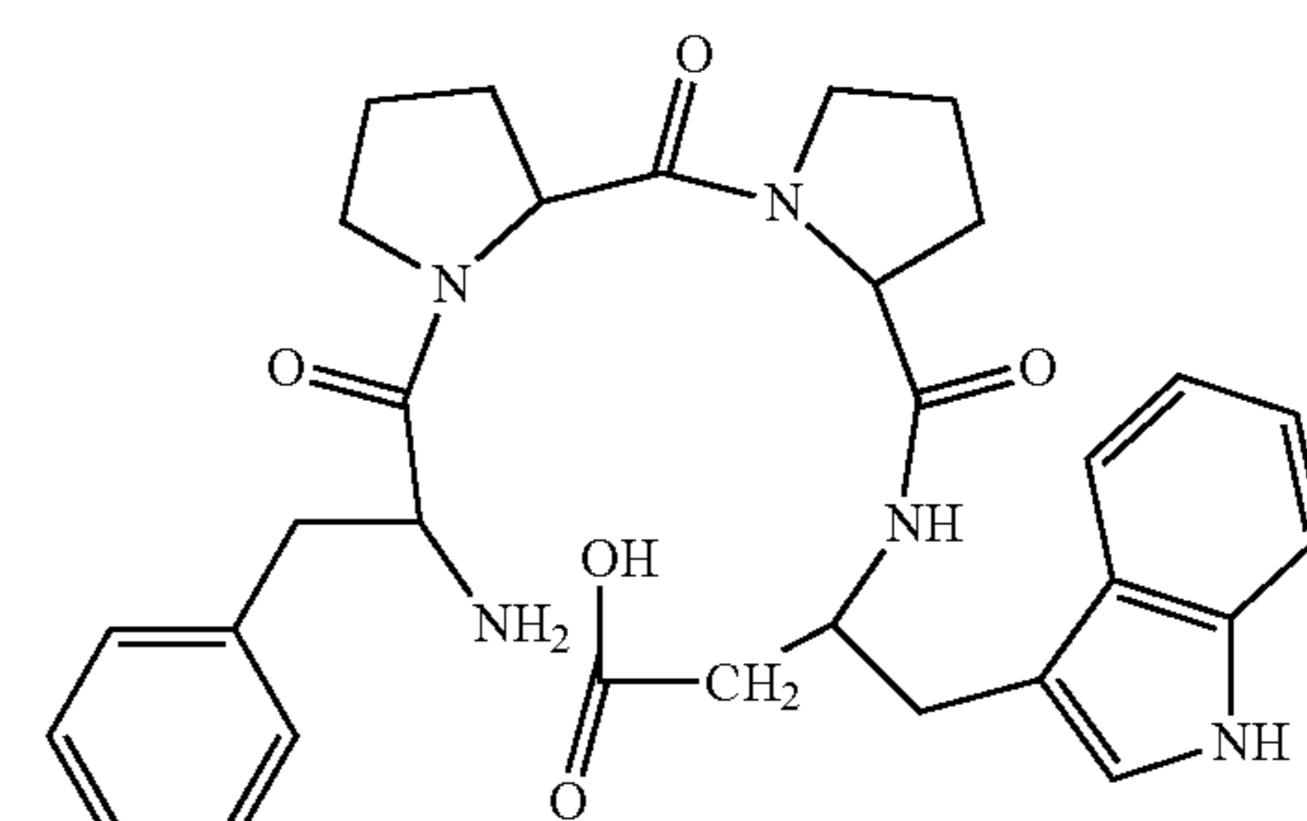
(H-Phe-Pro-Pro-β 3 hoTrp-OH)
