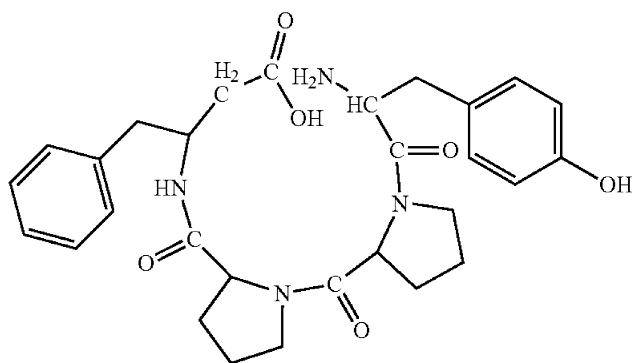
(H-Tyr-Pro-Pro-β 3 hoPhe-OH)
