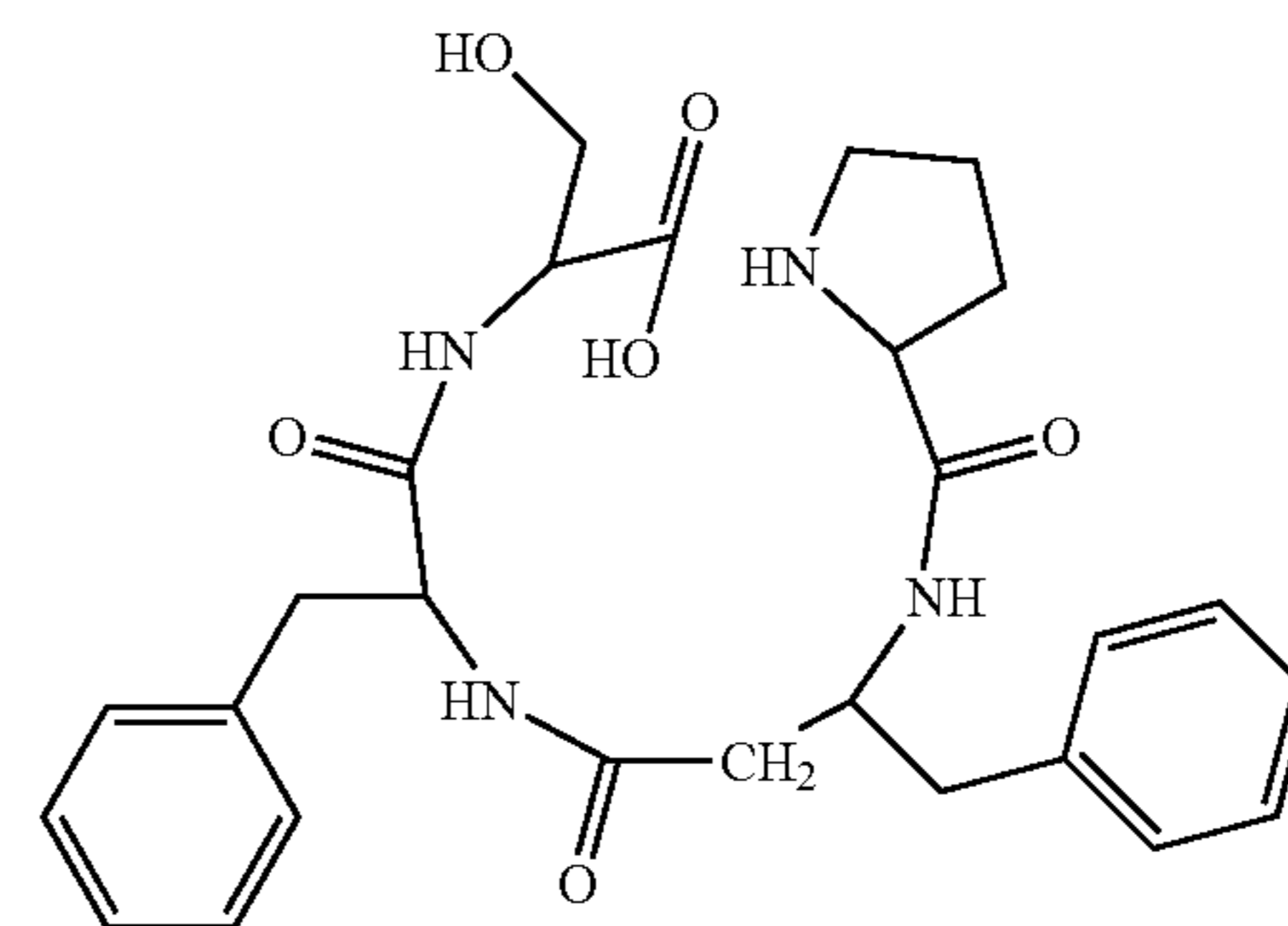
(H-Pro-β³hoPhe-Phe-Ser-OH)
