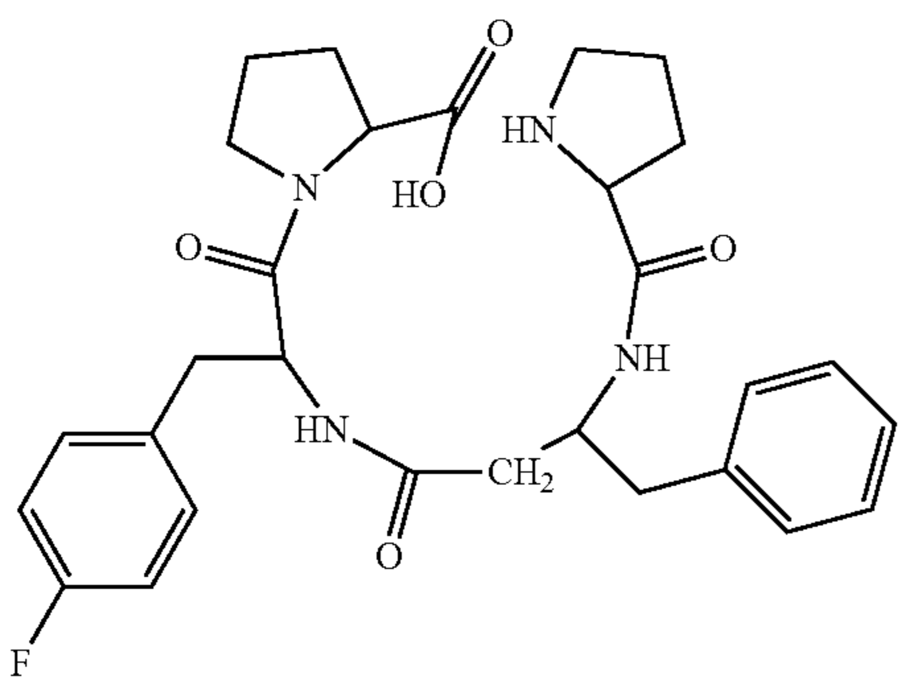
(H-Pro-β 3 hoPhe-Phe(4F)-Pro-OH)
