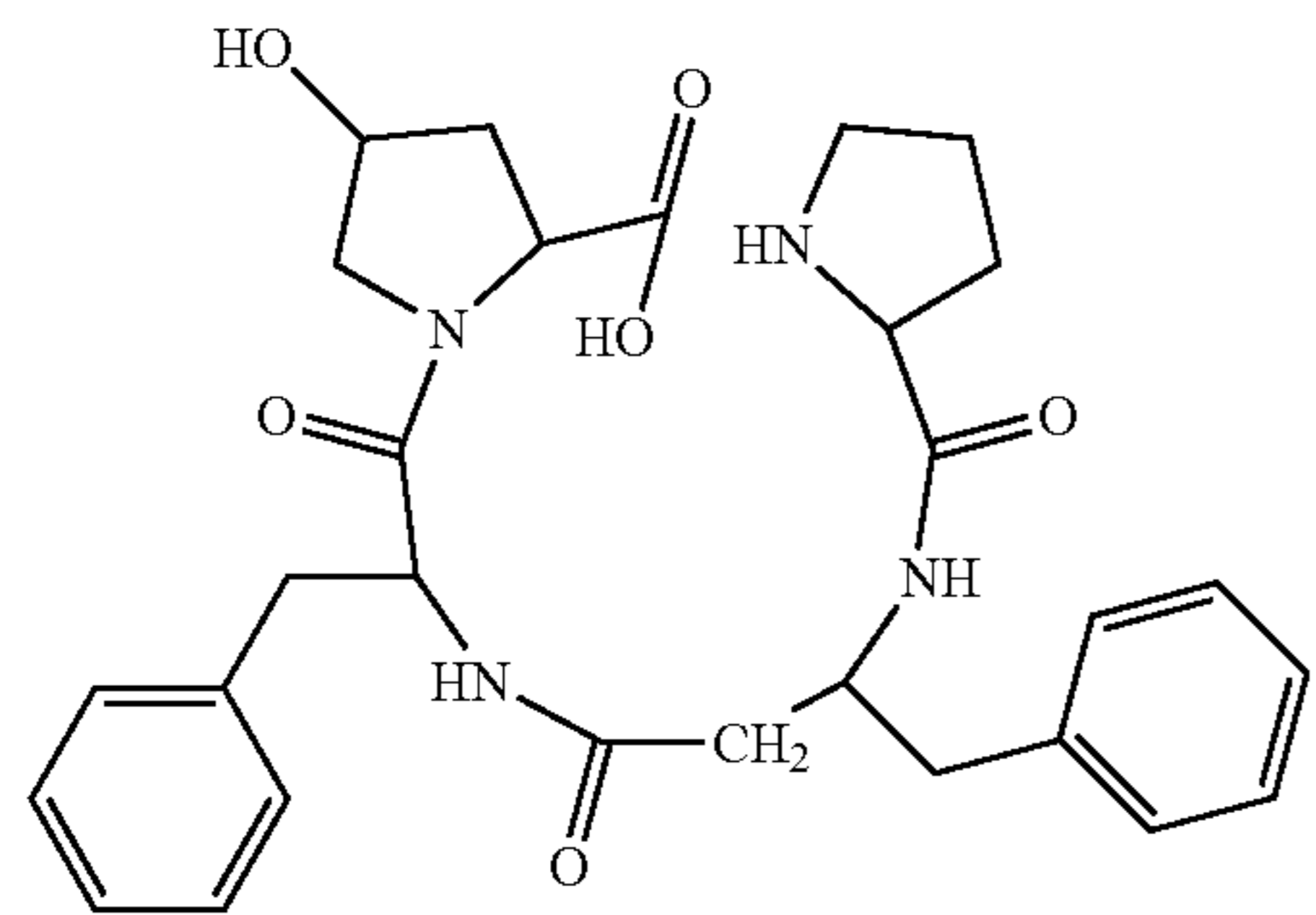
(H-Pro-β³hoPhe-Phe-Hyp-OH)
