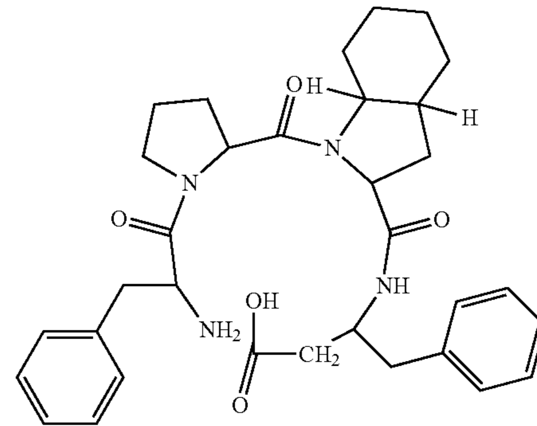
(H-Phe-Pro-Oic-β 3 hoPhe-OH)
