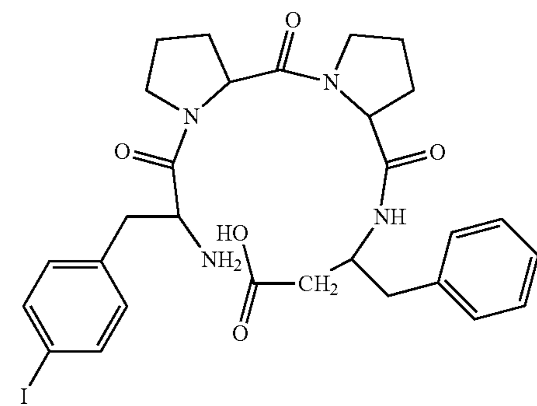
(H-Phe(4I)-Pro-Pro-β 3 hoPhe-OH)
