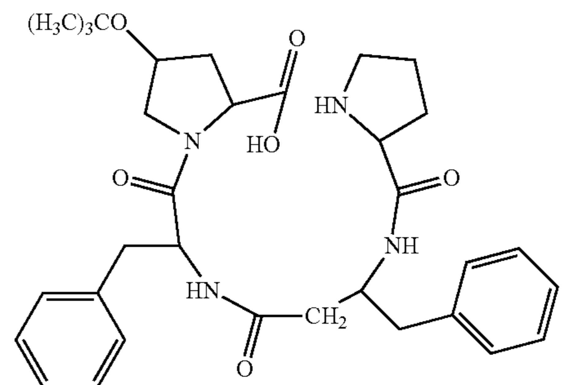
(H-Pro-β 3 hoPhe-Phe-Hyp(tBu)-OH)
