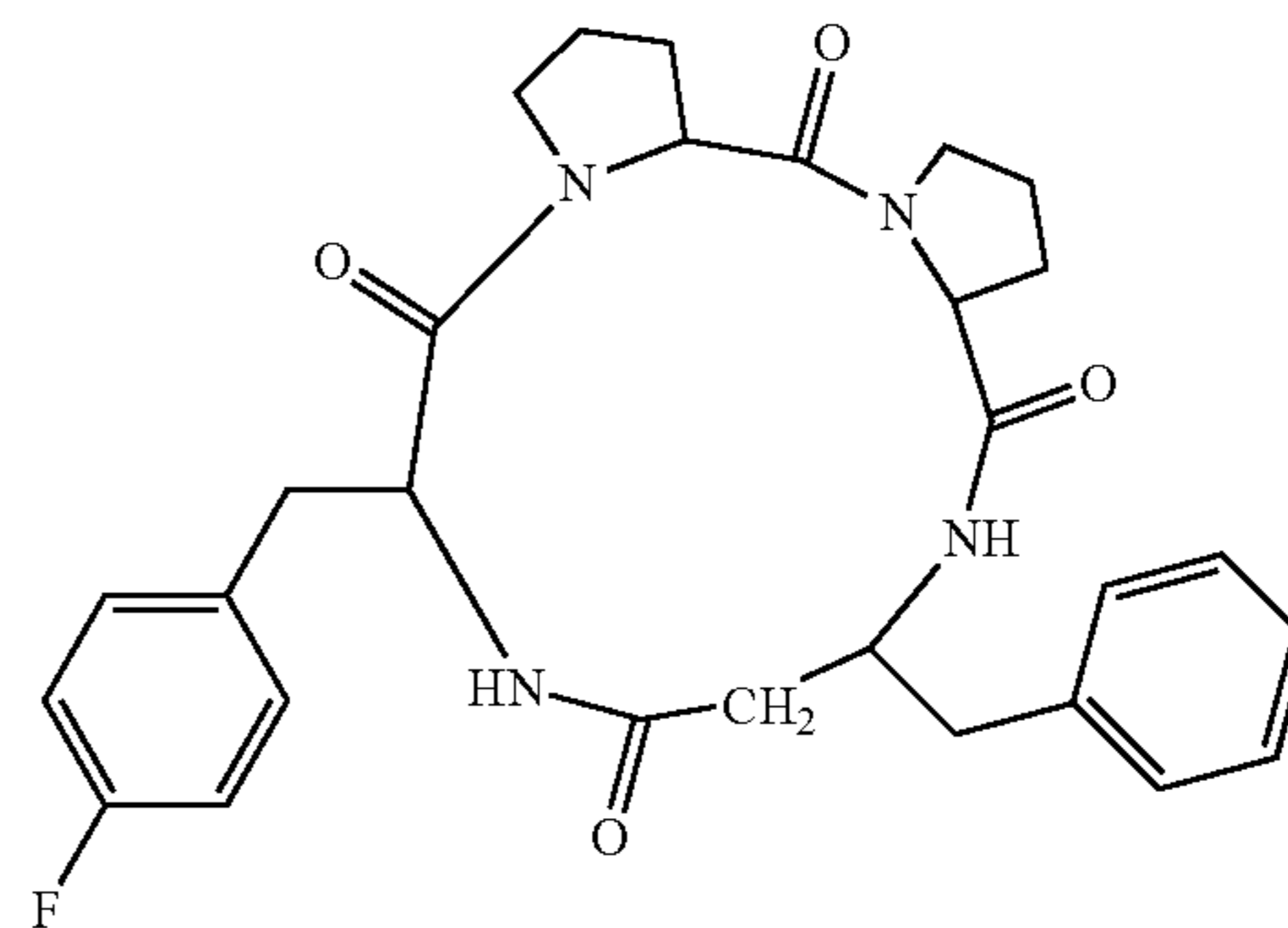
(cyclo(-Pro-Pro-β³hoPhe-Phe(4F)))
