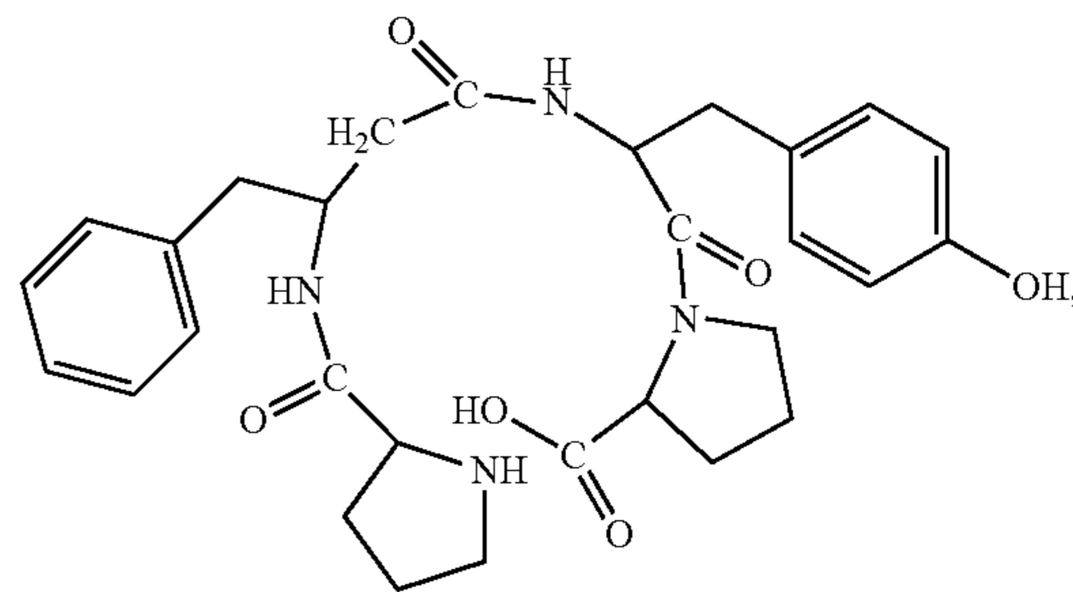
(H-Pro-β 3 hoPhe-Tyr-Pro-OH)
