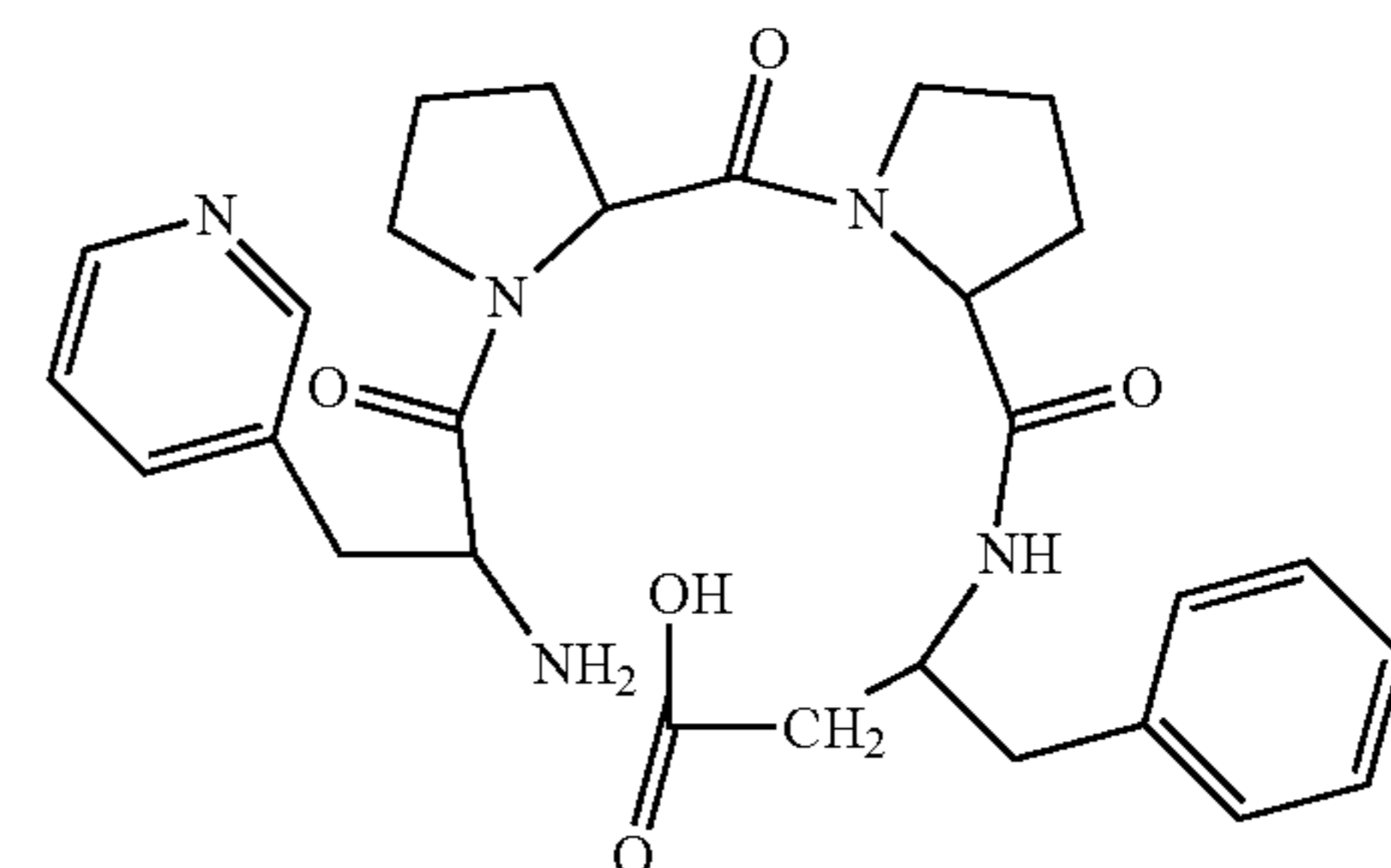
(H-Pal-Pro-Pro-β 3 hoPhe-OH)
