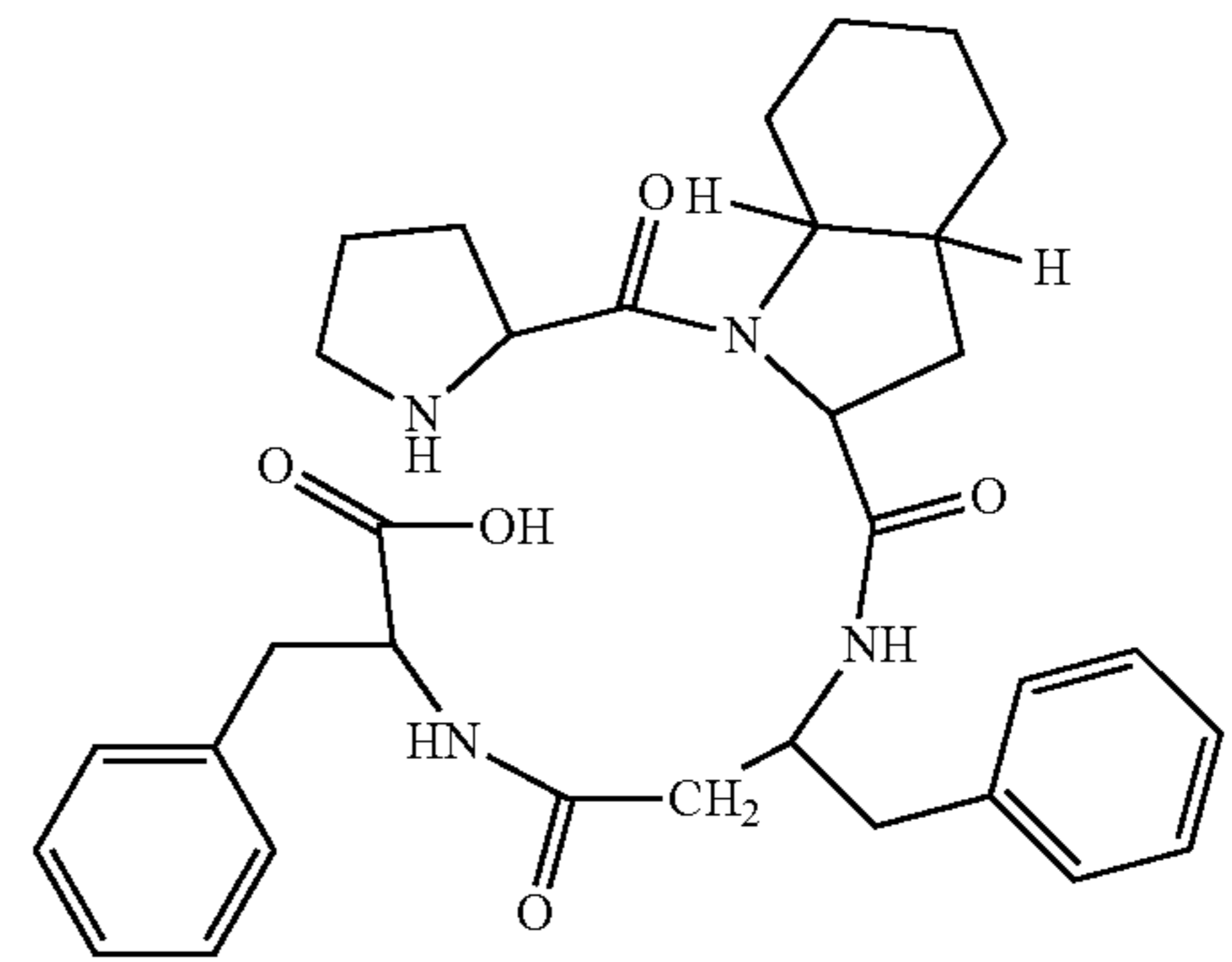
(H-Pro-Oic-β 3 hoPhe-Phe-OH)
