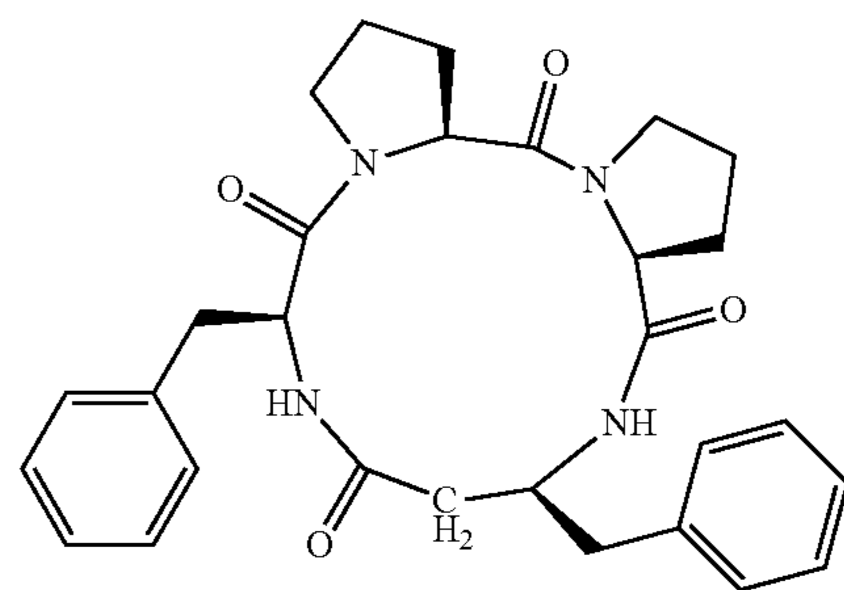
((cyclo(-L-Pro-L-Pro-L-β 3 hoPhe-L-Phe-))
