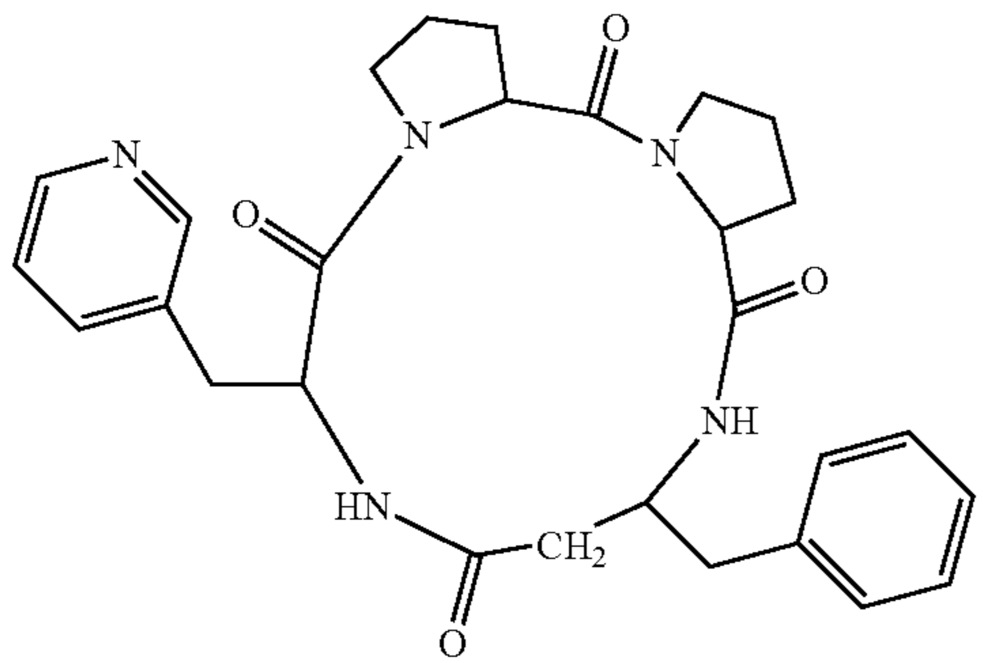
(cyclo(-Pro-Pro-β³hoPhe-3Pal))
