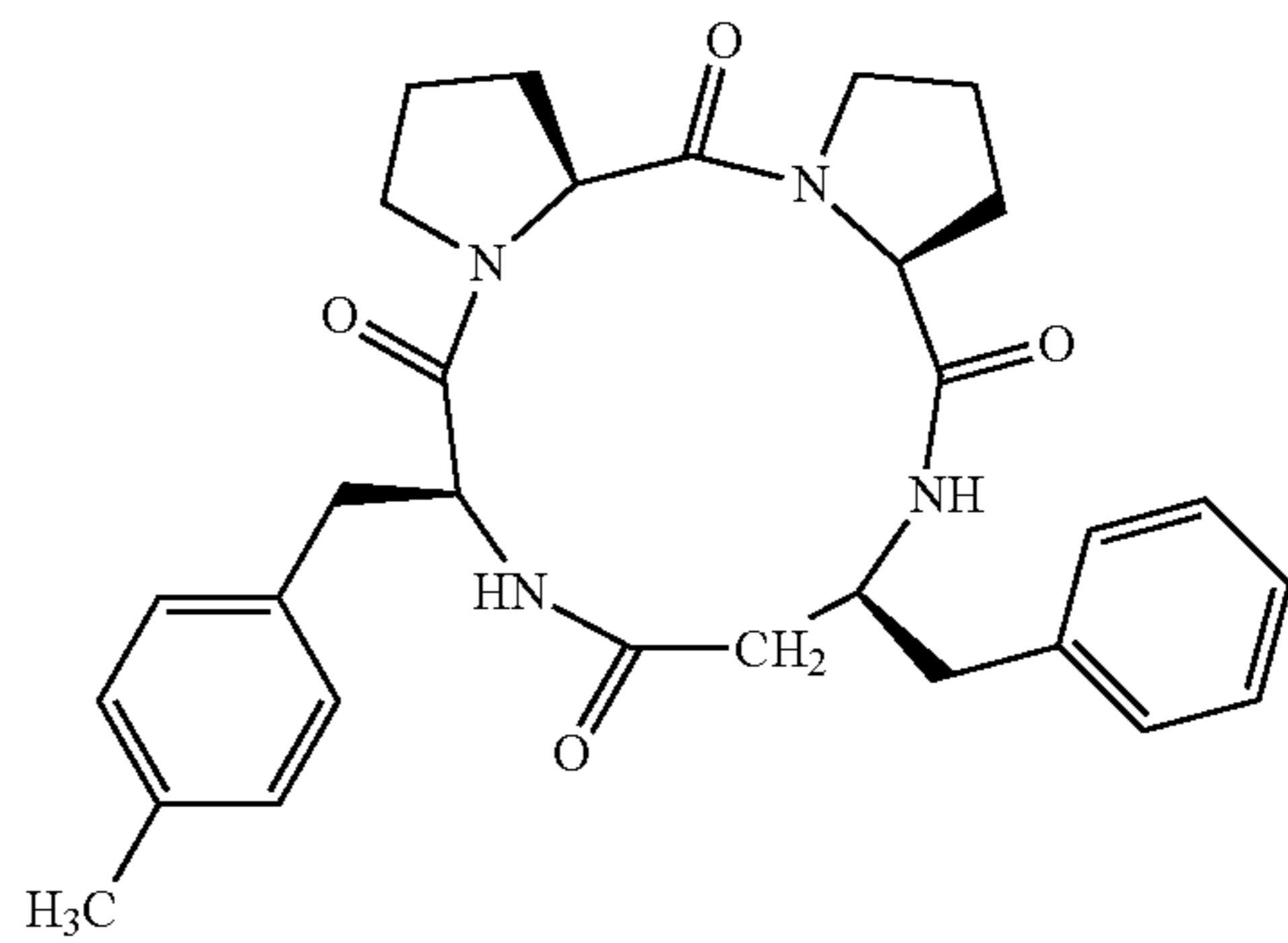
cyclo(-L-Pro-L-Pro-L-β³hoPhe-L-Phe(4Me))
