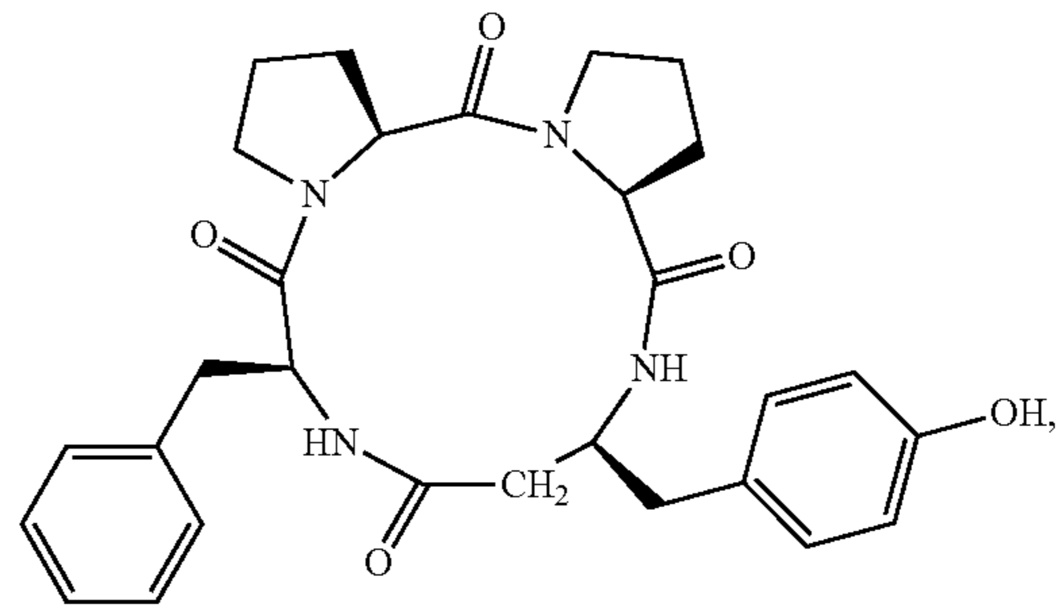
(cyclo(-L-Pro-L-Pro-L-β³hoTyr-L-Phe))
