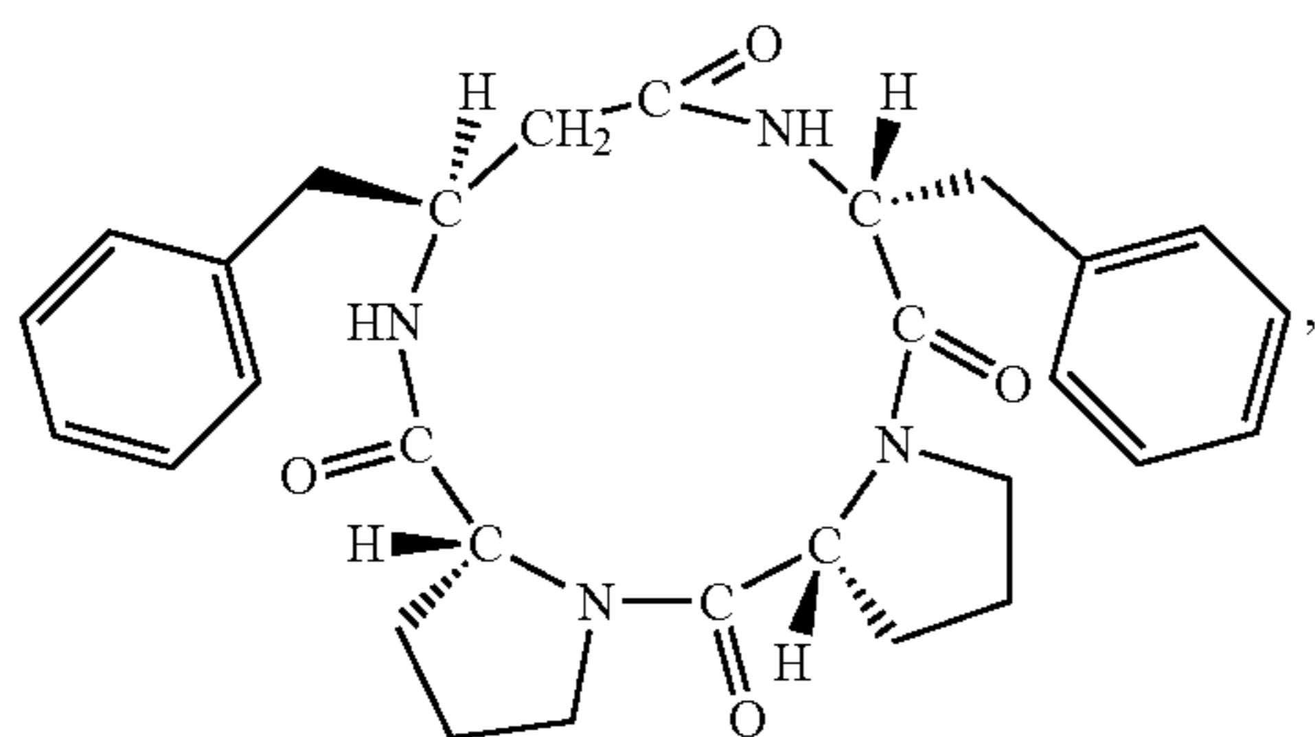
(cyclo(-D-Pro-D-Pro-L-β 3 HoPhe-D-Phe-))
