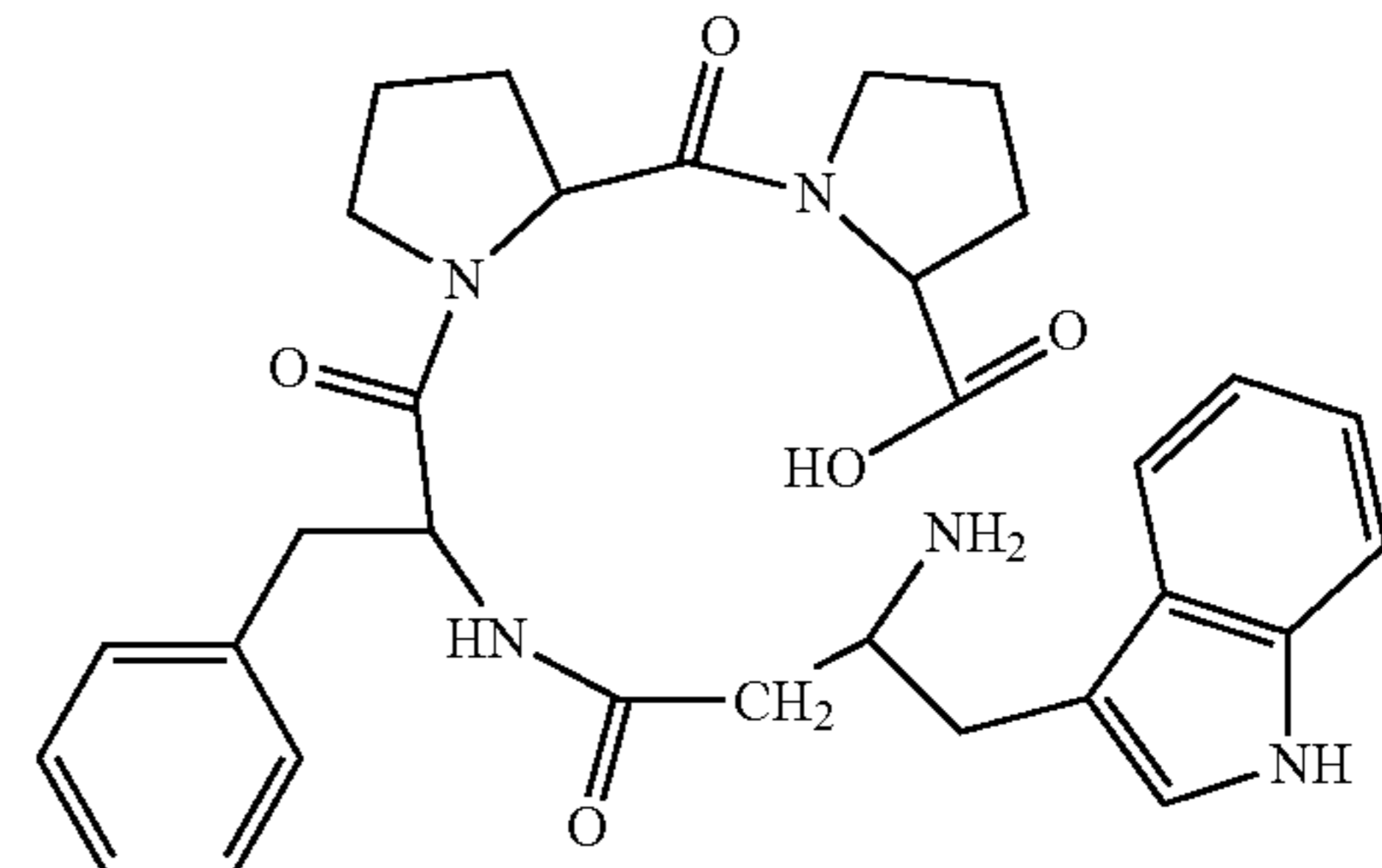
(H-β 3 hoTrp-Phe-Pro-Pro-OH)
