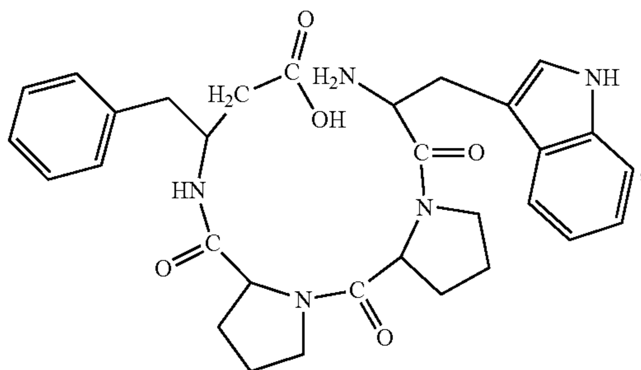
(H-Trp-Pro-Pro-β 3 hoPhe-OH)
