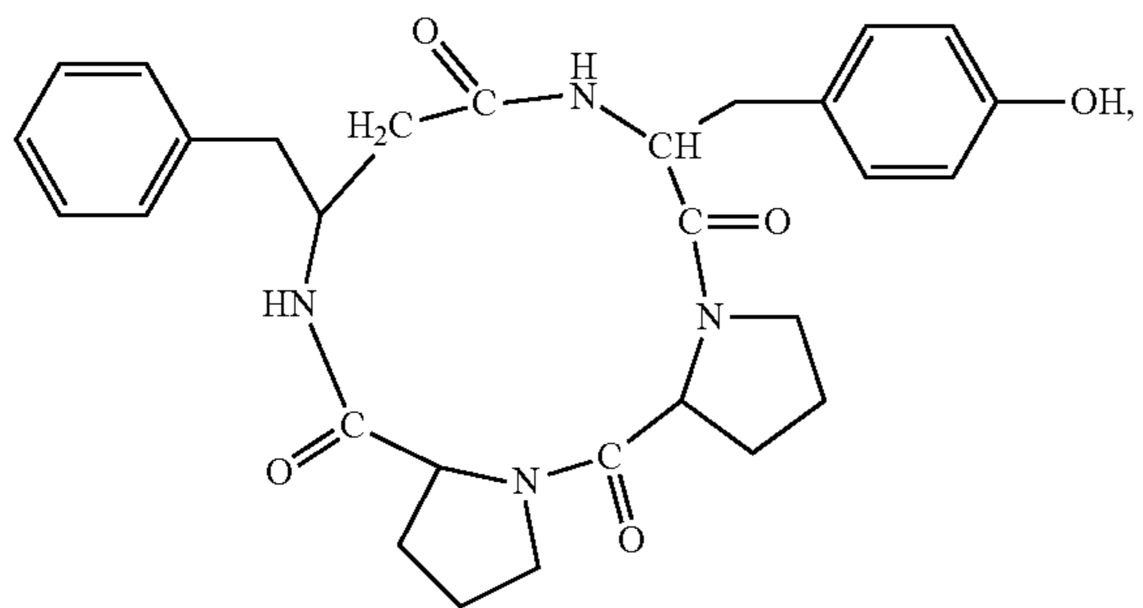
(cyclo(-Pro-Pro-β 3 hoPhe-Tyr-))
