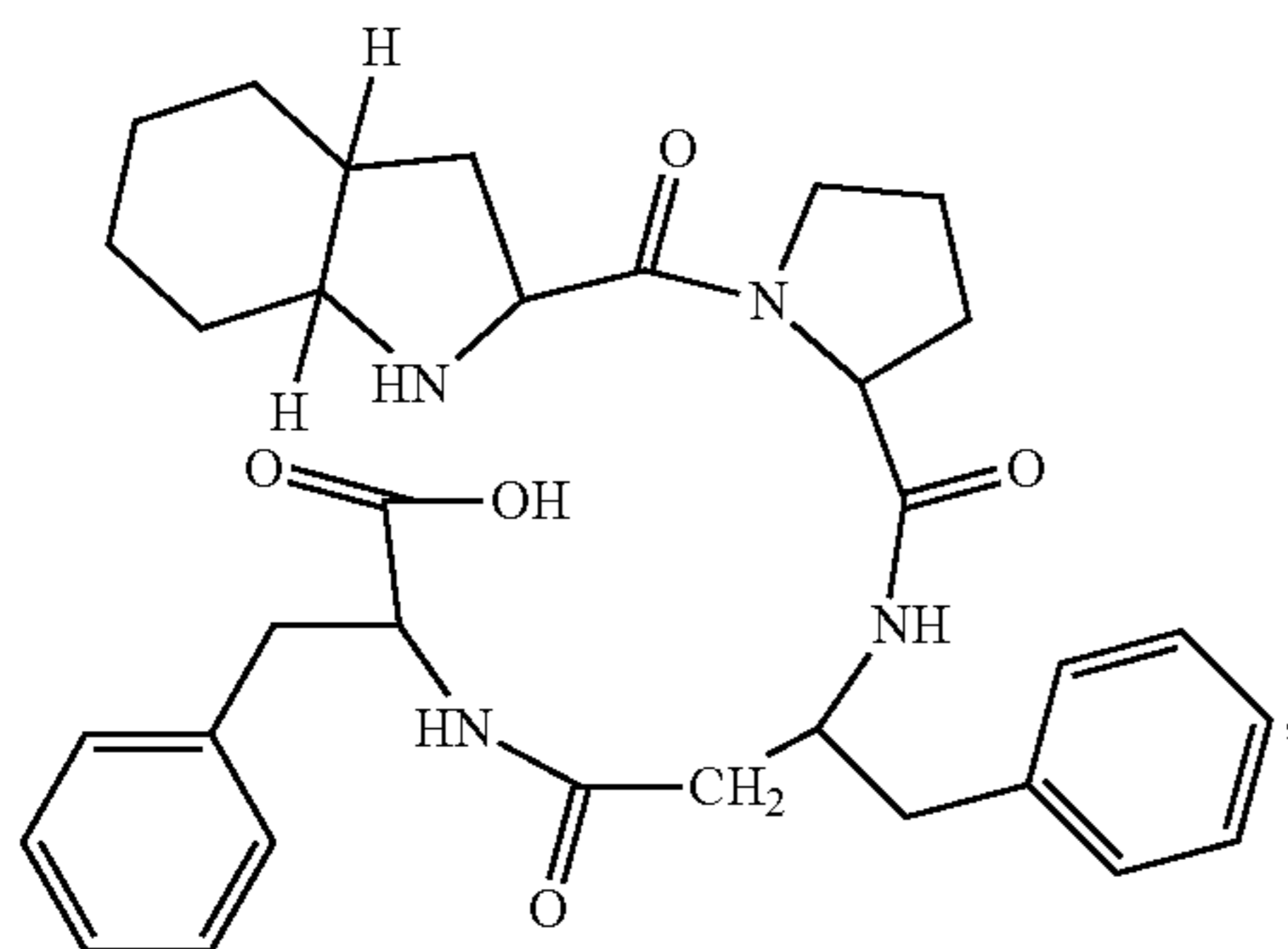
(H-Oic-Pro-β 3 hoPhe-Phe-OH)
