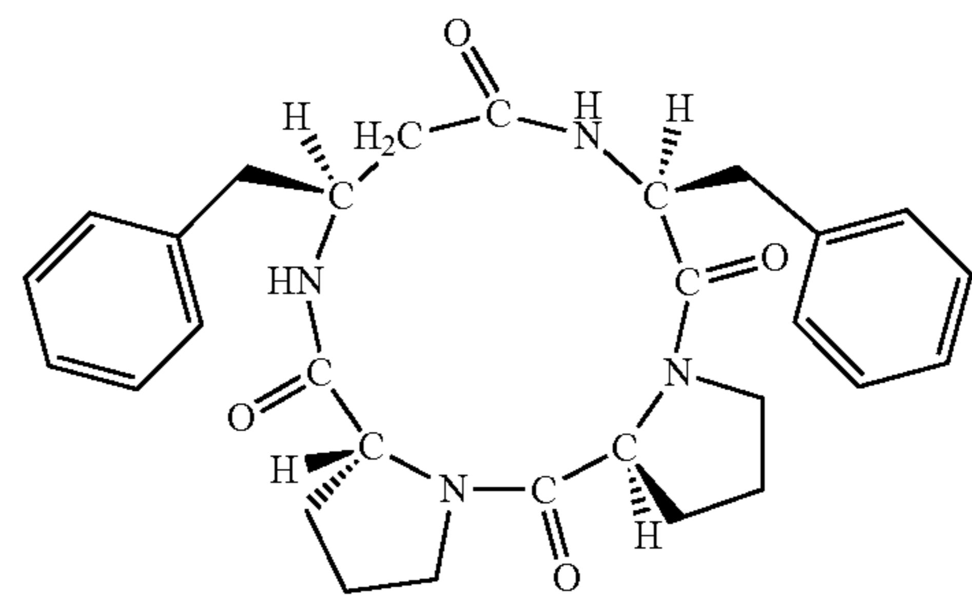
(cyclo(-L-Pro-D-Pro-L-β 3 HoPhe-L-Phe-))
