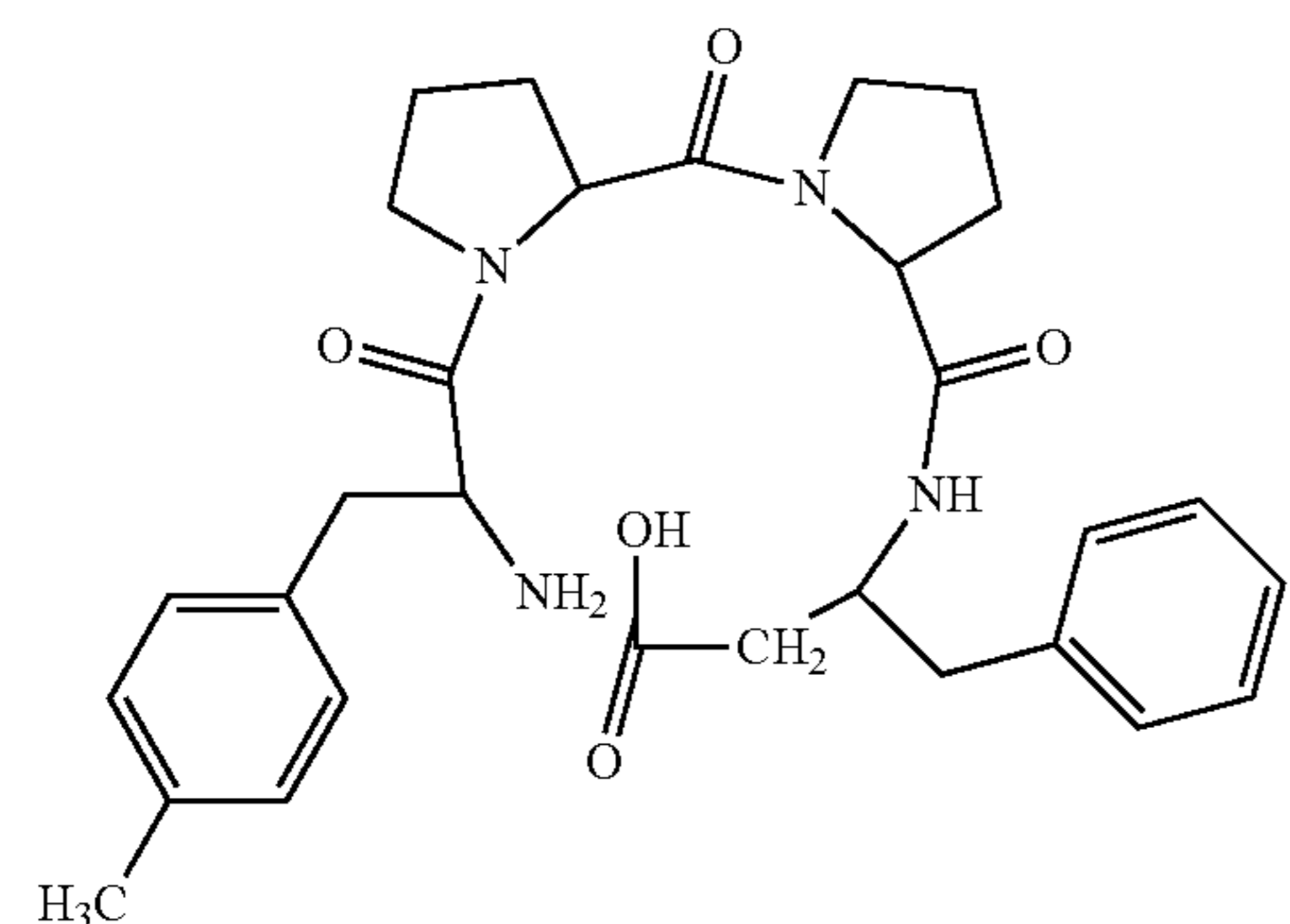
(H-Phe(4Me)-Pro-Pro-β 3 hoPhe-OH)
