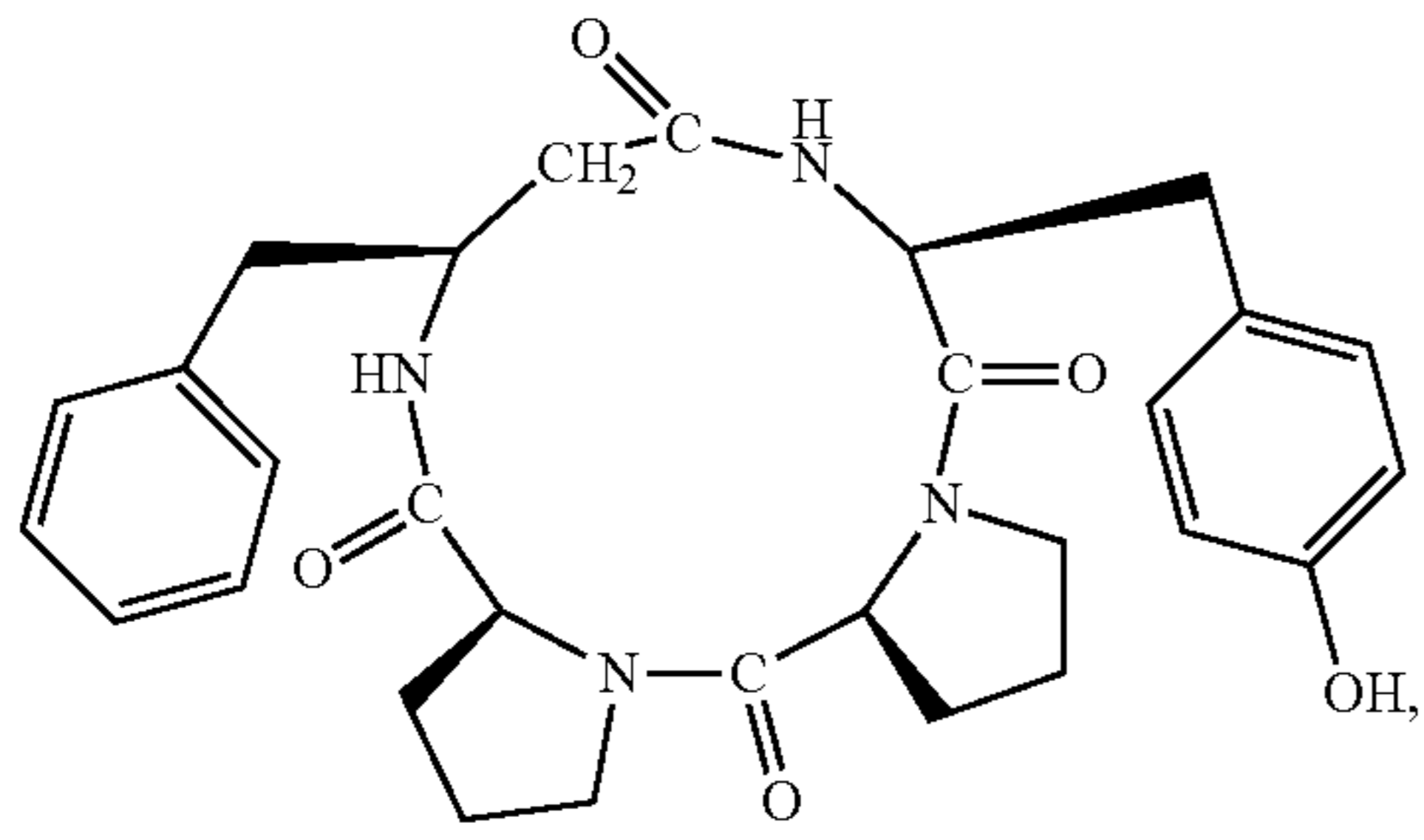
(c(-L-Pro-L-Pro-L-β 3 HoPhe-L-Tyr-))
