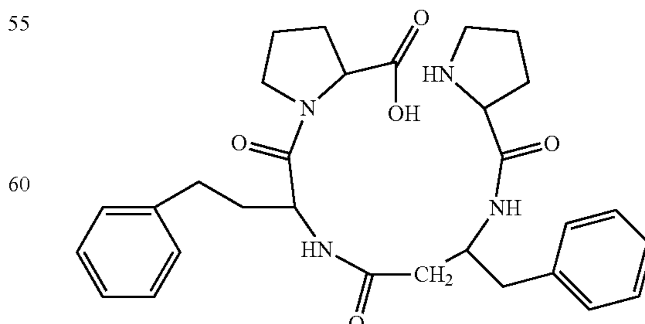
(H-Pro-β³hoPhe-hoPhe-Pro-OH)
