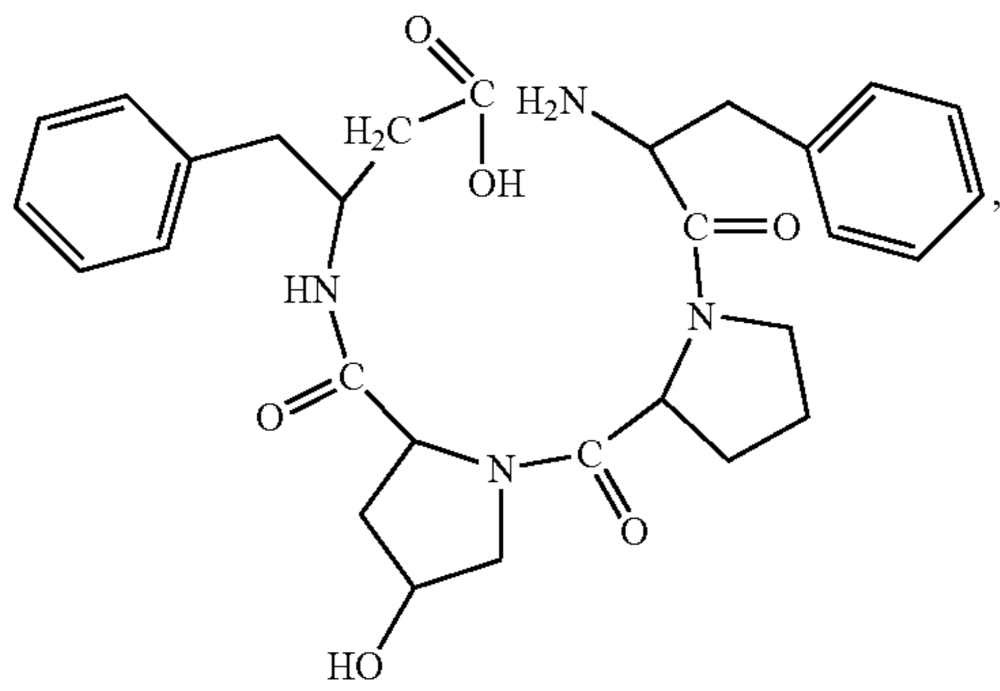
(H-Phe-Pro-Hyp-β 3 hoPhe-OH)
