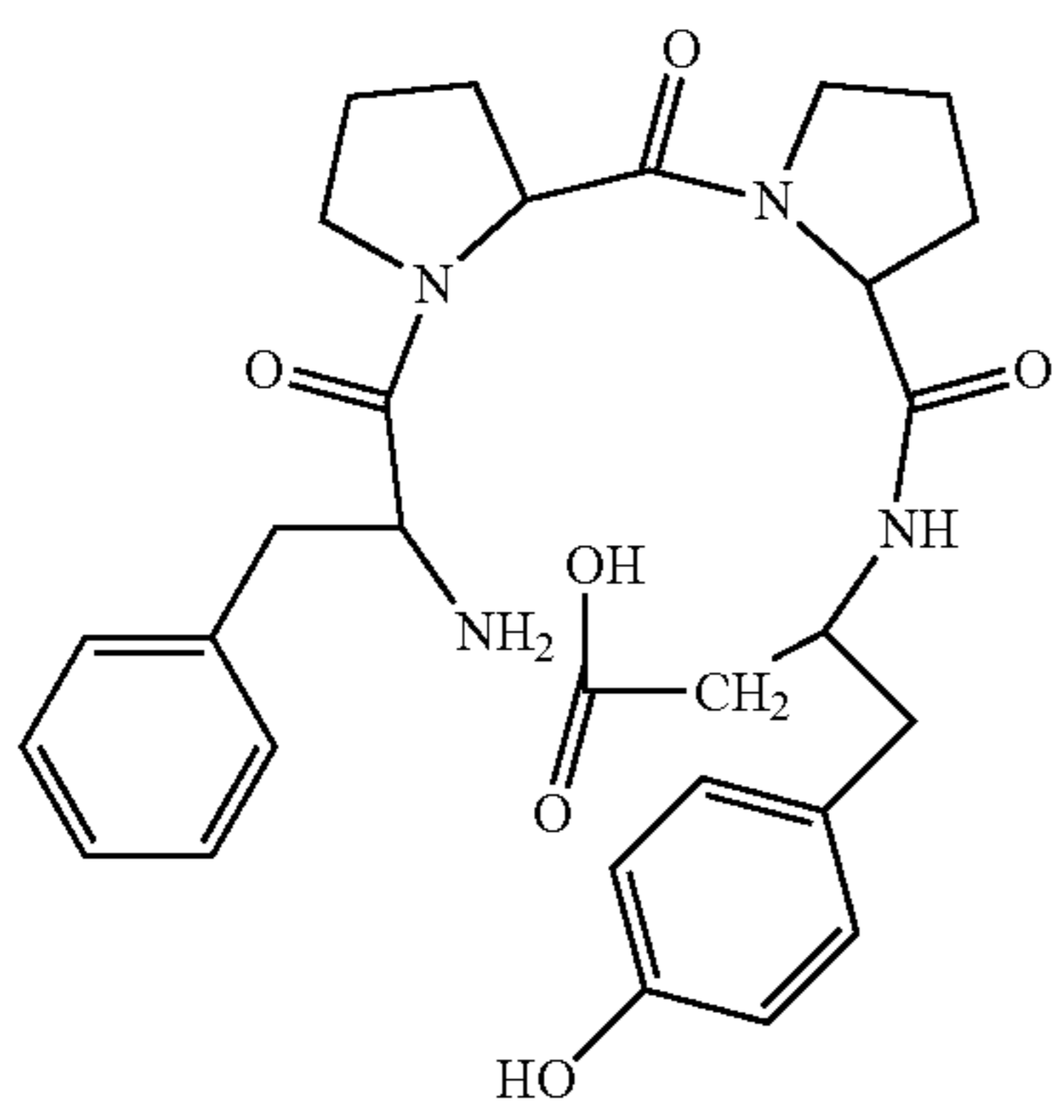
(H-Phe-Pro-Pro-β³hoTyr-OH)
