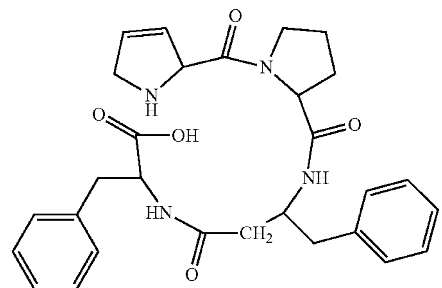
(H-ΔPro-Pro-β³hoPhe-Phe-OH)
