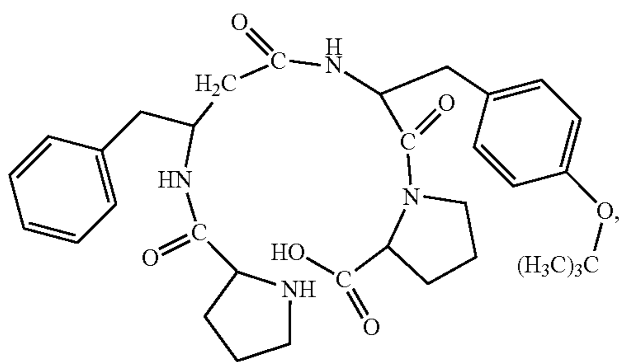
(H-Pro-β 3 hoPhe-Tyr(t-Bu)-Pro-OH)
