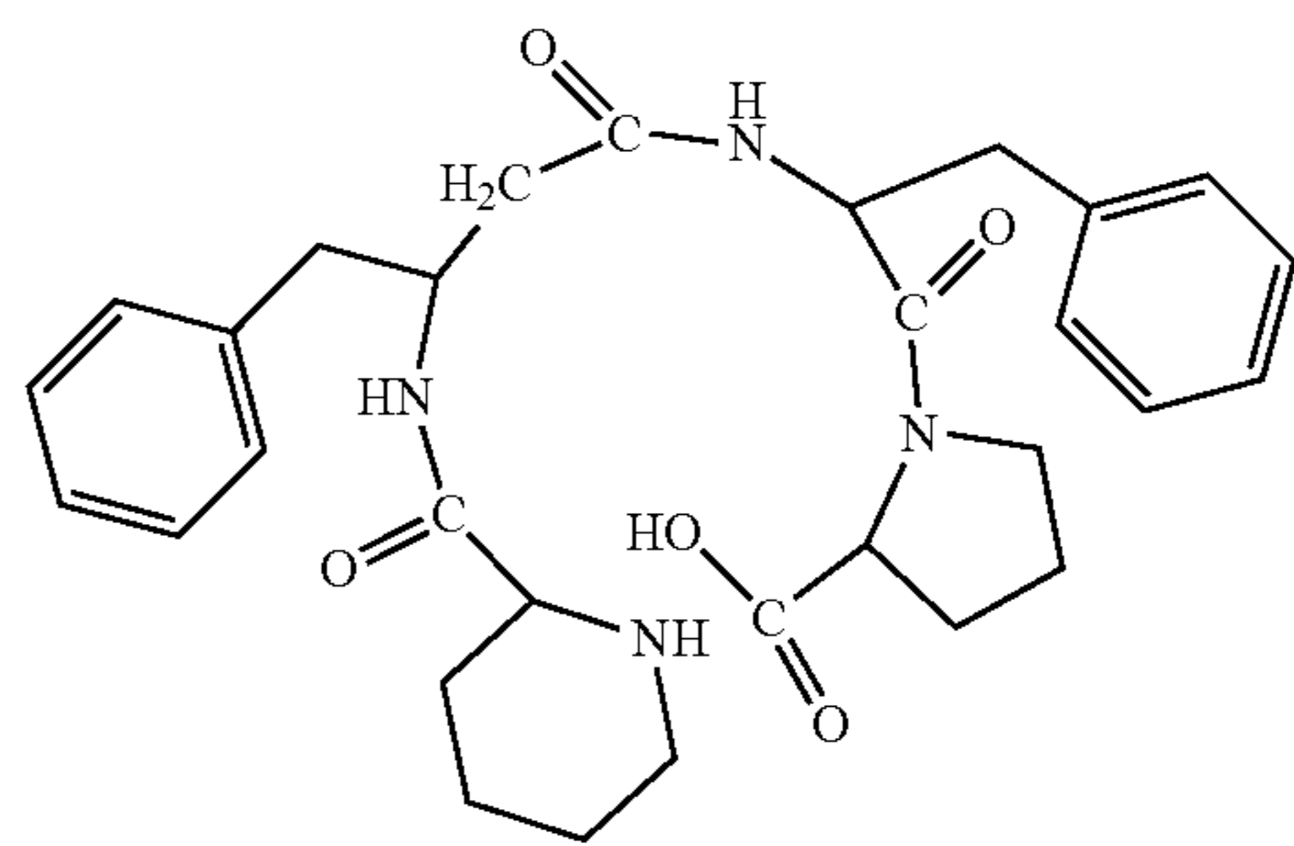
(H-Pip-β 3 hoPhe-Pre-Pro-OH)
