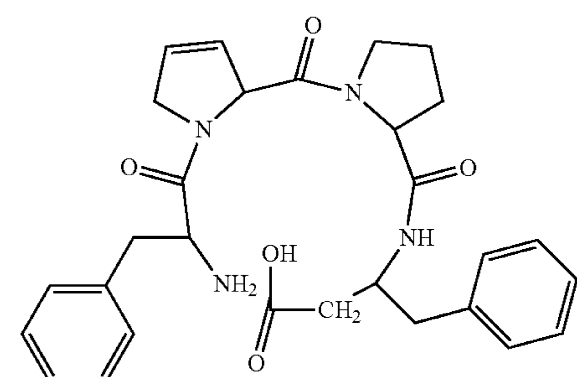
(H-Phe-ΔPro-Pro-β³hoPhe-OH)
