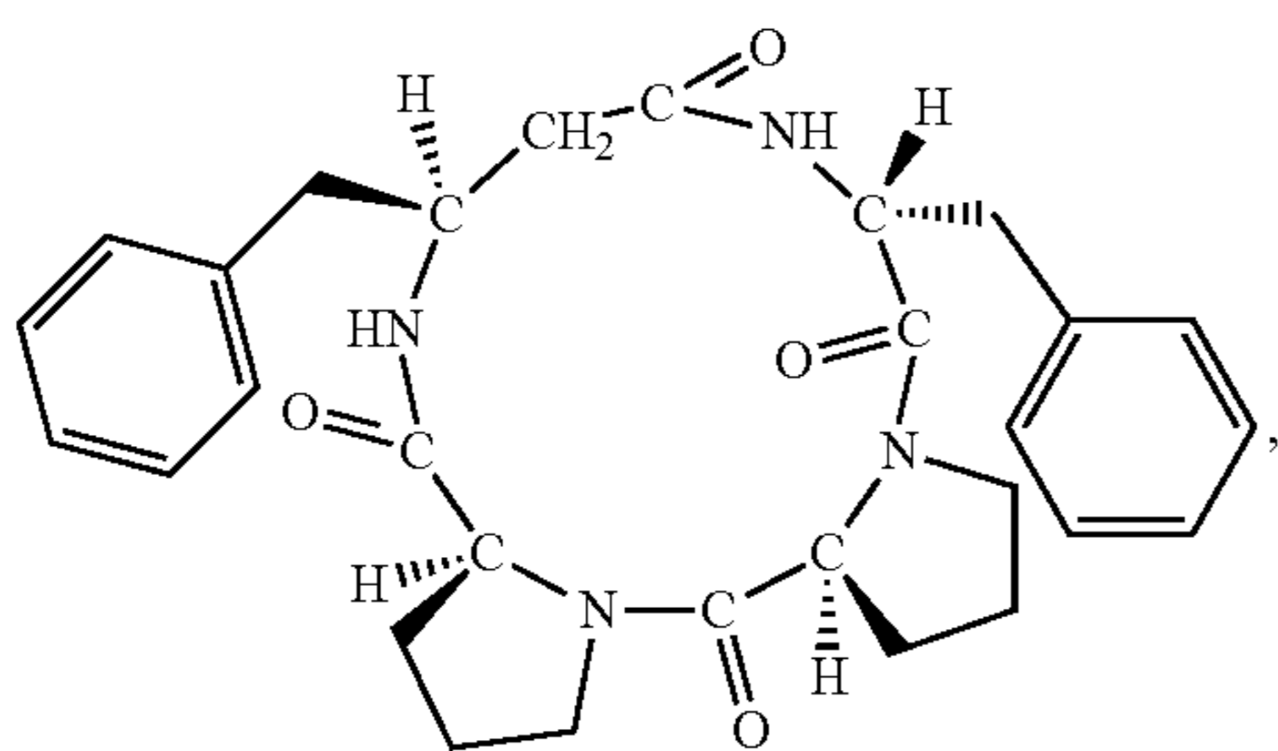
(cyclo(-L-Pro-L-Pro-L-β 3 HoPhe-D-Phe-))
