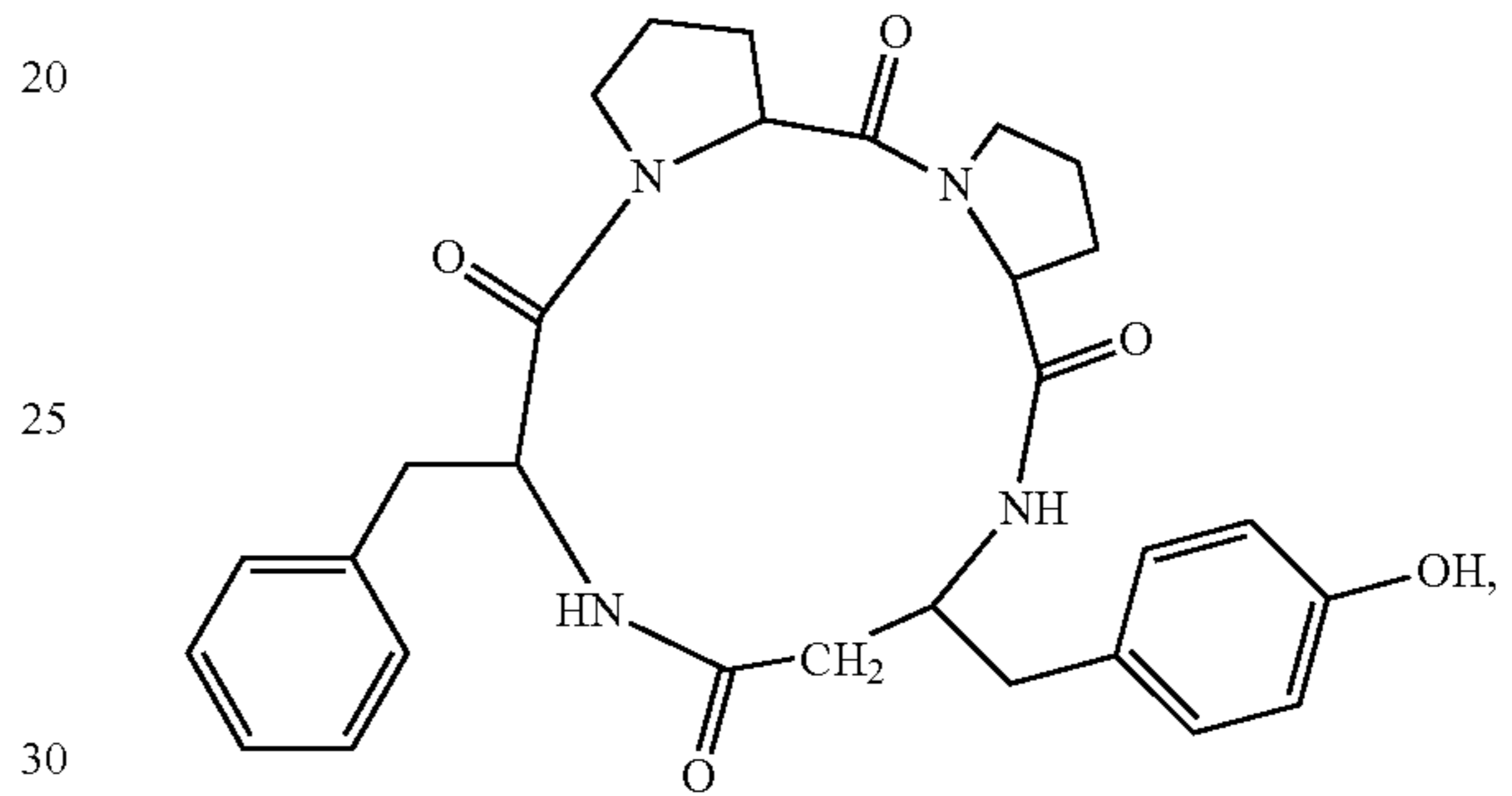
(cyclo(-Pro-Pro-β³hoTyr-Phe-))
