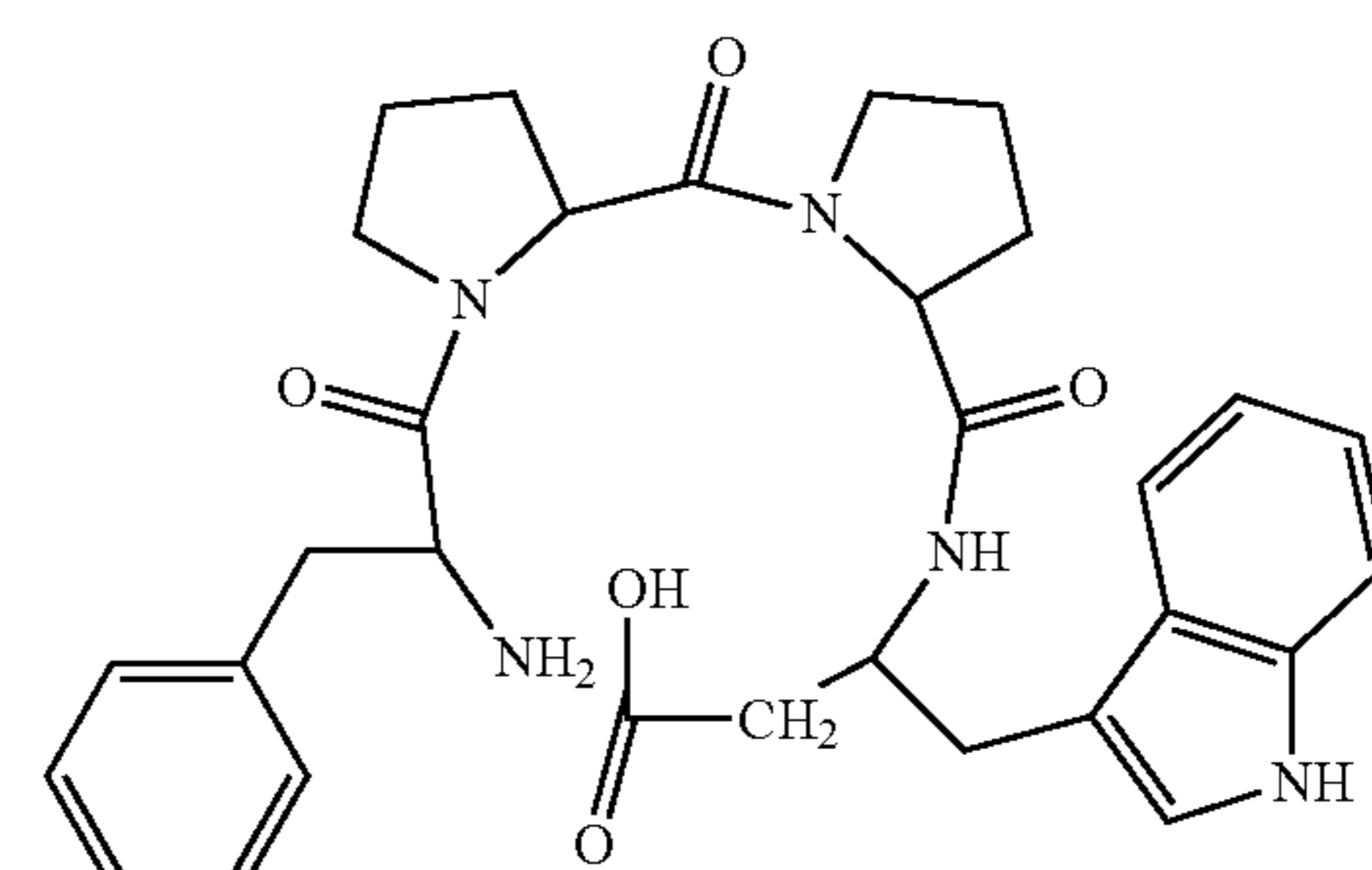
(H-Phe-Pro-Pro-β 3 hoTrp-OH)
