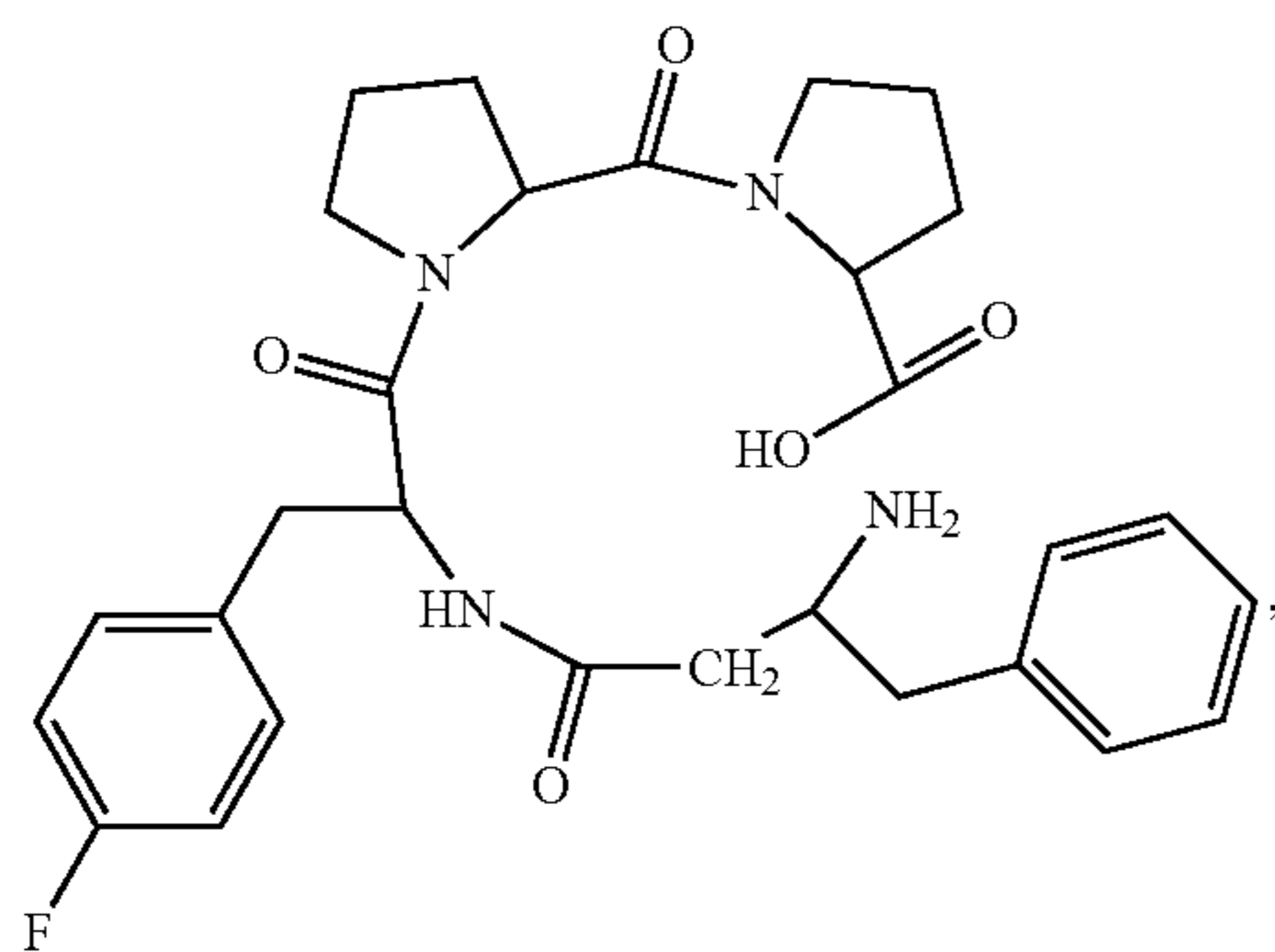
(H-β 3 hoPhe-Phe(4F)-Pro-Pro-OH)
