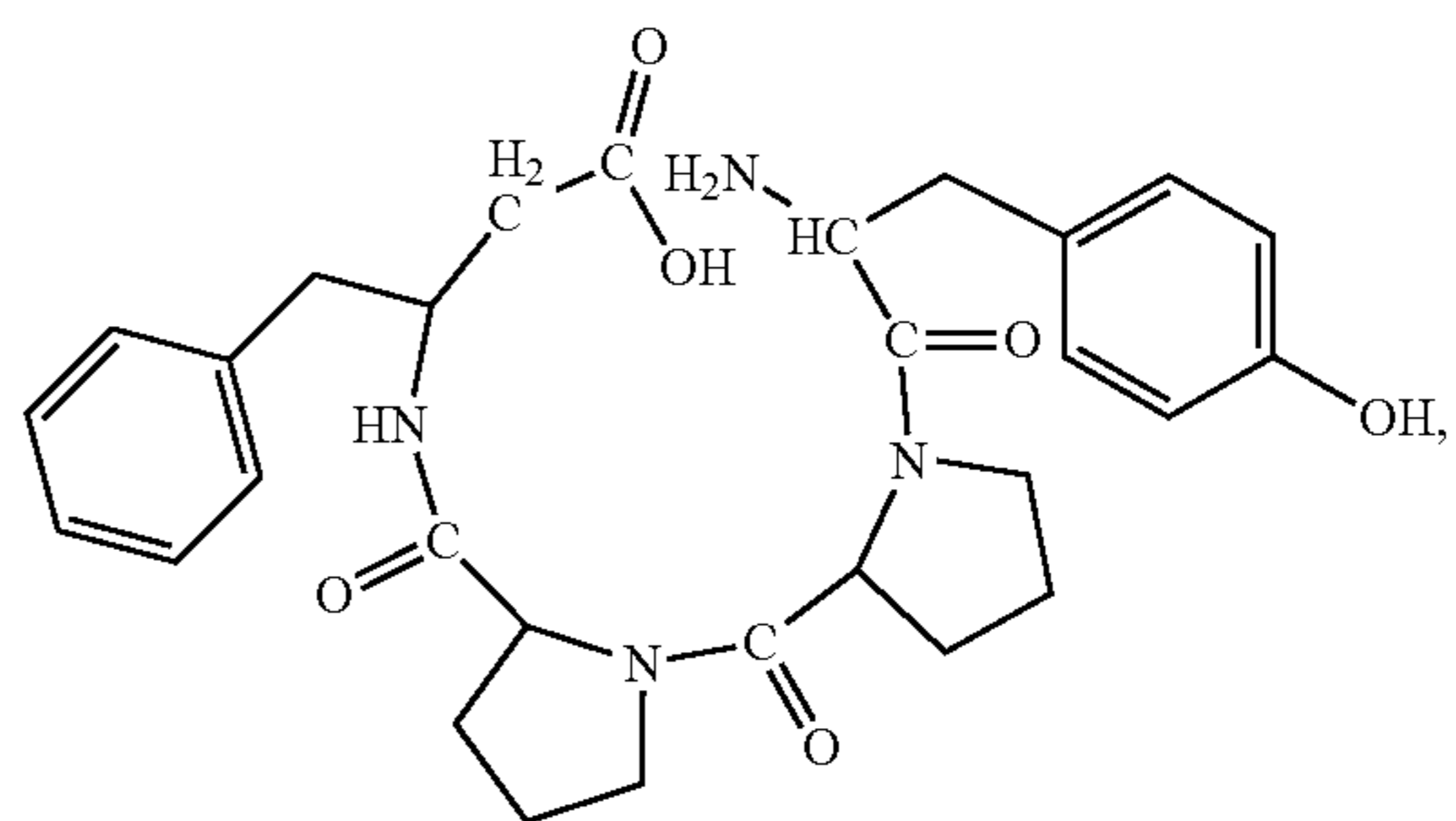
(H-Tyr-Pro-Pro-β 3 hoPhe-OH)
