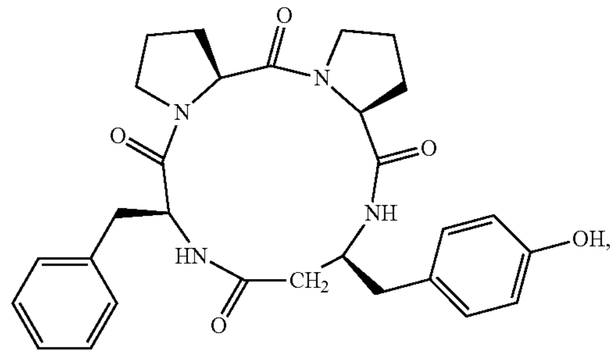
(cyclo(-L-Pro-L-Pro-L-β³hoTyr-L-Phe))
