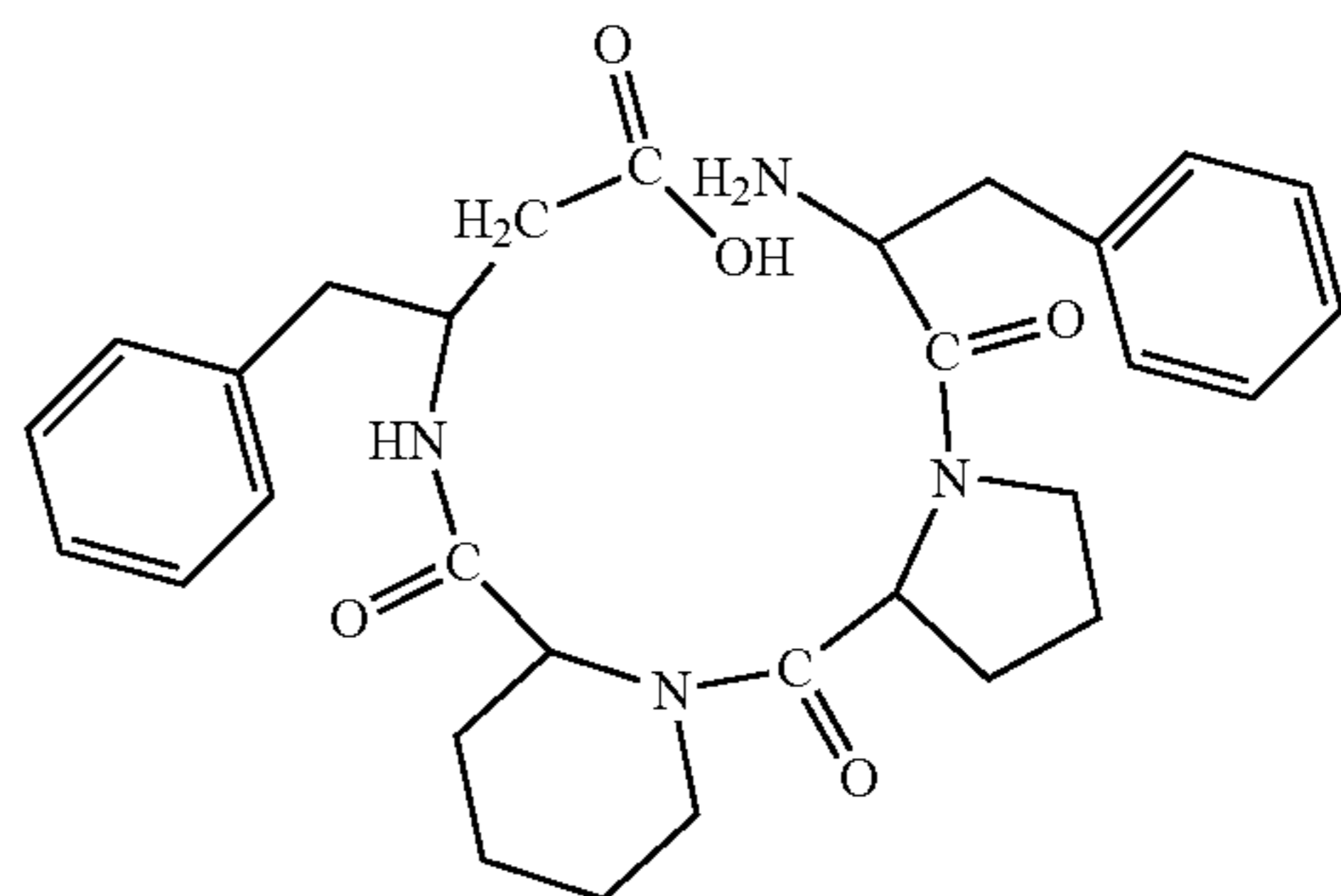
(H-Pre-Pro-Pip-β 3 hoPhe-OH)
