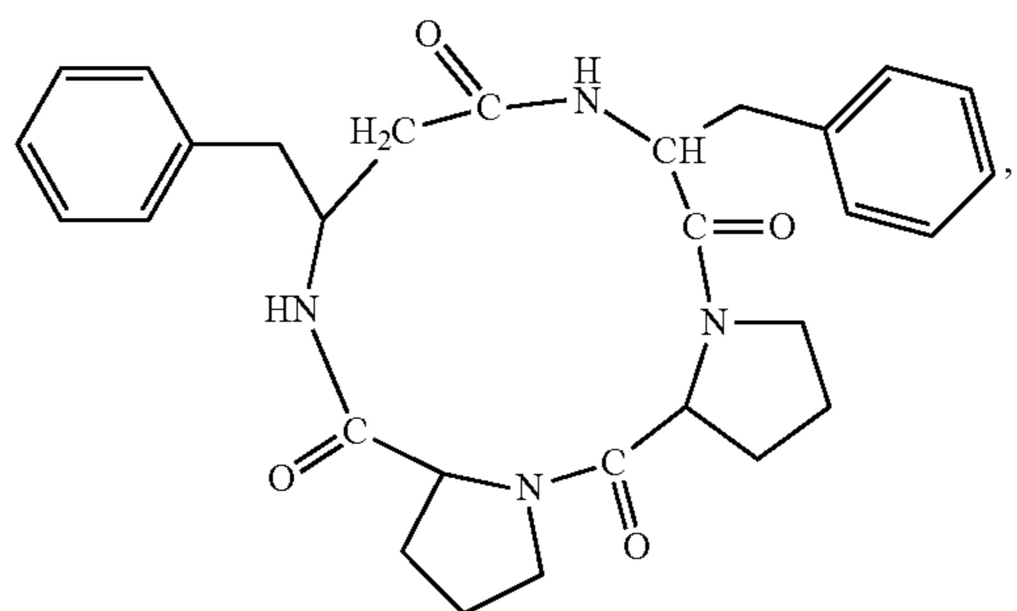
(cyclo(-Pro-Pip-β 3 hoPhe-Phe-))
