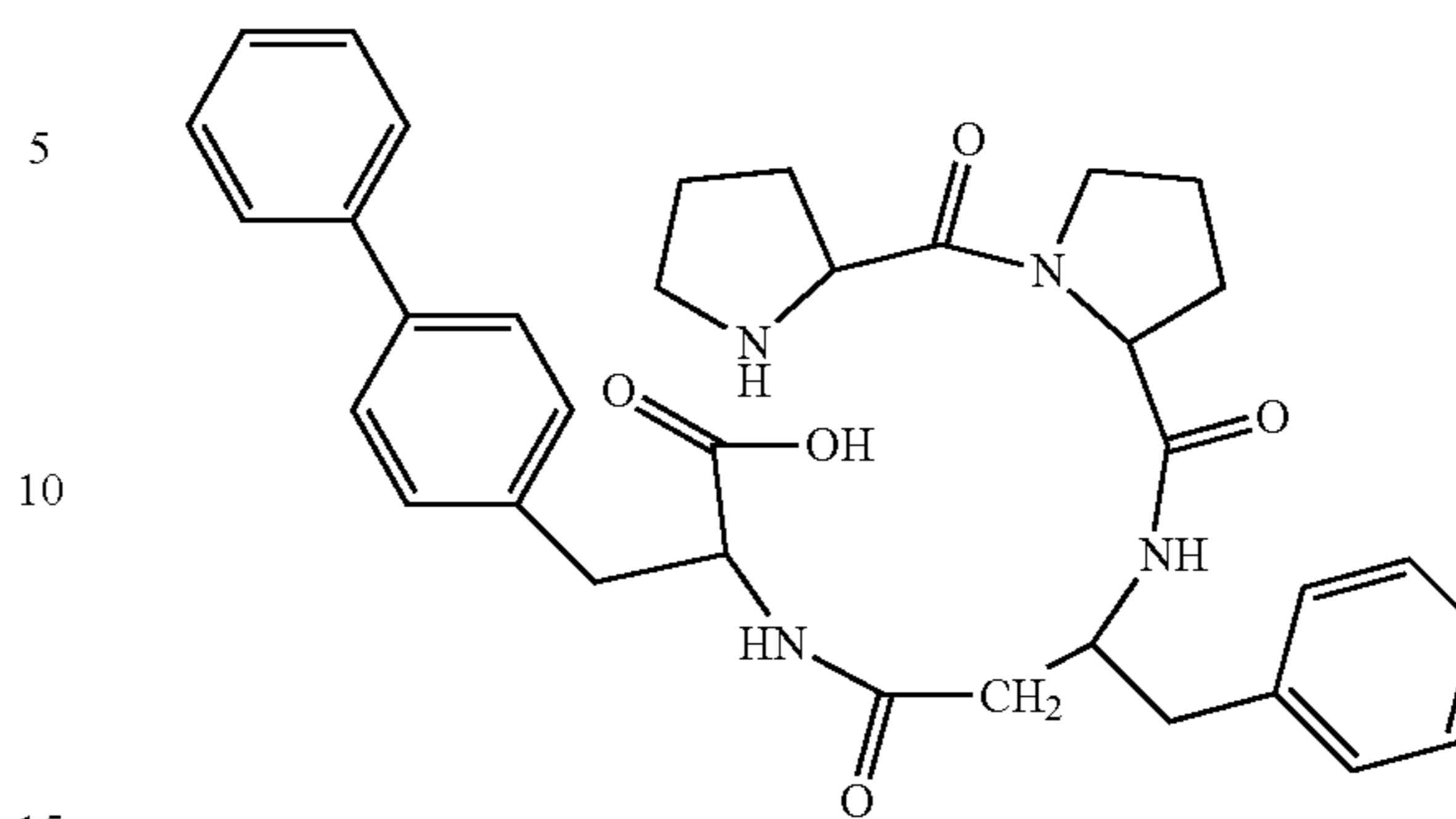
(H-Pro-Pro-β³hoPhe-Bip-OH)
