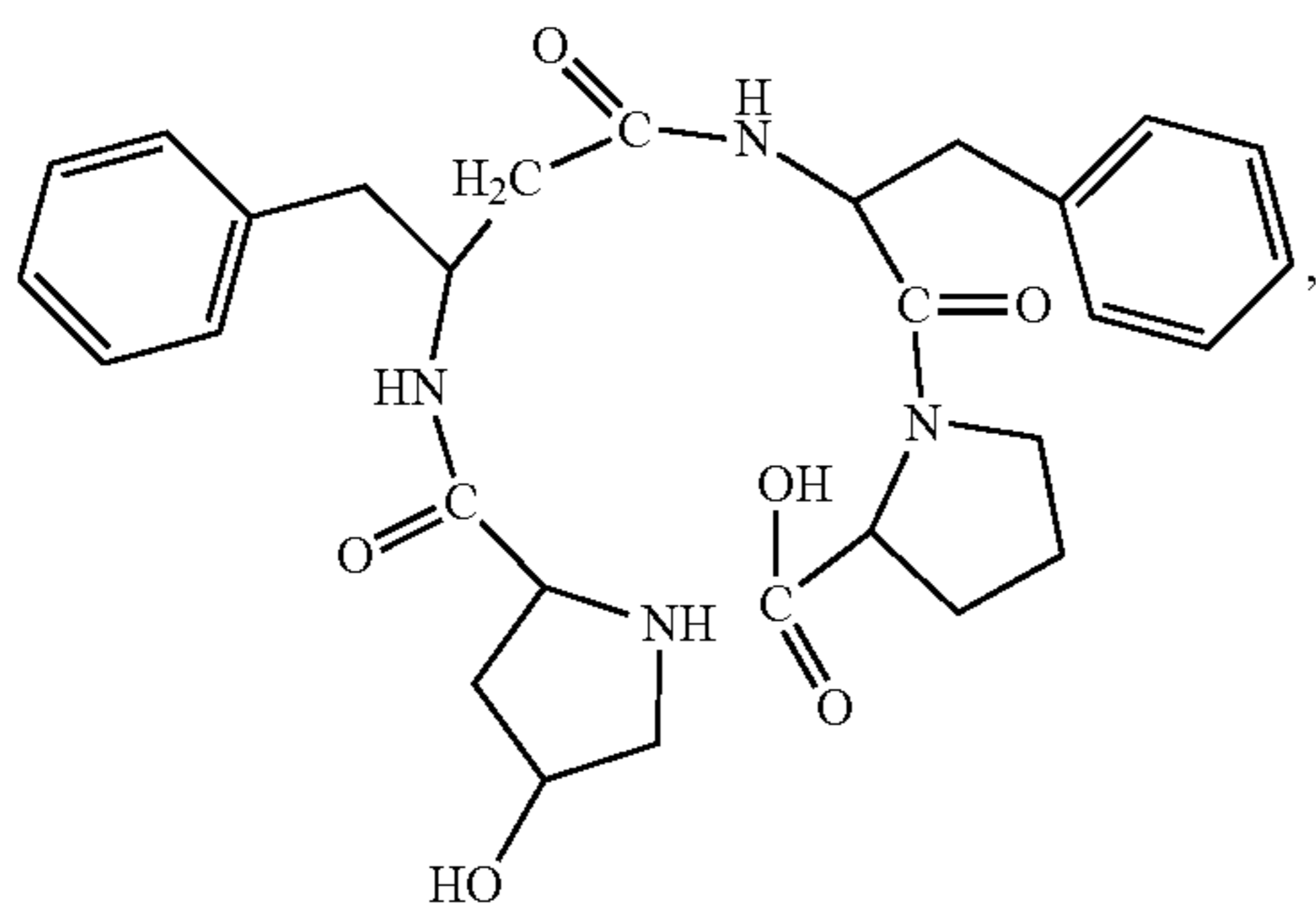
(H-Hyp-β 3 hoPhe-Pre-Pro-OH)
