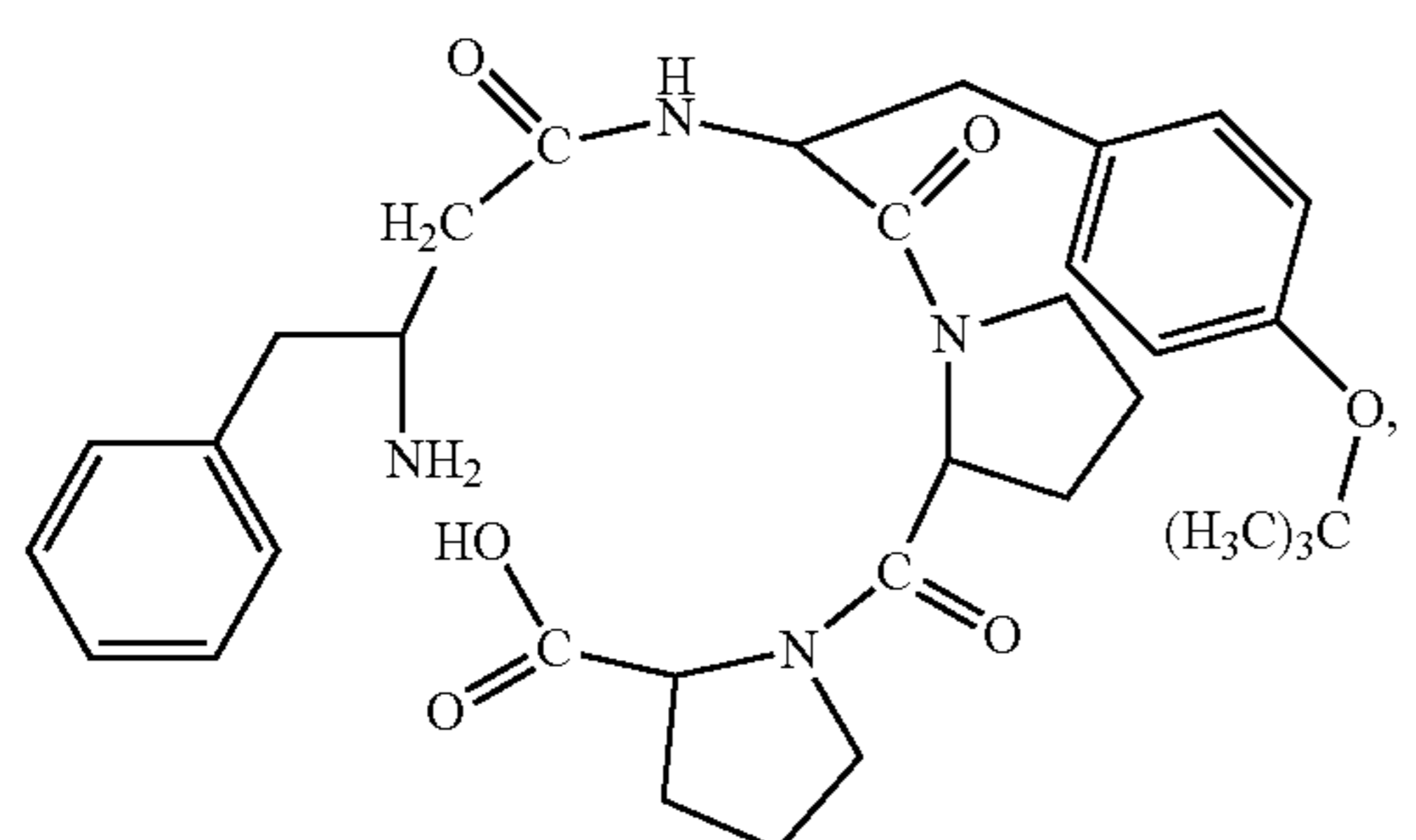
(H-β 3 hoPhe-Tyr(t-Bu)-Pro-Pro-OH)
