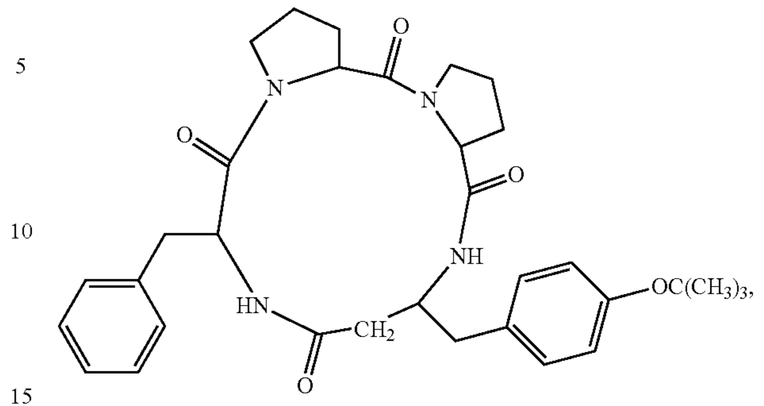
(cyclo(-Pro-Pro-β³hoTyr(tBu)-Phe-))
