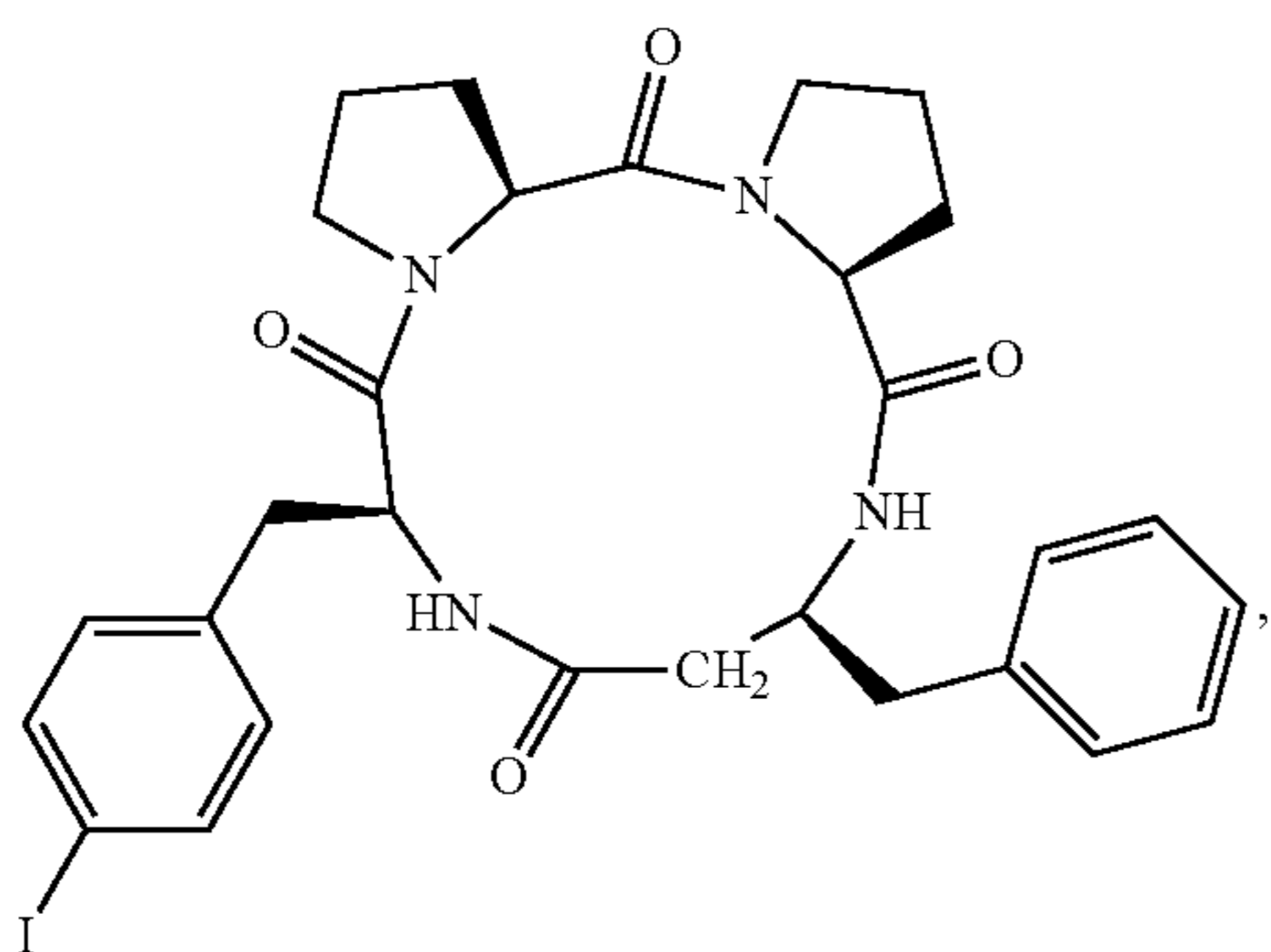
(cyclo(-L-Pro-L-Pro-L-β³hoPhe-L-Phe(4I)))
