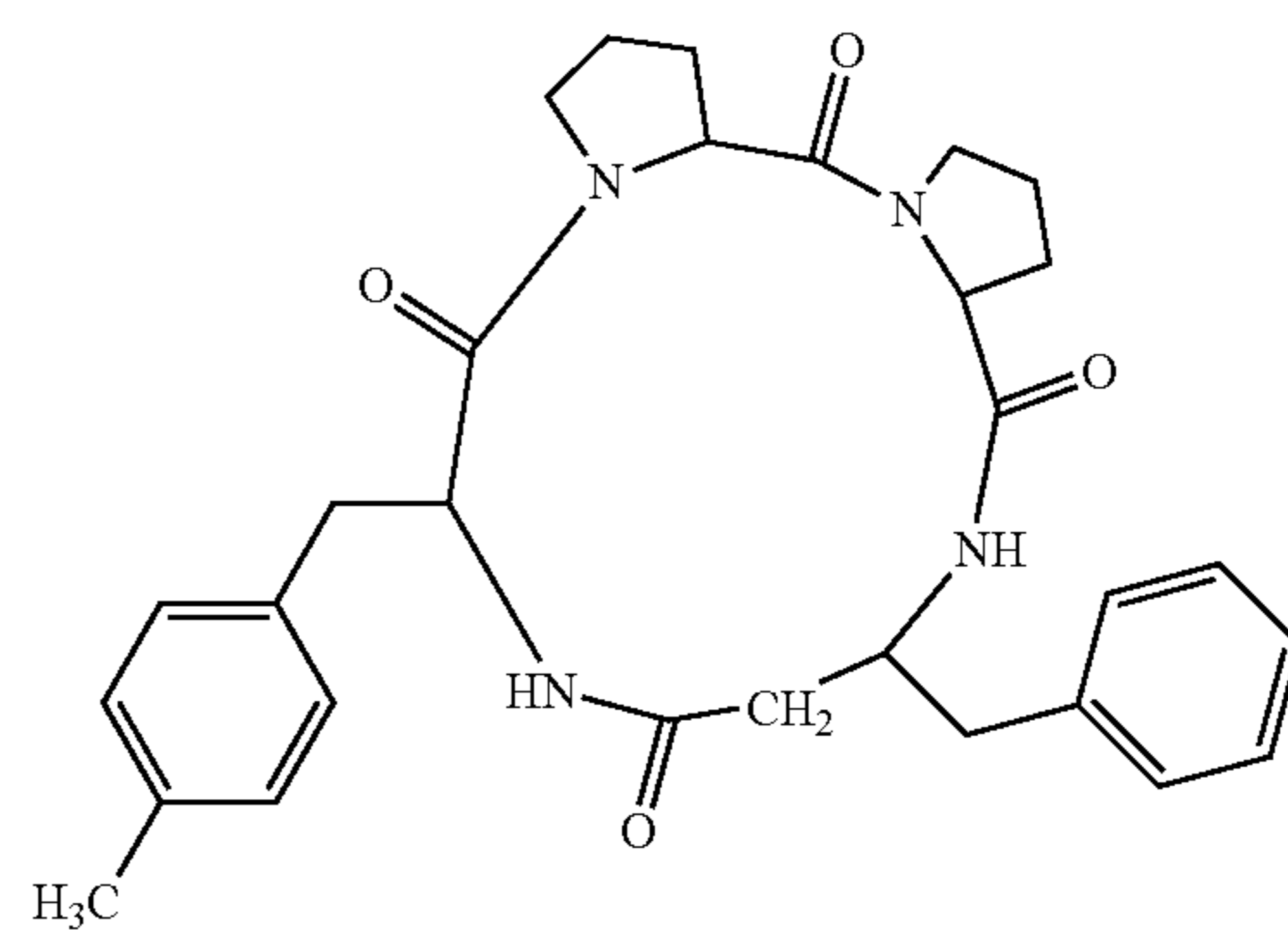
(cyclo(-Pro-Pro-β³hoPhe-Phe(4Me)))
