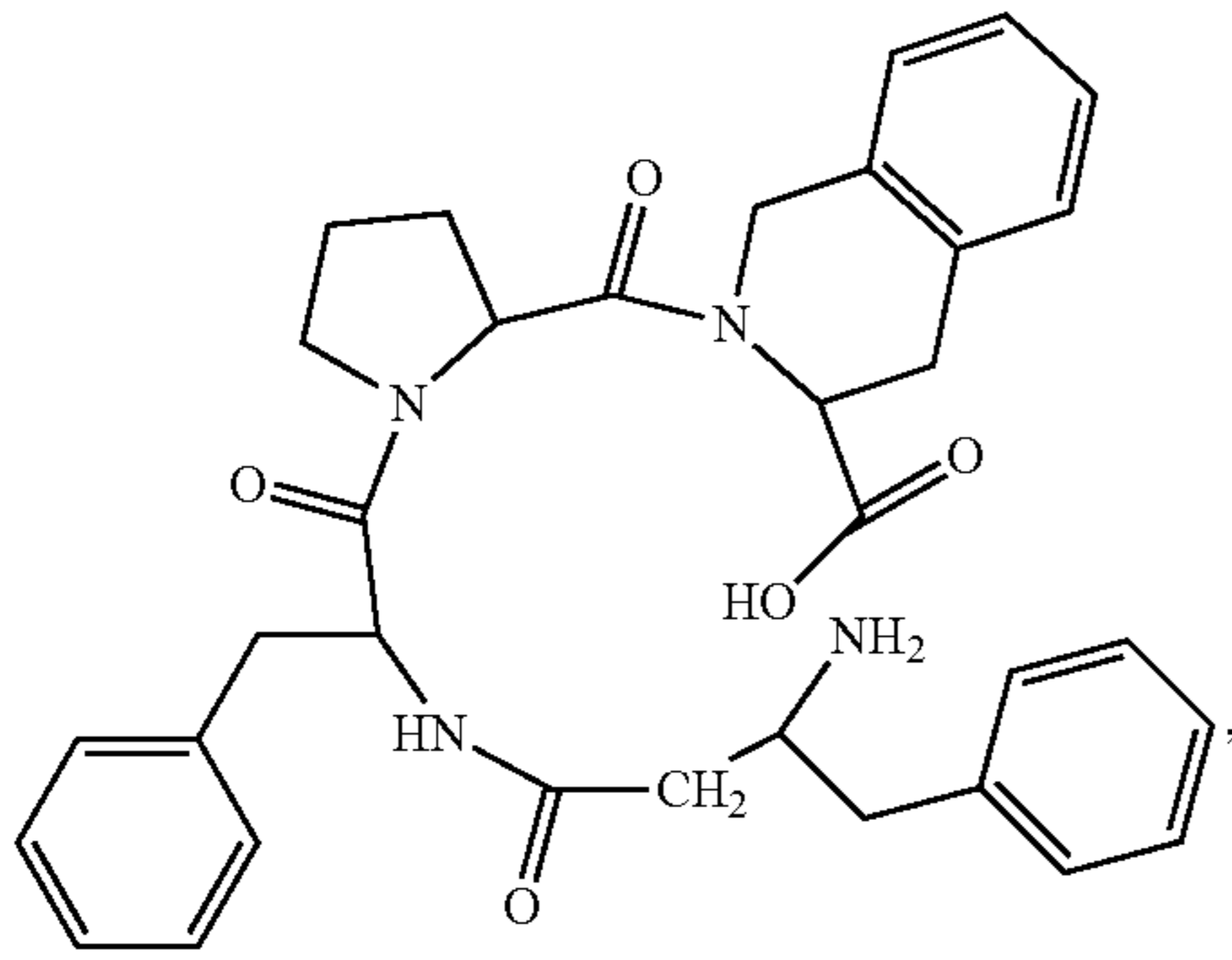
(H-β 3 hoPhe-Phe-Pro-Tic-OH)
