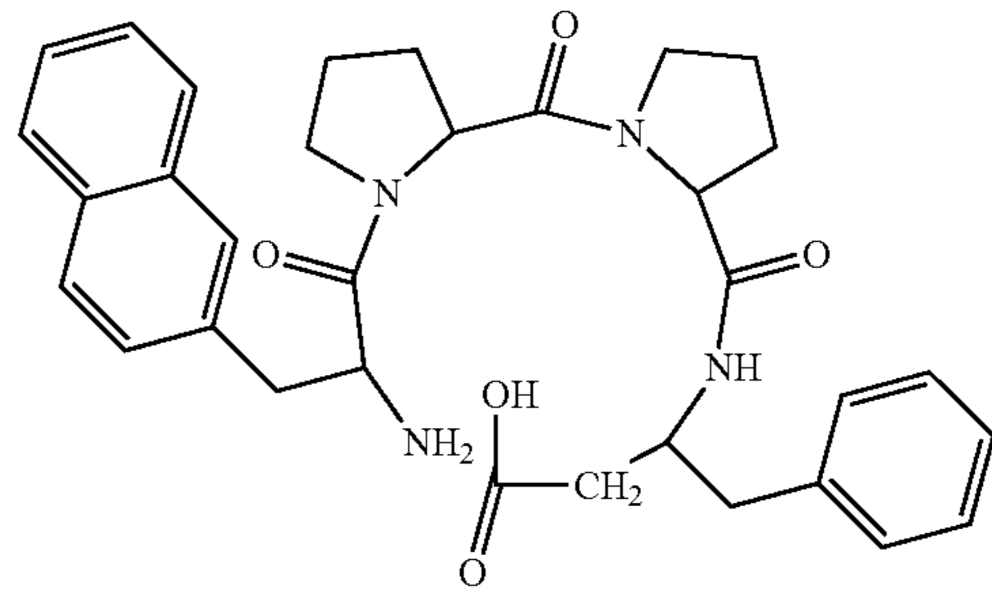
(H-2Nal-Pro-Pro-β 3 hoPhe-OH)
