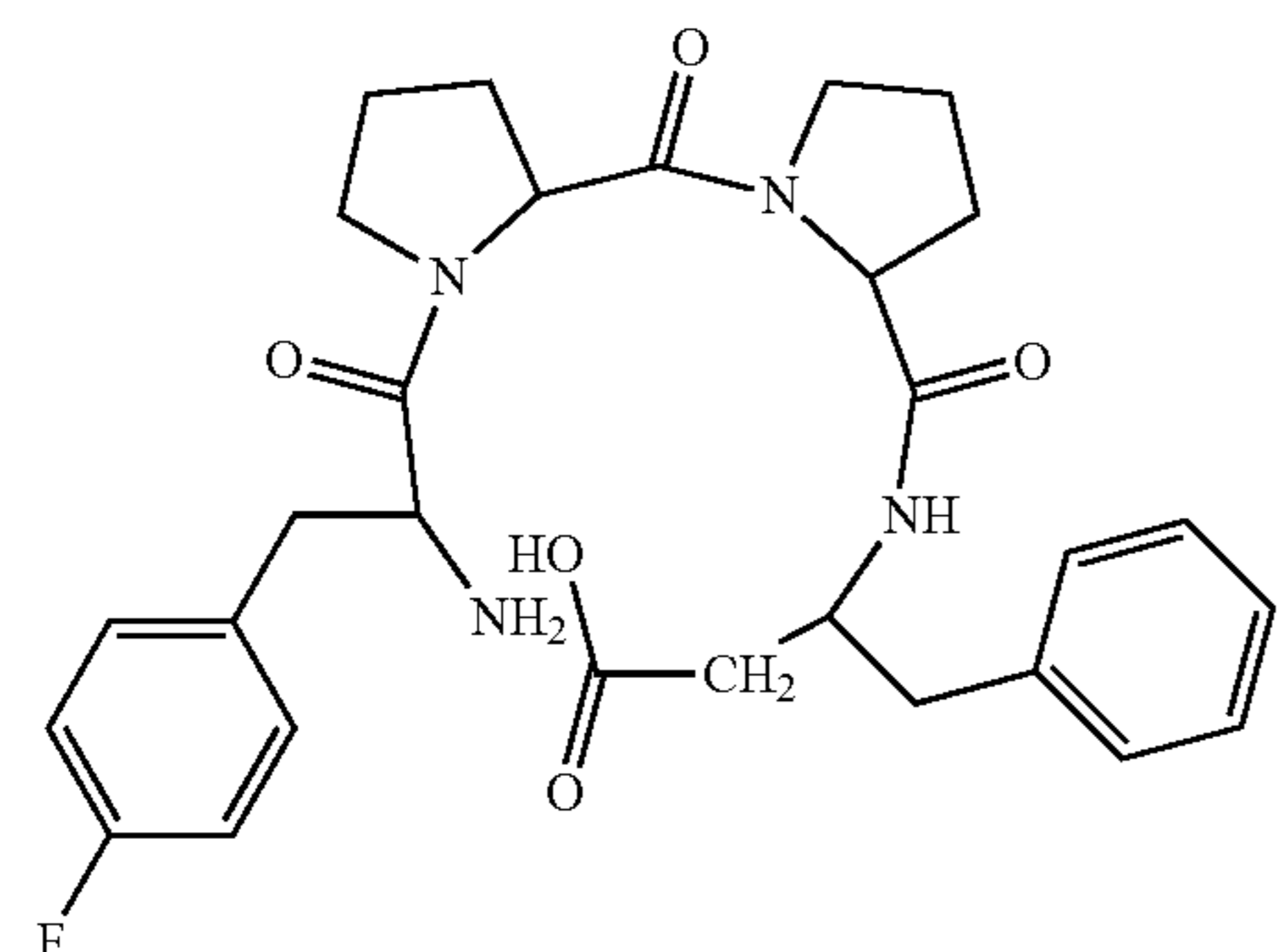
(H-Phe(4F)-Pro-Pro-β 3 hoPhe-OH)
