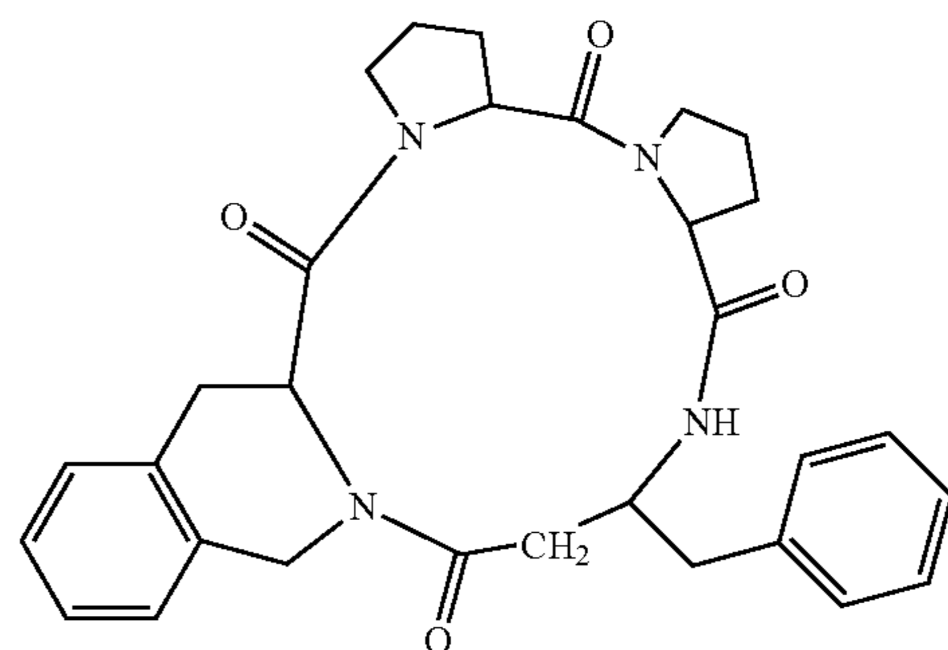
(cyclo(-Pro-Pro-β 3 hoPhe-Tic))
