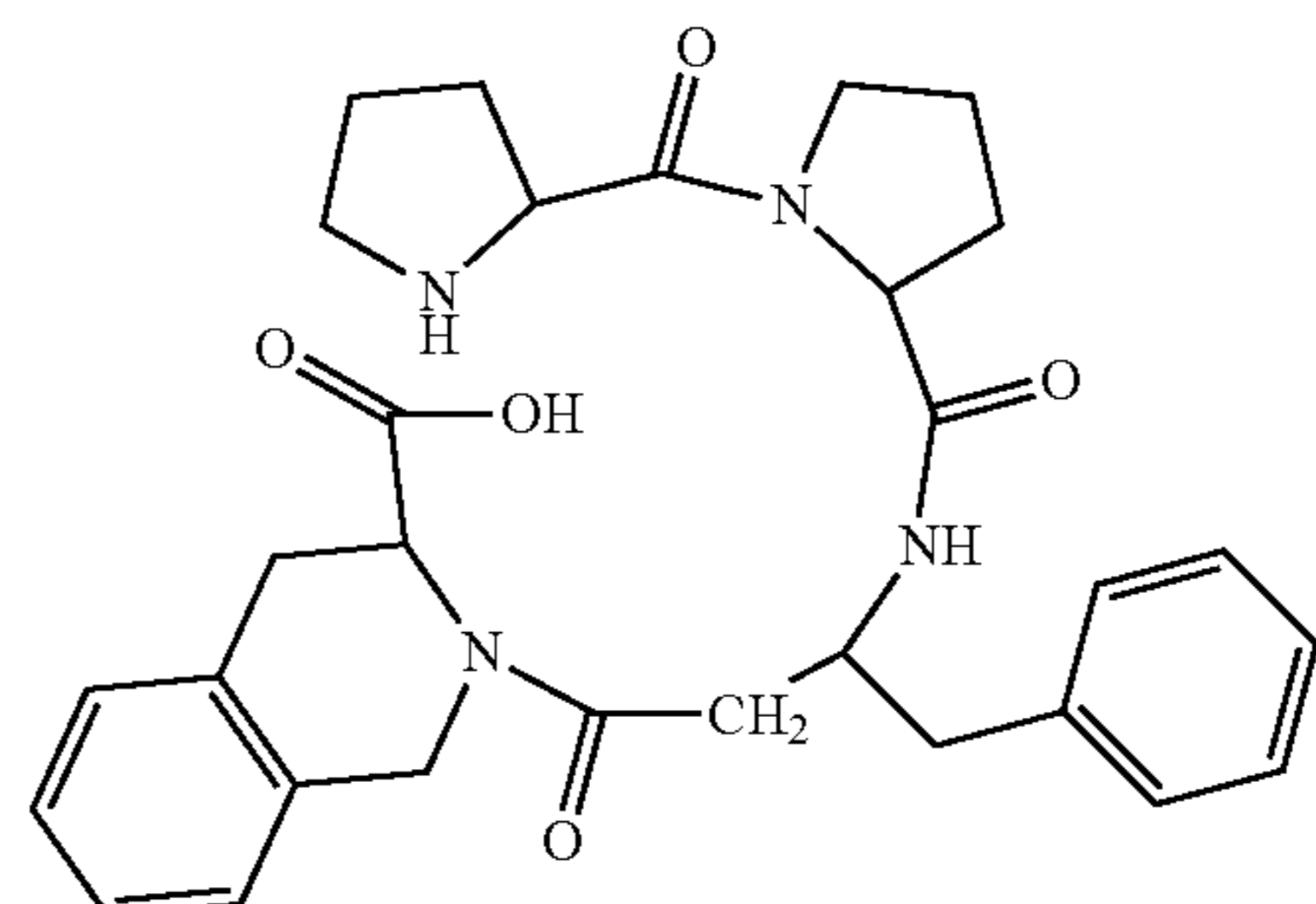
(H-Pro-Pro-β 3 hoPhe-Tic-OH)
