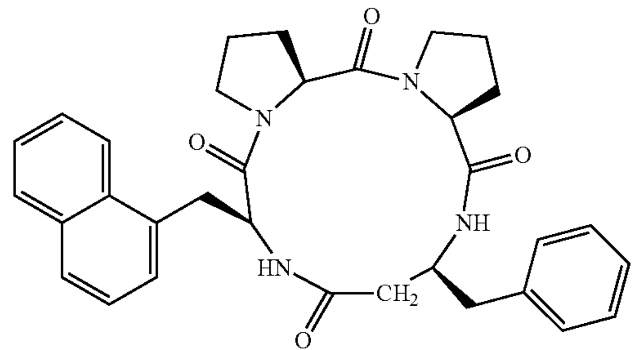
(cyclo(-L-Pro-L-Pro-L-β 3 hoPhe-L-1Nal))
