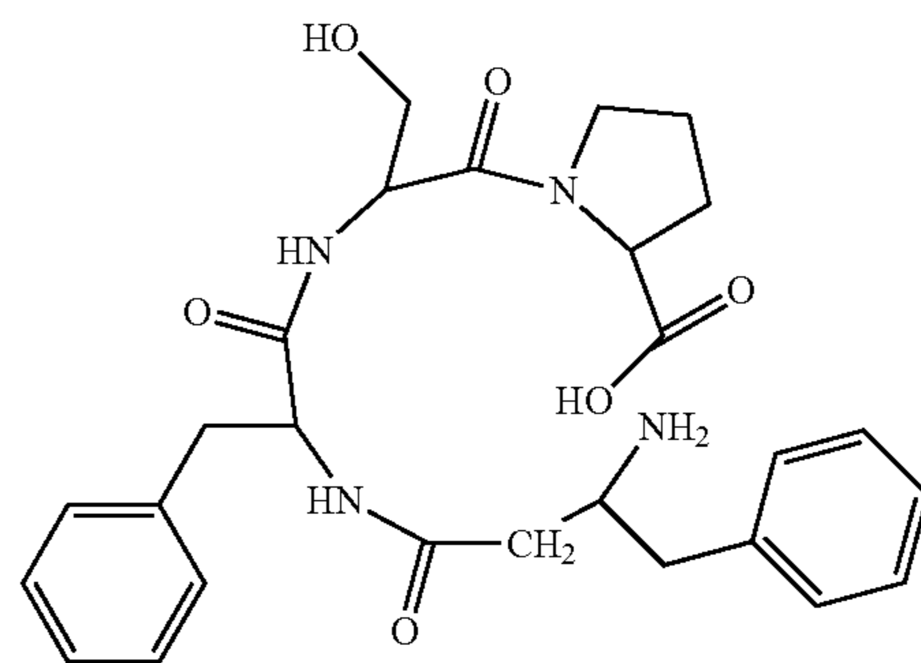
(H-β³hoPhe-Phe-Ser-Pro-OH)
