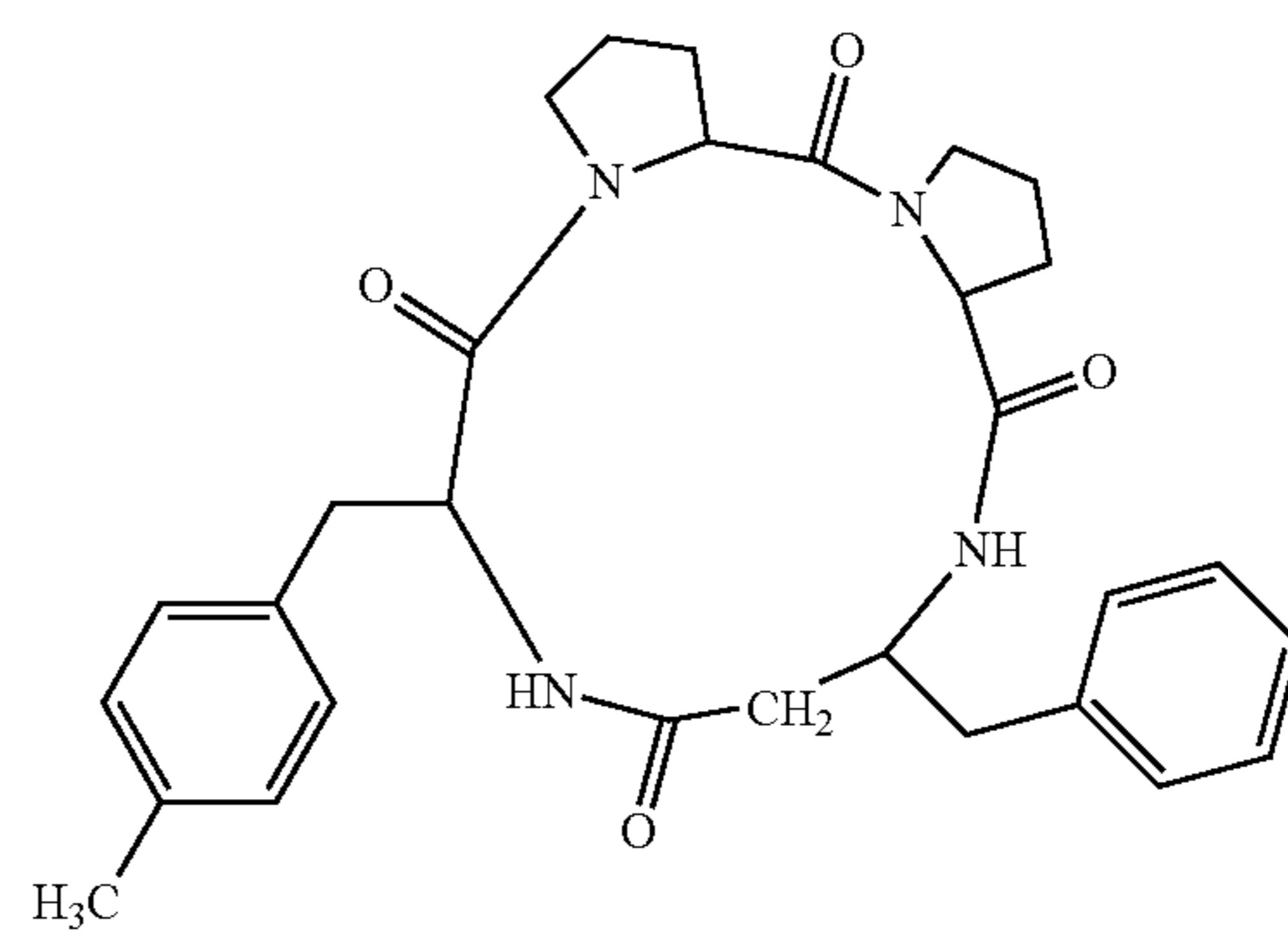
(cyclo(-Pro-Pro-β 3 hoPhe-Phe(4Me)))
