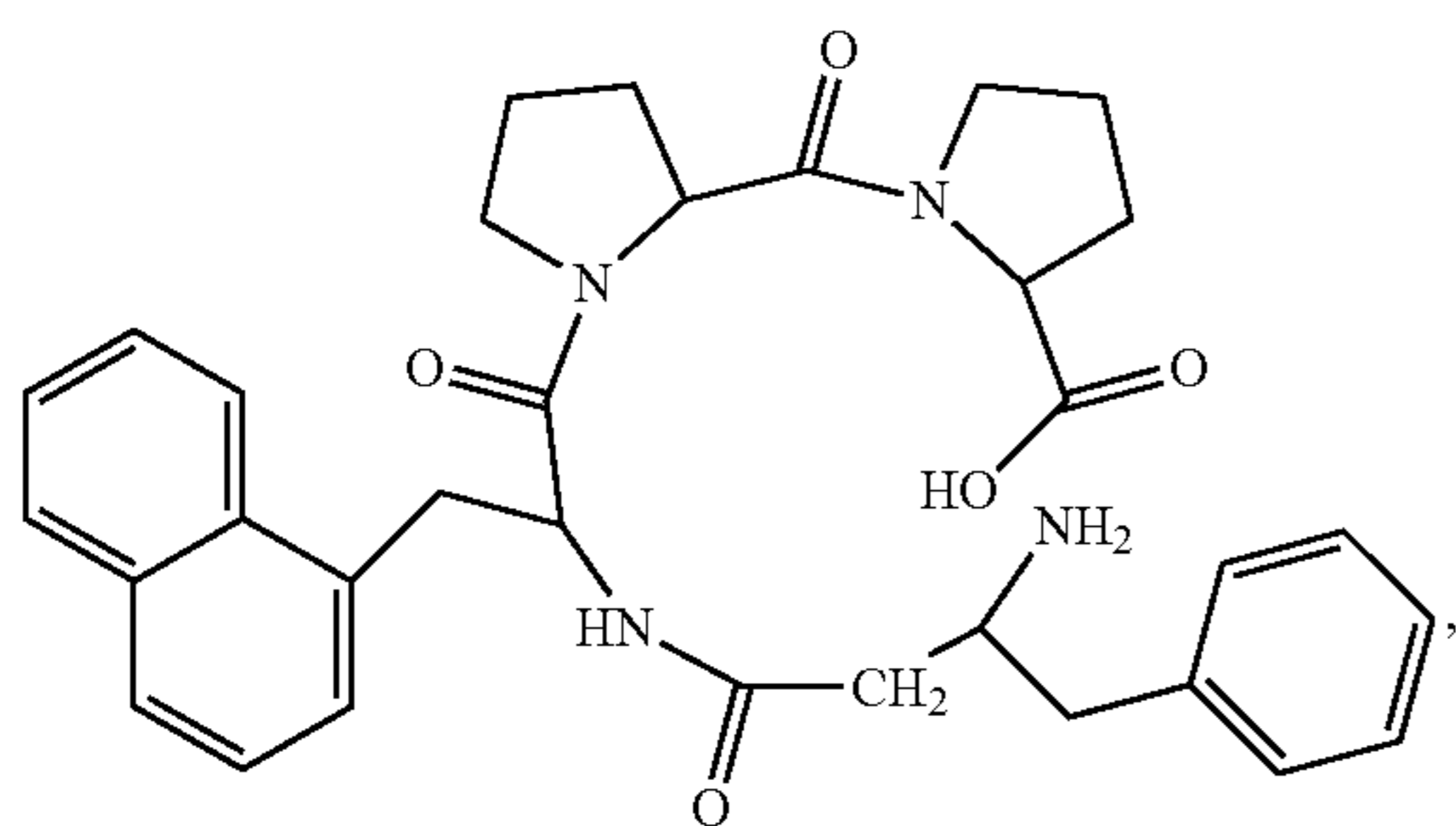
(H-β 3 hoPhe-1Nal-Pro-Pro-OH)
