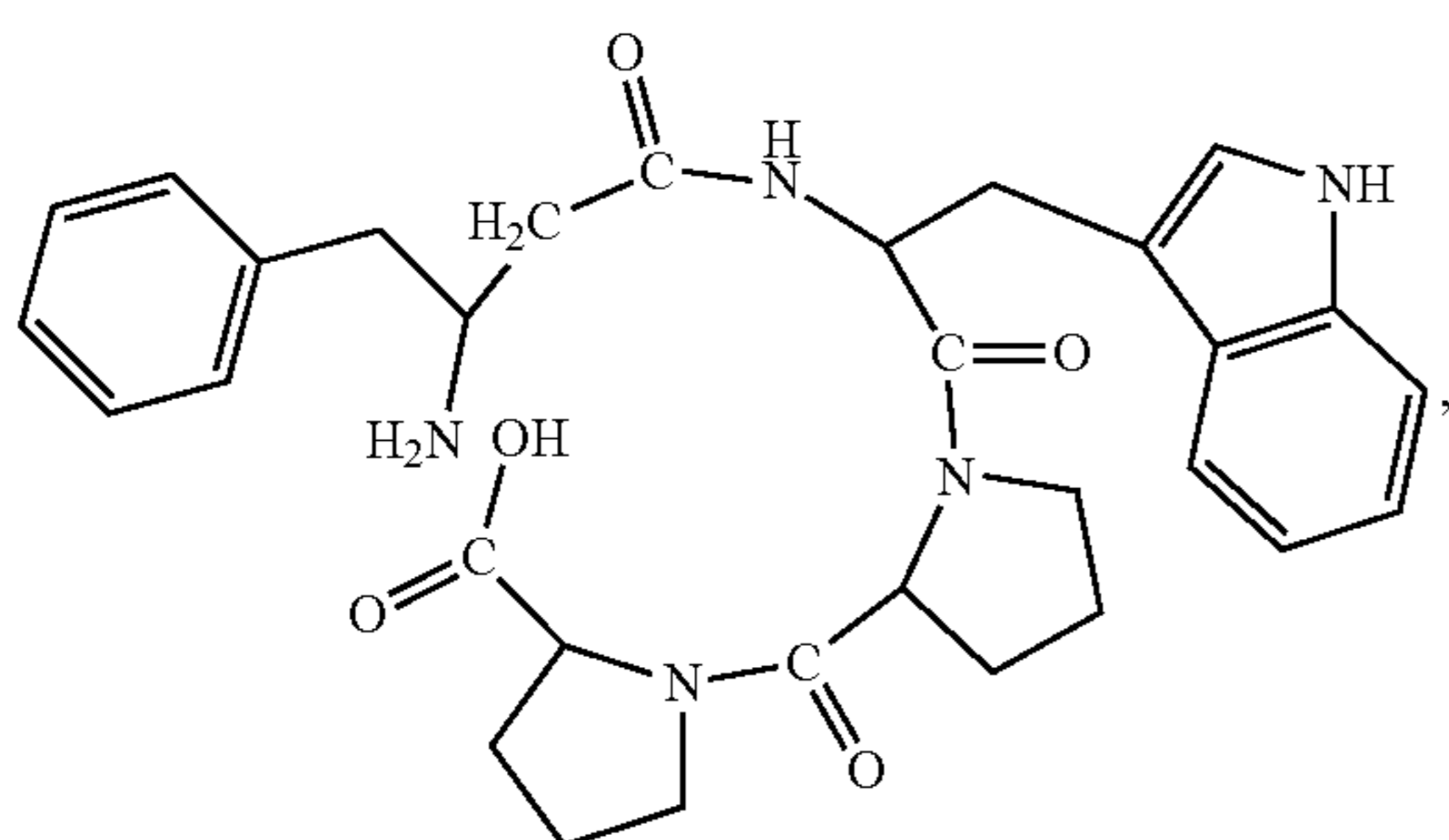
(H-β 3 hoPhe-Trp-Pro-Pro-OH)
