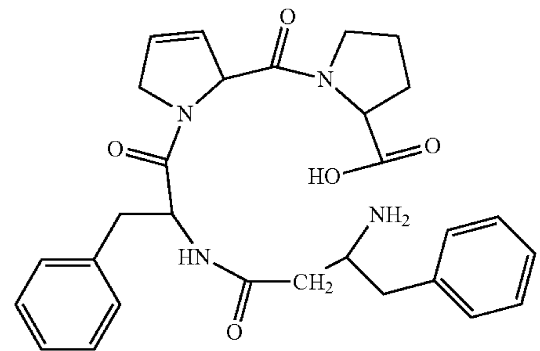
(H-β³hoPhe-Phe-ΔPro-Pro-OH)
