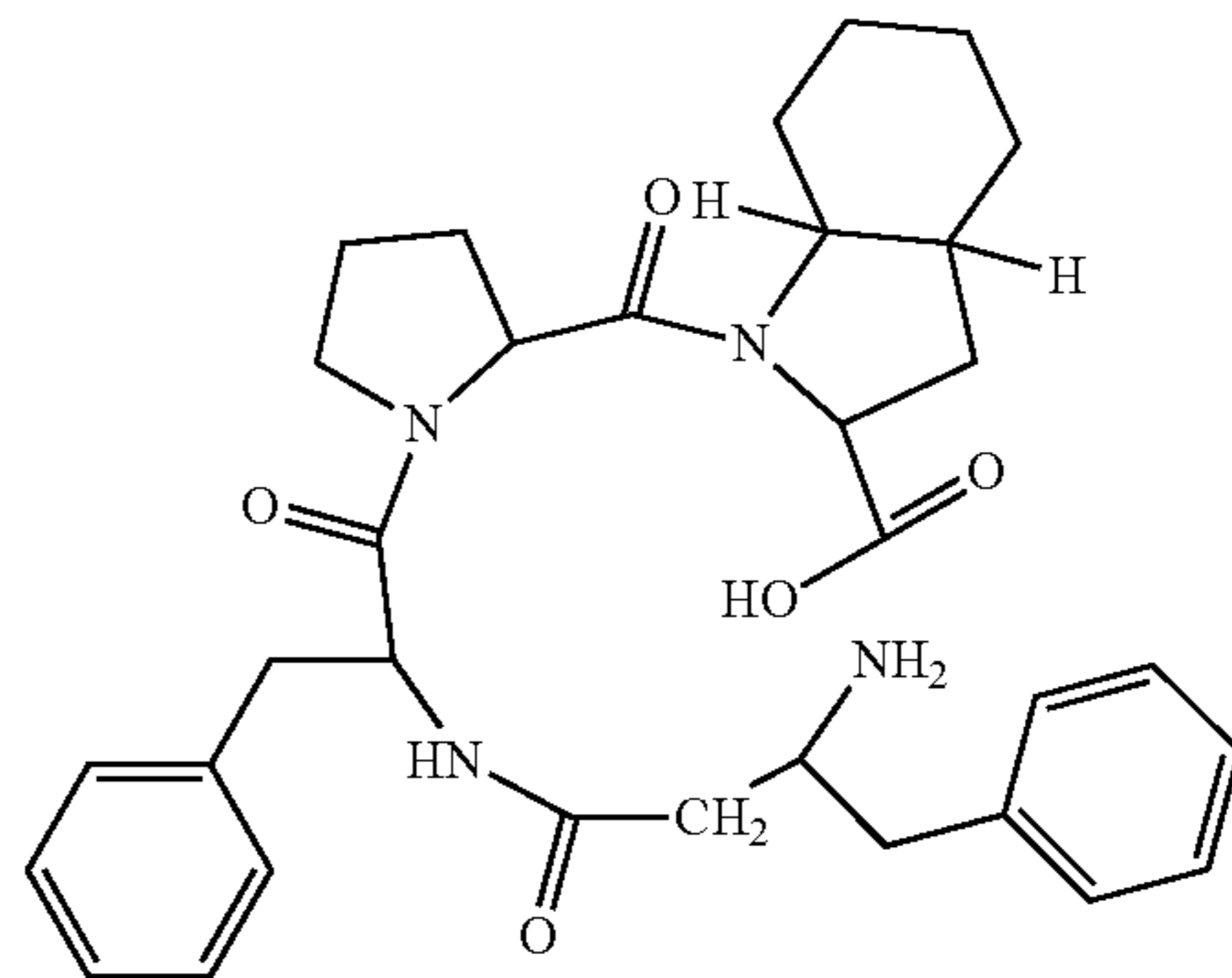
(H-β 3 hoPhe-Phe-Pro-Oic-OH)
