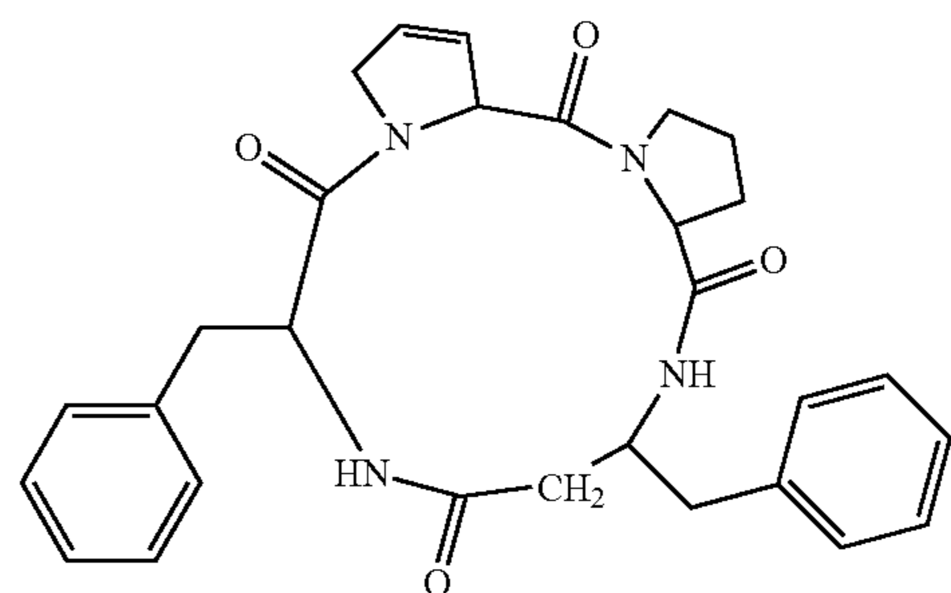
(cyclo(-ΔPro-Pro-β 3 hoPhe-Phe-))
