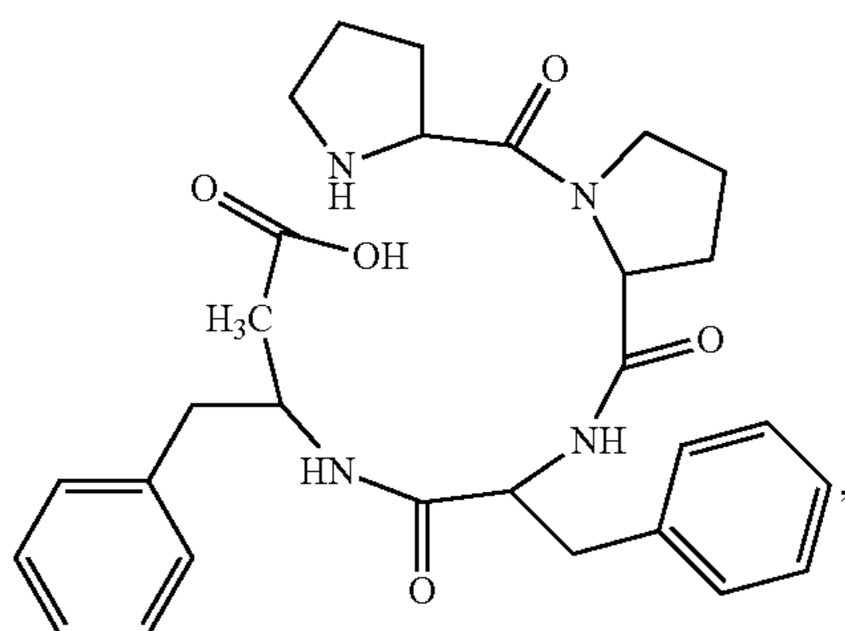
(H-Pro-Pro-Pre-β 3 hoPhe-OH)
