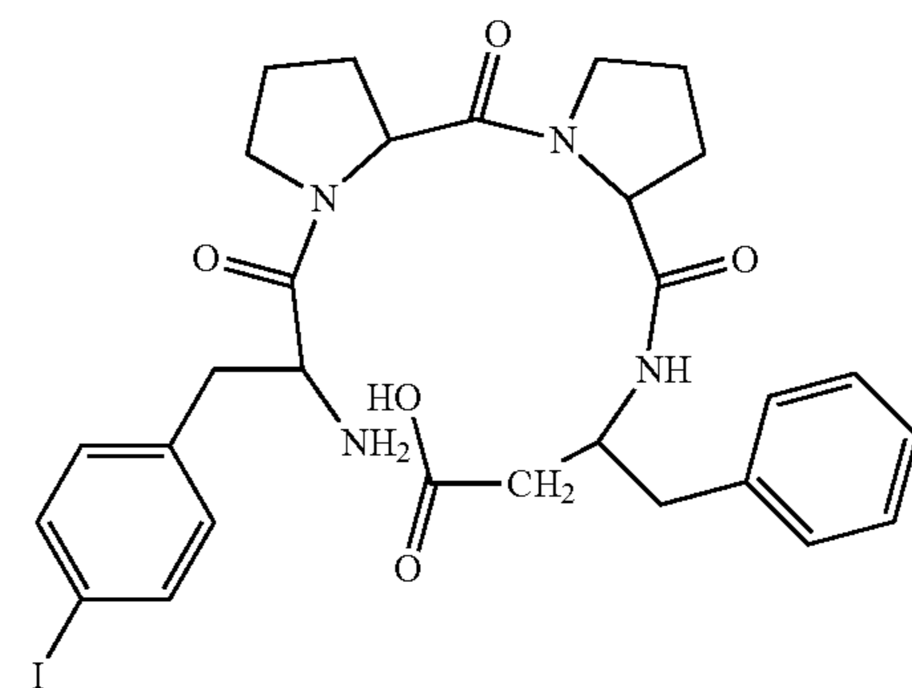
(H-Phe(4I)-Pro-Pro-β 3 hoPhe-OH)
