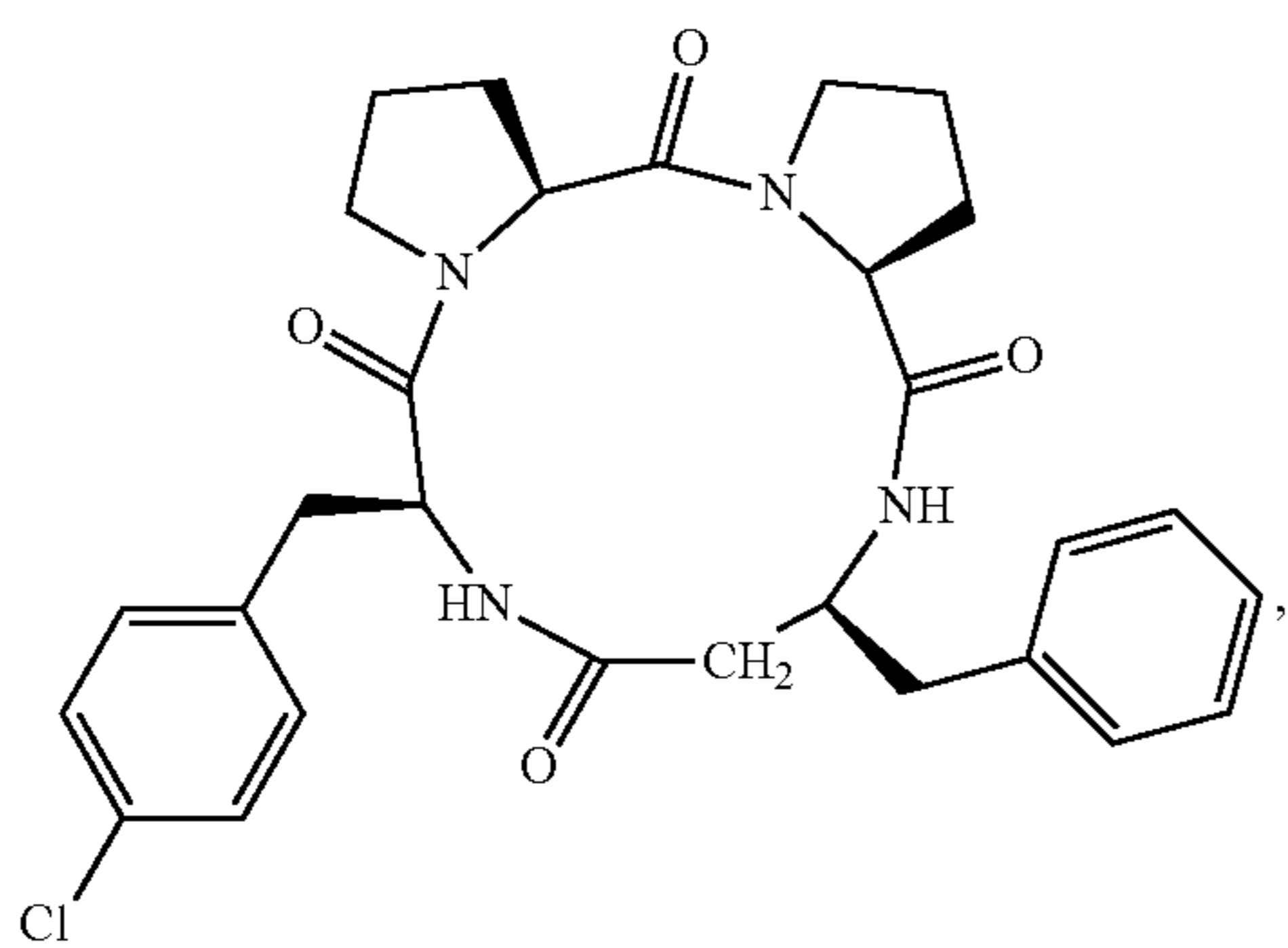
(cyclo(-L-Pro-L-Pro-L-β³hoPhe-L-Phe(4Cl)))
