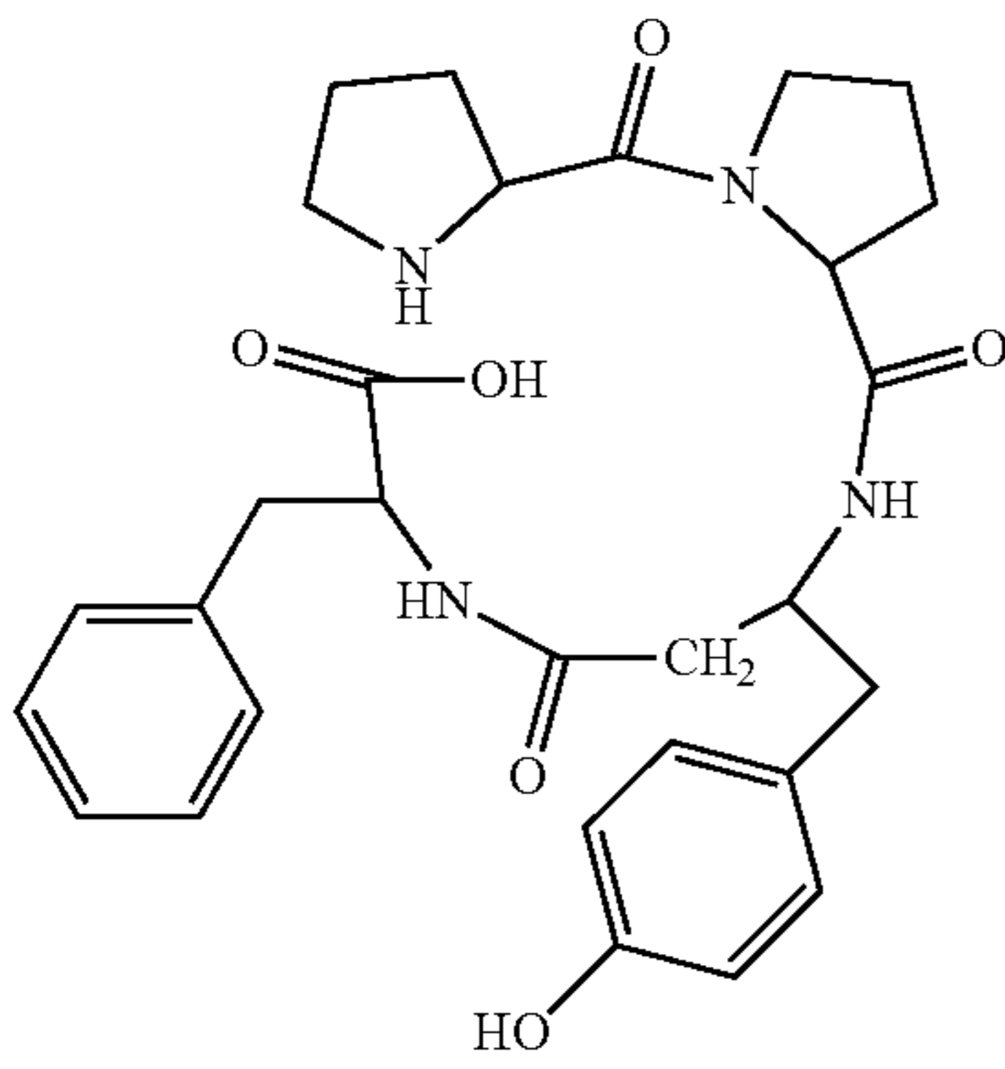
(H-Pro-Pro-β³hoTyr-Phe-OH)
