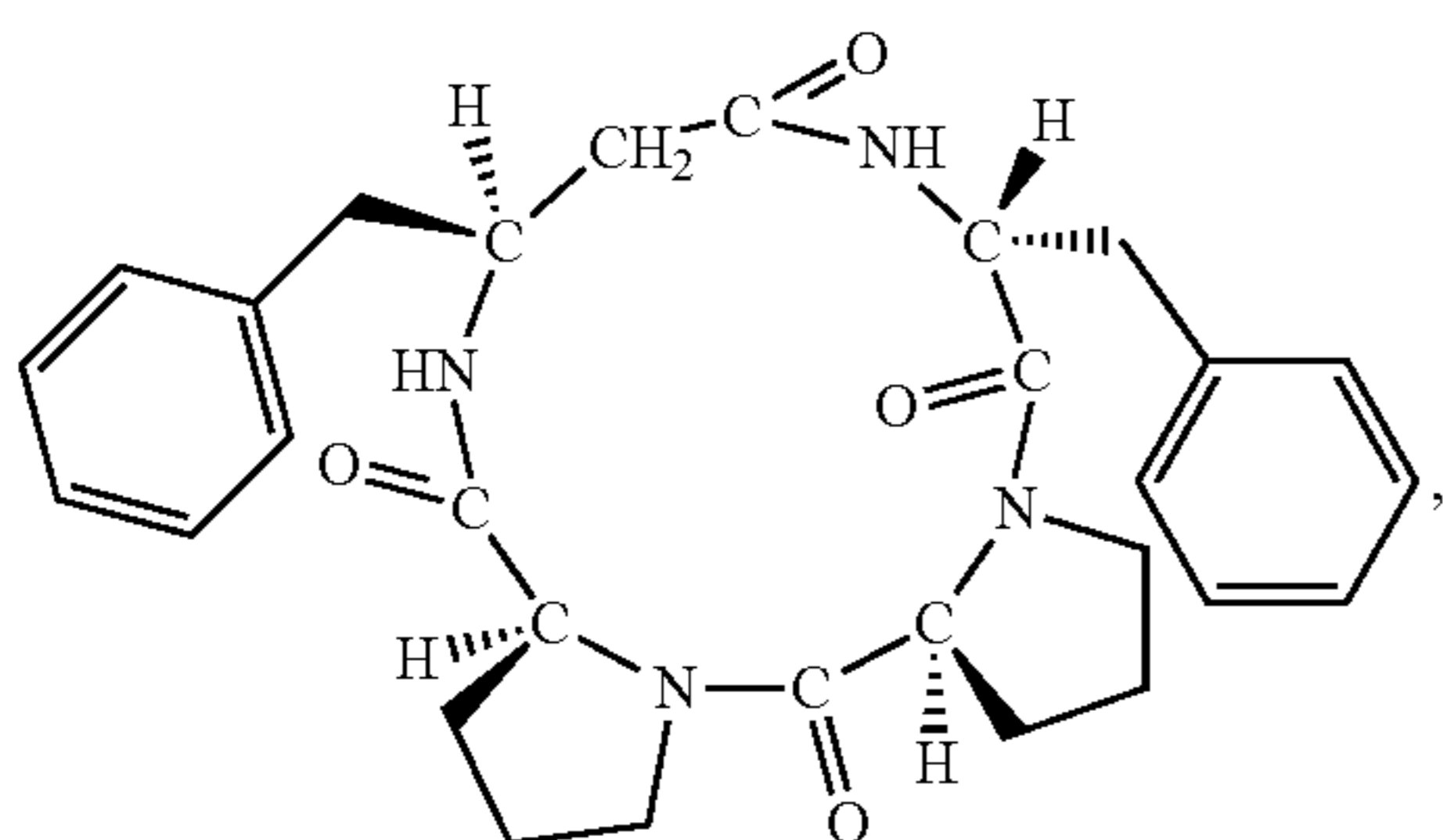
(cyclo(-L-Pro-L-Pro-L-β 3 HoPhe-D-Phe-))
