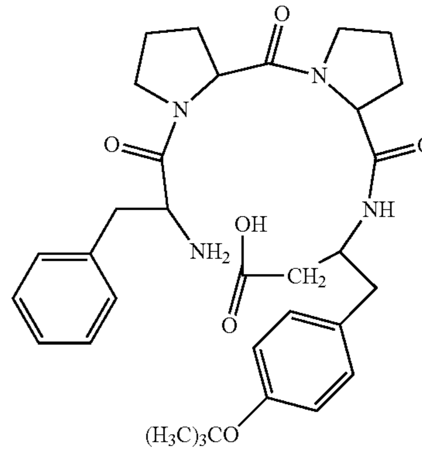
(H-Phe-Pro-Pro-β 3 hoTyr(tBu)-OH)
