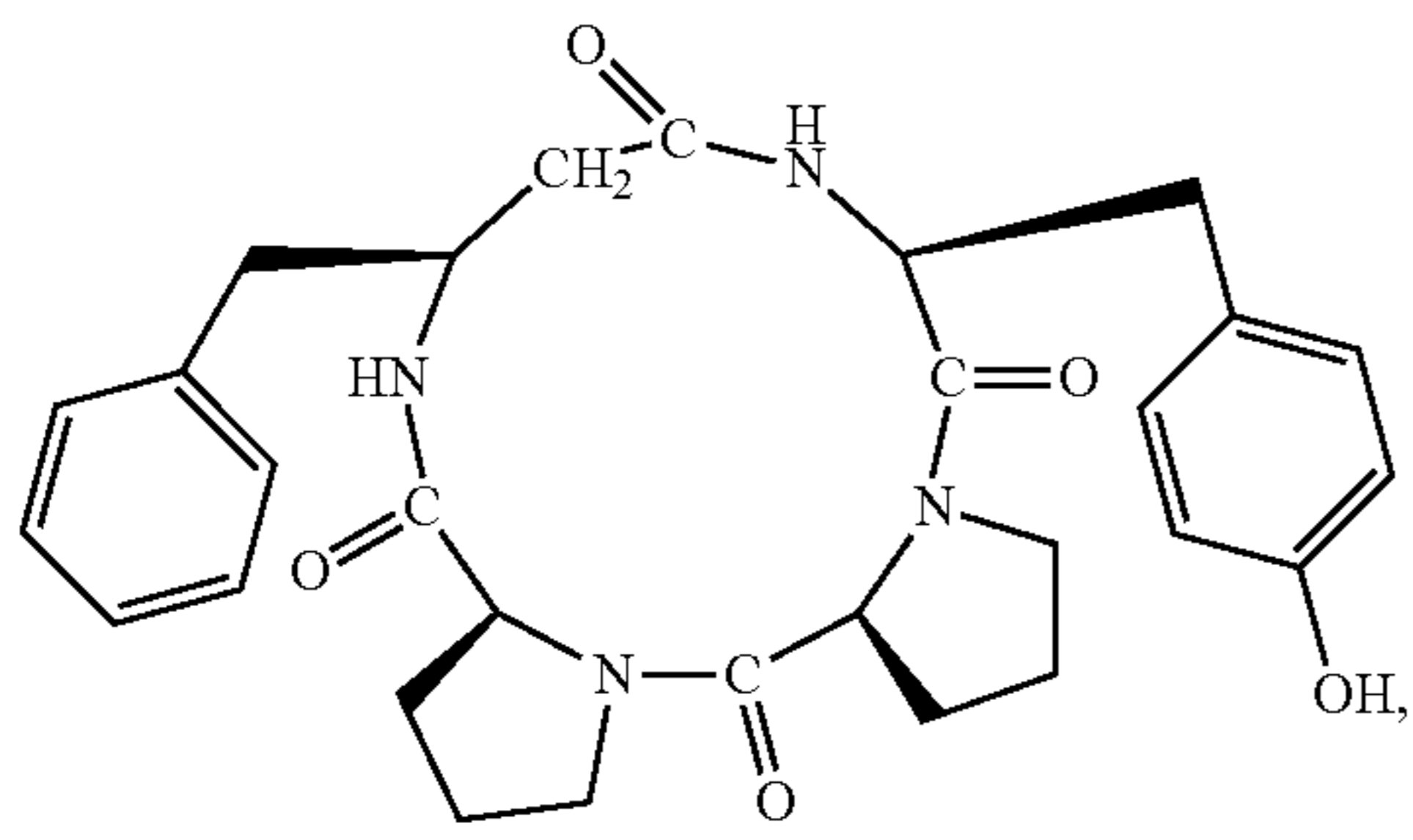
(c(-L-Pro-L-Pro-L-β 3 HoPhe-L-Tyr-))
