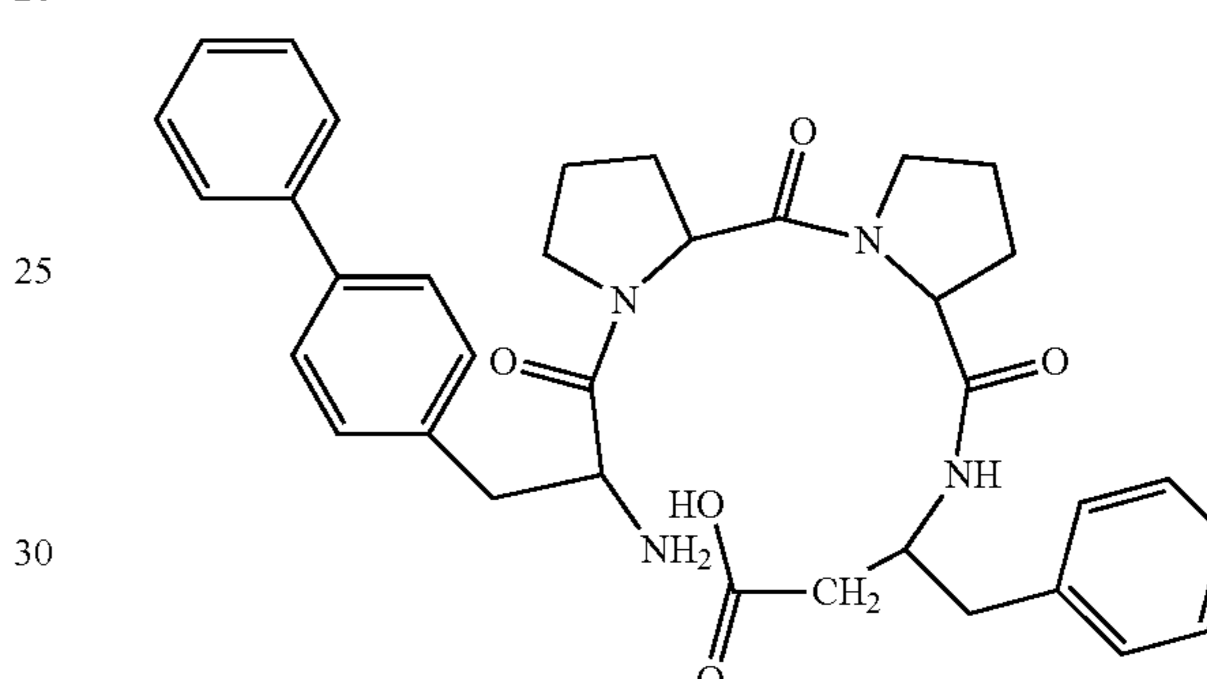
(H-Bip-Pro-Pro-β³hoPhe-OH)
