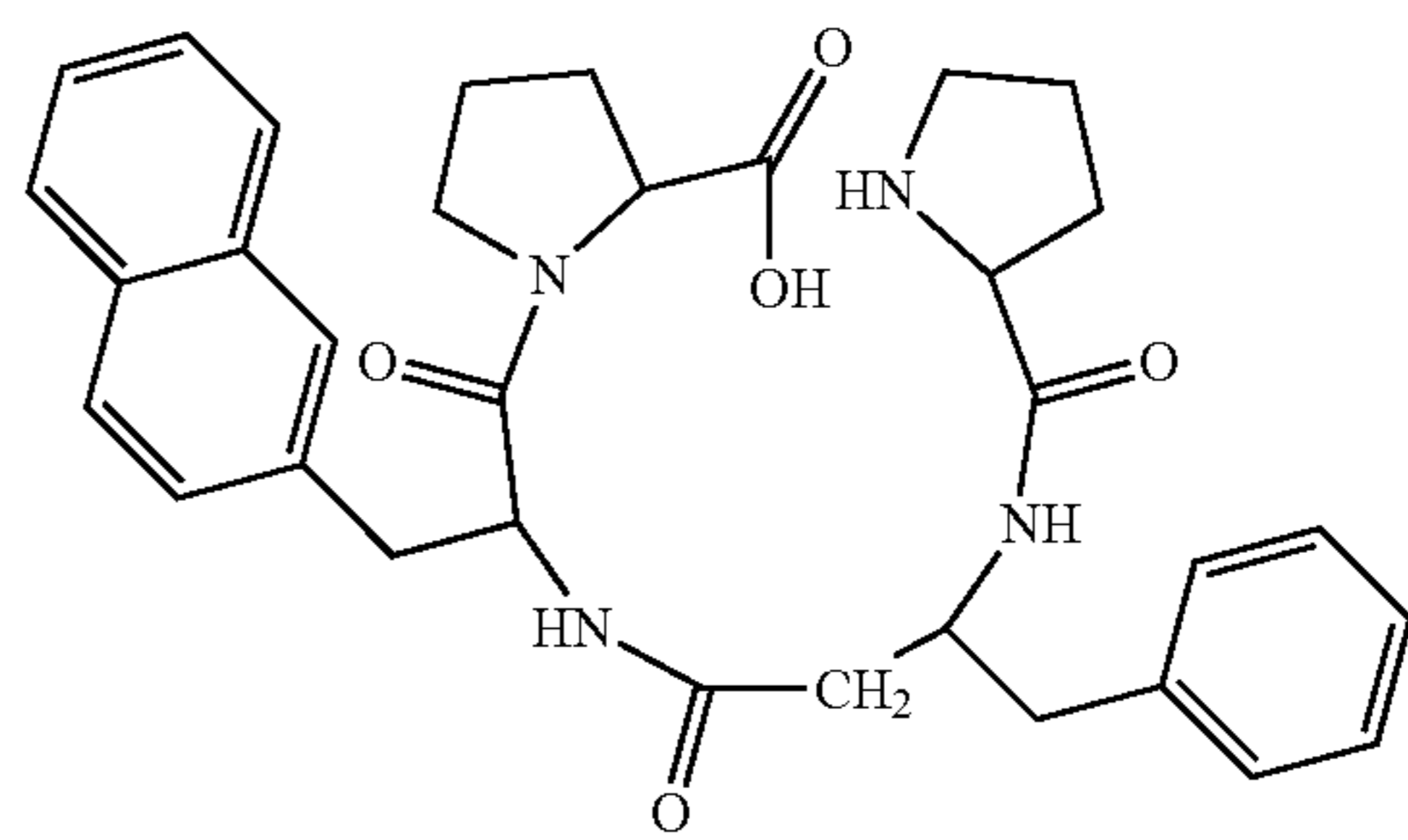
(H-Pro-β 3 hoPhe-2Nal-Pro-OH)
