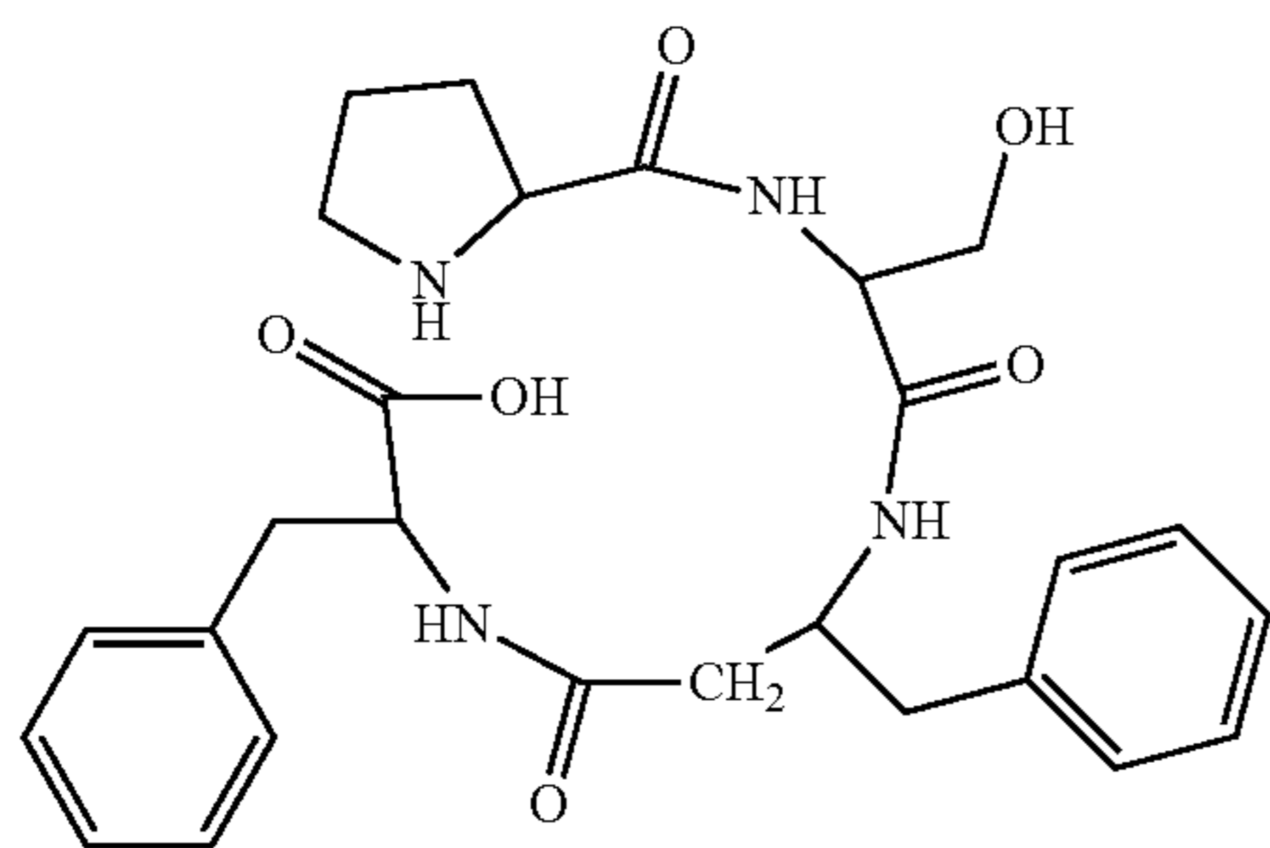
(H-Pro-Ser-β³hoPhe-Phe-OH)
