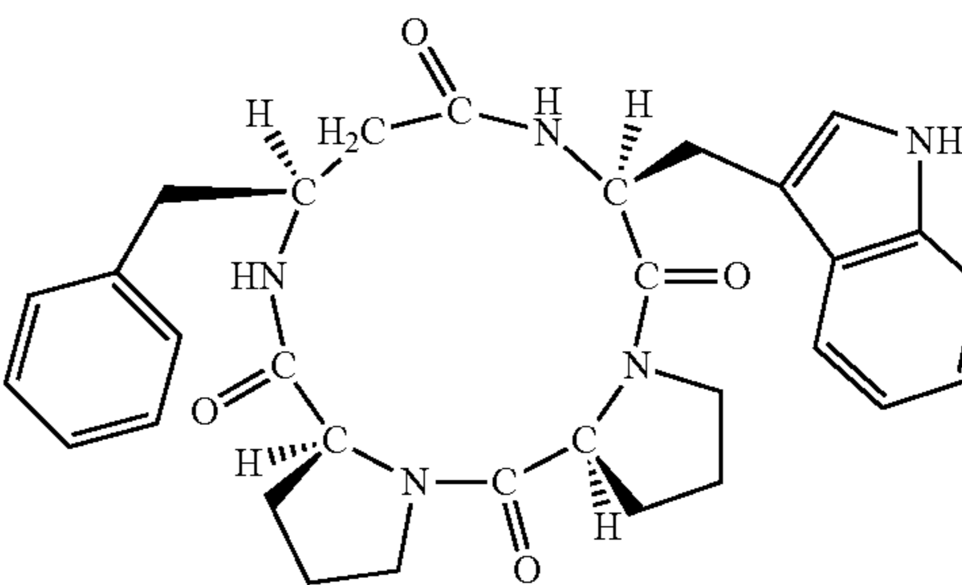
(cyclo(-L-Pro-L-Pro-L-β 3 HoPhe-L-Trp-))
