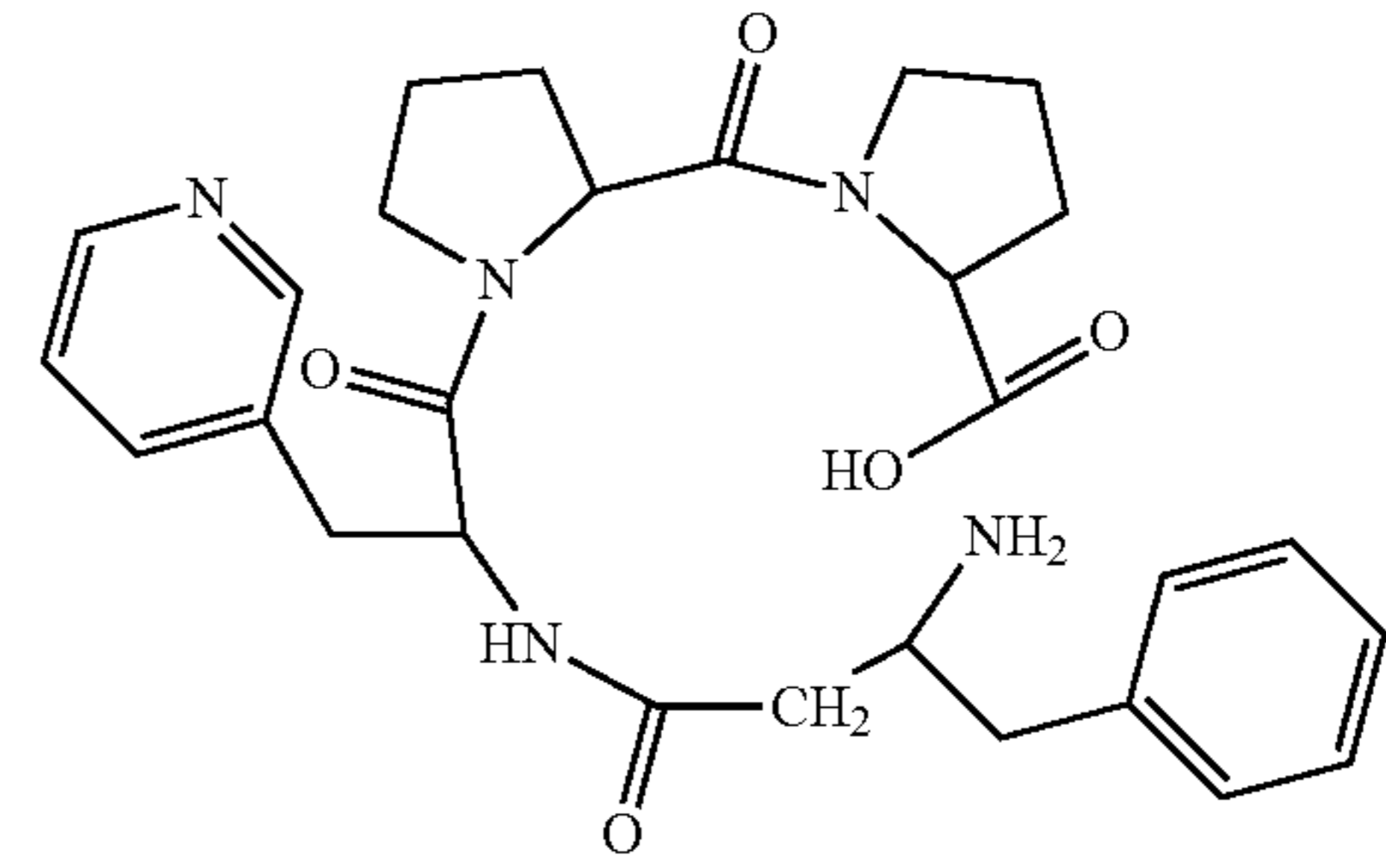
(H-β 3 hoPhe-Pal-Pro-Pro-OH)
