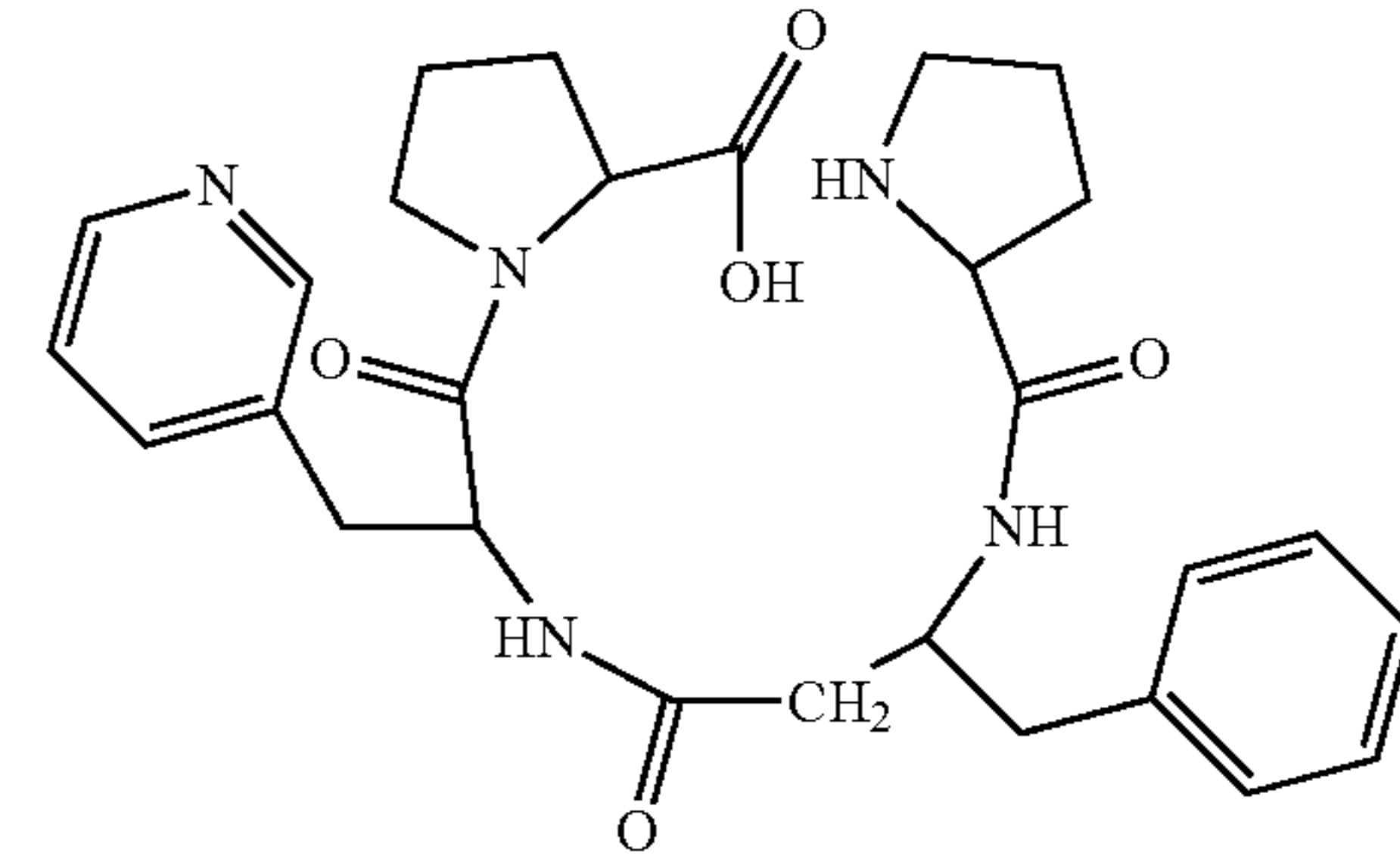
(H-Pro-β 3 hoPhe-Pal-Pro-OH)
