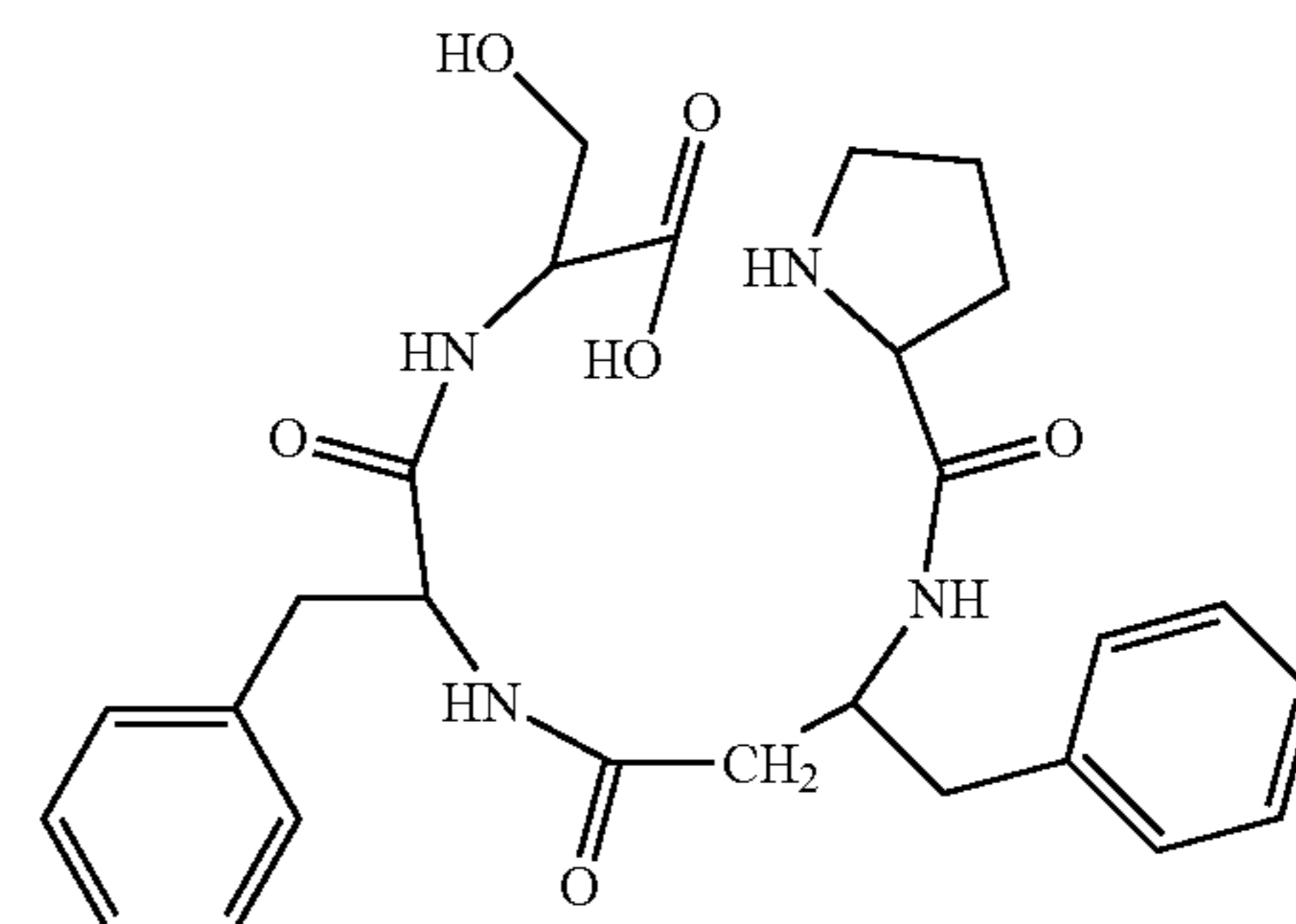
(H-Pro-β³hoPhe-Phe-Ser-OH)
