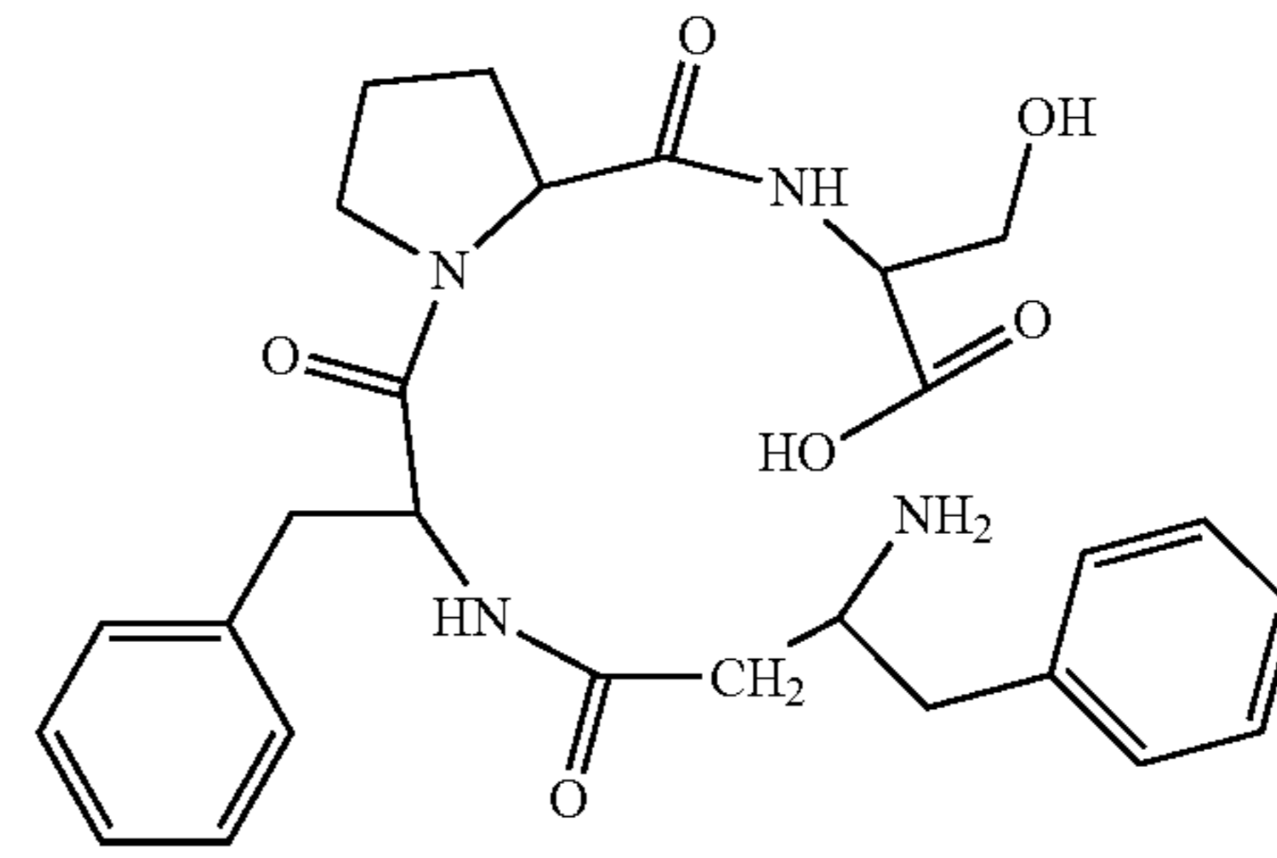
(H-β³hoPhe-Phe-Pro-Ser-OH)
