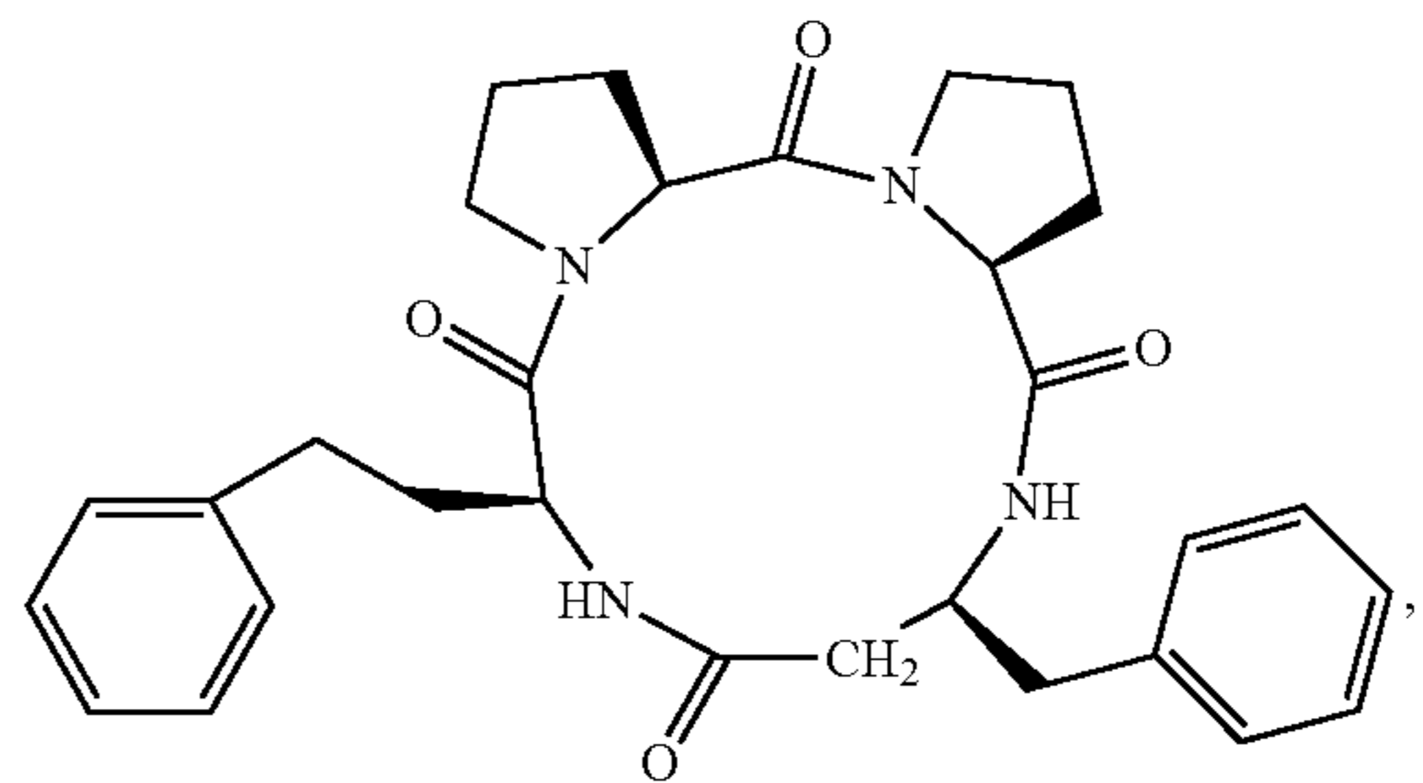
(cyclo(-L-Pro-L-Pro-L-β³hoPhe-L-hoPhe))
