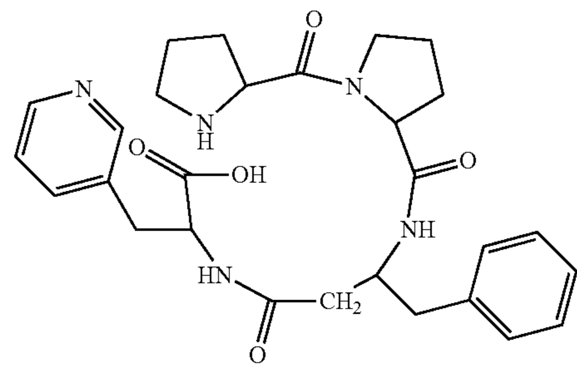
(H-Pro-Pro-β 3 hoPhe-Pal-OH)
