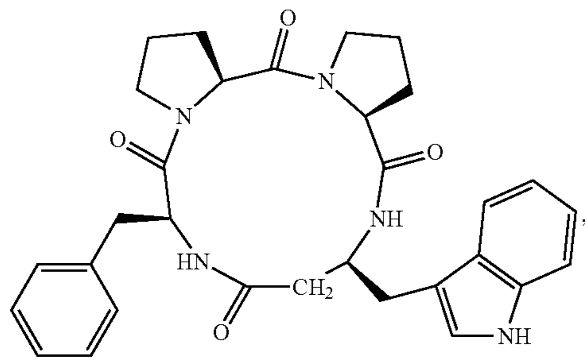
(cyclo(-L-Pro-L-Pro-L-β³hoPhe-L-Phe))
