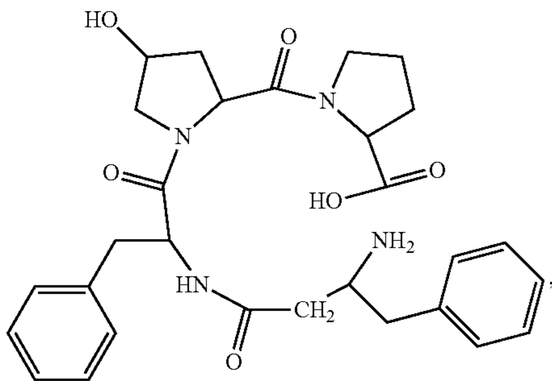
(H-β³hoPhe-Phe-Hyp-Pro-OH)
