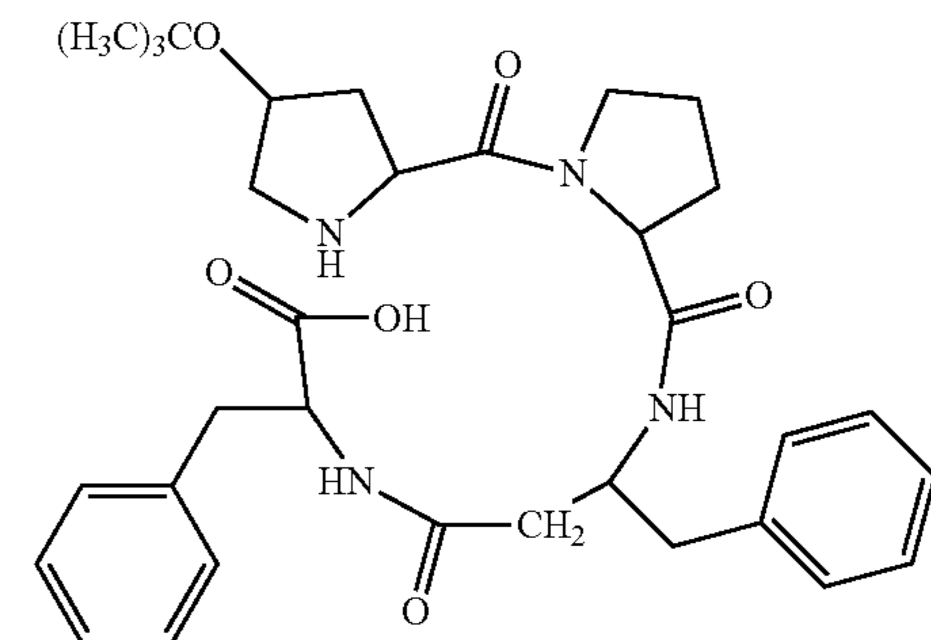
(H-Hyp(tBu)-Pro-β 3 hoPhe-Phe-OH)
