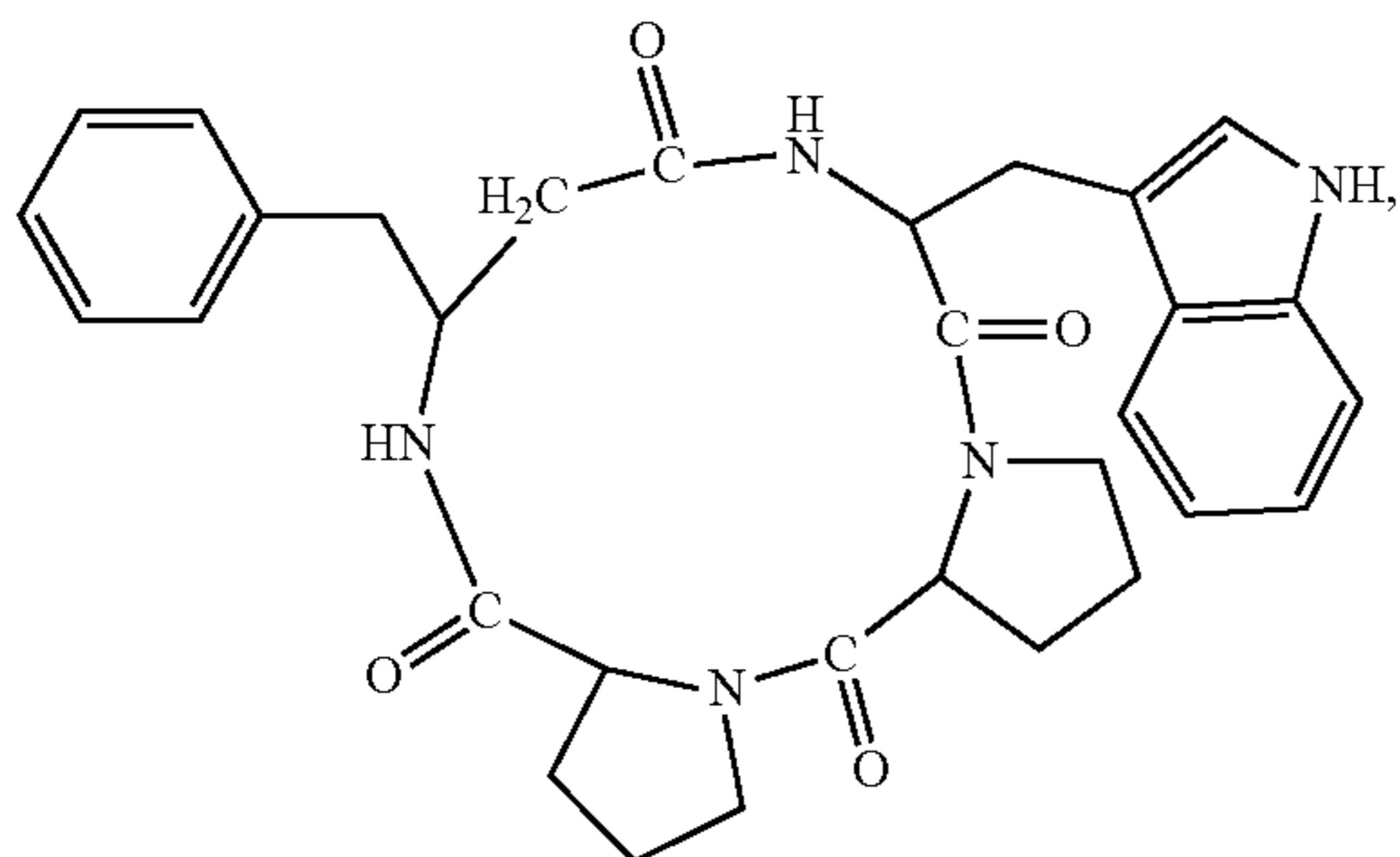
(cyclo(-Pro-Pro-β 3 hoPhe-Trp-))
