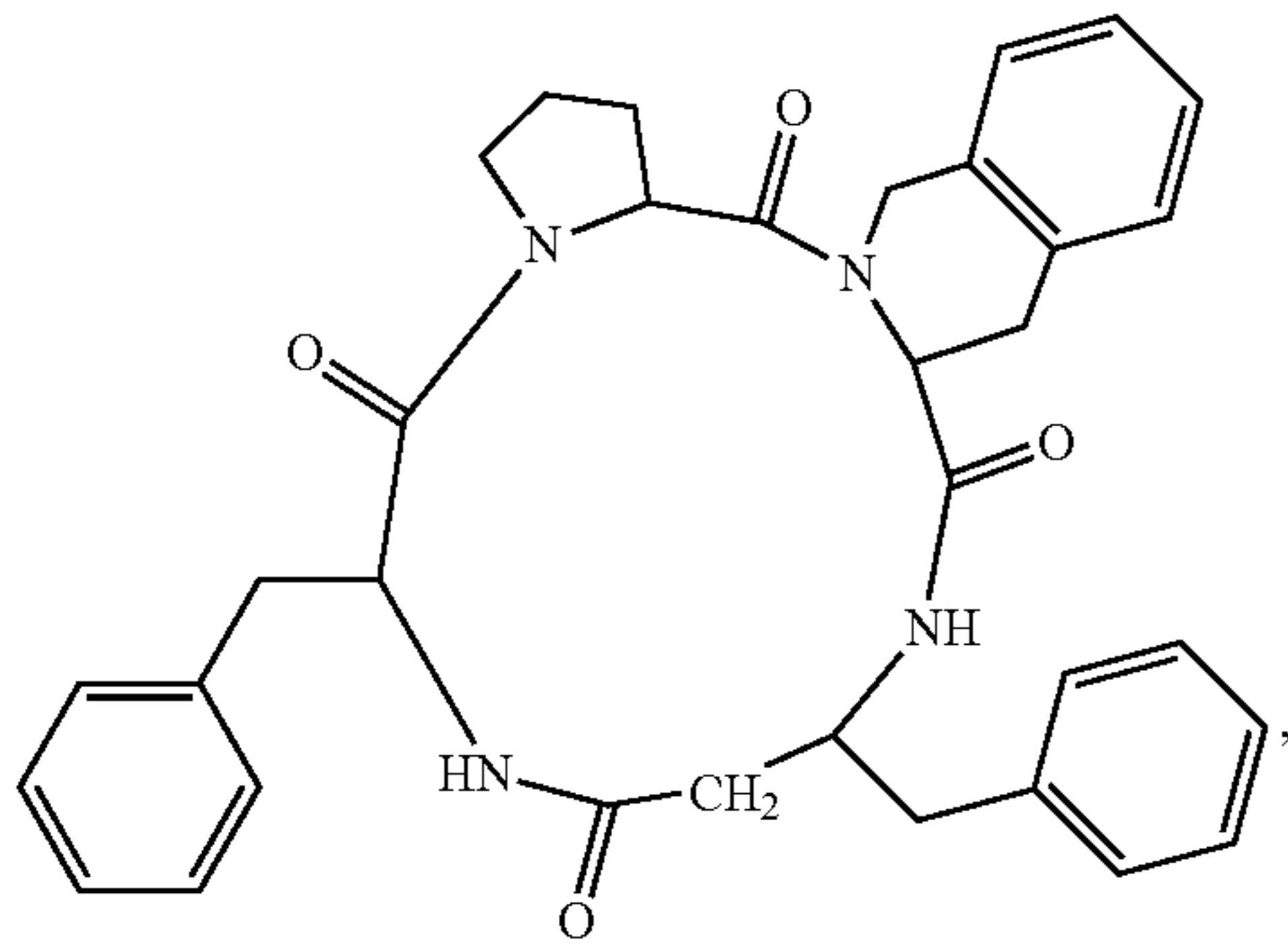
(cyclo(-Pro-Tic-β³hoPhe-Phe-))
