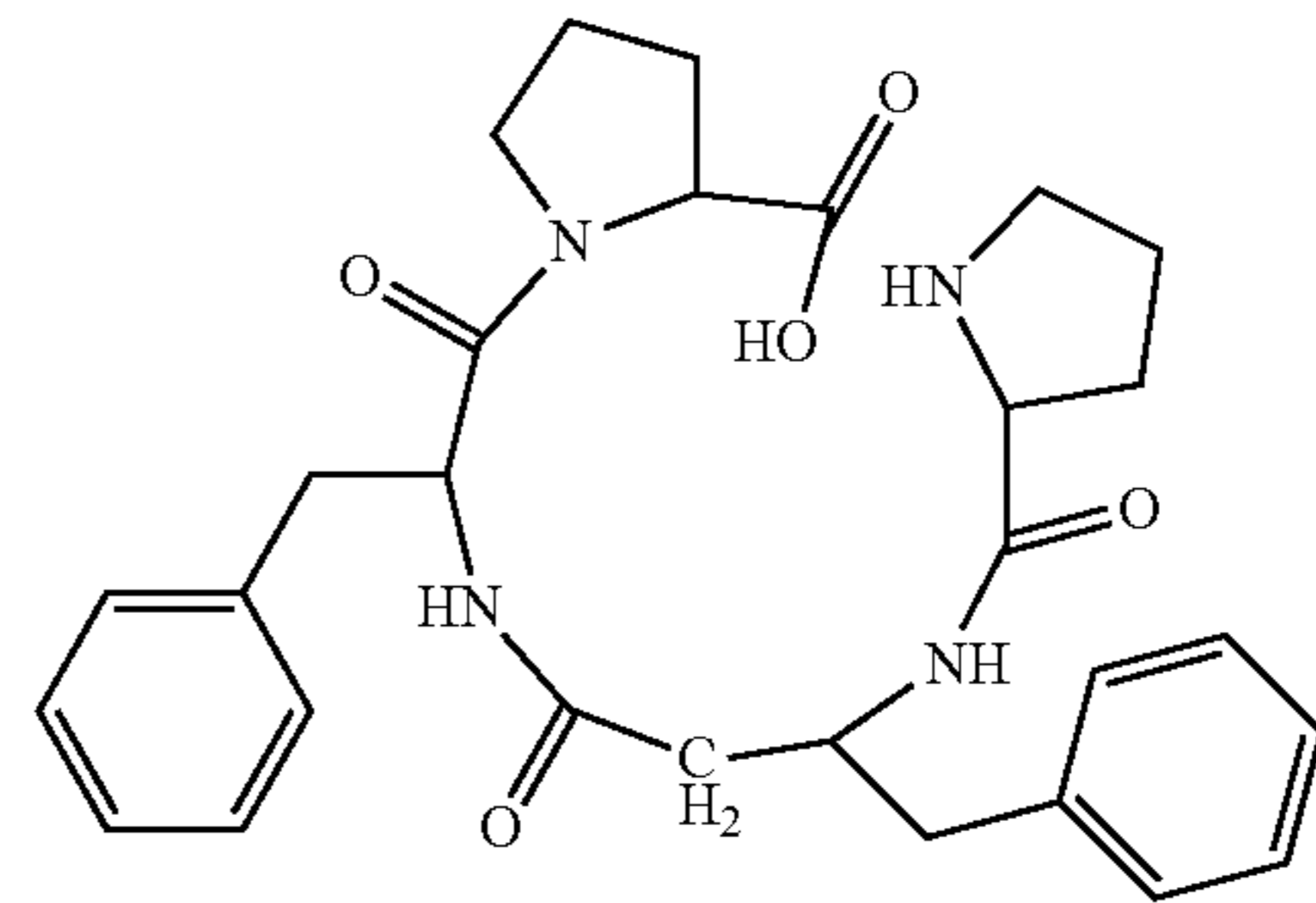
(H-Pro-β 3 hoPhe-Phe-Pro-OH)
