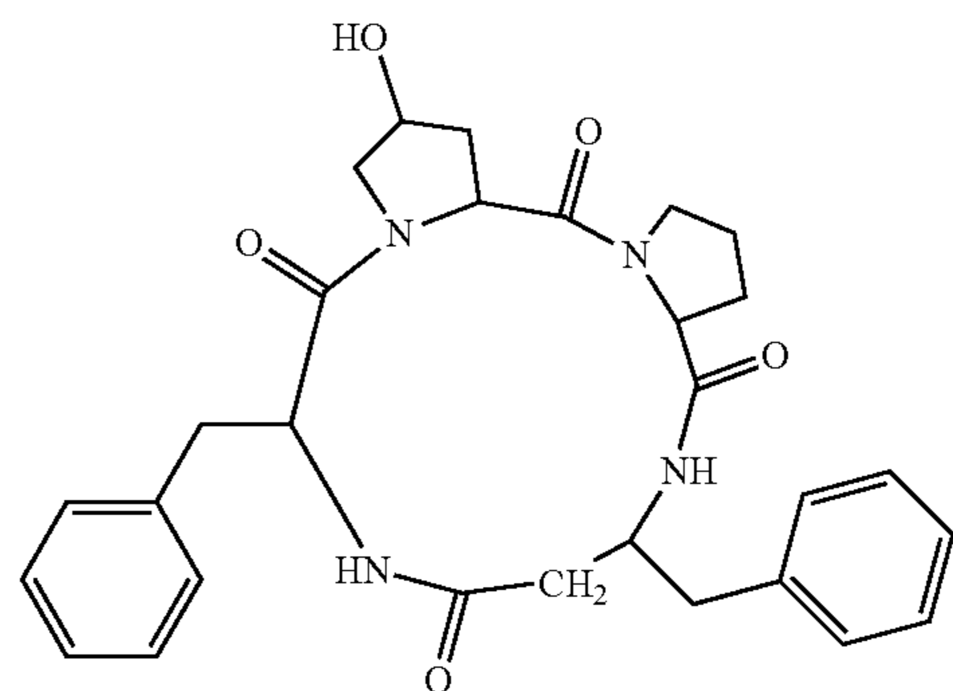
(cyclo(-Hyp-Pro-β 3 hoPhe-Phe-))
