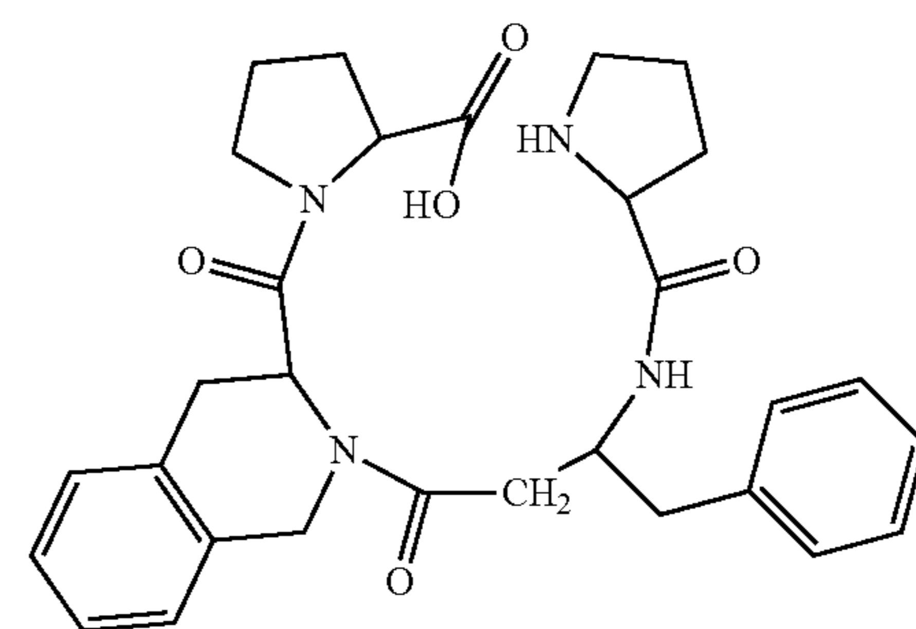
(H-Pro-β 3 hoPhe-Tic-Pro-OH)
