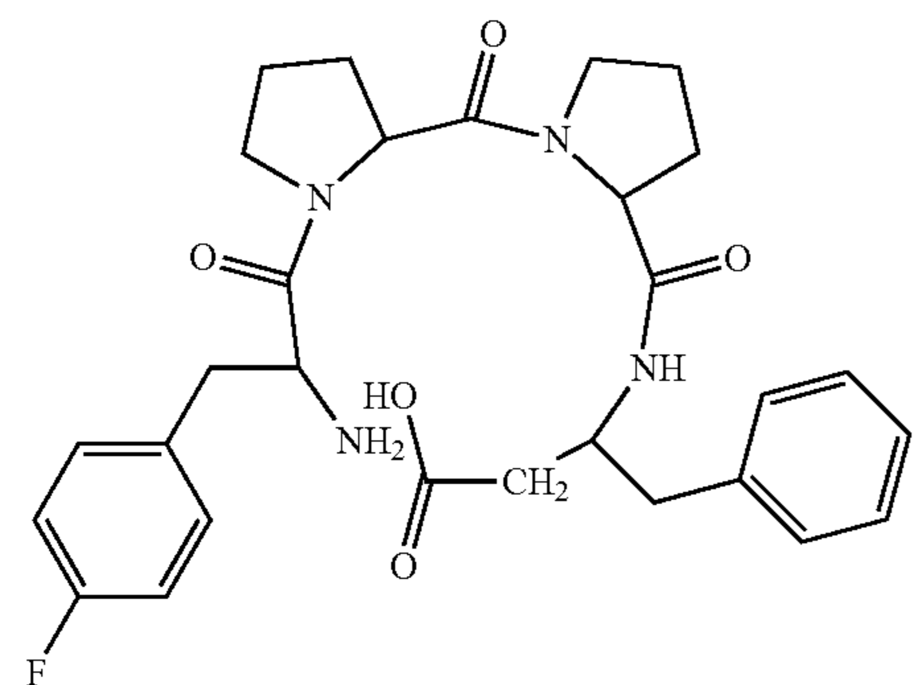
(H-Phe(4F)-Pro-Pro-β 3 hoPhe-OH)
