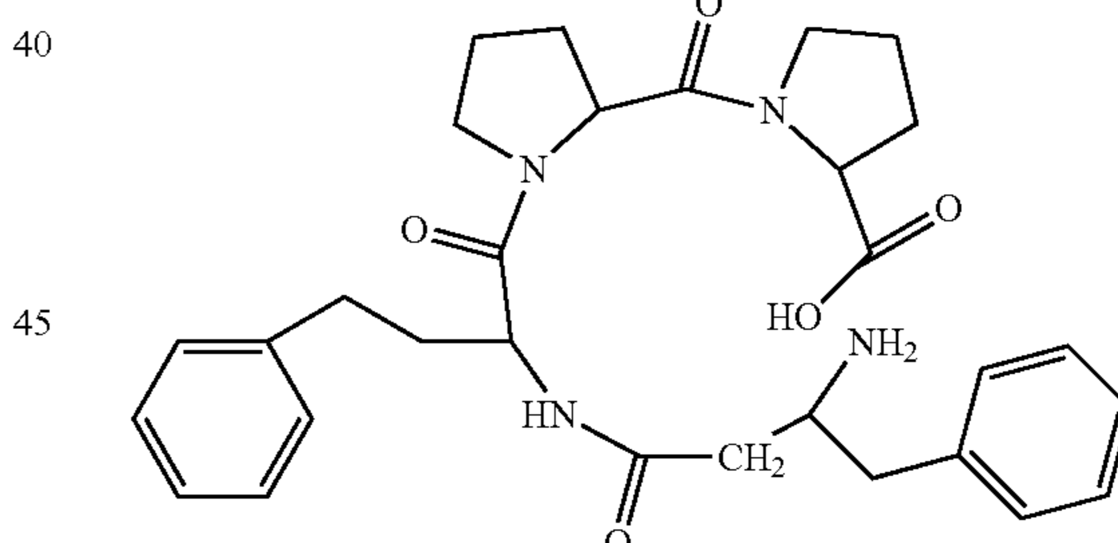
(H-β³hoPhe-hoPhe-Pro-Pro-OH)
