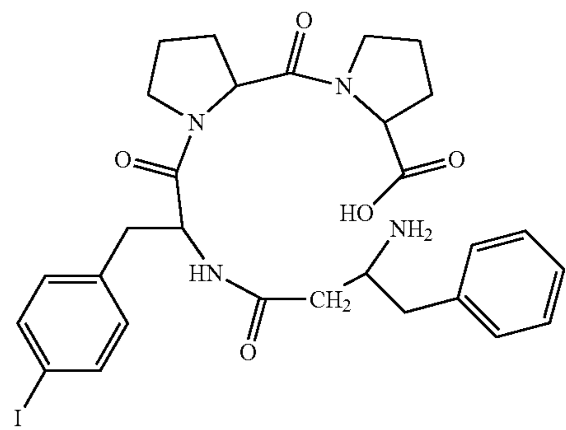
(H-β 3 hoPhe-Phe(4I)-Pro-Pro-OH)
