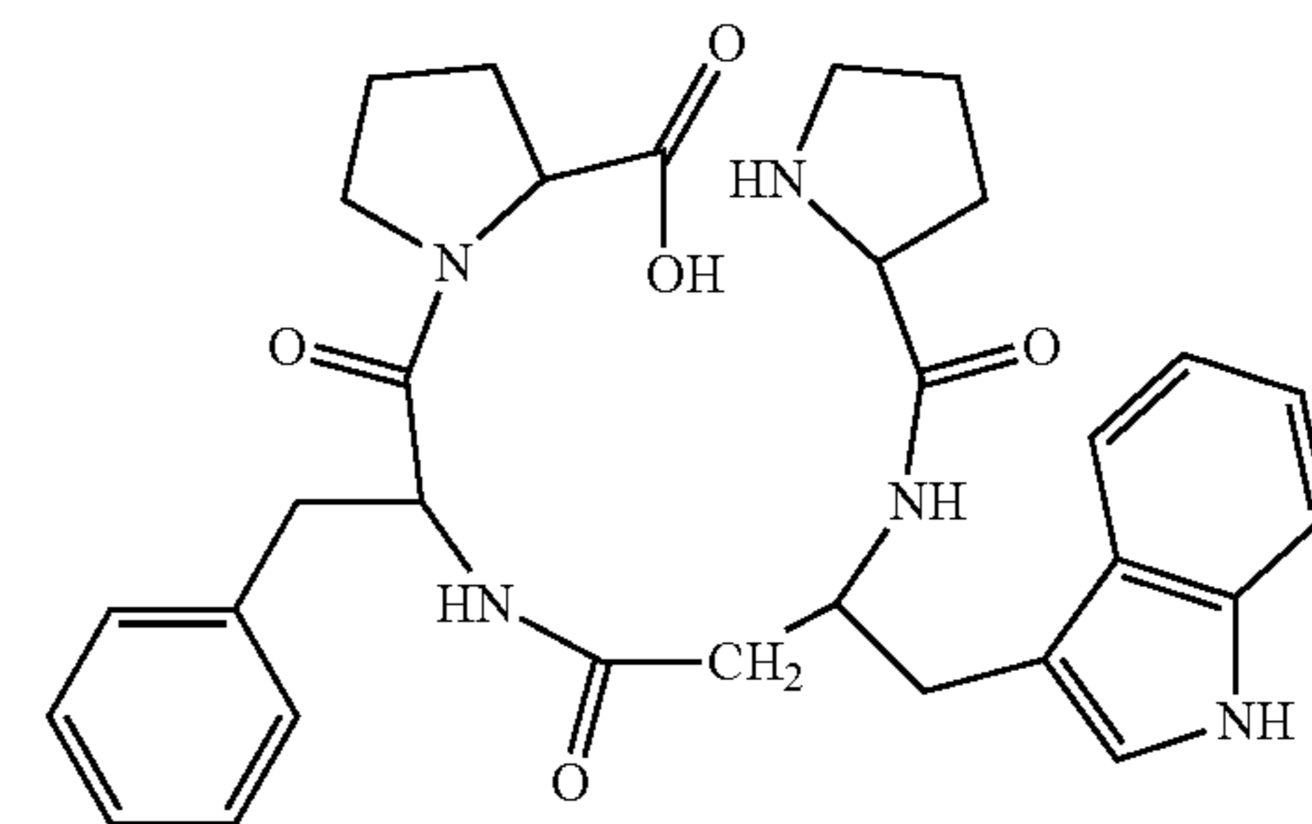
(H-Pro-β 3 hoTrp-Phe-Pro-OH)
