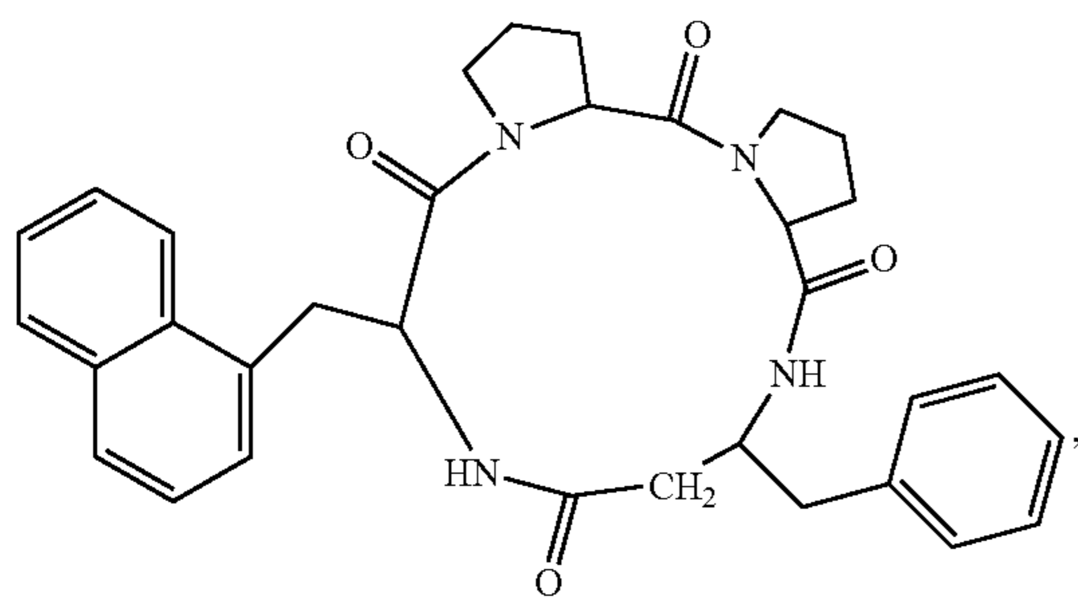
(cyclo(-Pro-Pro-β 3 hoPhe-1Nal))
