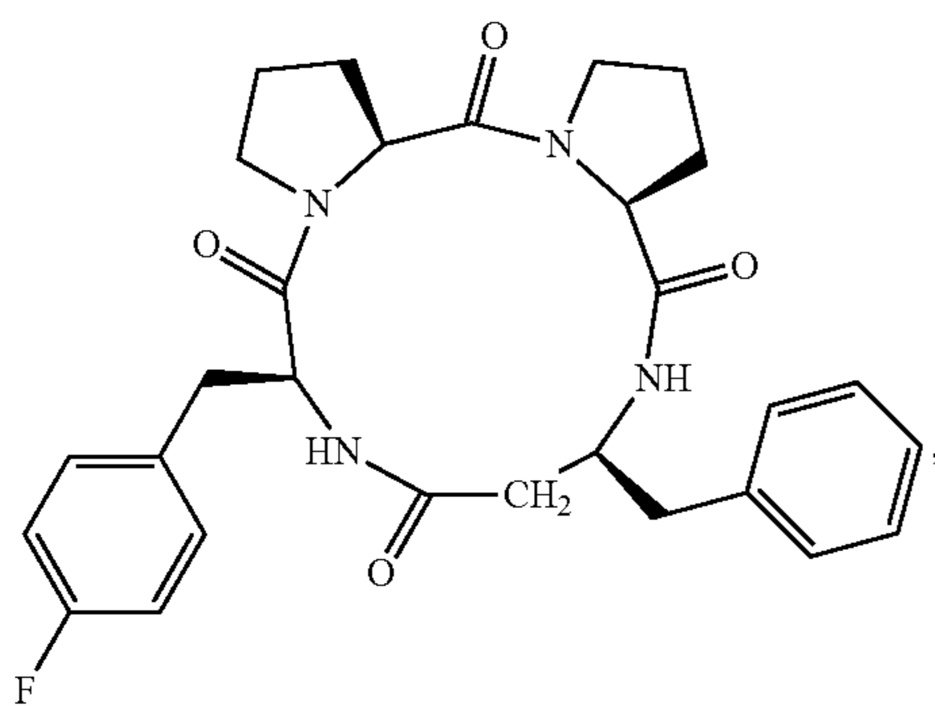
cyclo(-L-Pro-L-Pro-L-β³hoPhe-L-Phe(4F)))
