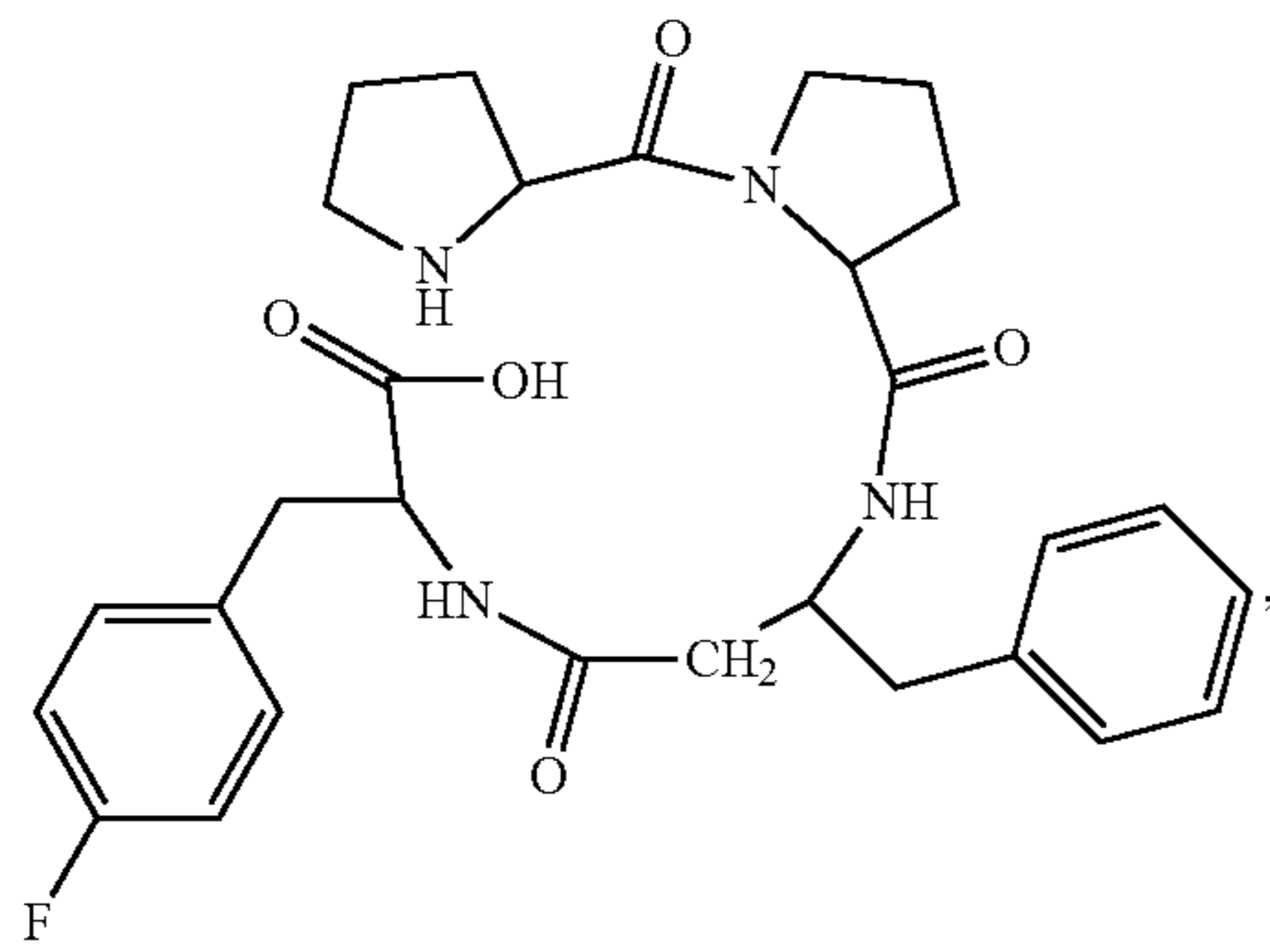
(H-Pro-Pro-β 3 hoPhe-Phe(4F)-OH)
