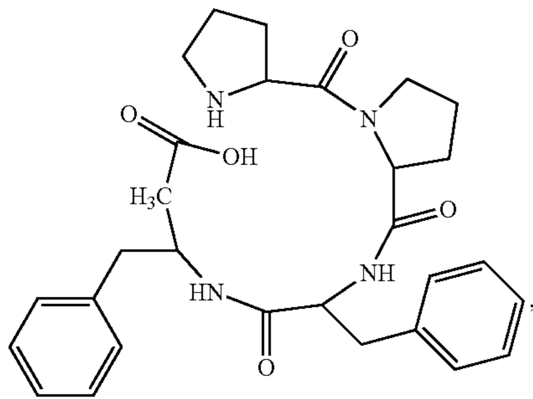
(H-Pro-Pro-Pre-β 3 hoPhe-OH)
