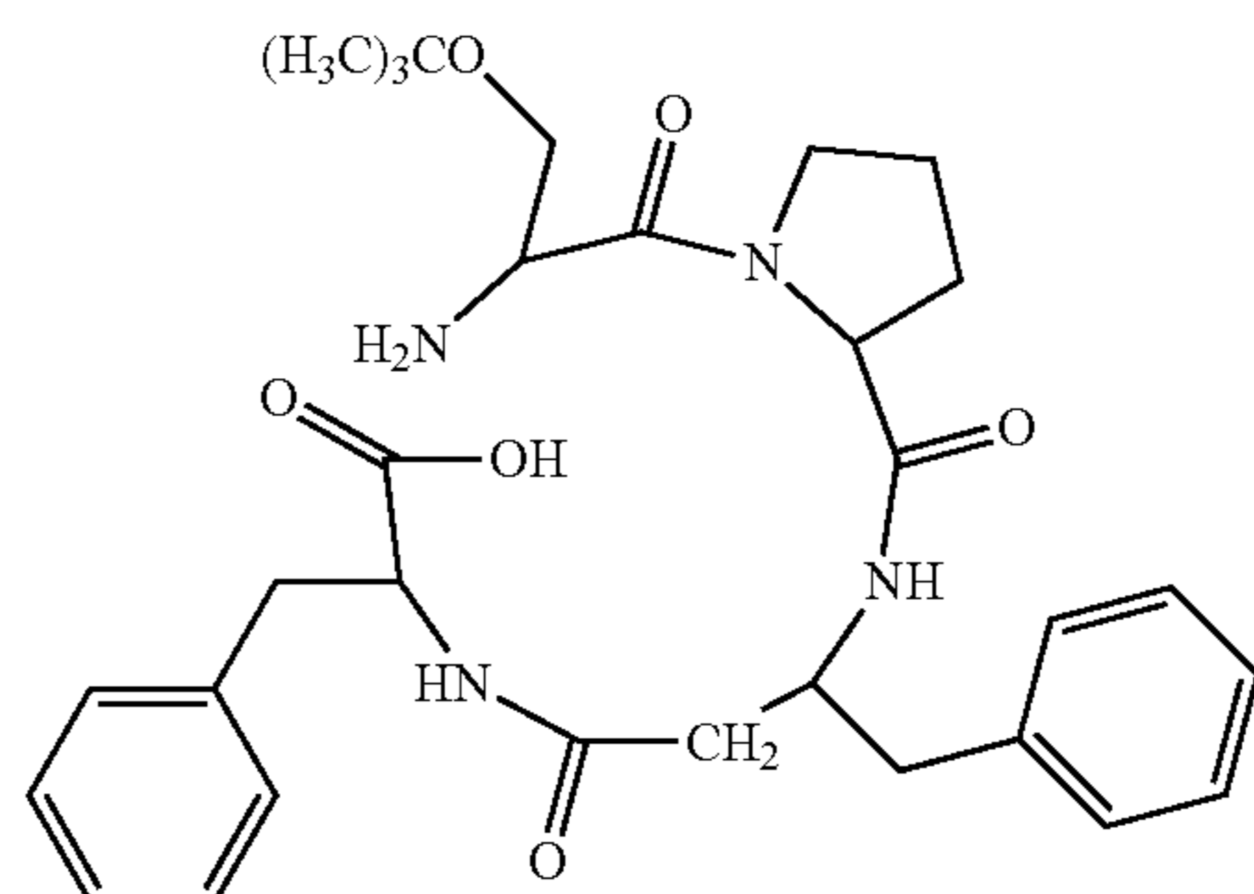
(H-Ser(tBu)-Pro-β³hoPhe-Phe-OH)
