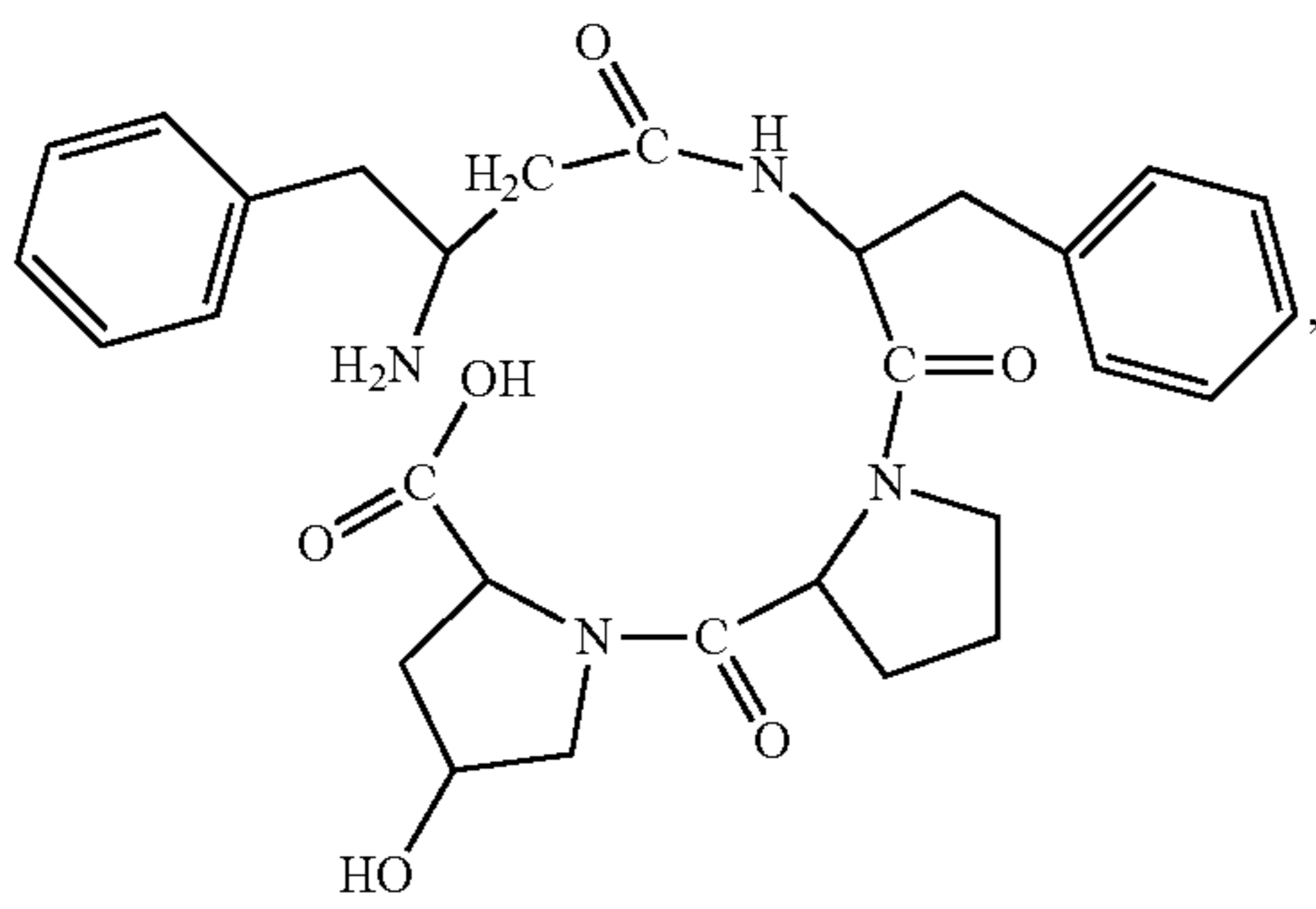
(H-β 3 hoPhe-Phe-Pro-Hyp-OH)
