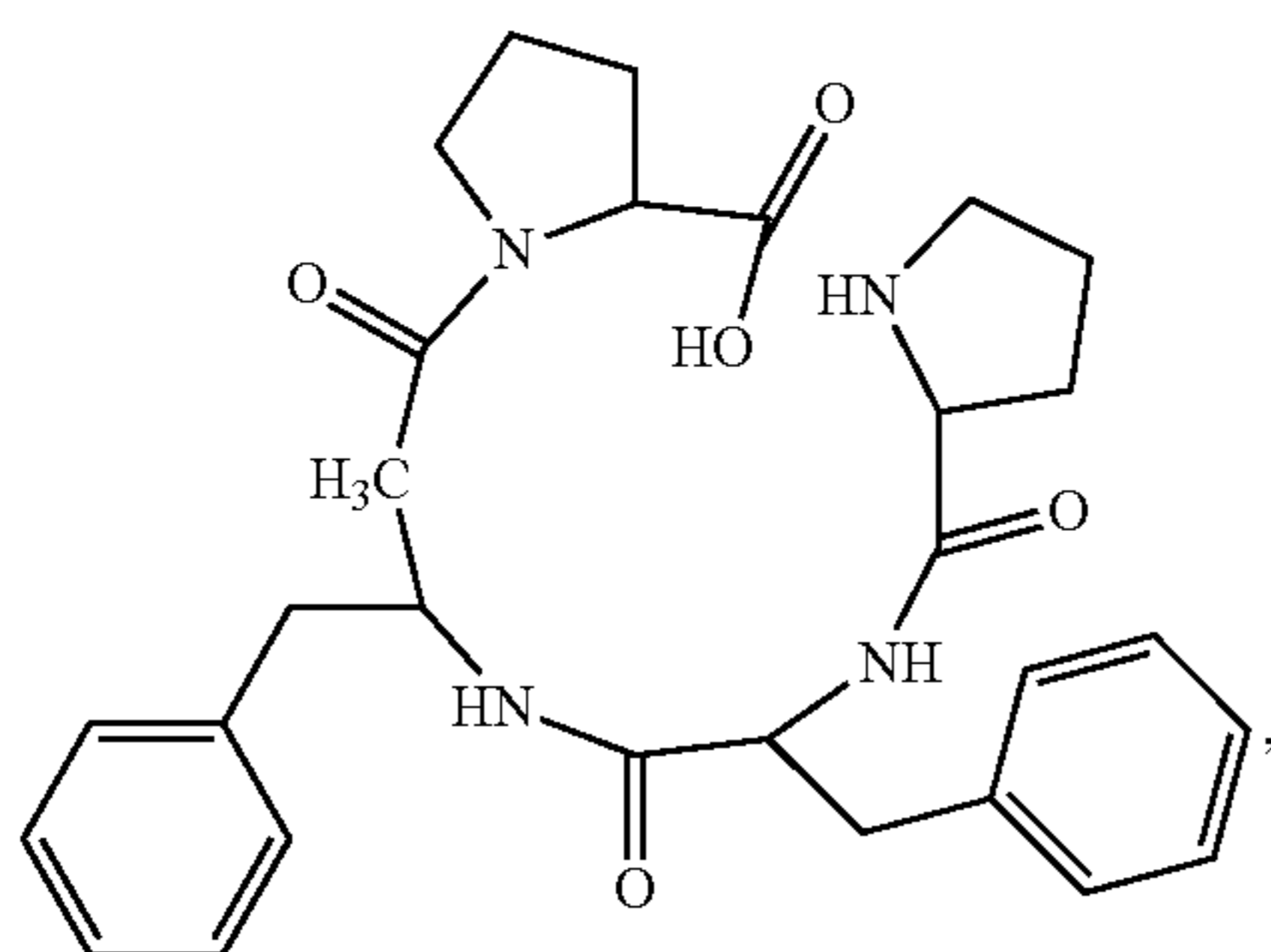
(H-Pro-Pro-Phe-β 3 hoPhe-OH)
