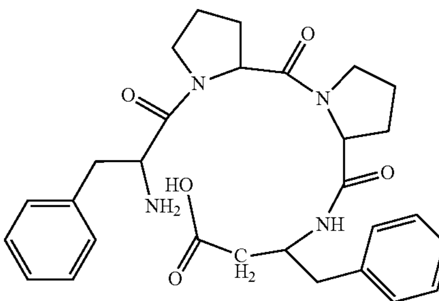
(H-Phe-Pro-Pro-β 3 hoPhe-OH)
