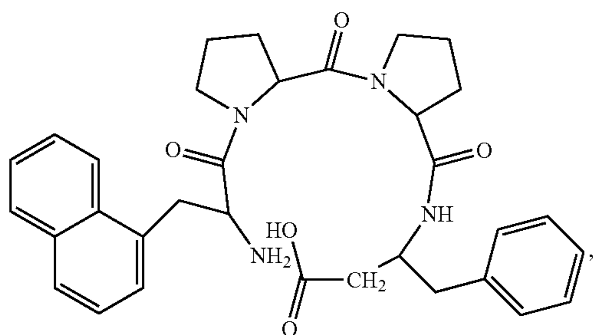
(H-1Nal-Pro-Pro-β 3 hoPhe-OH)
