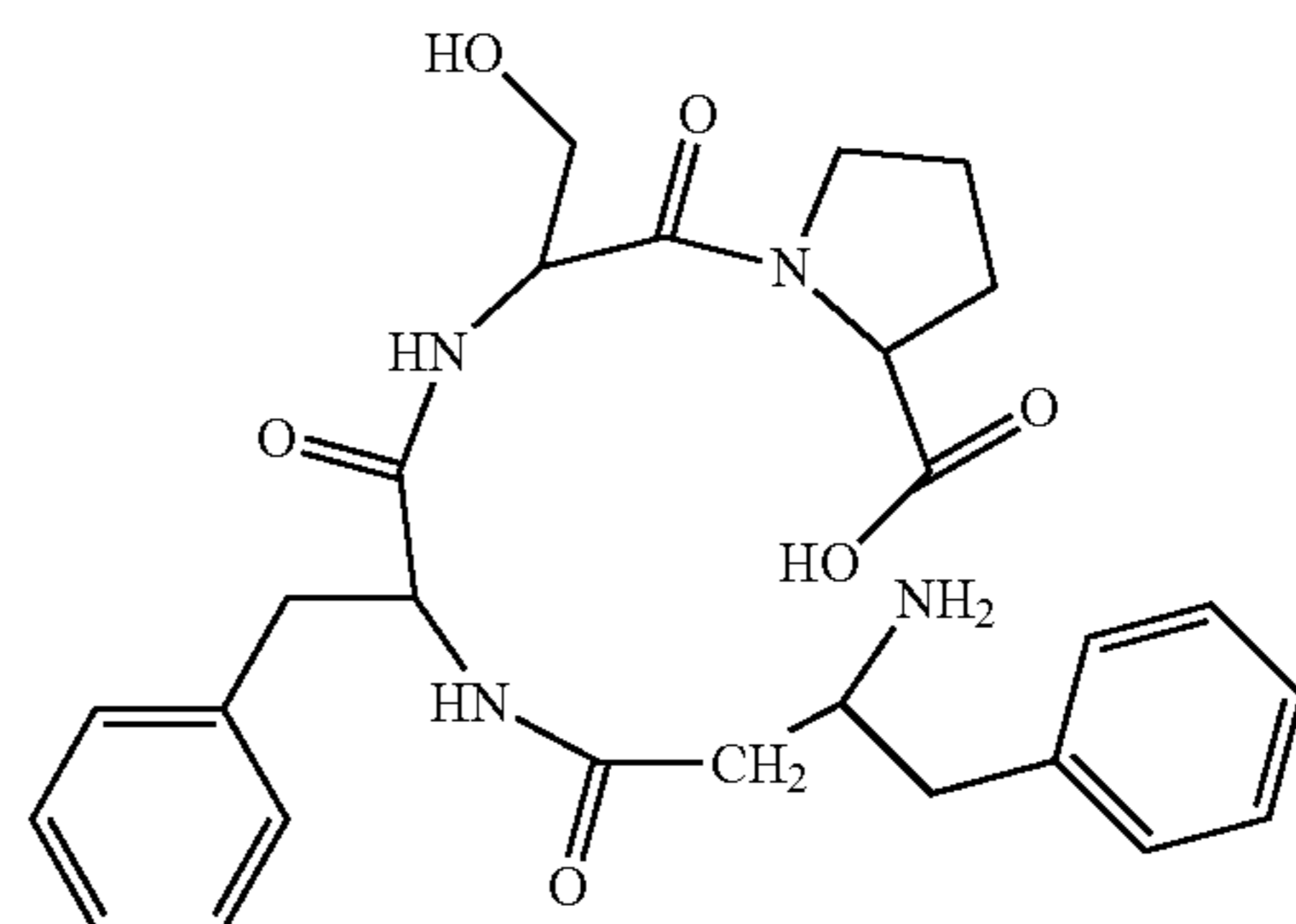
(H-β³hoPhe-Phe-Ser-Pro-OH)
