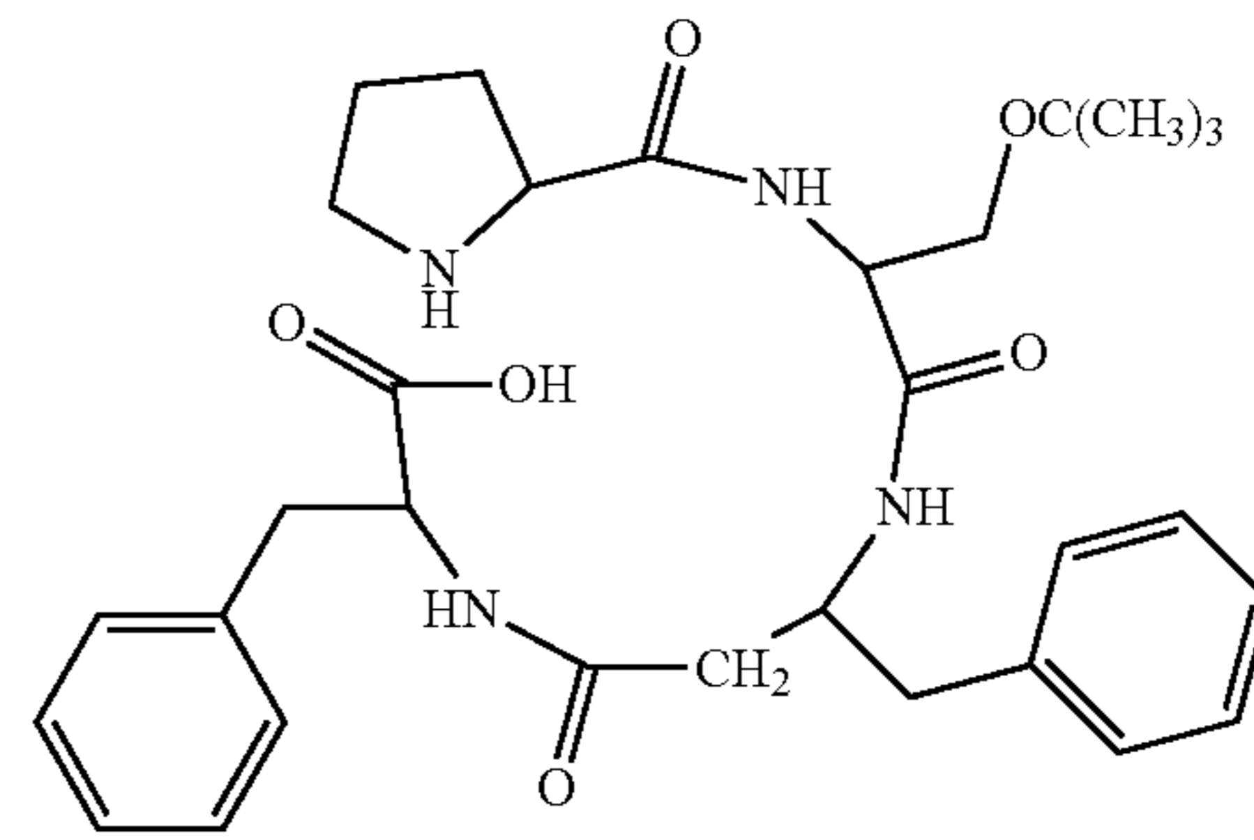
(H-Pro-Ser(tBu)-β³hoPhe-Phe-OH)
