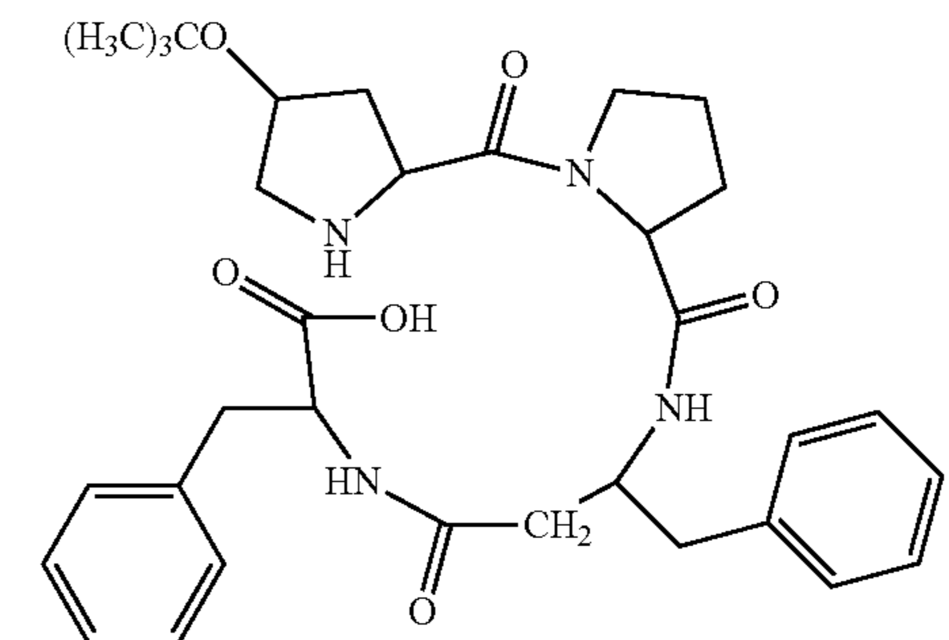
(H-Hyp(tBu)-Pro-β 3 hoPhe-Phe-OH)
