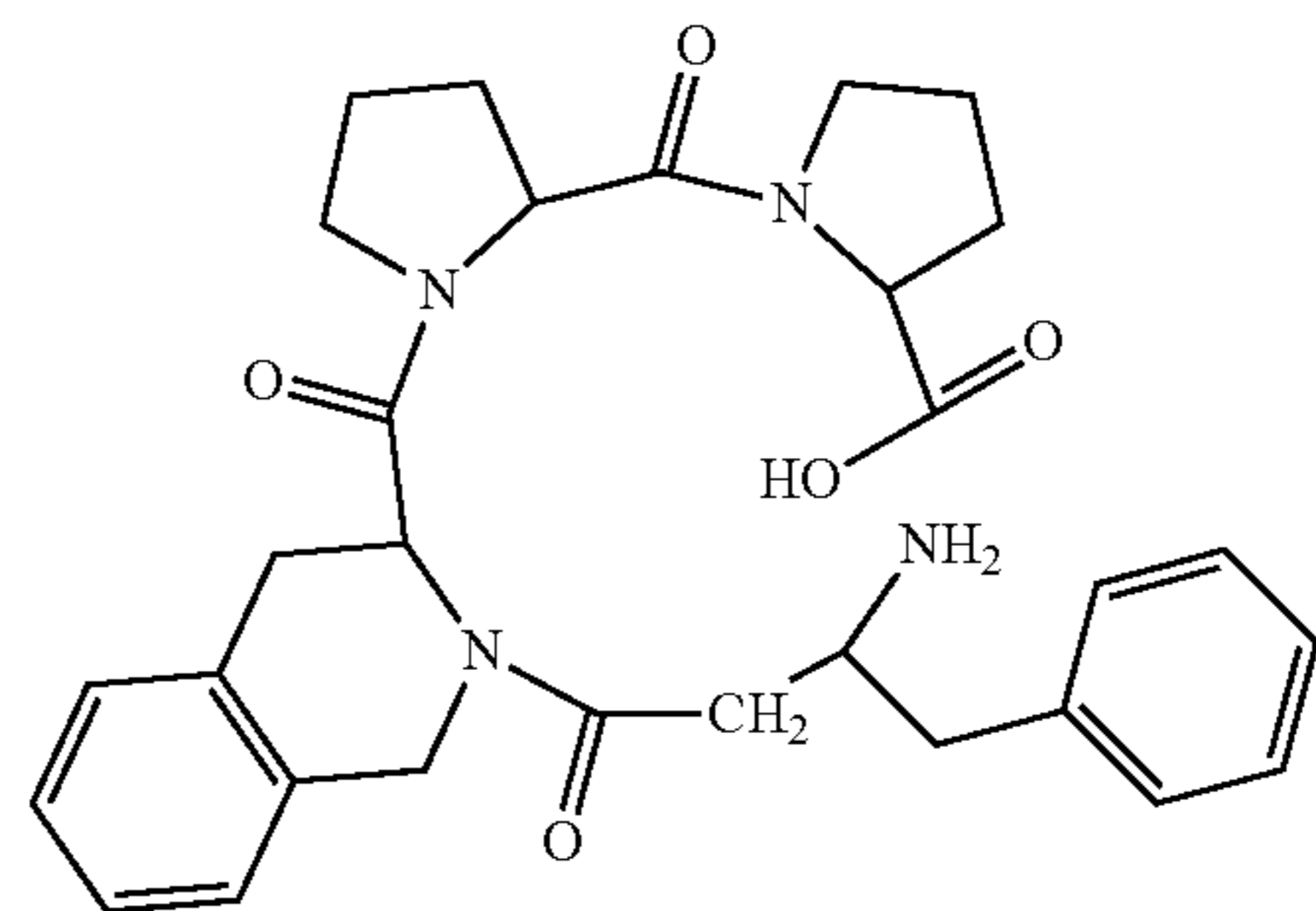
(H-β 3 hoPhe-Tic-Pro-Pro-OH)
