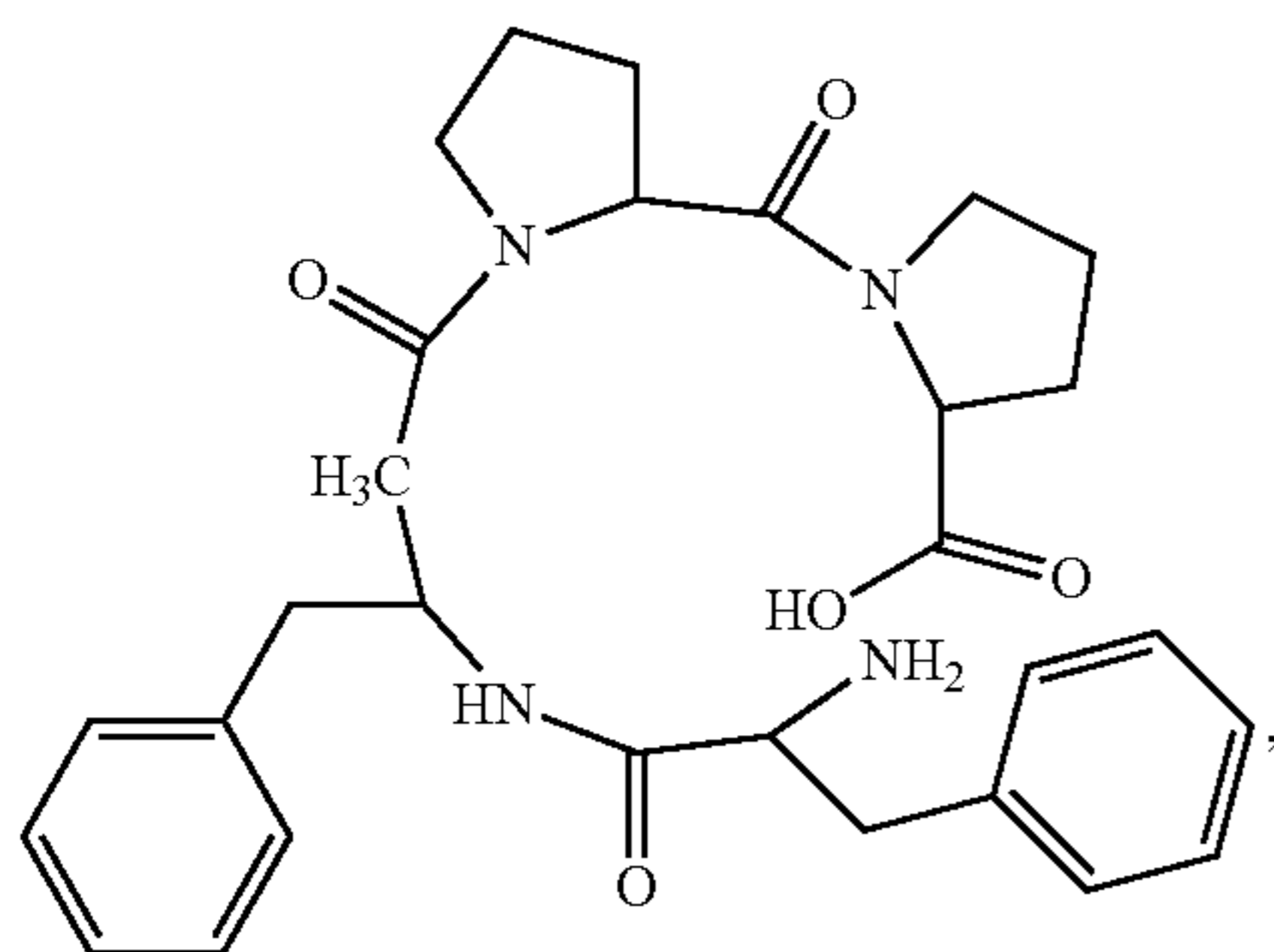
(H-Phe-β 3 hoPhe-Pro-Pro-OH)
