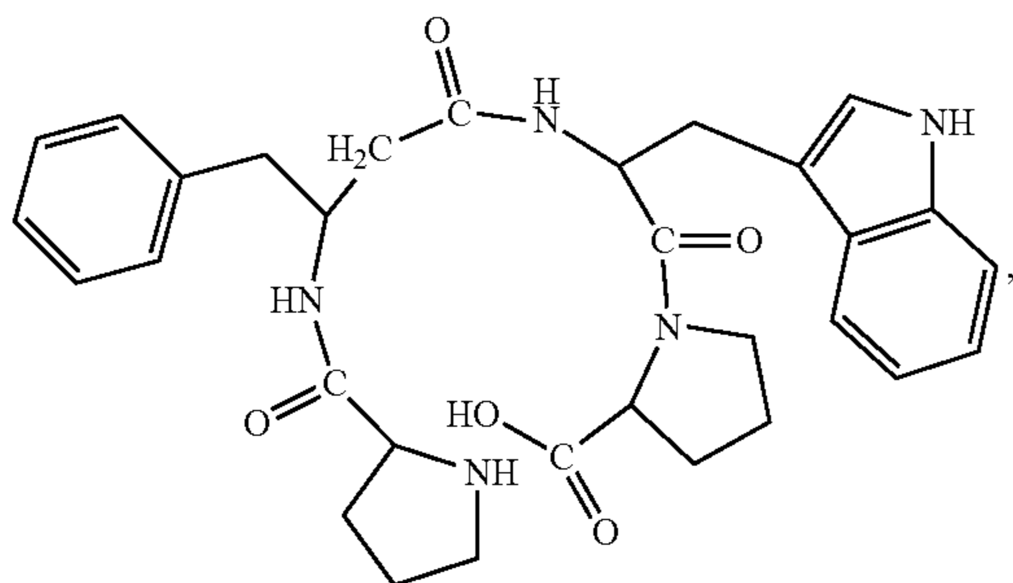
(H-Pro-Pro-β 3 hoPhe-Trp-Pro-OH)
