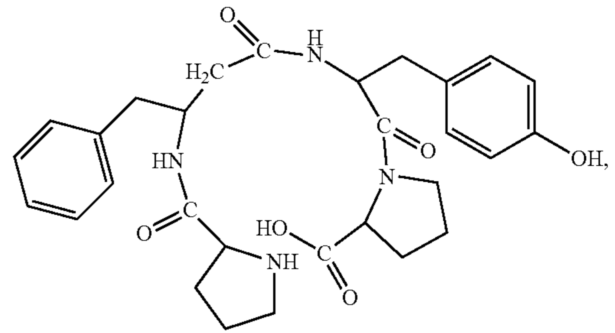
(H-Pro-β 3 hoPhe-Tyr-Pro-OH)
