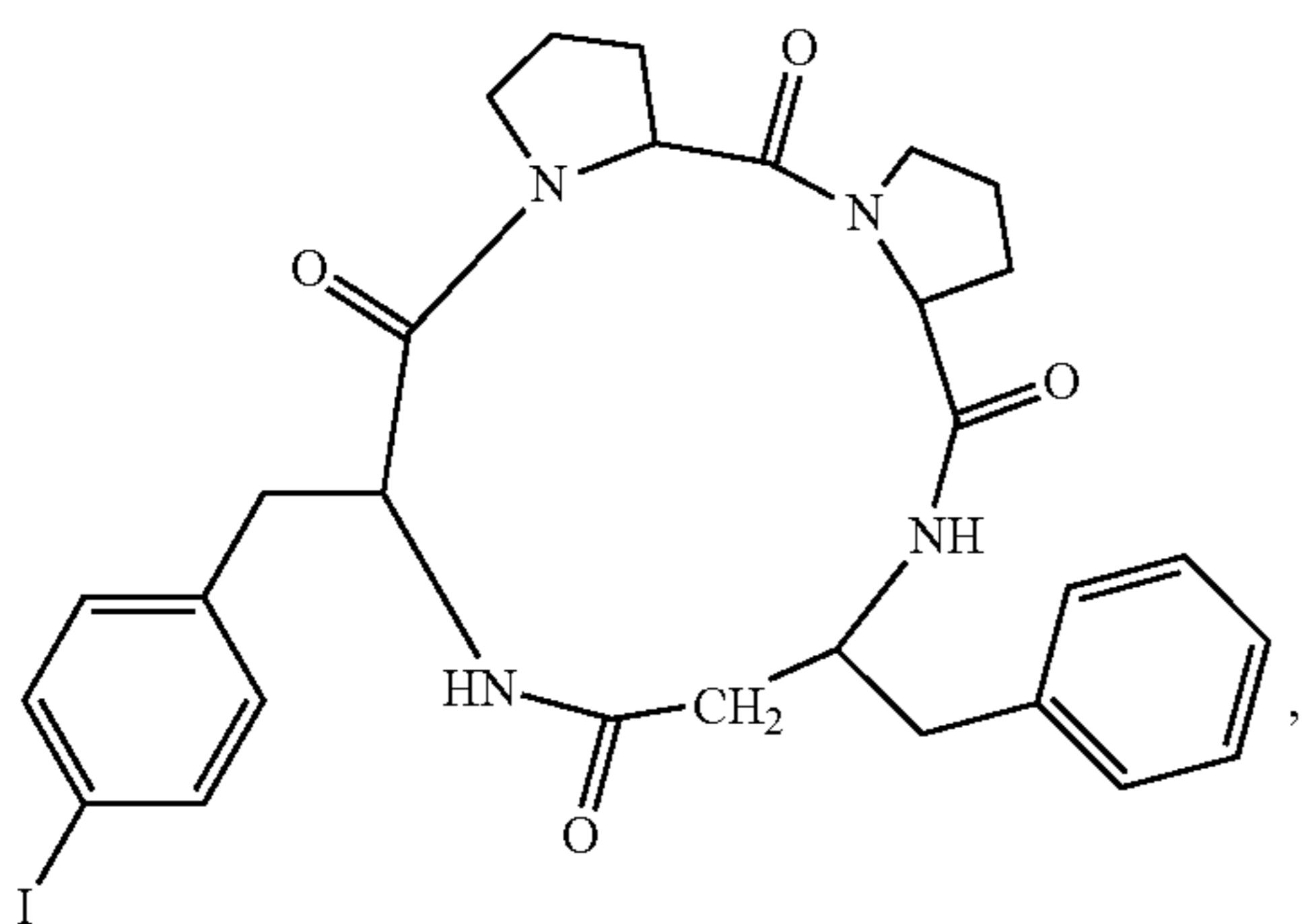
(cyclo(-Pro-Pro-β 3 hoPhe-Phe(4I)))
