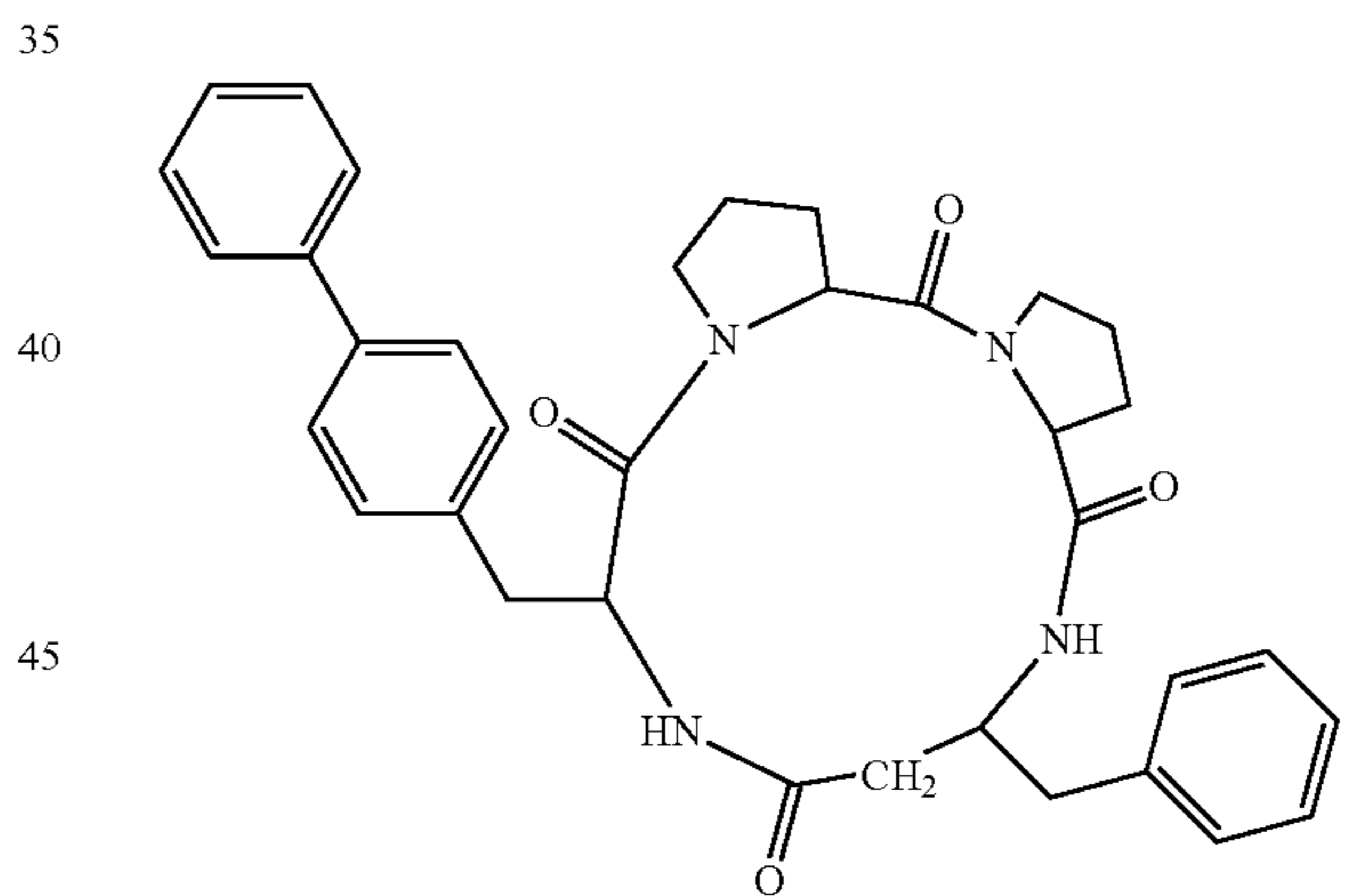
(cyclo(-Pro-Pro-β³hoPhe-Bip))
