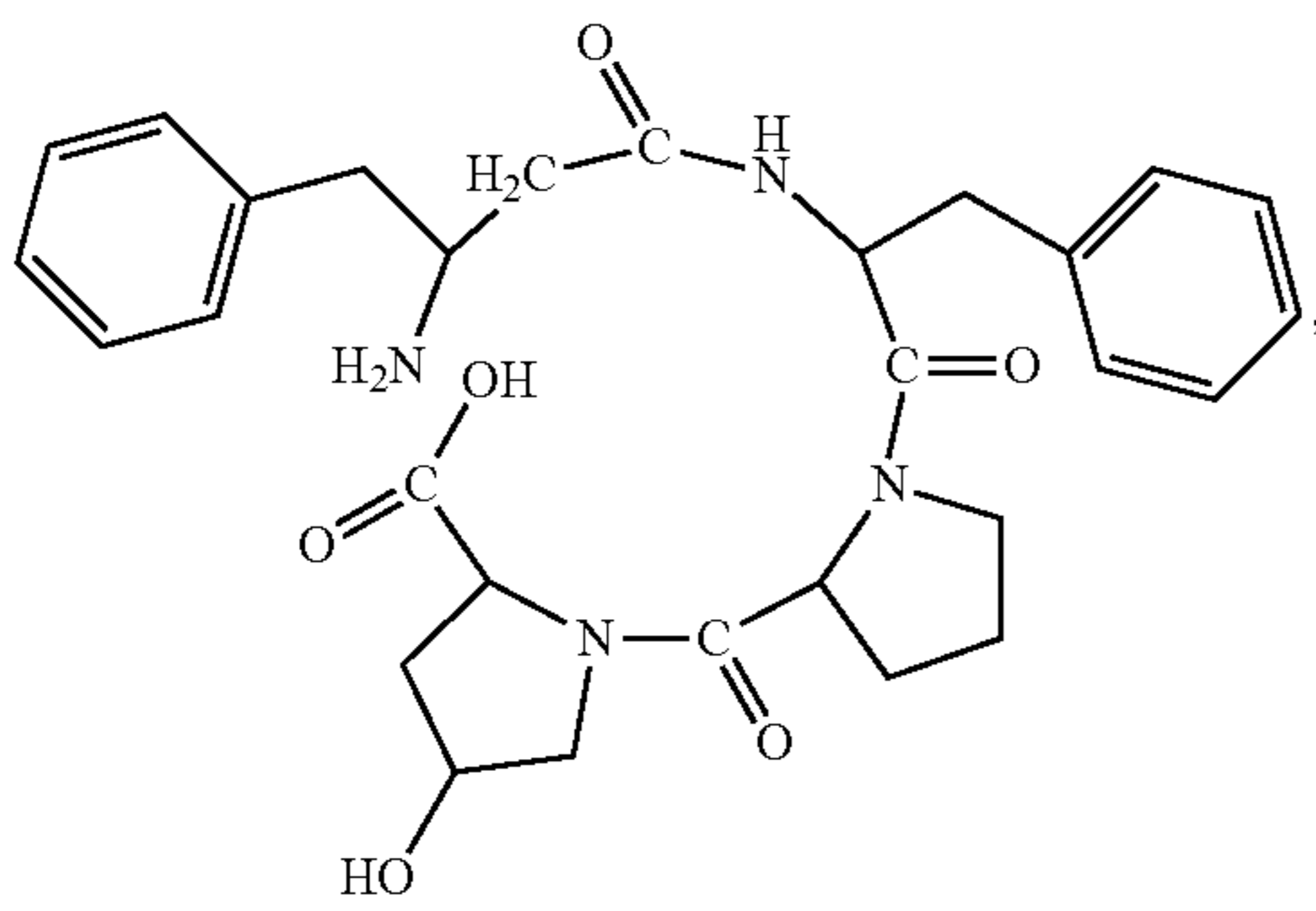
(H-β 3 hoPhe-Phe-Pro-Hyp-OH)
