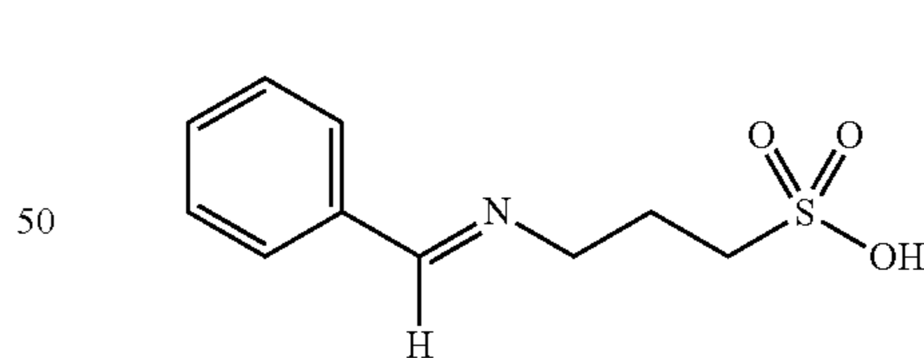
Compound D8
