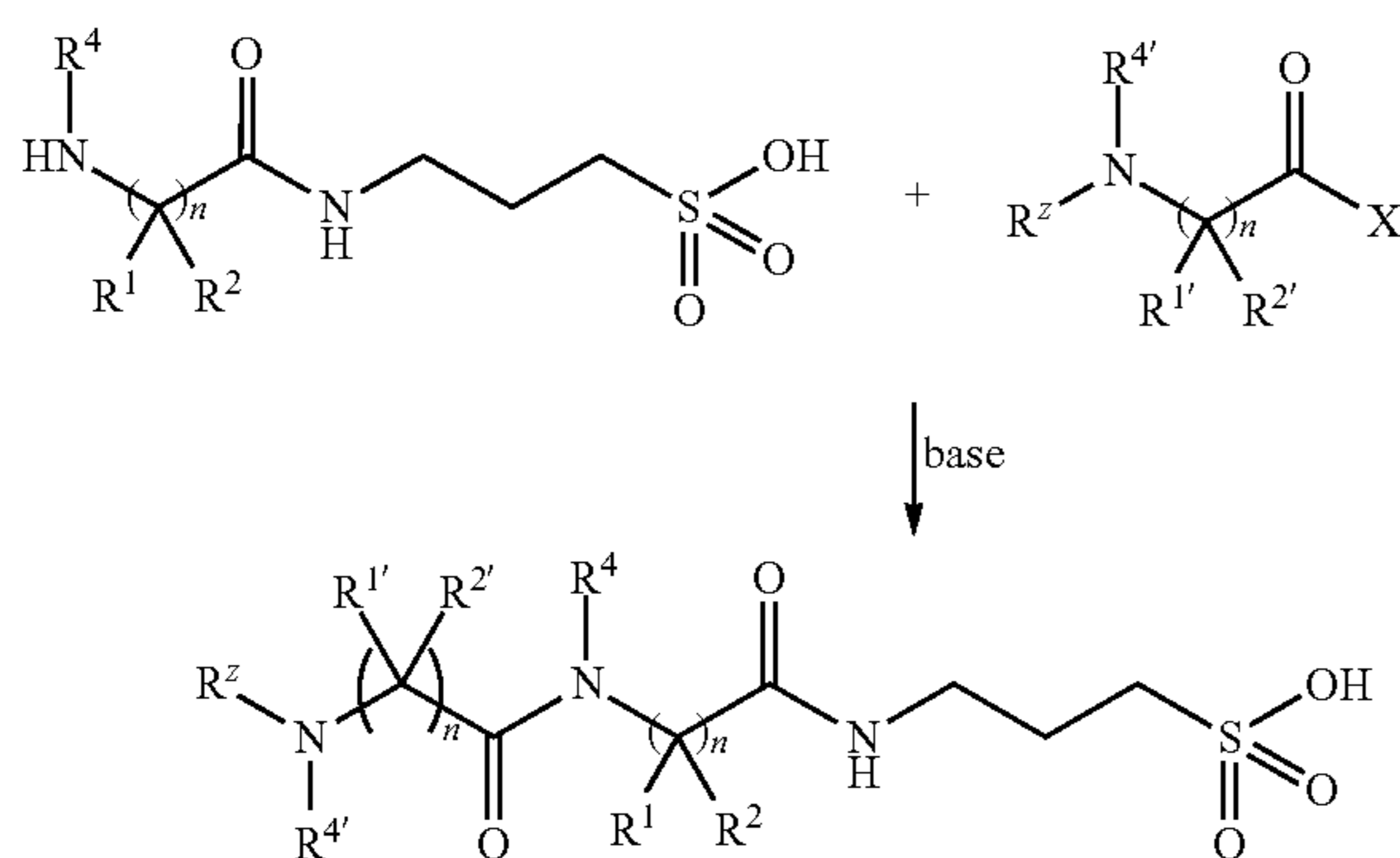
Scheme 2:
