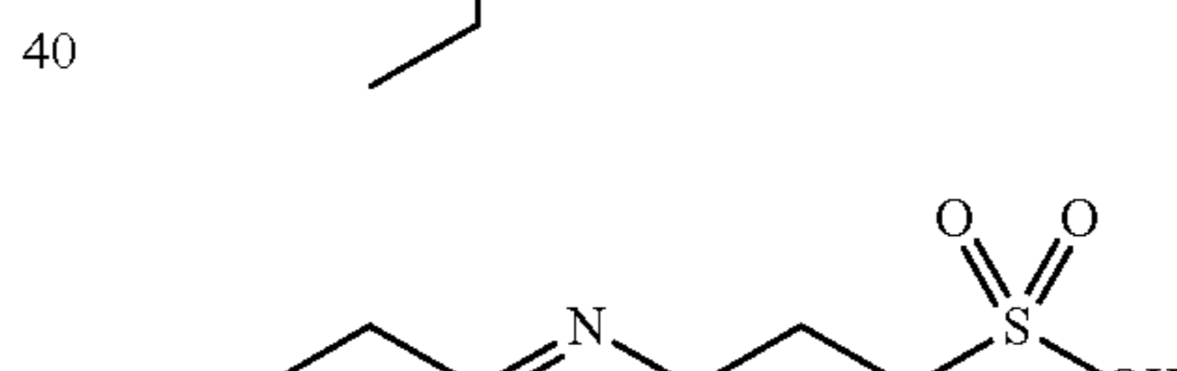
Compound D7
