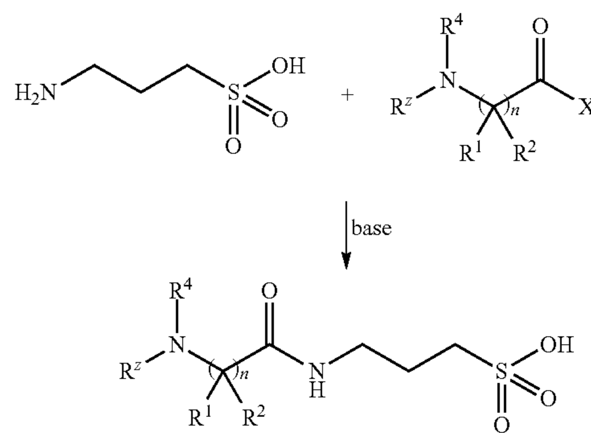
Scheme 1:
