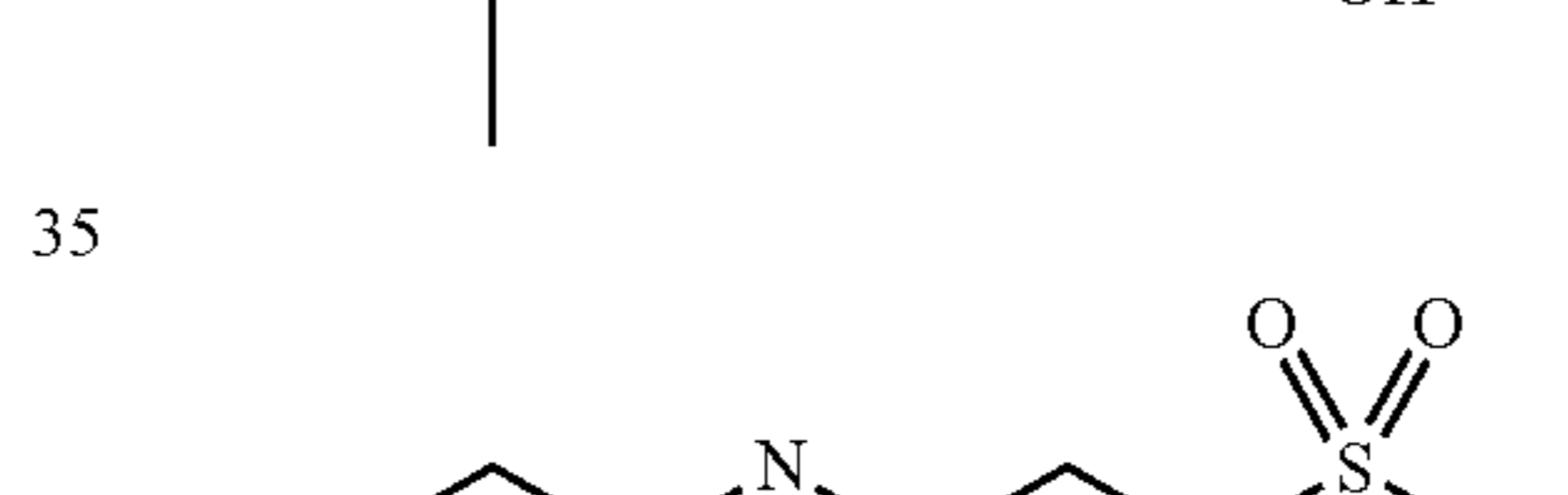
Compound D6
