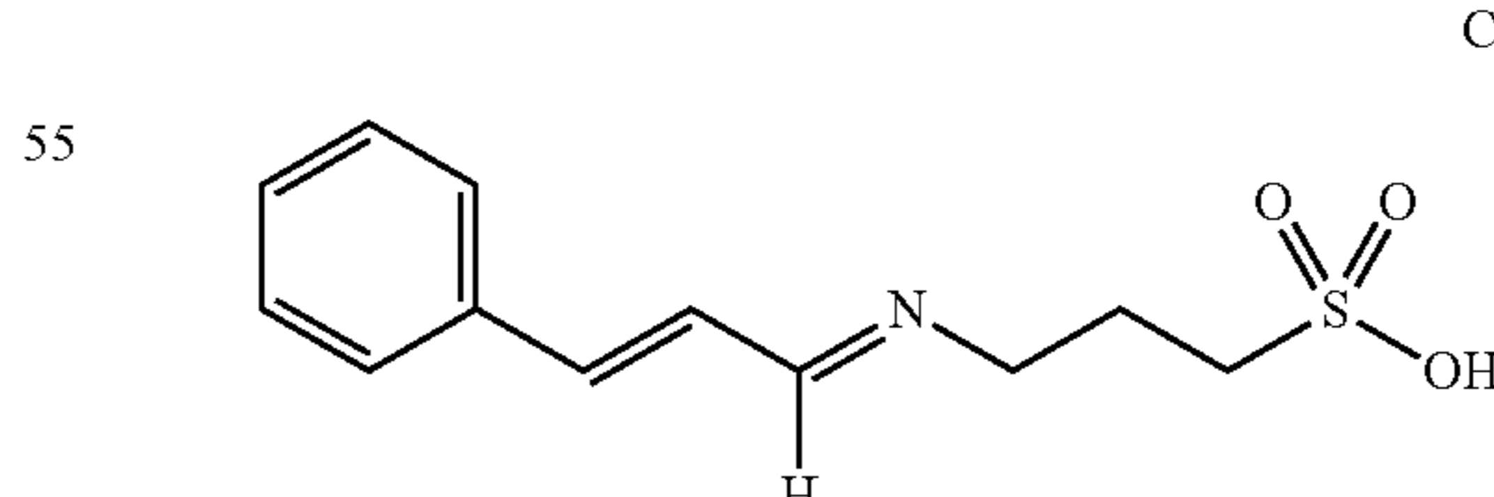
Compound D9
