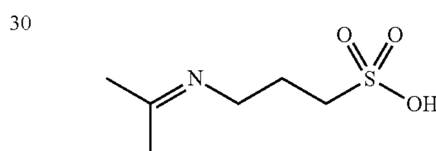
Compound D5
