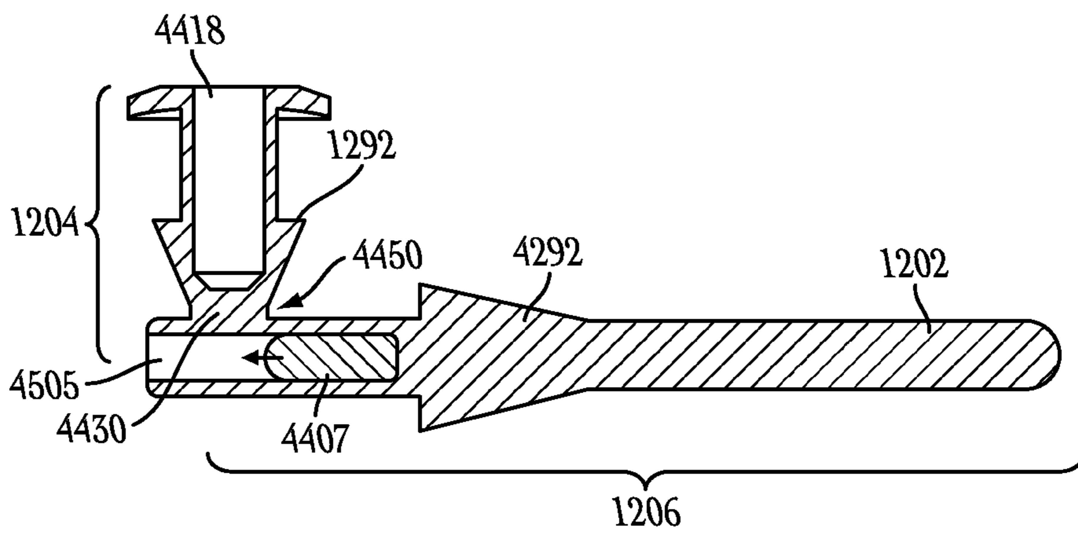
SECTION 45B-45B
