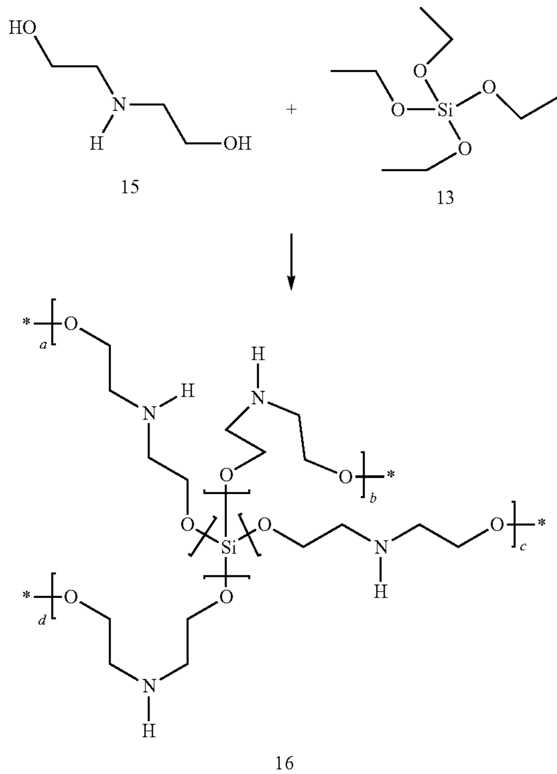
REACTION SCHEME 6
