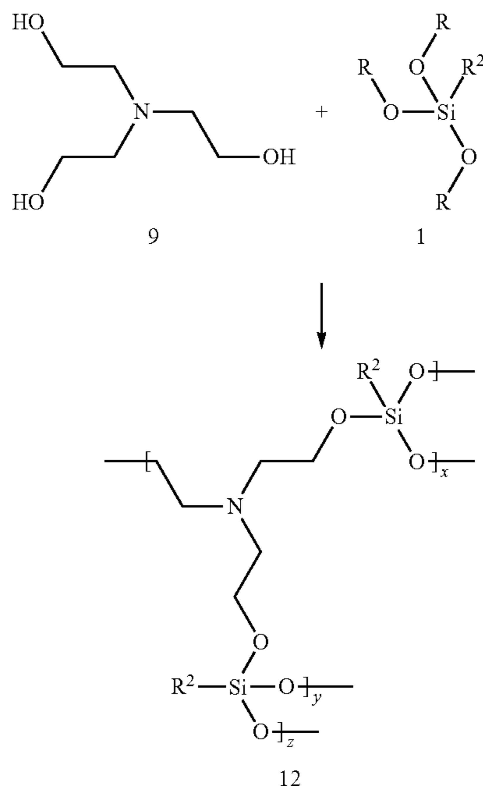
REACTION SCHEME 4
