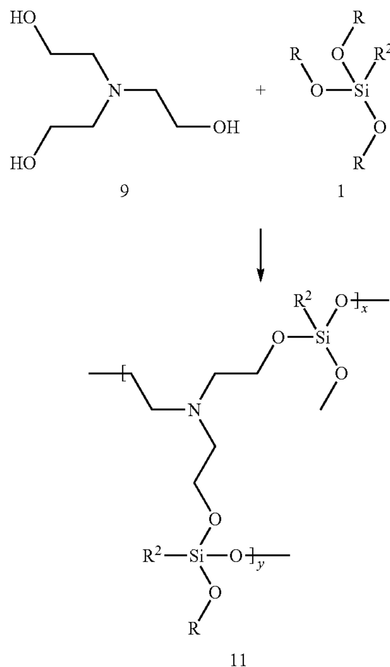
REACTION SCHEME 3
