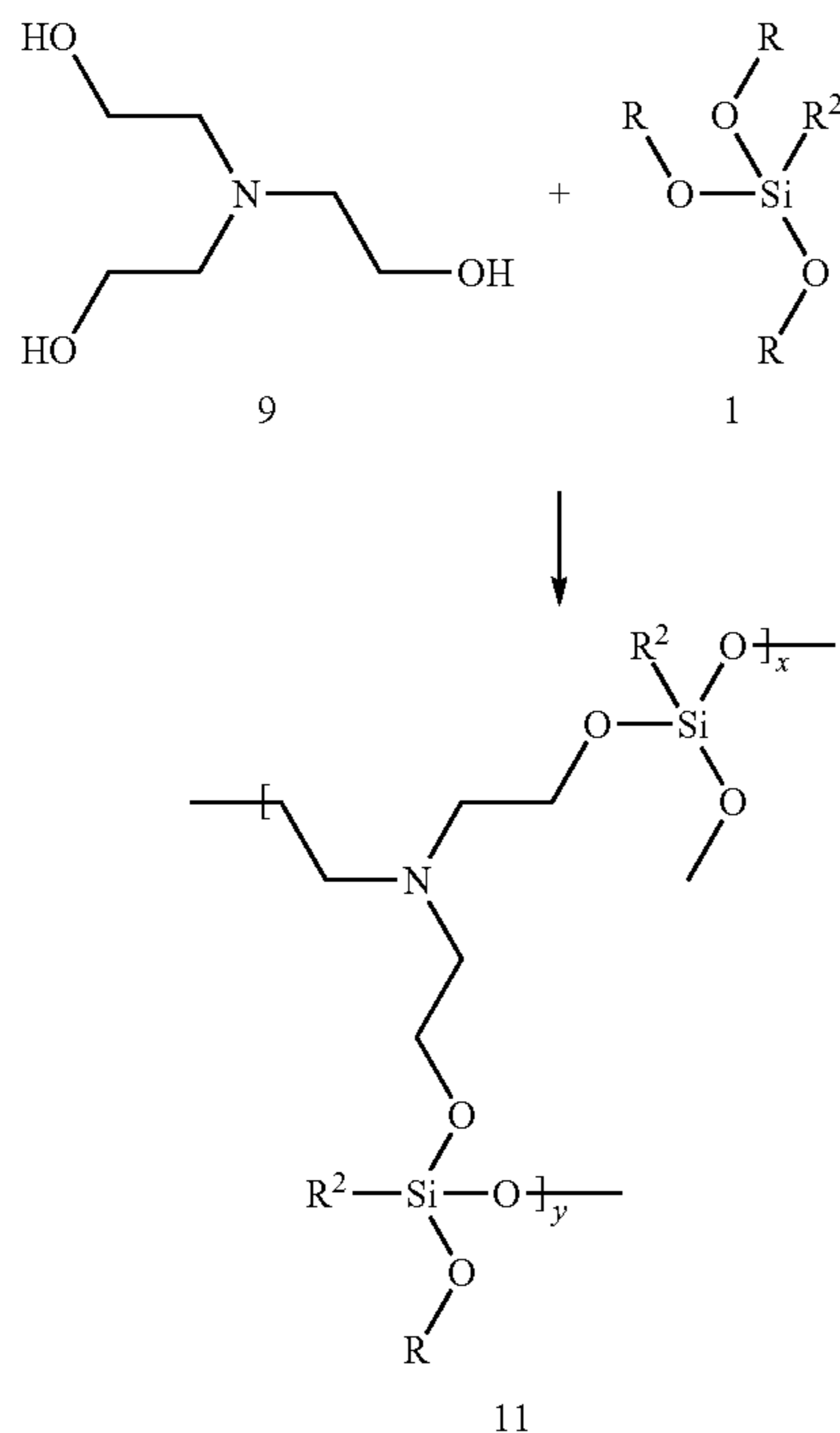
REACTION SCHEME 3
