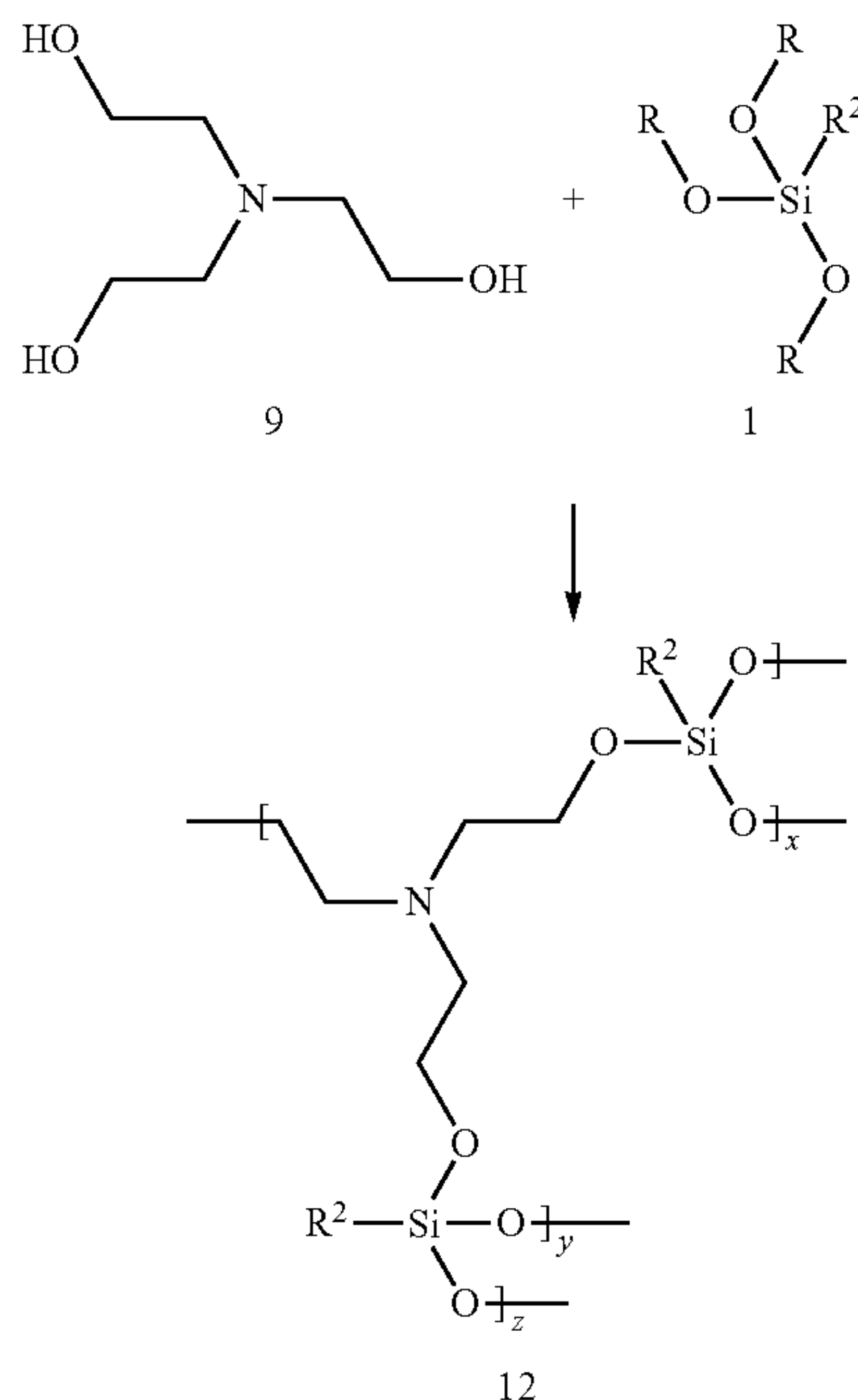
REACTION SCHEME 4
