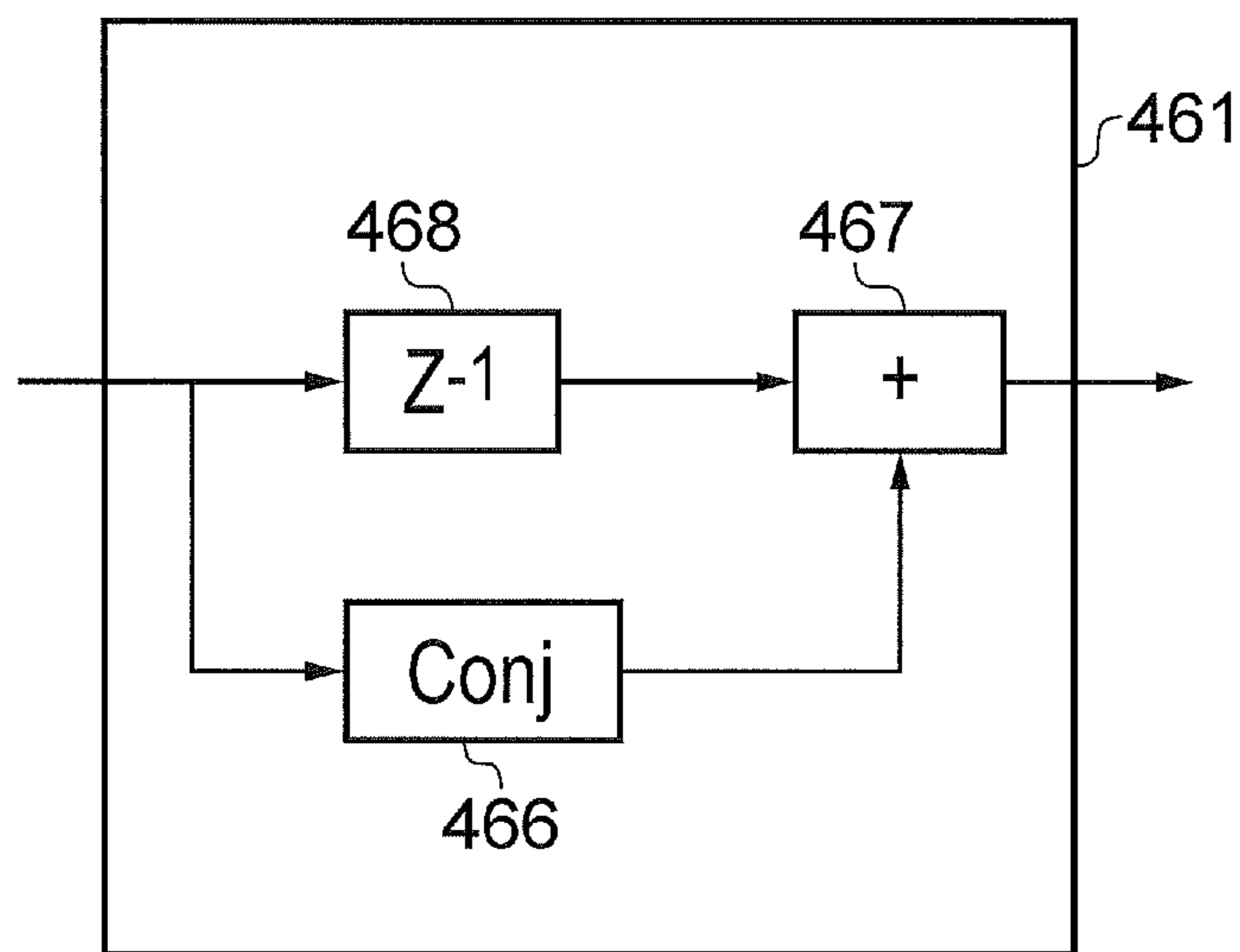
Differential Encoder
