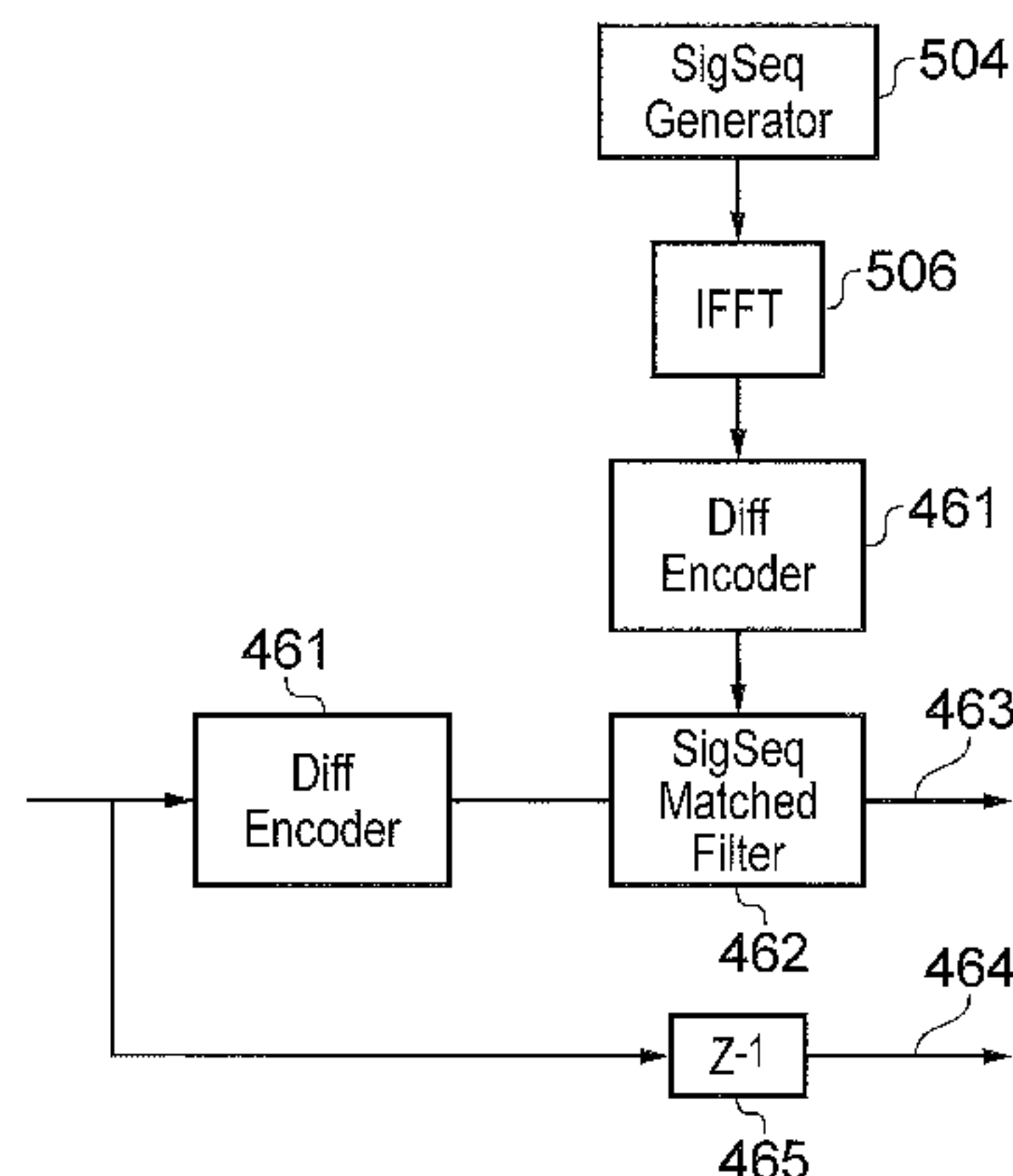
Alternative coarse frequency offset synchroniser
